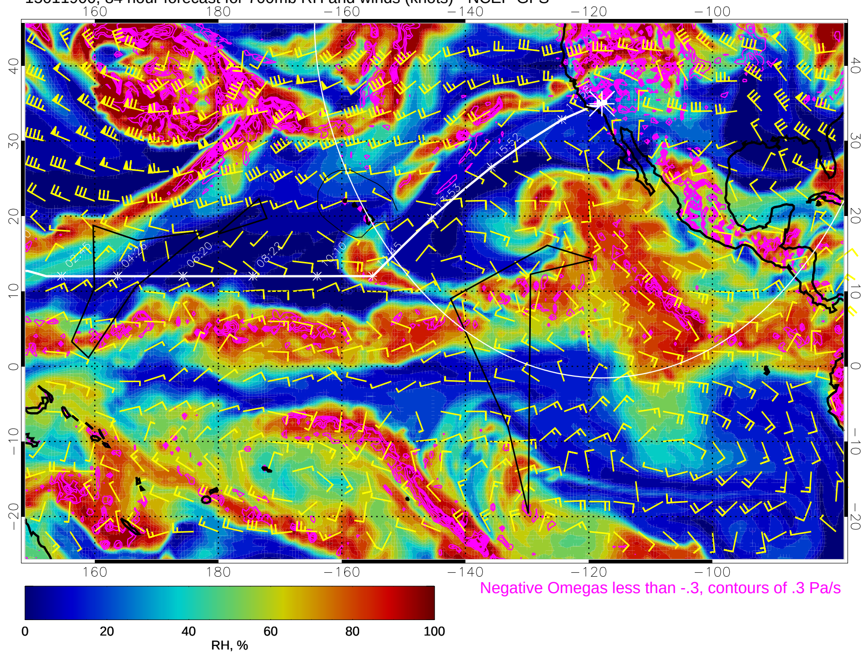
15011900, 84 hour forecast for 700mb RH and winds (knots) - NCEP GFS
