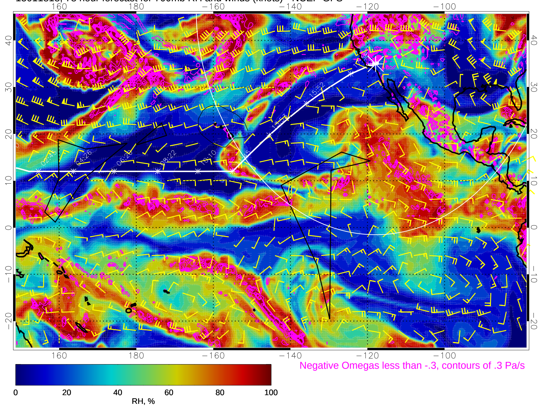
15011818, 78 hour forecast for 700mb RH and winds (knots) - NCEP GFS
