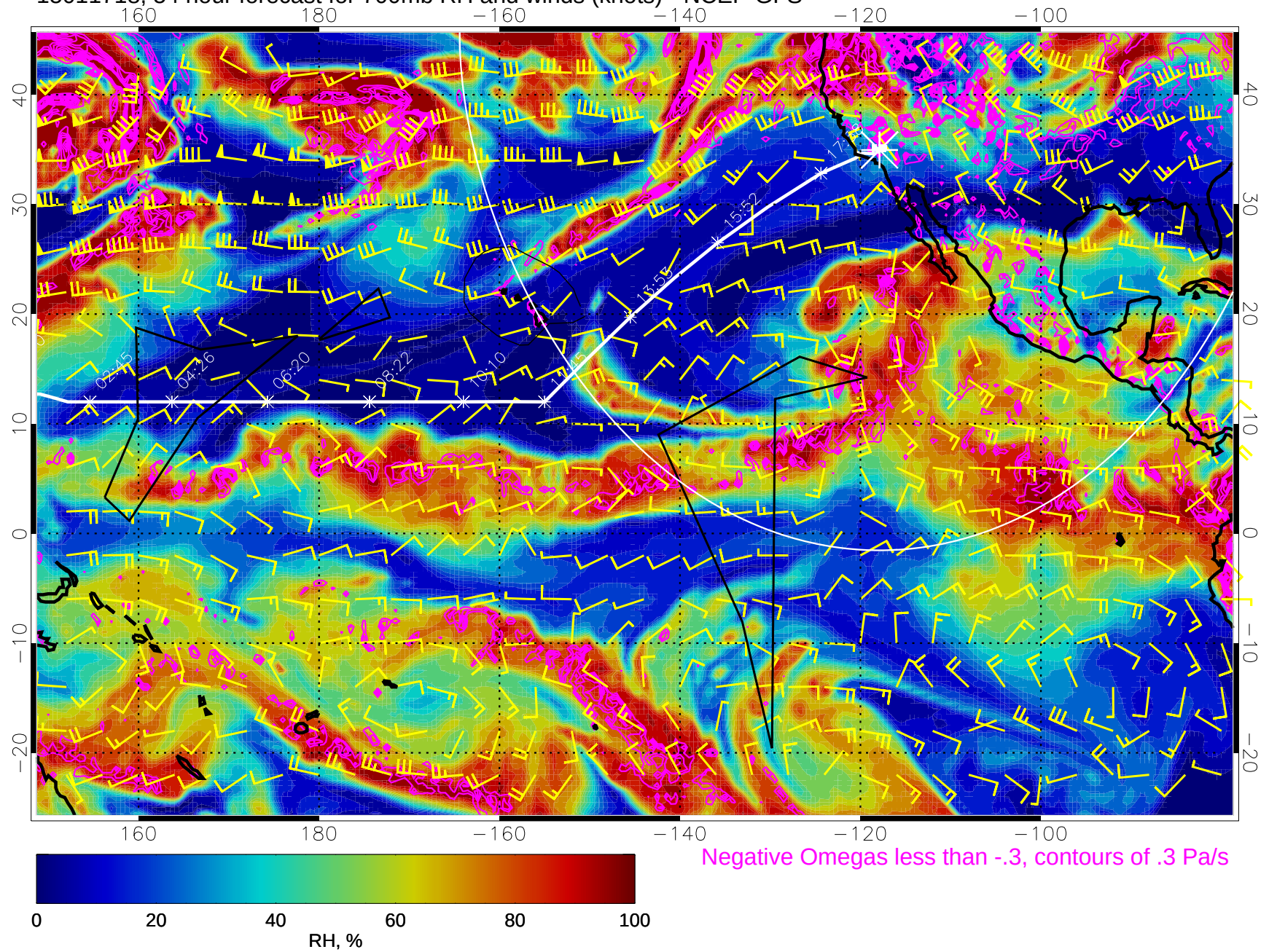
15011718, 54 hour forecast for 700mb RH and winds (knots) - NCEP GFS
