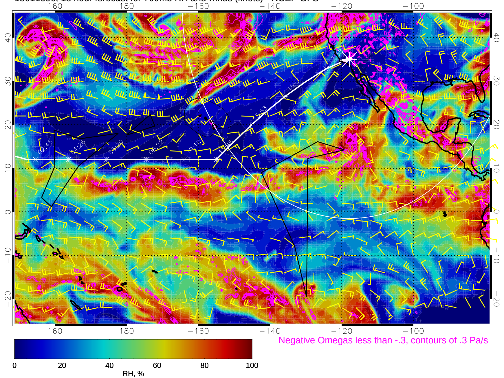
15011606, 18 hour forecast for 700mb RH and winds (knots) - NCEP GFS
