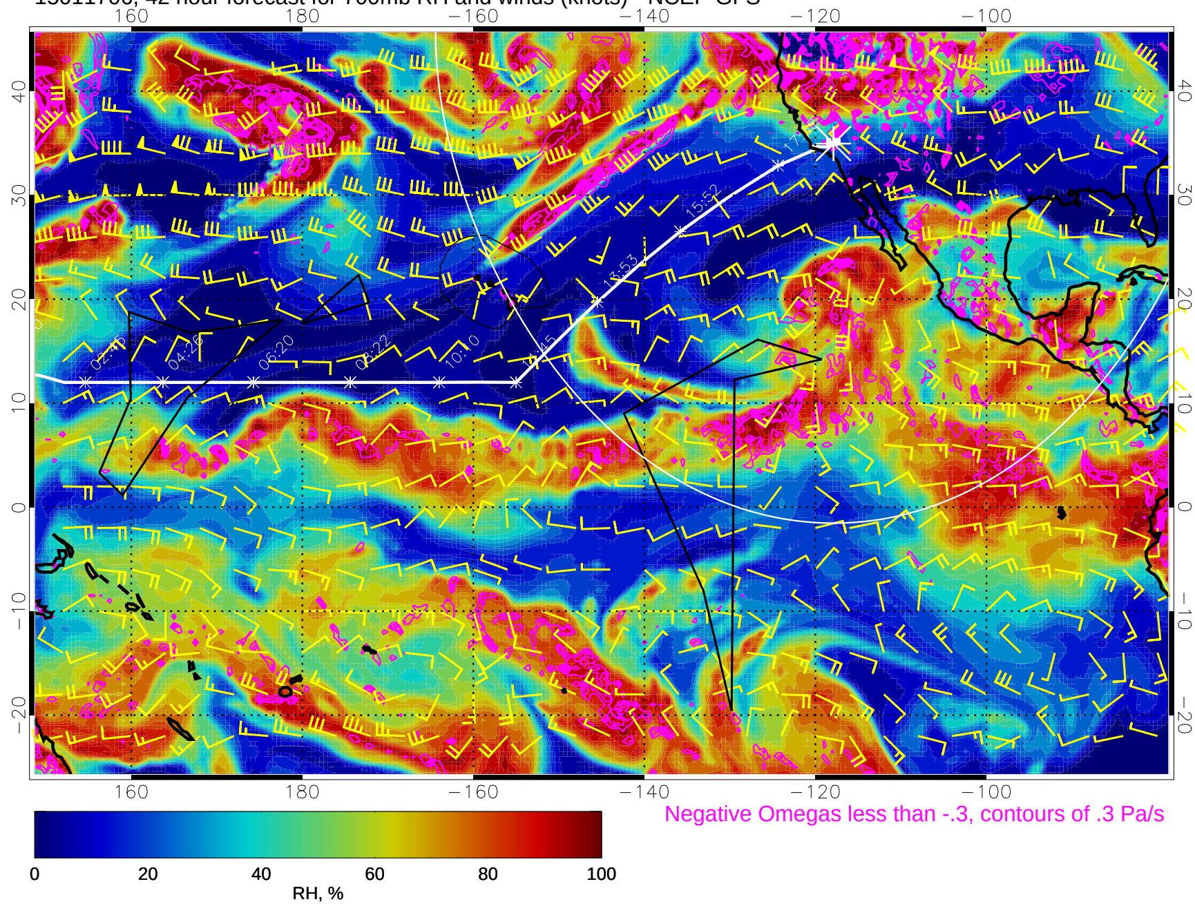
15011706, 42 hour forecast for 700mb RH and winds (knots) - NCEP GFS
