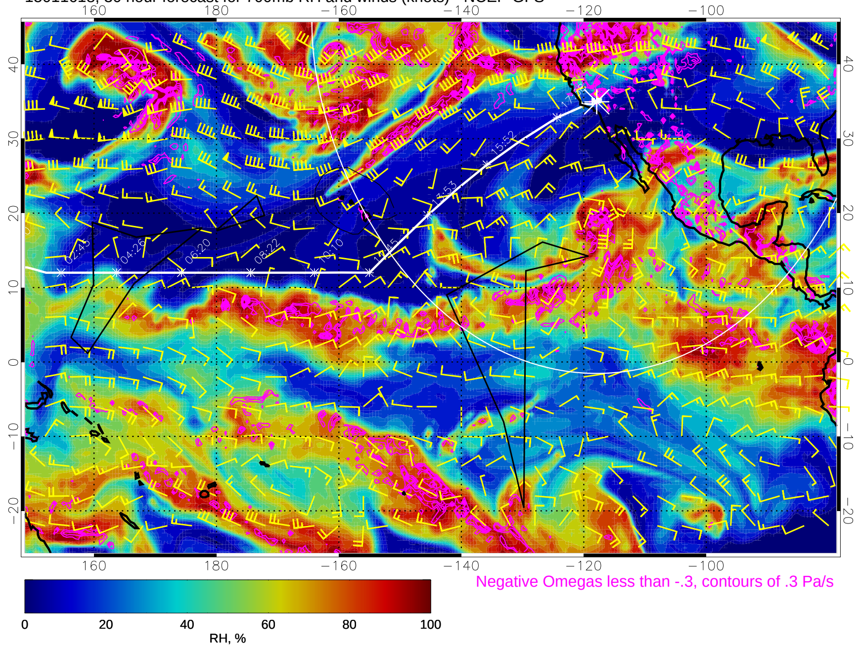
15011618, 30 hour forecast for 700mb RH and winds (knots) - NCEP GFS
