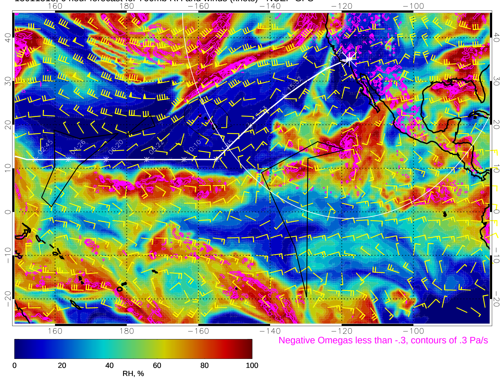
15011518, 6 hour forecast for 700mb RH and winds (knots) - NCEP GFS
