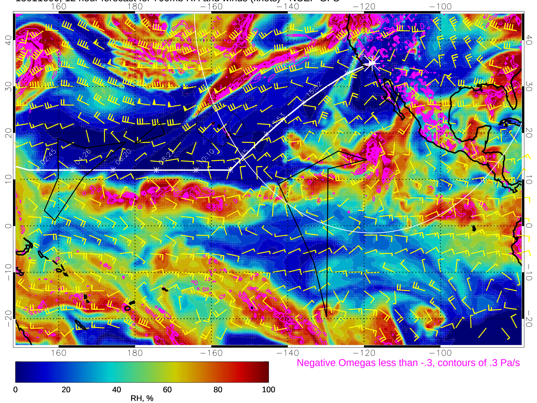
15011600, 12 hour forecast for 700mb RH and winds (knots) - NCEP GFS
