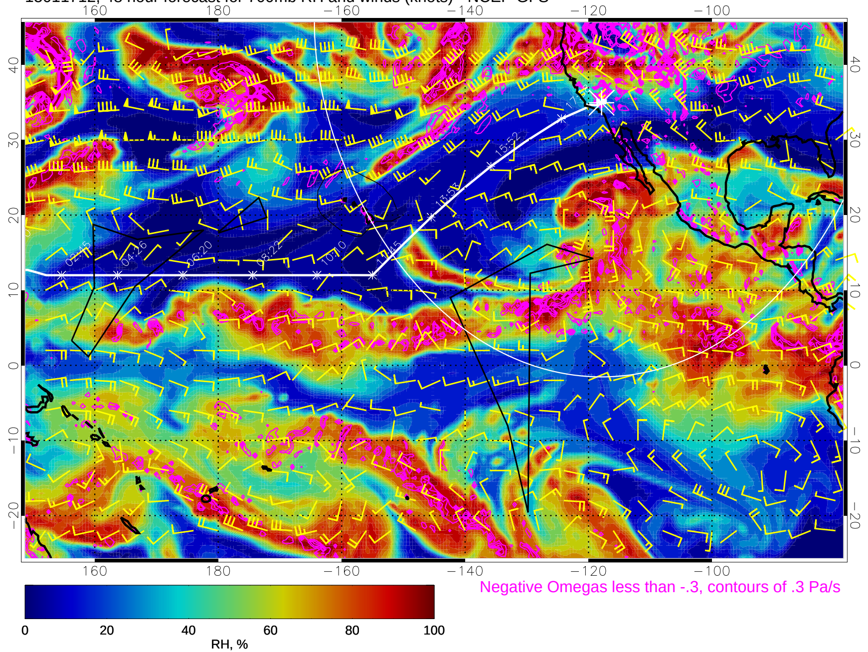
15011712, 48 hour forecast for 700mb RH and winds (knots) - NCEP GFS
