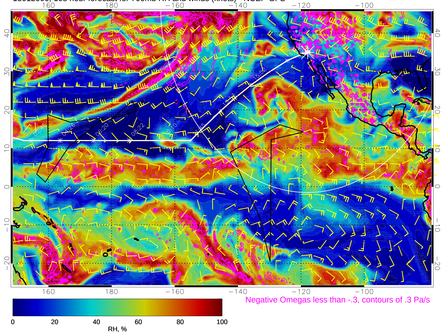
15012000, 108 hour forecast for 700mb RH and winds (knots) - NCEP GFS
