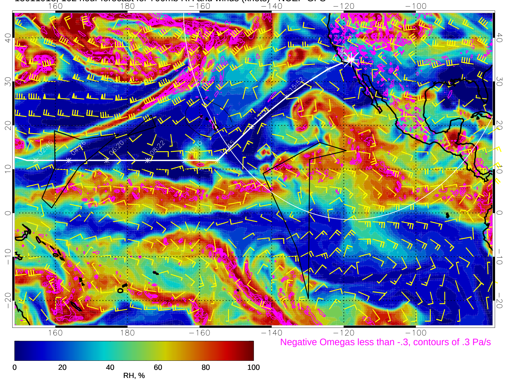
15011918, 102 hour forecast for 700mb RH and winds (knots) - NCEP GFS
