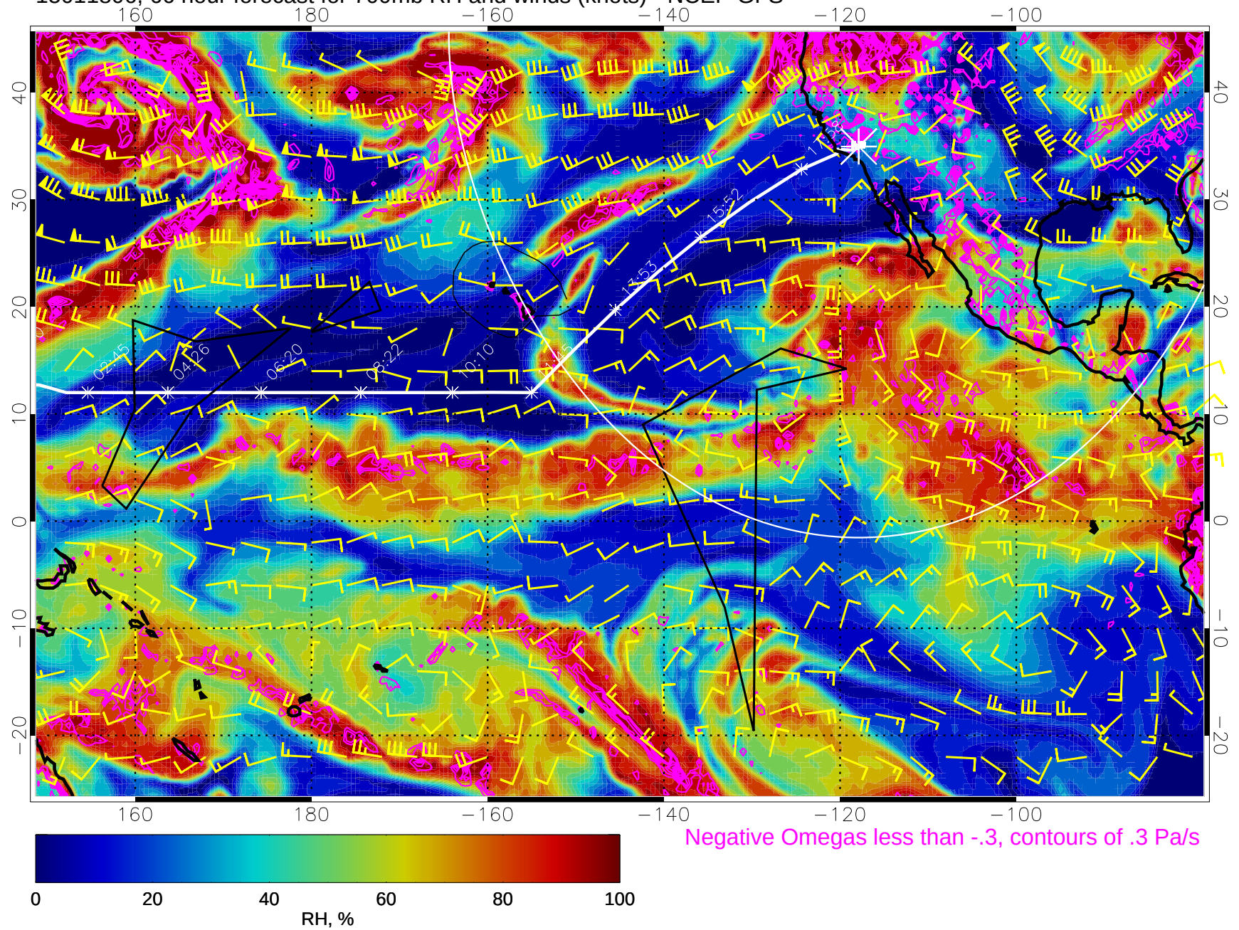
15011806, 66 hour forecast for 700mb RH and winds (knots) - NCEP GFS
