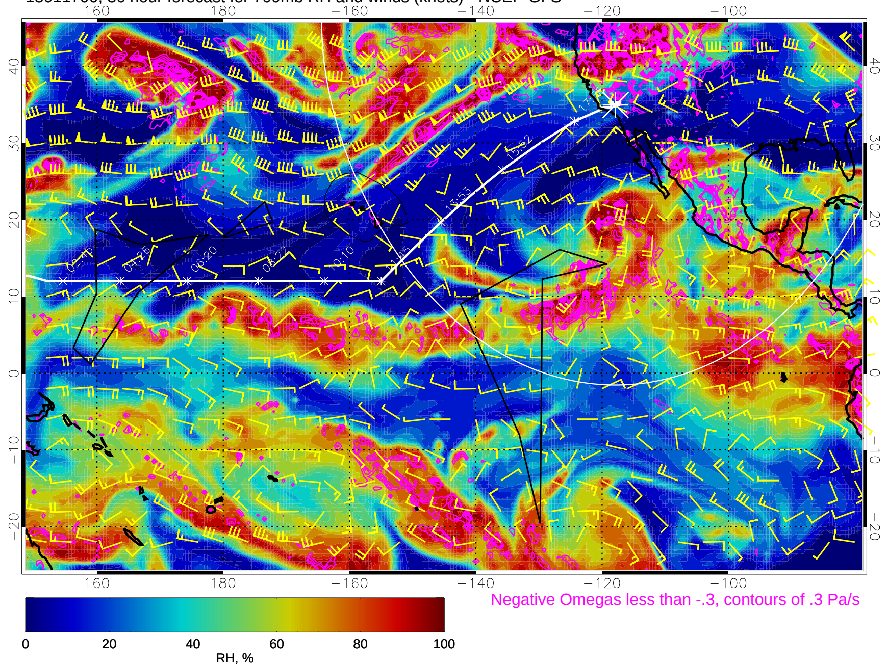
15011700, 36 hour forecast for 700mb RH and winds (knots) - NCEP GFS
