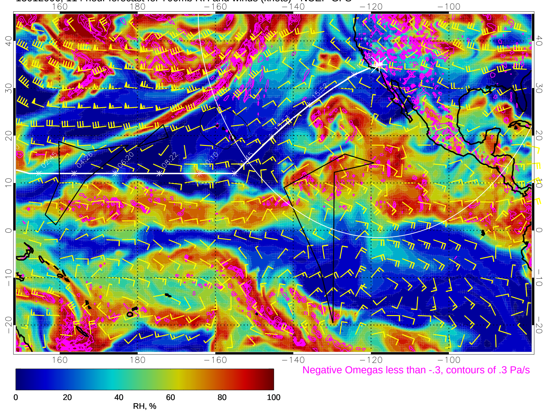
15012006, 114 hour forecast for 700mb RH and winds (knots) - NCEP GFS
