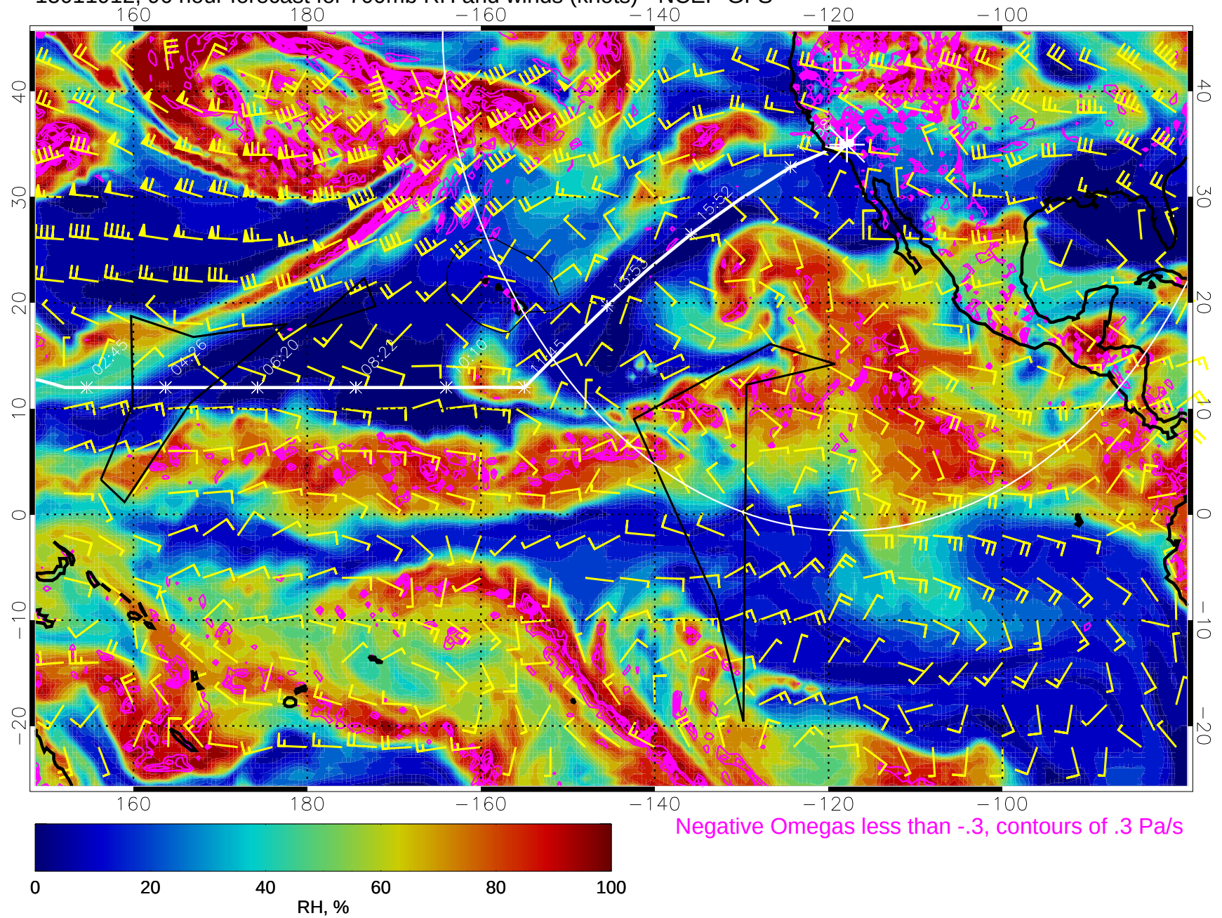
15011912, 96 hour forecast for 700mb RH and winds (knots) - NCEP GFS
