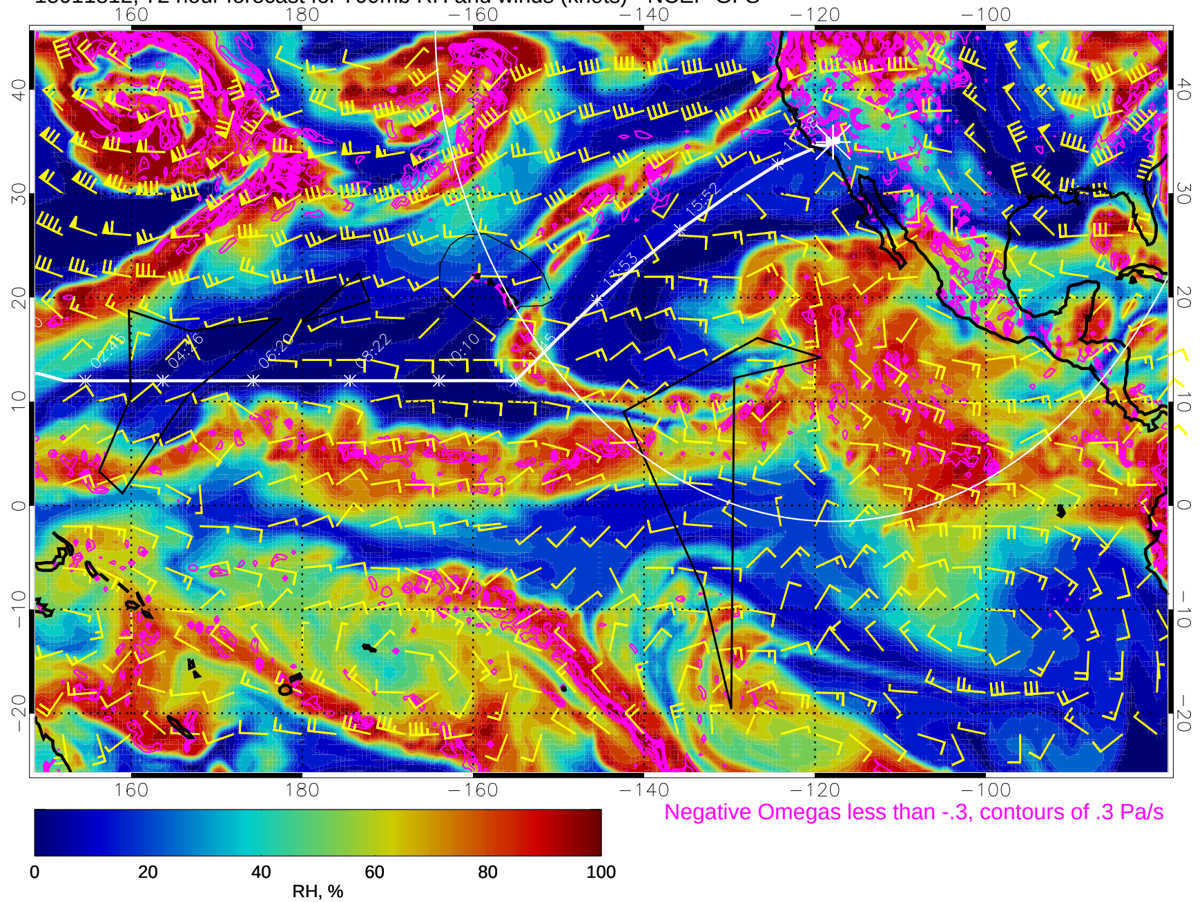
15011812, 72 hour forecast for 700mb RH and winds (knots) - NCEP GFS
