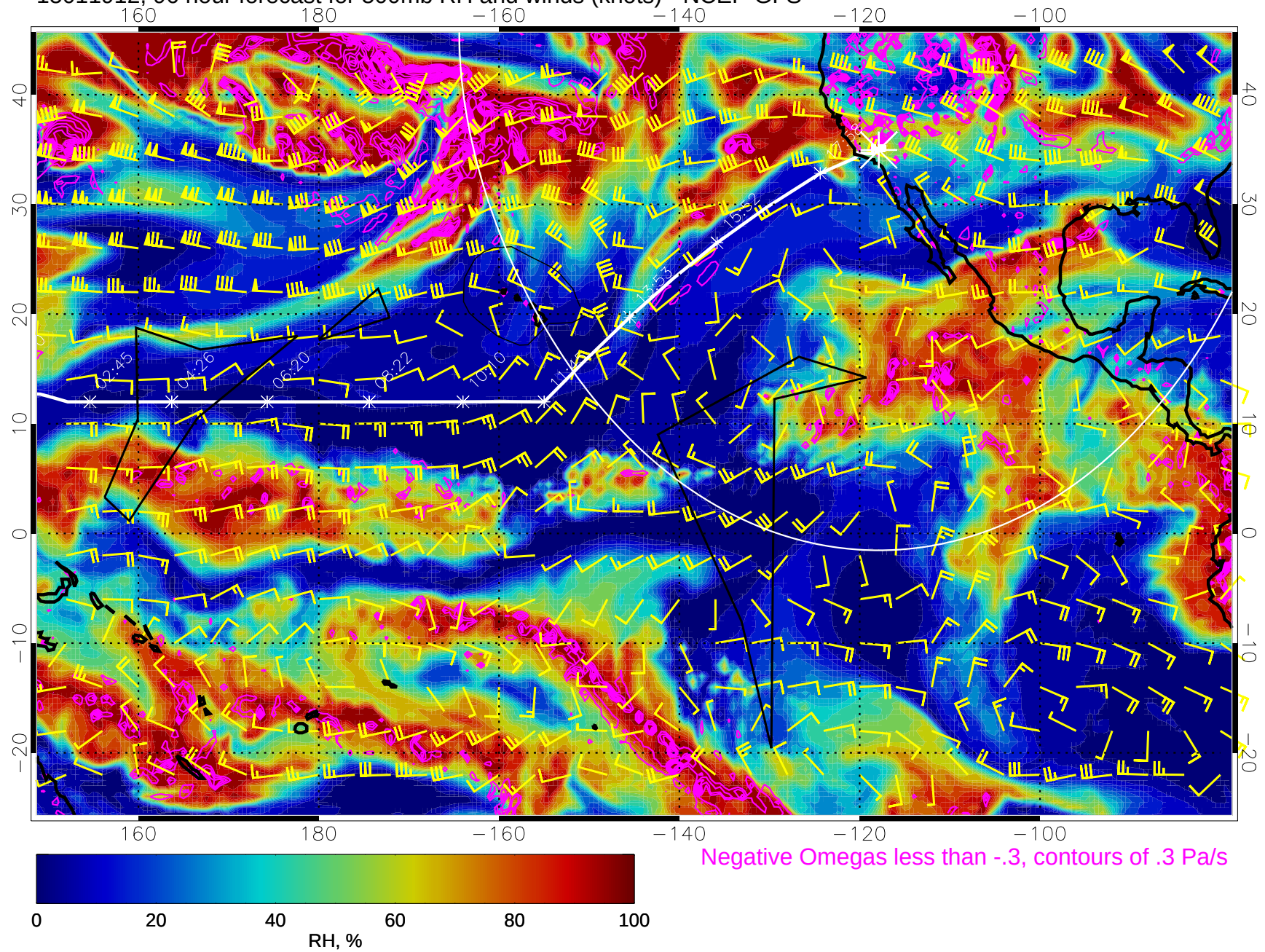
15011912, 96 hour forecast for 500mb RH and winds (knots) - NCEP GFS
