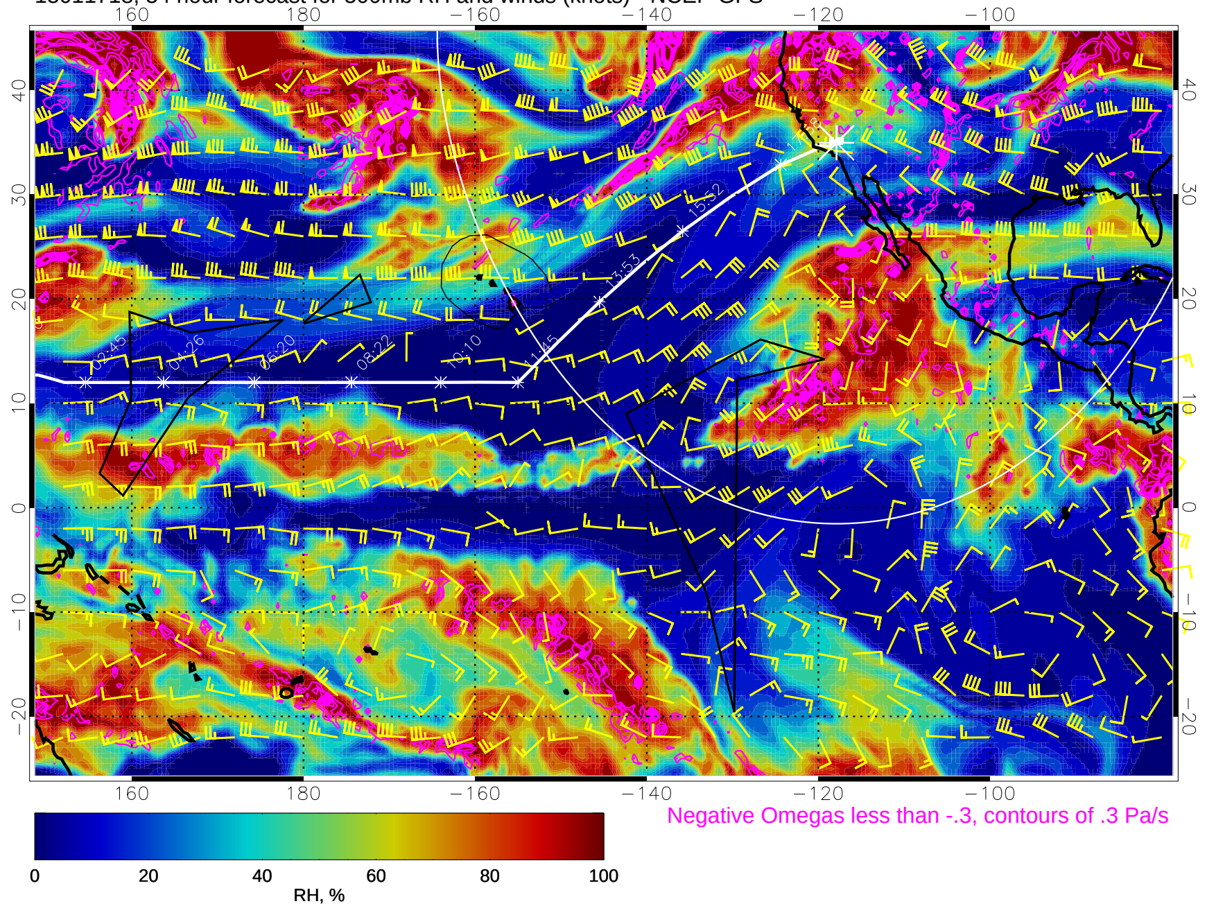
15011718, 54 hour forecast for 500mb RH and winds (knots) - NCEP GFS
