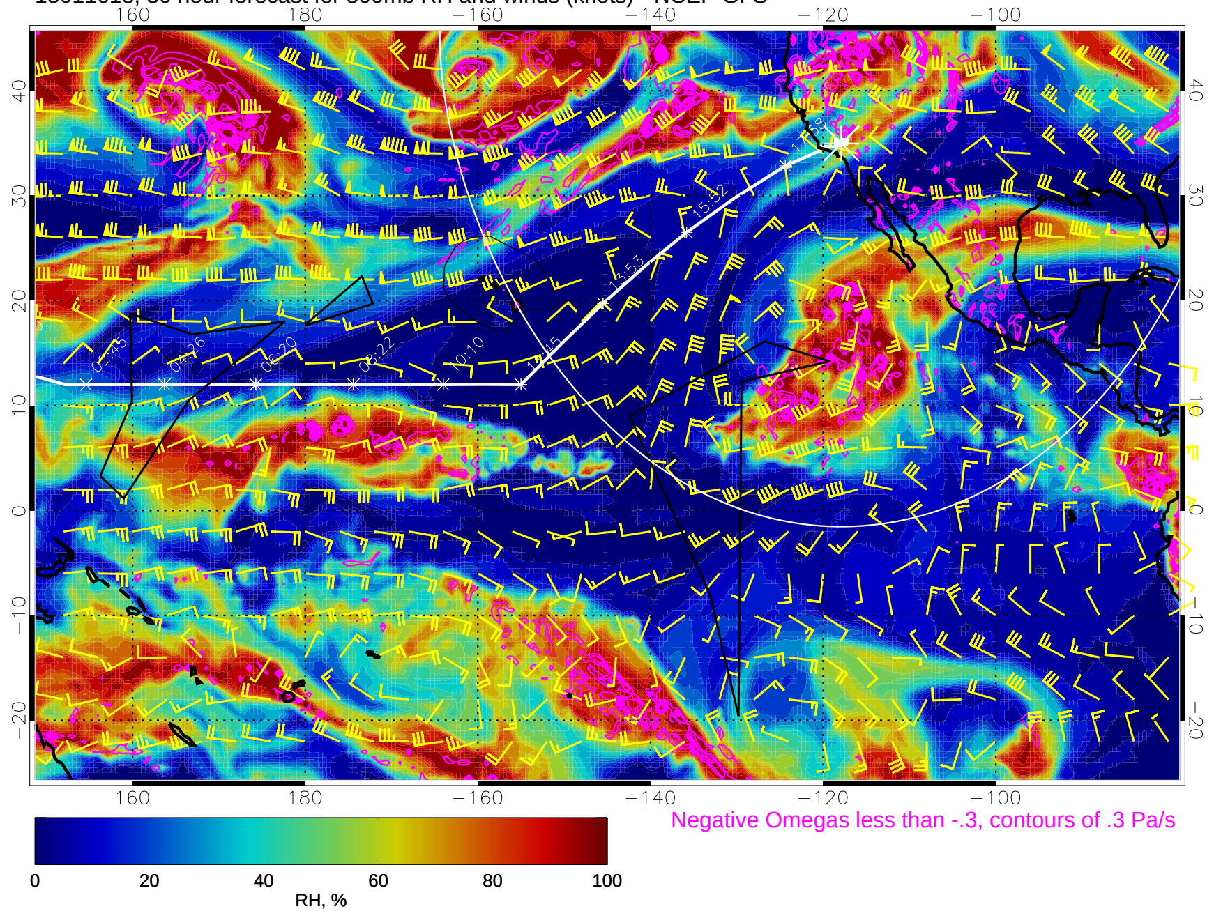
15011618, 30 hour forecast for 500mb RH and winds (knots) - NCEP GFS
