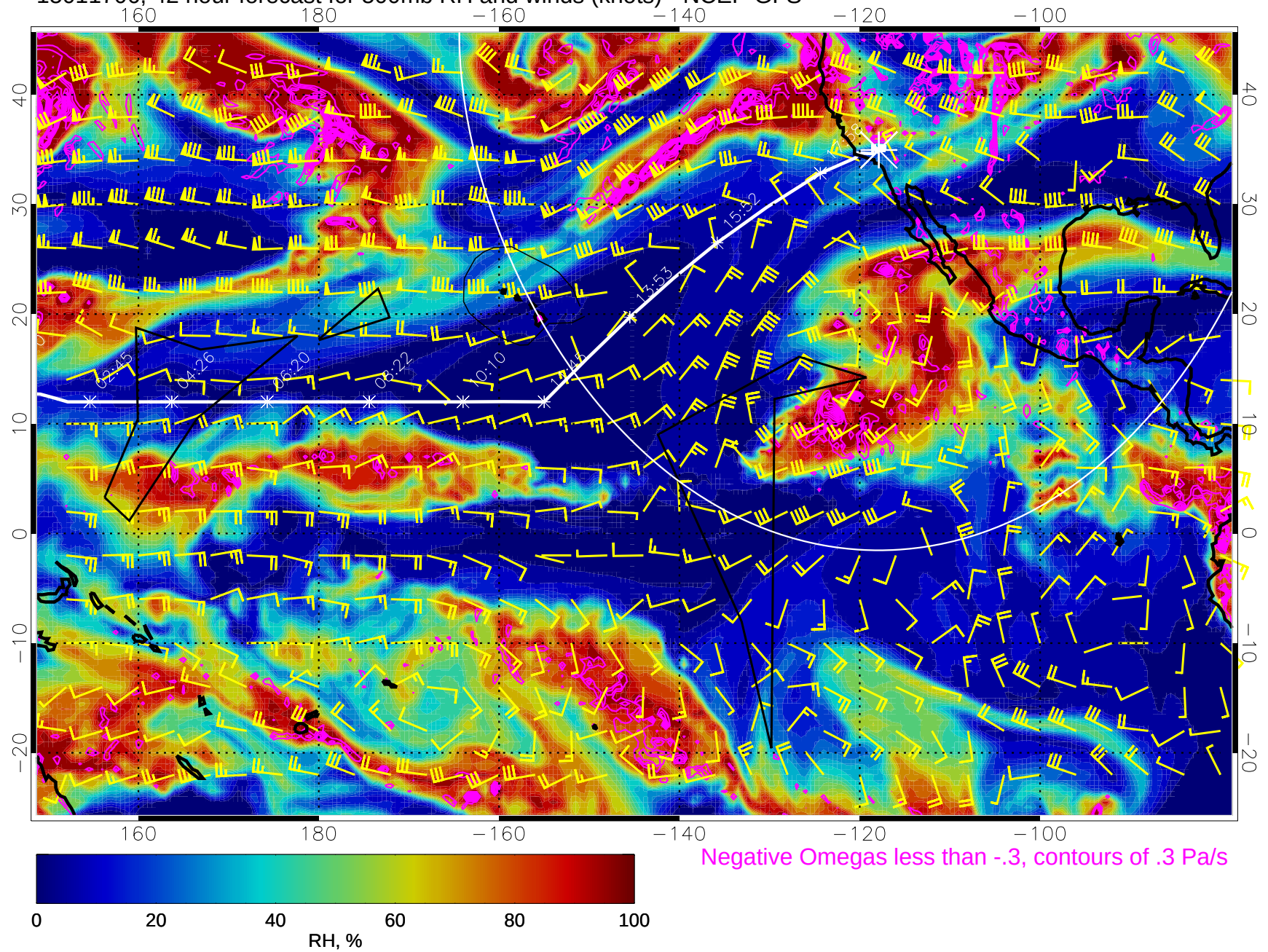
15011706, 42 hour forecast for 500mb RH and winds (knots) - NCEP GFS
