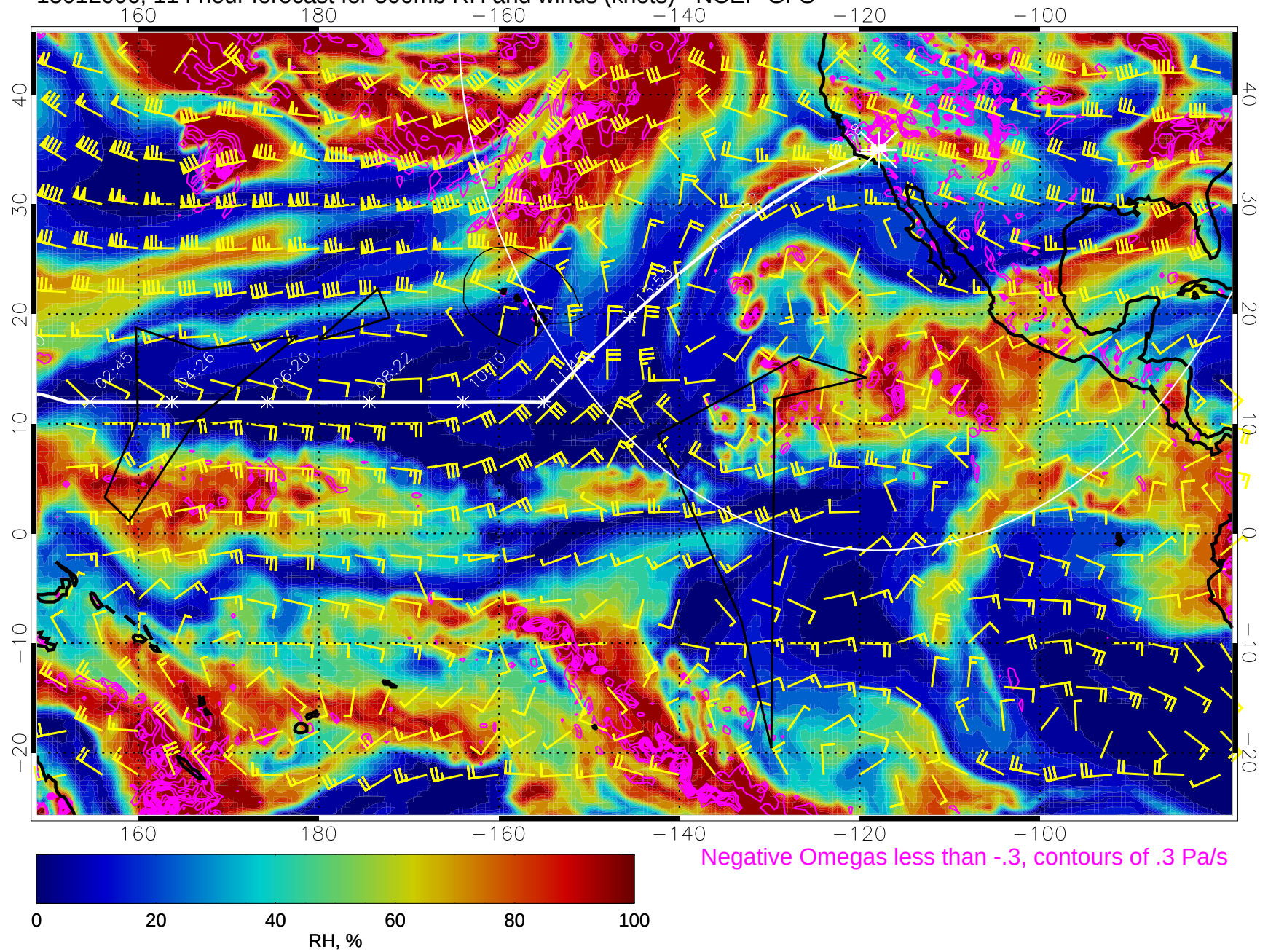
15012006, 114 hour forecast for 500mb RH and winds (knots) - NCEP GFS
