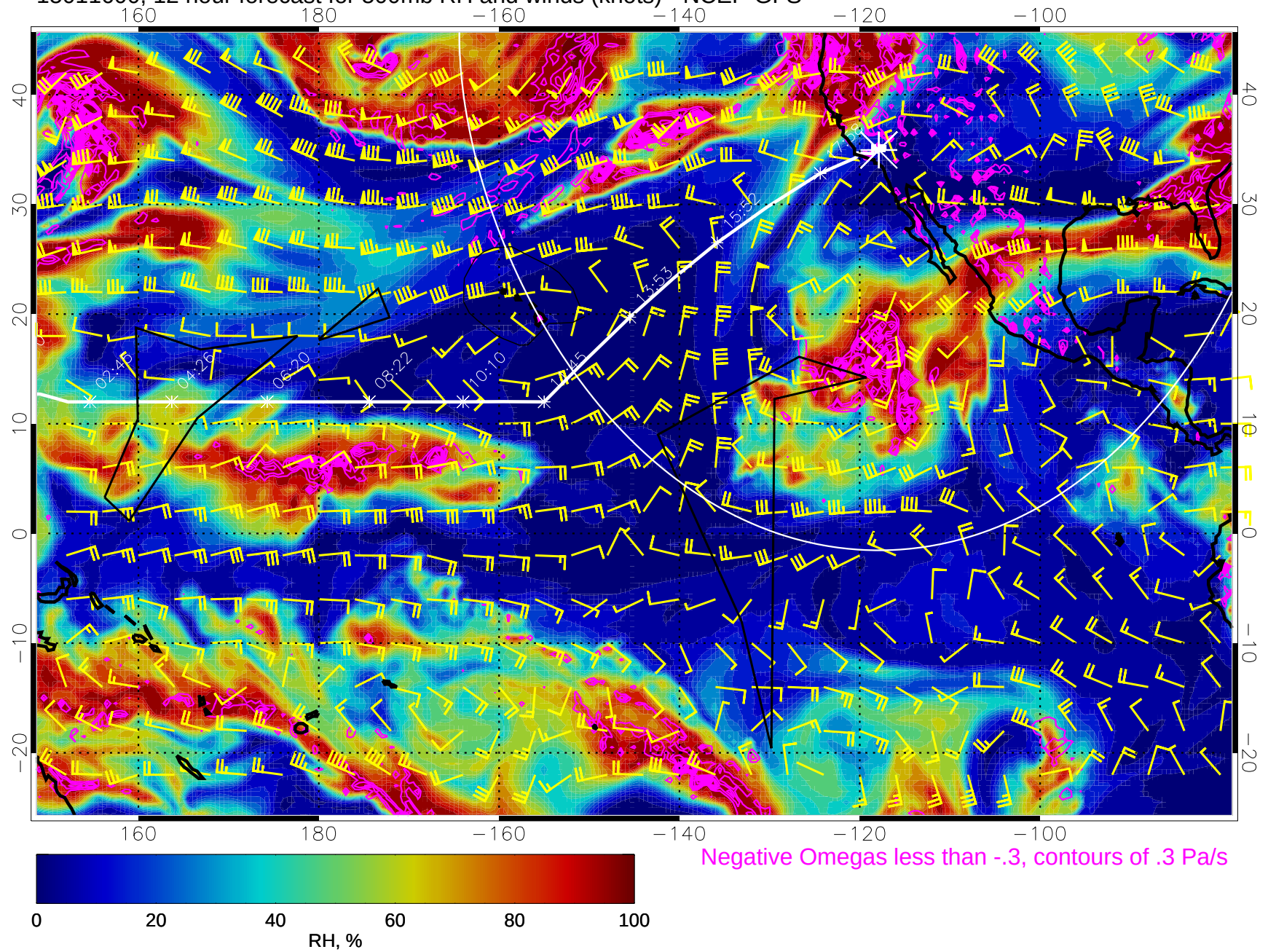
15011600, 12 hour forecast for 500mb RH and winds (knots) - NCEP GFS
