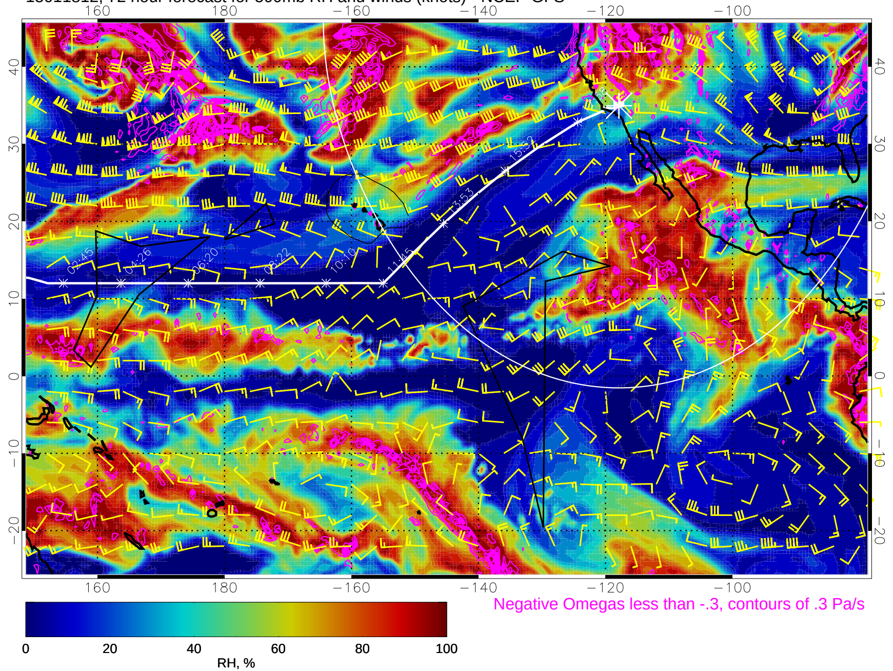
15011812, 72 hour forecast for 500mb RH and winds (knots) - NCEP GFS
