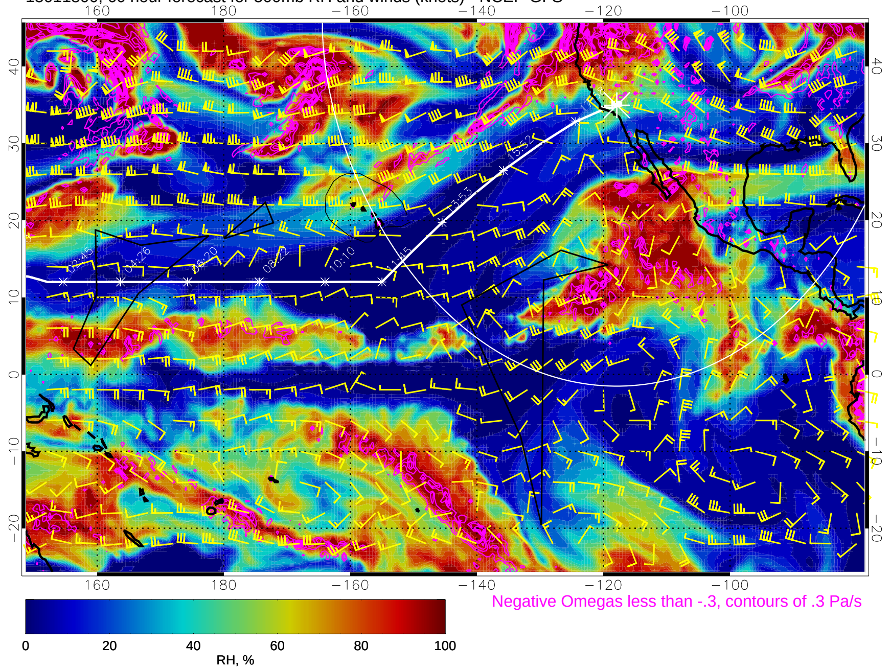
15011800, 60 hour forecast for 500mb RH and winds (knots) - NCEP GFS
