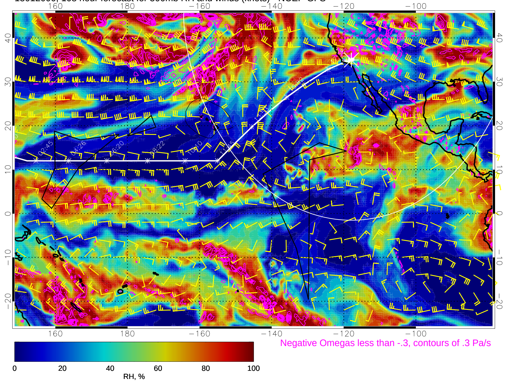
15012000, 108 hour forecast for 500mb RH and winds (knots) - NCEP GFS
