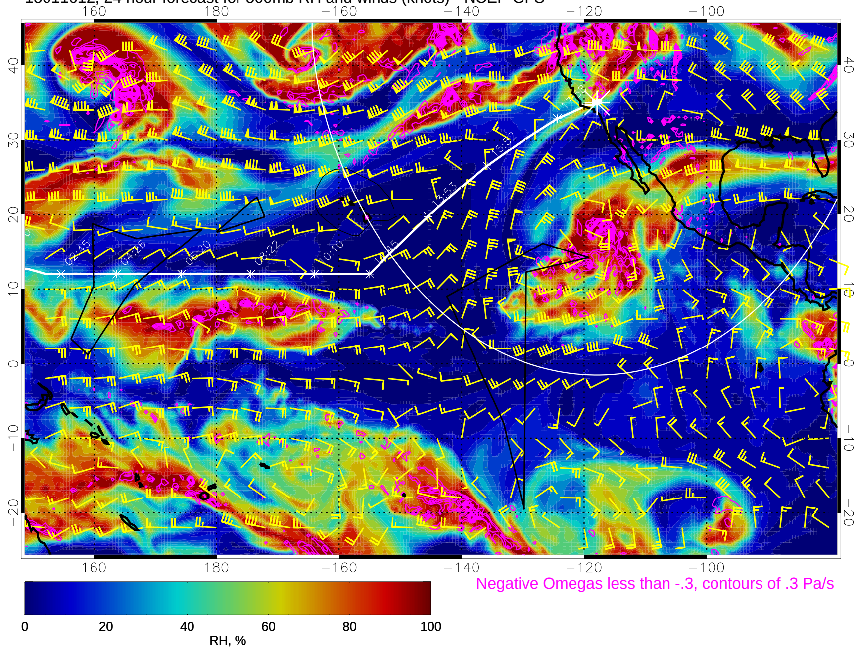
15011612, 24 hour forecast for 500mb RH and winds (knots) - NCEP GFS
