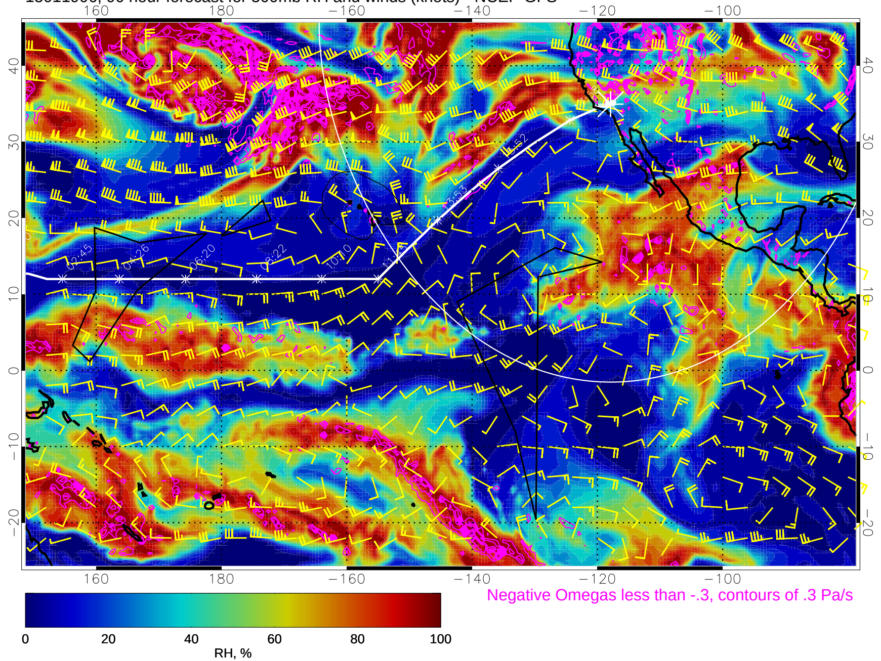
15011906, 90 hour forecast for 500mb RH and winds (knots) - NCEP GFS
