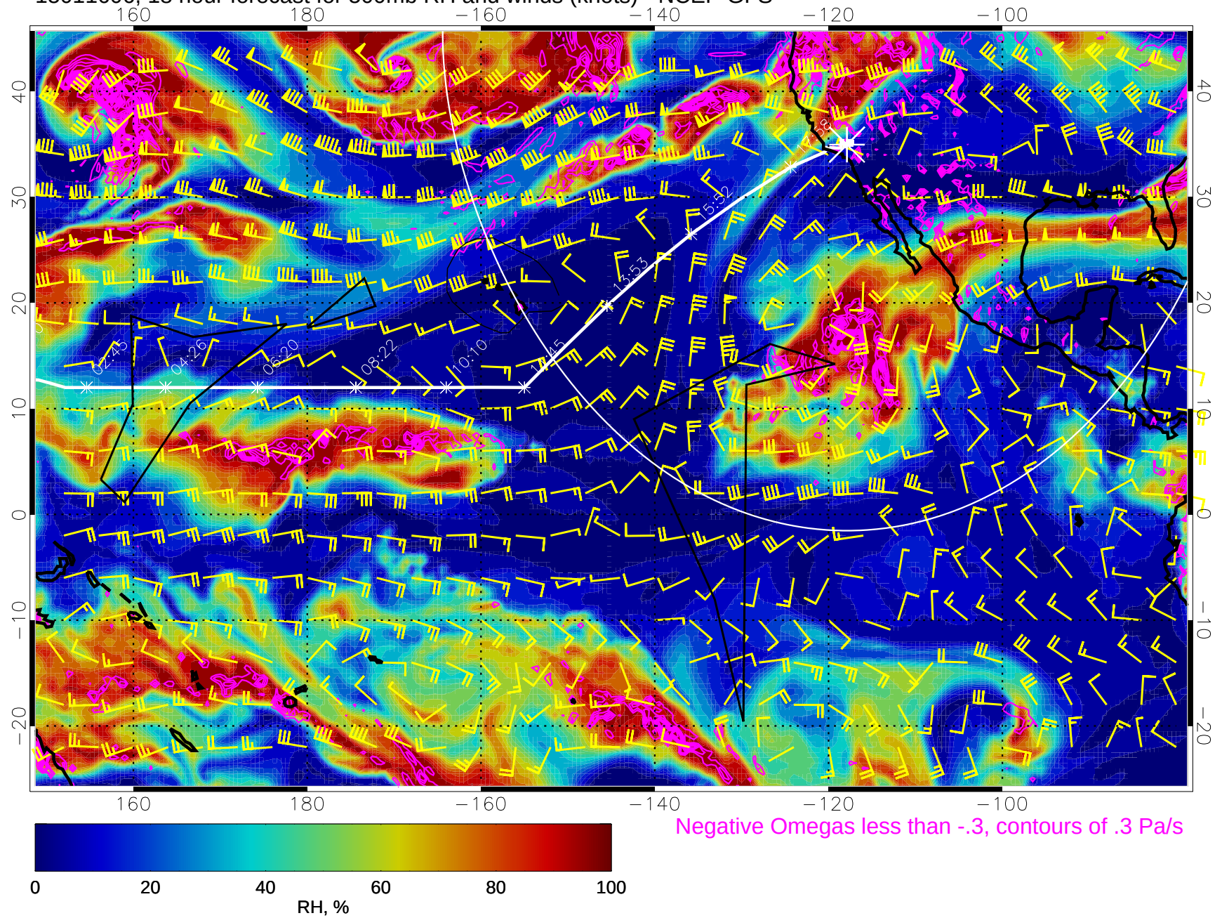
15011606, 18 hour forecast for 500mb RH and winds (knots) - NCEP GFS
