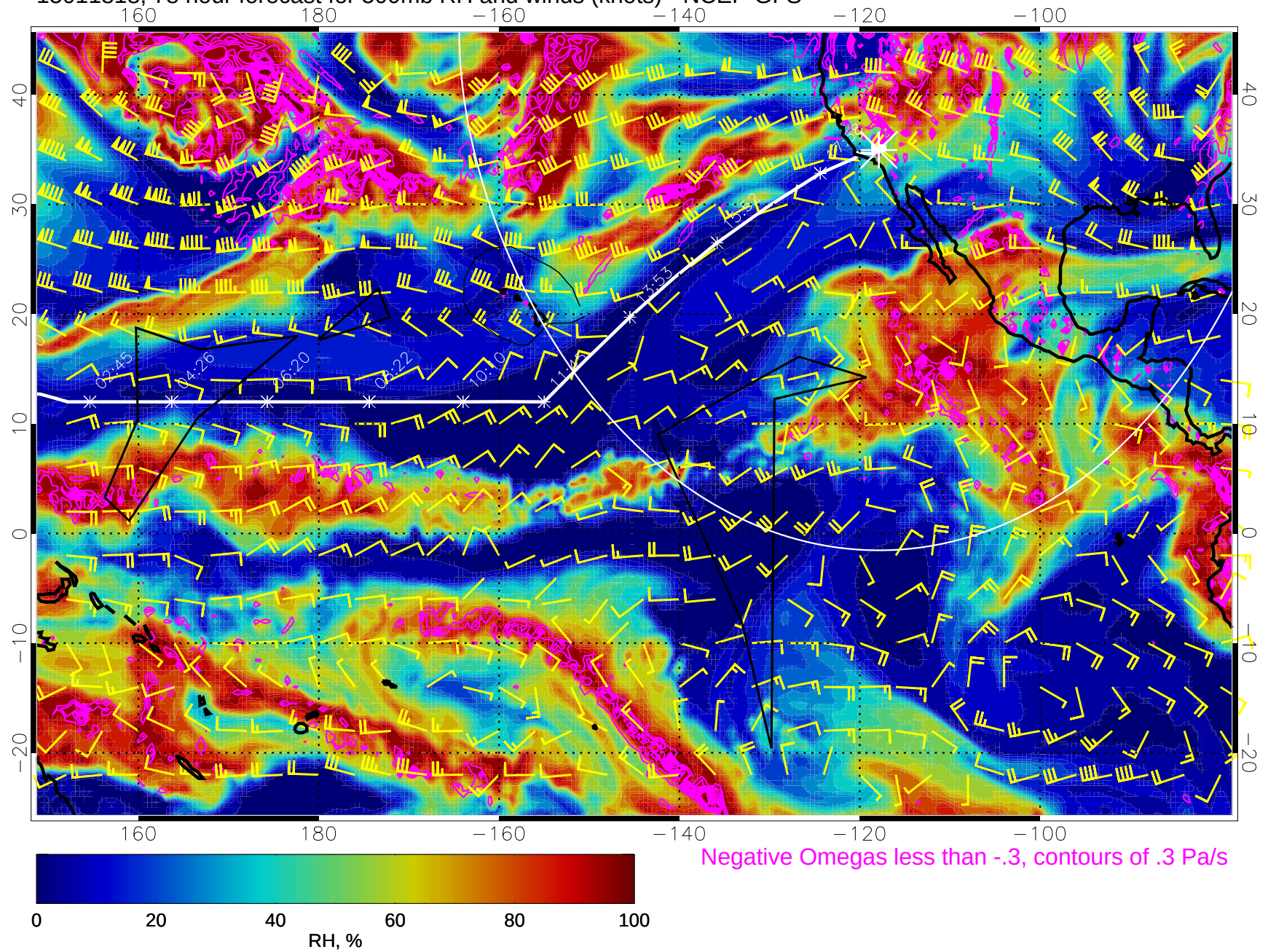
15011818, 78 hour forecast for 500mb RH and winds (knots) - NCEP GFS
