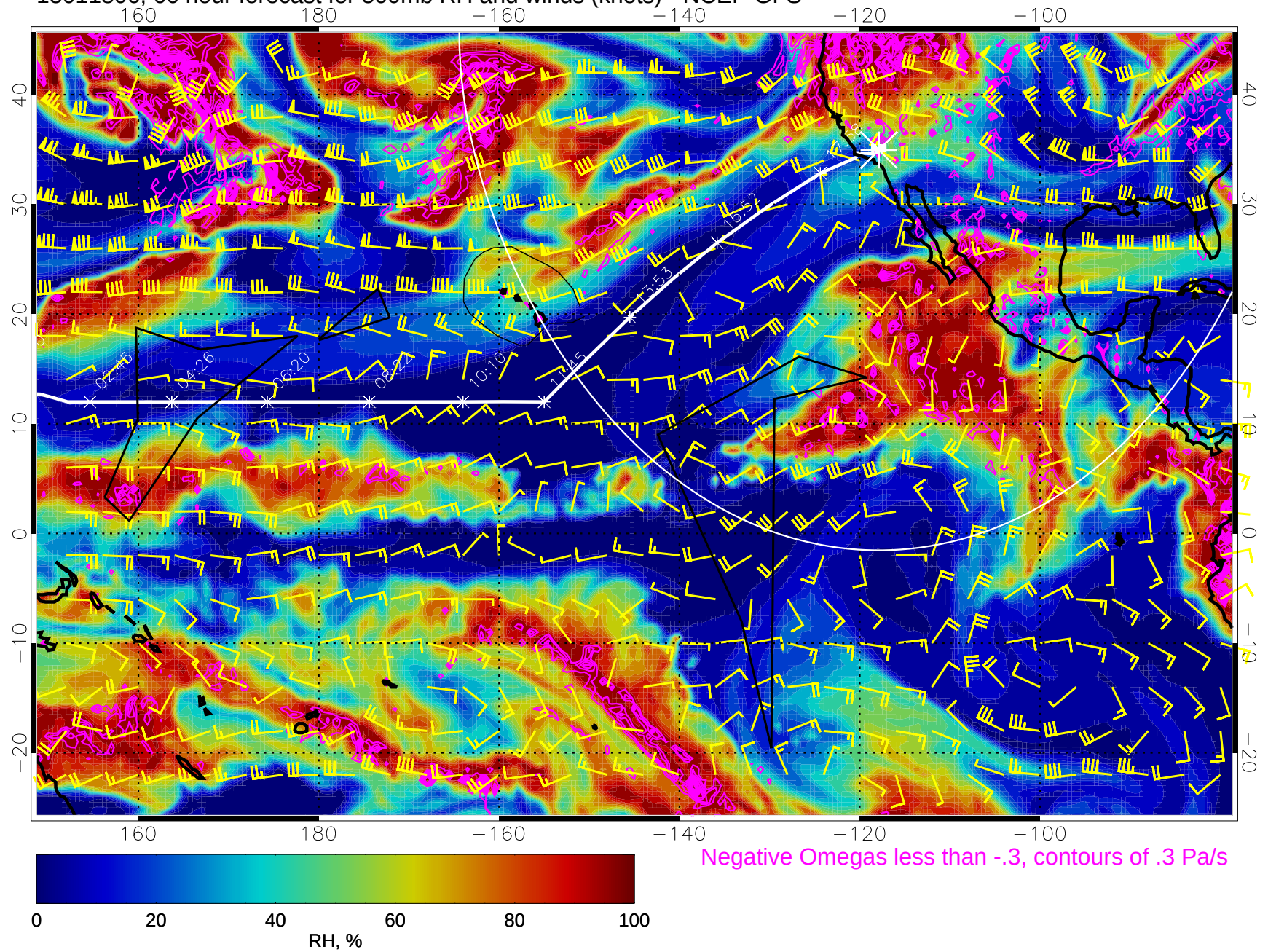
15011806, 66 hour forecast for 500mb RH and winds (knots) - NCEP GFS
