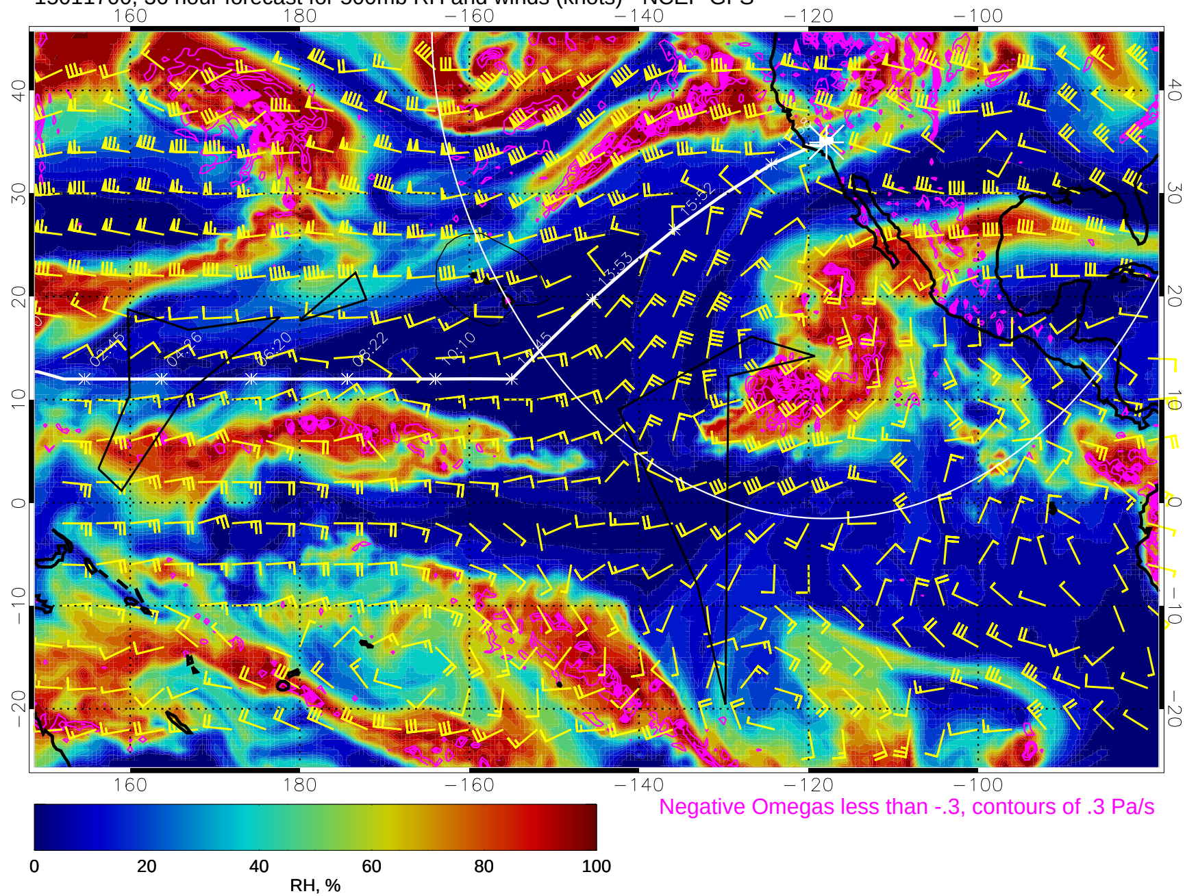
15011700, 36 hour forecast for 500mb RH and winds (knots) - NCEP GFS
