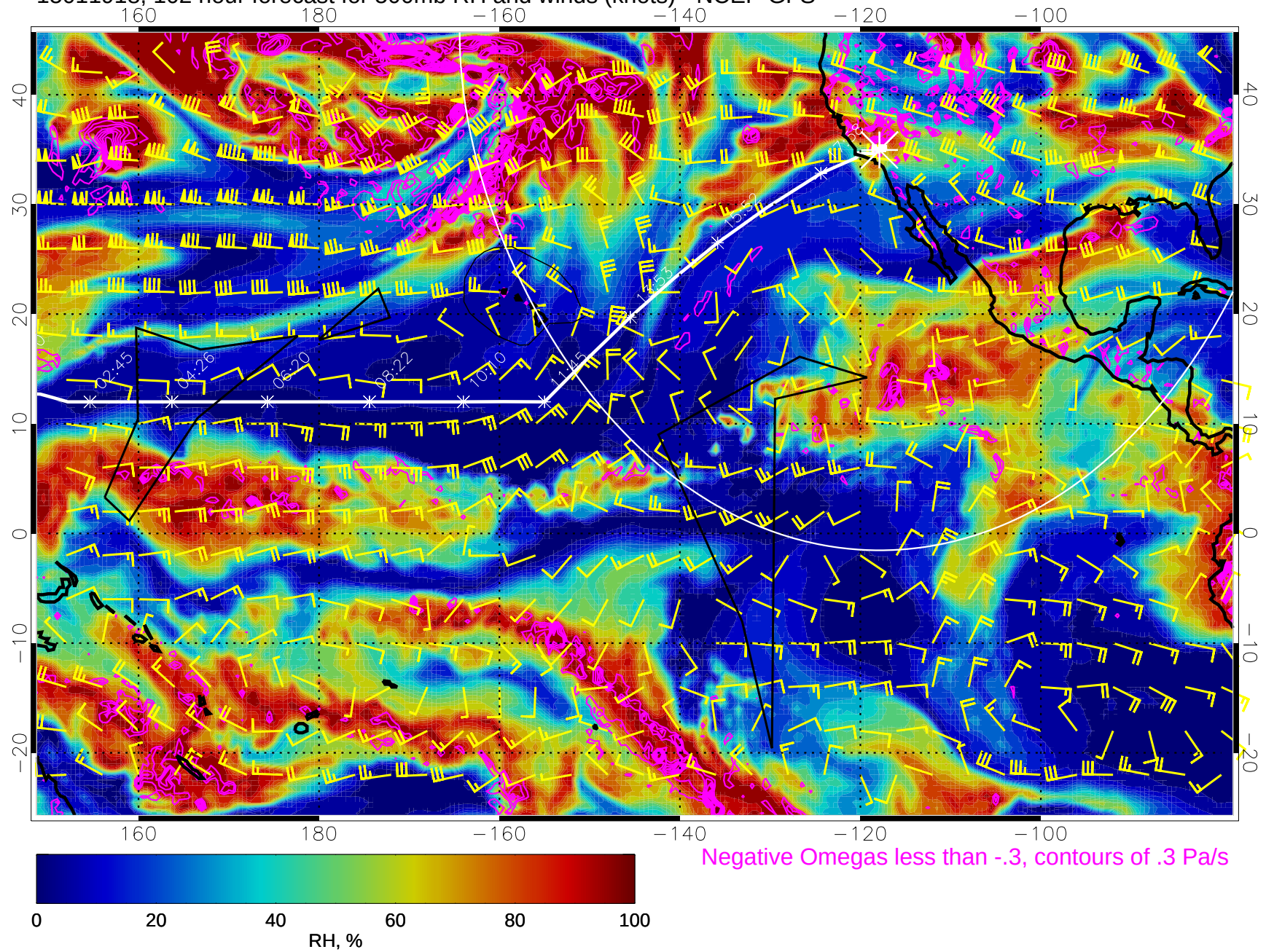
15011918, 102 hour forecast for 500mb RH and winds (knots) - NCEP GFS
