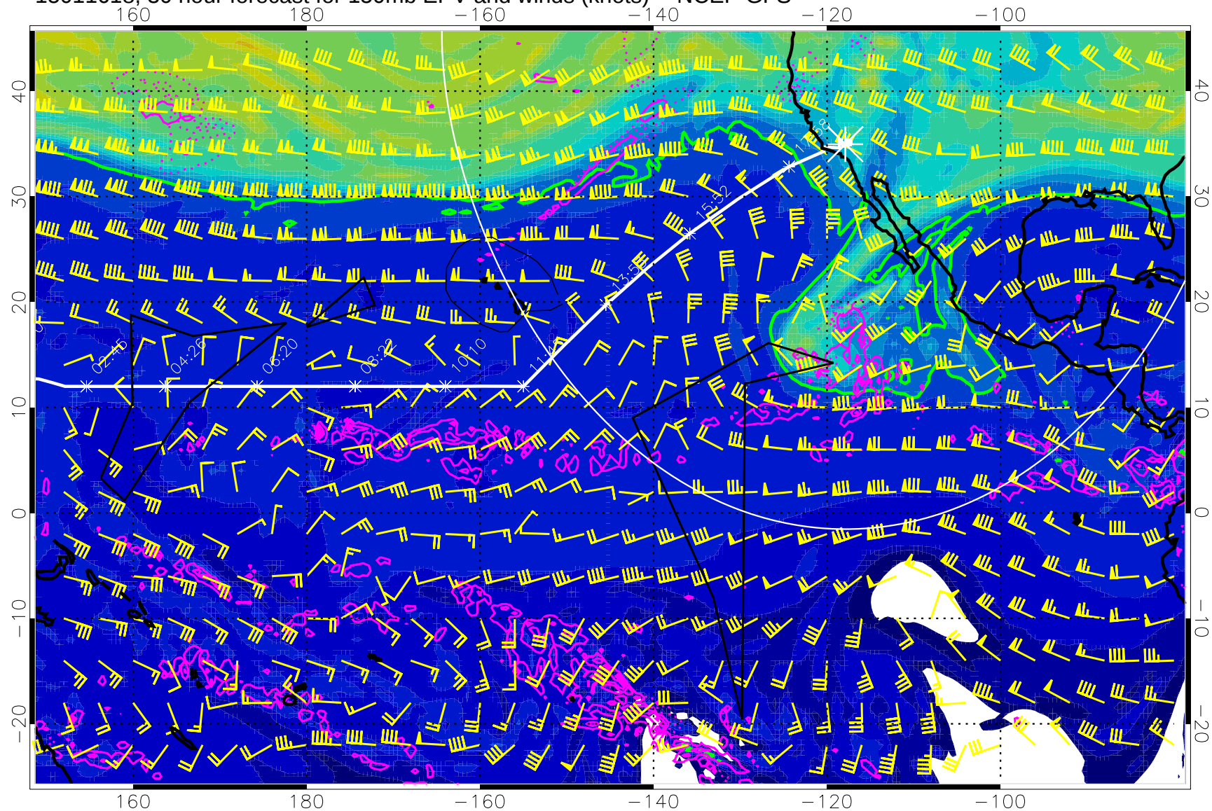
15011618, 30 hour forecast for 150mb EPV and winds (knots) -- NCEP GFS
