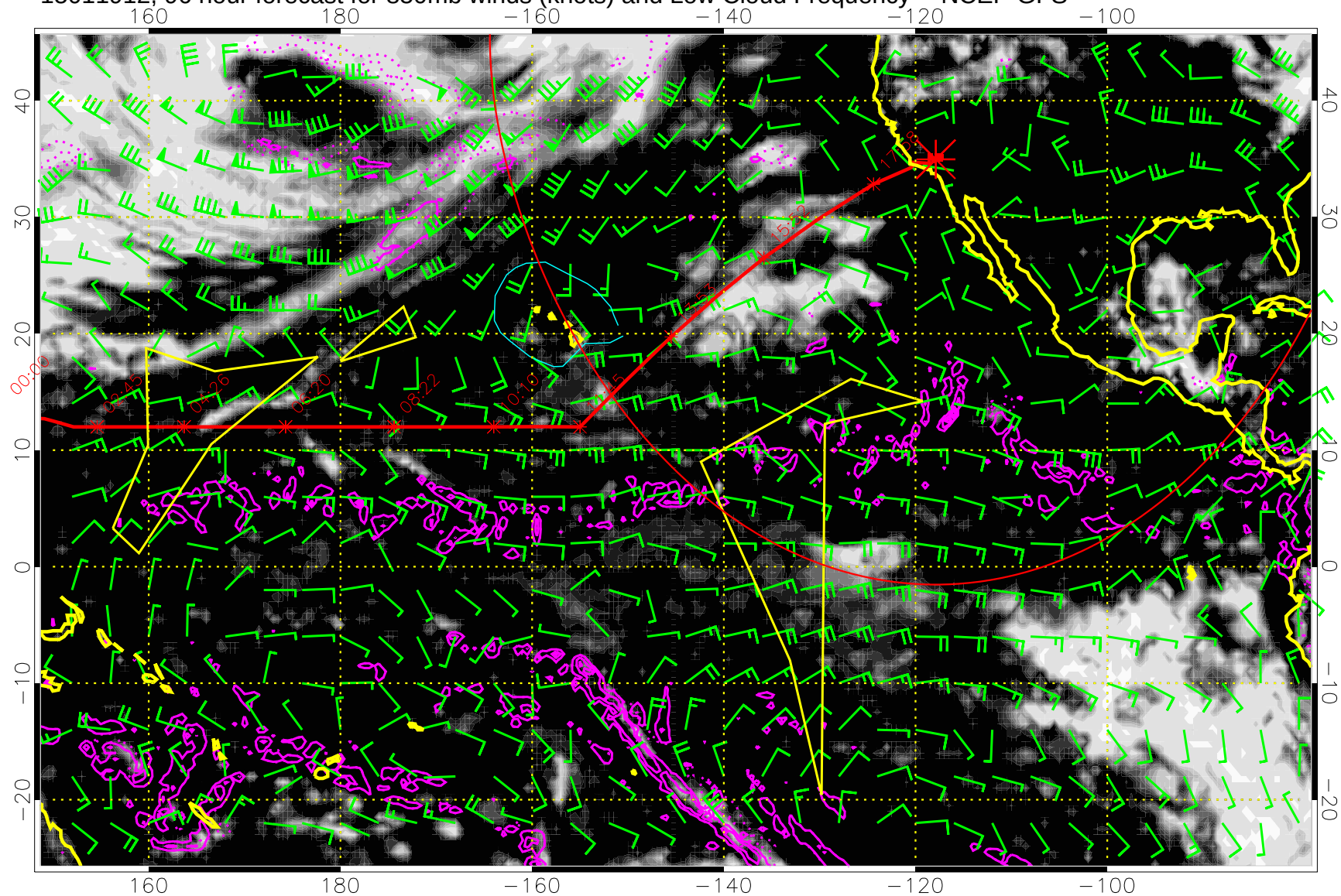
15011912, 96 hour forecast for 850mb winds (knots) and Low Cloud Frequency -- NCEP GFS
