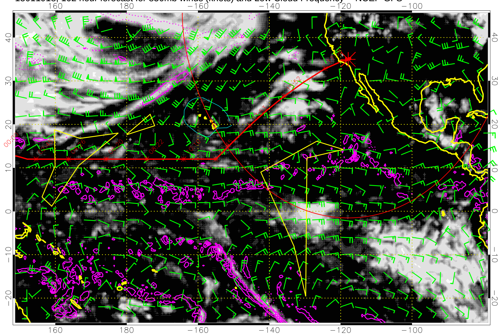
15011918, 102 hour forecast for 850mb winds (knots) and Low Cloud Frequency -- NCEP GFS
