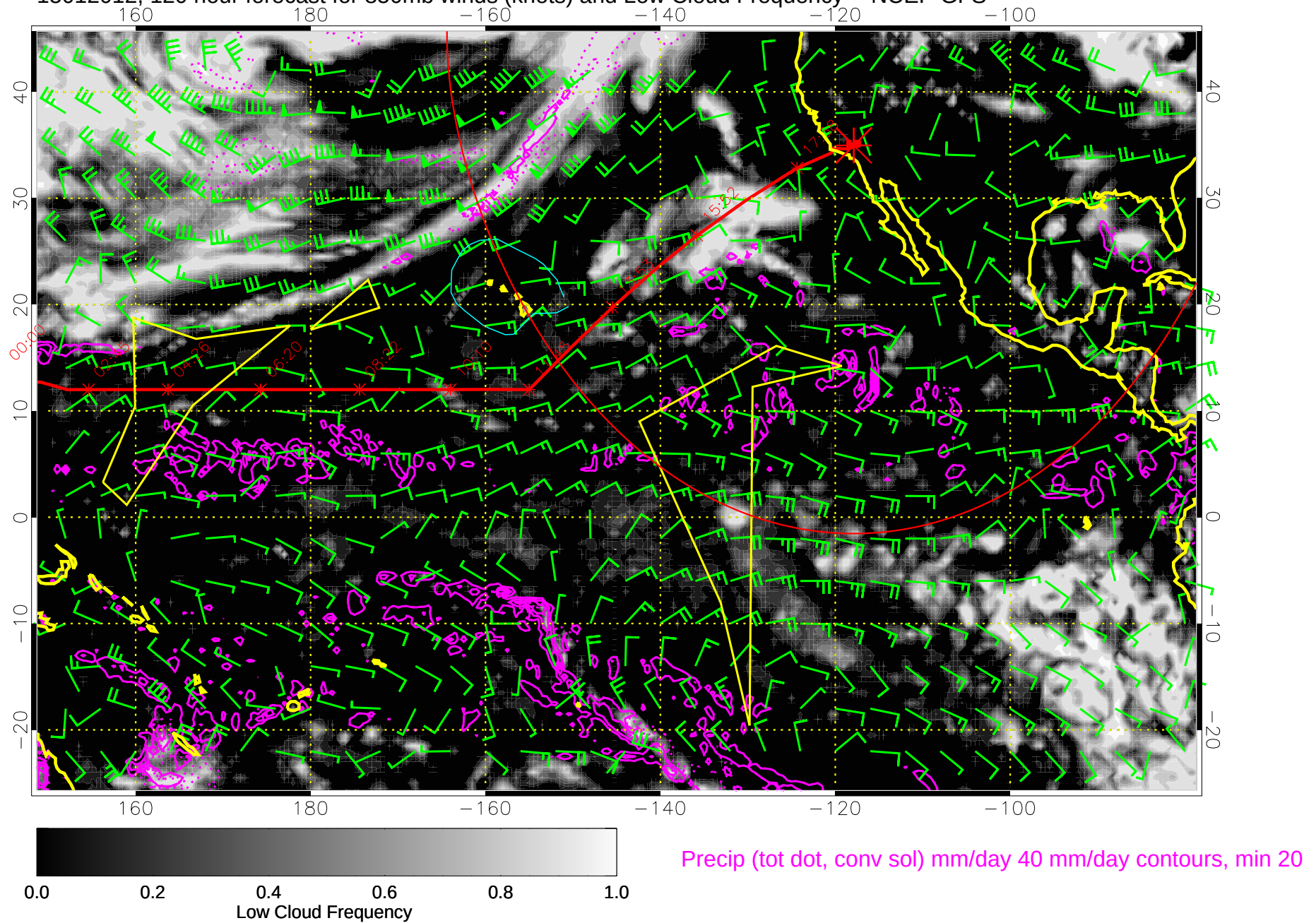
15012012, 120 hour forecast for 850mb winds (knots) and Low Cloud Frequency -- NCEP GFS
