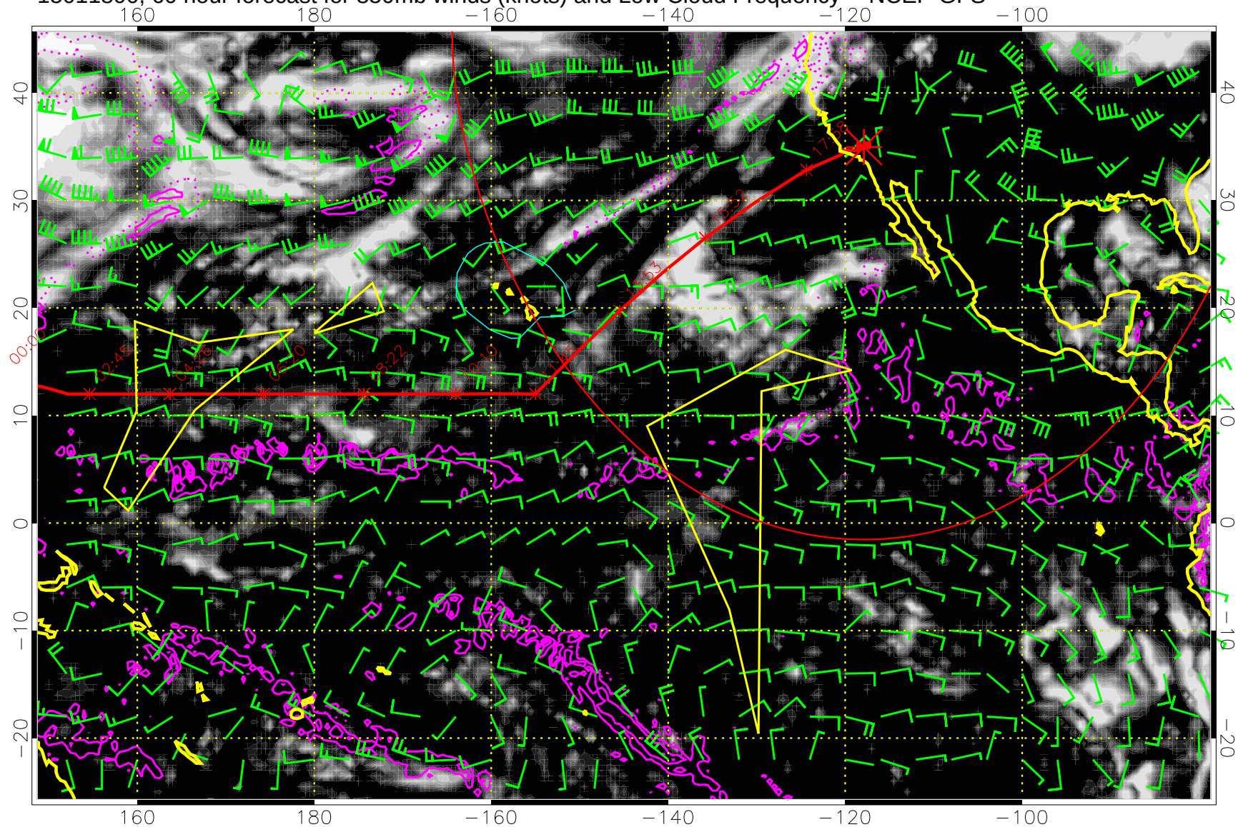
15011800, 60 hour forecast for 850mb winds (knots) and Low Cloud Frequency -- NCEP GFS
