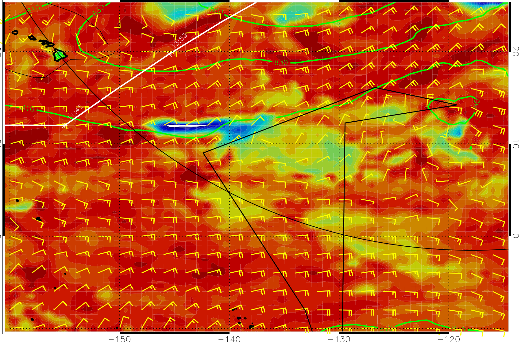
East for elements 1, 2, and 3 (km/s) \rightarrow 150 \rightarrow 140 \rightarrow 130 \rightarrow 120
