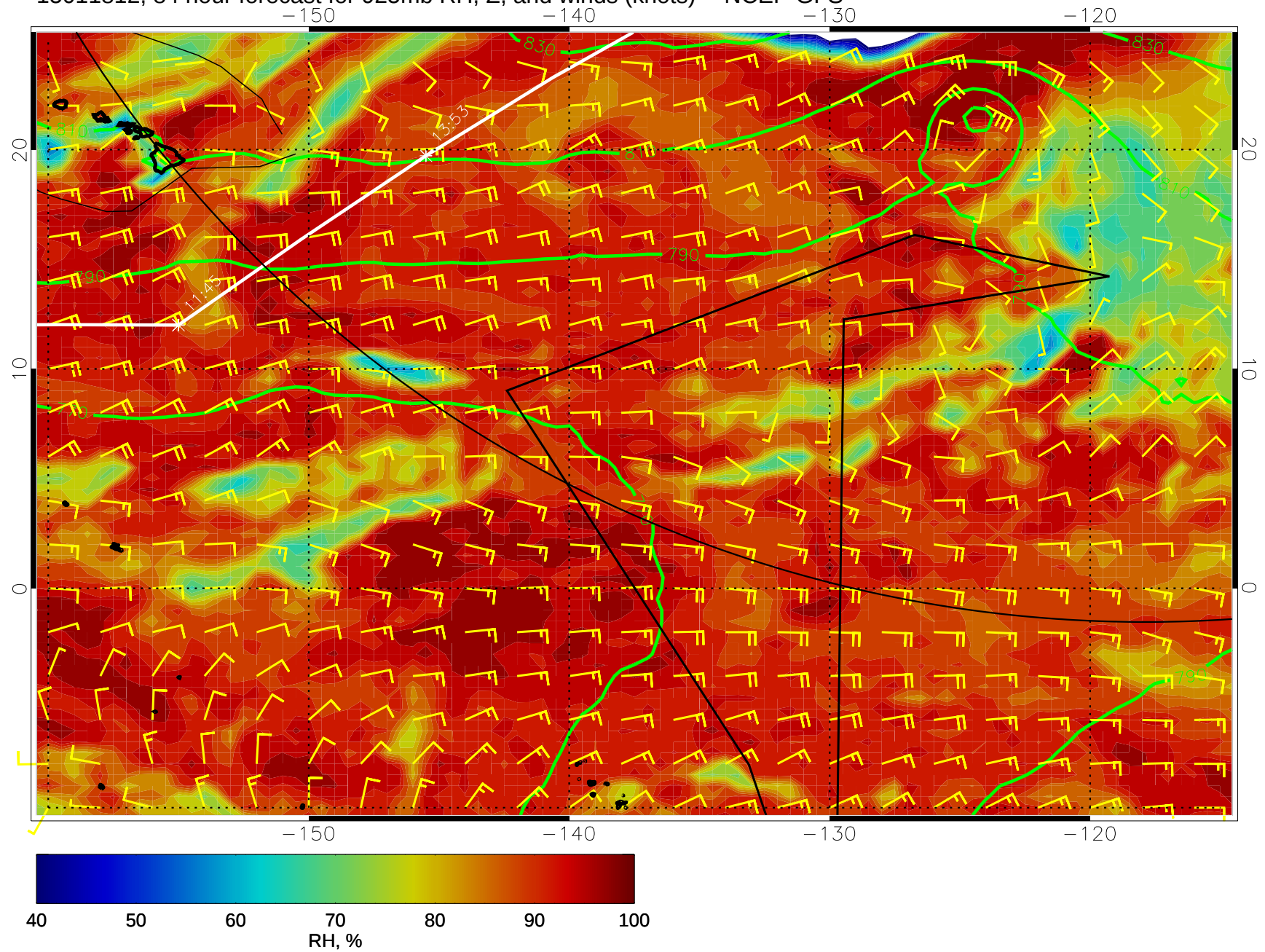
15011812, 84 hour forecast for 925mb RH, Z, and winds (knots) -- NCEP GFS
