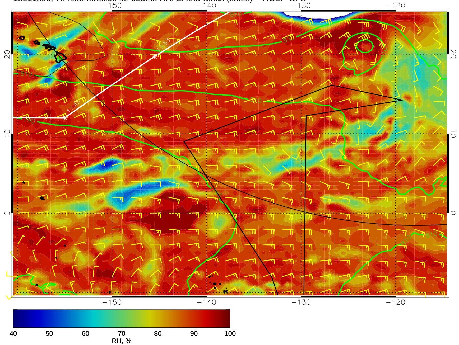
15011806, 78 hour forecast for 925mb RH, Z, and winds (knots) -- NCEP GFS
