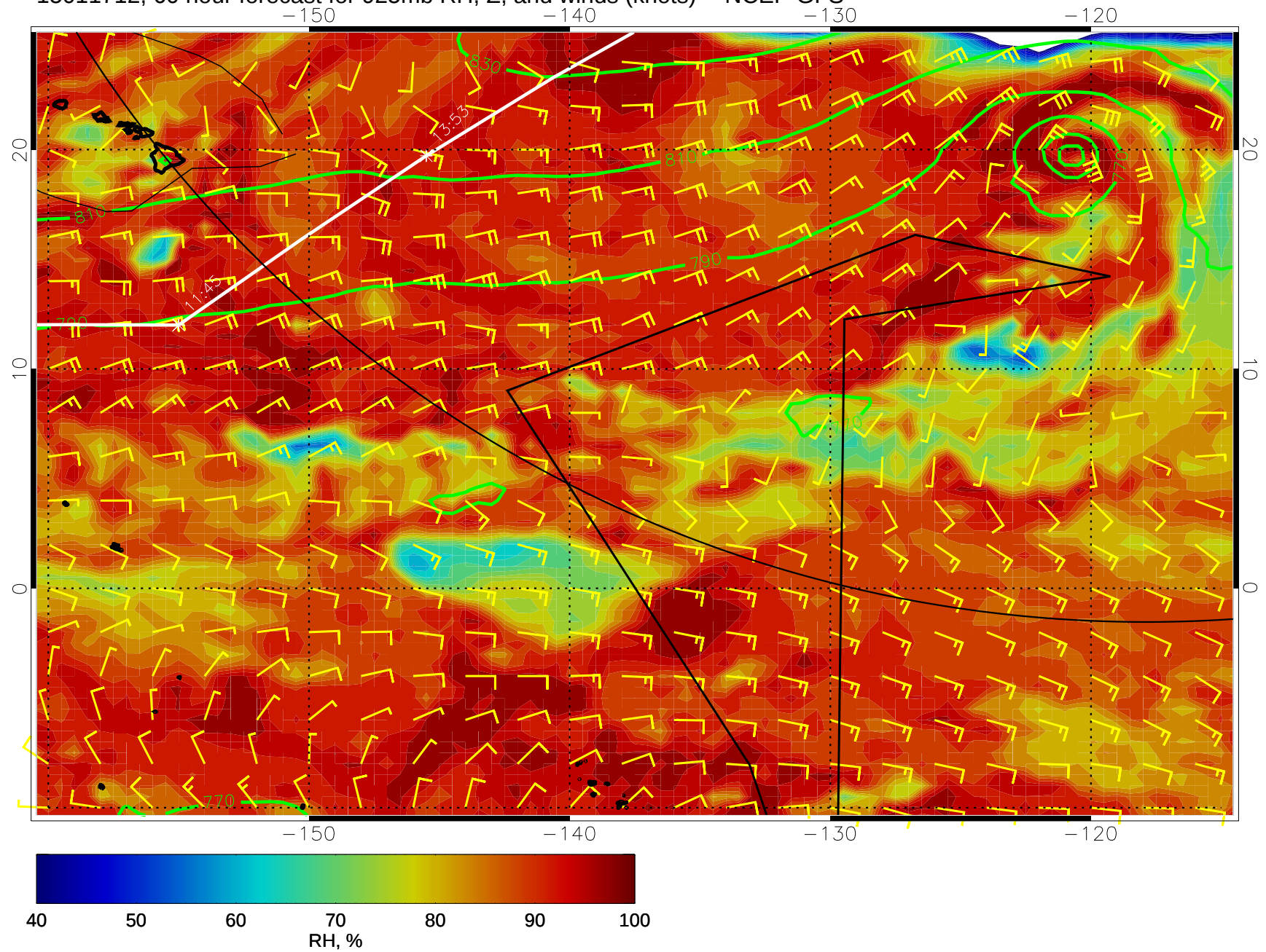
15011712, 60 hour forecast for 925mb RH, Z, and winds (knots) -- NCEP GFS
