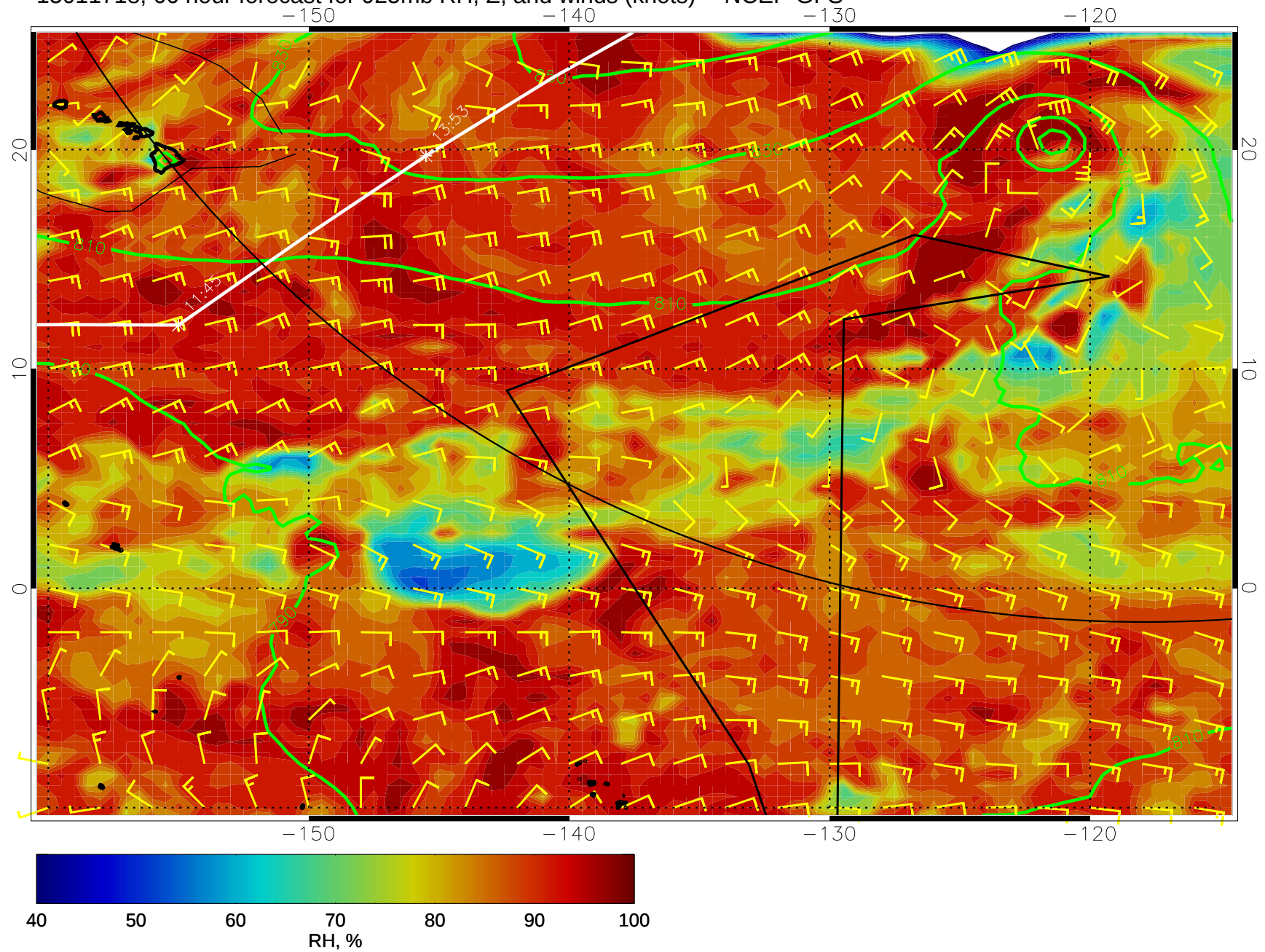
15011718, 66 hour forecast for 925mb RH, Z, and winds (knots) -- NCEP GFS
