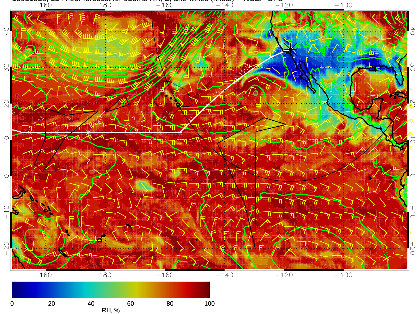
15011918, 114 hour forecast for 925mb RH, Z, and winds (knots) -- NCEP GFS
