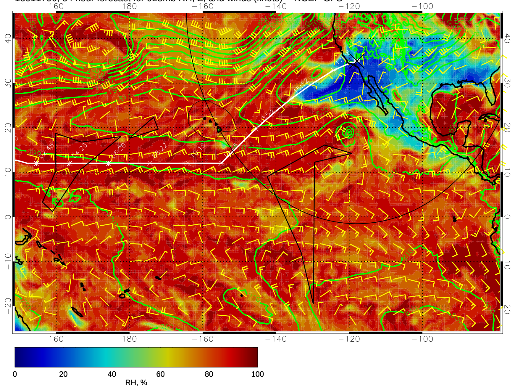
15011706, 54 hour forecast for 925mb RH, Z, and winds (knots) -- NCEP GFS
