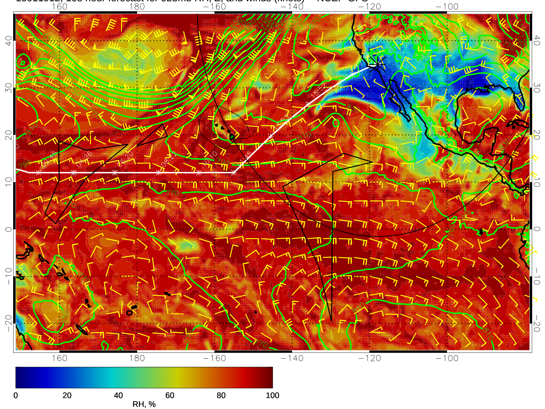
15011912, 108 hour forecast for 925mb RH, Z, and winds (knots) -- NCEP GFS
