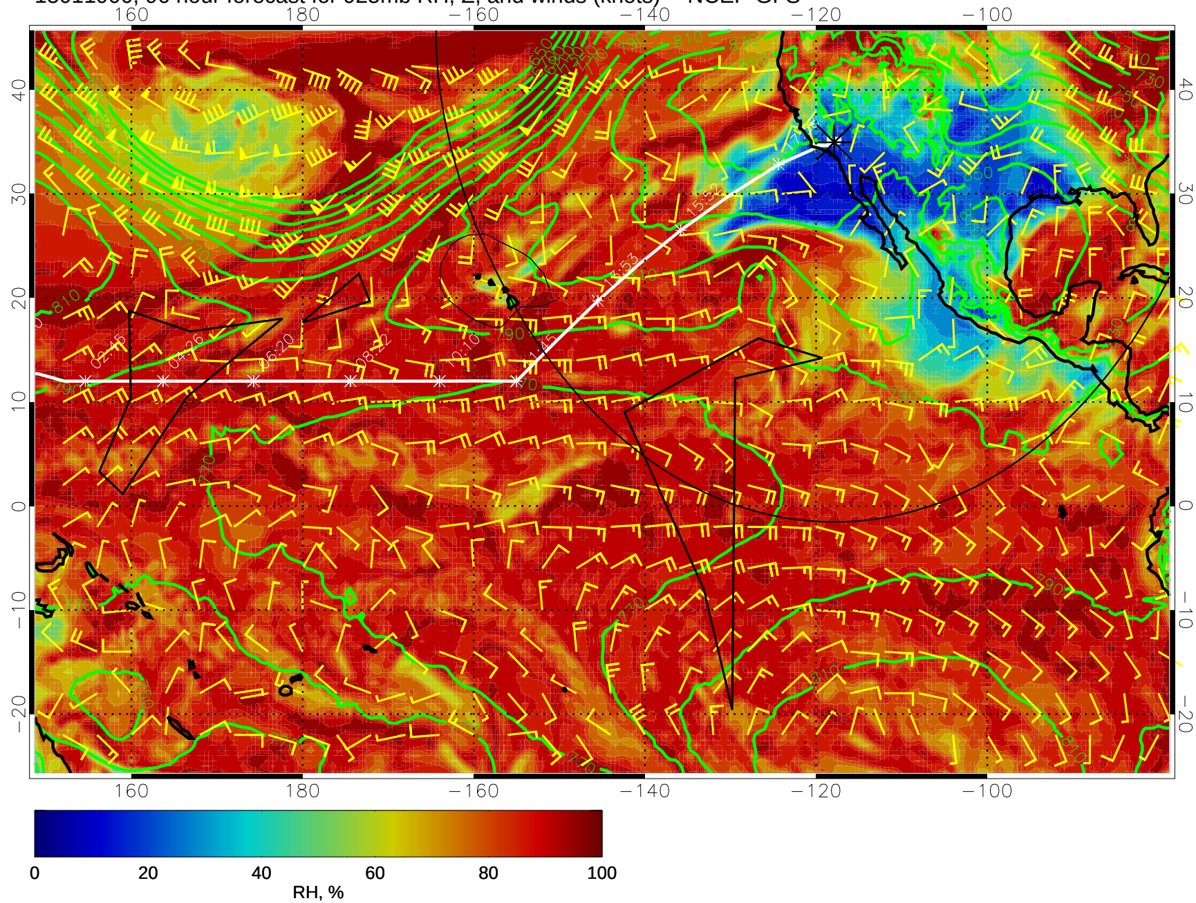
15011900, 96 hour forecast for 925mb RH, Z, and winds (knots) -- NCEP GFS
