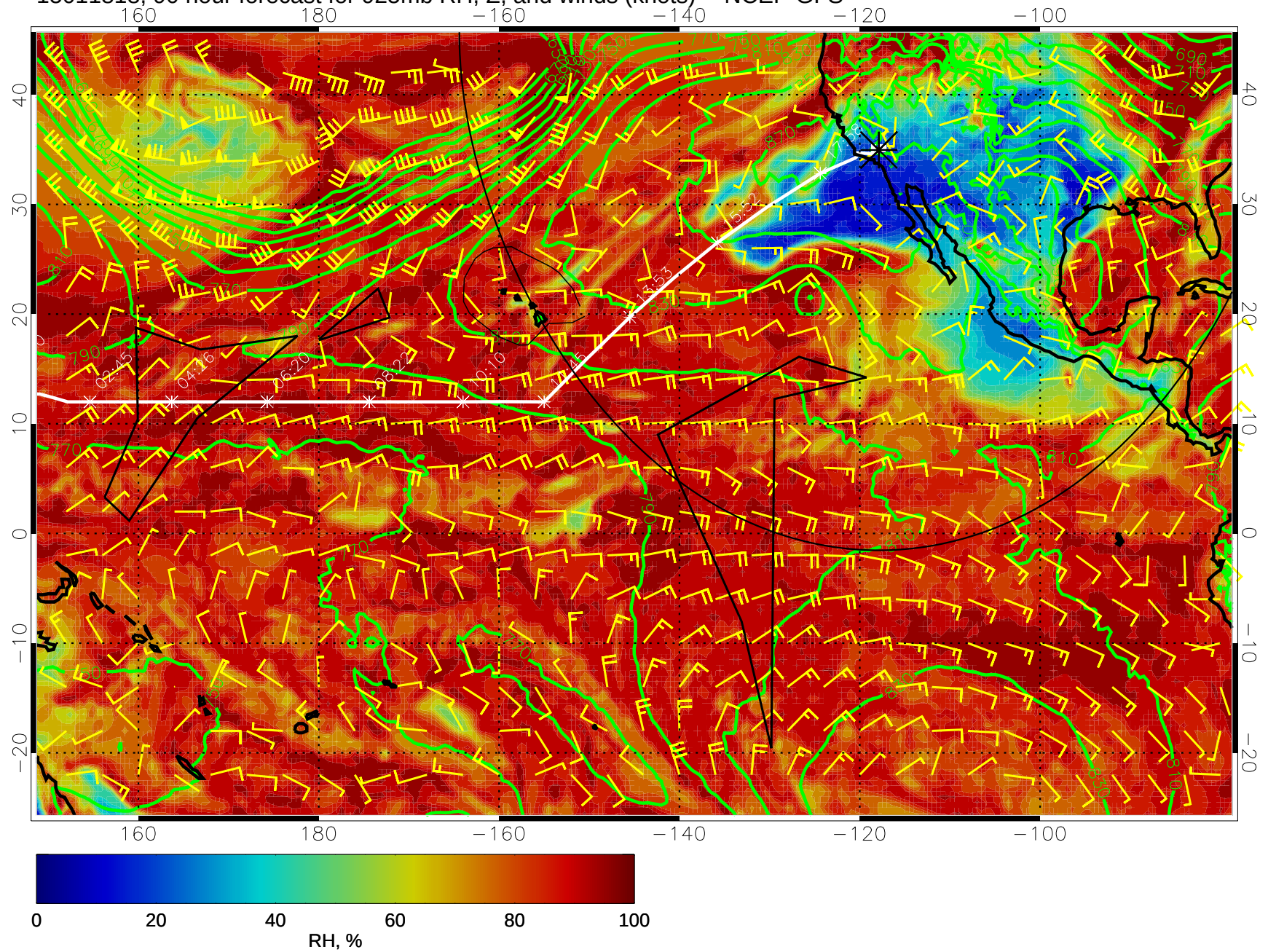
15011818, 90 hour forecast for 925mb RH, Z, and winds (knots) -- NCEP GFS
