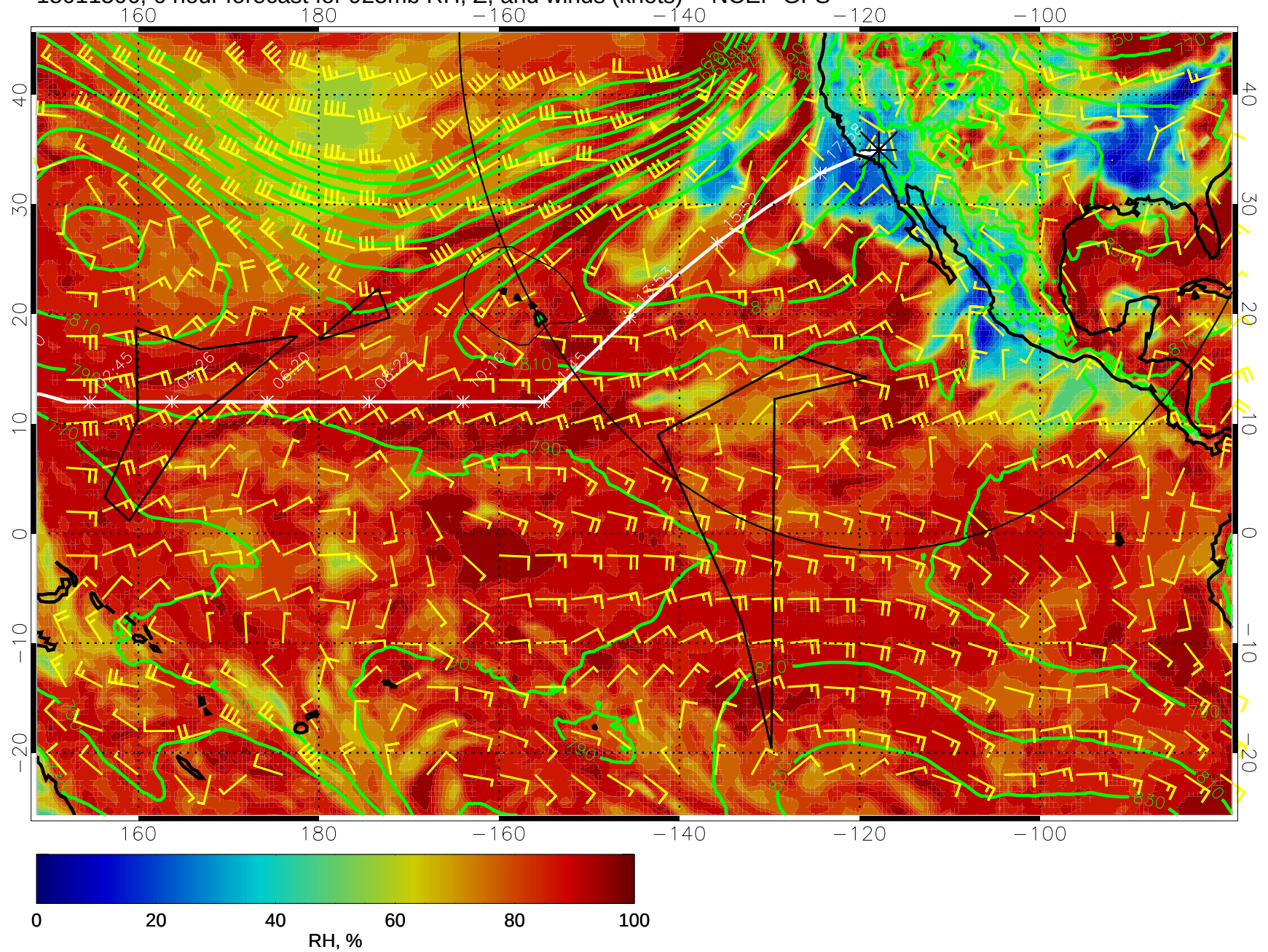
15011506, 6 hour forecast for 925mb RH, Z, and winds (knots) -- NCEP GFS
