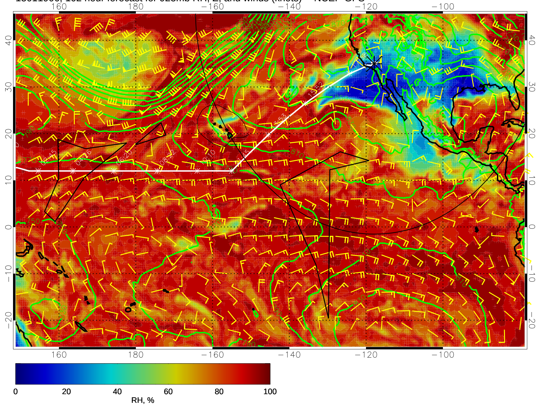
15011906, 102 hour forecast for 925mb RH, Z, and winds (knots) -- NCEP GFS
