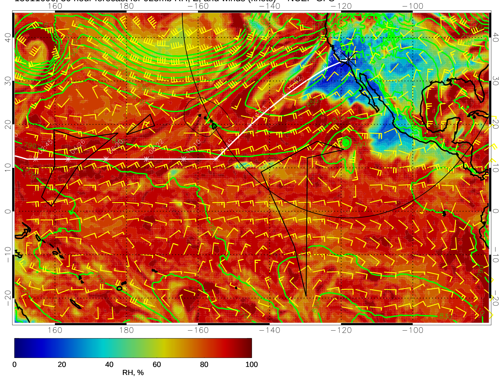
15011606, 30 hour forecast for 925mb RH, Z, and winds (knots) -- NCEP GFS
