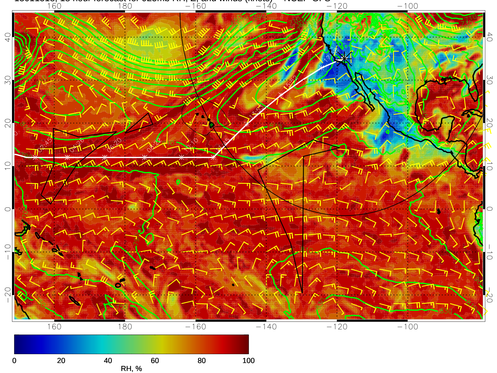
15011518, 18 hour forecast for 925mb RH, Z, and winds (knots) -- NCEP GFS
