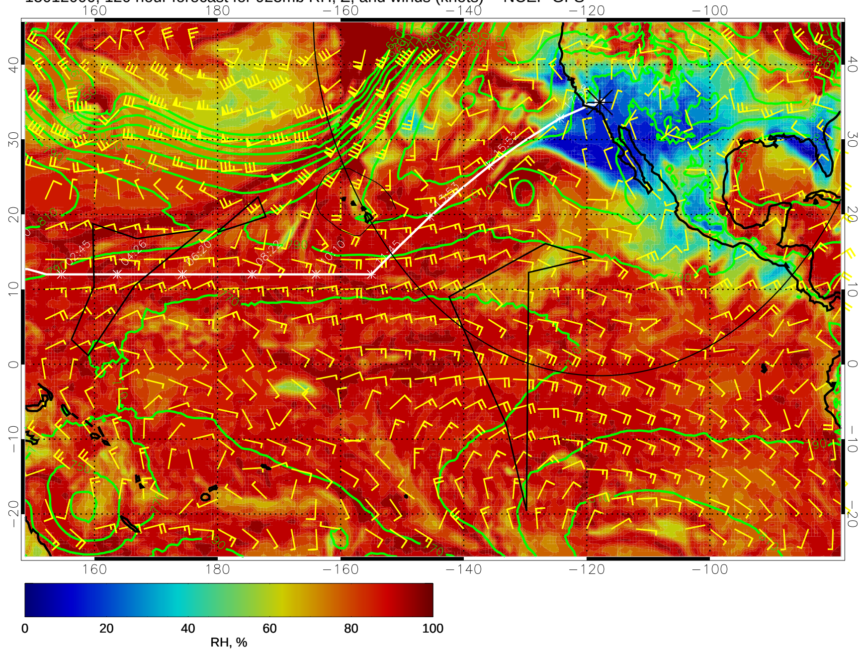
15012000, 120 hour forecast for 925mb RH, Z, and winds (knots) -- NCEP GFS
