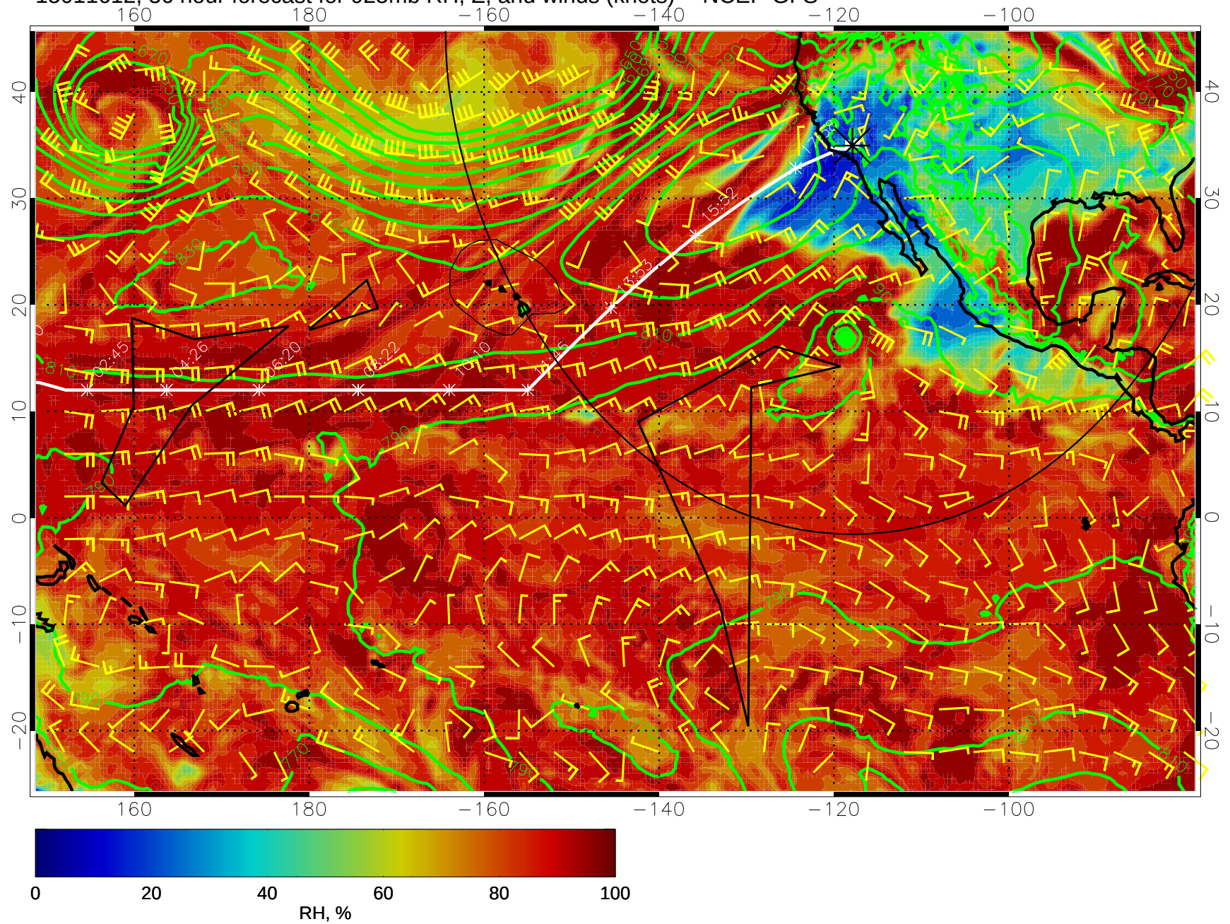
15011612, 36 hour forecast for 925mb RH, Z, and winds (knots) -- NCEP GFS
