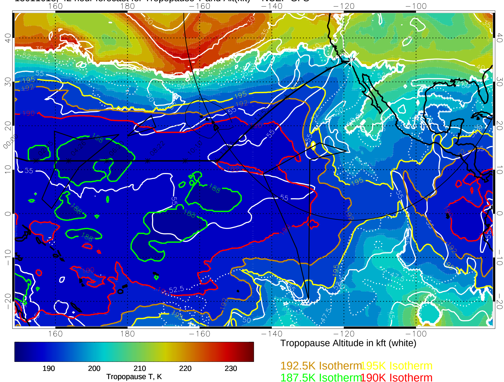
15011618, 42 hour forecast for Tropopause T and Alt(kft) -- NCEP GFS
