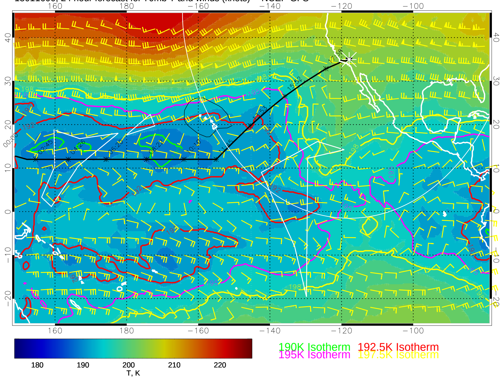
15011600, 24 hour forecast for 70mb T and winds (knots) -- NCEP GFS
