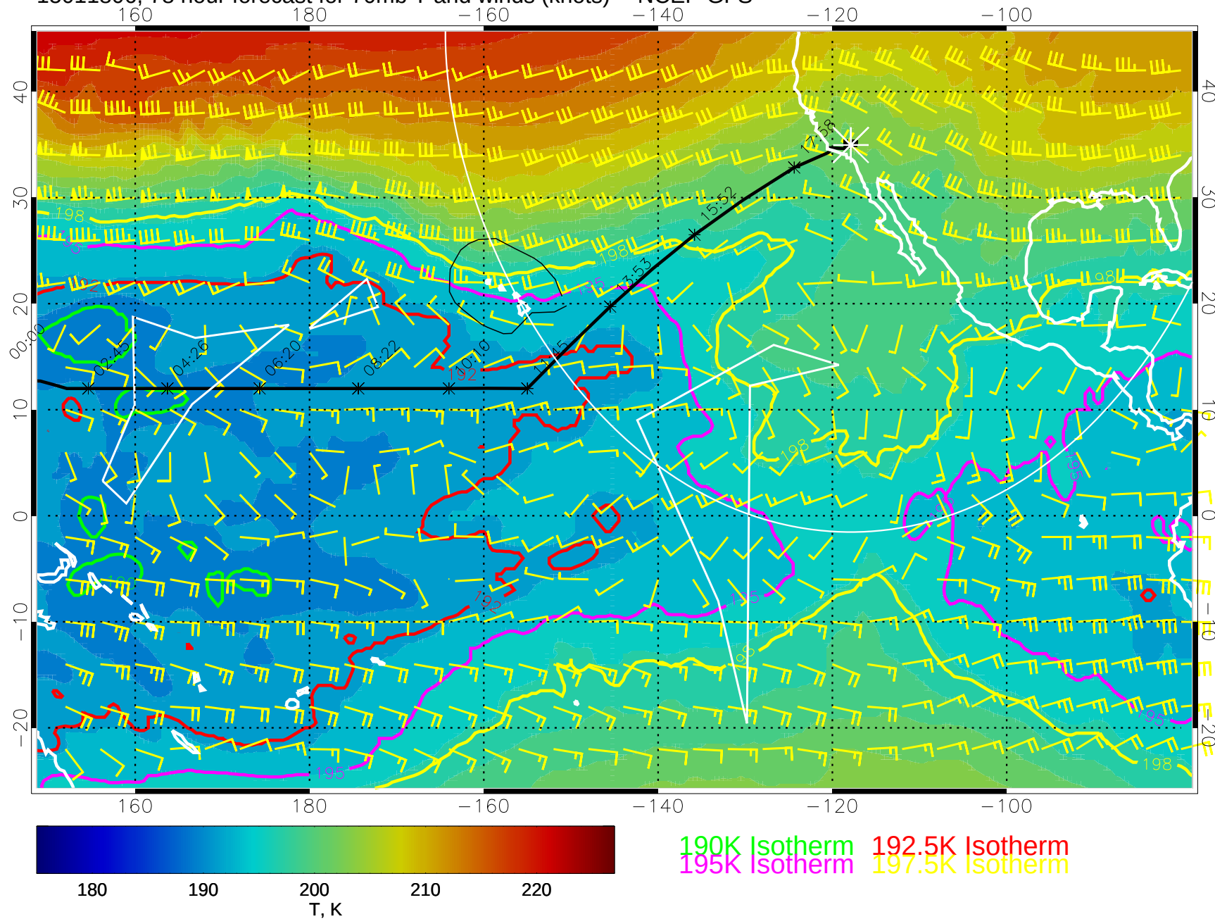
15011806, 78 hour forecast for 70mb T and winds (knots) -- NCEP GFS
