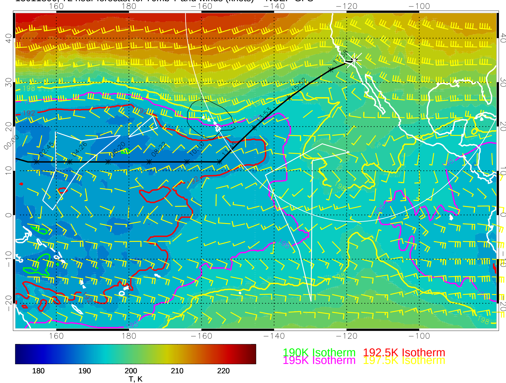
15011800, 72 hour forecast for 70mb T and winds (knots) -- NCEP GFS
