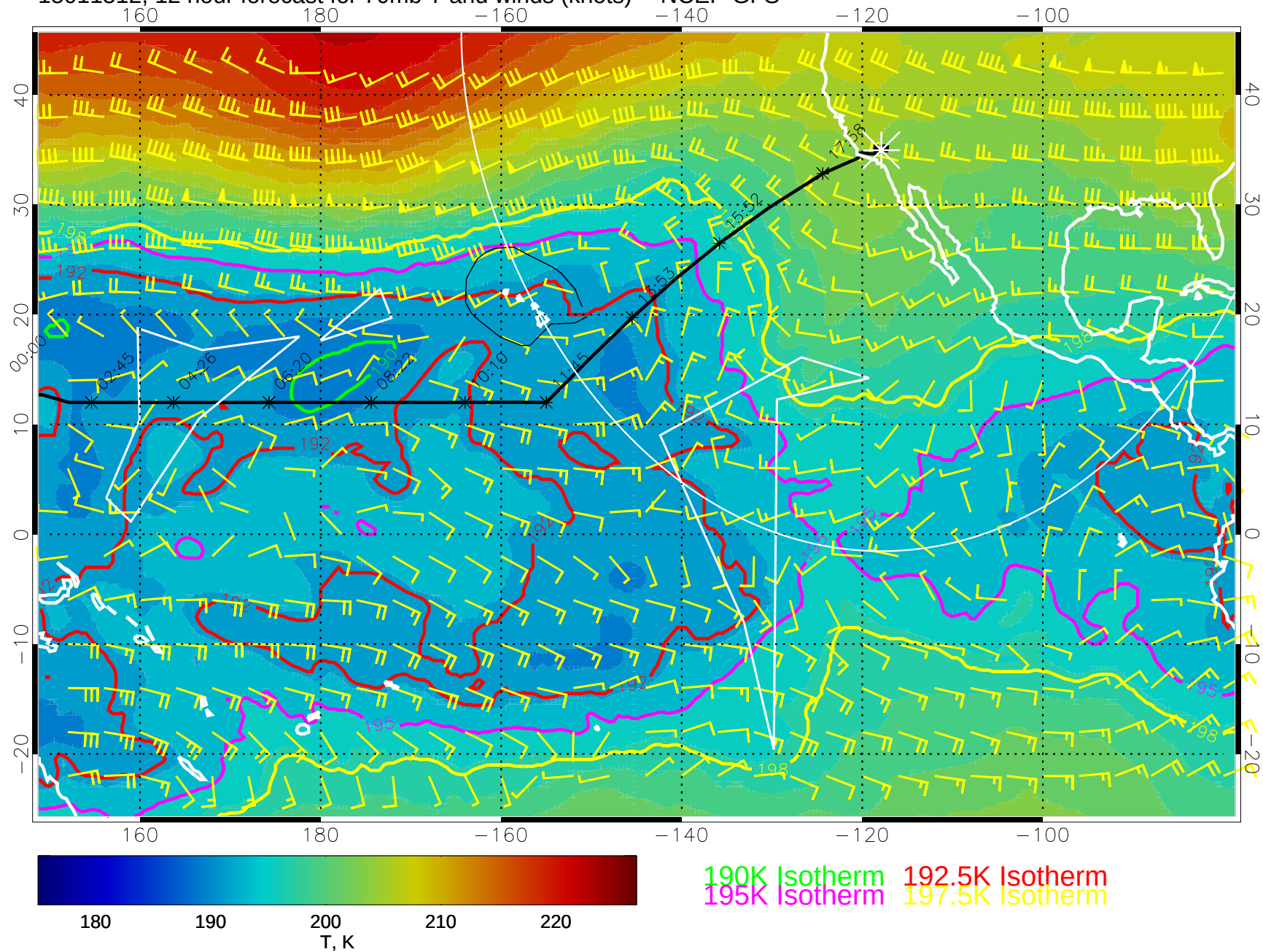
15011512, 12 hour forecast for 70mb T and winds (knots) -- NCEP GFS
