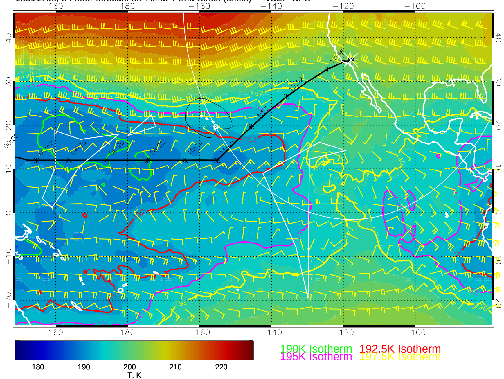
15011706, 54 hour forecast for 70mb T and winds (knots) -- NCEP GFS
