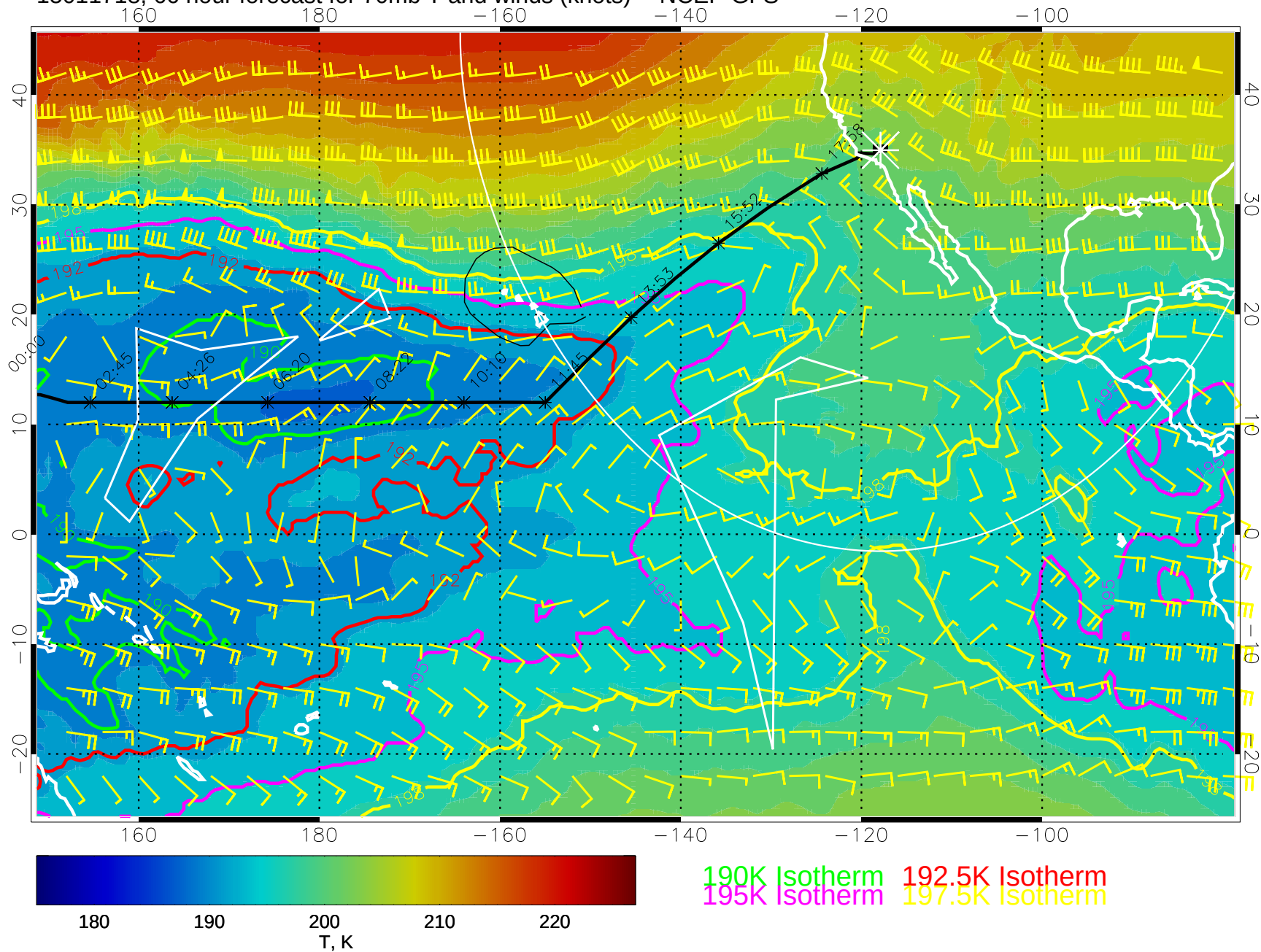
15011718, 66 hour forecast for 70mb T and winds (knots) -- NCEP GFS
