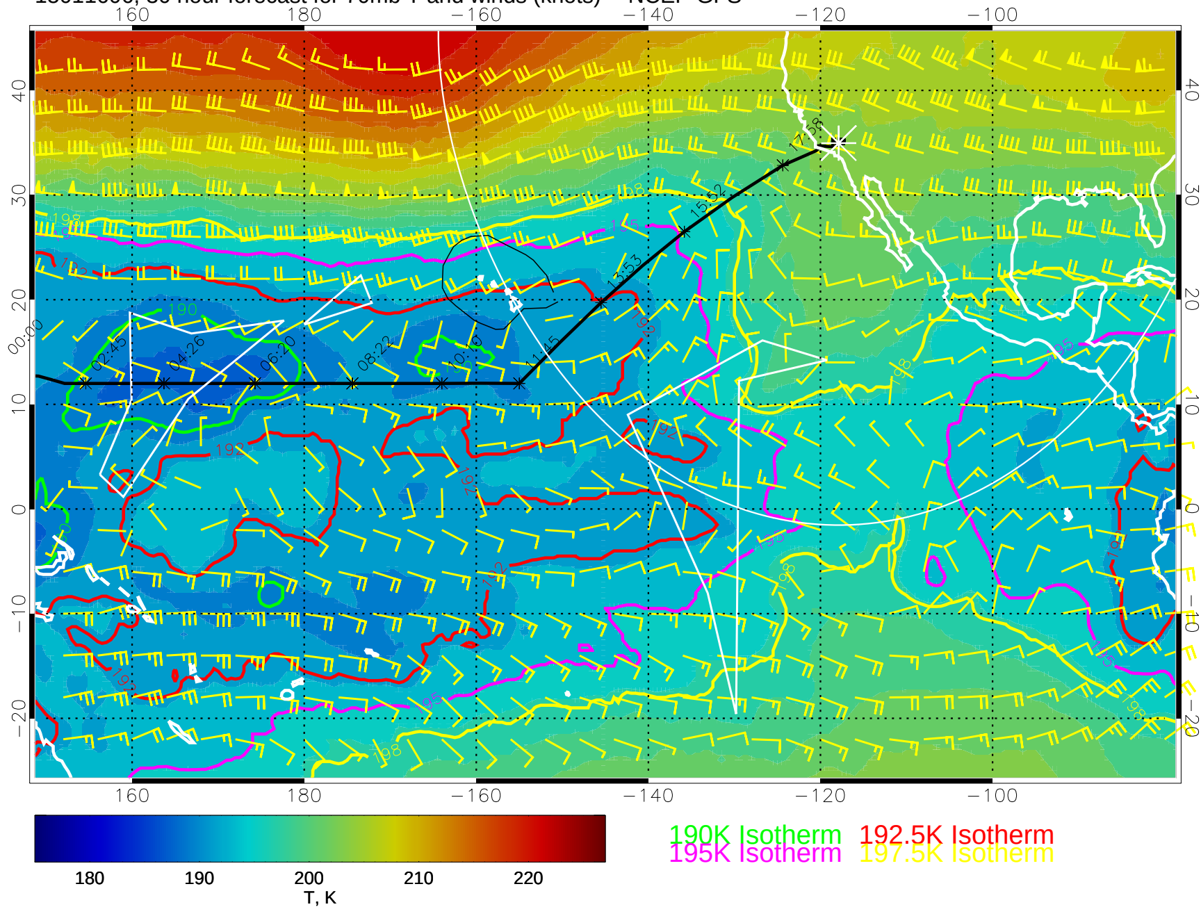
15011606, 30 hour forecast for 70mb T and winds (knots) -- NCEP GFS
