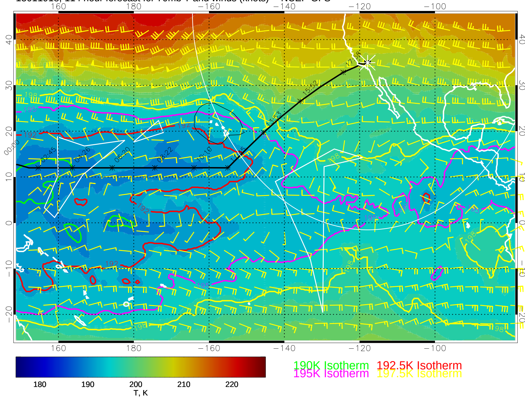
15011918, 114 hour forecast for 70mb T and winds (knots) -- NCEP GFS
