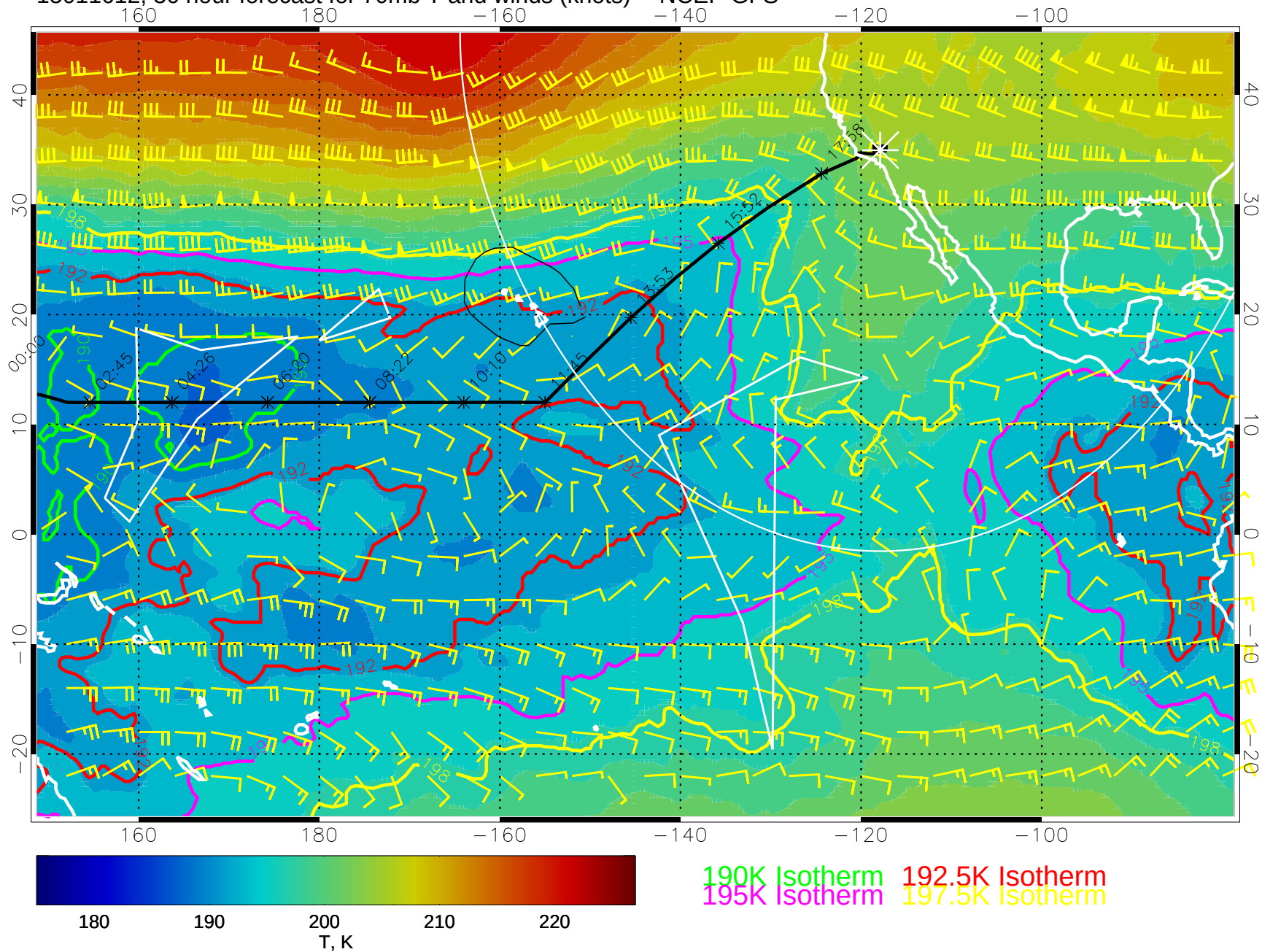
15011612, 36 hour forecast for 70mb T and winds (knots) -- NCEP GFS
