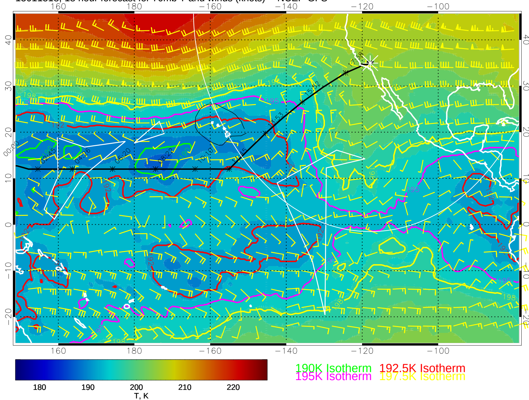
15011518, 18 hour forecast for 70mb T and winds (knots) -- NCEP GFS
