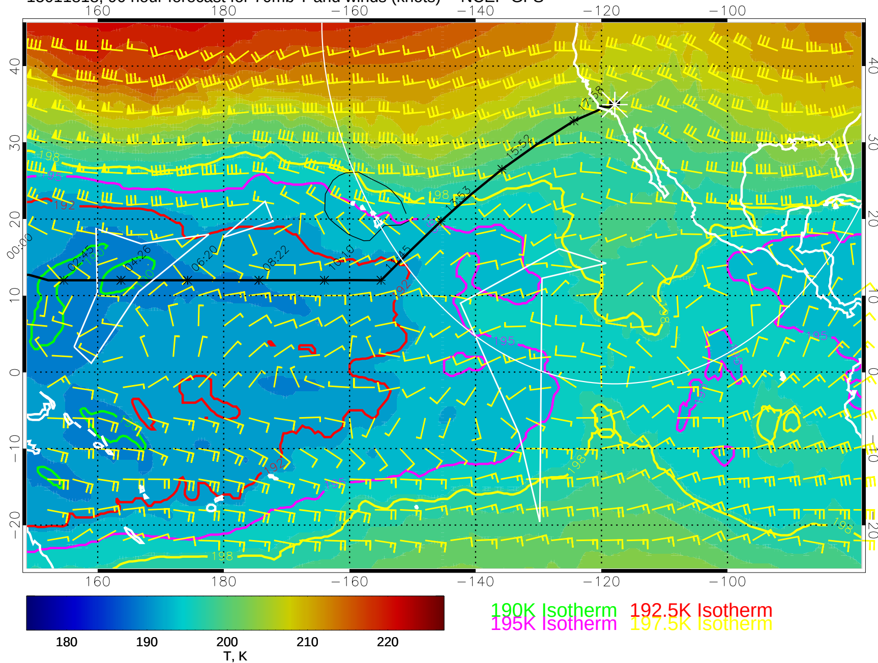
15011818, 90 hour forecast for 70mb T and winds (knots) -- NCEP GFS
