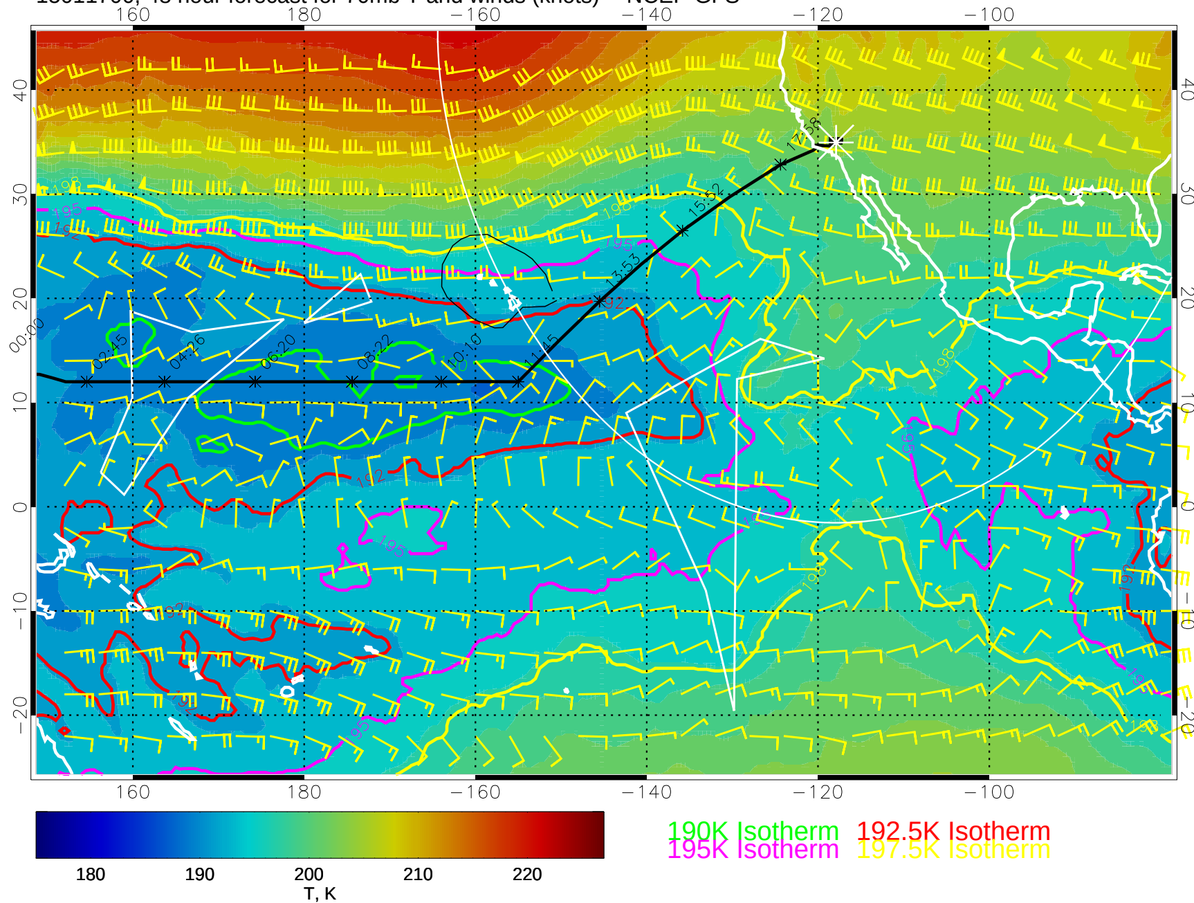
15011700, 48 hour forecast for 70mb T and winds (knots) -- NCEP GFS
