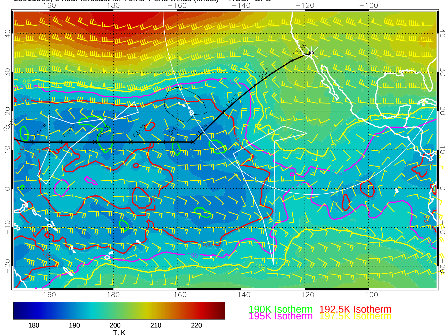
15011506, 6 hour forecast for 70mb T and winds (knots) -- NCEP GFS
