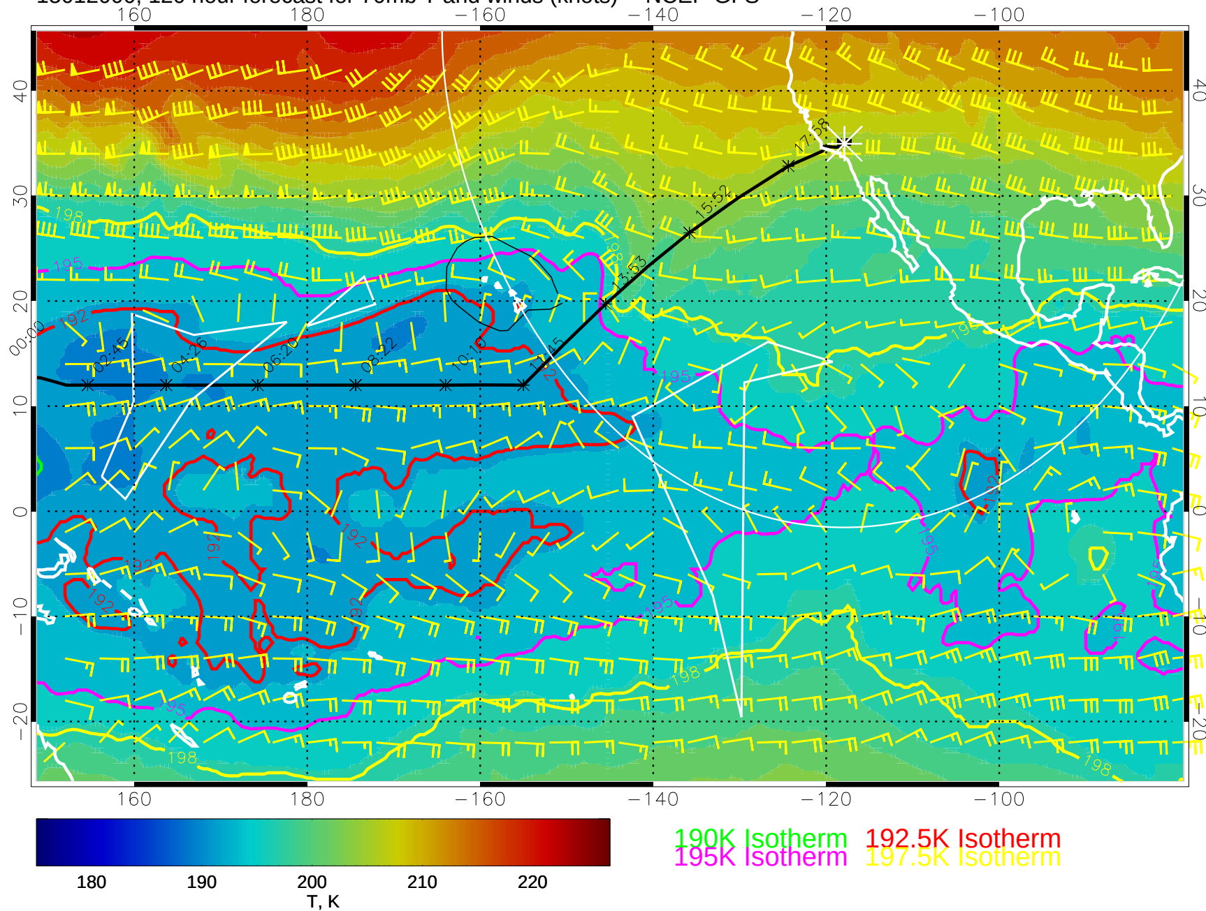
15012000, 120 hour forecast for 70mb T and winds (knots) -- NCEP GFS
