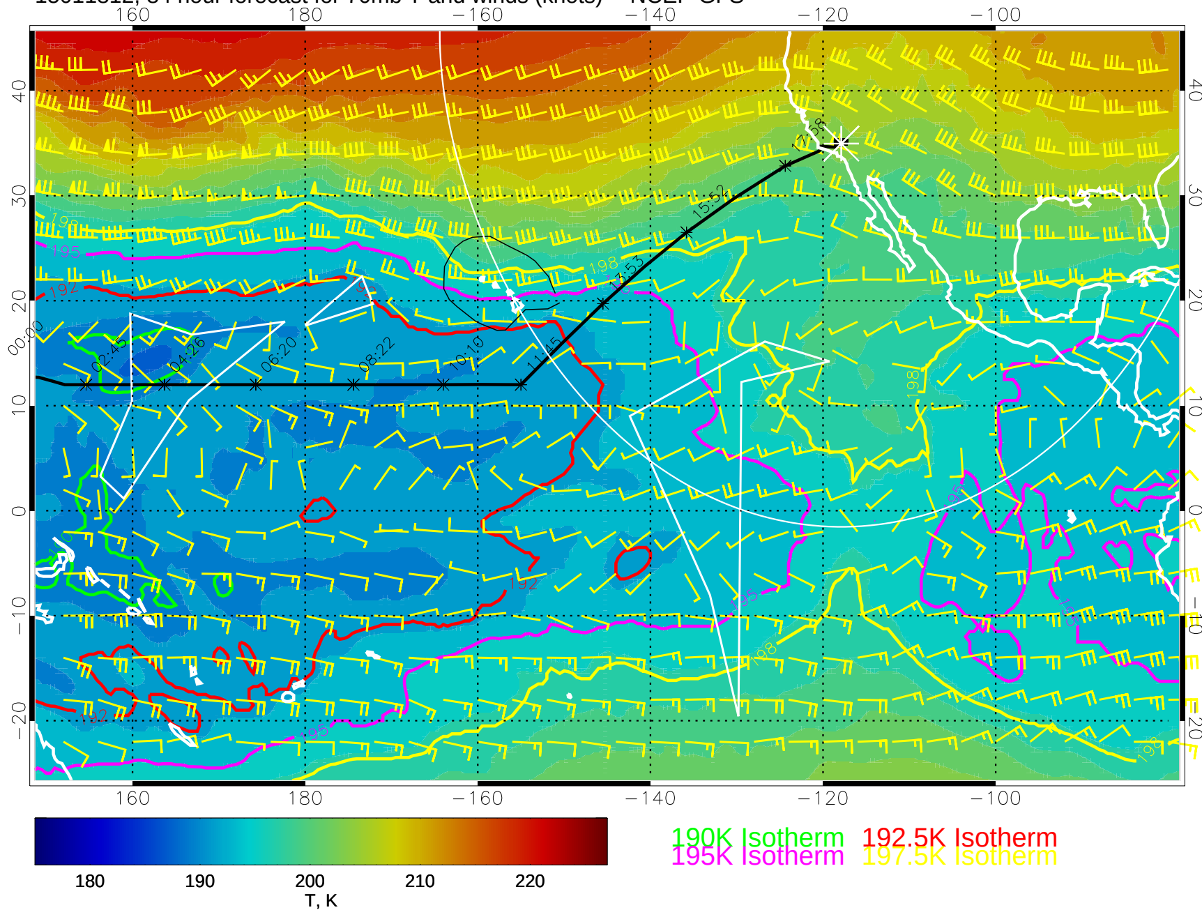
15011812, 84 hour forecast for 70mb T and winds (knots) -- NCEP GFS
