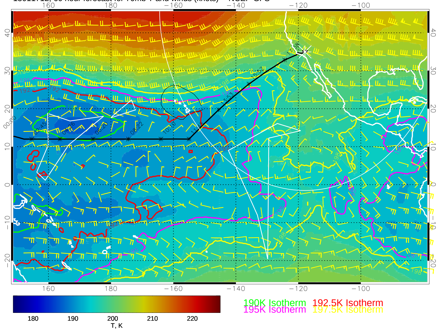
15011712, 60 hour forecast for 70mb T and winds (knots) -- NCEP GFS
