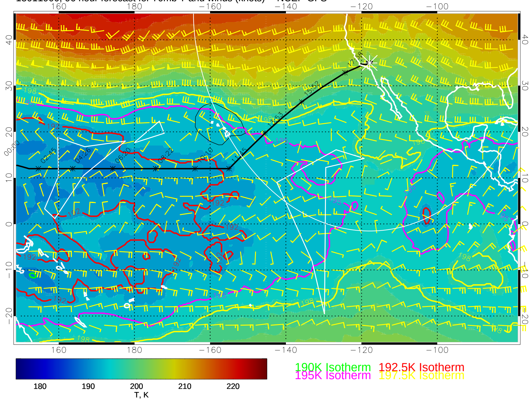
15011900, 96 hour forecast for 70mb T and winds (knots) -- NCEP GFS
