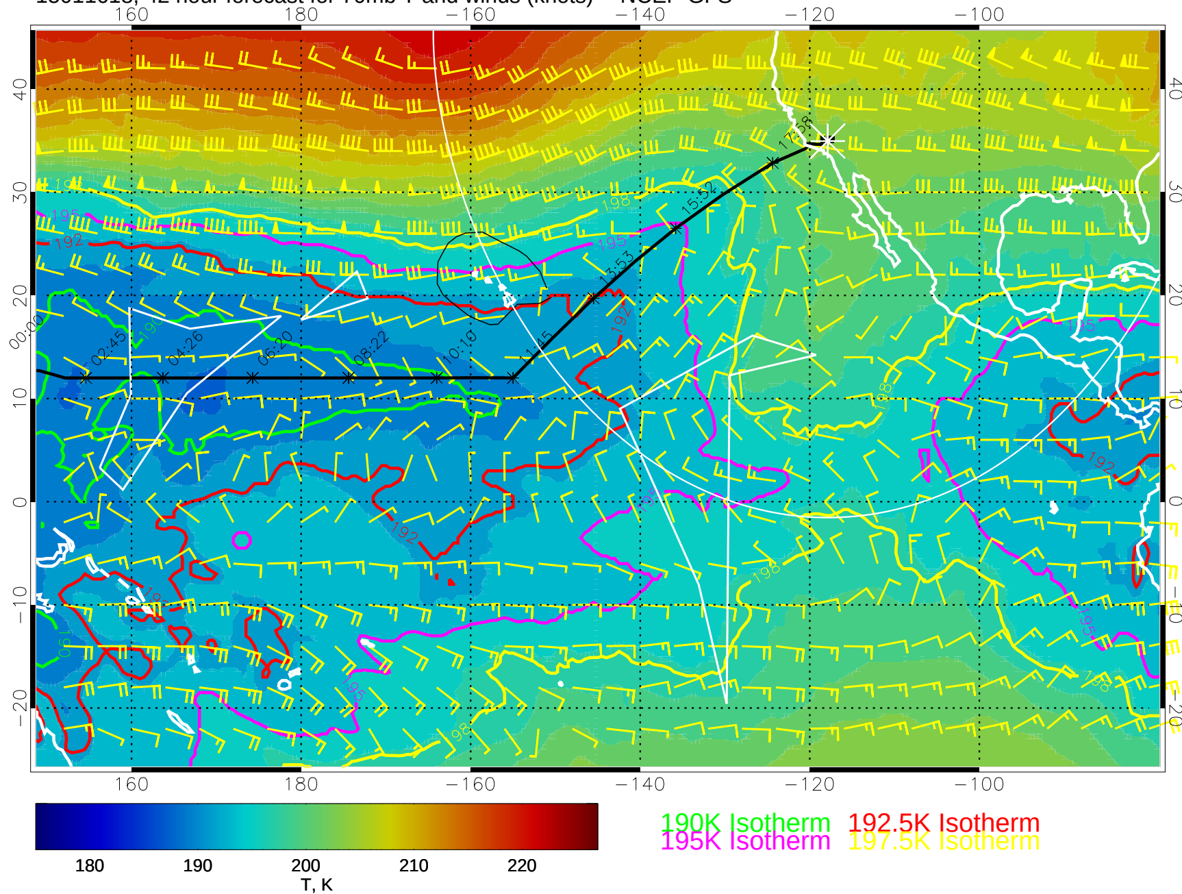
15011618, 42 hour forecast for 70mb T and winds (knots) -- NCEP GFS
