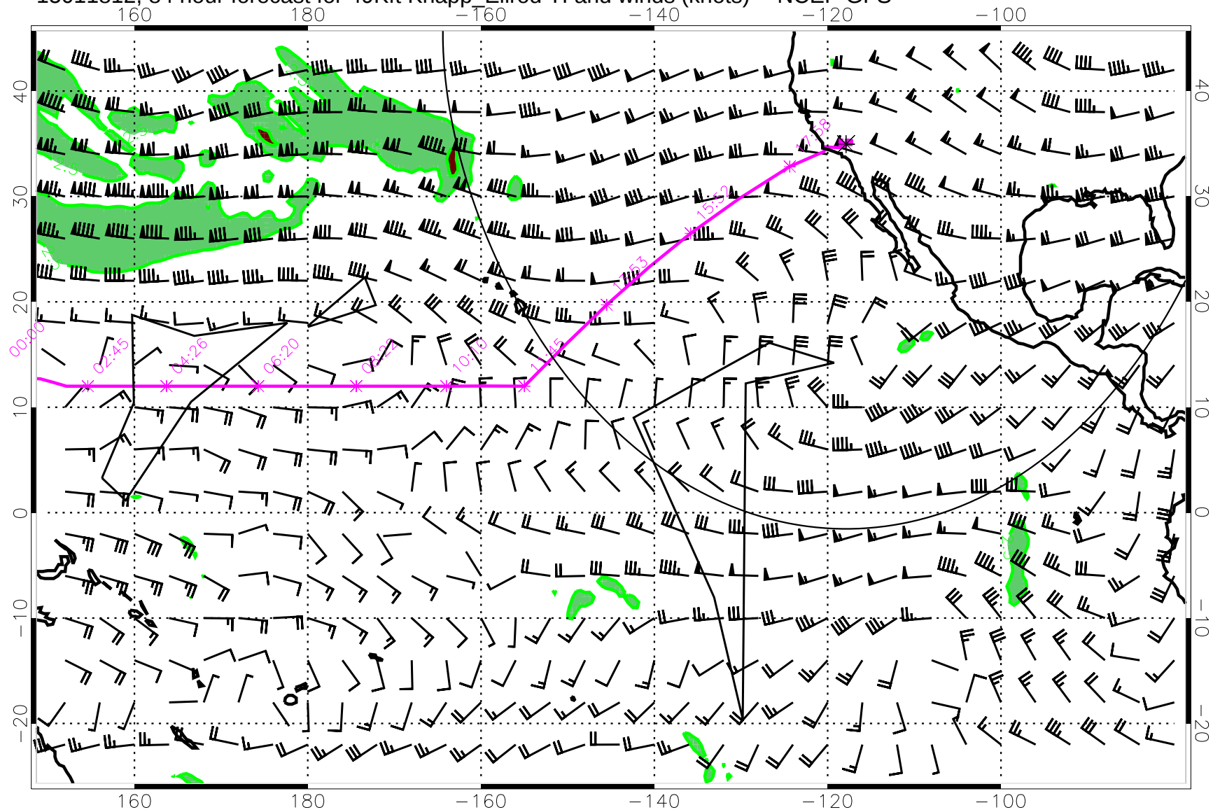
15011812, 84 hour forecast for 49Kft Knapp_Ellrod TI and winds (knots) -- NCEP GFS
