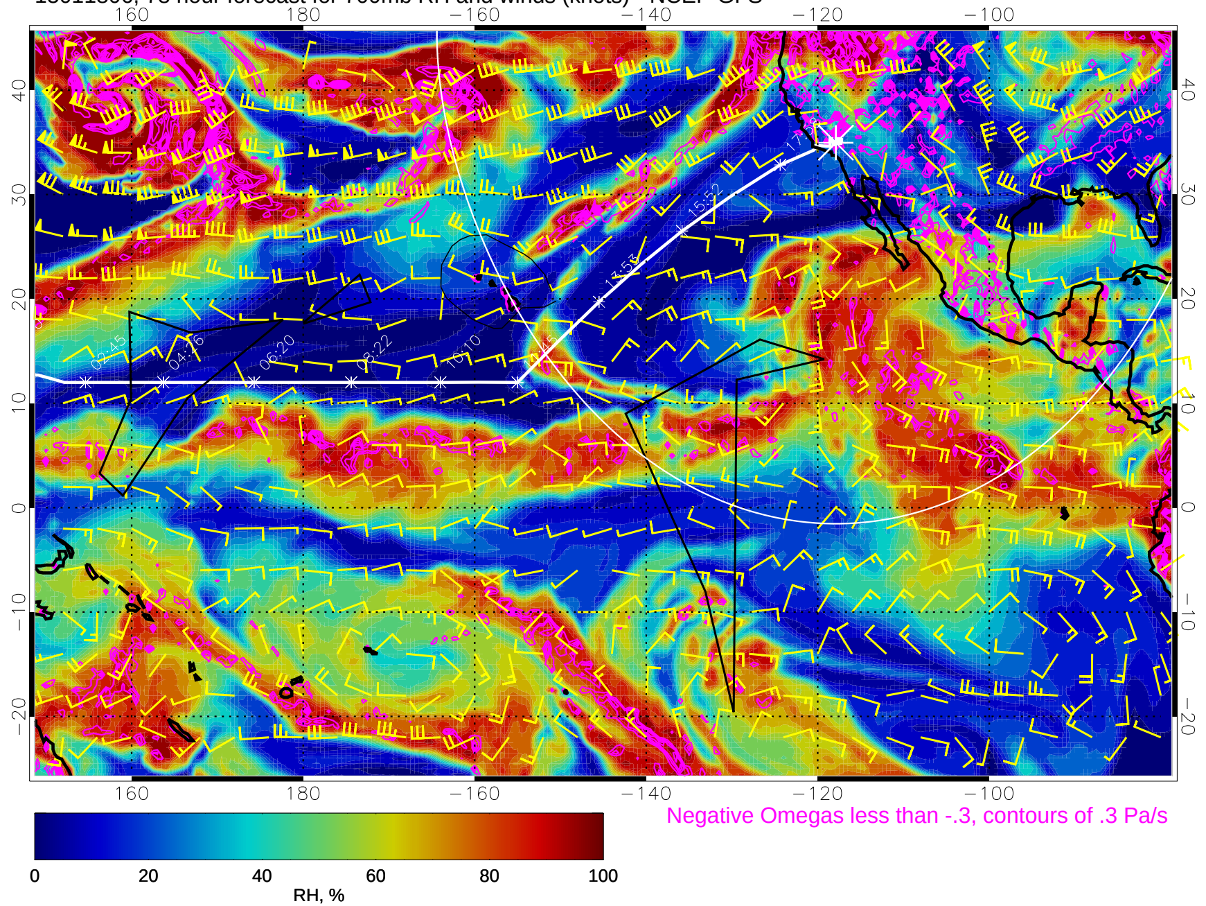
15011806, 78 hour forecast for 700mb RH and winds (knots) - NCEP GFS
