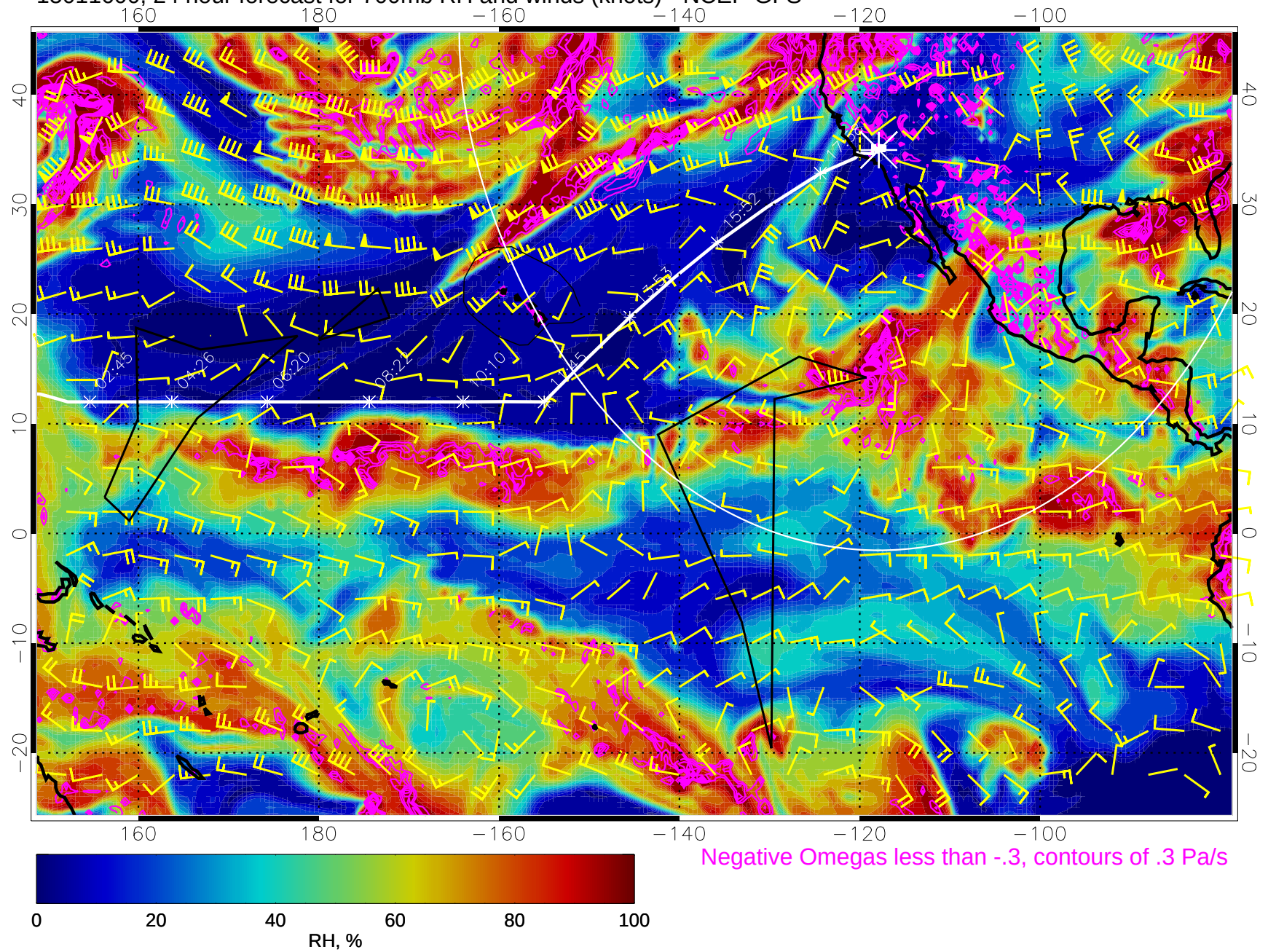
15011600, 24 hour forecast for 700mb RH and winds (knots) - NCEP GFS
