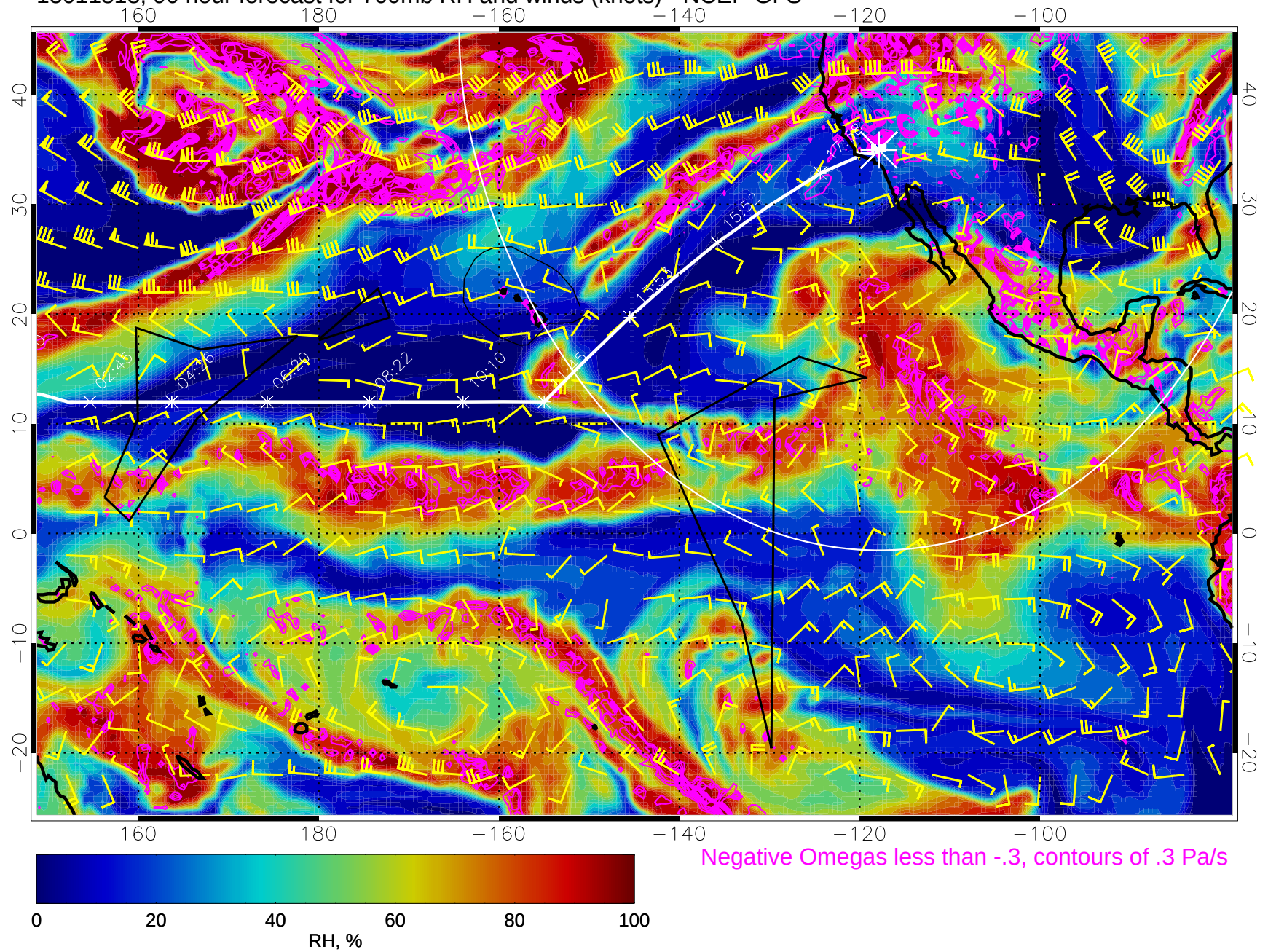
15011818, 90 hour forecast for 700mb RH and winds (knots) - NCEP GFS
