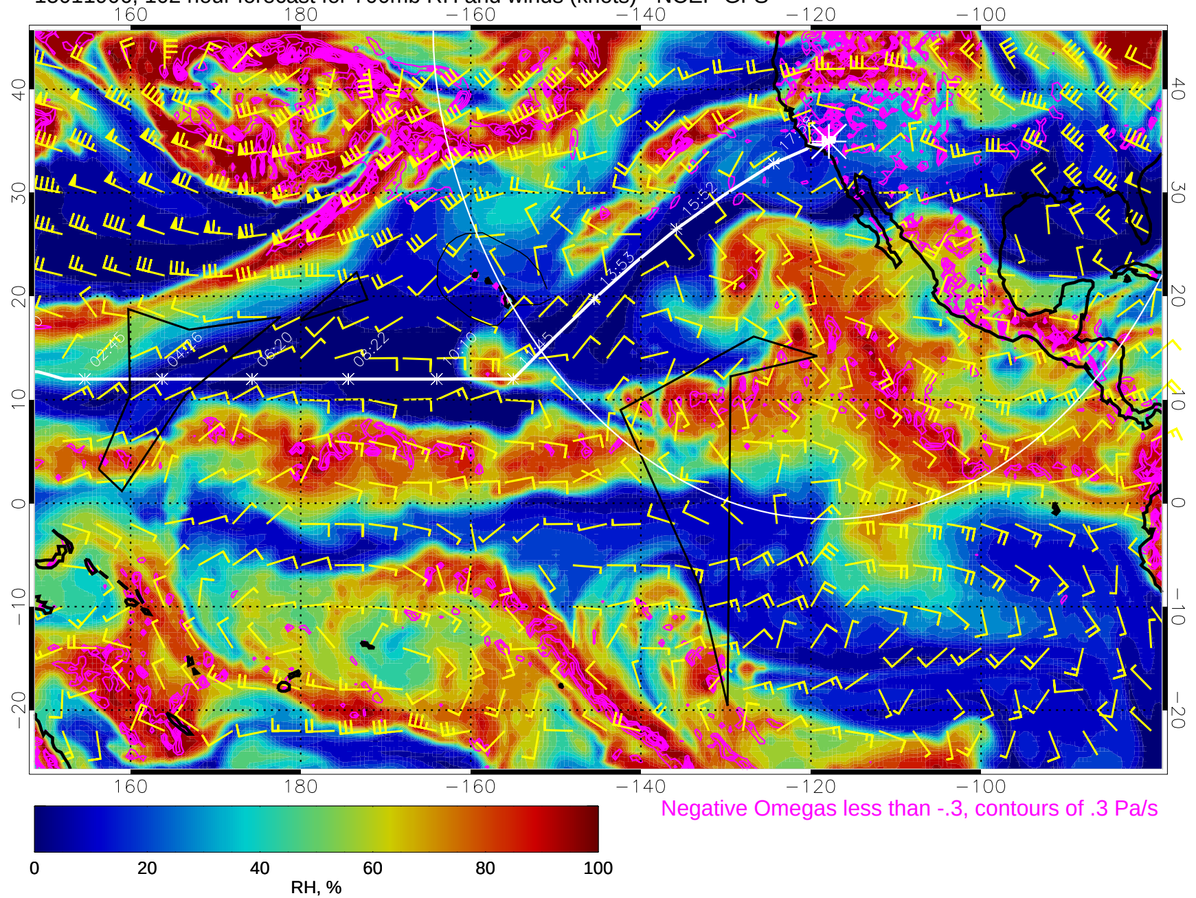
15011906, 102 hour forecast for 700mb RH and winds (knots) - NCEP GFS
