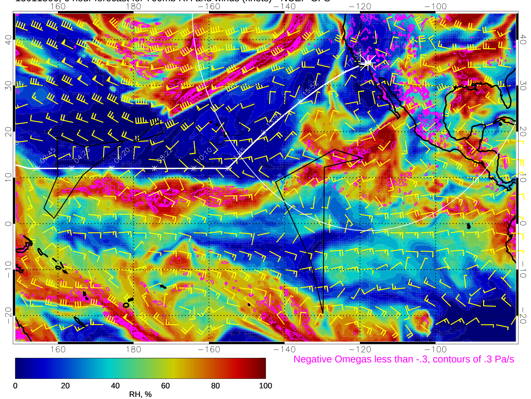
15011506, 6 hour forecast for 700mb RH and winds (knots) - NCEP GFS
