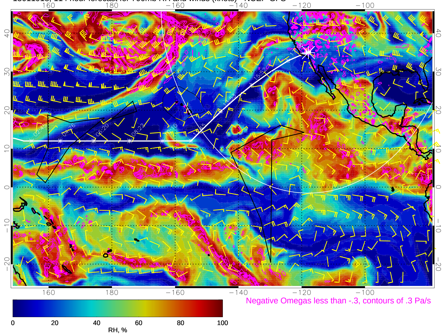
15011918, 114 hour forecast for 700mb RH and winds (knots) - NCEP GFS
