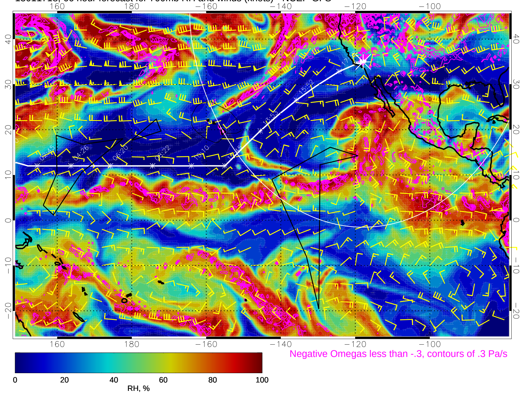
15011718, 66 hour forecast for 700mb RH and winds (knots) - NCEP GFS
