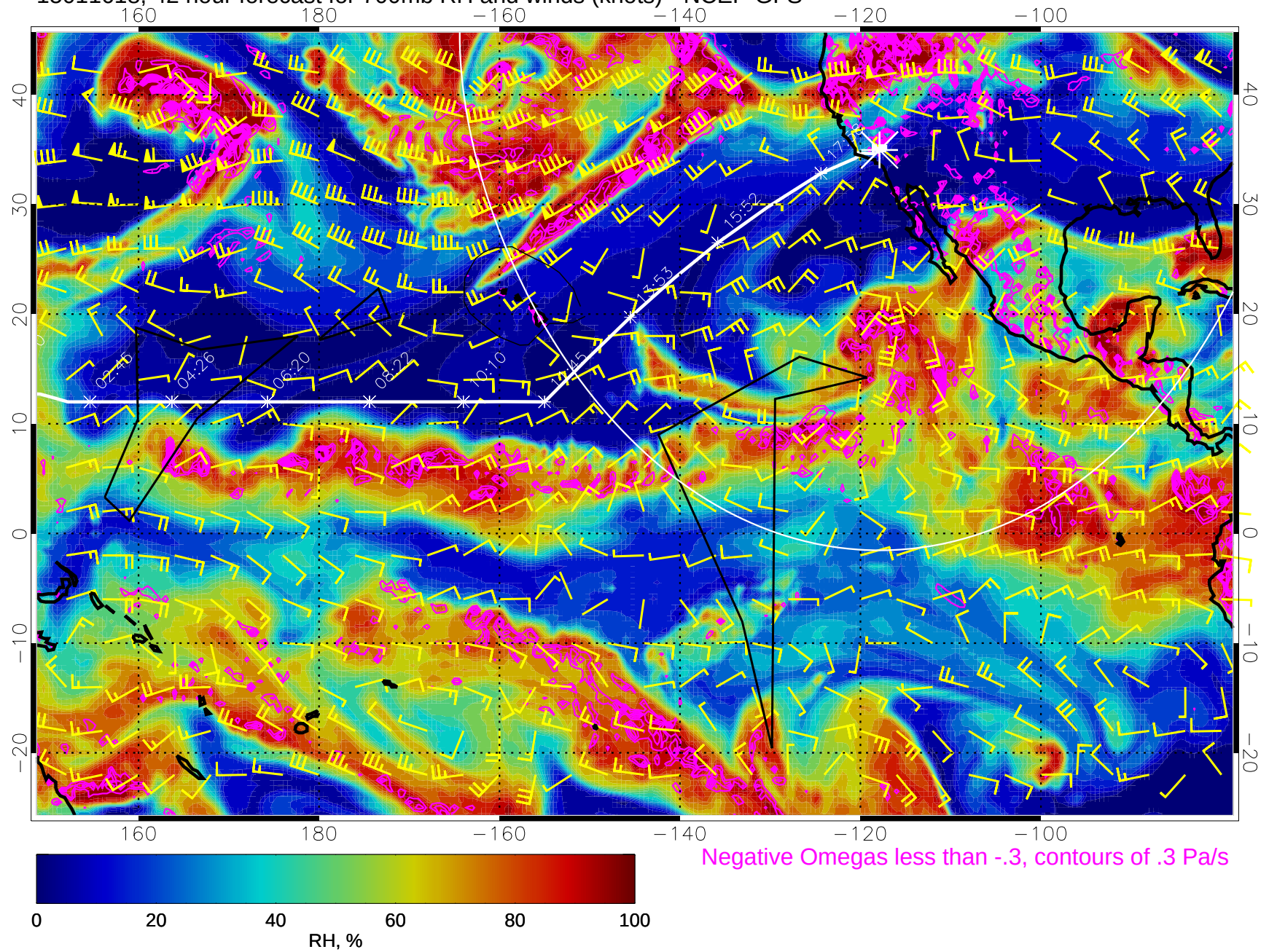
15011618, 42 hour forecast for 700mb RH and winds (knots) - NCEP GFS
