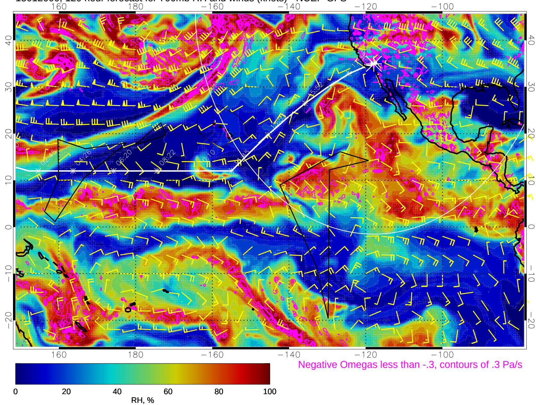
15012000, 120 hour forecast for 700mb RH and winds (knots) - NCEP GFS
