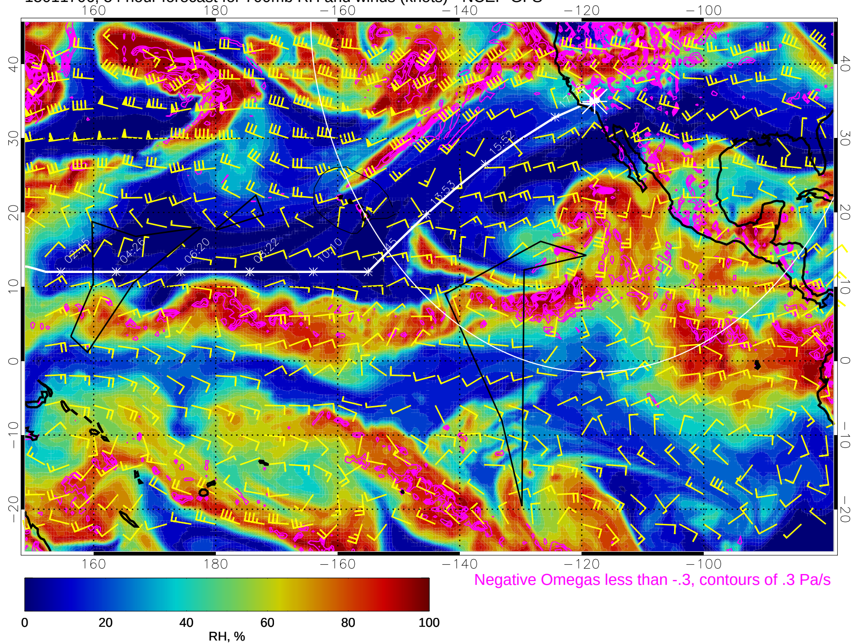
15011706, 54 hour forecast for 700mb RH and winds (knots) - NCEP GFS
