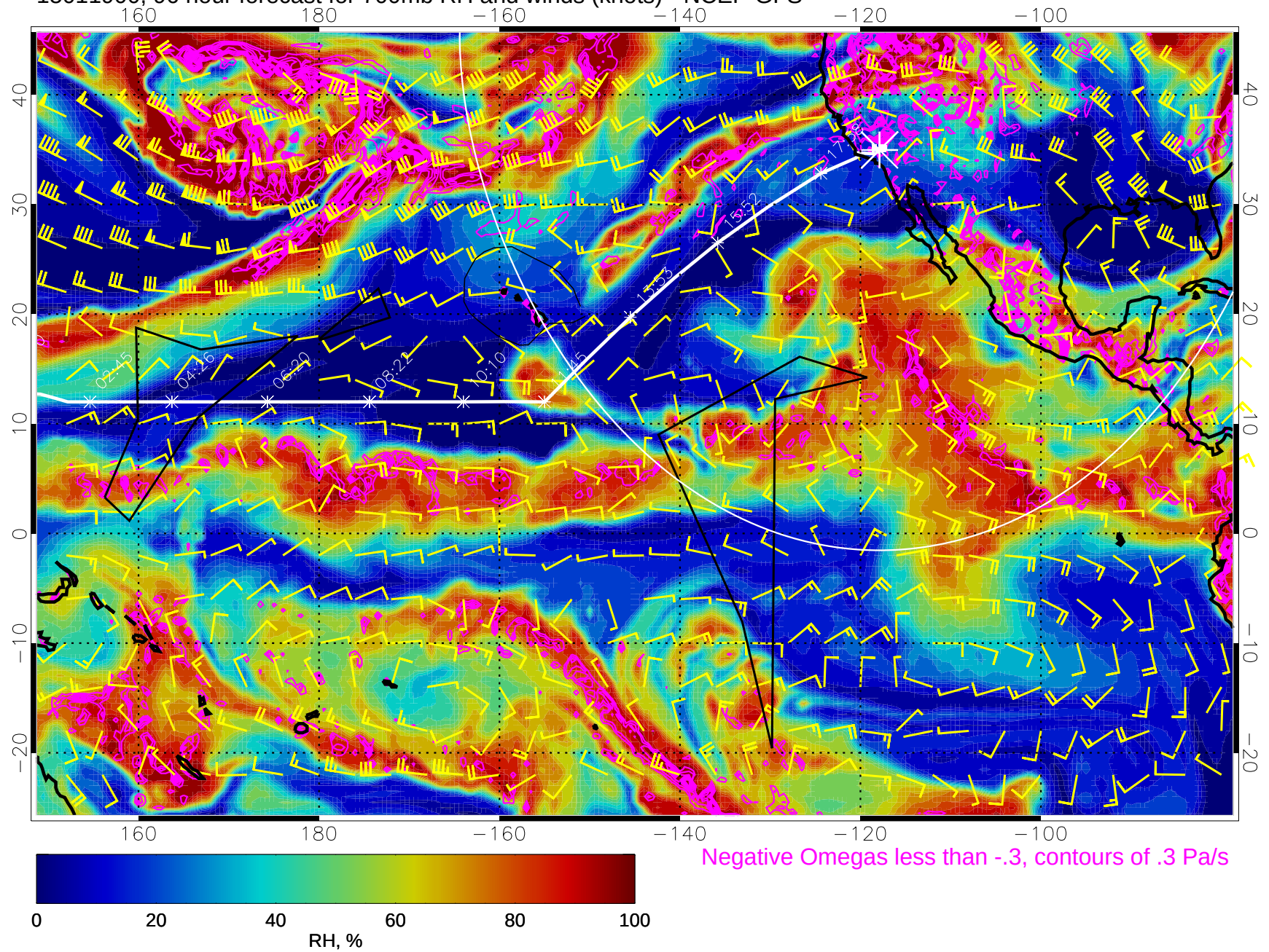
15011900, 96 hour forecast for 700mb RH and winds (knots) - NCEP GFS
