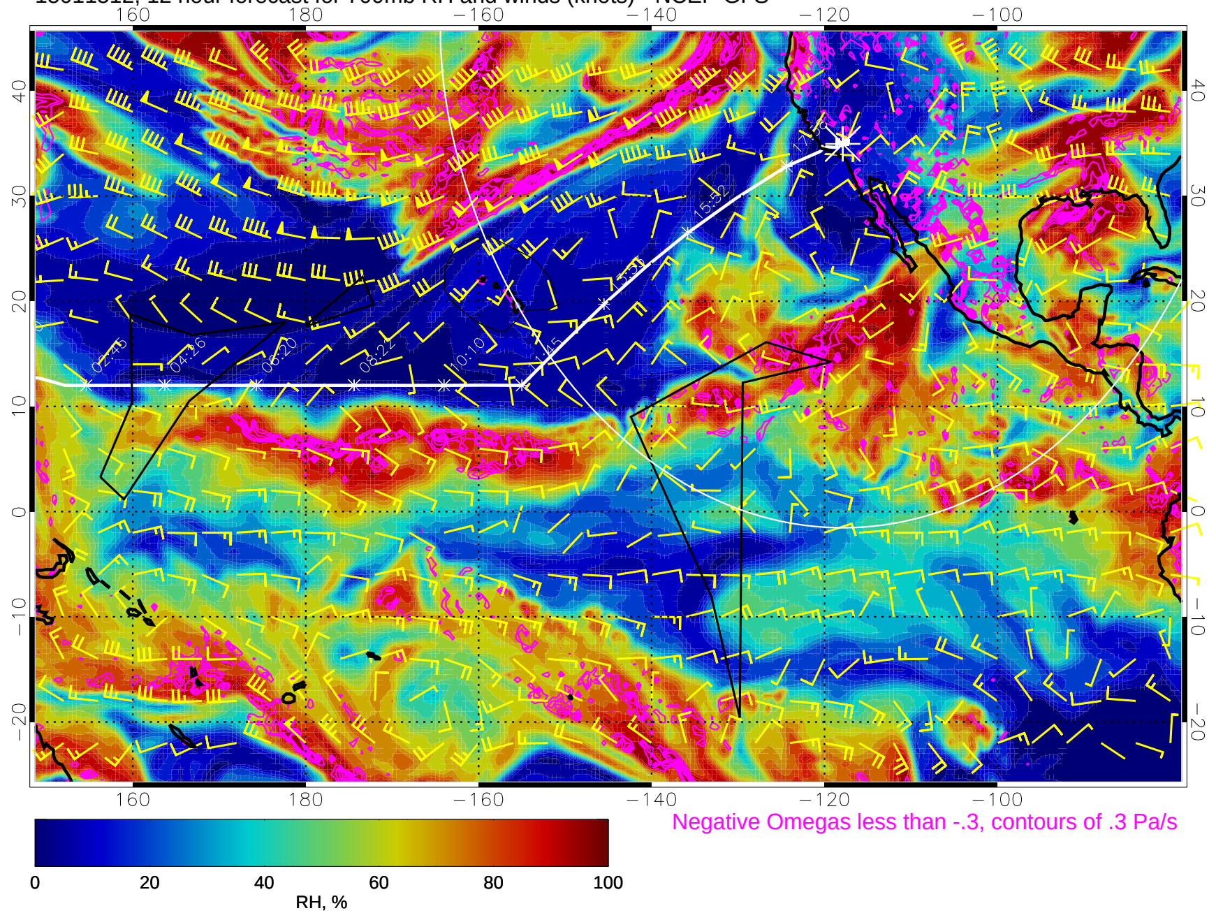
15011512, 12 hour forecast for 700mb RH and winds (knots) - NCEP GFS
