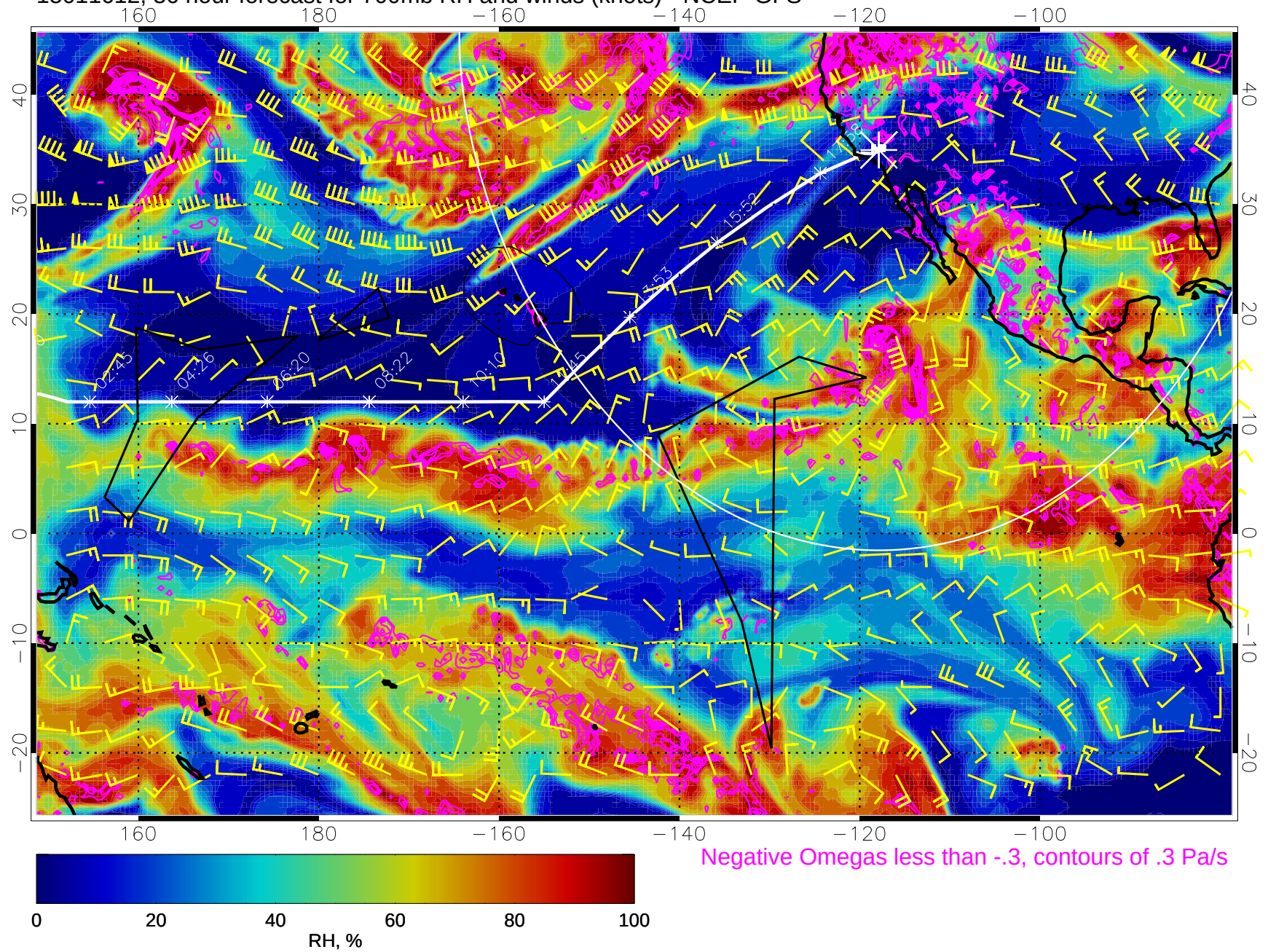
15011612, 36 hour forecast for 700mb RH and winds (knots) - NCEP GFS
