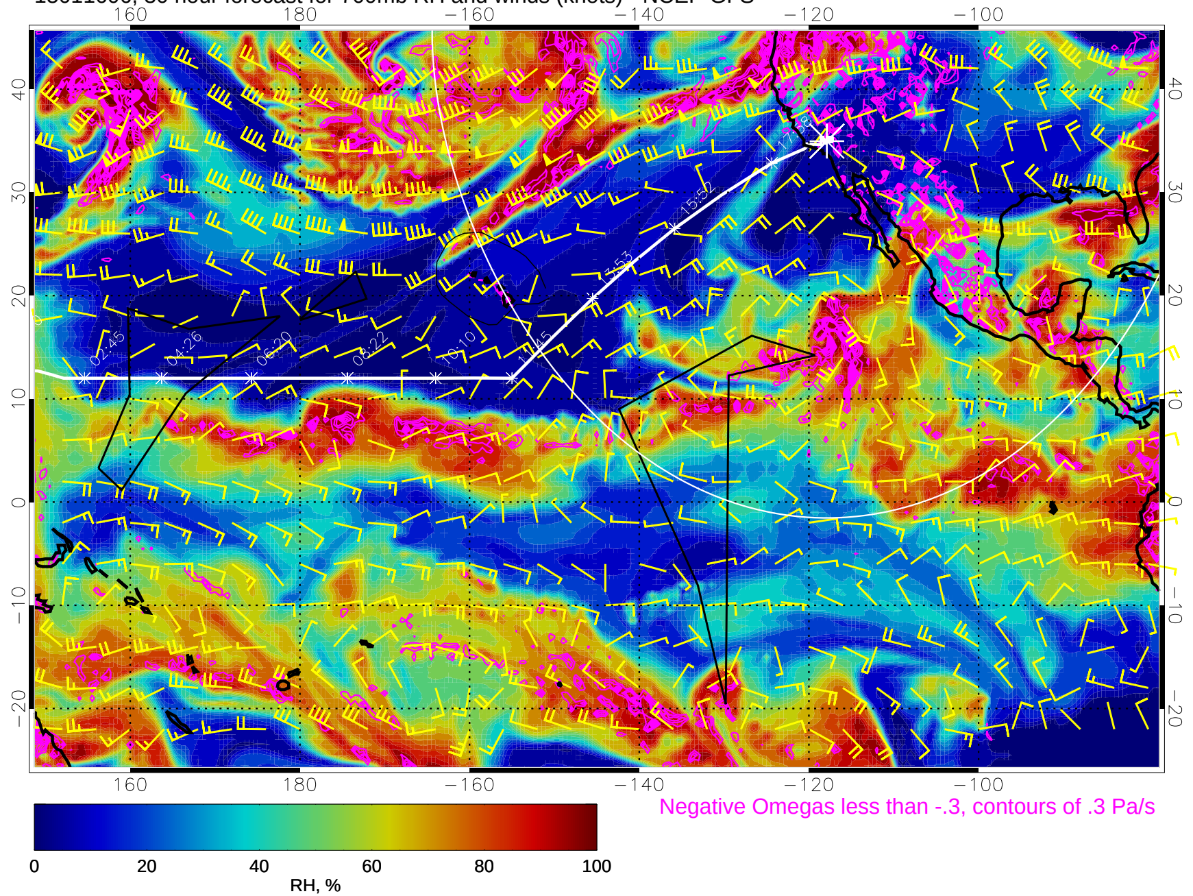
15011606, 30 hour forecast for 700mb RH and winds (knots) - NCEP GFS
