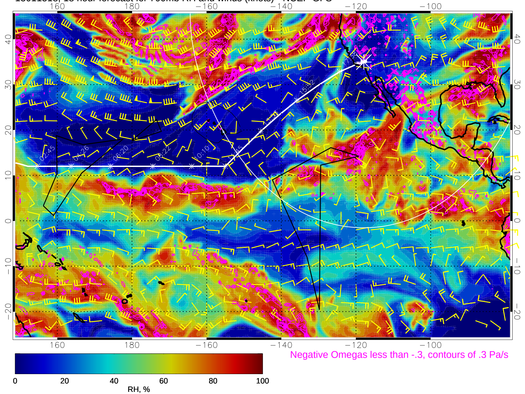
15011518, 18 hour forecast for 700mb RH and winds (knots) - NCEP GFS
