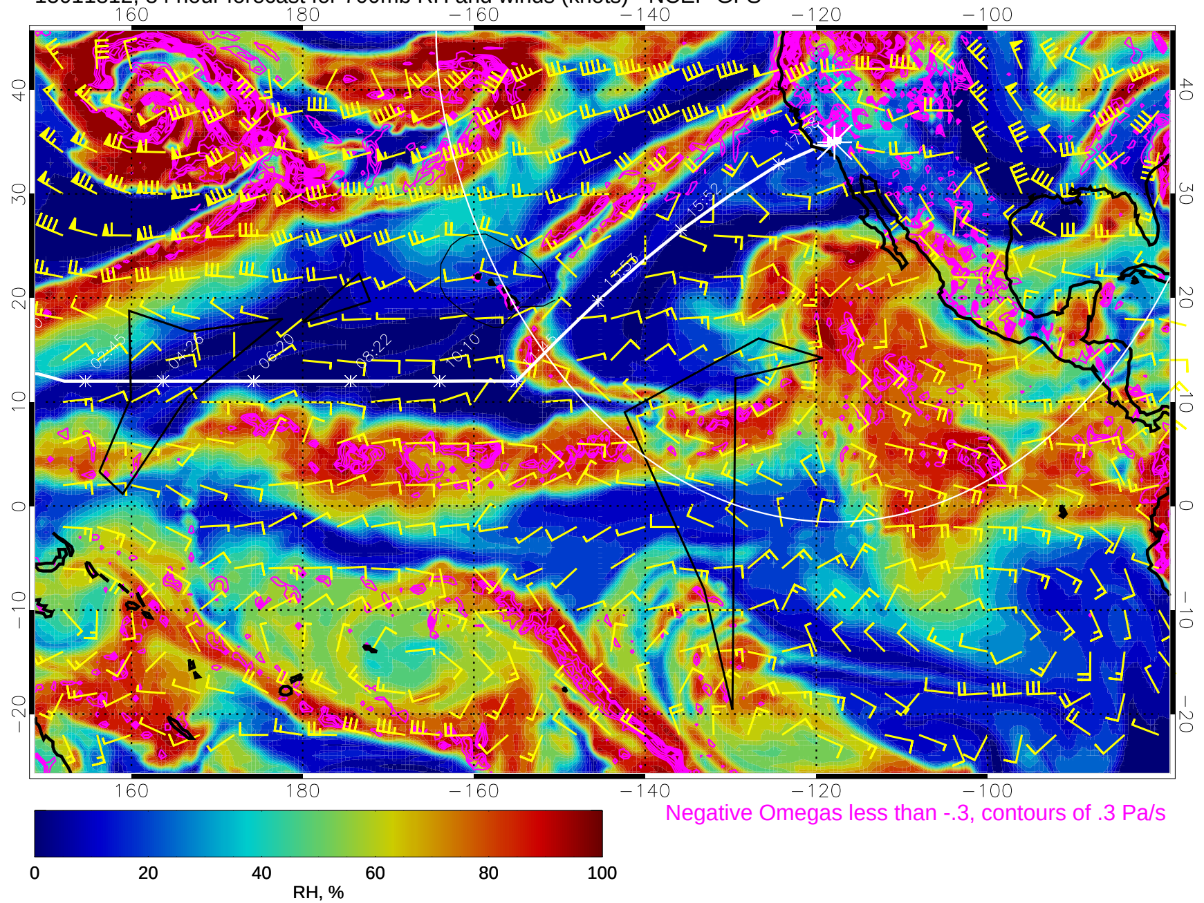
15011812, 84 hour forecast for 700mb RH and winds (knots) - NCEP GFS
