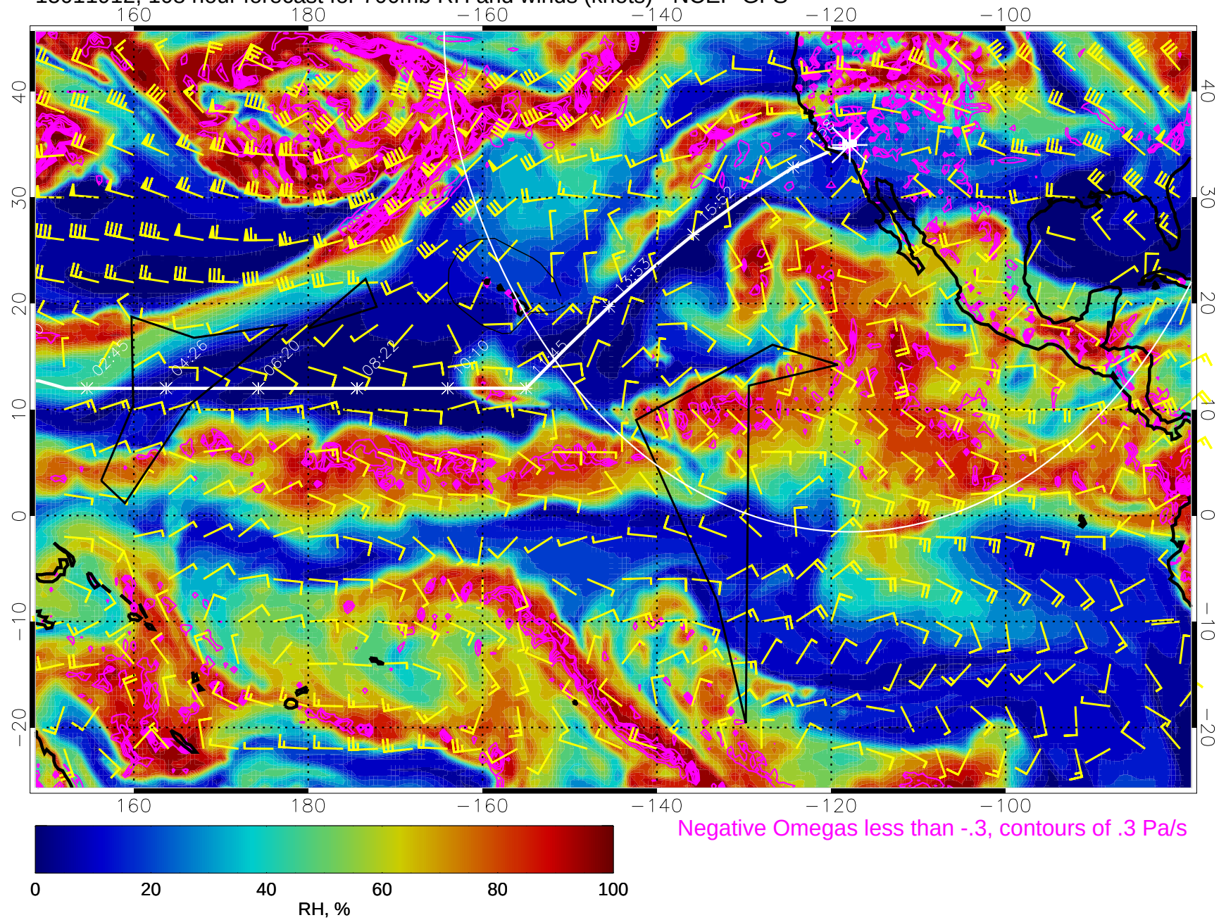
15011912, 108 hour forecast for 700mb RH and winds (knots) - NCEP GFS
