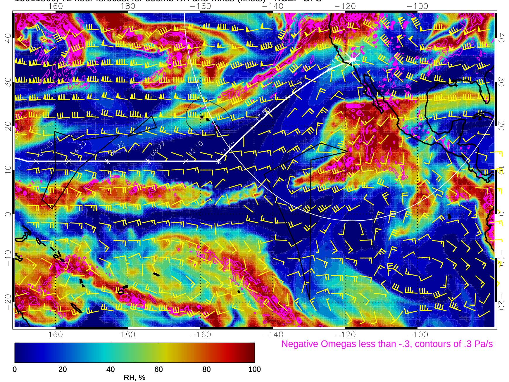
15011800, 72 hour forecast for 500mb RH and winds (knots) - NCEP GFS
