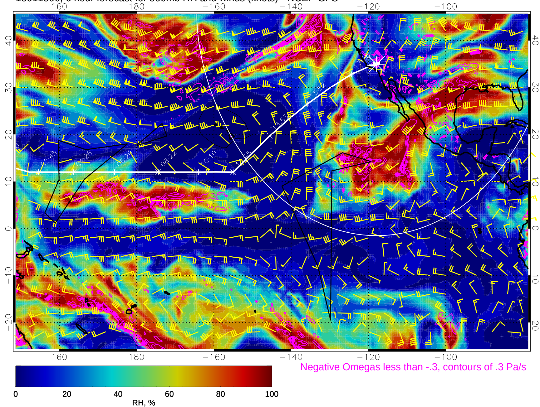
15011506, 6 hour forecast for 500mb RH and winds (knots) - NCEP GFS
