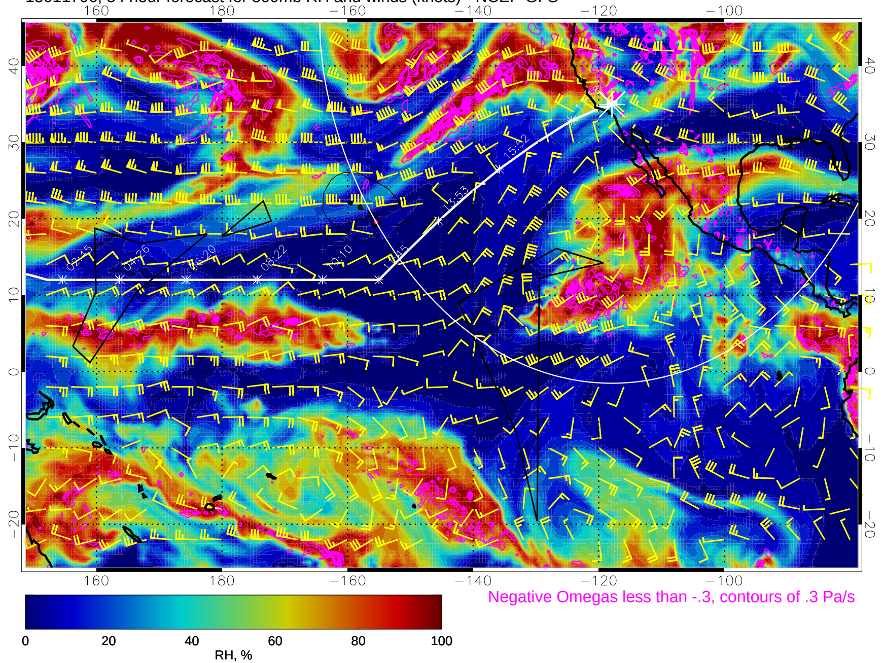
15011706, 54 hour forecast for 500mb RH and winds (knots) - NCEP GFS
