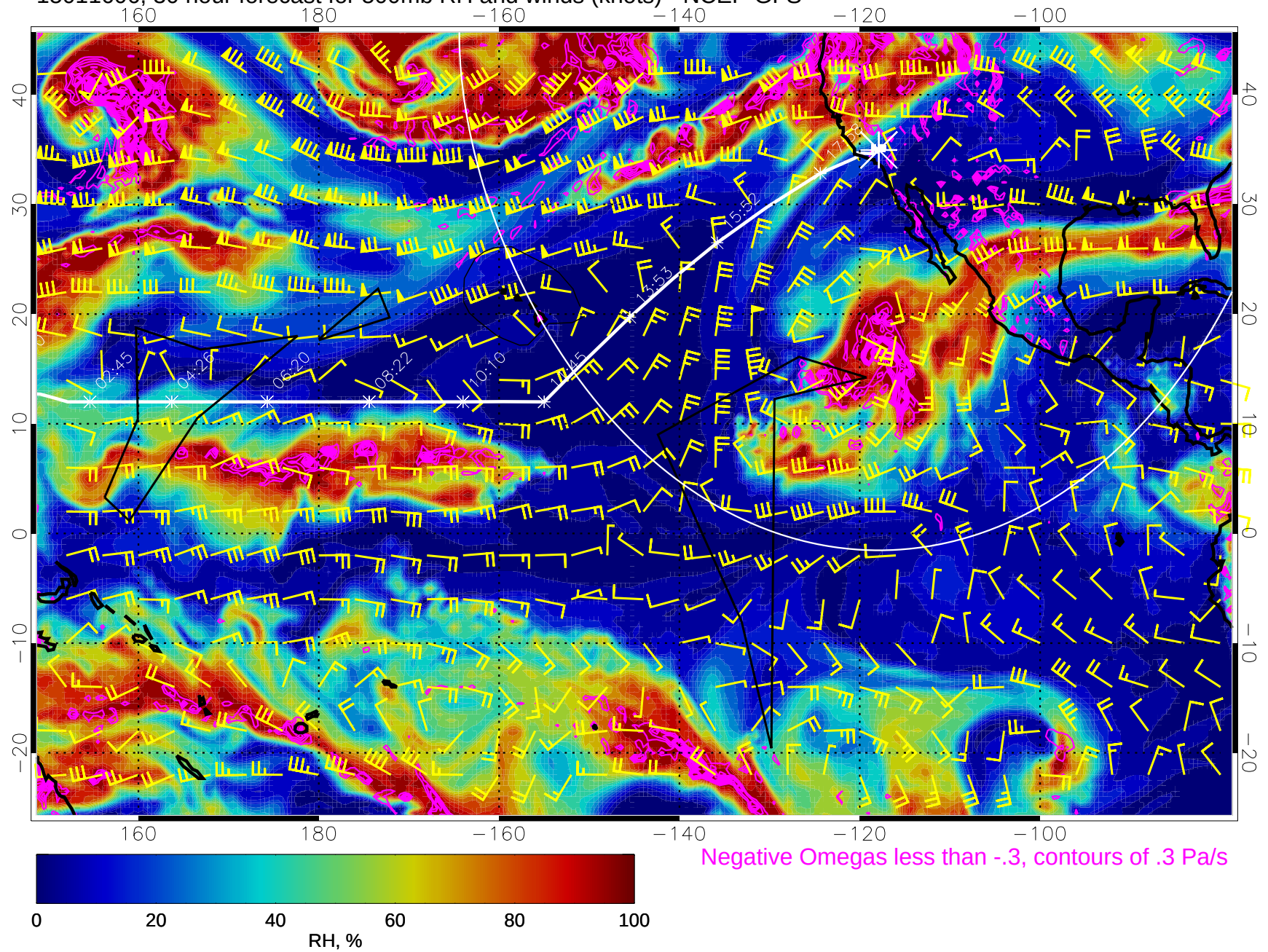
15011606, 30 hour forecast for 500mb RH and winds (knots) - NCEP GFS
