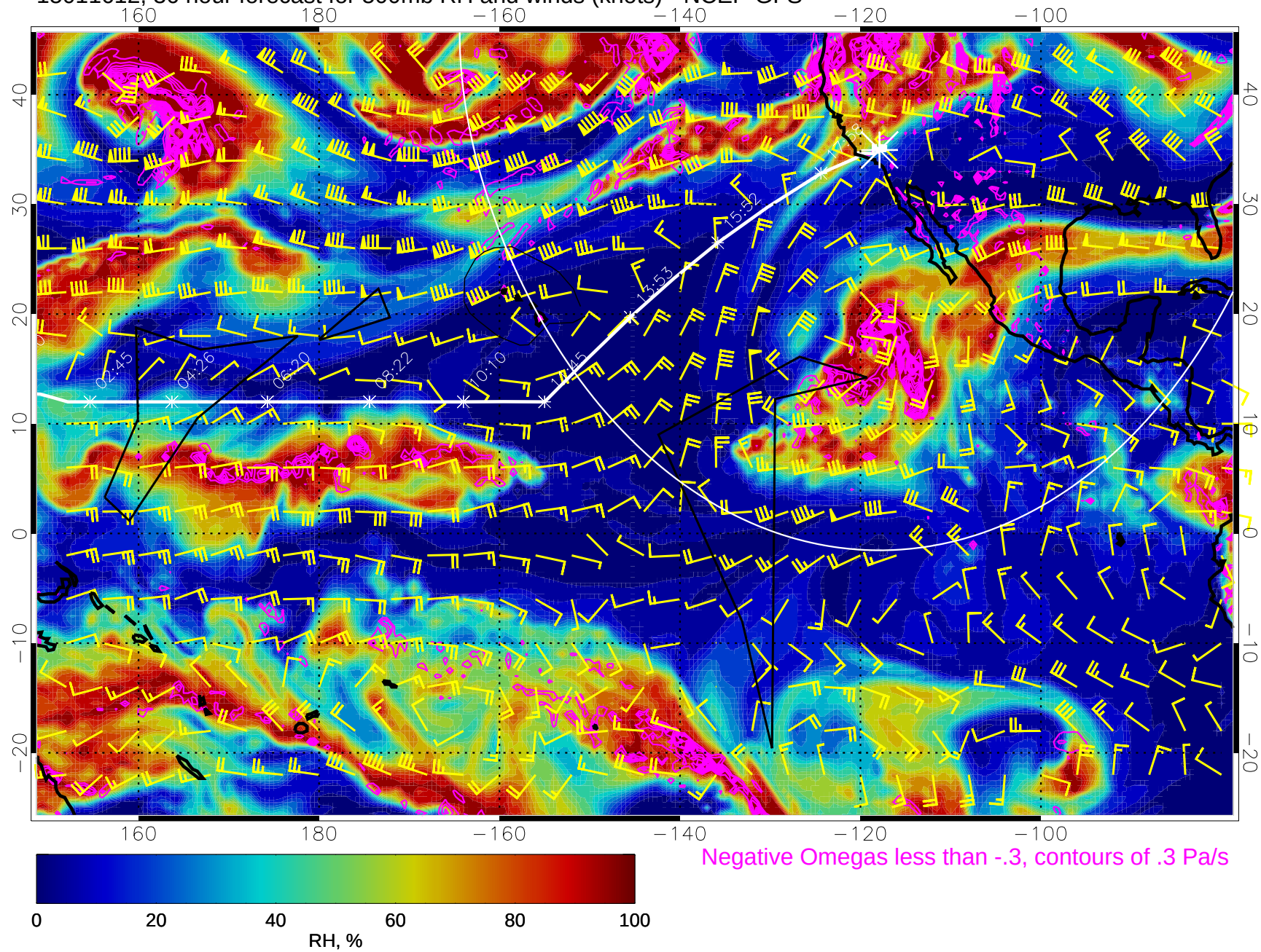
15011612, 36 hour forecast for 500mb RH and winds (knots) - NCEP GFS
