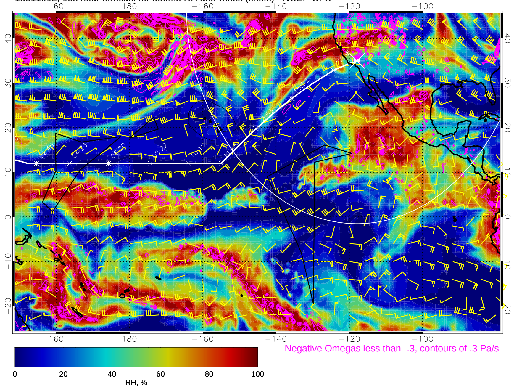
15011912, 108 hour forecast for 500mb RH and winds (knots) - NCEP GFS
