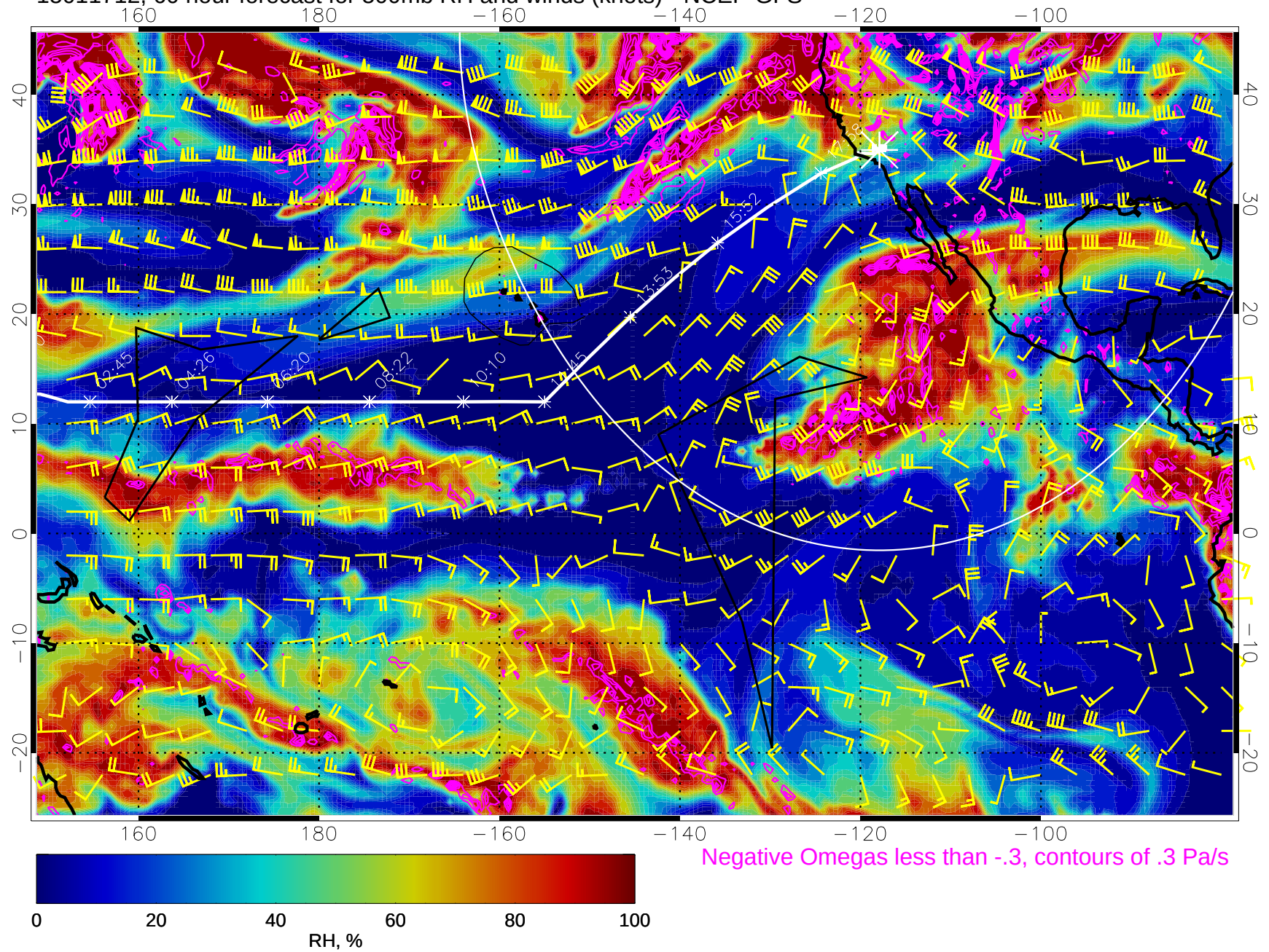
15011712, 60 hour forecast for 500mb RH and winds (knots) - NCEP GFS
