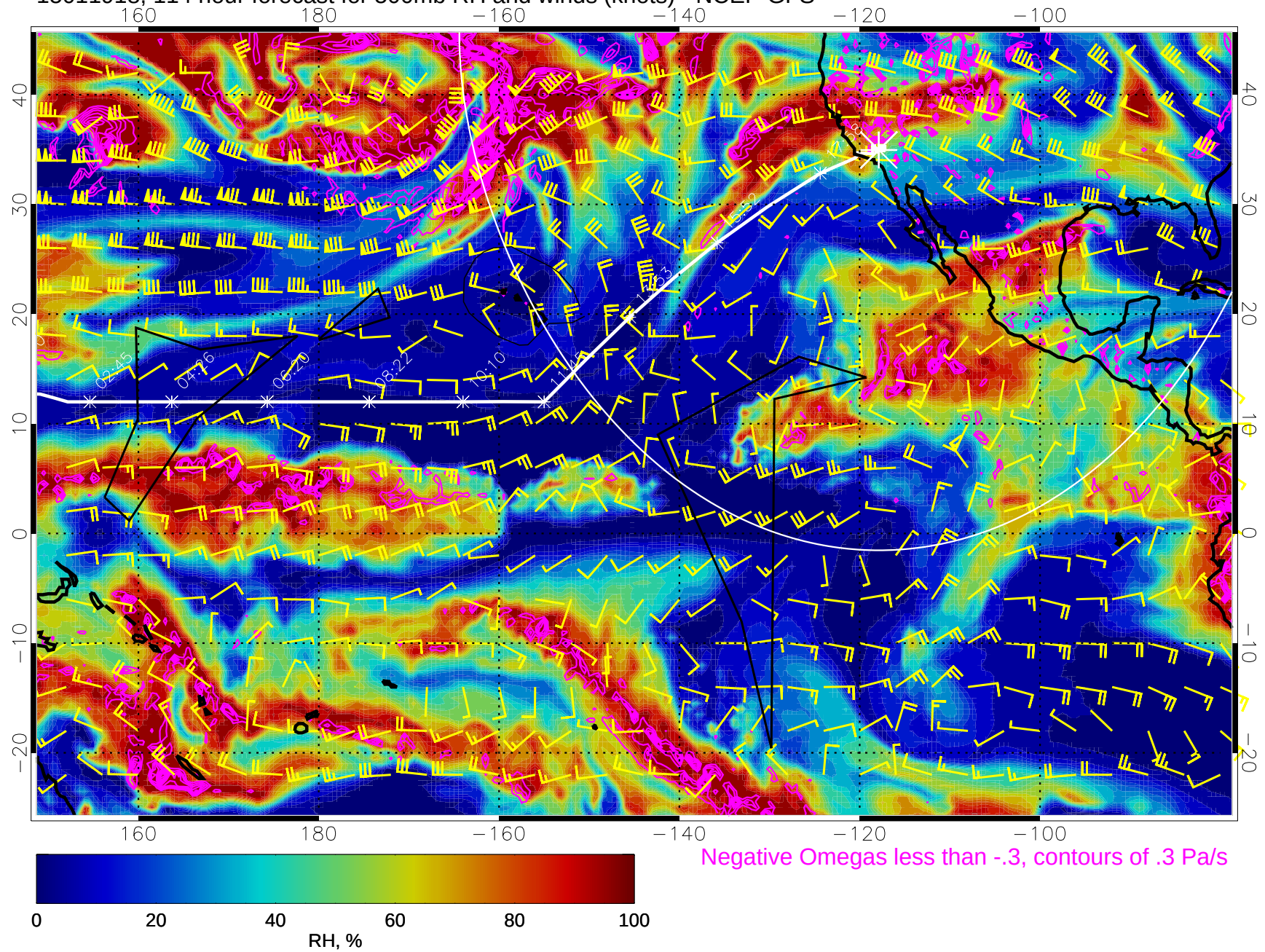
15011918, 114 hour forecast for 500mb RH and winds (knots) - NCEP GFS
