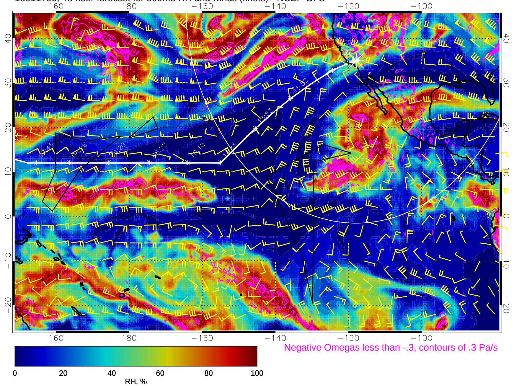
15011700, 48 hour forecast for 500mb RH and winds (knots) - NCEP GFS
