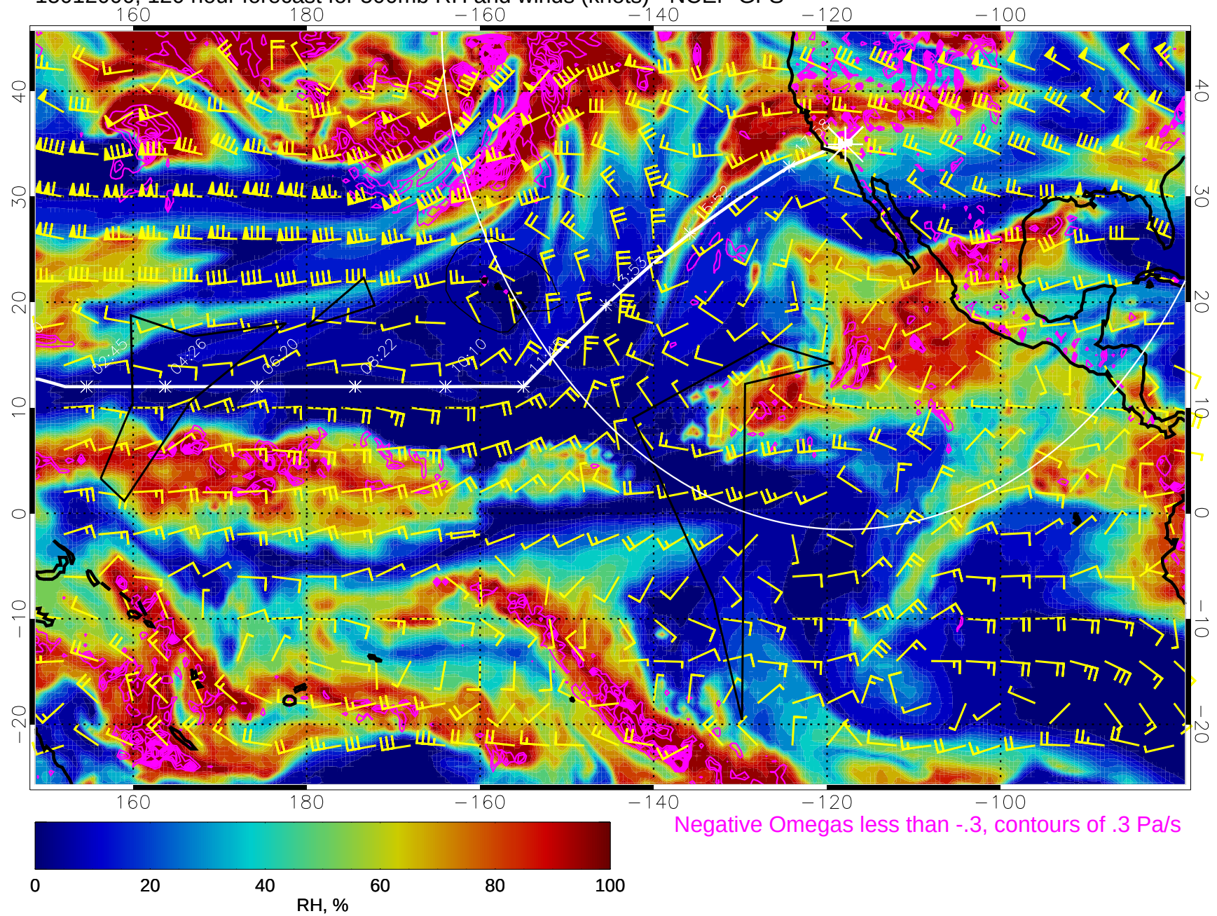
15012000, 120 hour forecast for 500mb RH and winds (knots) - NCEP GFS
