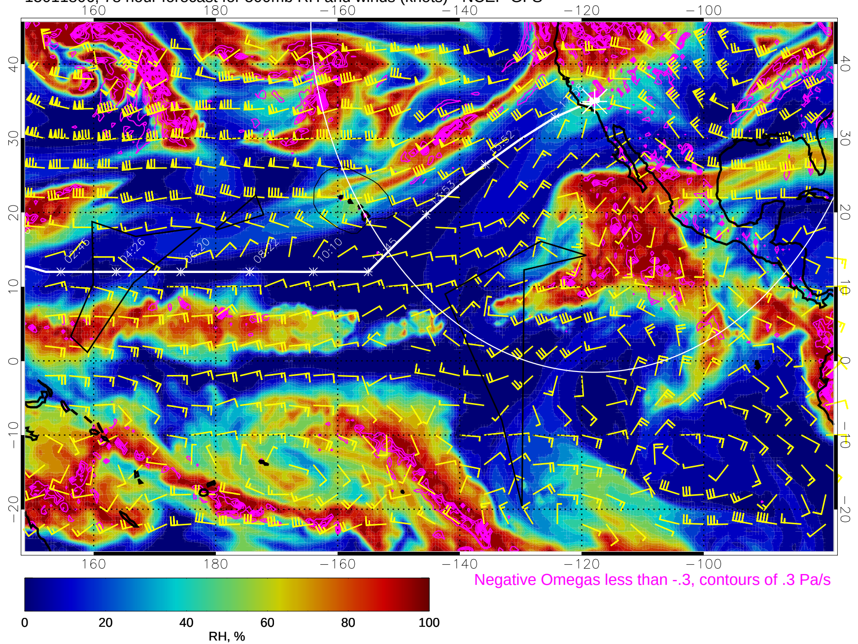
15011806, 78 hour forecast for 500mb RH and winds (knots) - NCEP GFS
