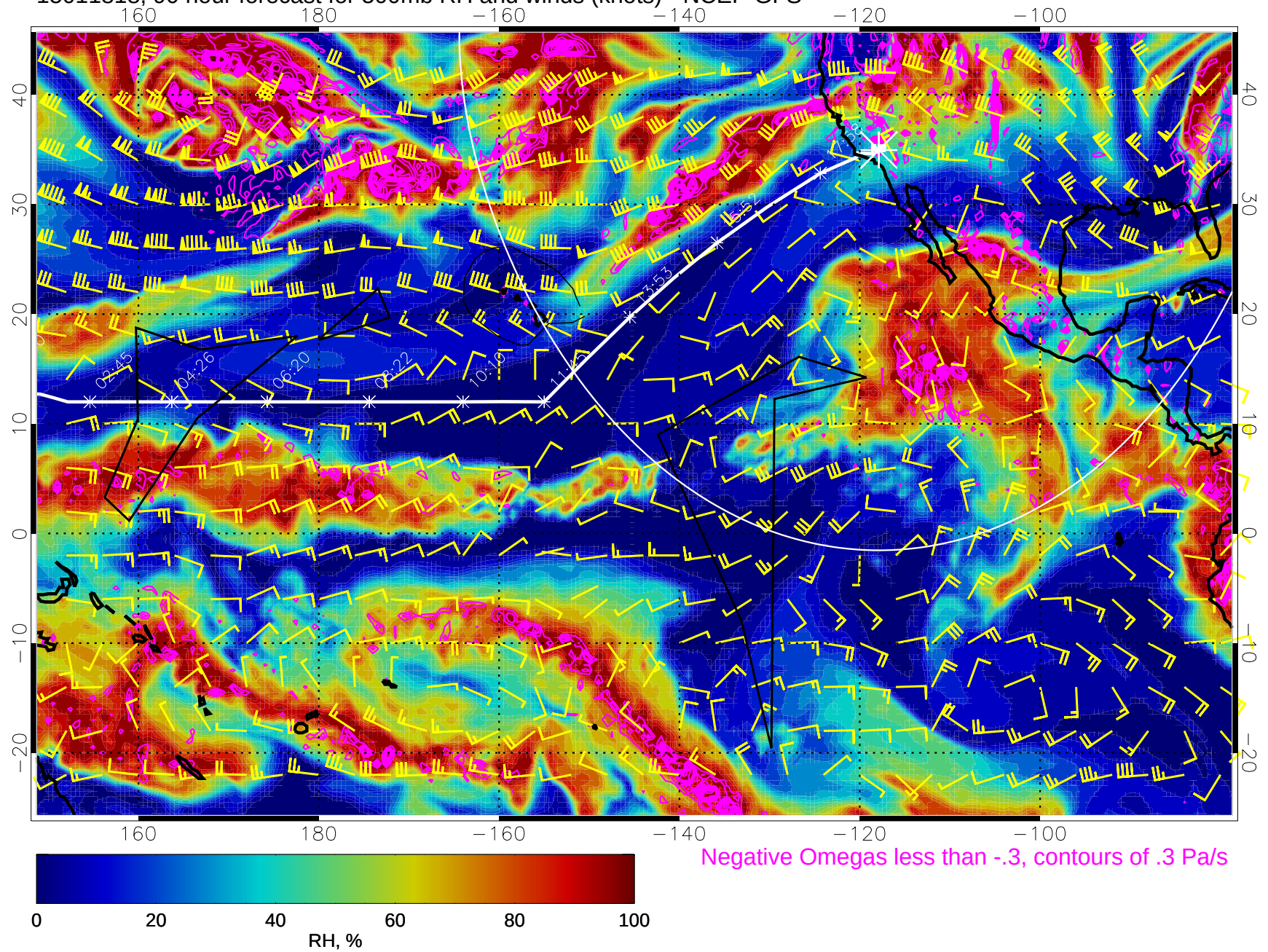
15011818, 90 hour forecast for 500mb RH and winds (knots) - NCEP GFS
