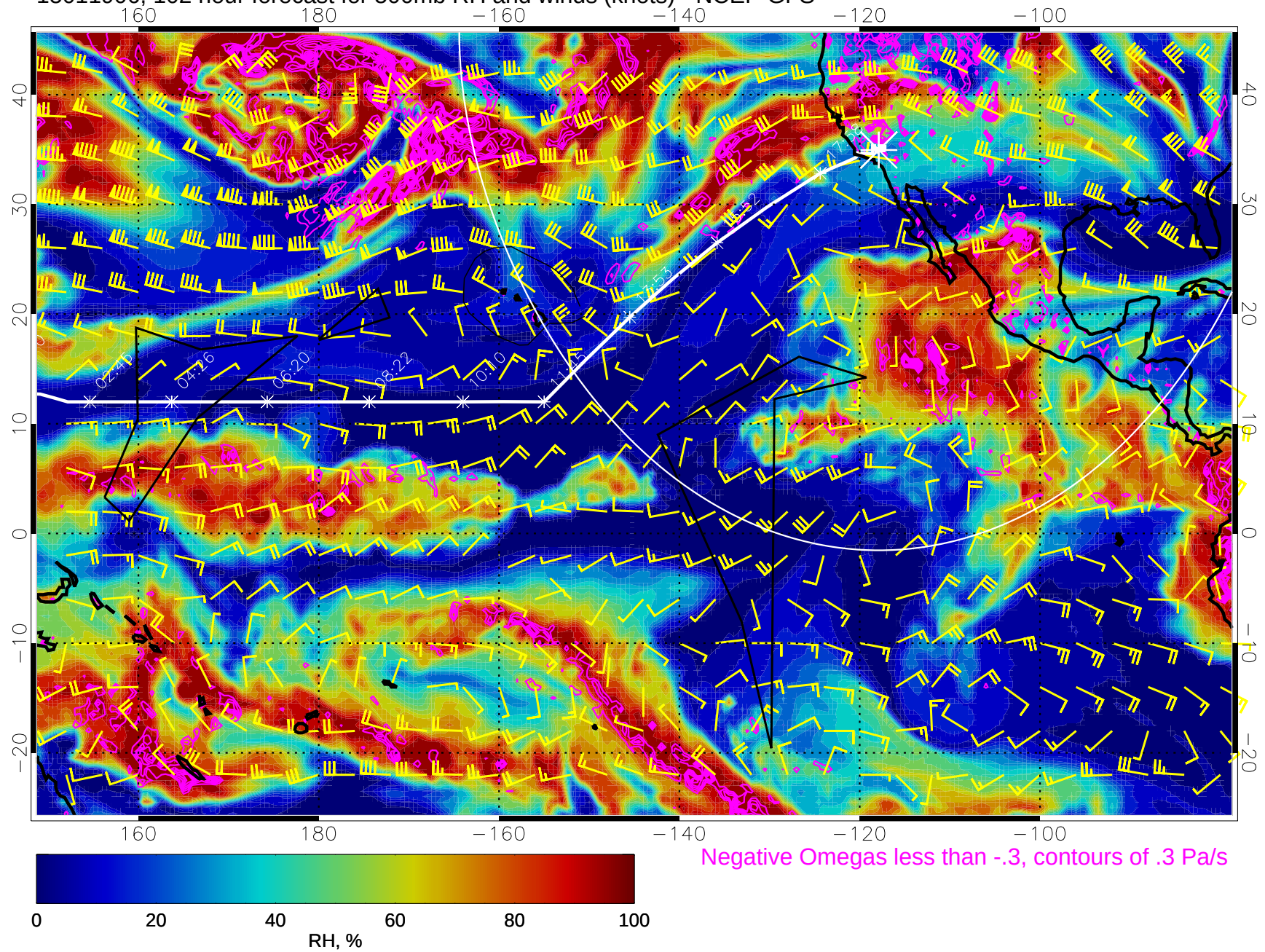
15011906, 102 hour forecast for 500mb RH and winds (knots) - NCEP GFS
