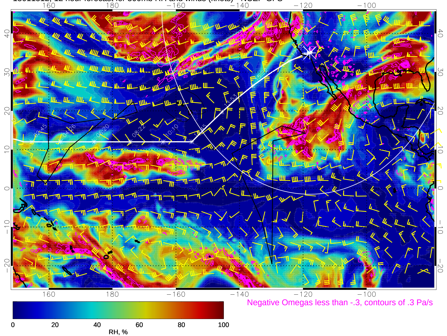
15011512, 12 hour forecast for 500mb RH and winds (knots) - NCEP GFS
