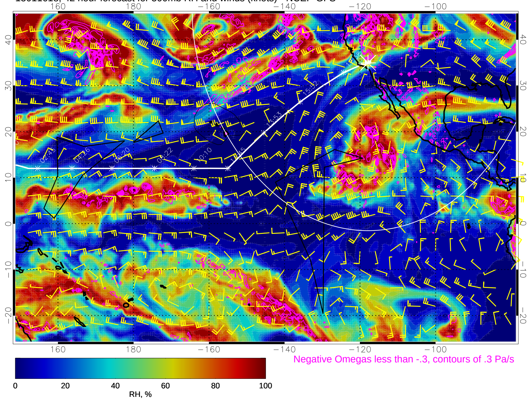
15011618, 42 hour forecast for 500mb RH and winds (knots) - NCEP GFS
