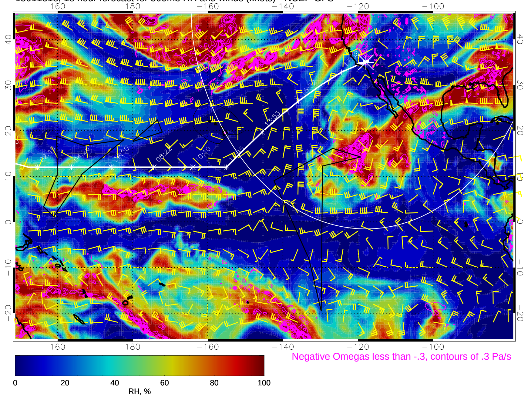
15011518, 18 hour forecast for 500mb RH and winds (knots) - NCEP GFS
