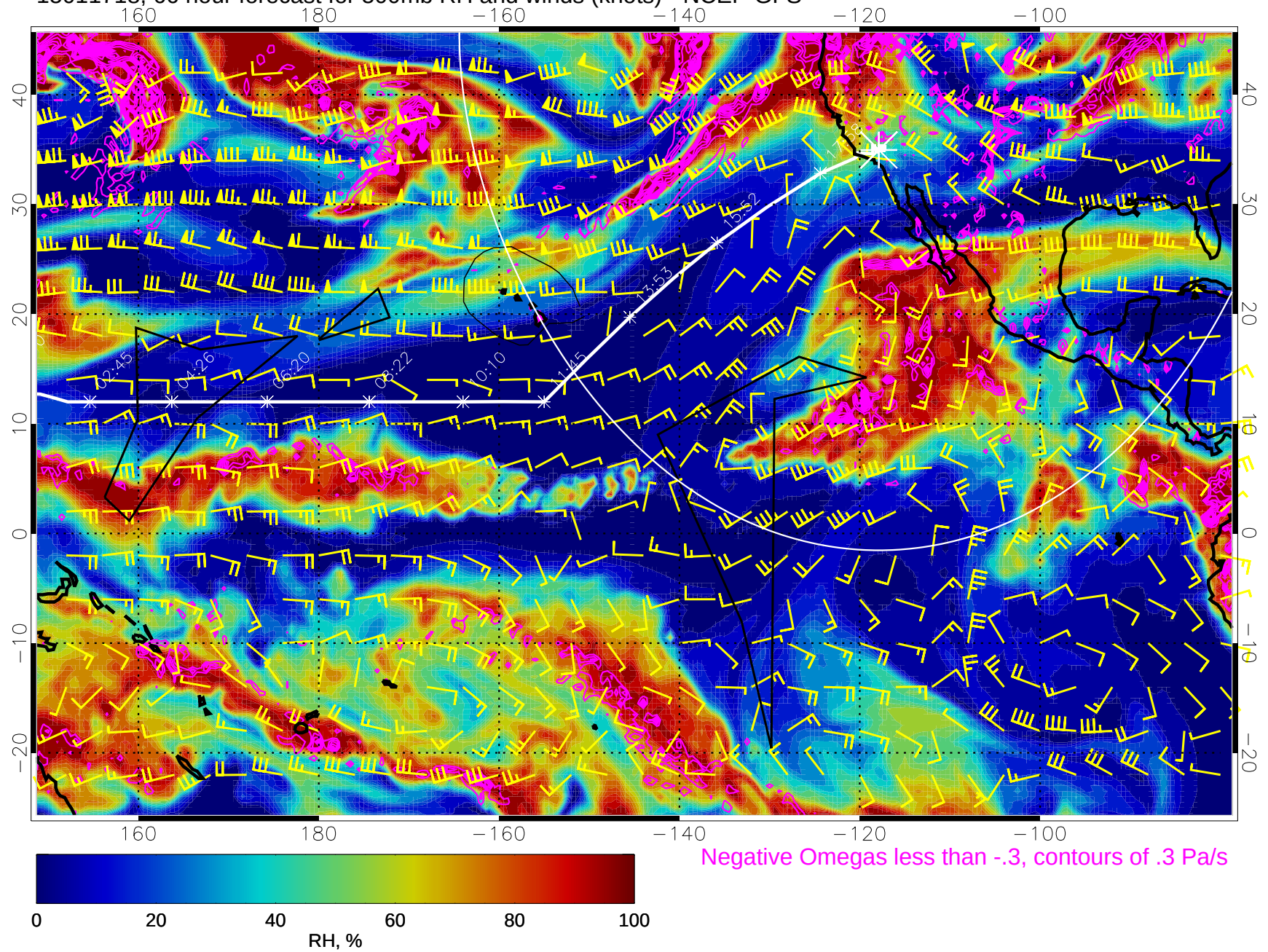
15011718, 66 hour forecast for 500mb RH and winds (knots) - NCEP GFS
