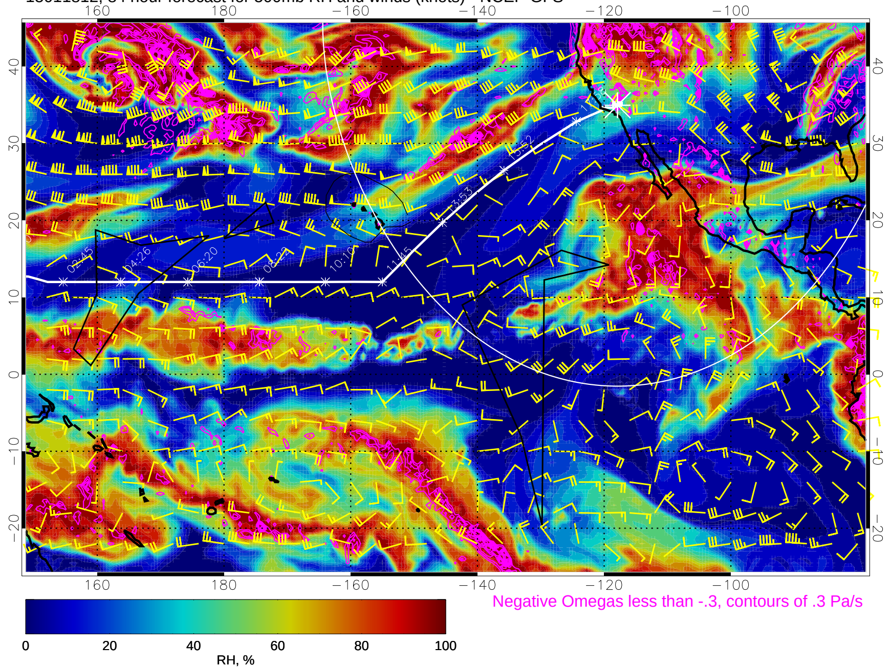
15011812, 84 hour forecast for 500mb RH and winds (knots) - NCEP GFS
