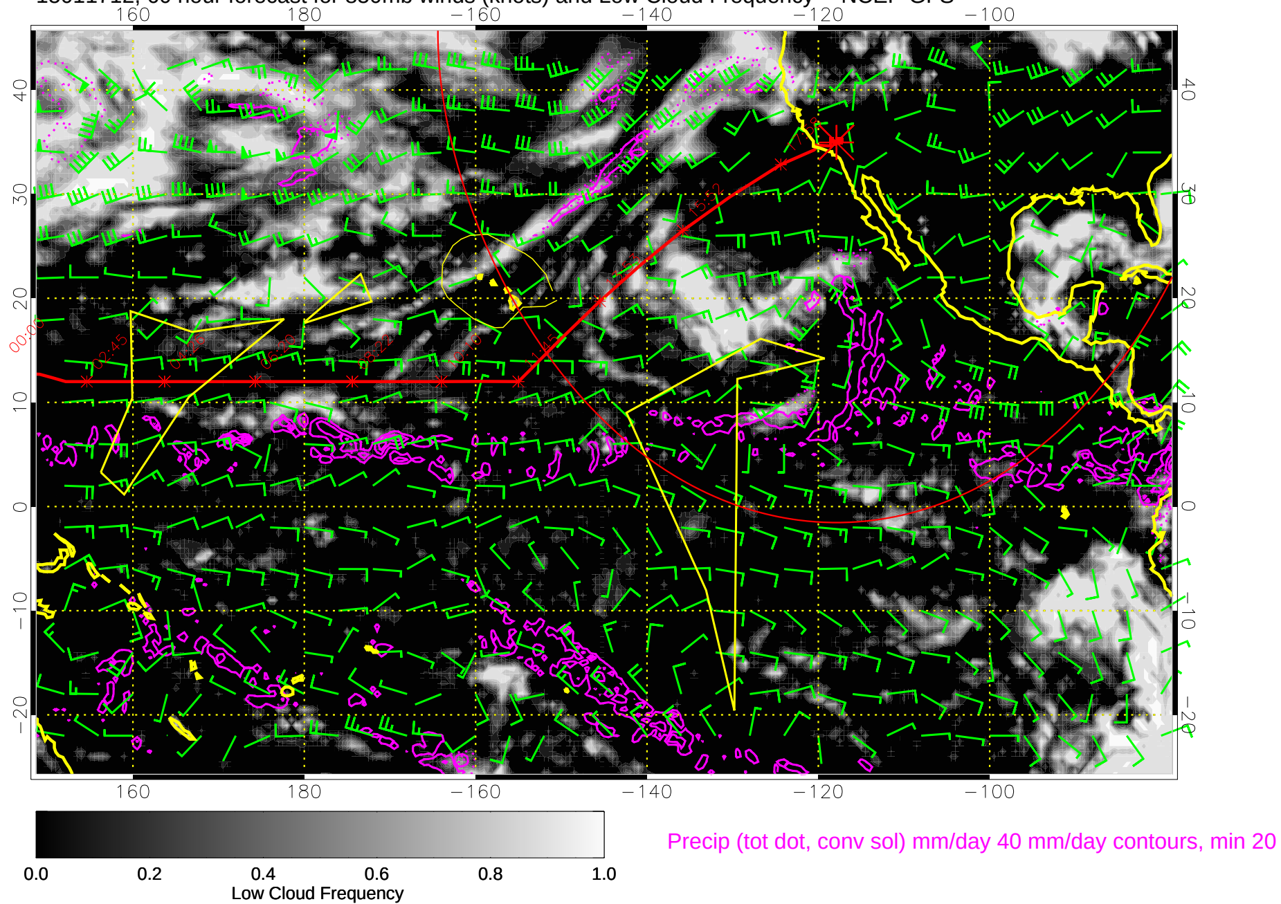
15011712, 60 hour forecast for 850mb winds (knots) and Low Cloud Frequency -- NCEP GFS
