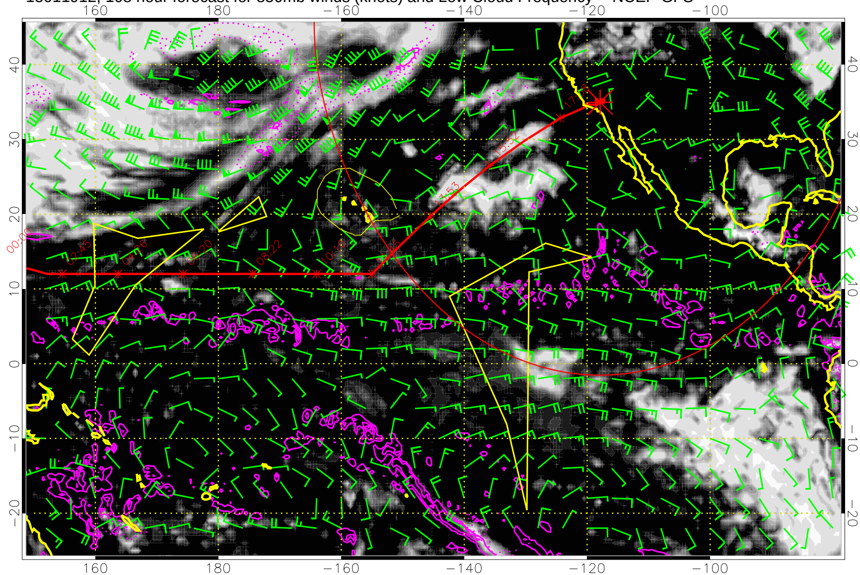
15011912, 108 hour forecast for 850mb winds (knots) and Low Cloud Frequency -- NCEP GFS
