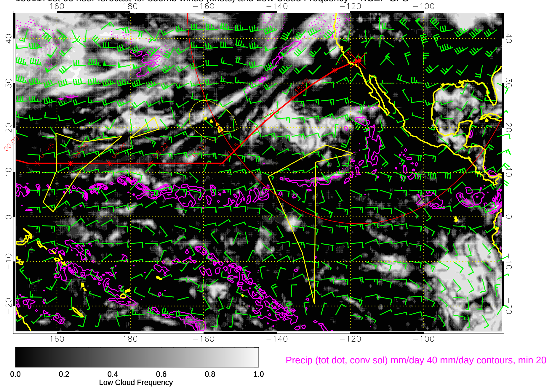
15011718, 66 hour forecast for 850mb winds (knots) and Low Cloud Frequency -- NCEP GFS
