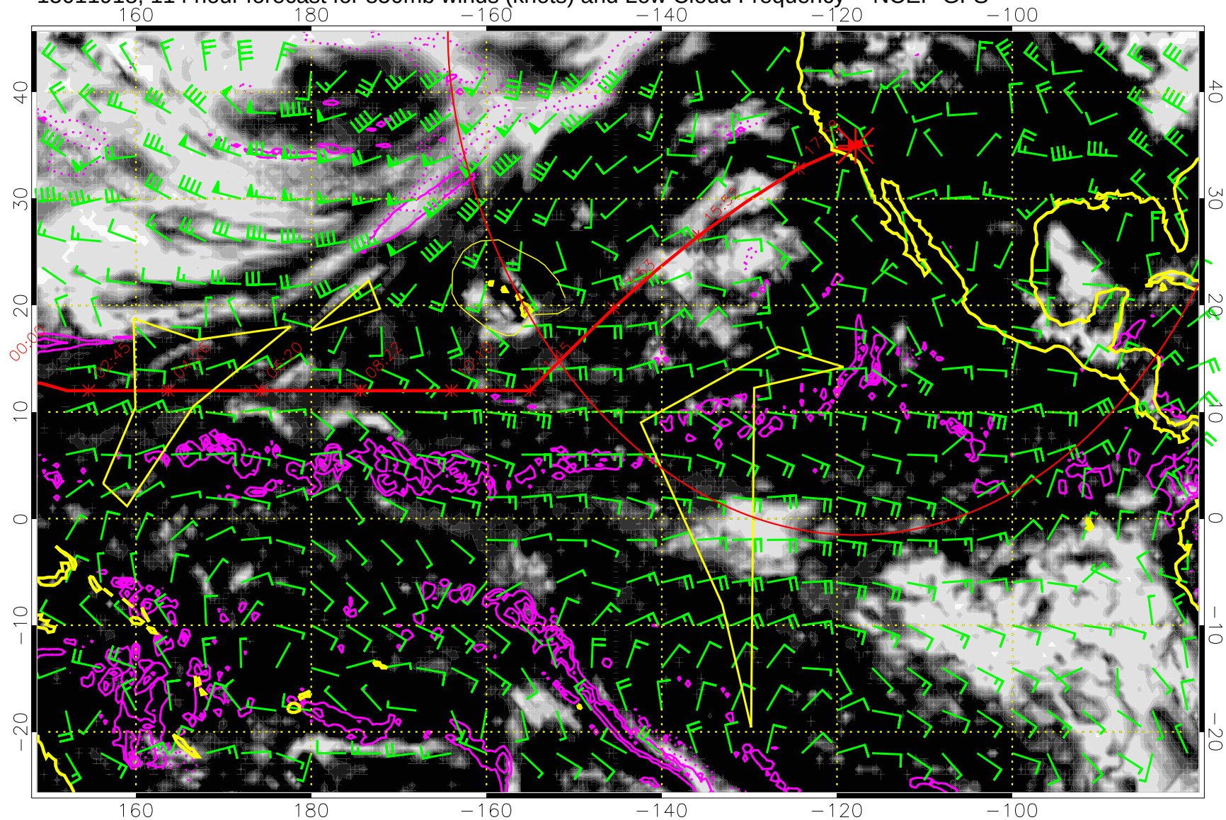
15011918, 114 hour forecast for 850mb winds (knots) and Low Cloud Frequency -- NCEP GFS
