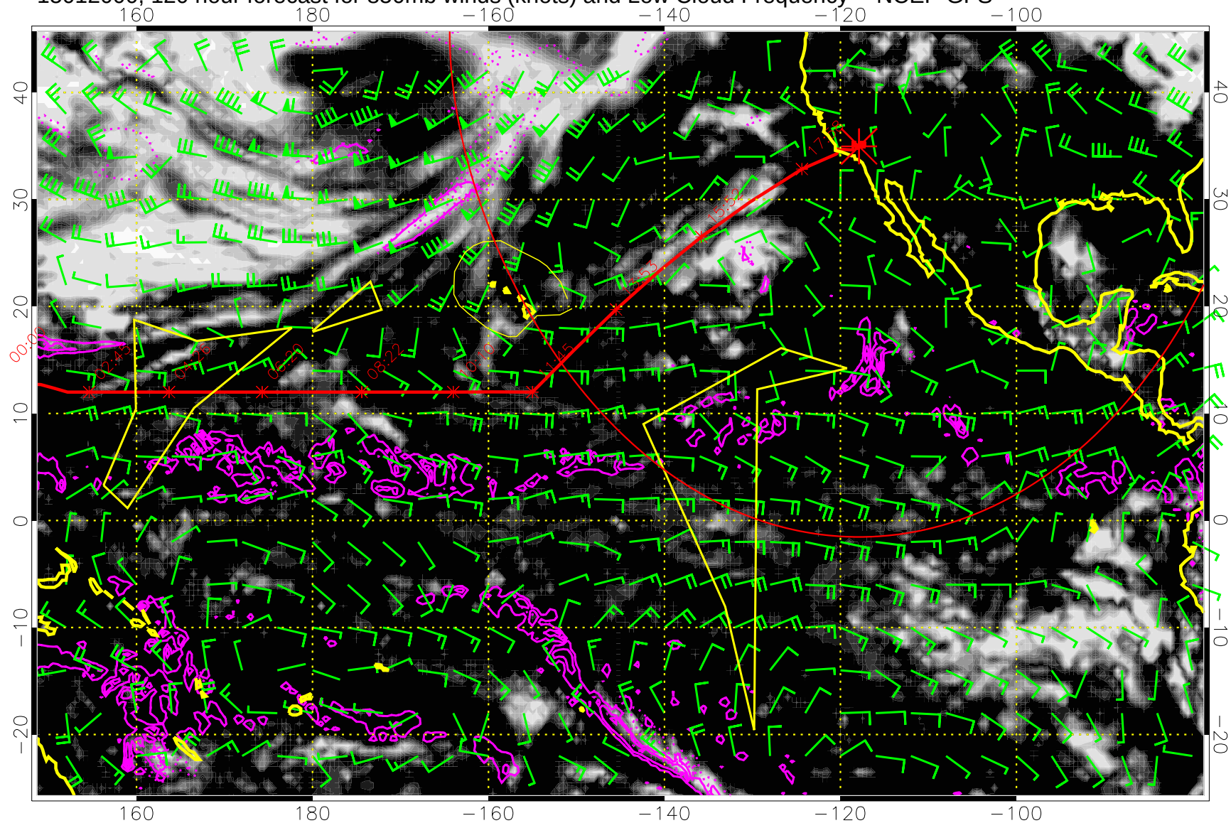
15012000, 120 hour forecast for 850mb winds (knots) and Low Cloud Frequency -- NCEP GFS
