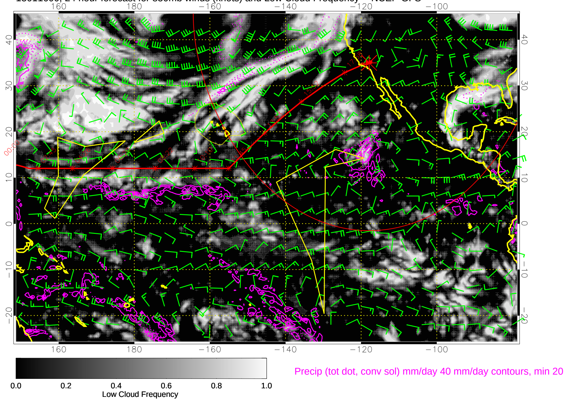
15011600, 24 hour forecast for 850mb winds (knots) and Low Cloud Frequency -- NCEP GFS
