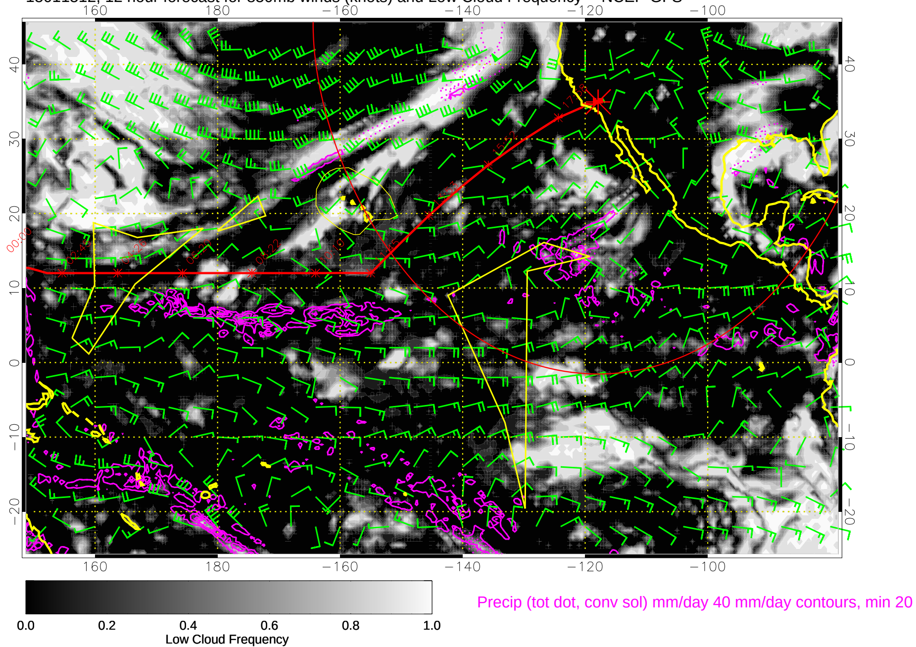
15011512, 12 hour forecast for 850mb winds (knots) and Low Cloud Frequency -- NCEP GFS
