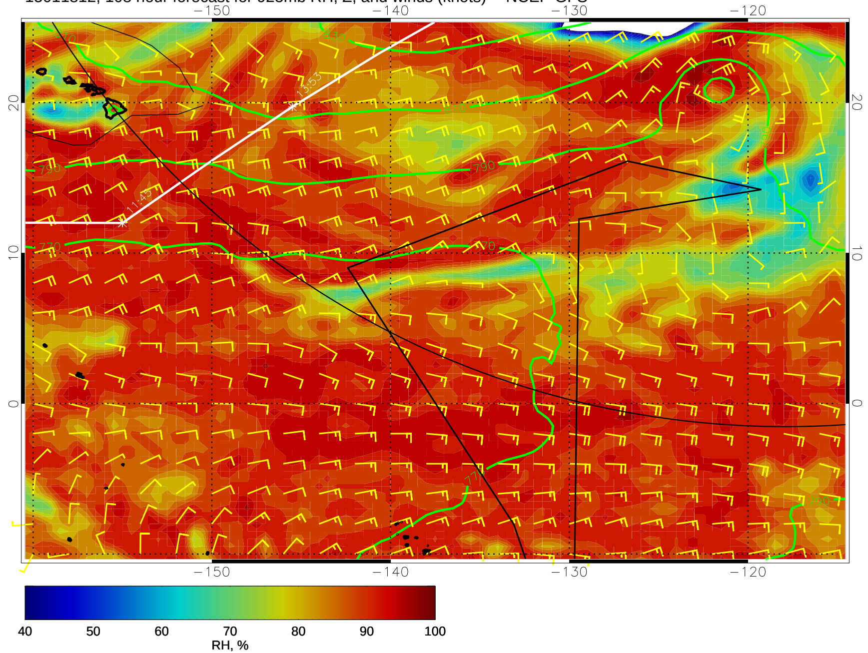
15011812, 108 hour forecast for 925mb RH, Z, and winds (knots) -- NCEP GFS
