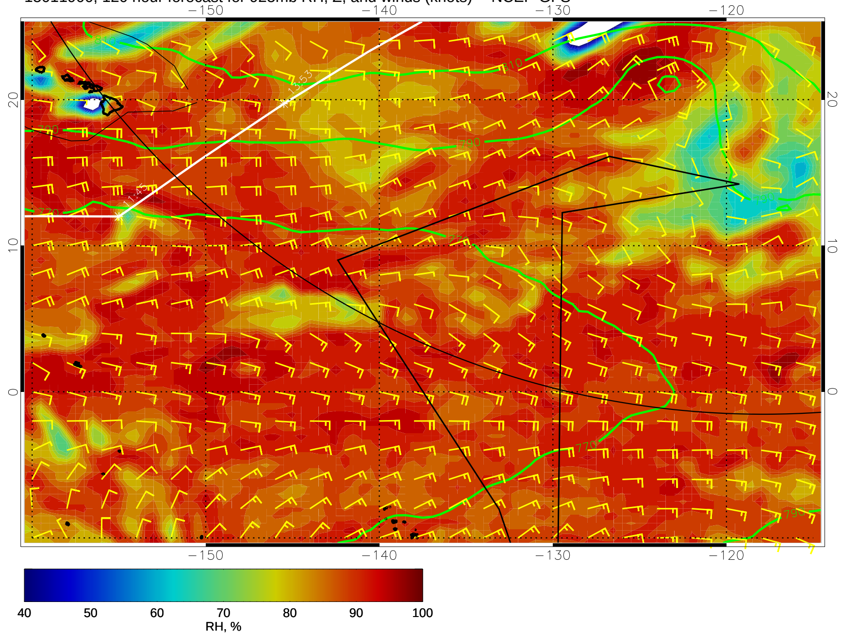
15011900, 120 hour forecast for 925mb RH, Z, and winds (knots) -- NCEP GFS
