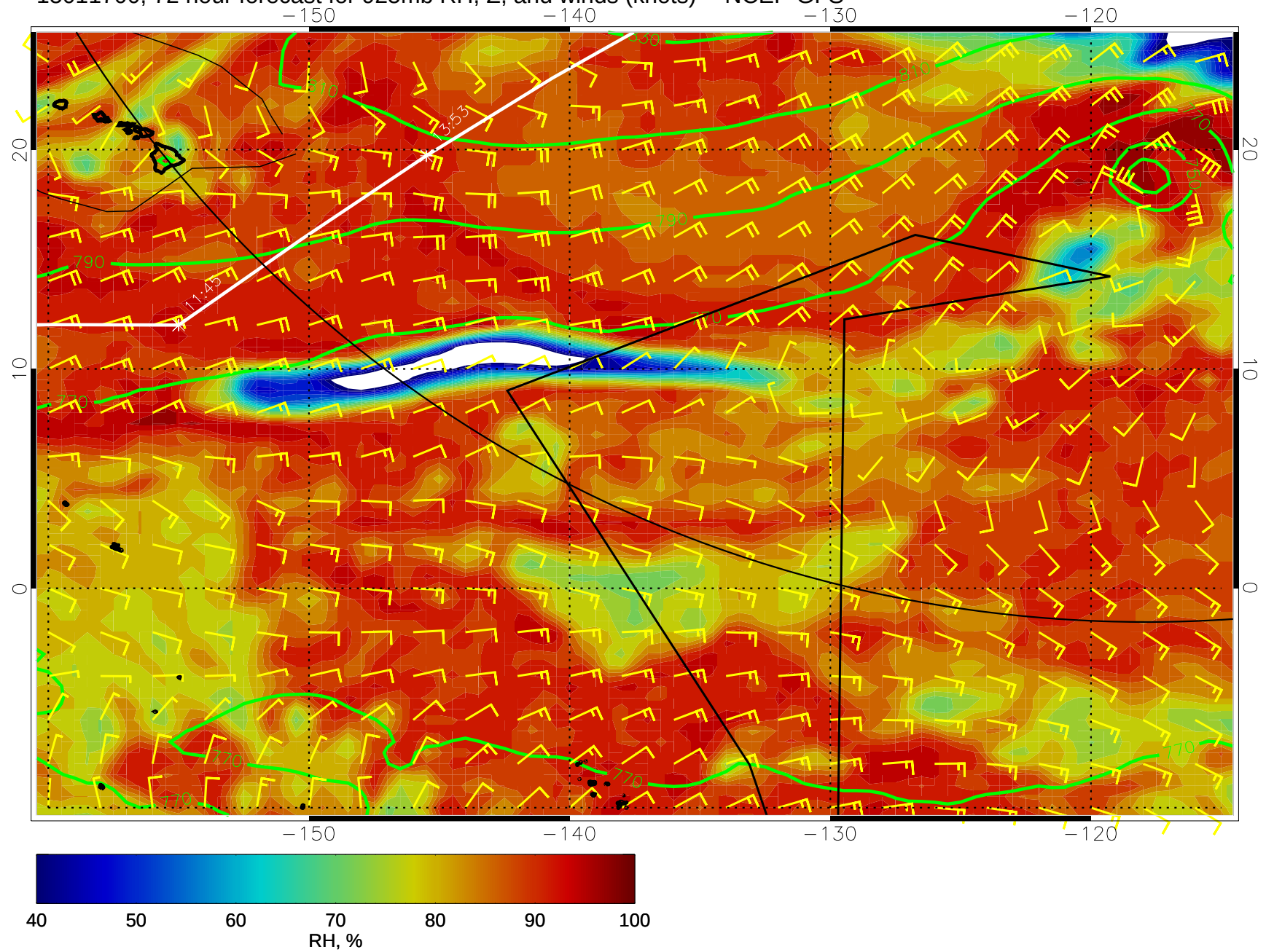
15011700, 72 hour forecast for 925mb RH, Z, and winds (knots) -- NCEP GFS
