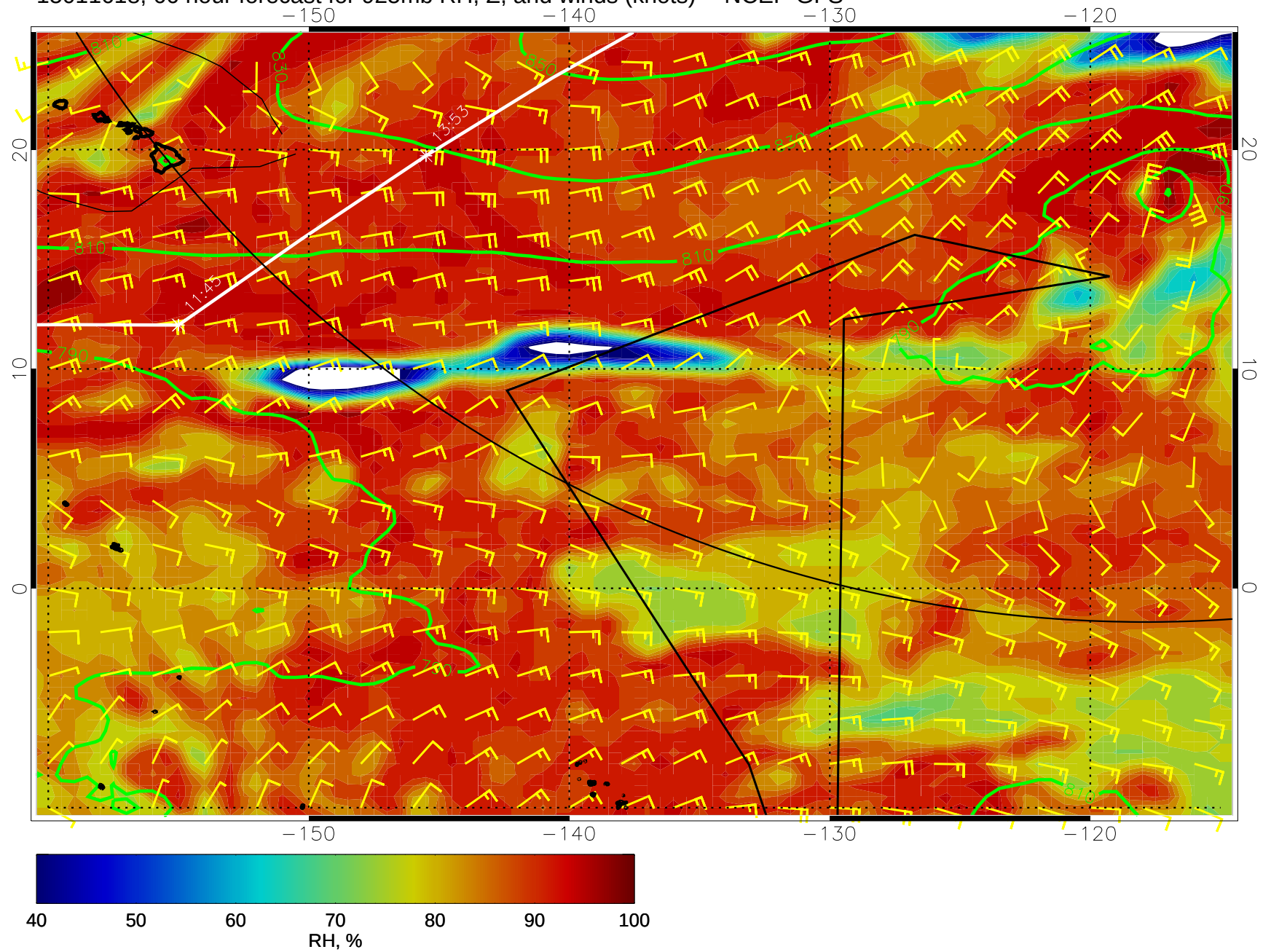
15011618, 66 hour forecast for 925mb RH, Z, and winds (knots) -- NCEP GFS
