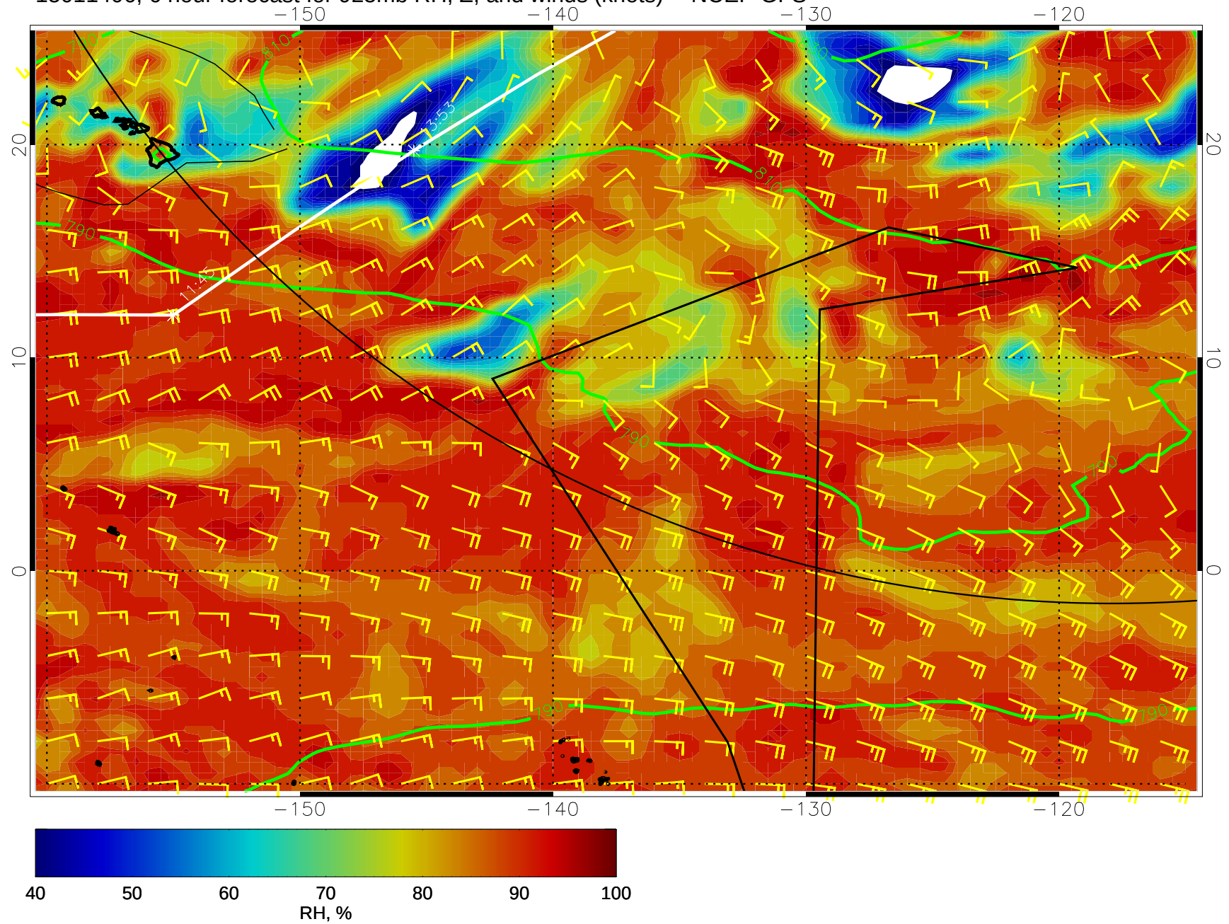
15011406, 6 hour forecast for 925mb RH, Z, and winds (knots) -- NCEP GFS
