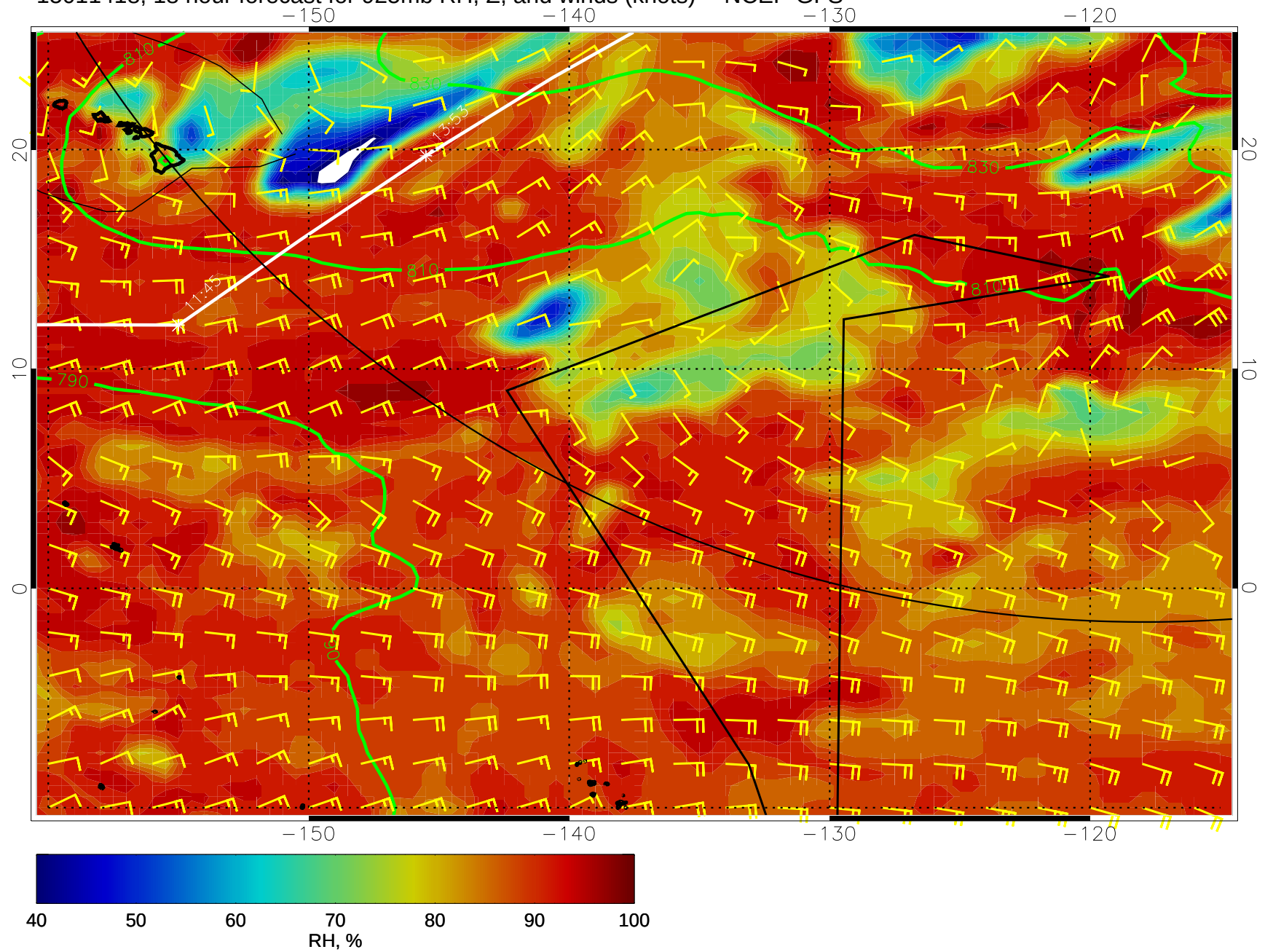
15011418, 18 hour forecast for 925mb RH, Z, and winds (knots) -- NCEP GFS
