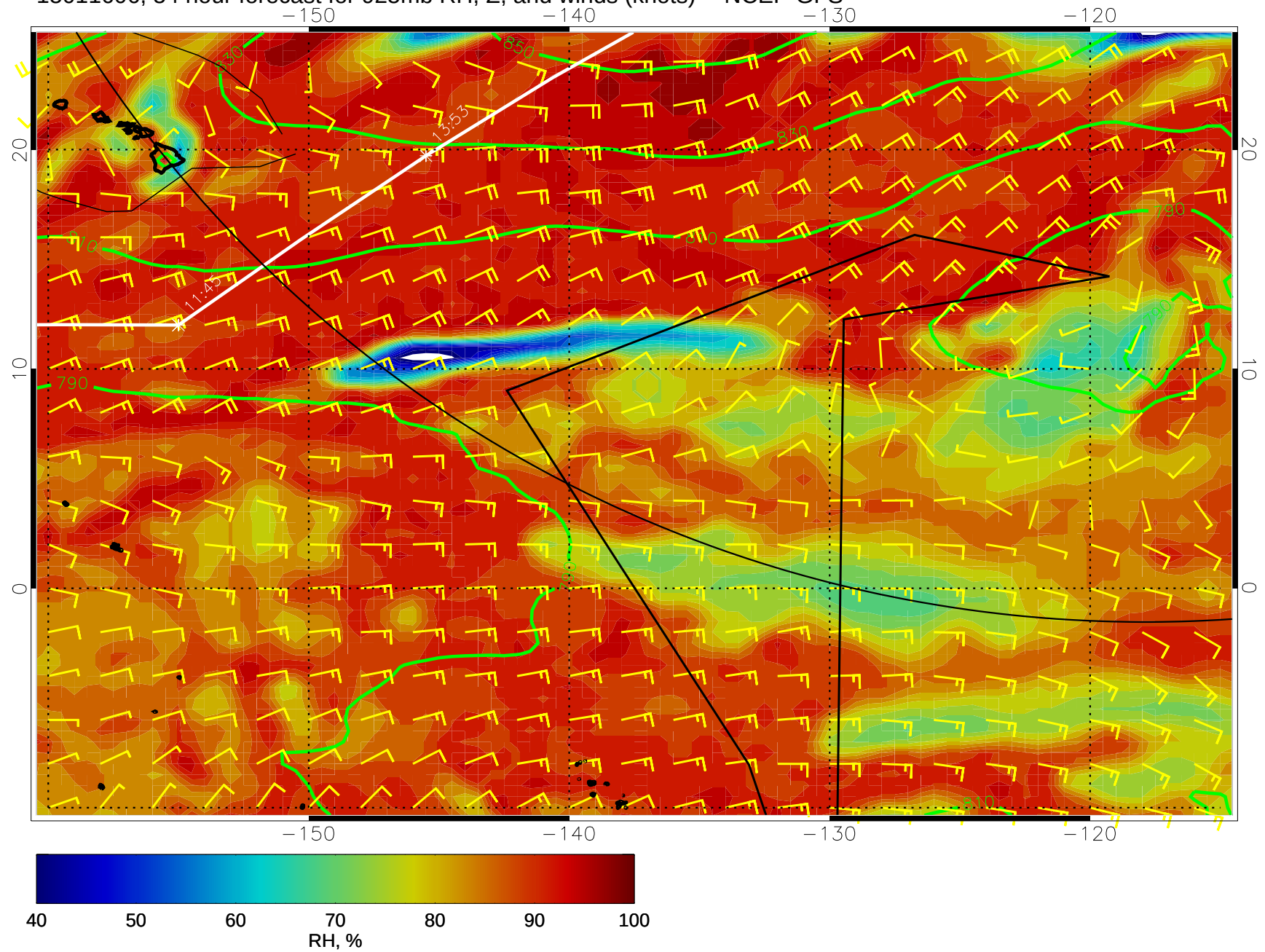
15011606, 54 hour forecast for 925mb RH, Z, and winds (knots) -- NCEP GFS
