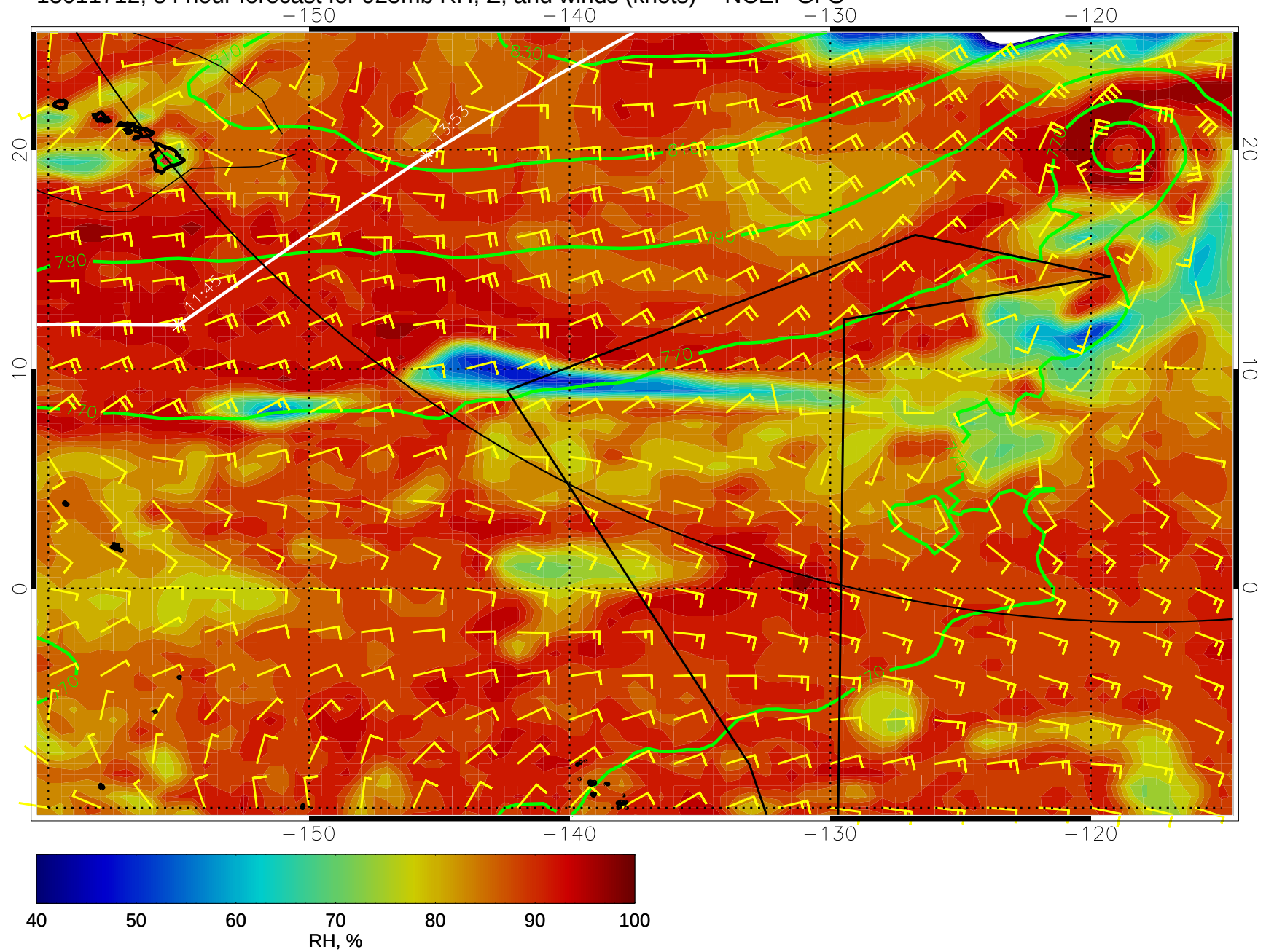
15011712, 84 hour forecast for 925mb RH, Z, and winds (knots) -- NCEP GFS
