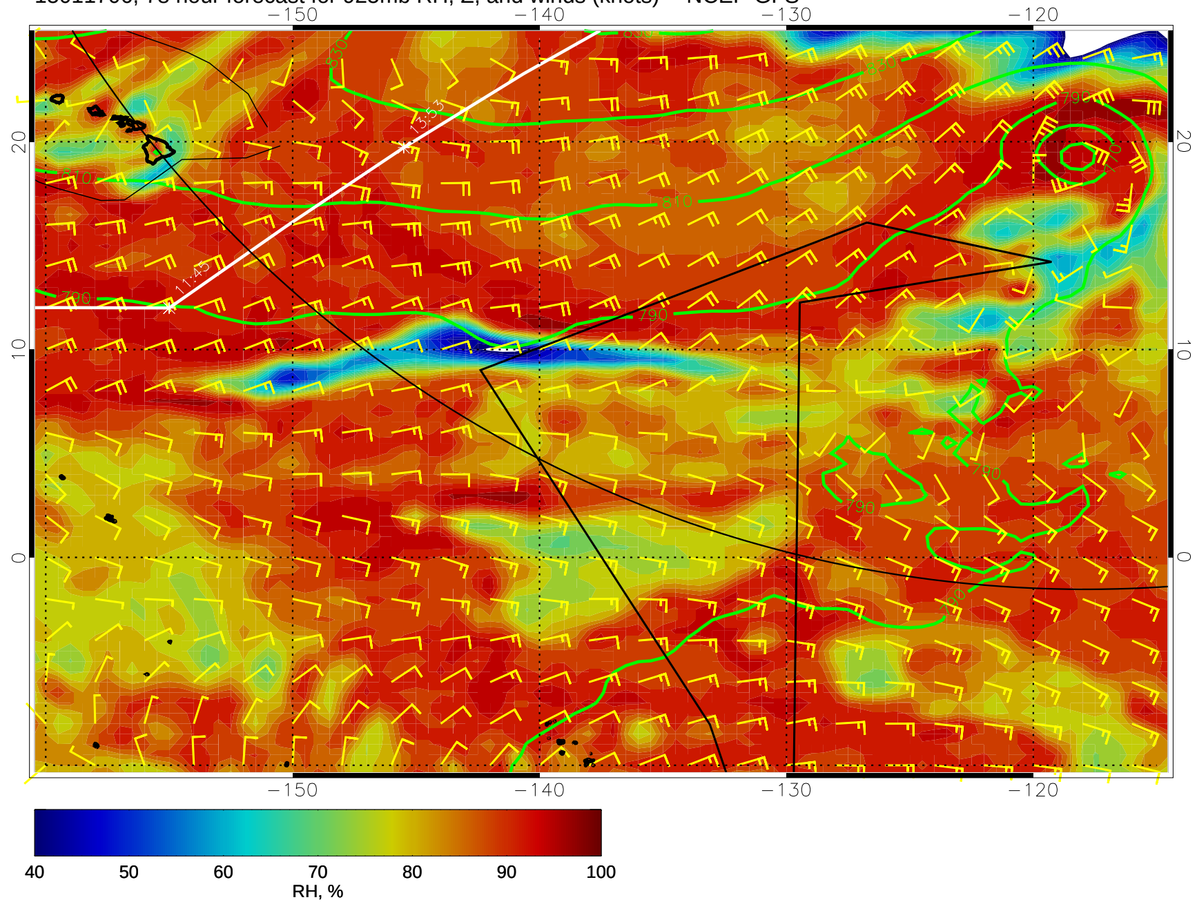
15011706, 78 hour forecast for 925mb RH, Z, and winds (knots) -- NCEP GFS
