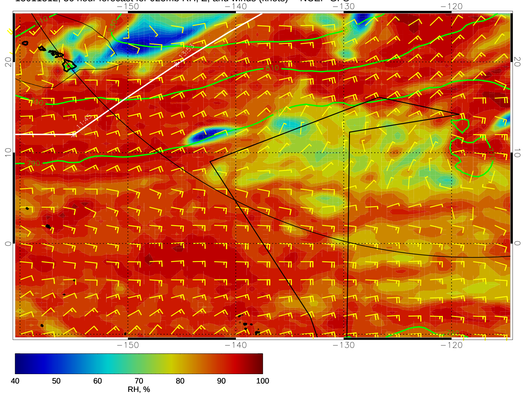
15011512, 36 hour forecast for 925mb RH, Z, and winds (knots) -- NCEP GFS
