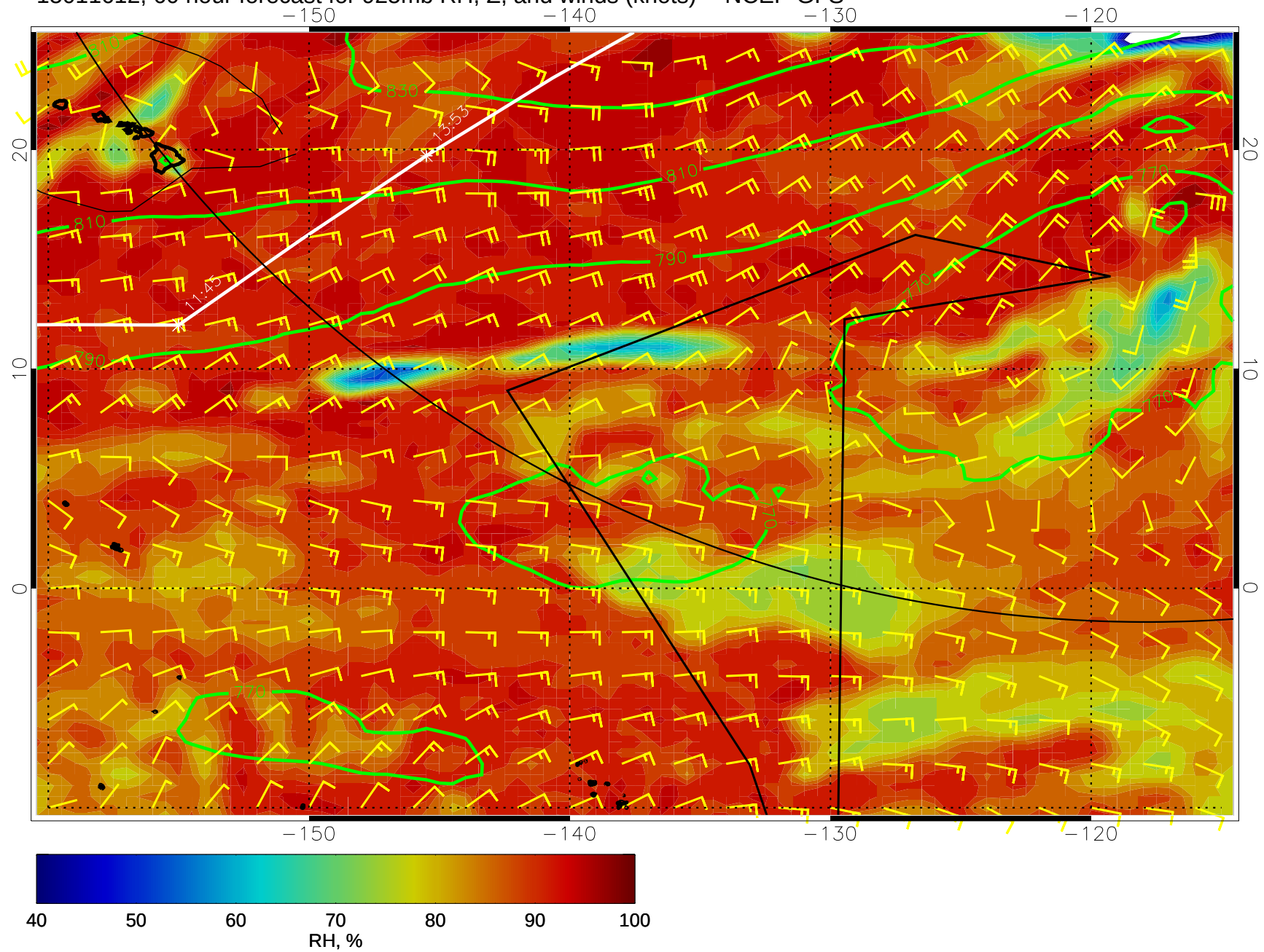
15011612, 60 hour forecast for 925mb RH, Z, and winds (knots) -- NCEP GFS
