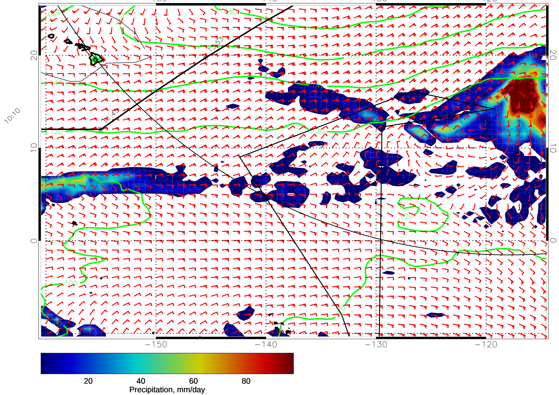
15011606, 54 hour forecast for precip, 1000mb Z, and winds (knots) -- NCEP GFS
