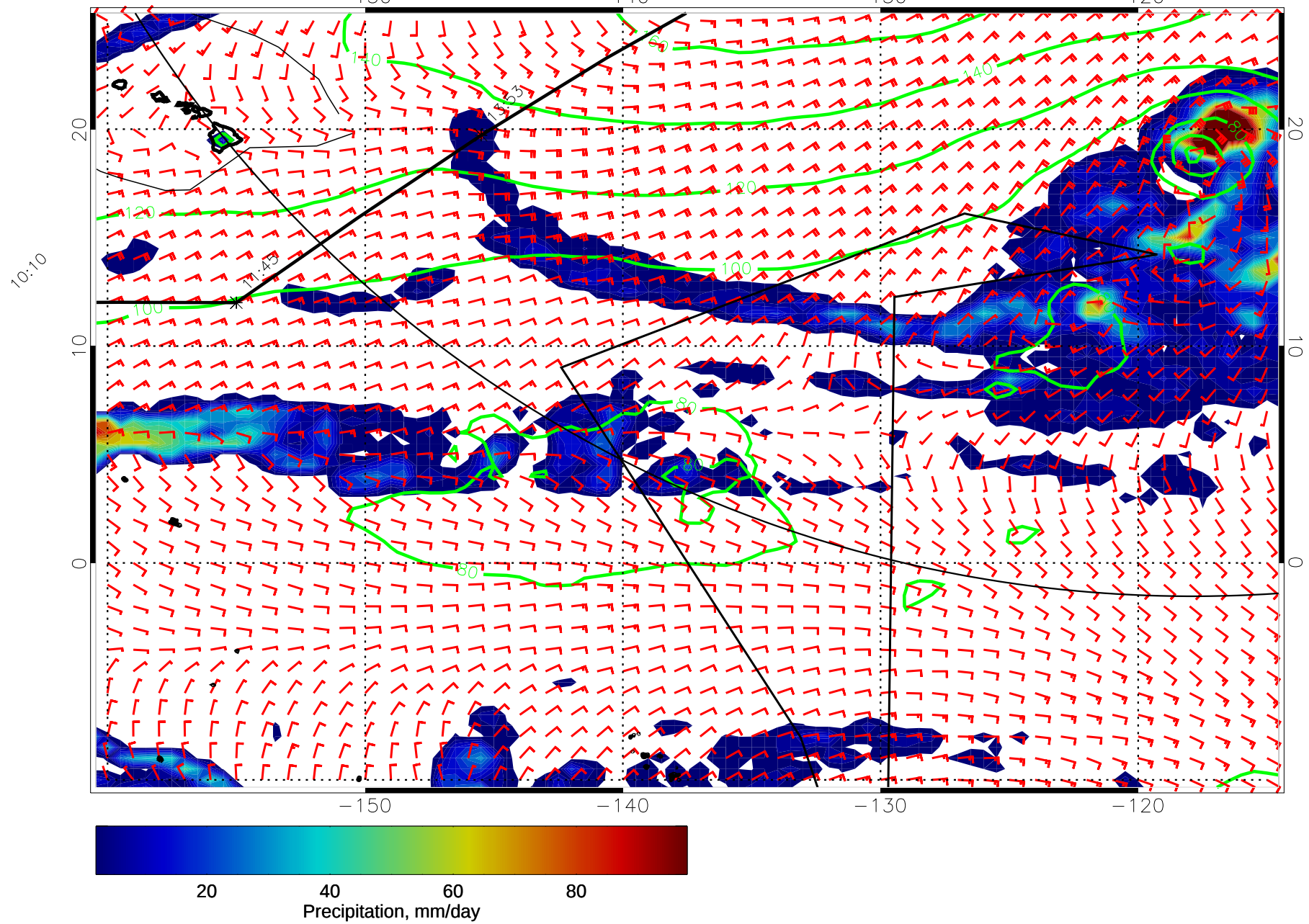
15011700, 72 hour forecast for precip, 1000mb Z, and winds (knots) -- NCEP GFS
