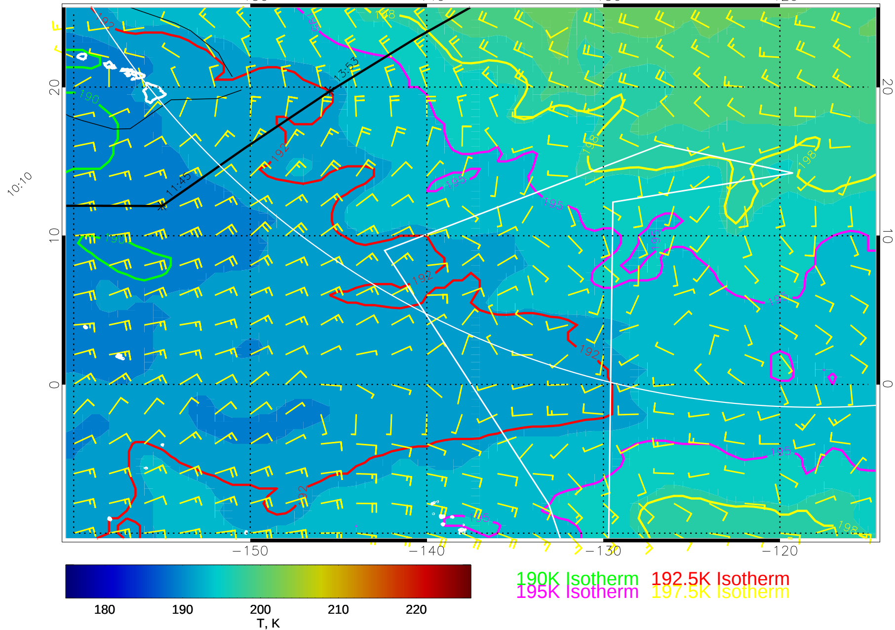
15011406, 6 hour forecast for 70mb T and winds (knots) -- NCEP GFS
