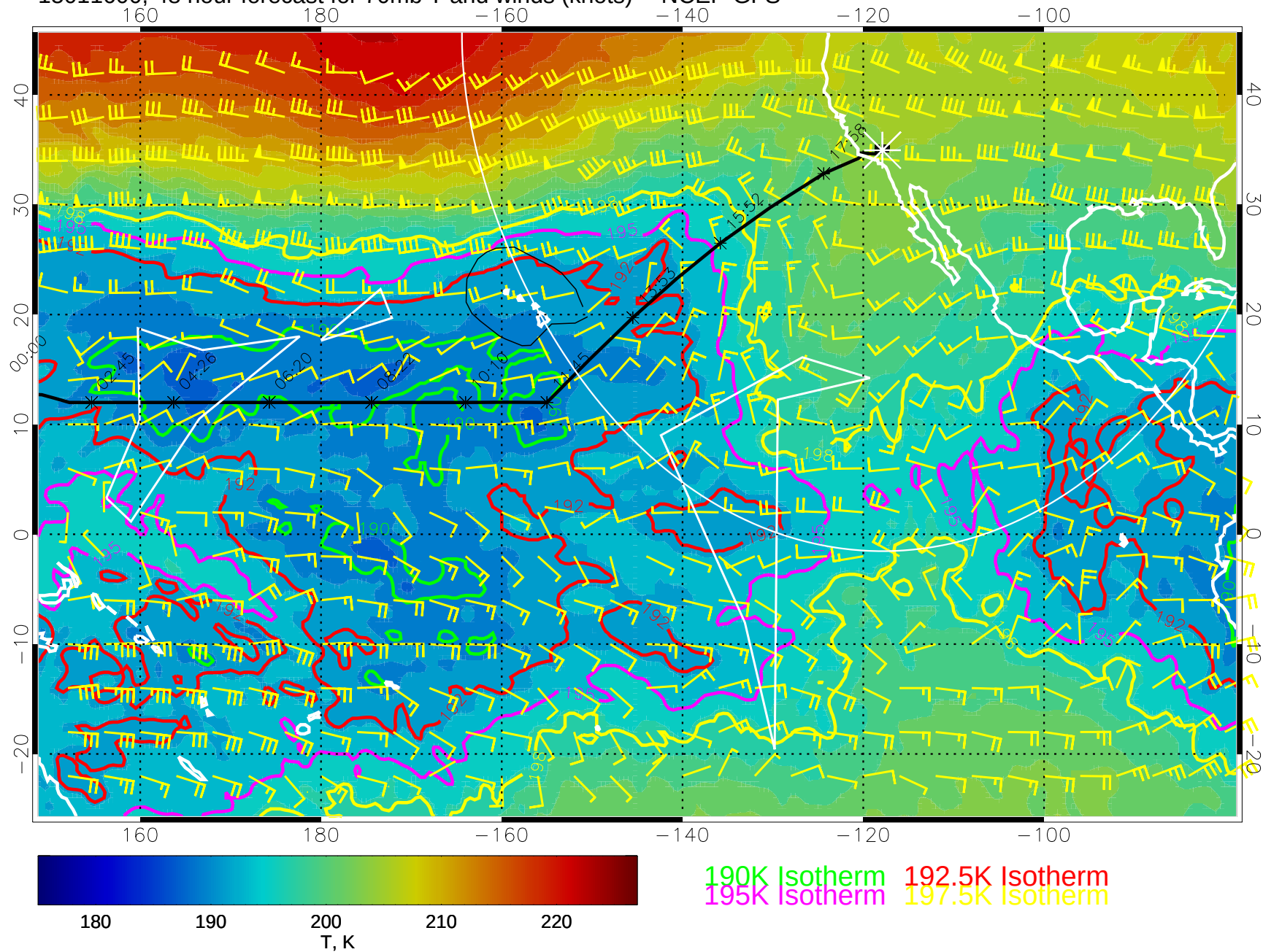
15011600, 48 hour forecast for 70mb T and winds (knots) -- NCEP GFS
