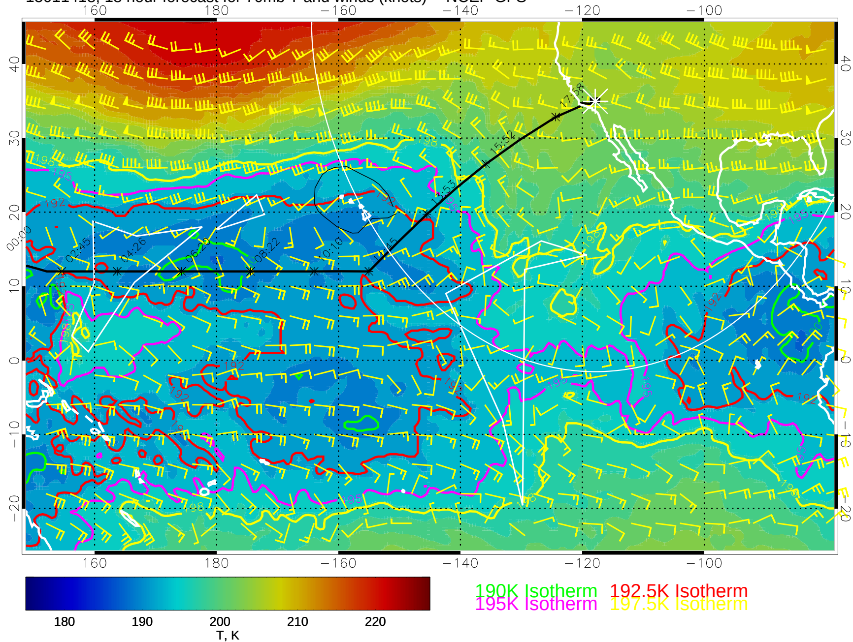
15011418, 18 hour forecast for 70mb T and winds (knots) -- NCEP GFS
