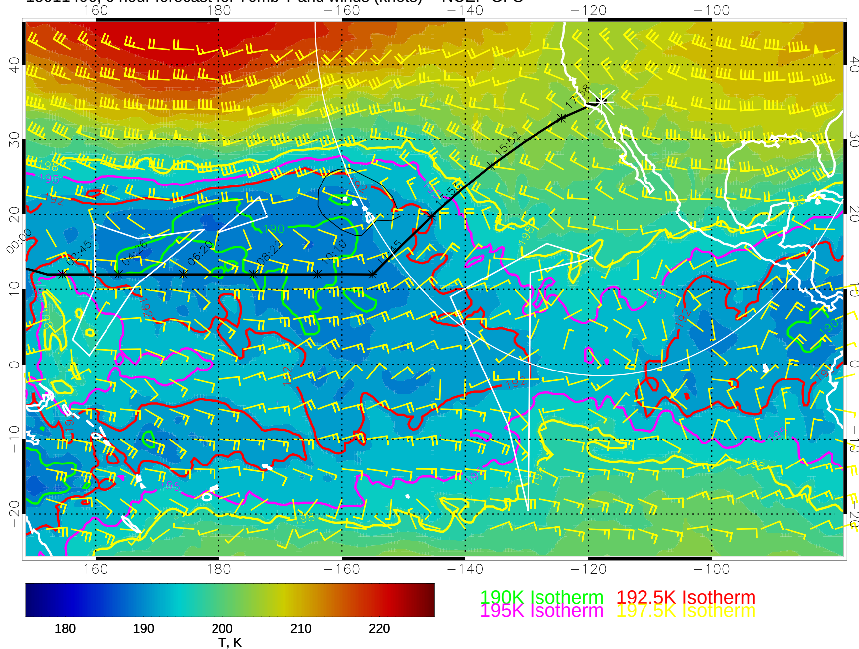
15011406, 6 hour forecast for 70mb T and winds (knots) -- NCEP GFS
