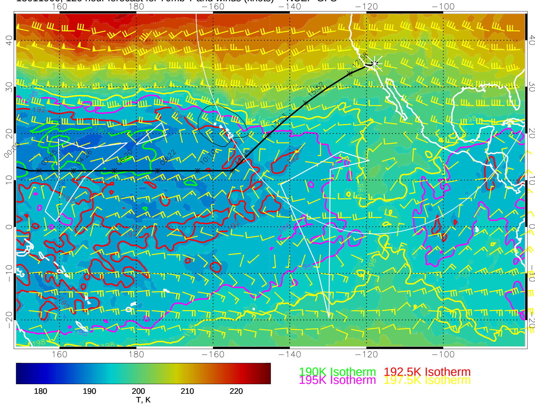
15011900, 120 hour forecast for 70mb T and winds (knots) -- NCEP GFS
