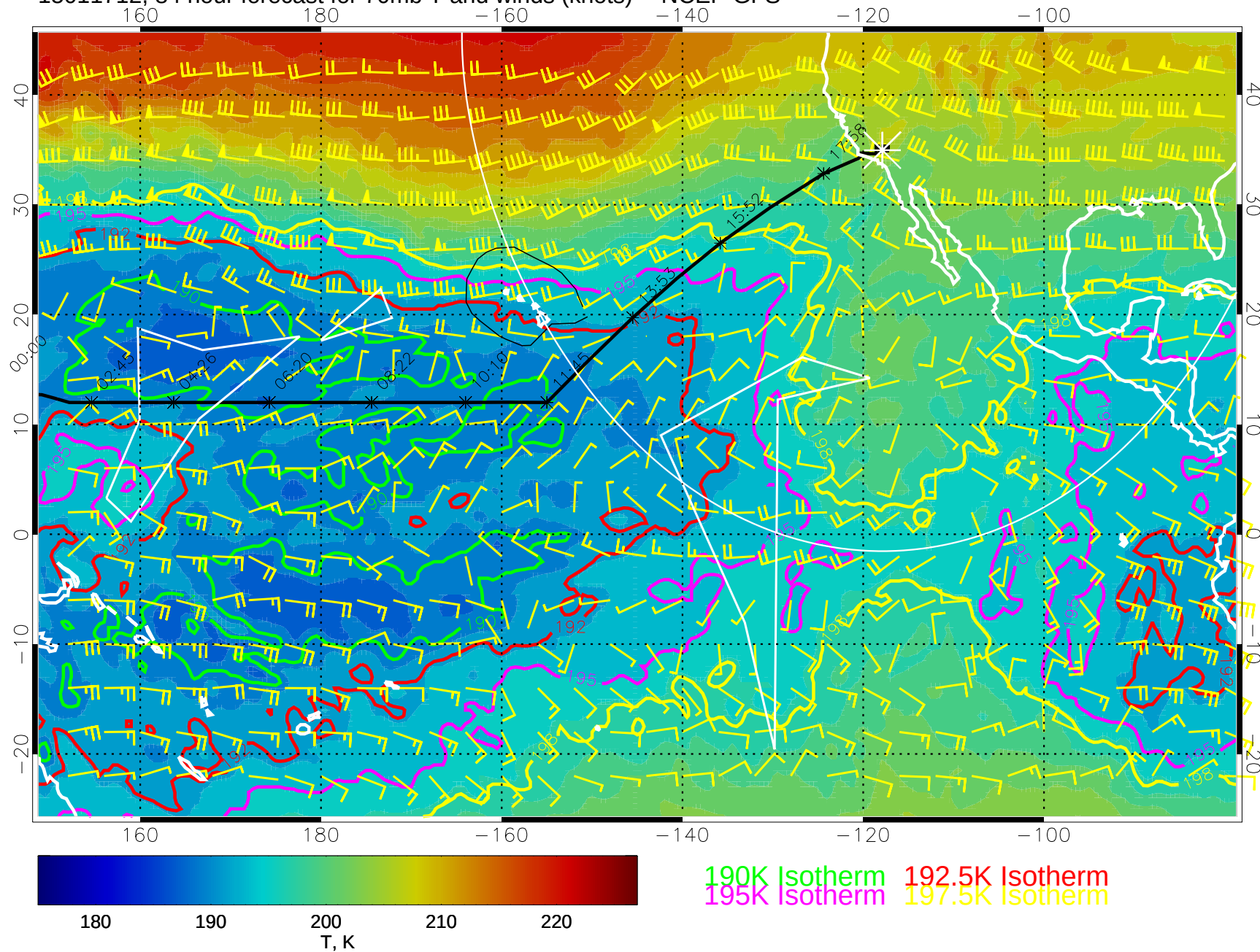
15011712, 84 hour forecast for 70mb T and winds (knots) -- NCEP GFS
