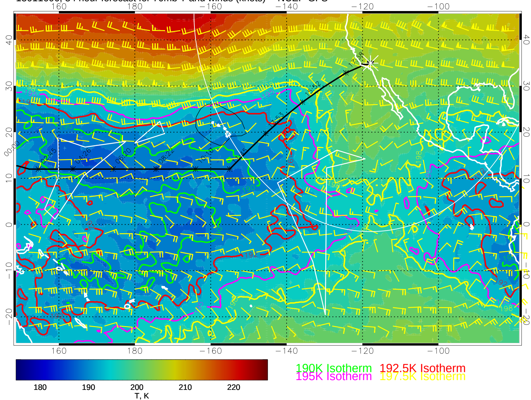
15011606, 54 hour forecast for 70mb T and winds (knots) -- NCEP GFS
