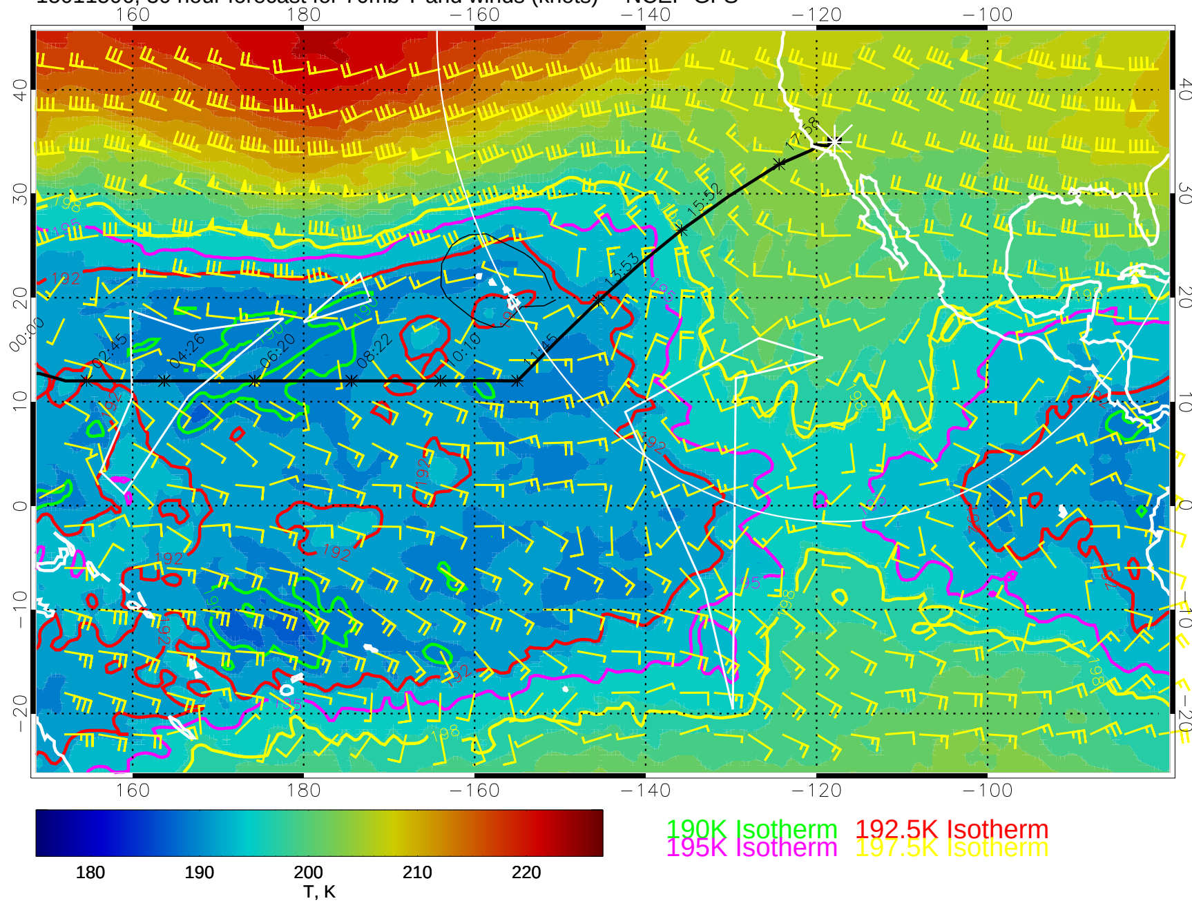
15011506, 30 hour forecast for 70mb T and winds (knots) -- NCEP GFS
