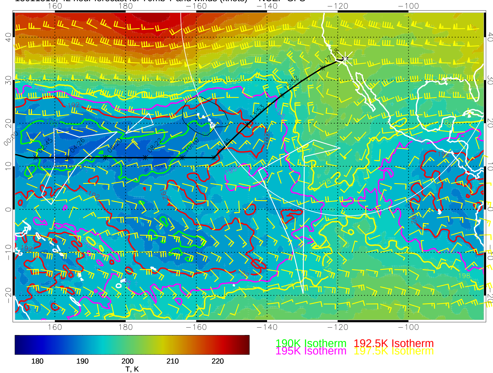
15011518, 42 hour forecast for 70mb T and winds (knots) -- NCEP GFS
