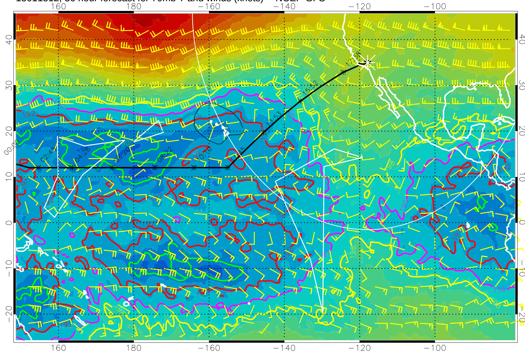
15011512, 36 hour forecast for 70mb T and winds (knots) -- NCEP GFS
