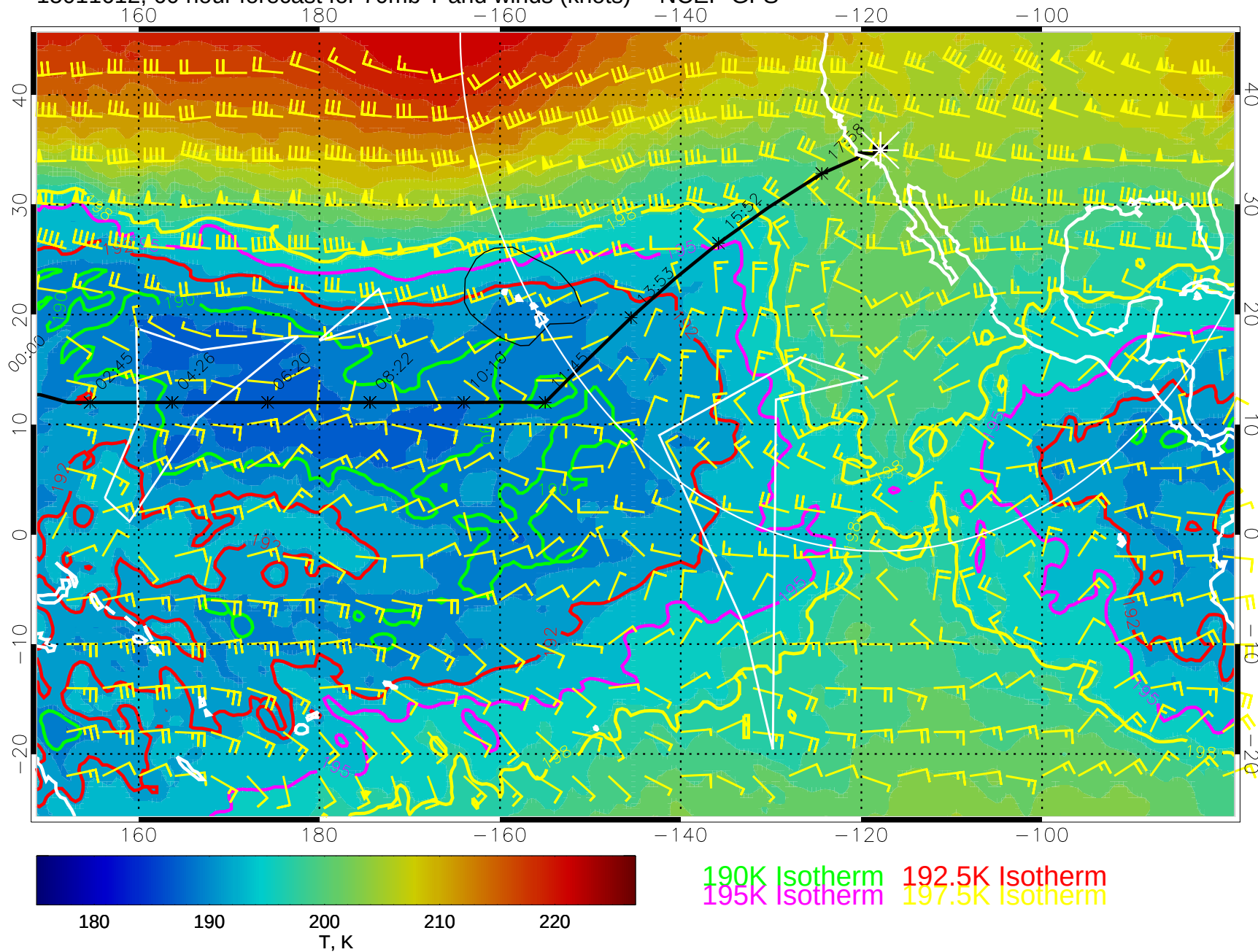
15011612, 60 hour forecast for 70mb T and winds (knots) -- NCEP GFS
