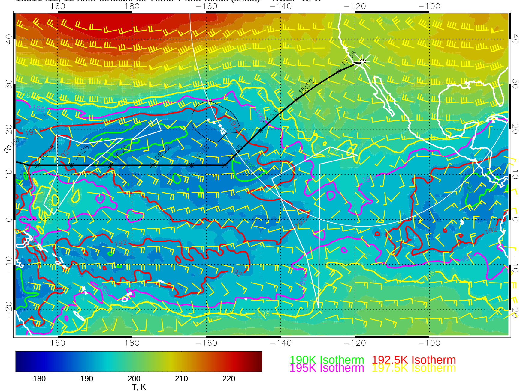
15011412, 12 hour forecast for 70mb T and winds (knots) -- NCEP GFS
