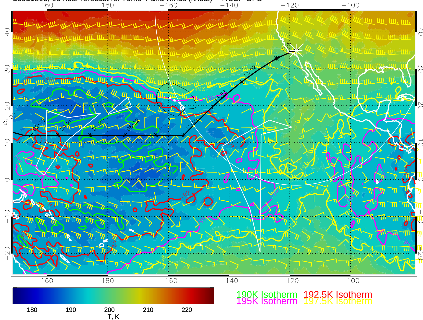
15011800, 96 hour forecast for 70mb T and winds (knots) -- NCEP GFS
