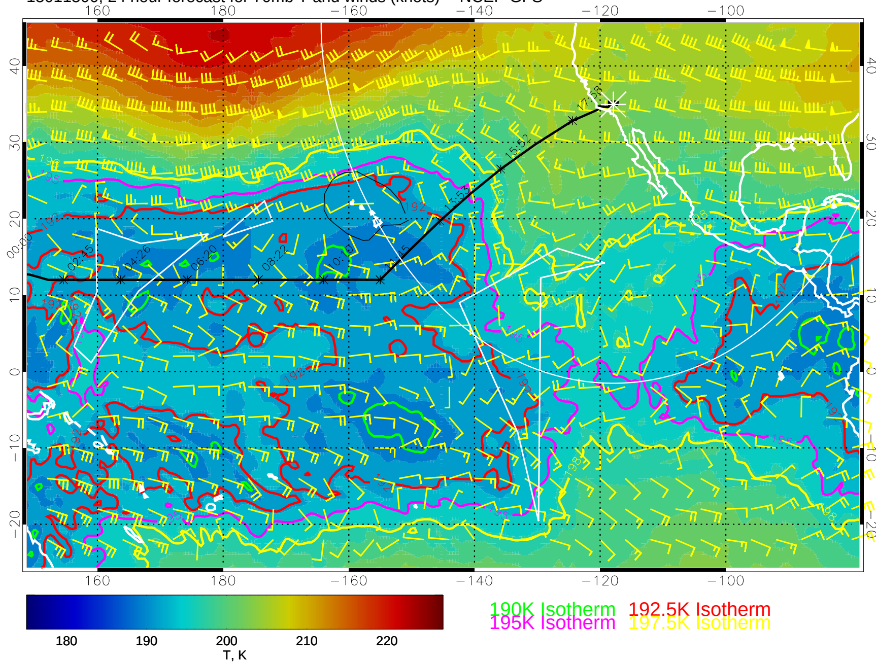
15011500, 24 hour forecast for 70mb T and winds (knots) -- NCEP GFS
