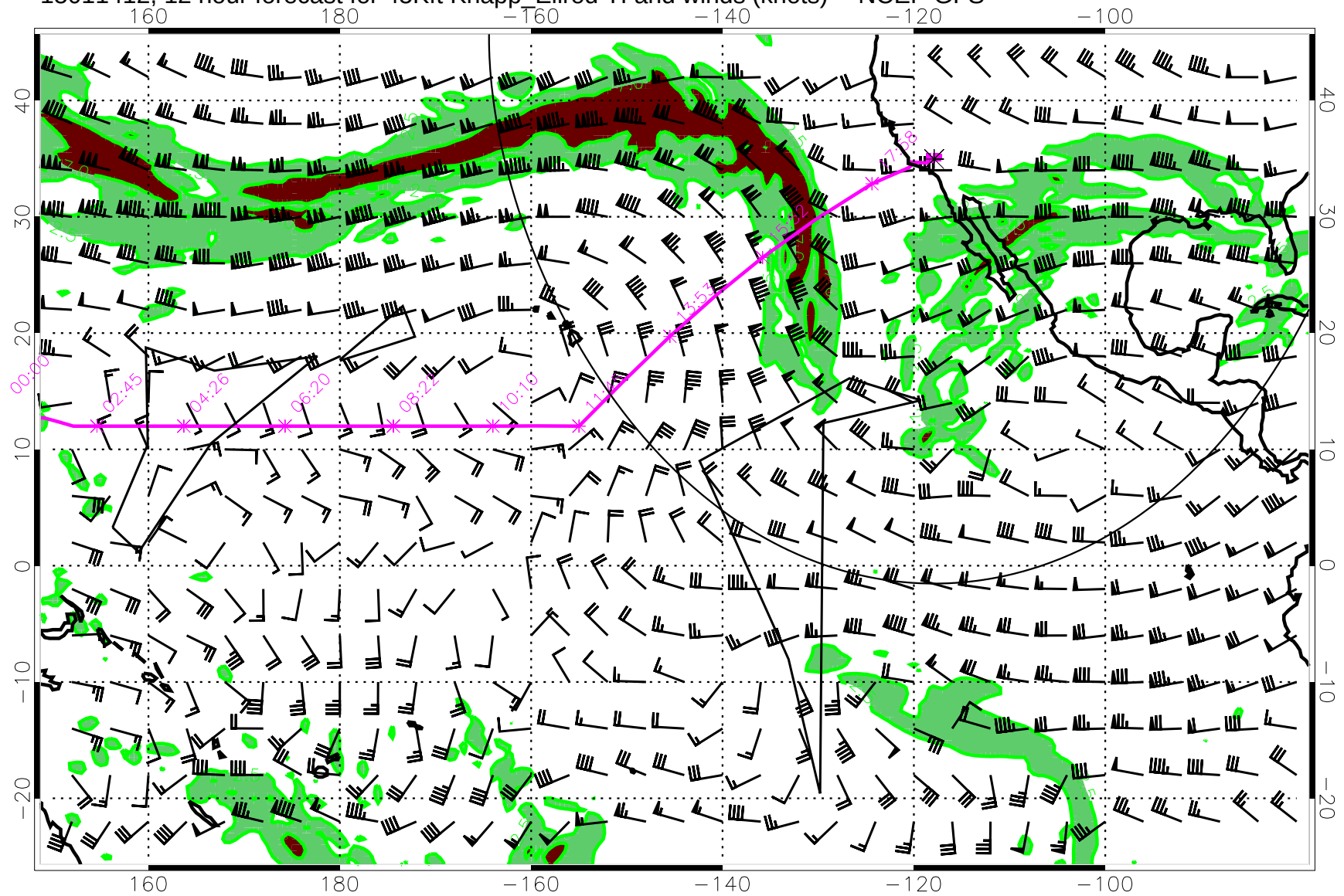
15011412, 12 hour forecast for 45Kft Knapp_Ellrod TI and winds (knots) -- NCEP GFS
