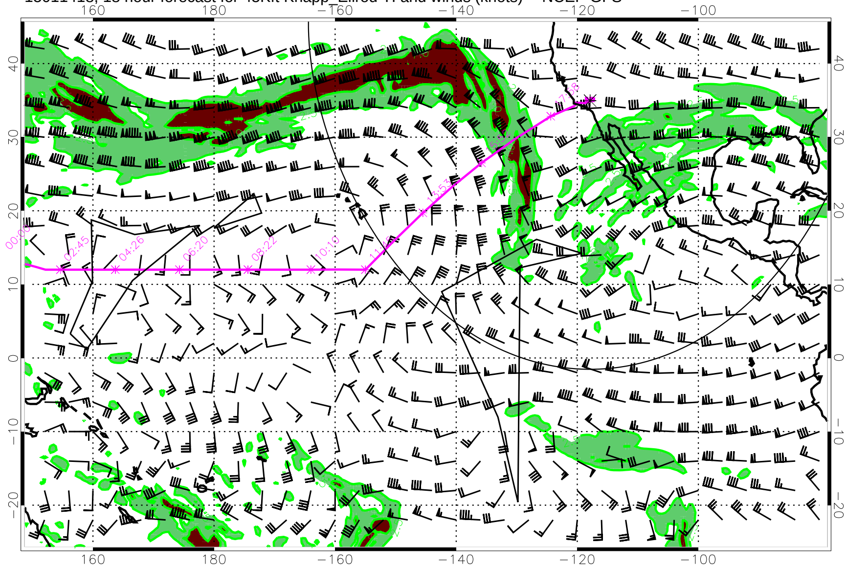
15011418, 18 hour forecast for 45Kft Knapp_Ellrod TI and winds (knots) -- NCEP GFS
