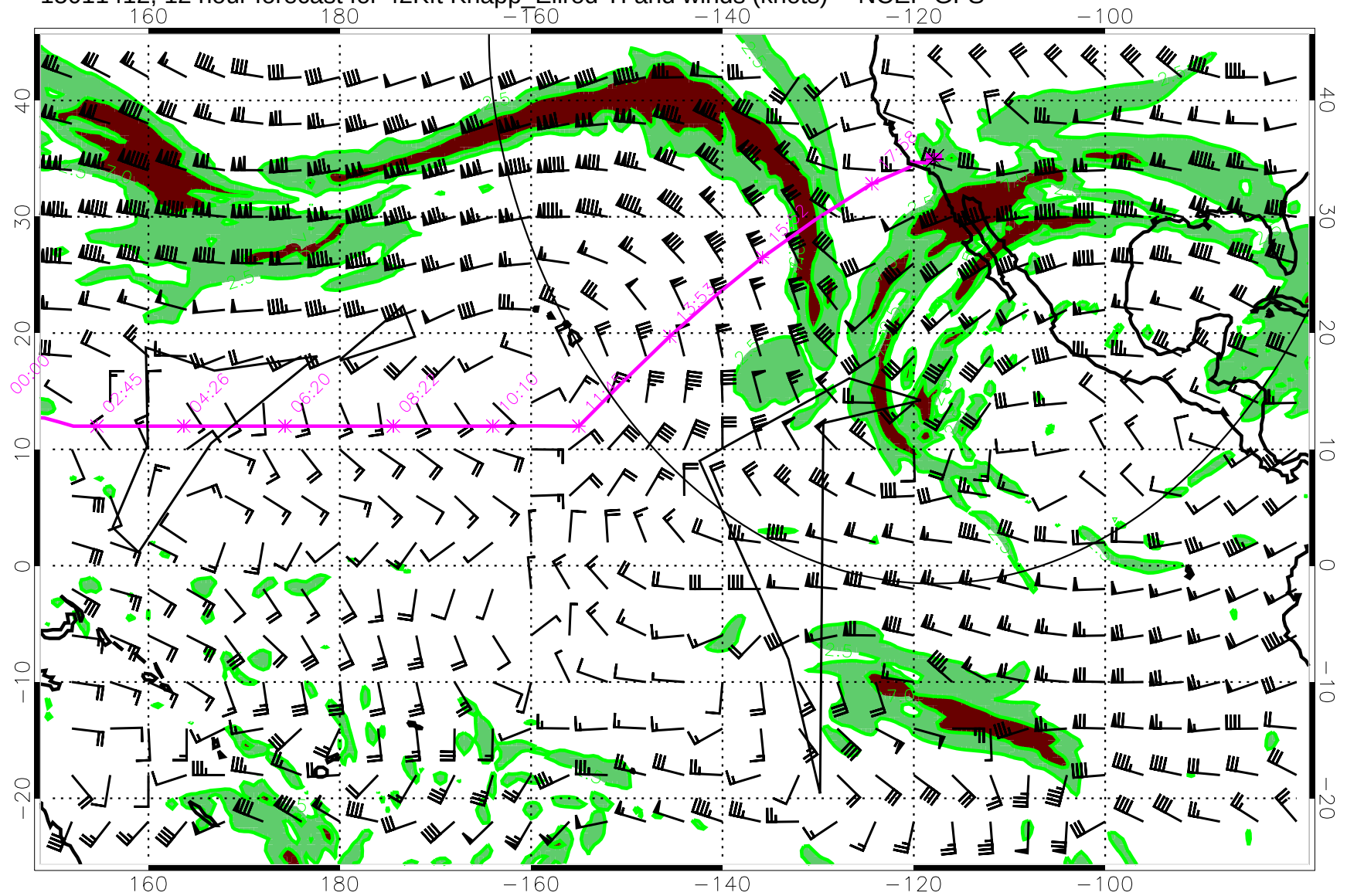
15011412, 12 hour forecast for 42Kft Knapp_Ellrod TI and winds (knots) -- NCEP GFS
