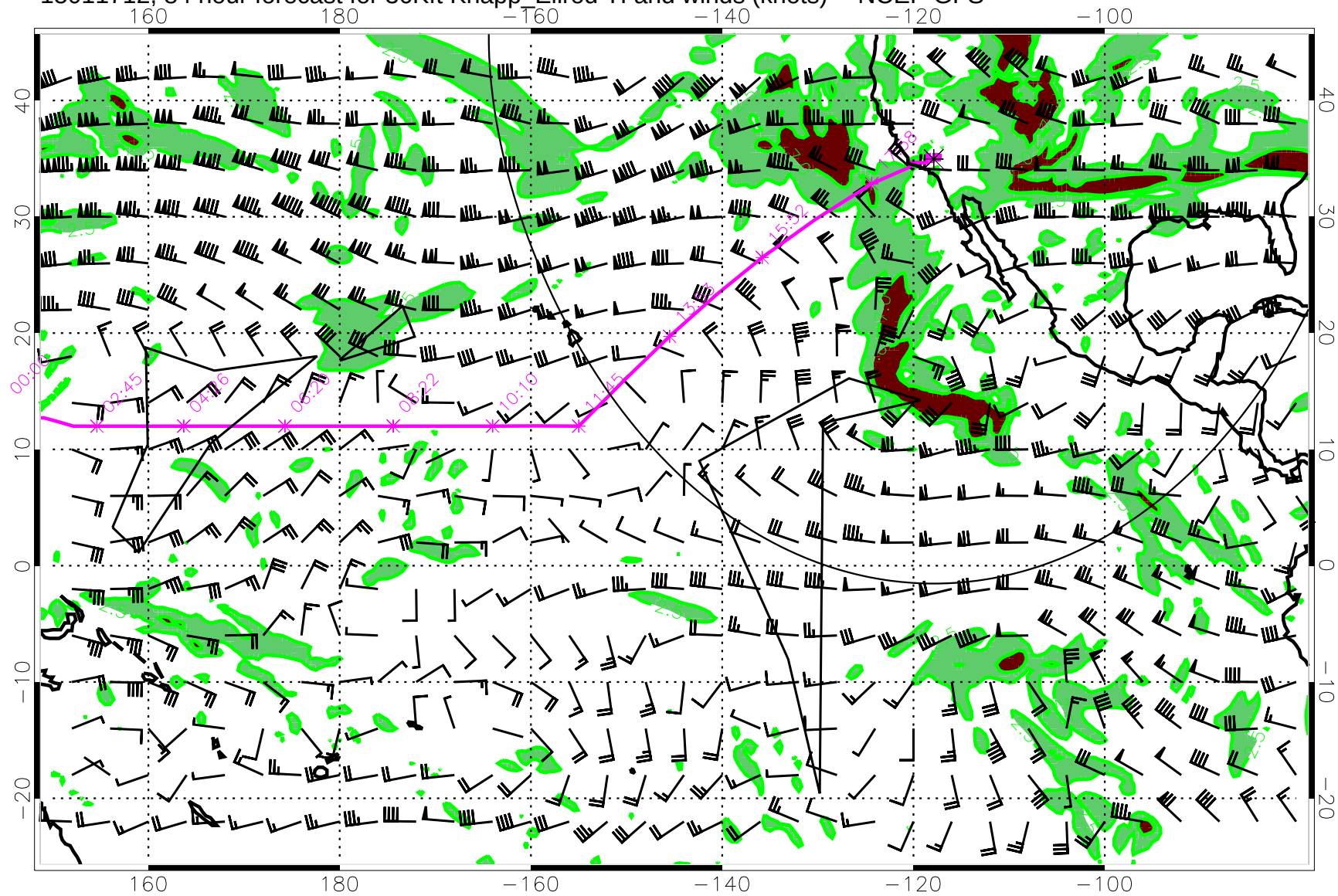
15011712, 84 hour forecast for 36Kft Knapp_Ellrod TI and winds (knots) -- NCEP GFS
