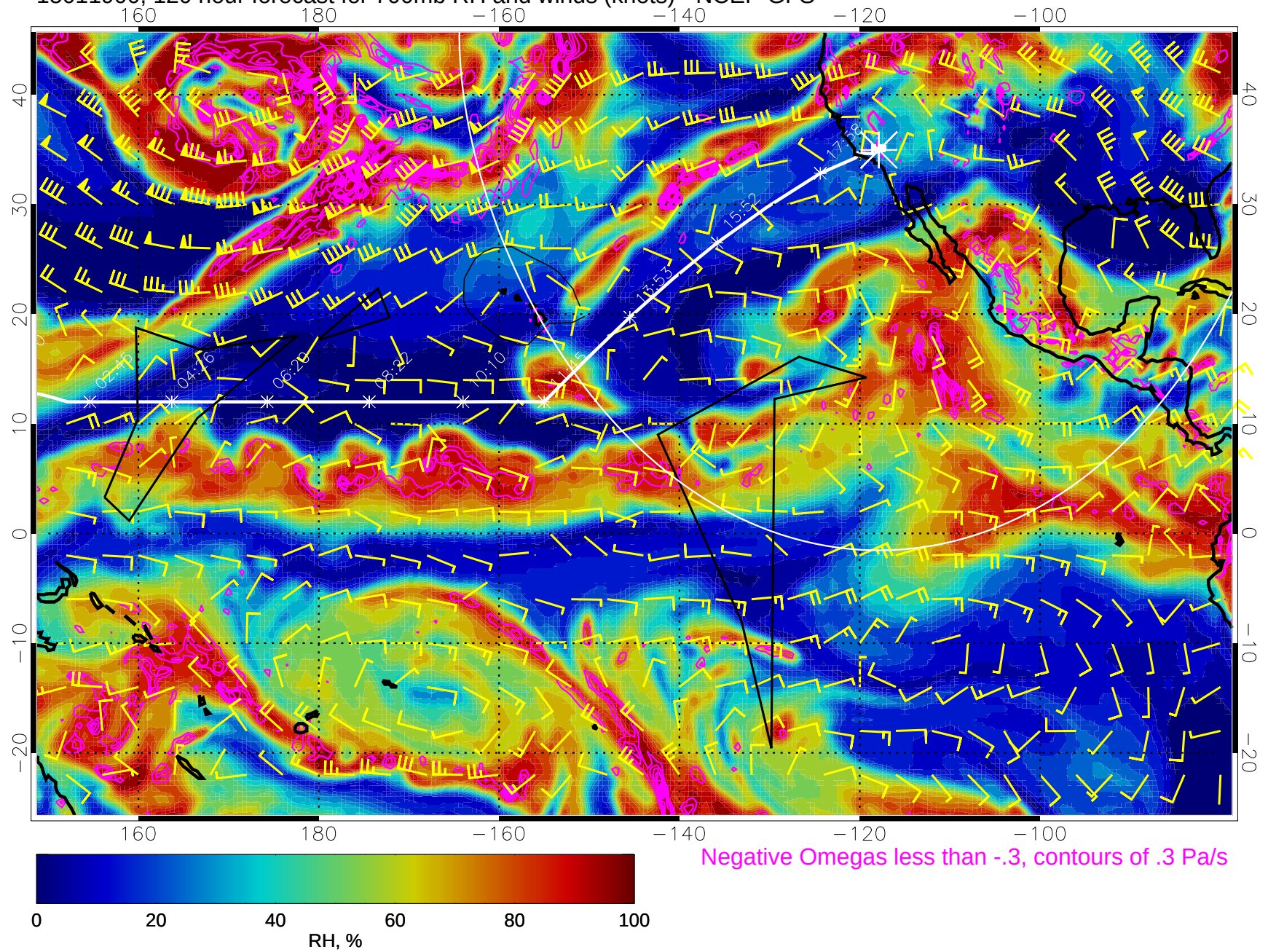
15011900, 120 hour forecast for 700mb RH and winds (knots) - NCEP GFS
