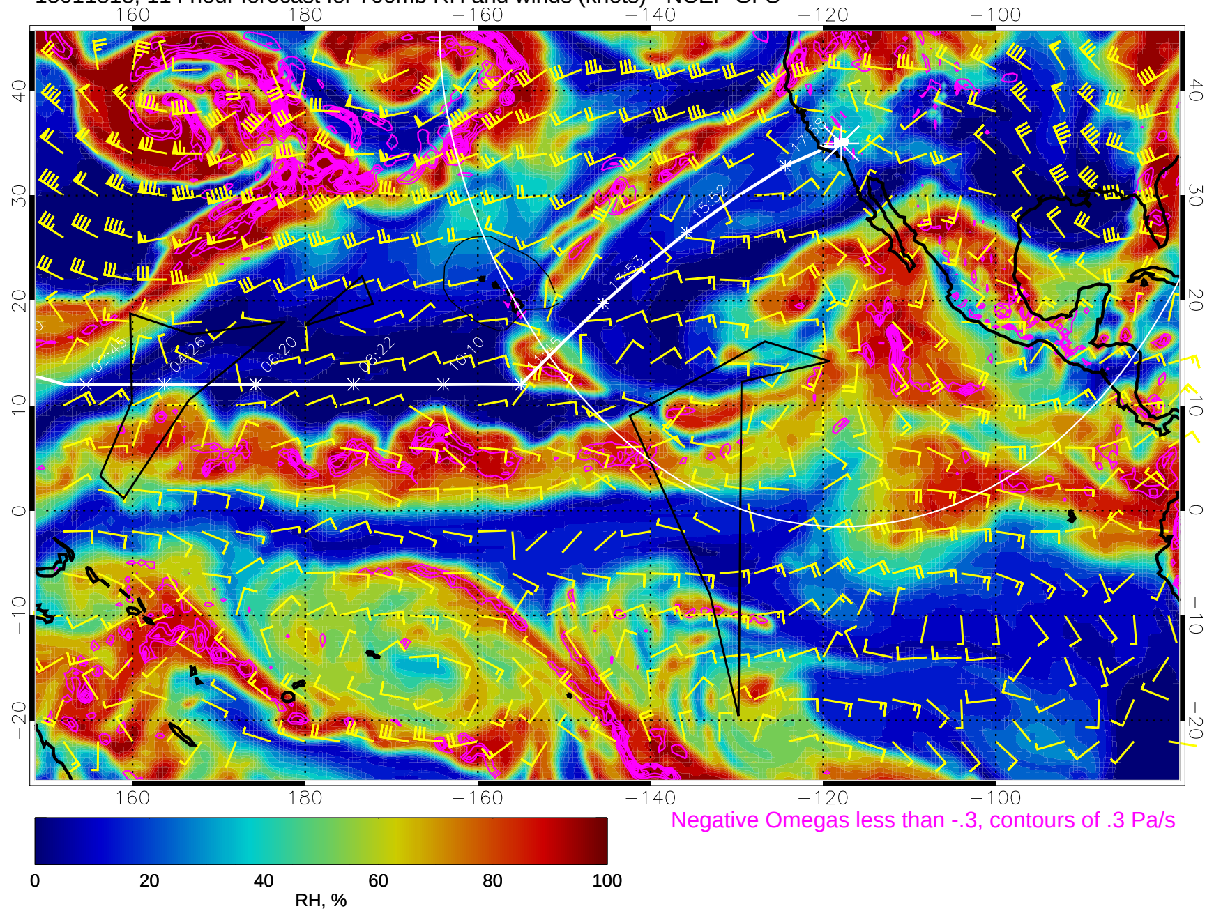
15011818, 114 hour forecast for 700mb RH and winds (knots) - NCEP GFS
