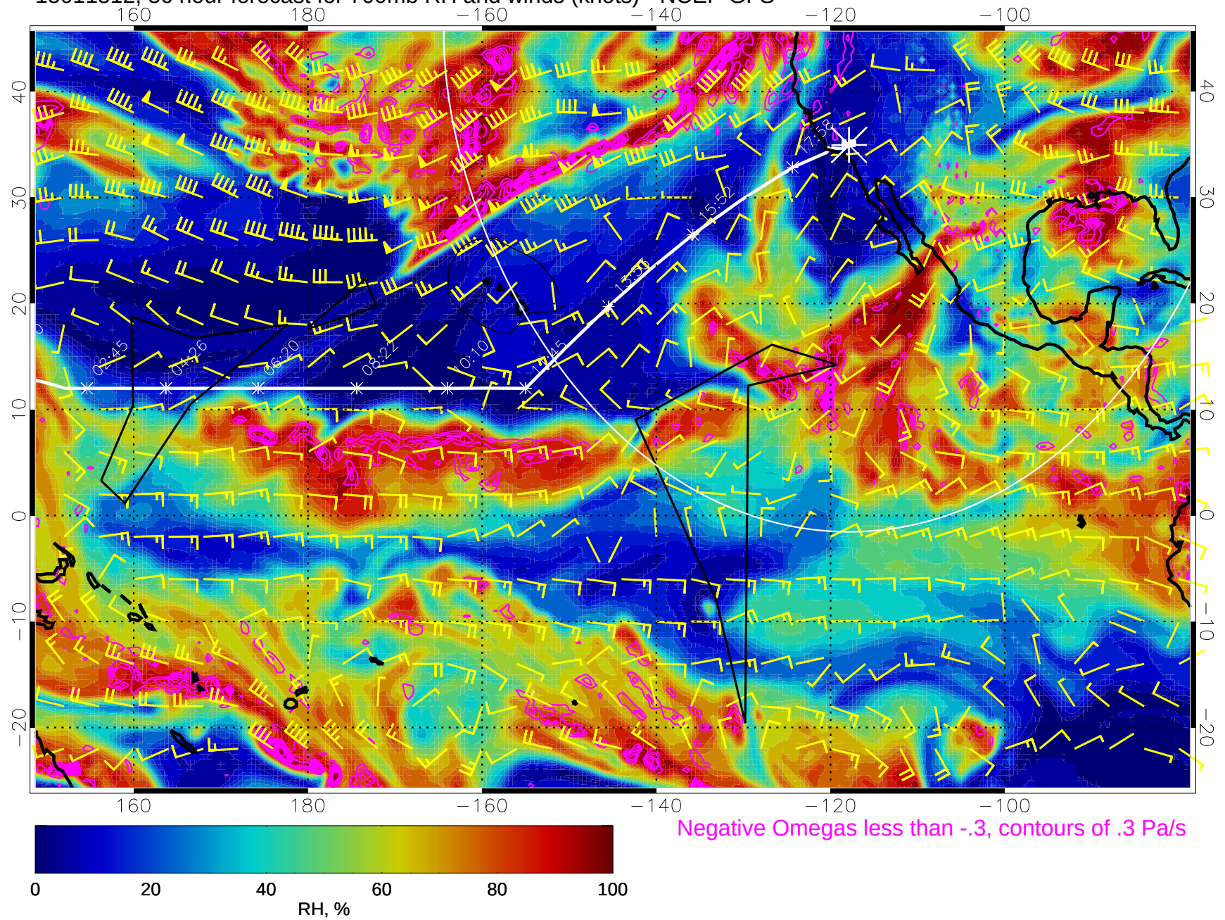
15011512, 36 hour forecast for 700mb RH and winds (knots) - NCEP GFS
