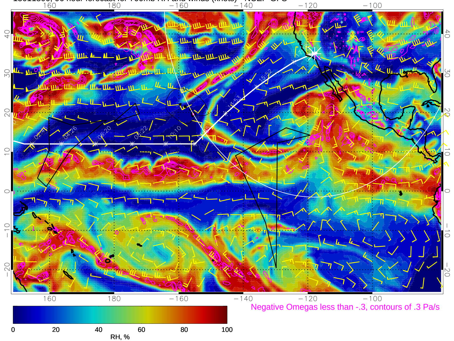
15011800, 96 hour forecast for 700mb RH and winds (knots) - NCEP GFS
