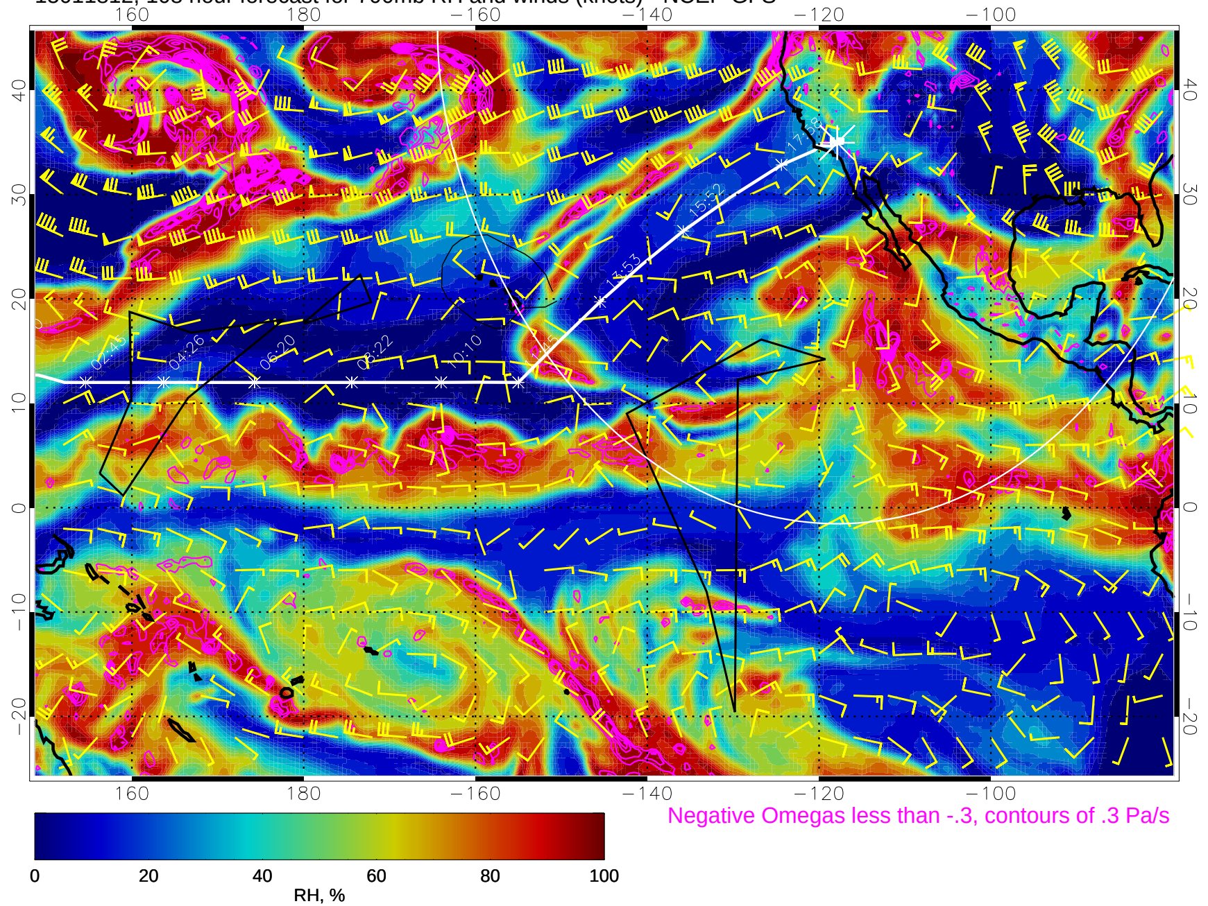
15011812, 108 hour forecast for 700mb RH and winds (knots) - NCEP GFS
