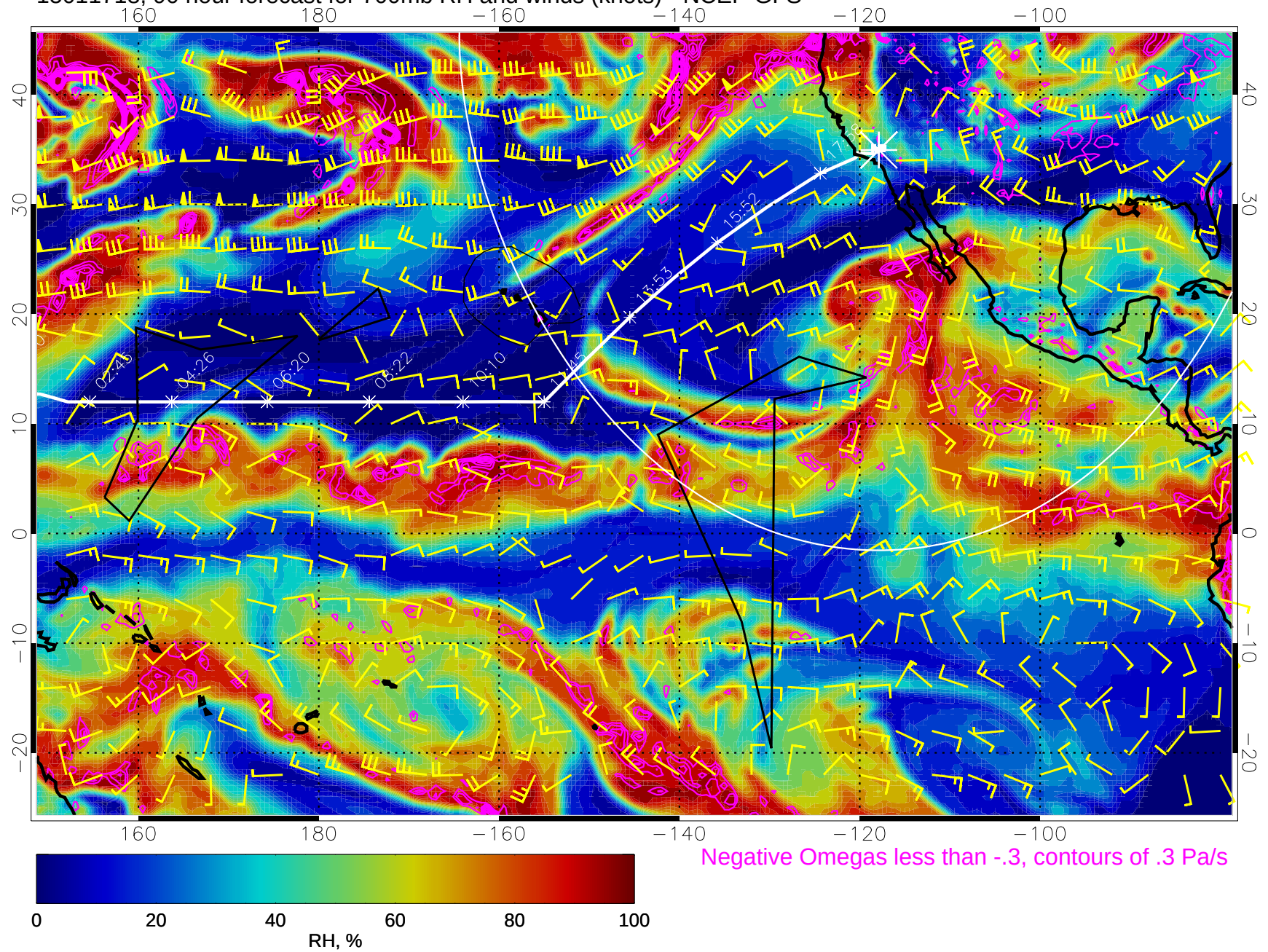
15011718, 90 hour forecast for 700mb RH and winds (knots) - NCEP GFS
