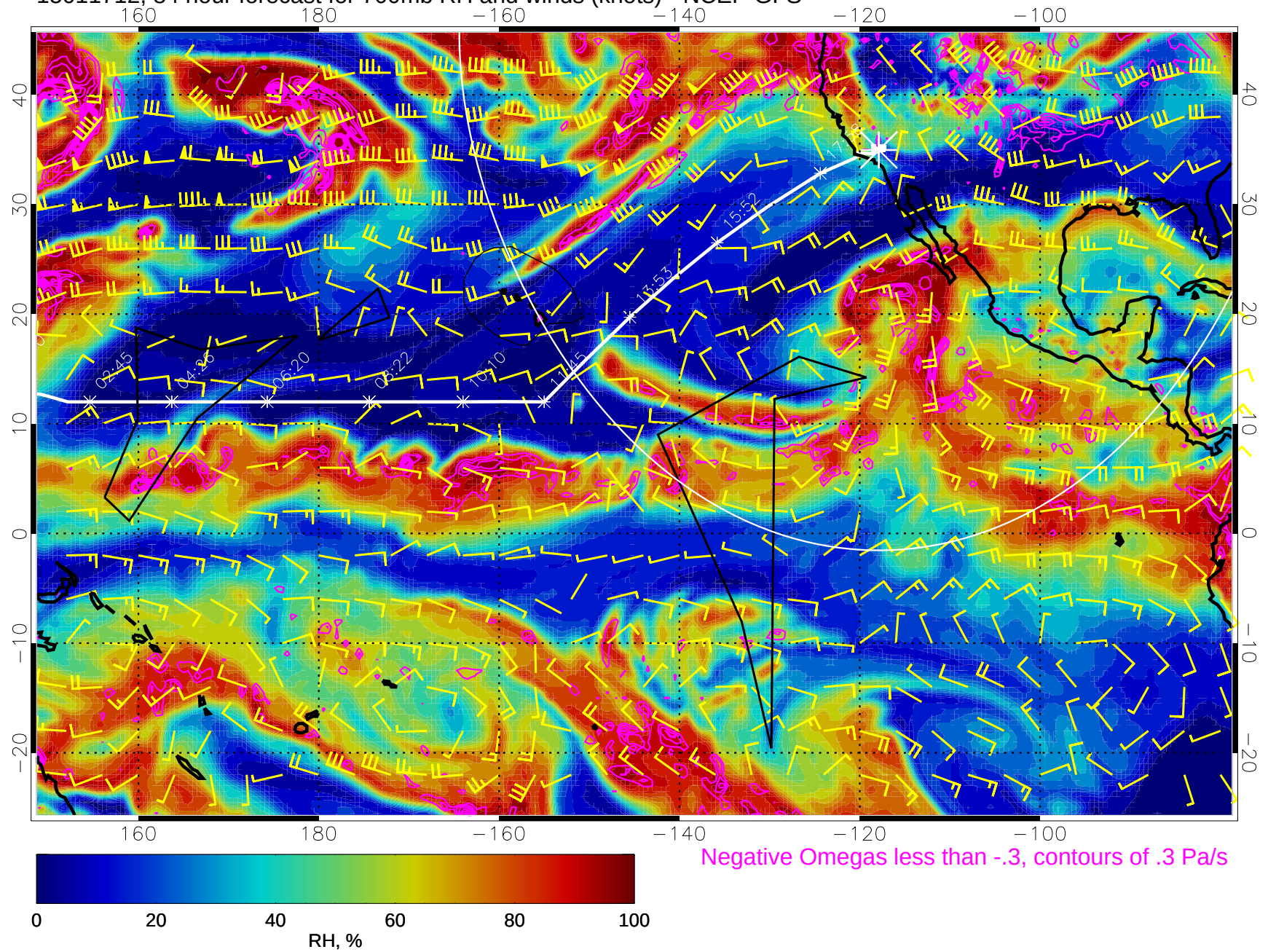
15011712, 84 hour forecast for 700mb RH and winds (knots) - NCEP GFS
