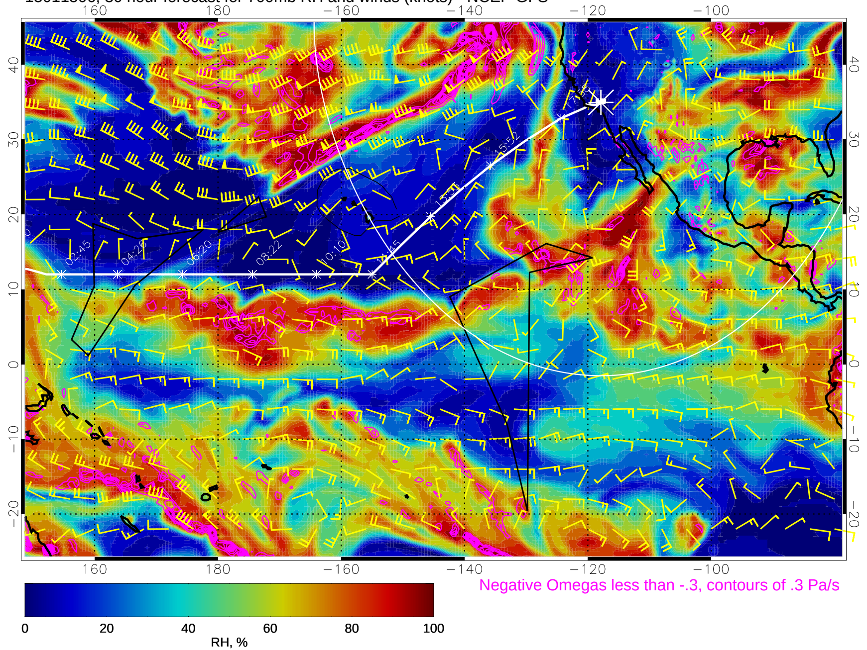
15011506, 30 hour forecast for 700mb RH and winds (knots) - NCEP GFS
