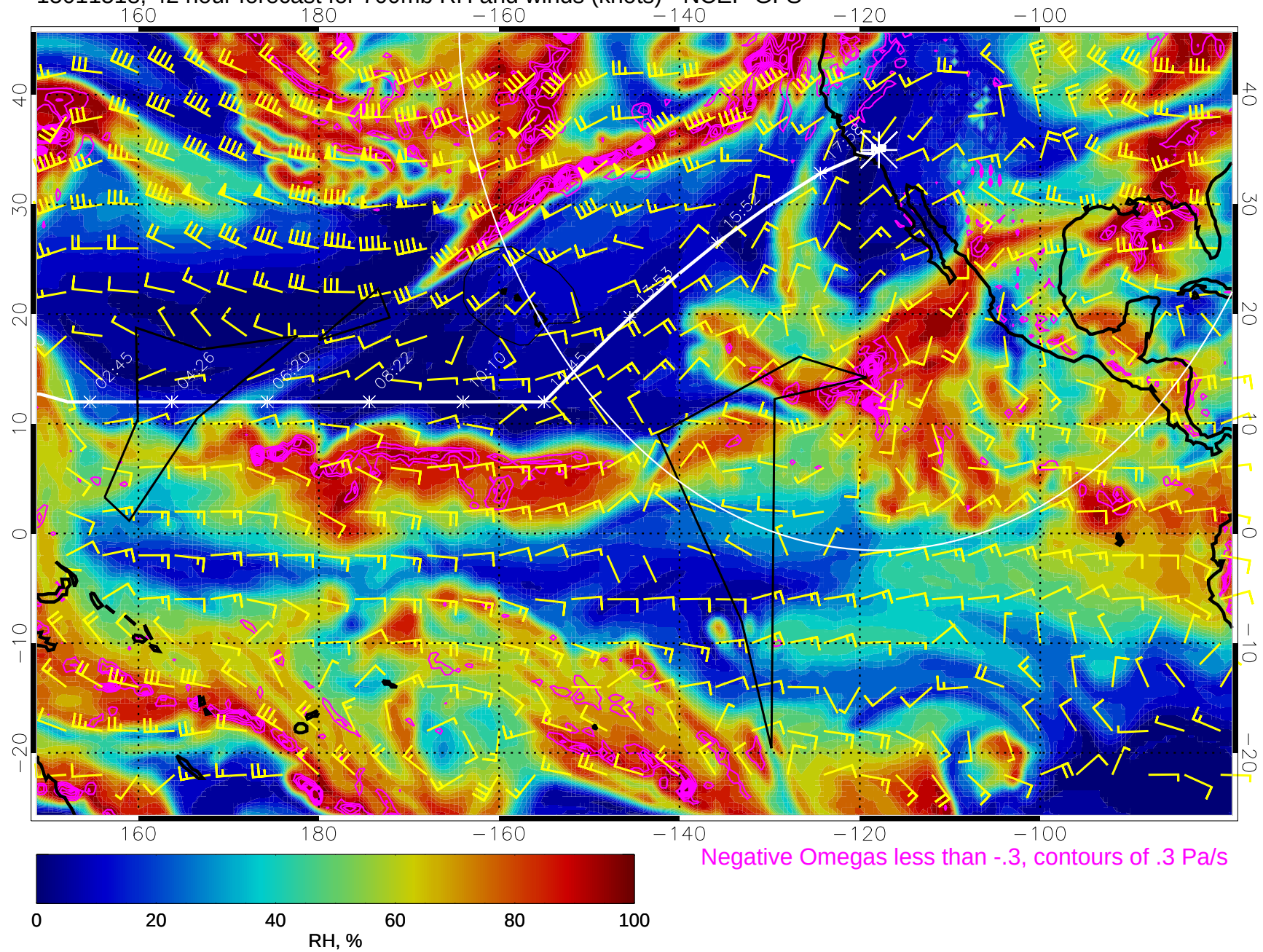
15011518, 42 hour forecast for 700mb RH and winds (knots) - NCEP GFS
