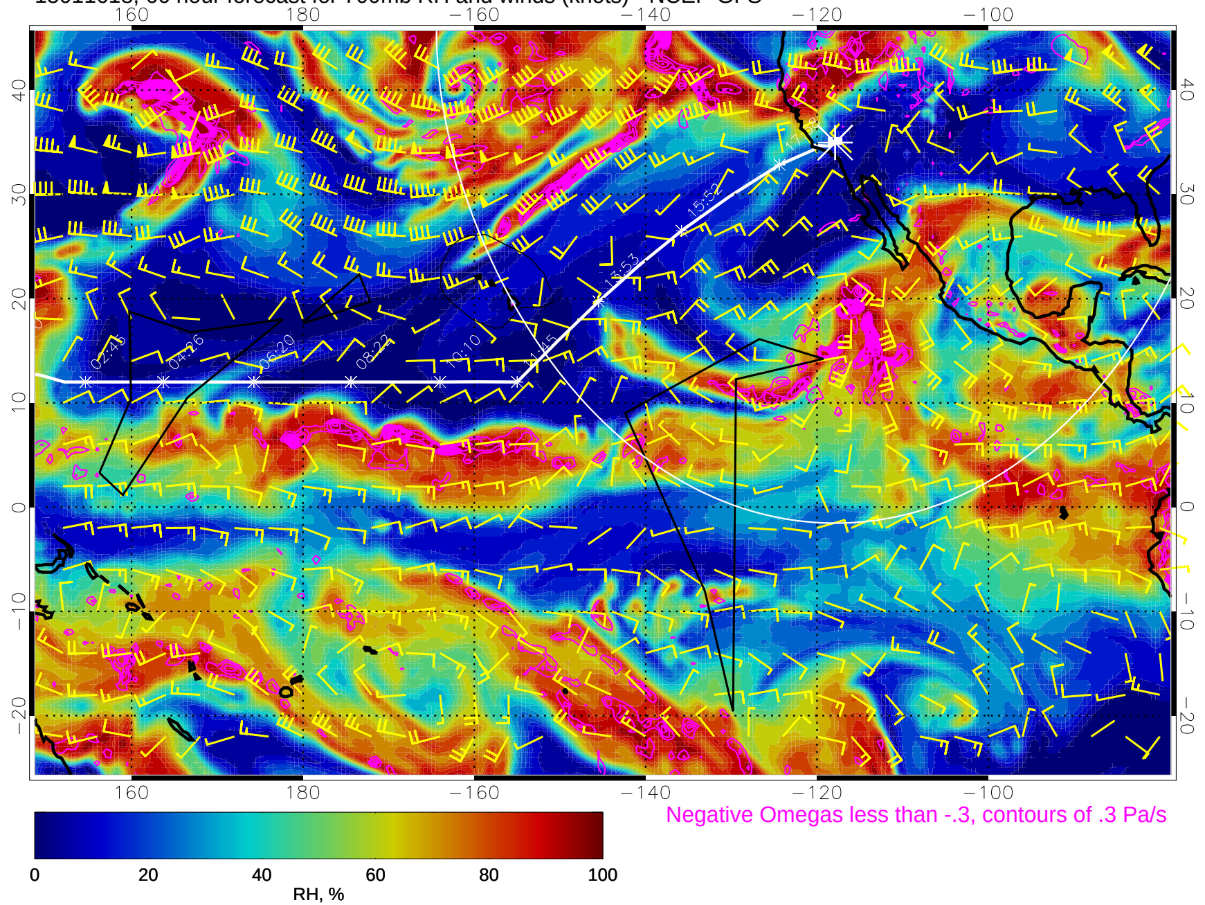
15011618, 66 hour forecast for 700mb RH and winds (knots) - NCEP GFS
