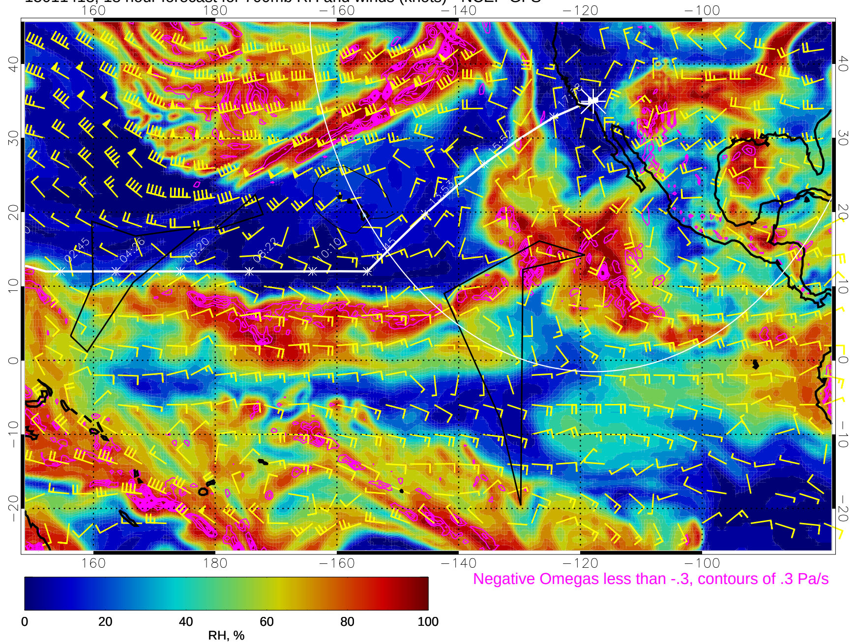
15011418, 18 hour forecast for 700mb RH and winds (knots) - NCEP GFS
