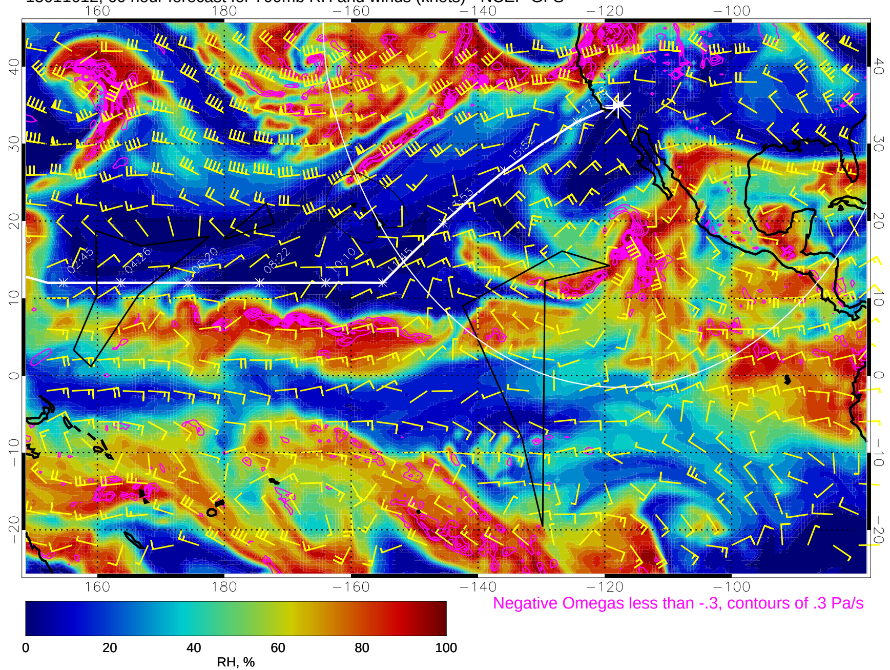
15011612, 60 hour forecast for 700mb RH and winds (knots) - NCEP GFS
