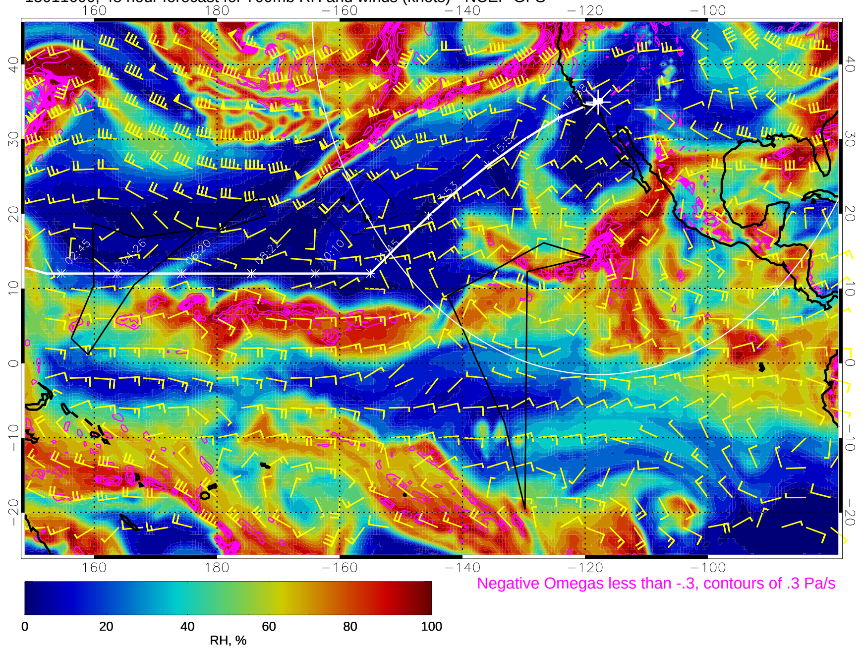
15011600, 48 hour forecast for 700mb RH and winds (knots) - NCEP GFS
