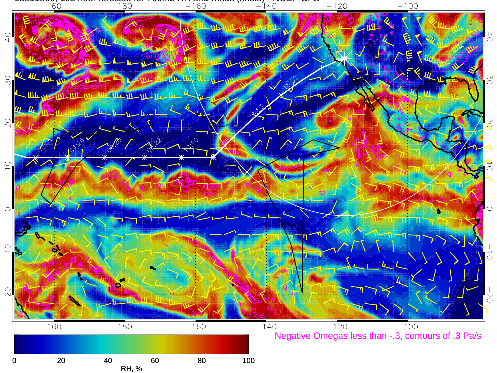
15011806, 102 hour forecast for 700mb RH and winds (knots) - NCEP GFS
