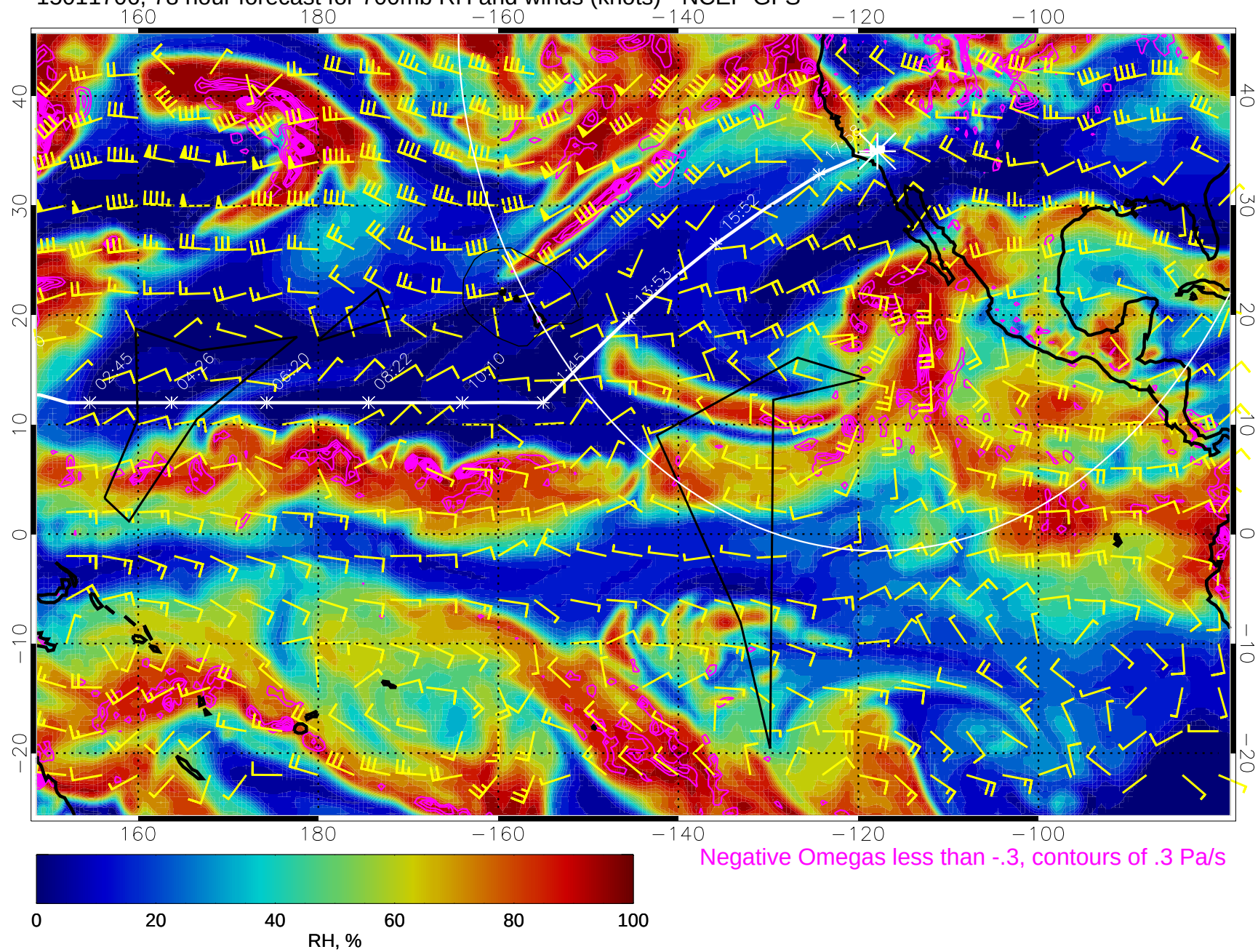
15011706, 78 hour forecast for 700mb RH and winds (knots) - NCEP GFS
