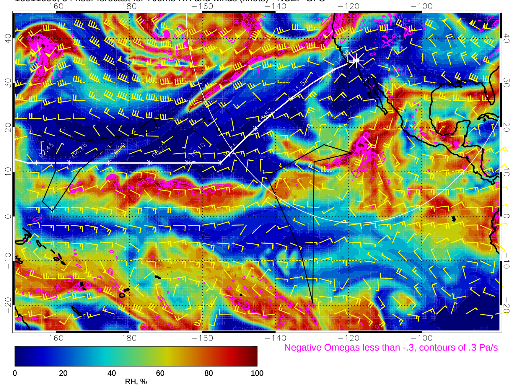
15011606, 54 hour forecast for 700mb RH and winds (knots) - NCEP GFS
