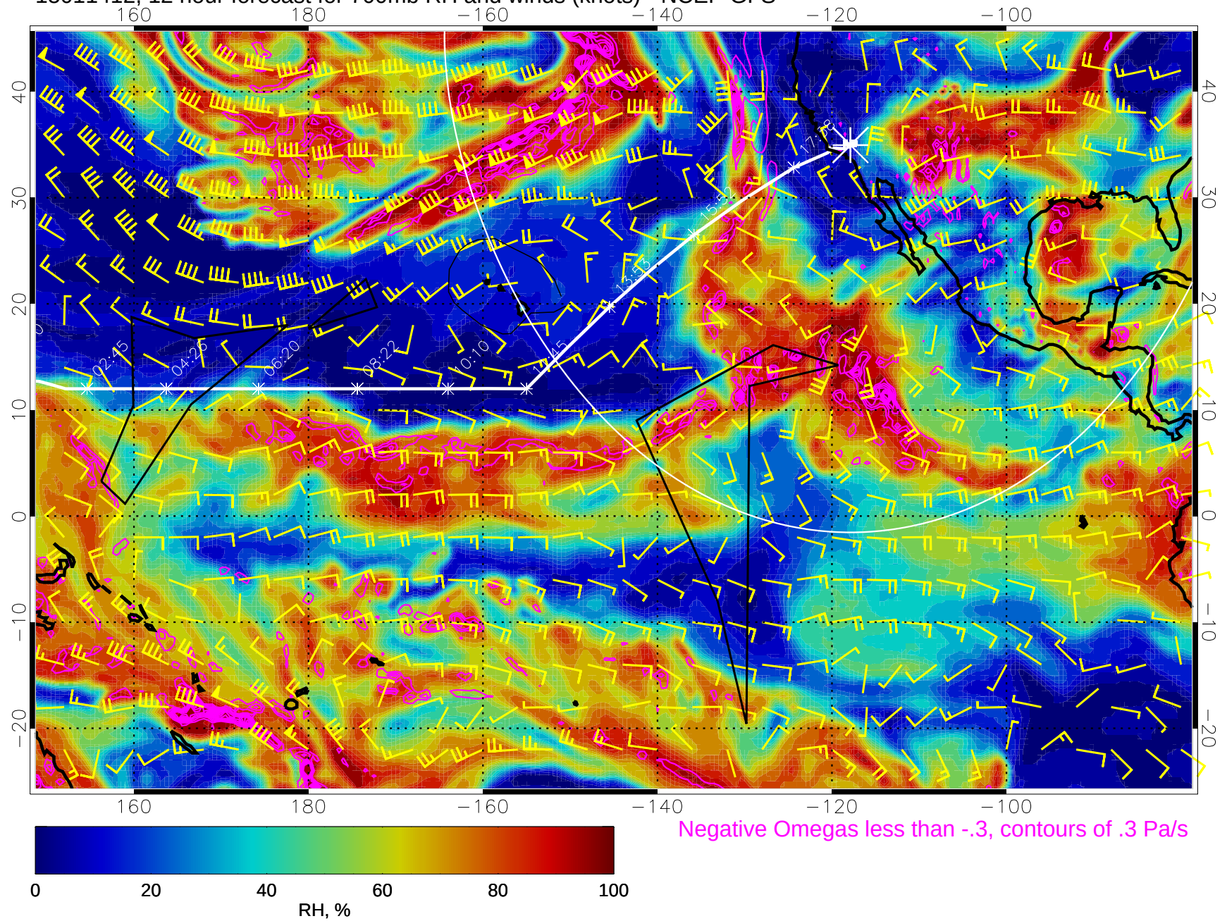
15011412, 12 hour forecast for 700mb RH and winds (knots) - NCEP GFS
