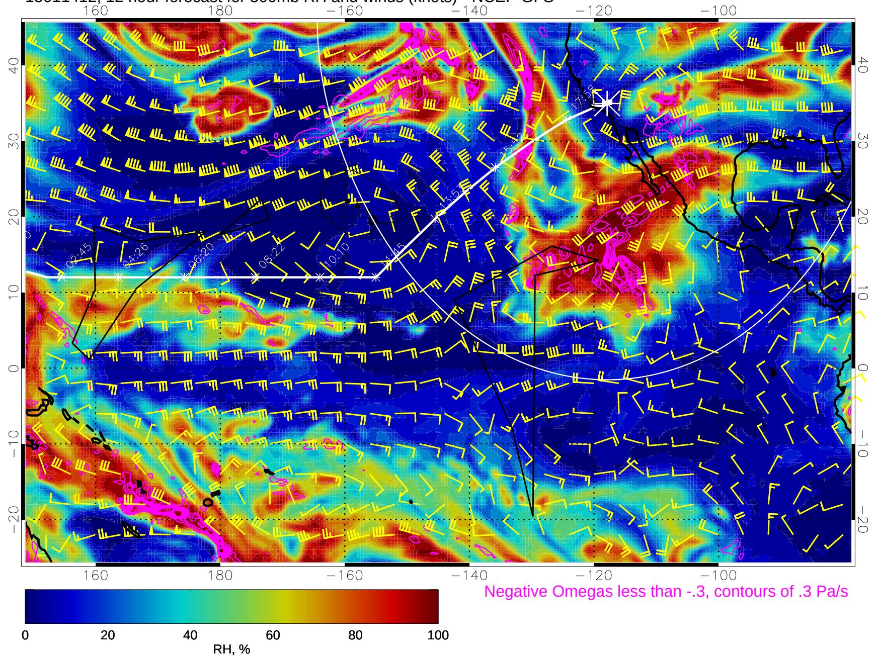
15011412, 12 hour forecast for 500mb RH and winds (knots) - NCEP GFS
