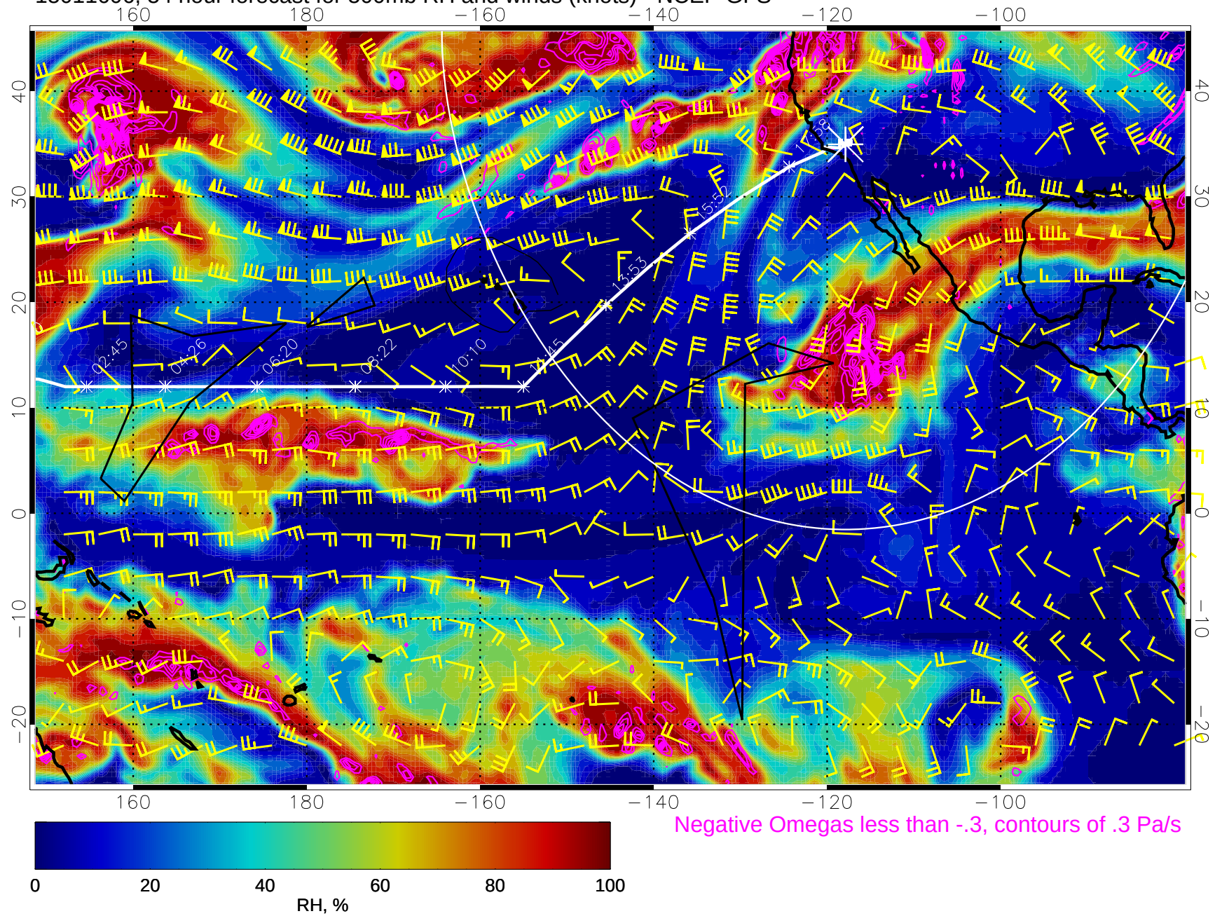
15011606, 54 hour forecast for 500mb RH and winds (knots) - NCEP GFS
