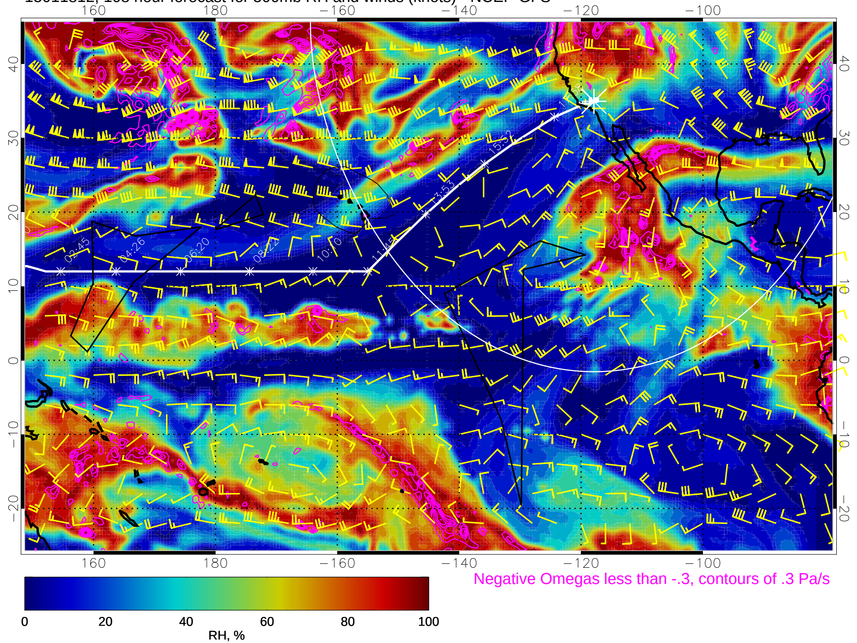
15011812, 108 hour forecast for 500mb RH and winds (knots) - NCEP GFS
