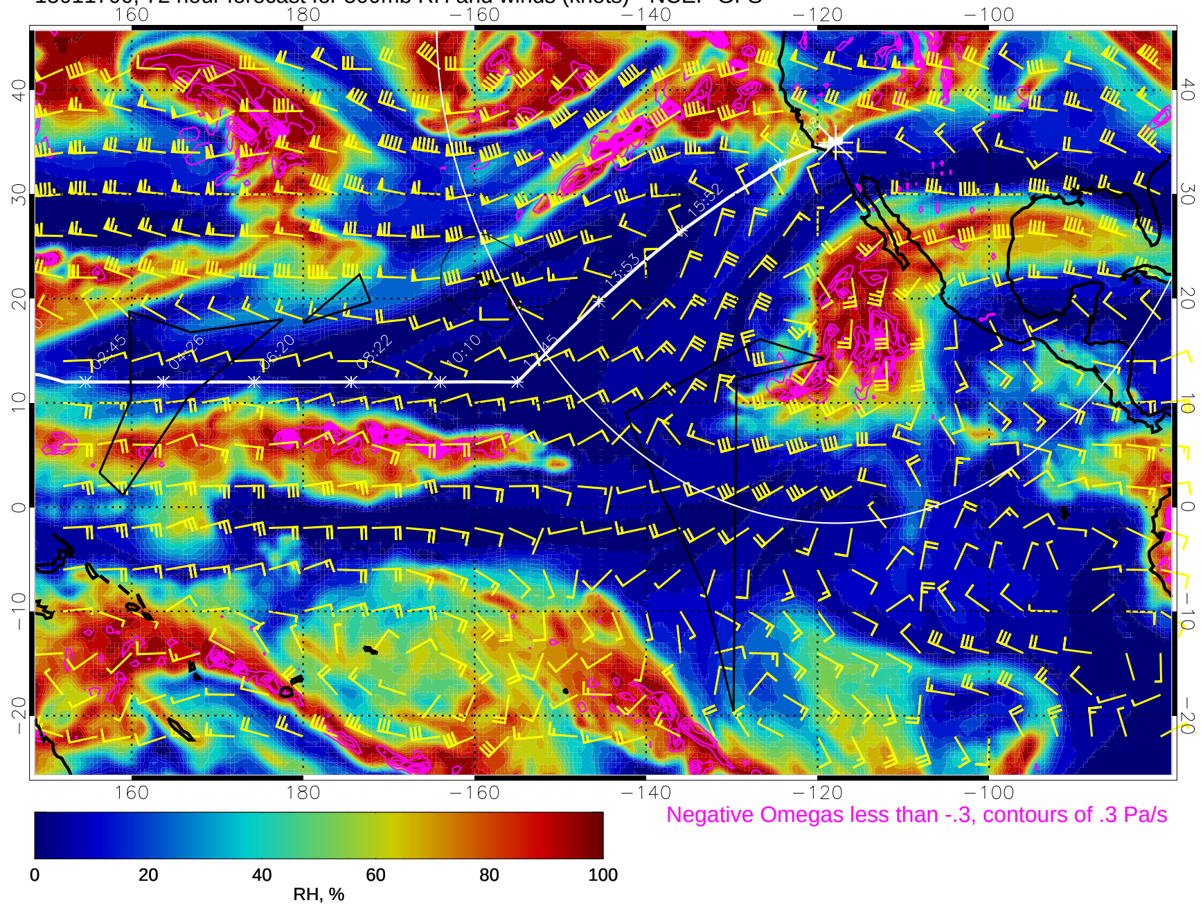
15011700, 72 hour forecast for 500mb RH and winds (knots) - NCEP GFS
