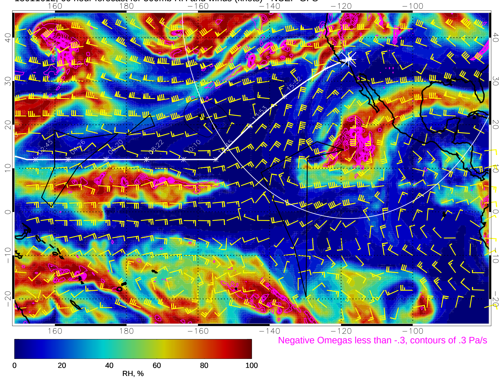
15011612, 60 hour forecast for 500mb RH and winds (knots) - NCEP GFS
