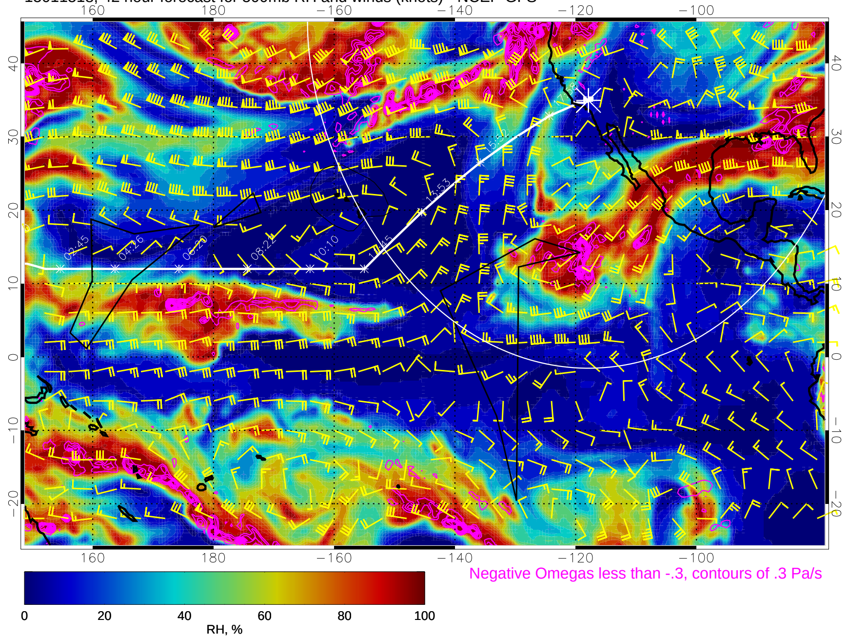
15011518, 42 hour forecast for 500mb RH and winds (knots) - NCEP GFS
