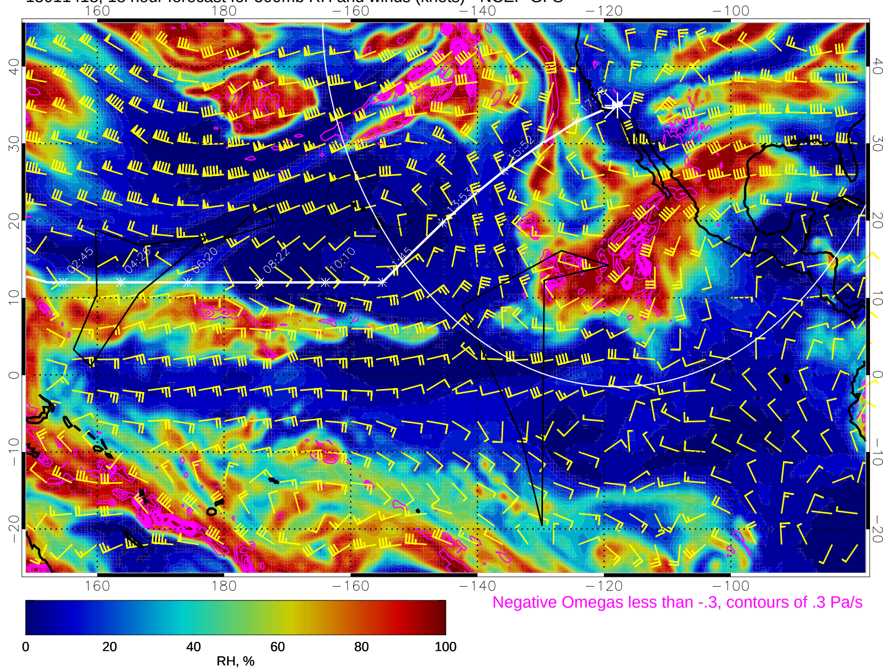
15011418, 18 hour forecast for 500mb RH and winds (knots) - NCEP GFS
