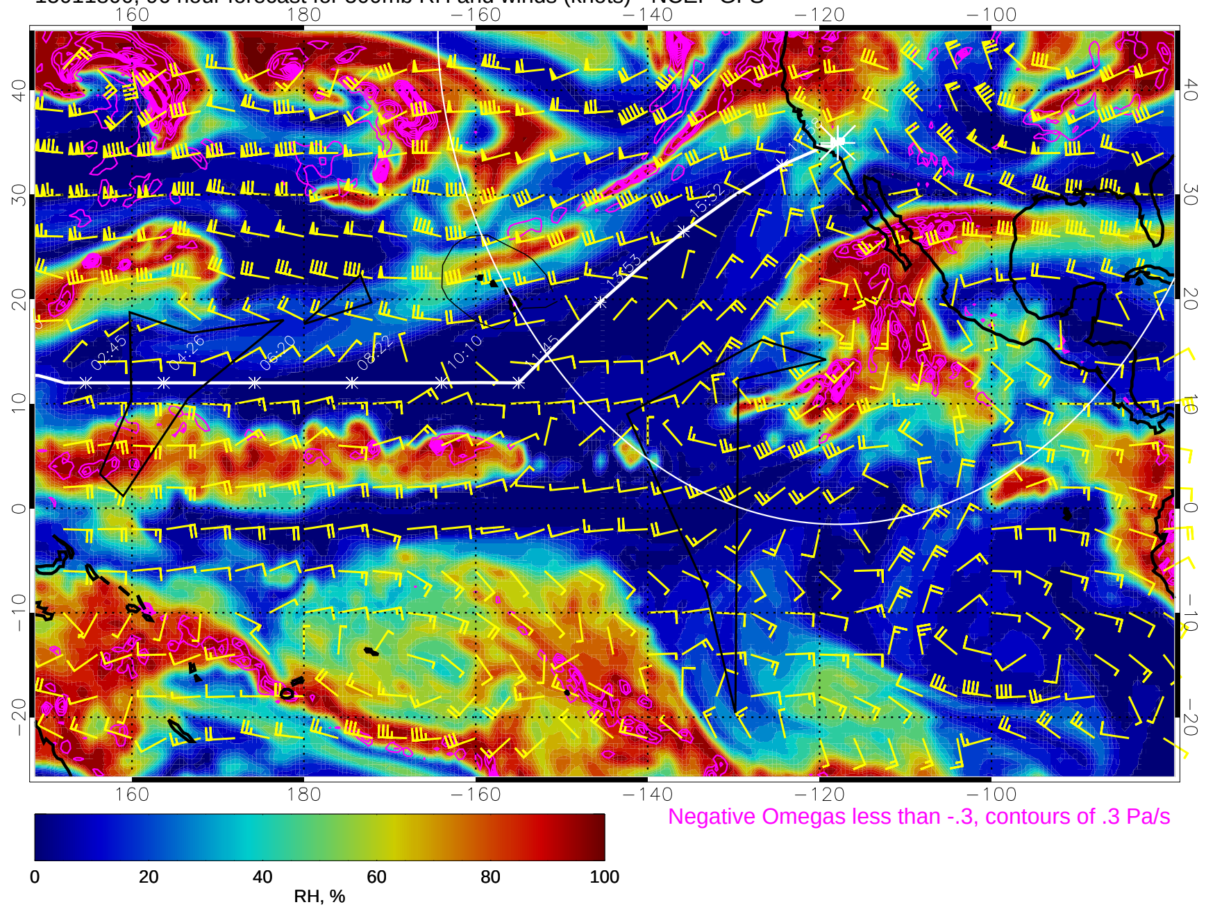
15011800, 96 hour forecast for 500mb RH and winds (knots) - NCEP GFS
