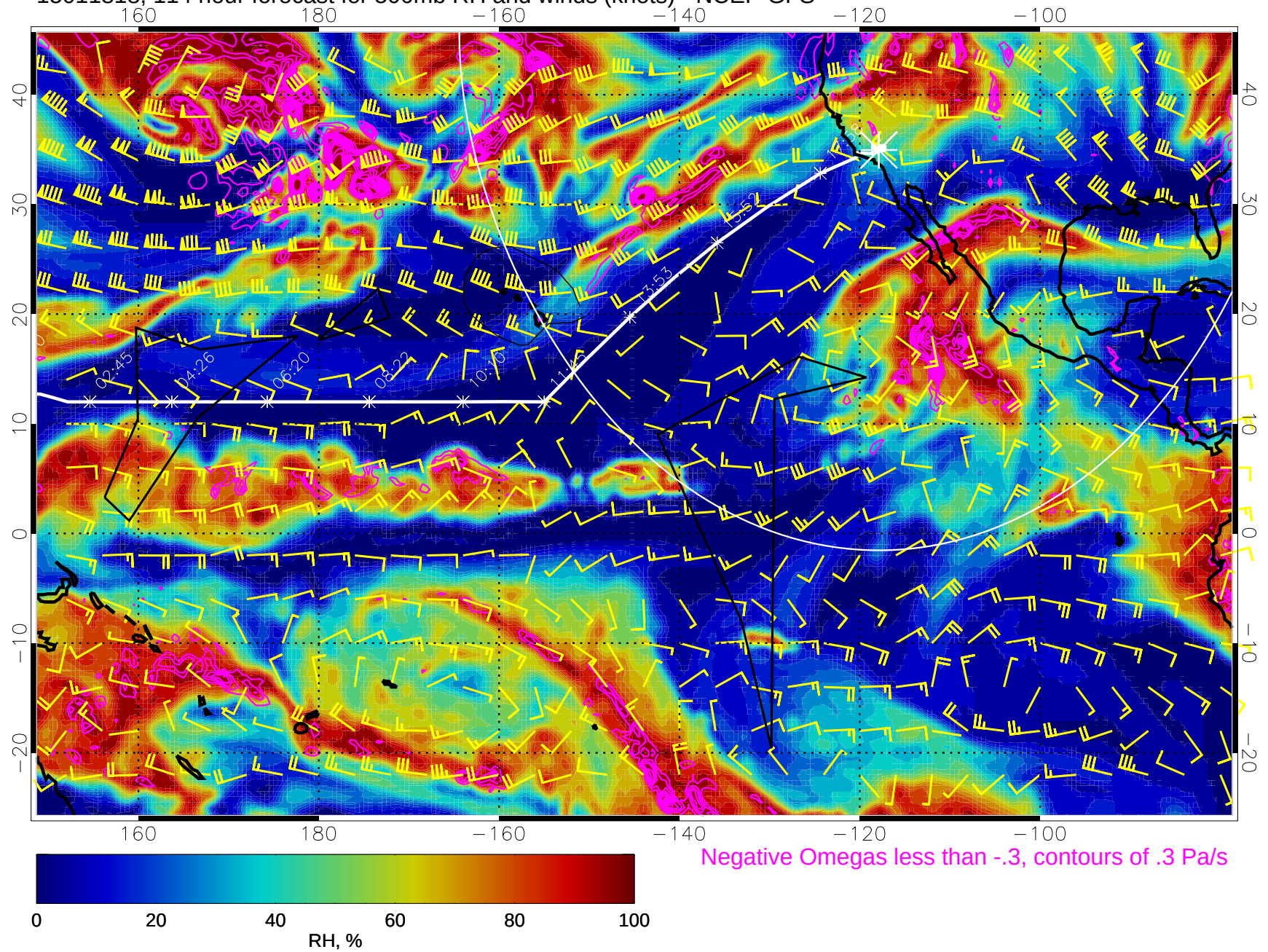
15011818, 114 hour forecast for 500mb RH and winds (knots) - NCEP GFS
