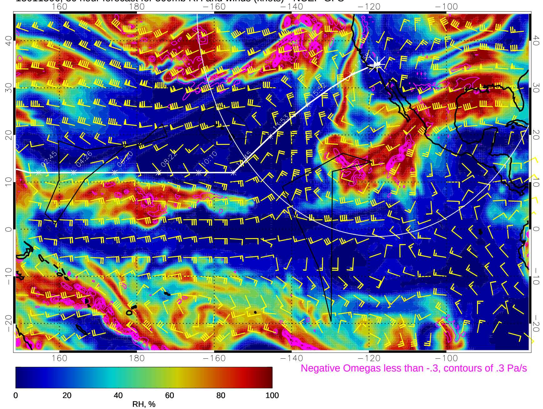
15011506, 30 hour forecast for 500mb RH and winds (knots) - NCEP GFS
