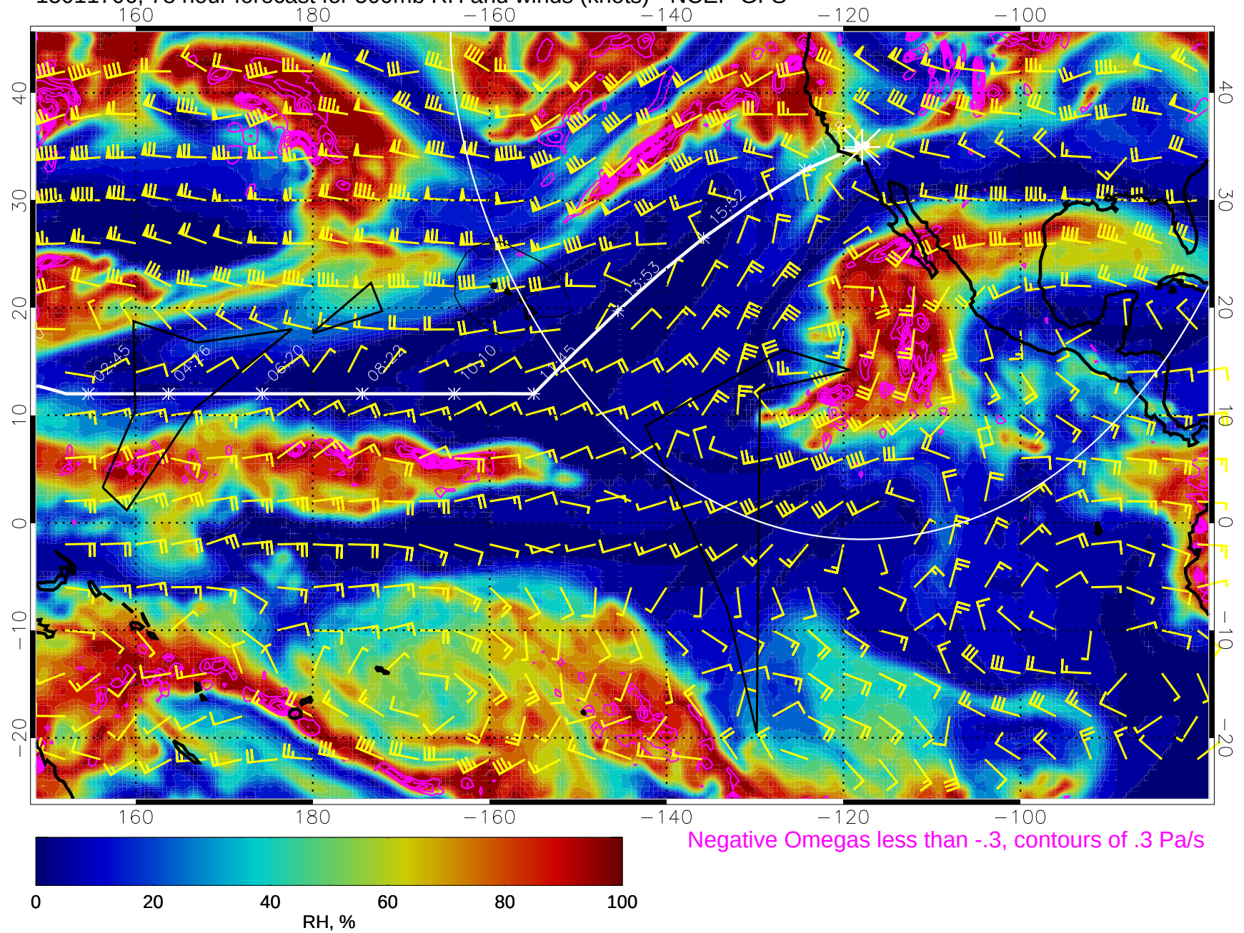
15011706, 78 hour forecast for 500mb RH and winds (knots) - NCEP GFS
