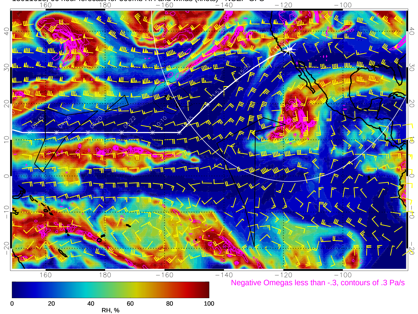
15011618, 66 hour forecast for 500mb RH and winds (knots) - NCEP GFS
