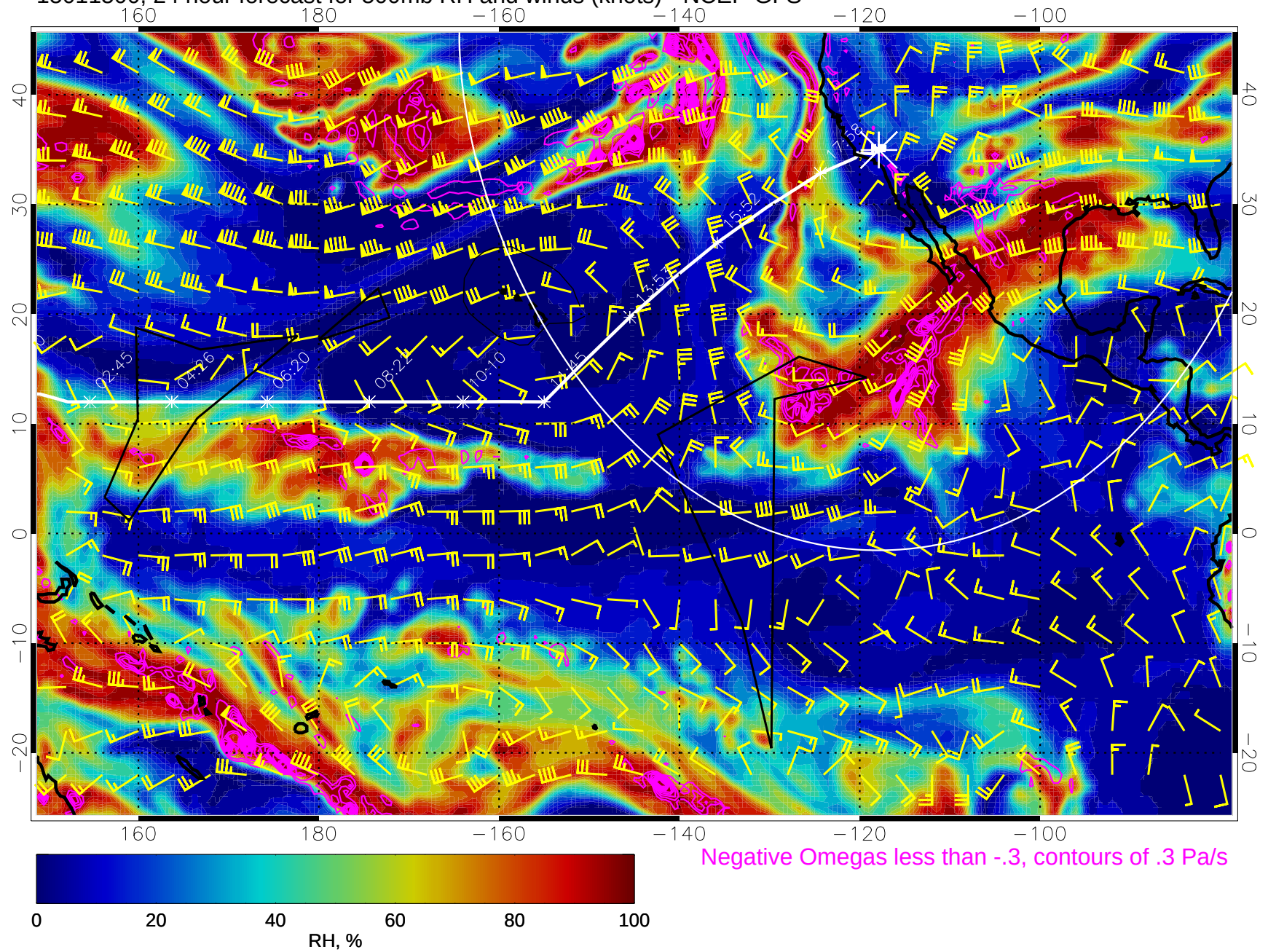
15011500, 24 hour forecast for 500mb RH and winds (knots) - NCEP GFS
