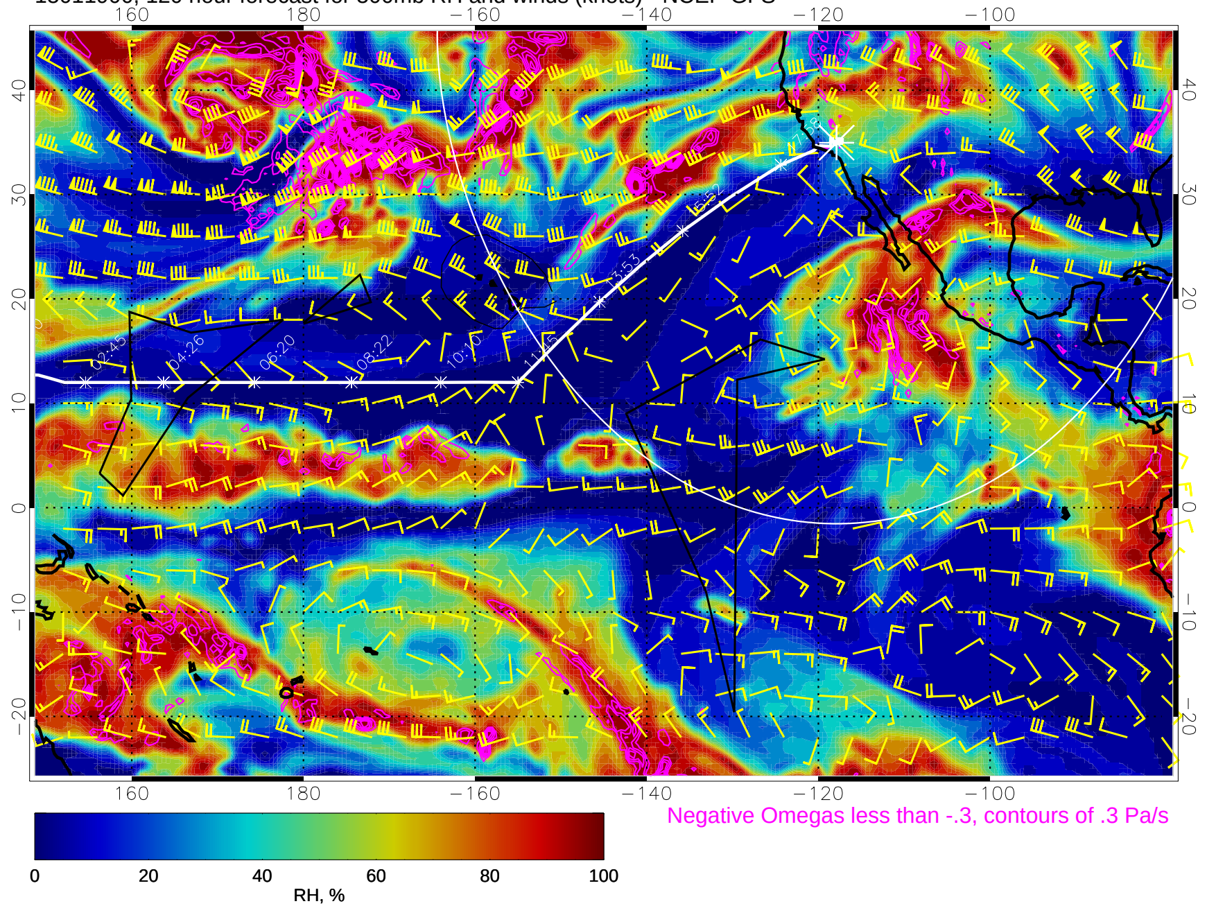
15011900, 120 hour forecast for 500mb RH and winds (knots) - NCEP GFS
