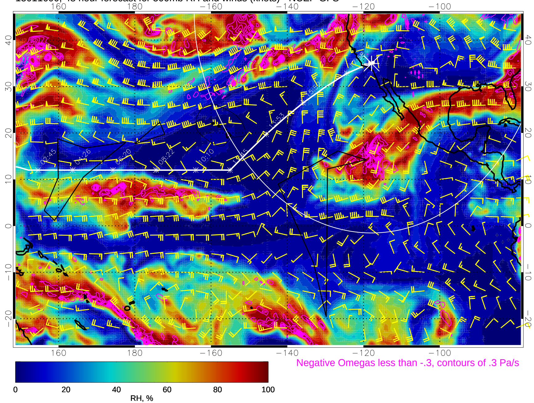
15011600, 48 hour forecast for 500mb RH and winds (knots) - NCEP GFS
