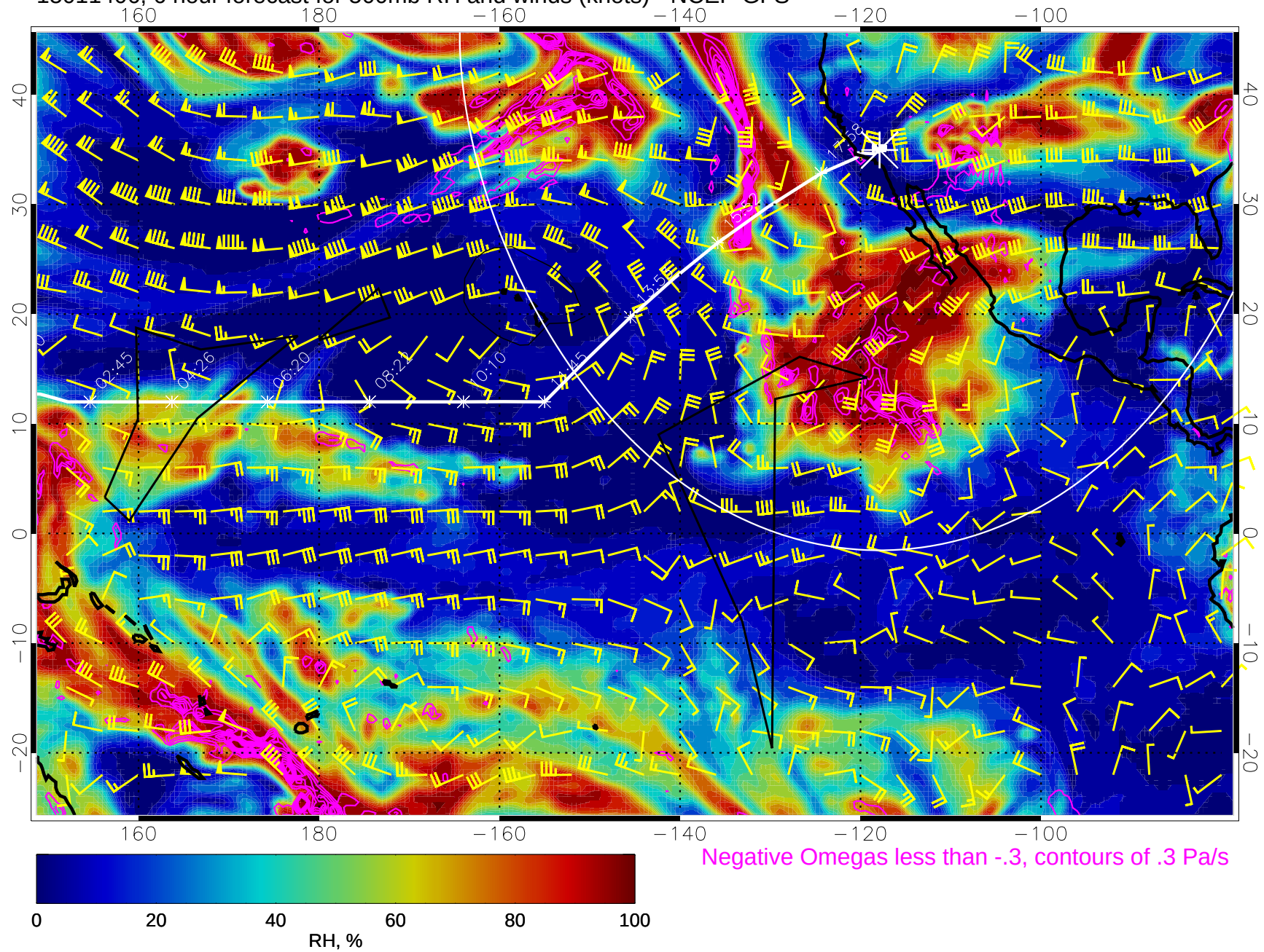
15011406, 6 hour forecast for 500mb RH and winds (knots) - NCEP GFS
