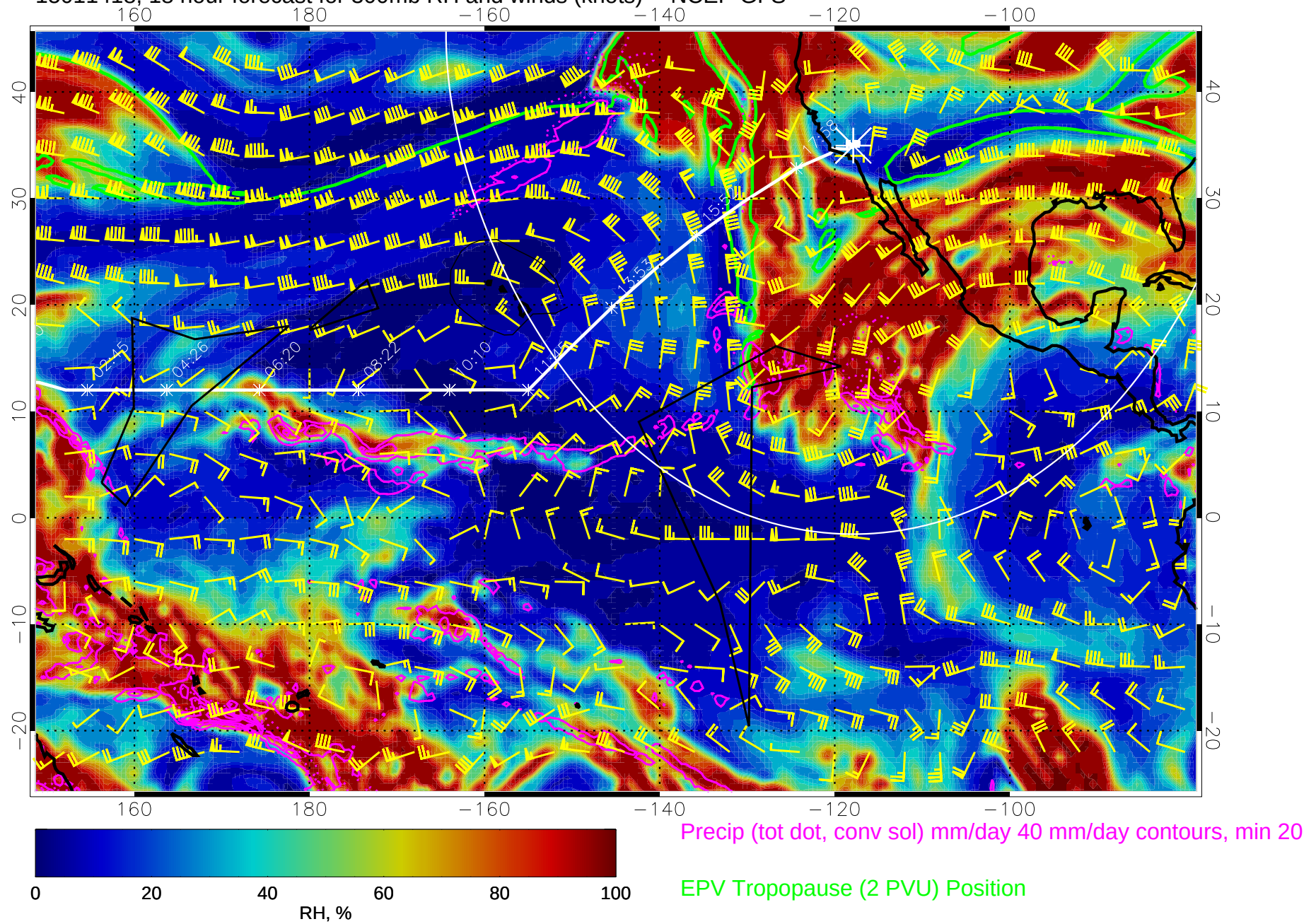
15011418, 18 hour forecast for 300mb RH and winds (knots) -- NCEP GFS
