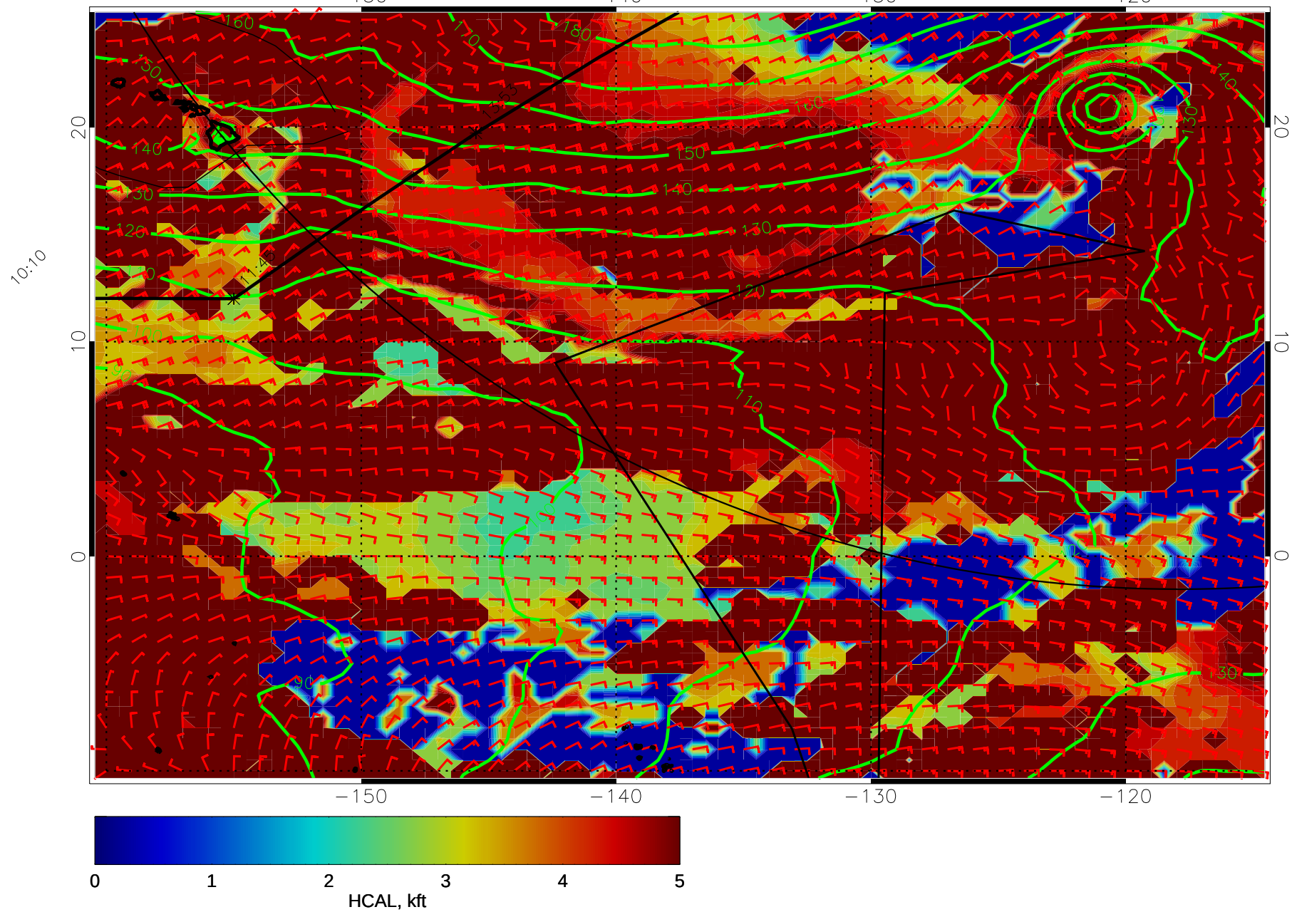
15011806, 102 hour forecast for HCAL, 1000mb Z, and winds (knots) -- NCEP GFS
