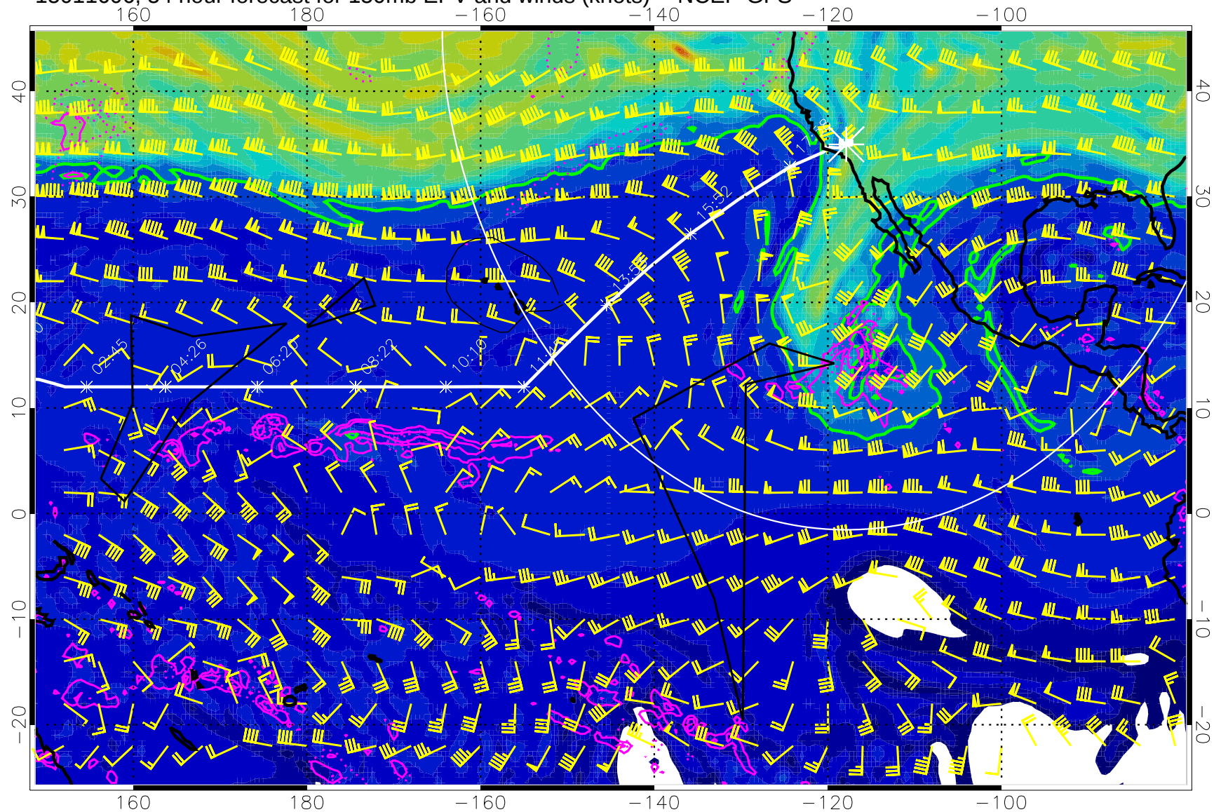
15011606, 54 hour forecast for 150mb EPV and winds (knots) -- NCEP GFS
