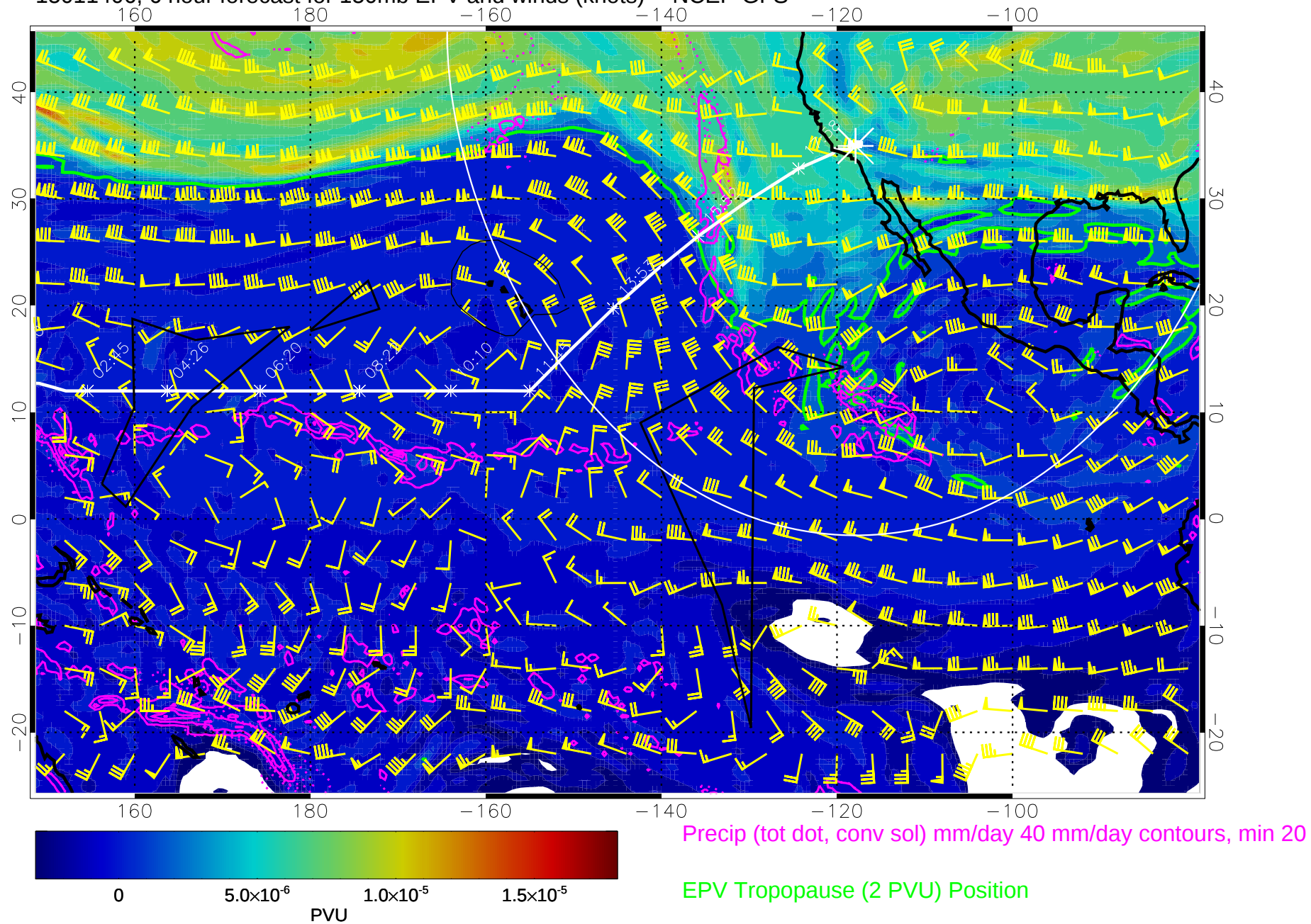
15011406, 6 hour forecast for 150mb EPV and winds (knots) -- NCEP GFS
