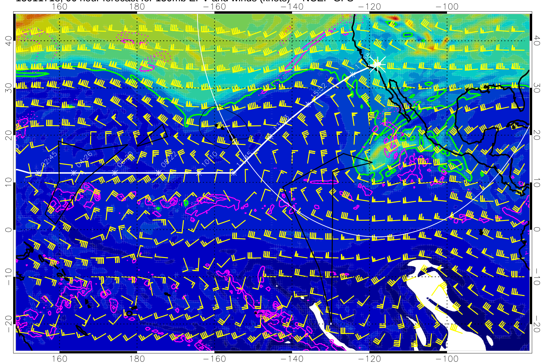
15011718, 90 hour forecast for 150mb EPV and winds (knots) -- NCEP GFS
