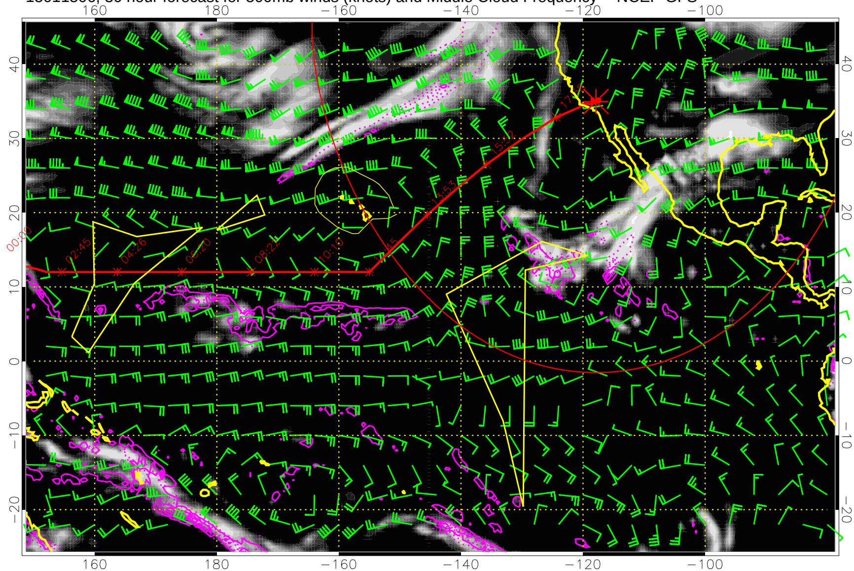
15011506, 30 hour forecast for 500mb winds (knots) and Middle Cloud Frequency -- NCEP GFS
