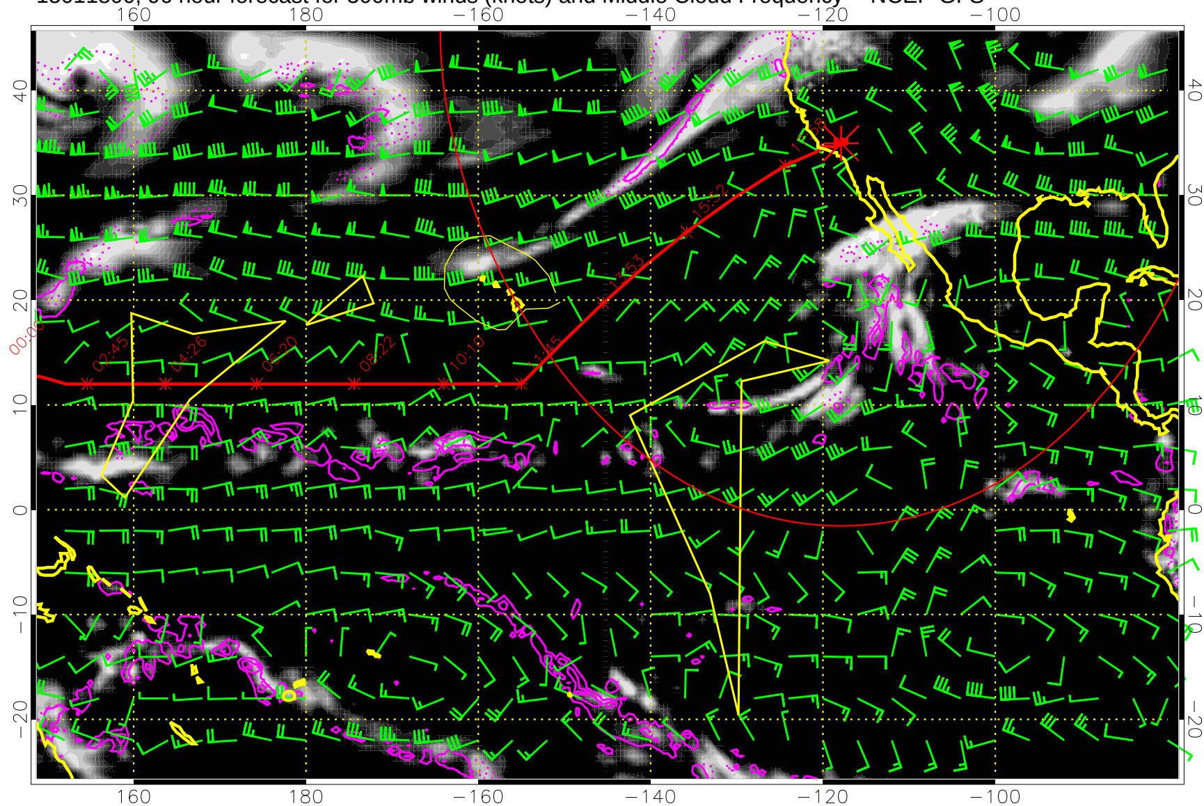
15011800, 96 hour forecast for 500mb winds (knots) and Middle Cloud Frequency -- NCEP GFS
