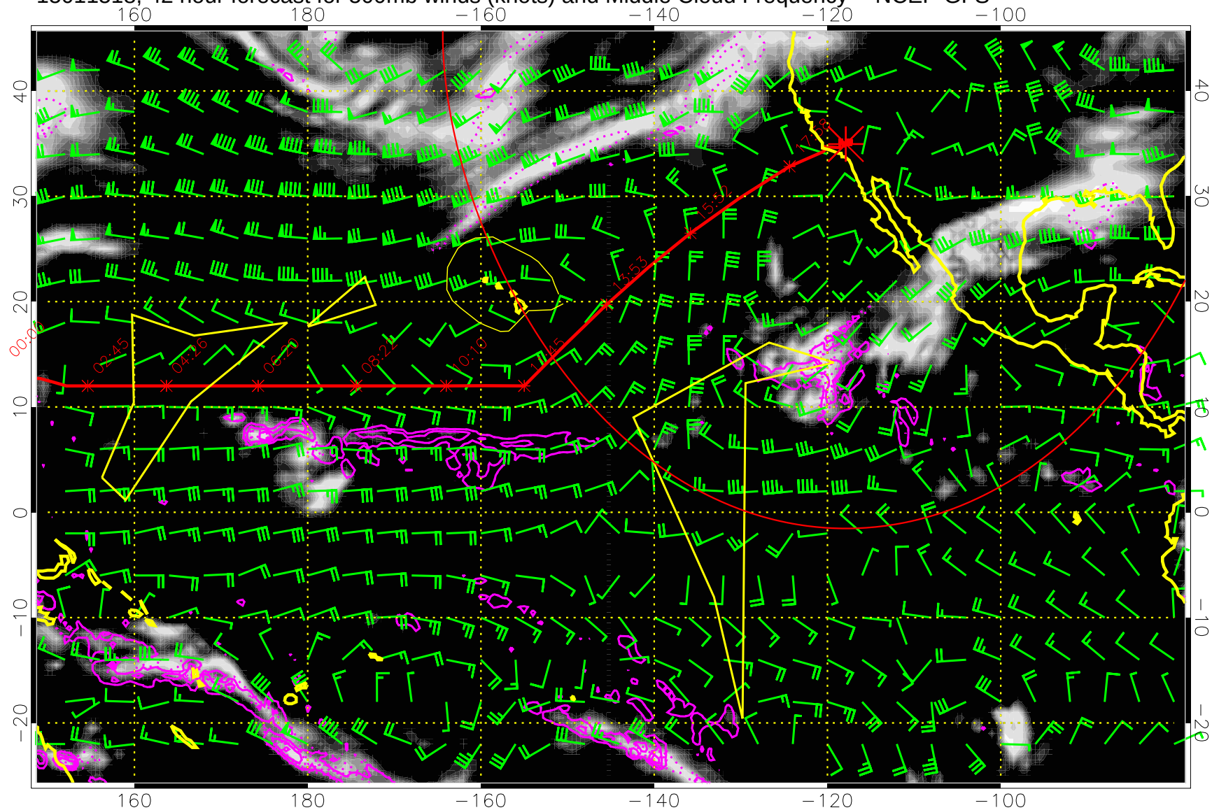
15011518, 42 hour forecast for 500mb winds (knots) and Middle Cloud Frequency -- NCEP GFS
