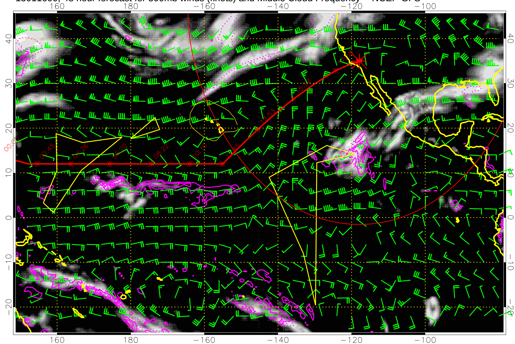
15011600, 48 hour forecast for 500mb winds (knots) and Middle Cloud Frequency -- NCEP GFS
