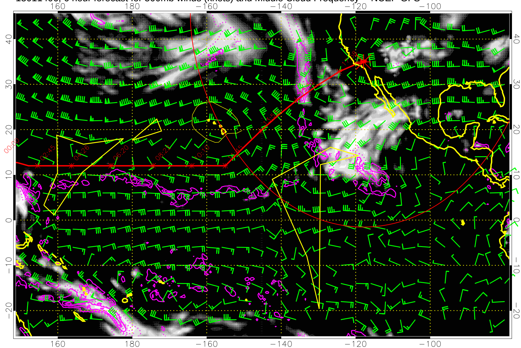
15011406, 6 hour forecast for 500mb winds (knots) and Middle Cloud Frequency -- NCEP GFS
