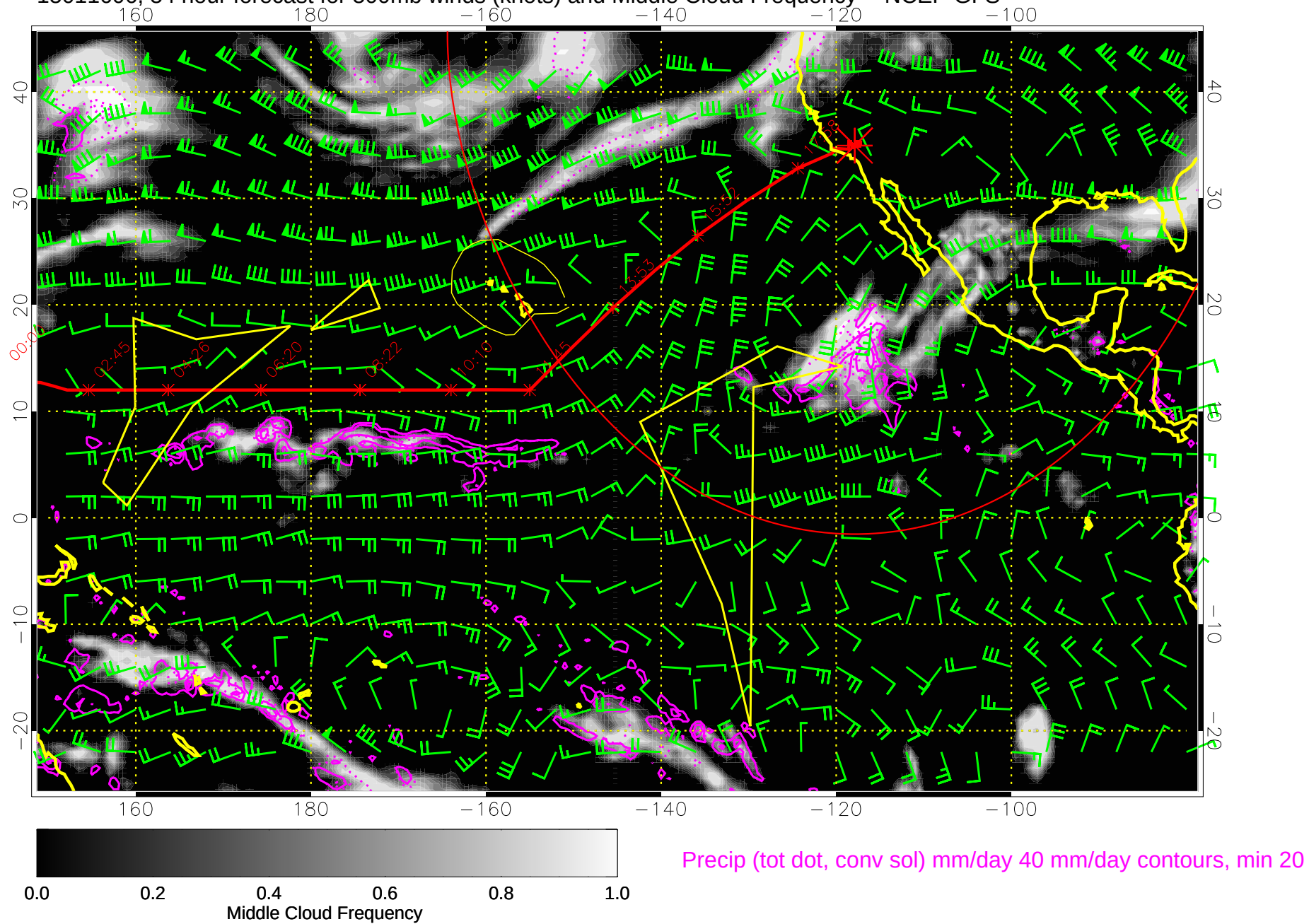
15011606, 54 hour forecast for 500mb winds (knots) and Middle Cloud Frequency -- NCEP GFS
