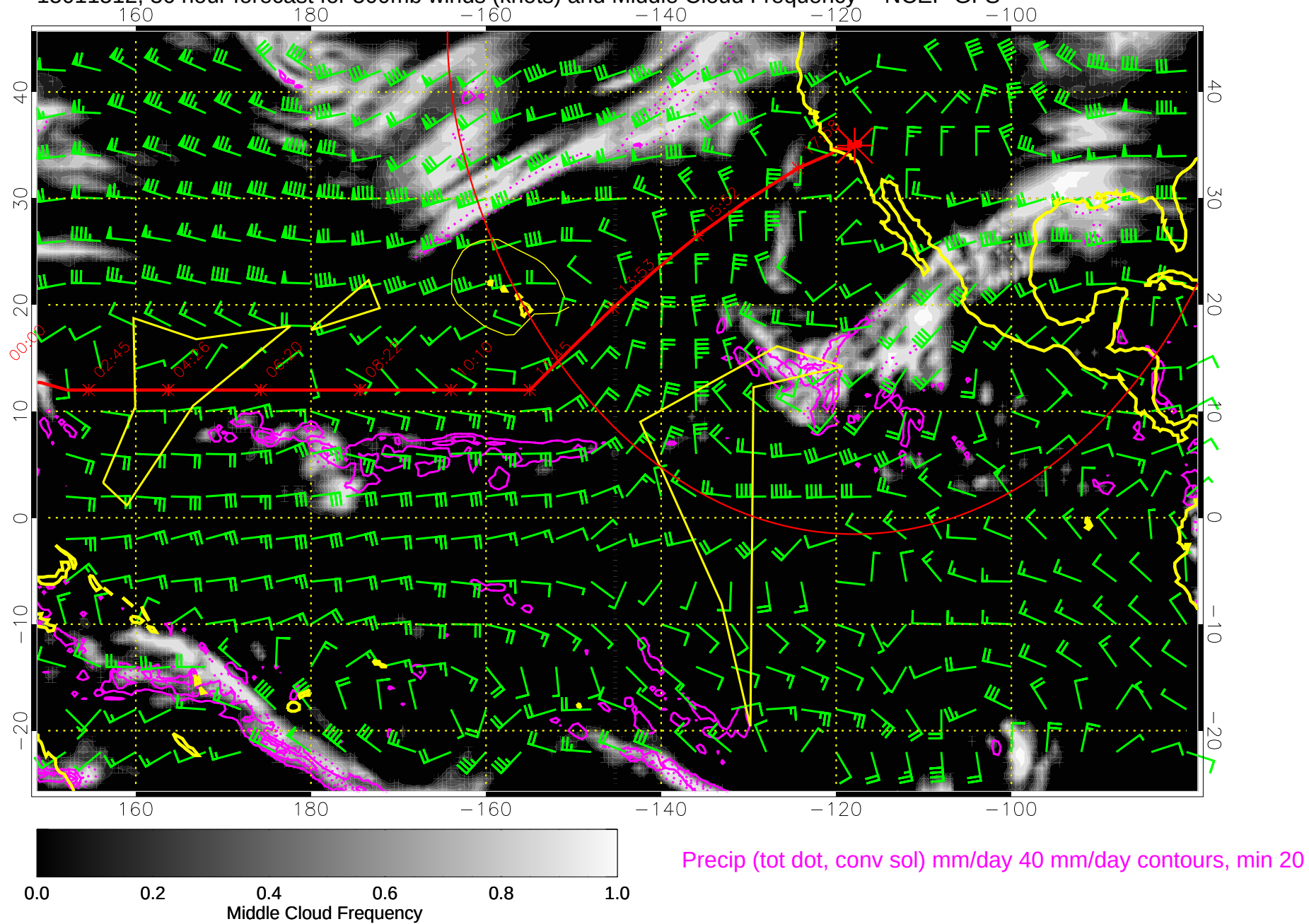
15011512, 36 hour forecast for 500mb winds (knots) and Middle Cloud Frequency -- NCEP GFS
