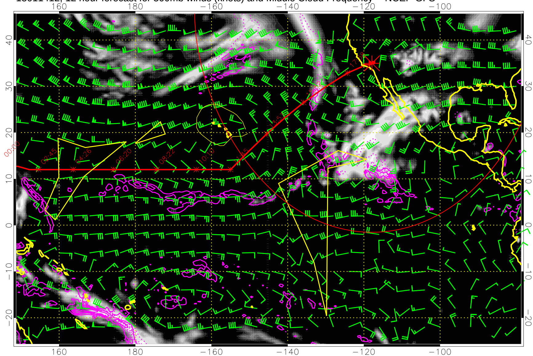
15011412, 12 hour forecast for 500mb winds (knots) and Middle Cloud Frequency -- NCEP GFS
