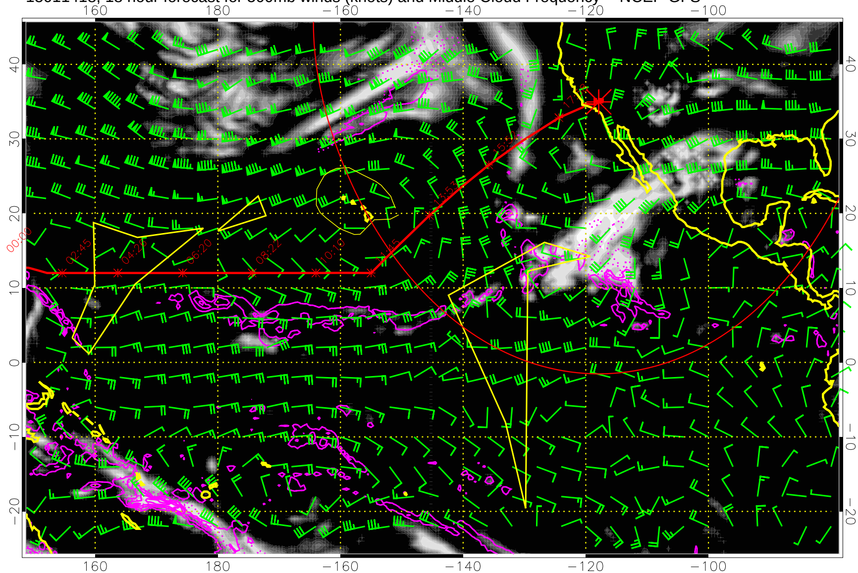
15011418, 18 hour forecast for 500mb winds (knots) and Middle Cloud Frequency -- NCEP GFS
