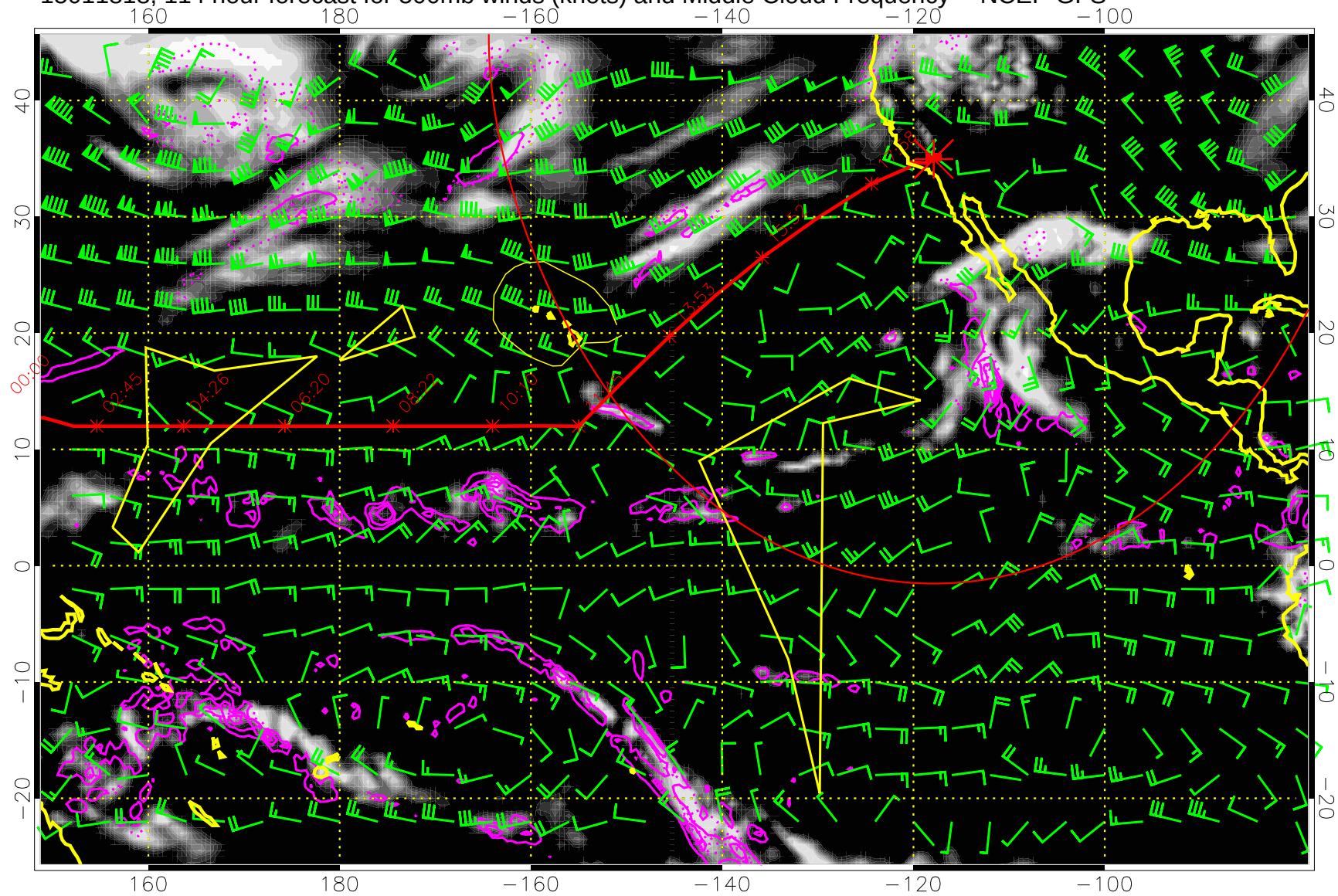
15011818, 114 hour forecast for 500mb winds (knots) and Middle Cloud Frequency -- NCEP GFS
