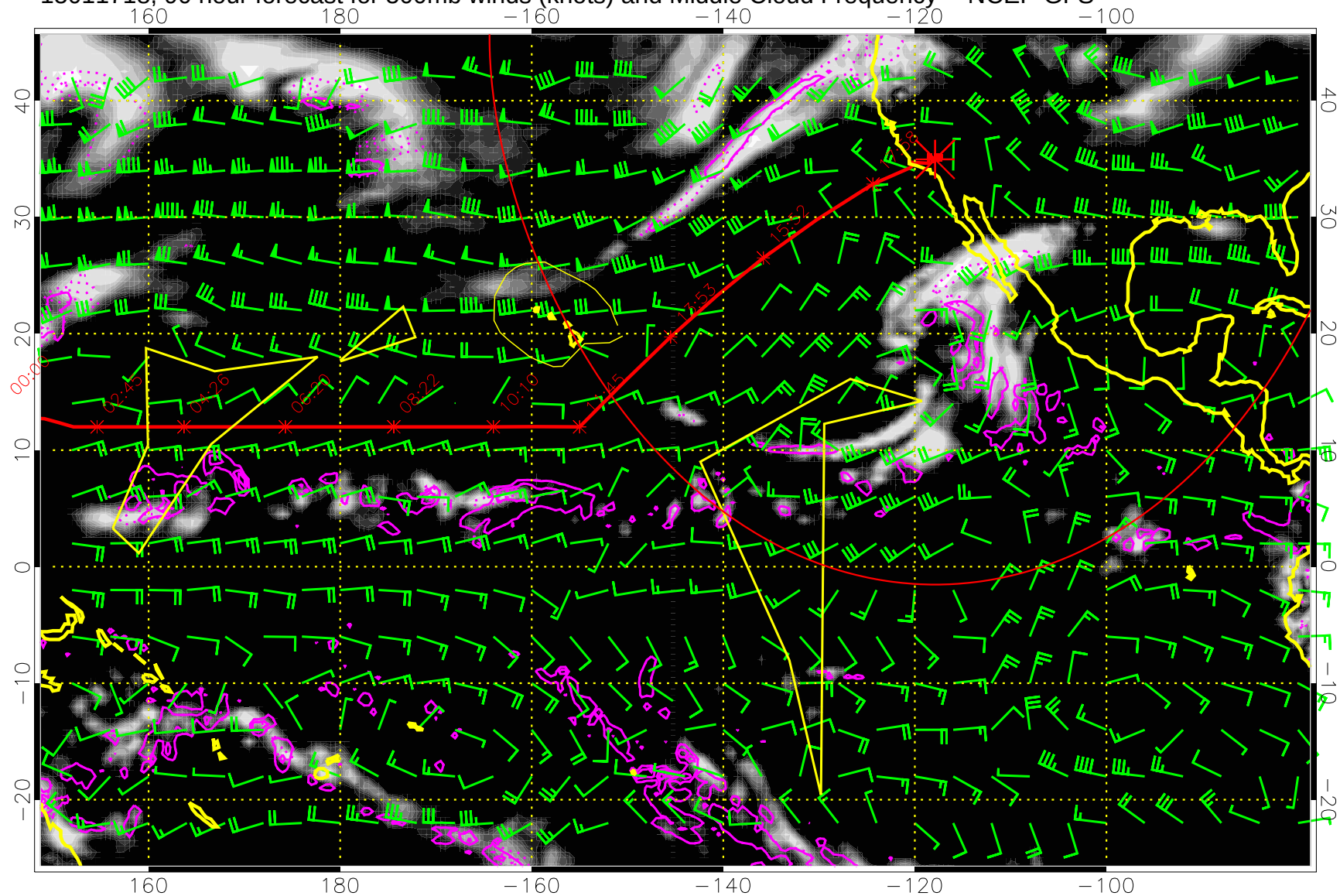
15011718, 90 hour forecast for 500mb winds (knots) and Middle Cloud Frequency -- NCEP GFS
