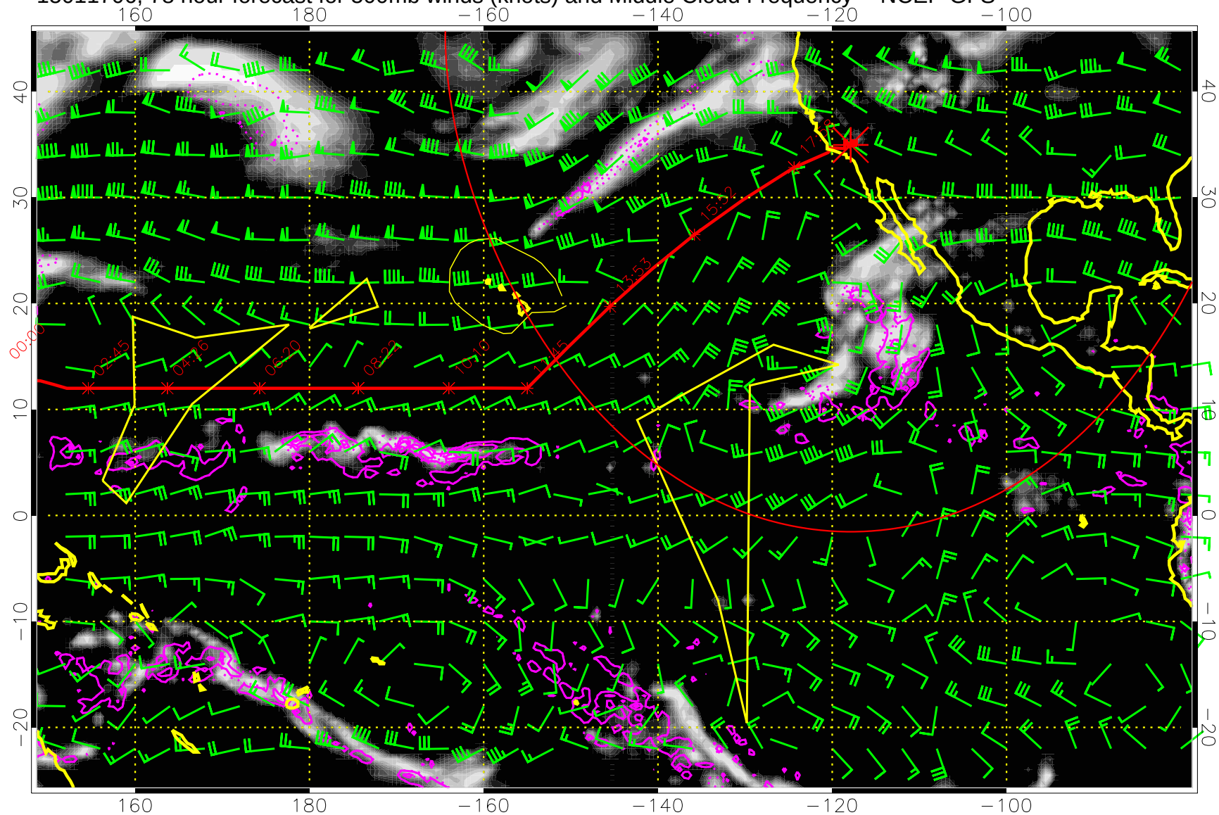
15011706, 78 hour forecast for 500mb winds (knots) and Middle Cloud Frequency -- NCEP GFS
