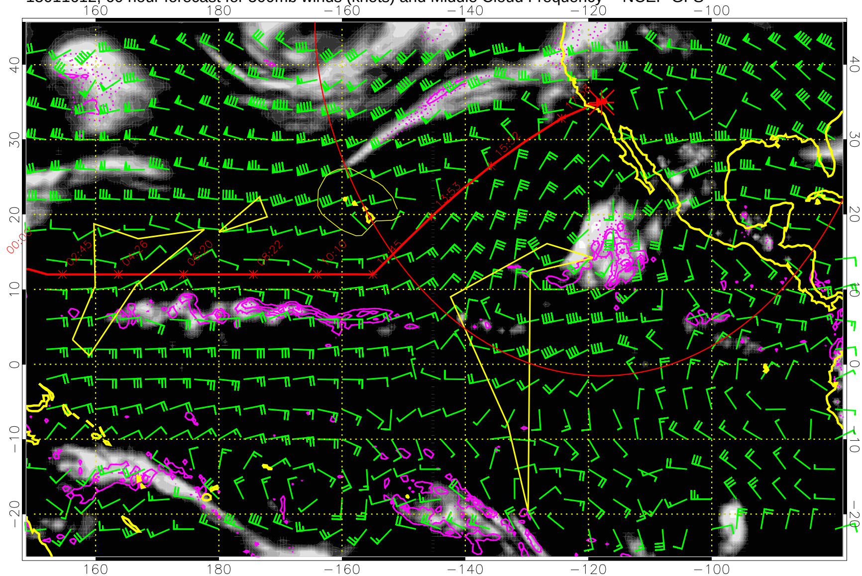
15011612, 60 hour forecast for 500mb winds (knots) and Middle Cloud Frequency -- NCEP GFS
