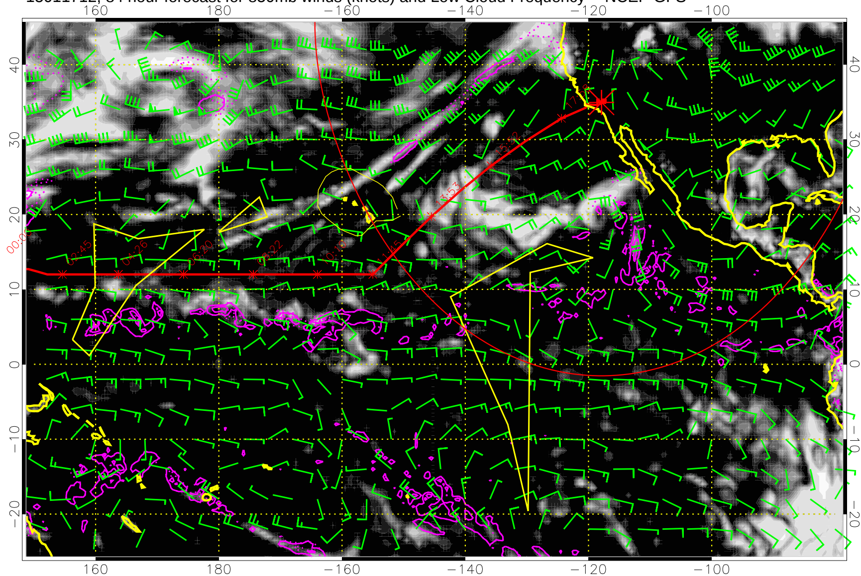
15011712, 84 hour forecast for 850mb winds (knots) and Low Cloud Frequency -- NCEP GFS
