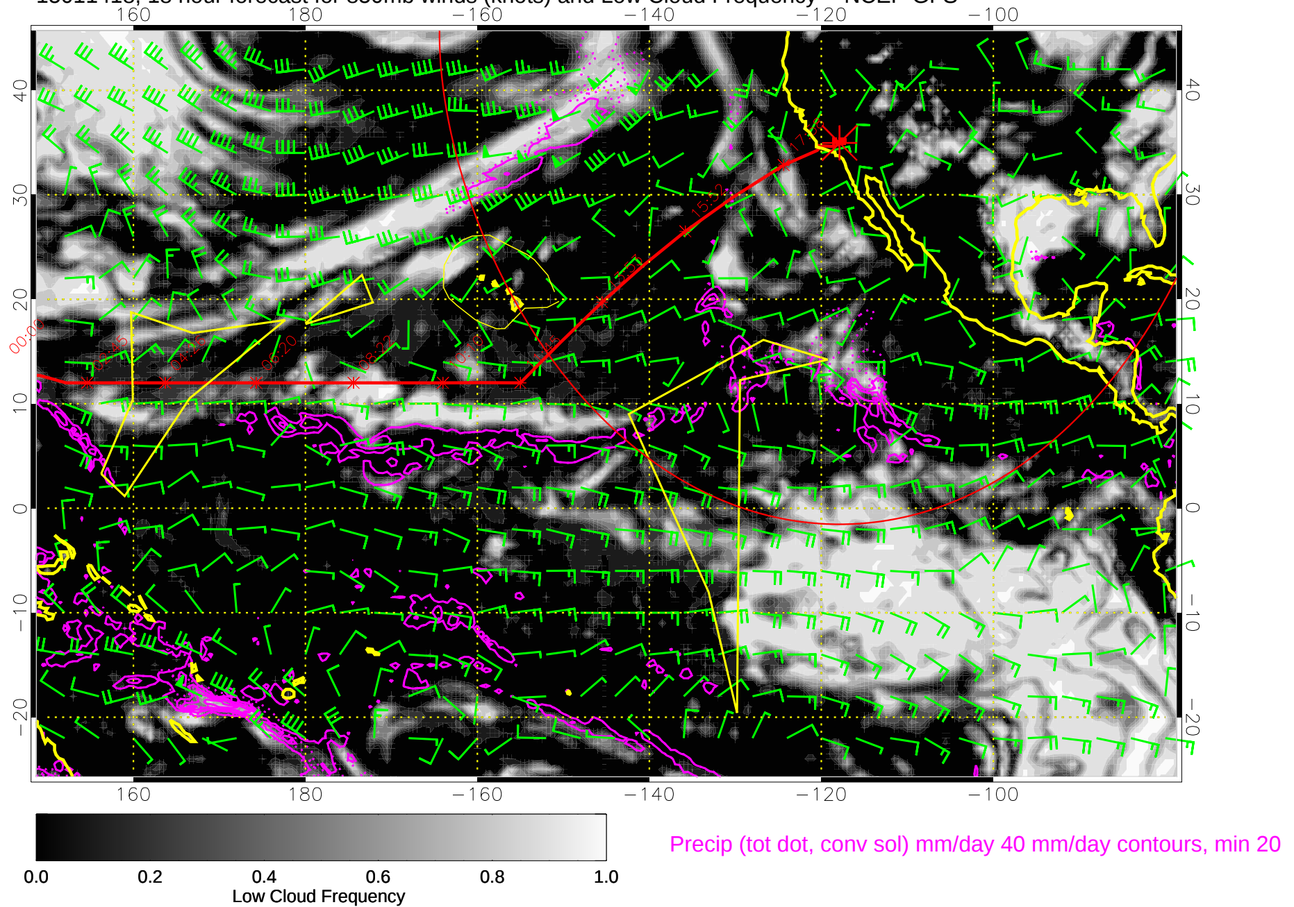
15011418, 18 hour forecast for 850mb winds (knots) and Low Cloud Frequency -- NCEP GFS
