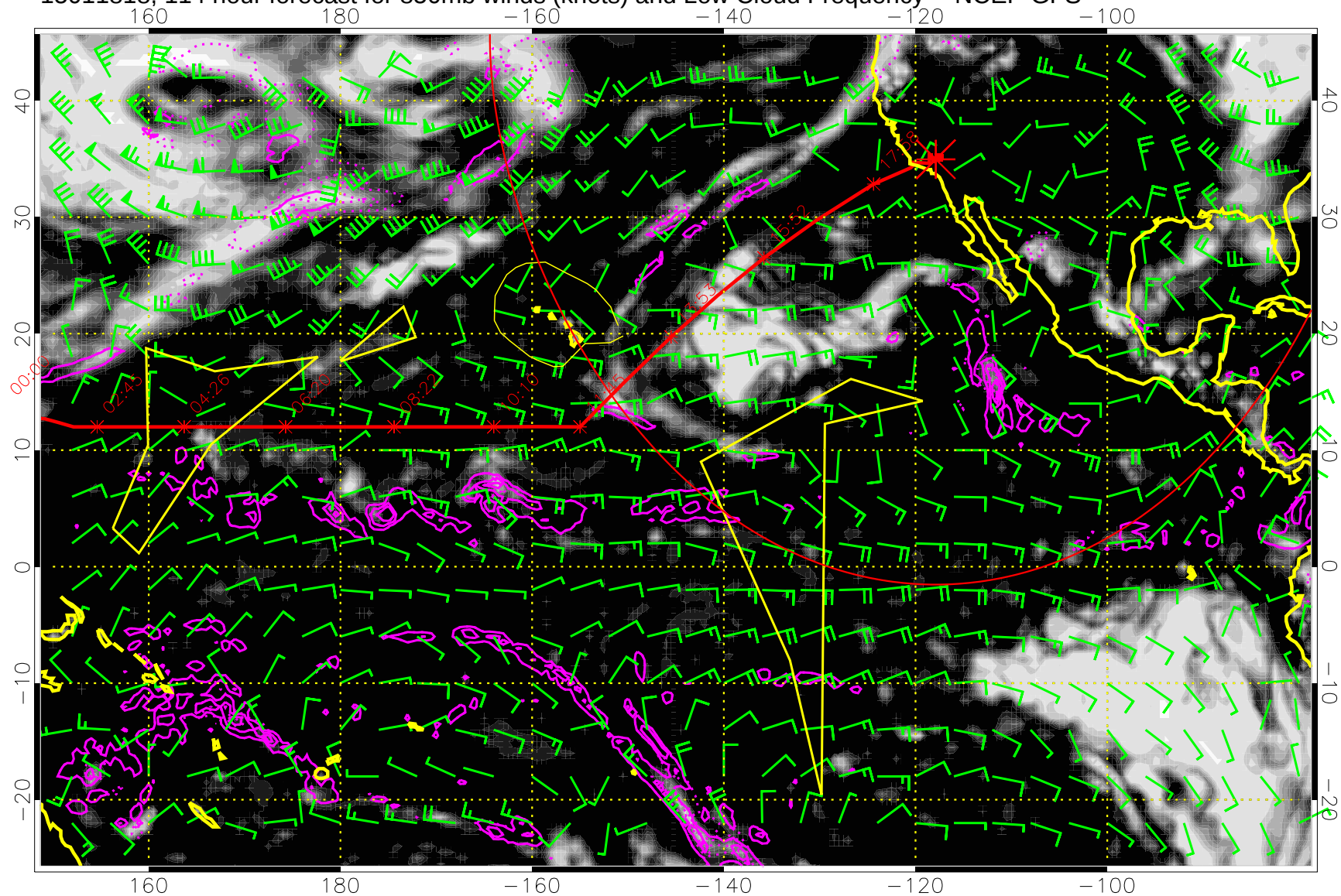
15011818, 114 hour forecast for 850mb winds (knots) and Low Cloud Frequency -- NCEP GFS
