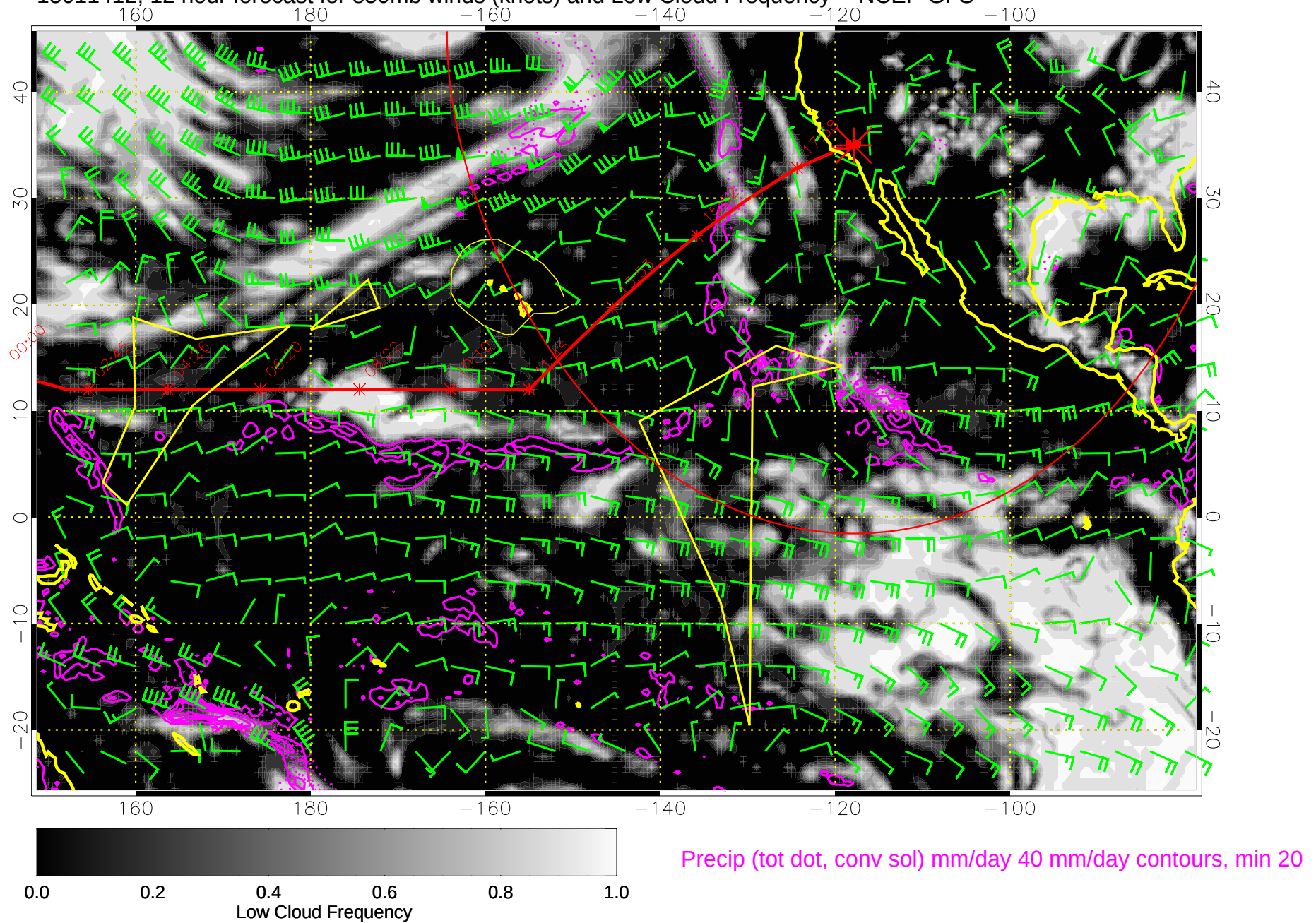
15011412, 12 hour forecast for 850mb winds (knots) and Low Cloud Frequency -- NCEP GFS
