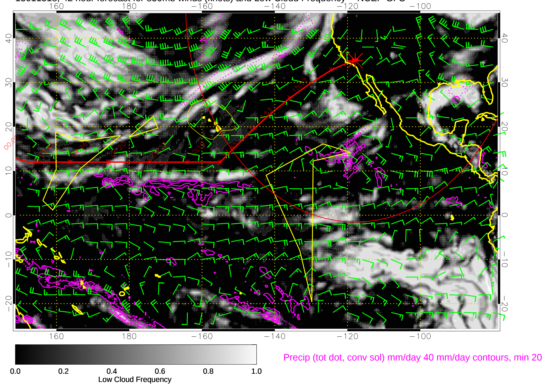
15011518, 42 hour forecast for 850mb winds (knots) and Low Cloud Frequency -- NCEP GFS
