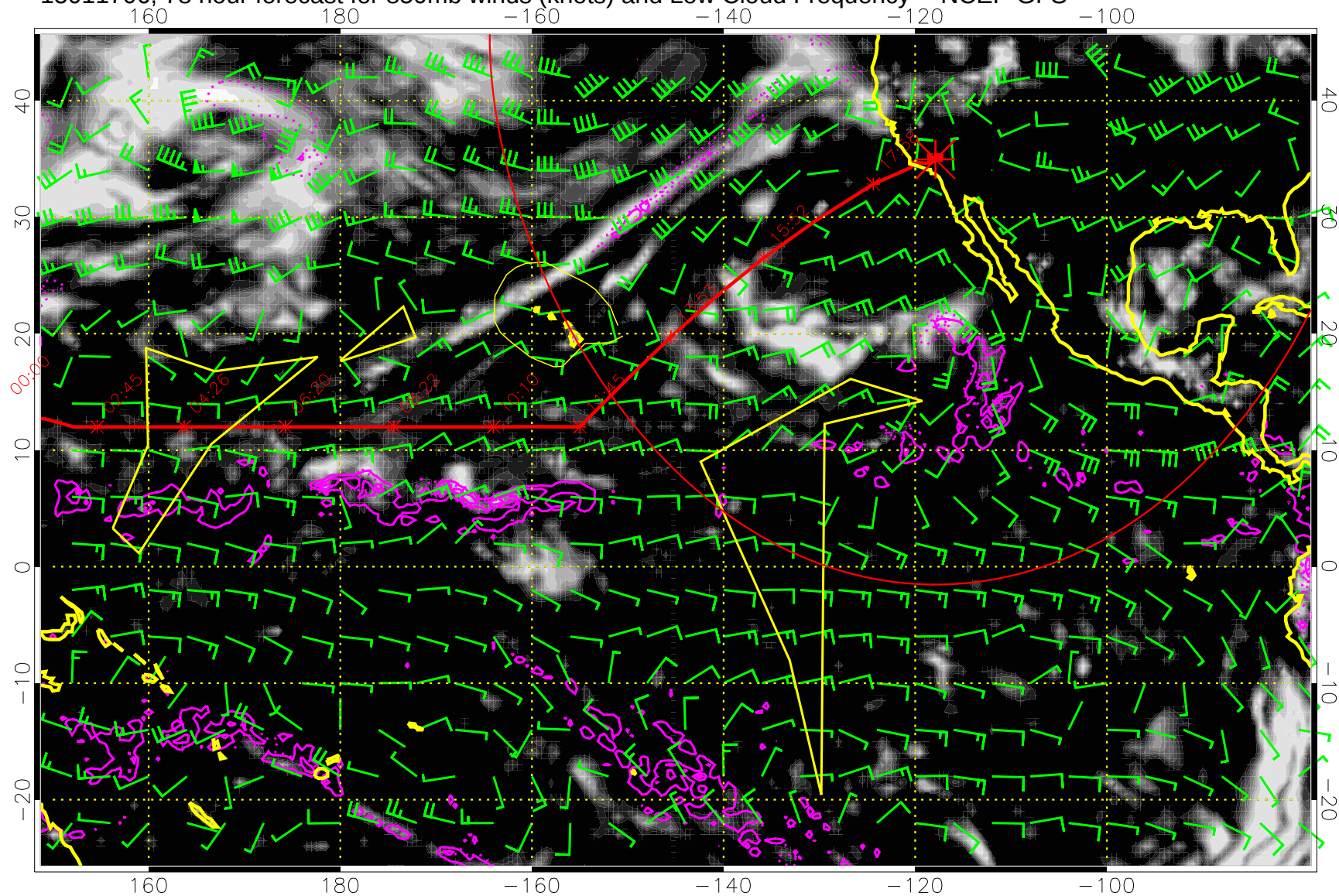
15011706, 78 hour forecast for 850mb winds (knots) and Low Cloud Frequency -- NCEP GFS
