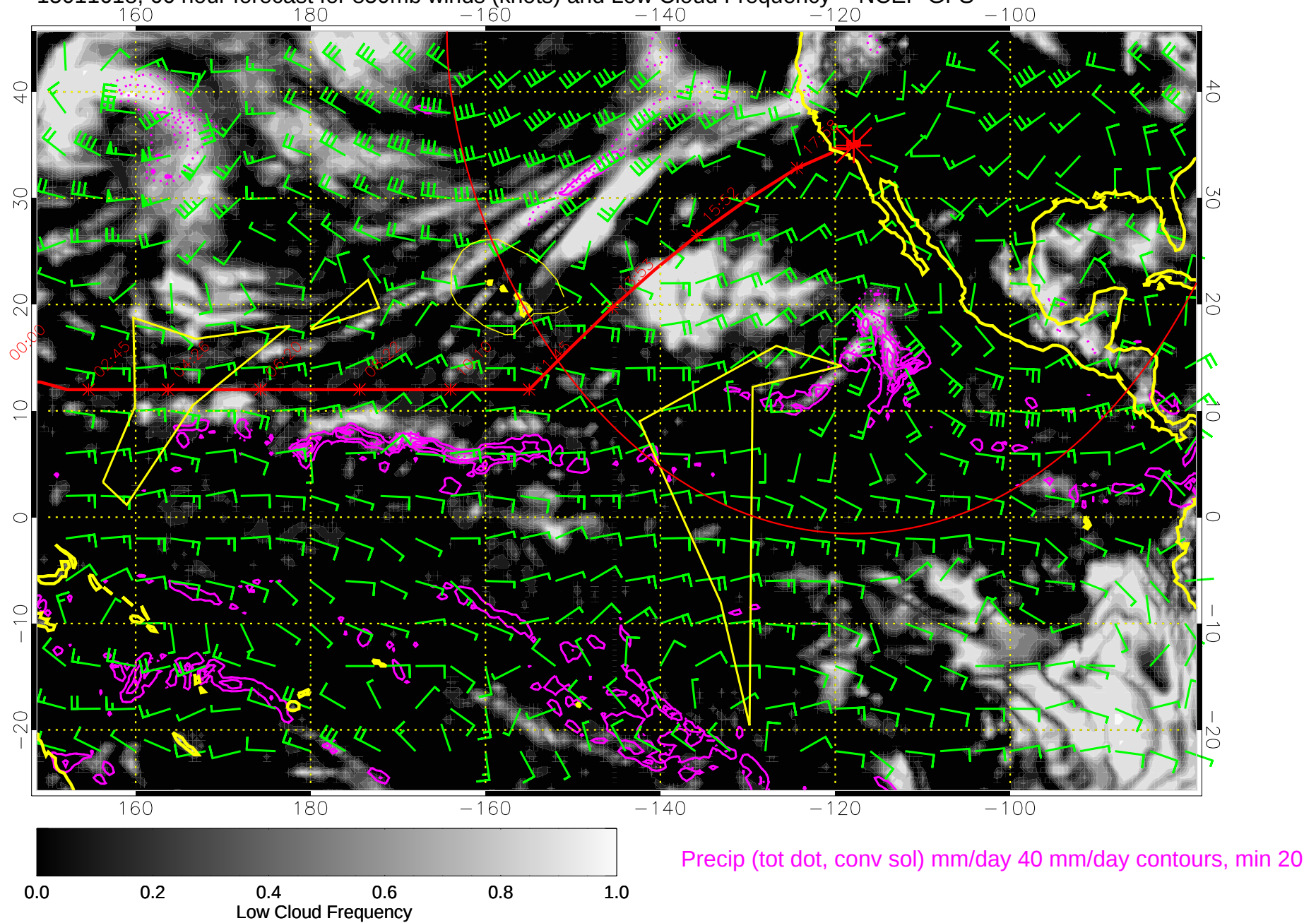
15011618, 66 hour forecast for 850mb winds (knots) and Low Cloud Frequency -- NCEP GFS
