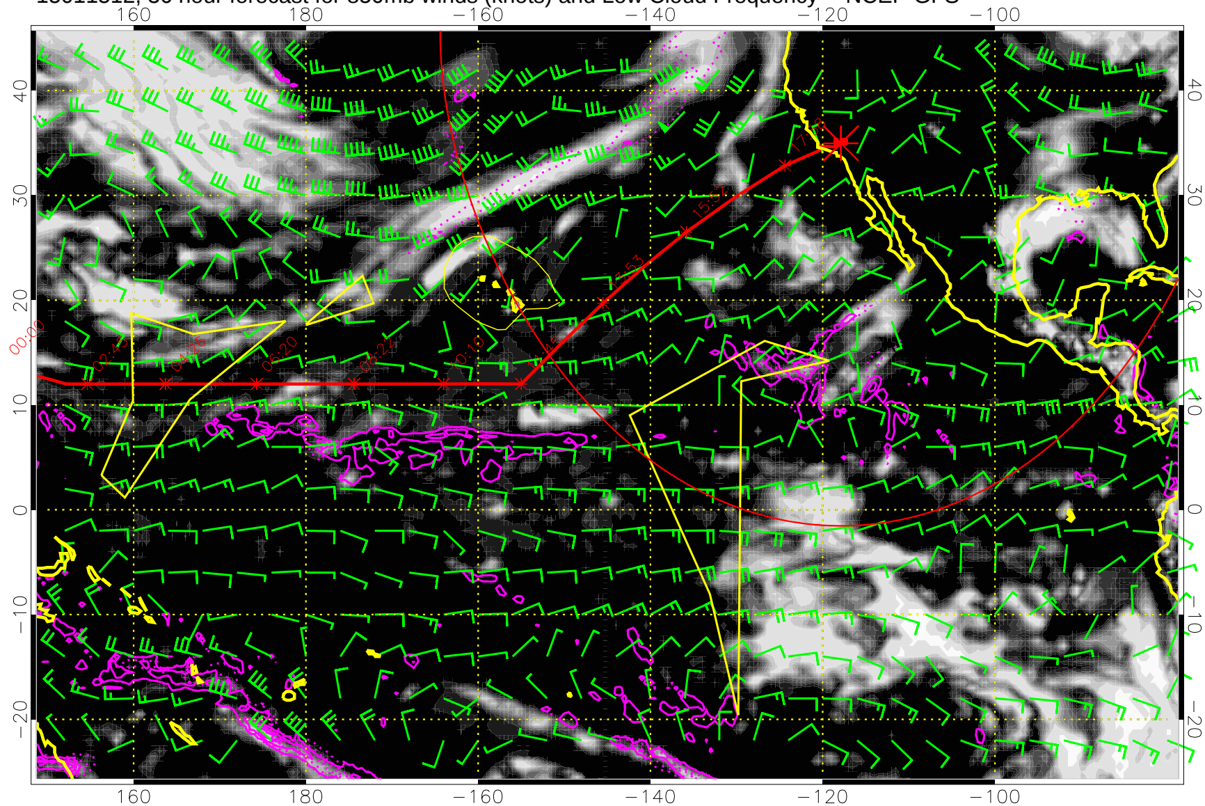
15011512, 36 hour forecast for 850mb winds (knots) and Low Cloud Frequency -- NCEP GFS
