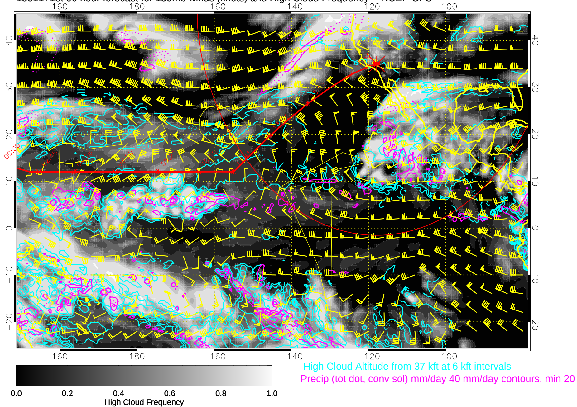
15011718, 90 hour forecast for 150mb winds (knots) and High Cloud Frequency -- NCEP GFS
