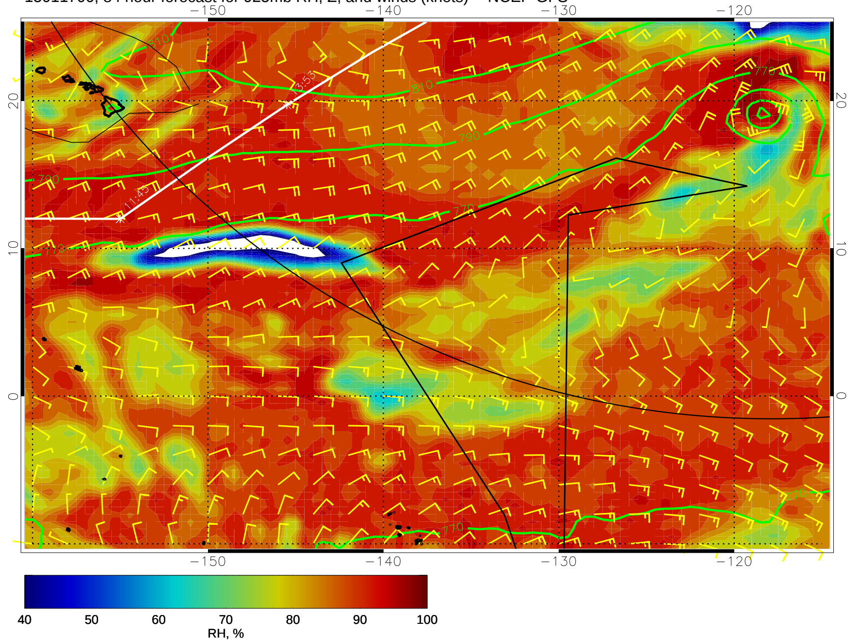
15011700, 84 hour forecast for 925mb RH, Z, and winds (knots) -- NCEP GFS
