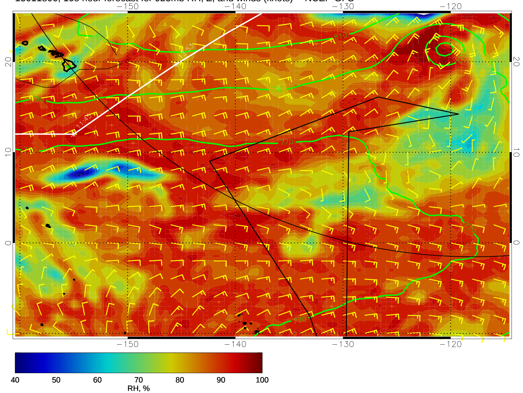
15011800, 108 hour forecast for 925mb RH, Z, and winds (knots) -- NCEP GFS
