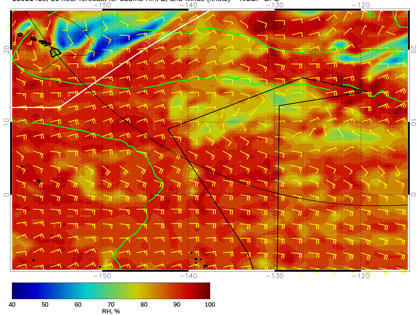
15011418, 30 hour forecast for 925mb RH, Z, and winds (knots) -- NCEP GFS
