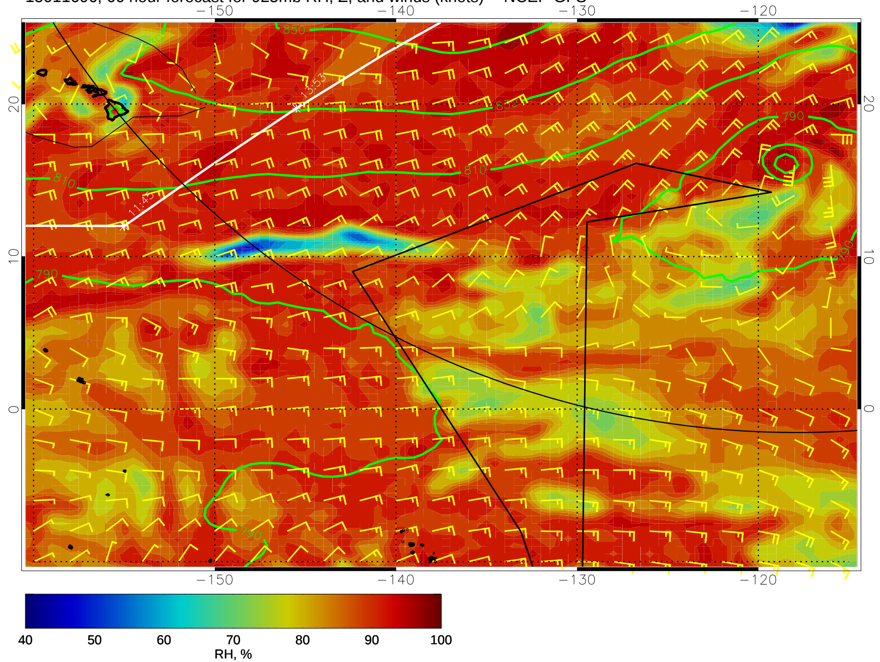
15011606, 66 hour forecast for 925mb RH, Z, and winds (knots) -- NCEP GFS
