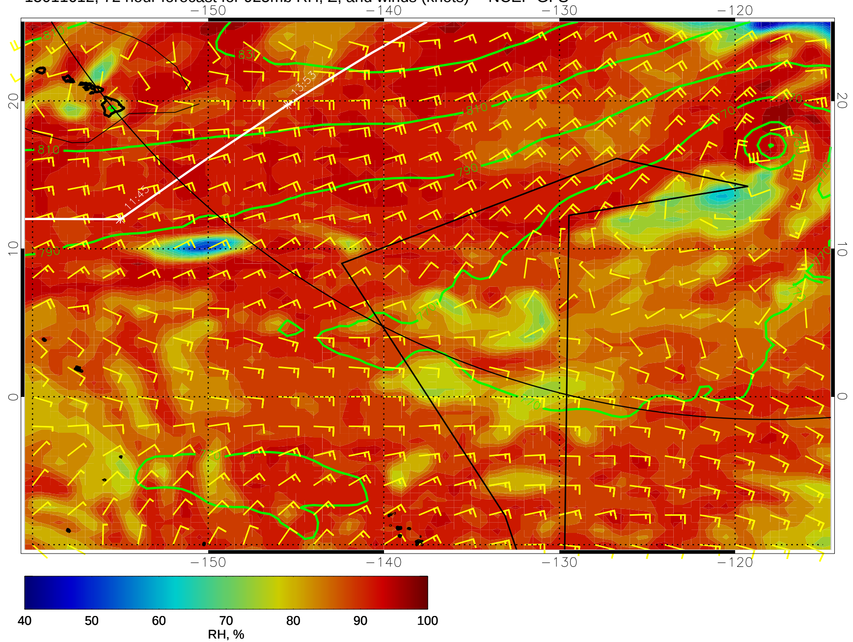
15011612, 72 hour forecast for 925mb RH, Z, and winds (knots) -- NCEP GFS
