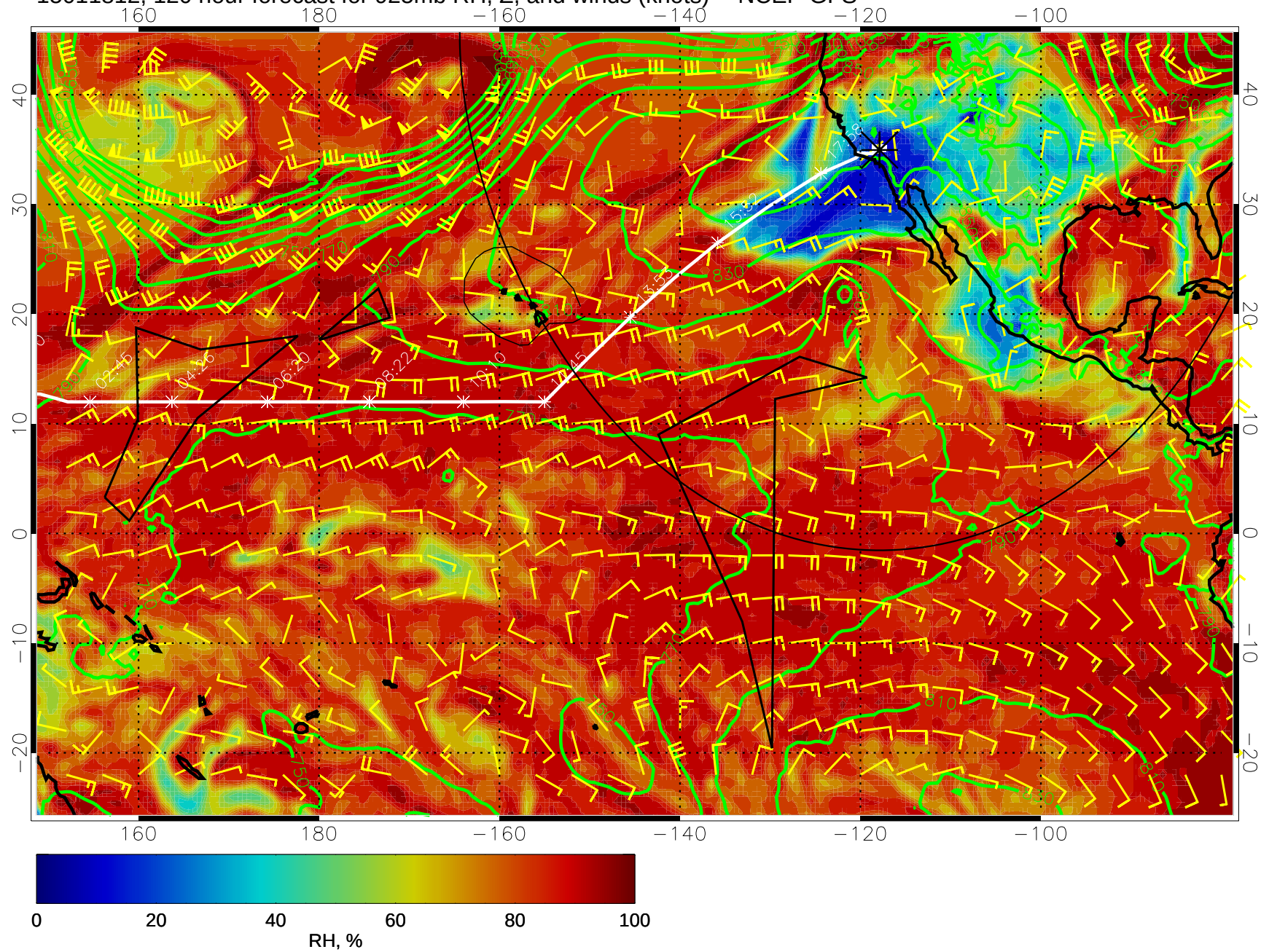
15011812, 120 hour forecast for 925mb RH, Z, and winds (knots) -- NCEP GFS
