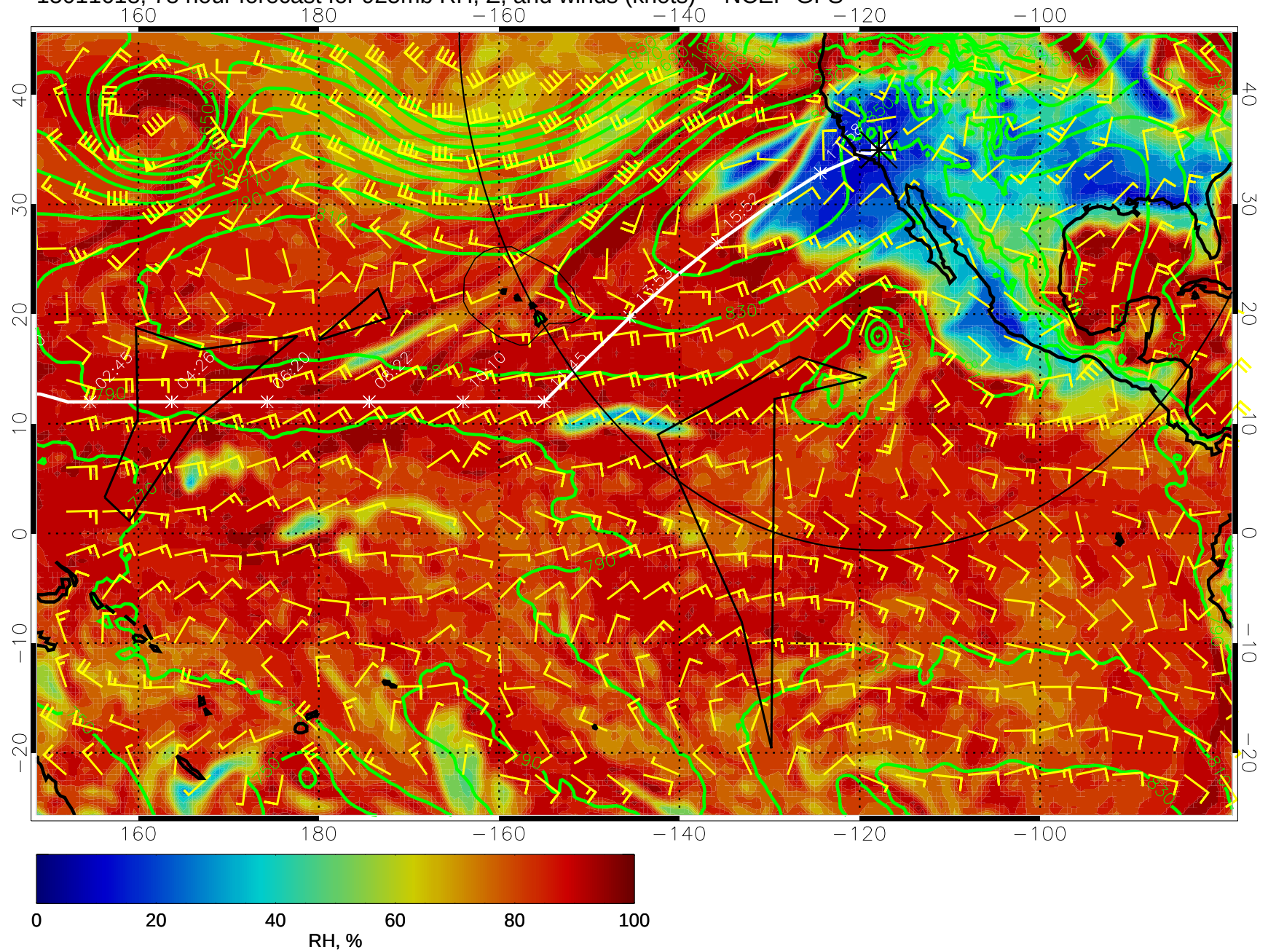
15011618, 78 hour forecast for 925mb RH, Z, and winds (knots) -- NCEP GFS
