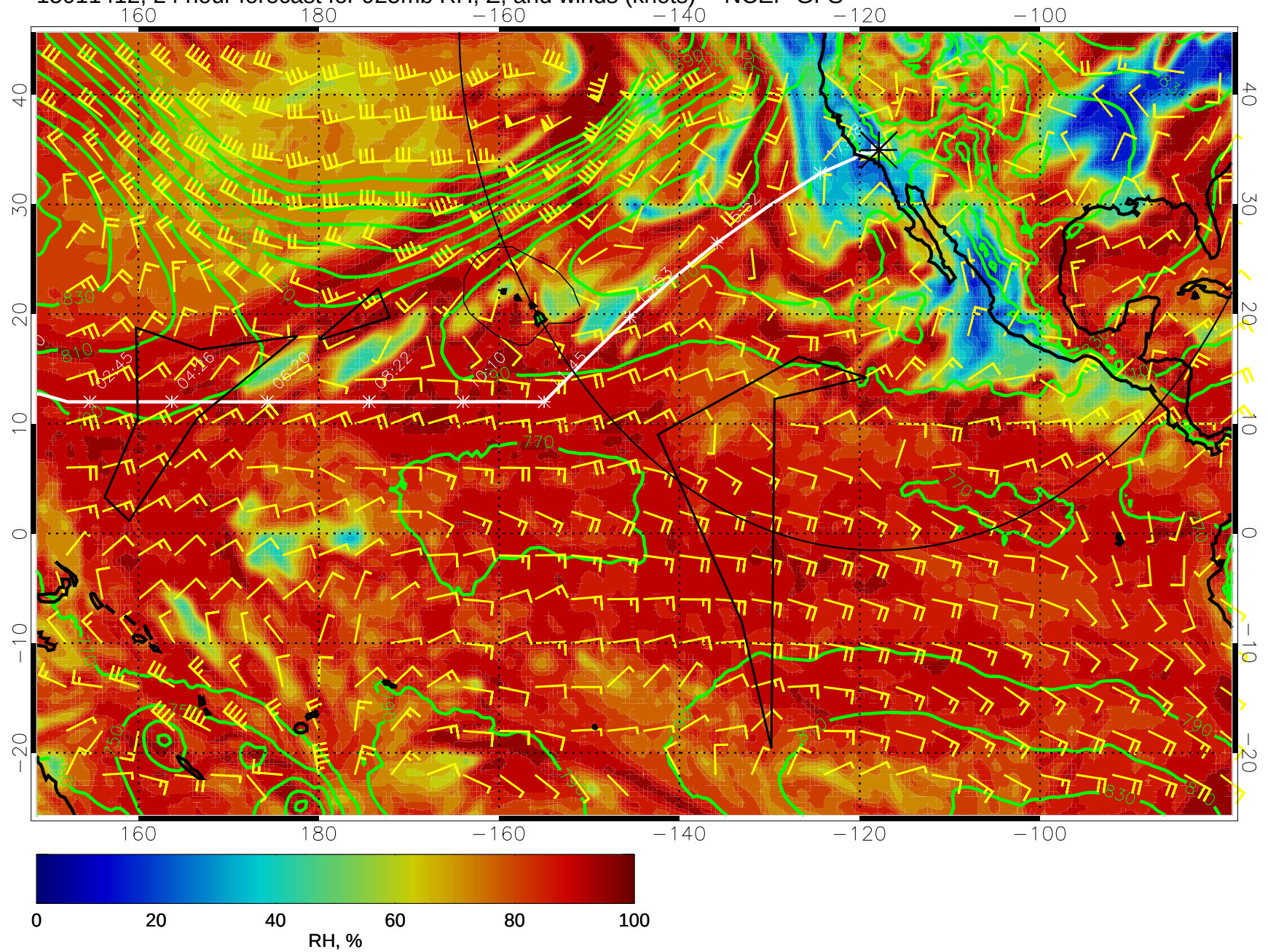
15011412, 24 hour forecast for 925mb RH, Z, and winds (knots) -- NCEP GFS
