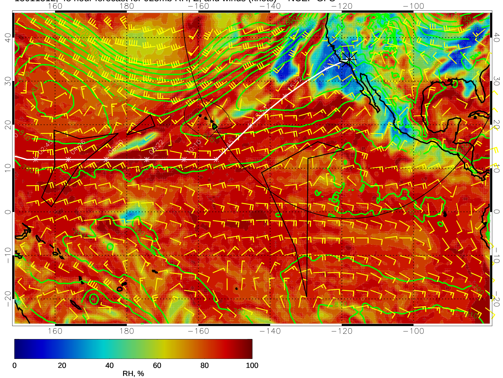
15011512, 48 hour forecast for 925mb RH, Z, and winds (knots) -- NCEP GFS
