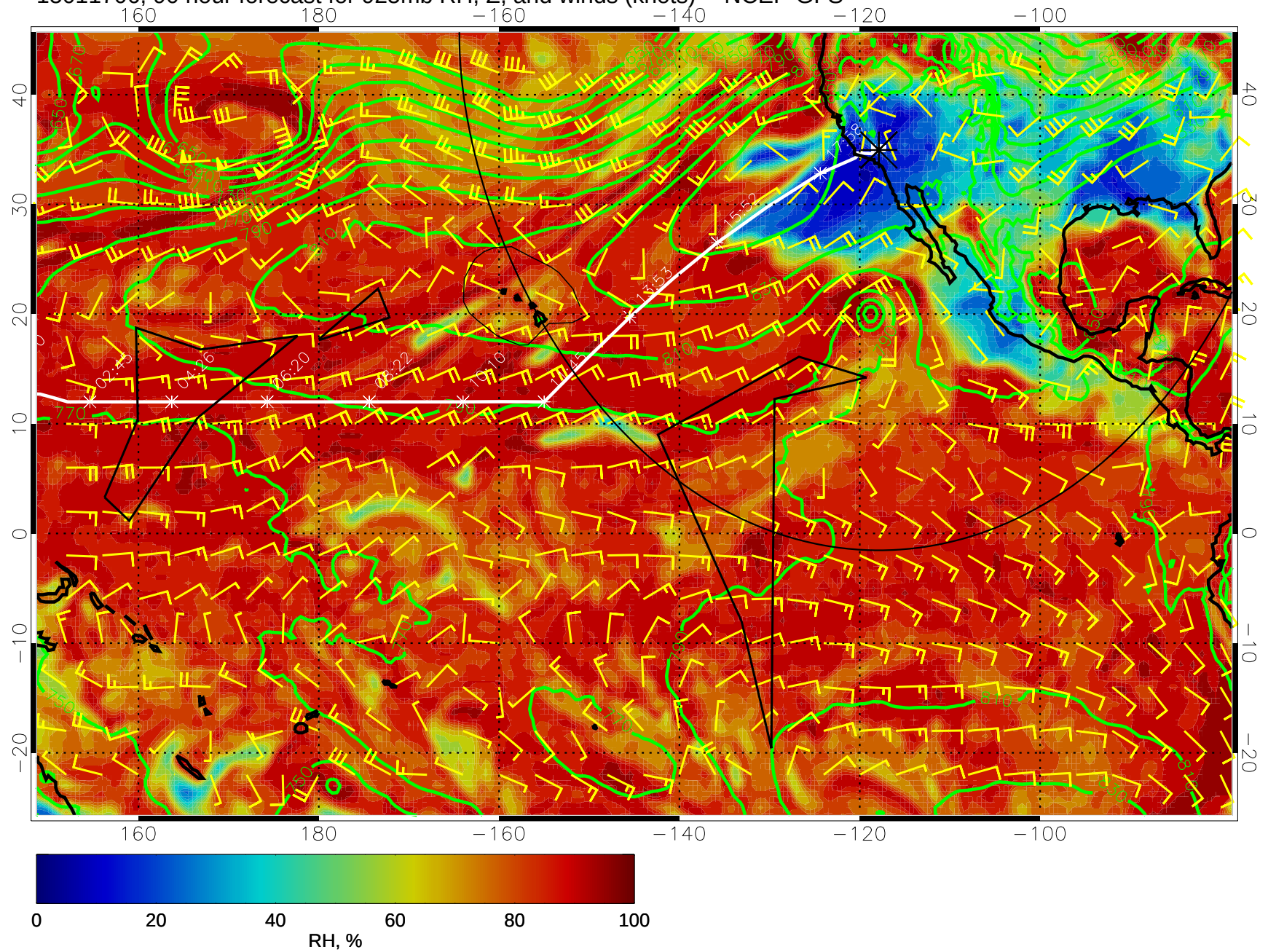
15011706, 90 hour forecast for 925mb RH, Z, and winds (knots) -- NCEP GFS
