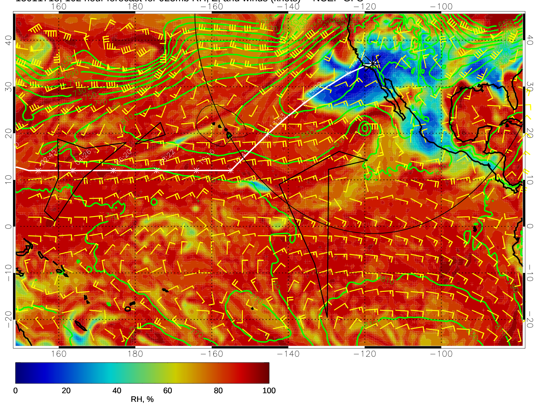
15011718, 102 hour forecast for 925mb RH, Z, and winds (knots) -- NCEP GFS
