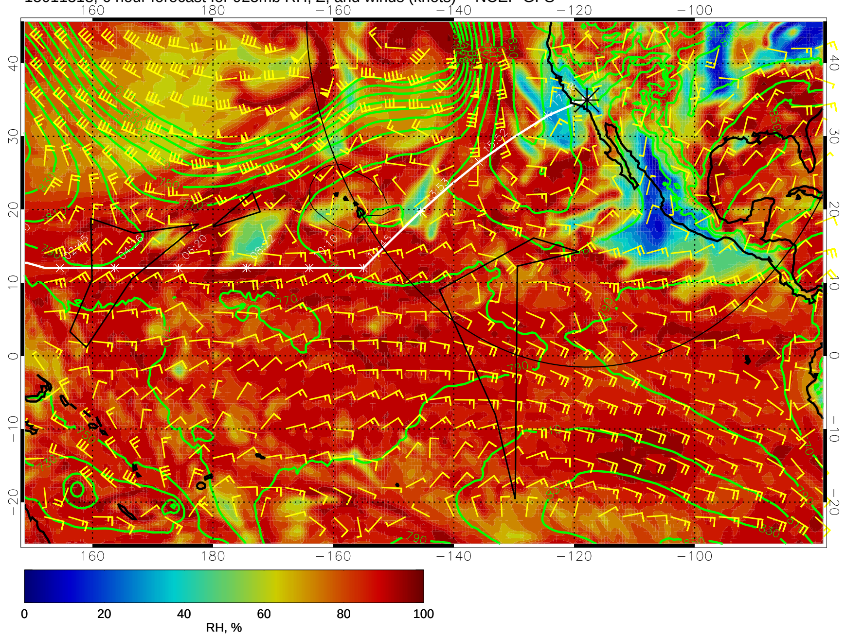
15011318, 6 hour forecast for 925mb RH, Z, and winds (knots) -- NCEP GFS
