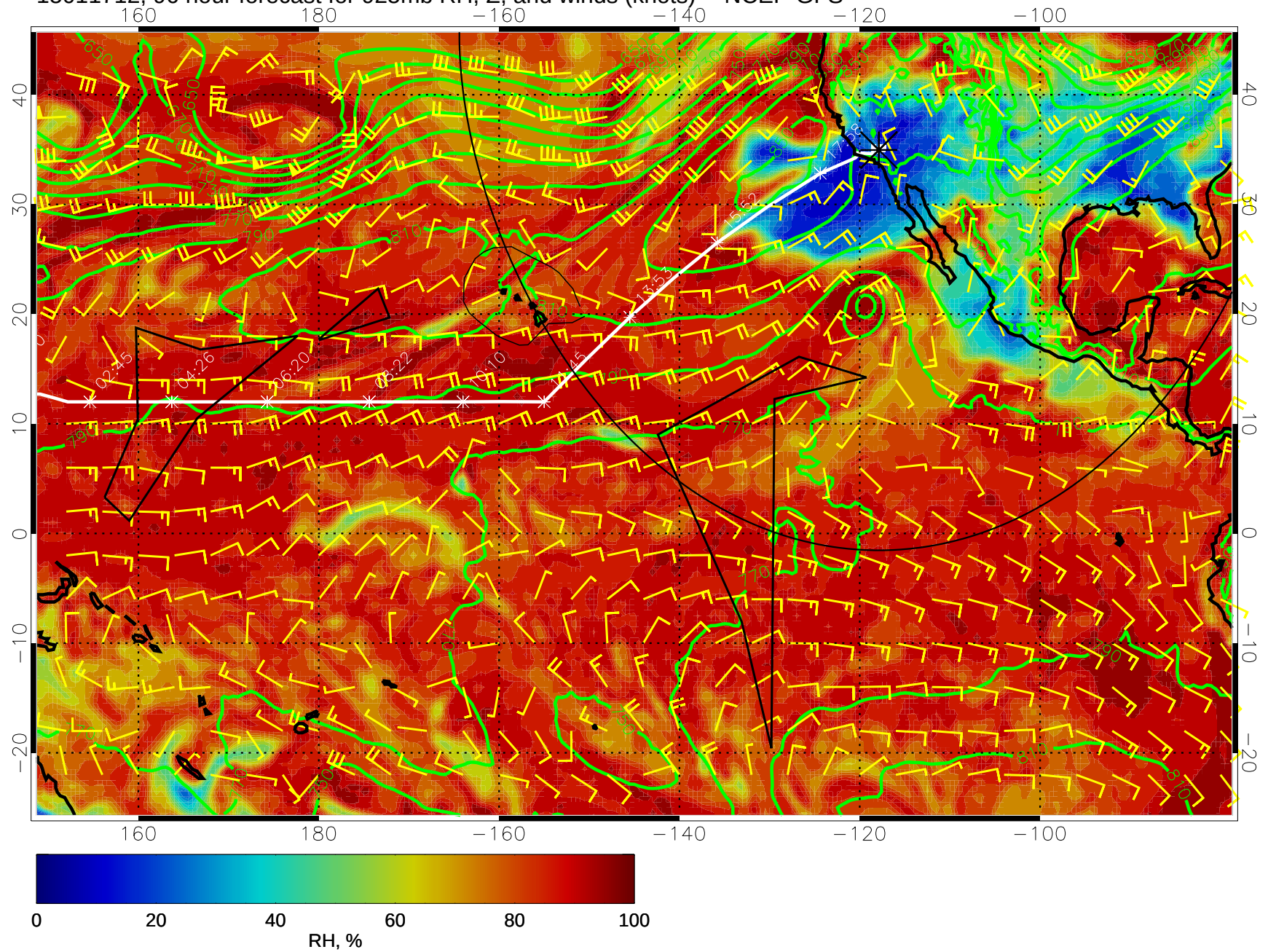
15011712, 96 hour forecast for 925mb RH, Z, and winds (knots) -- NCEP GFS
