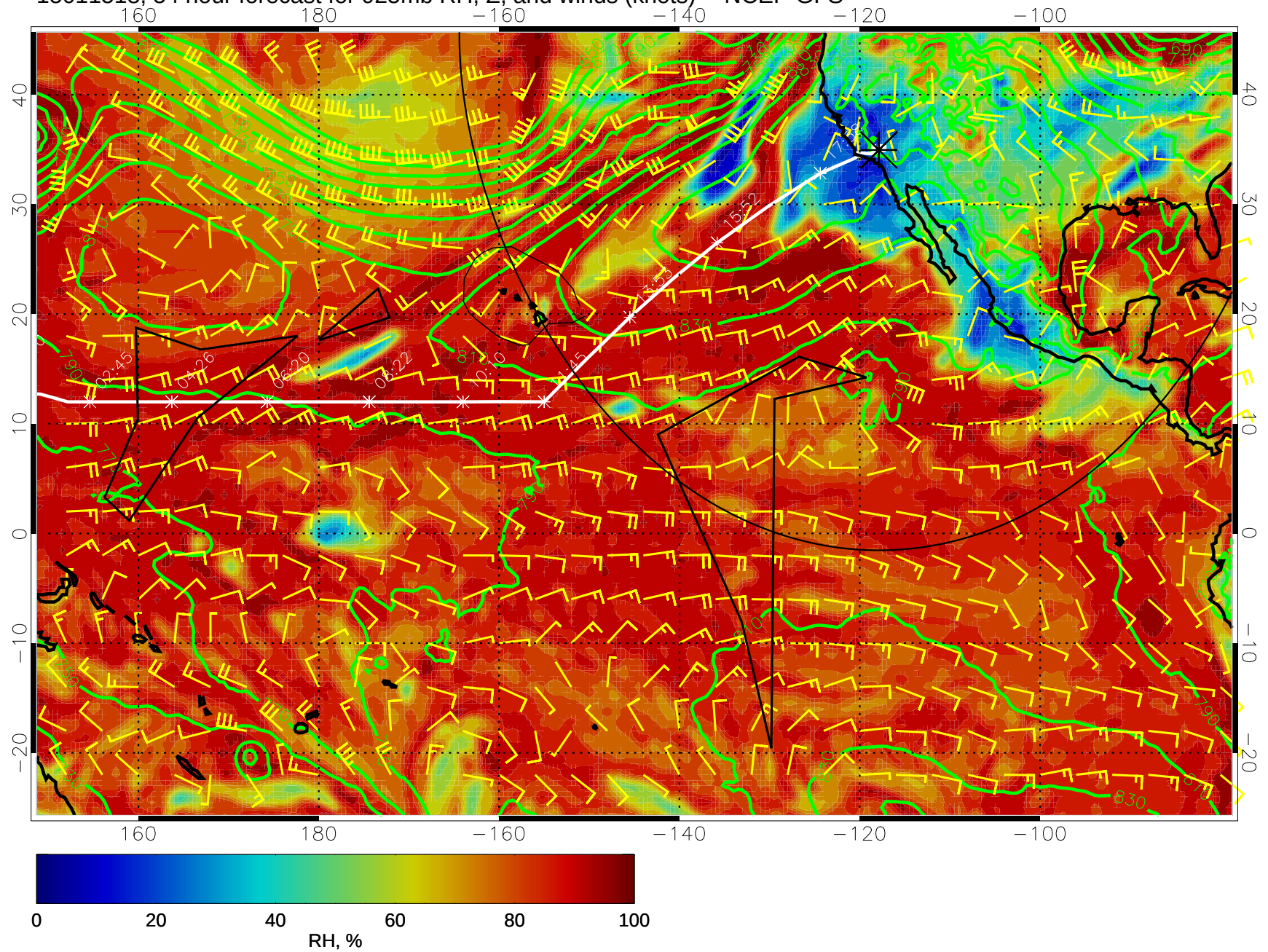
15011518, 54 hour forecast for 925mb RH, Z, and winds (knots) -- NCEP GFS
