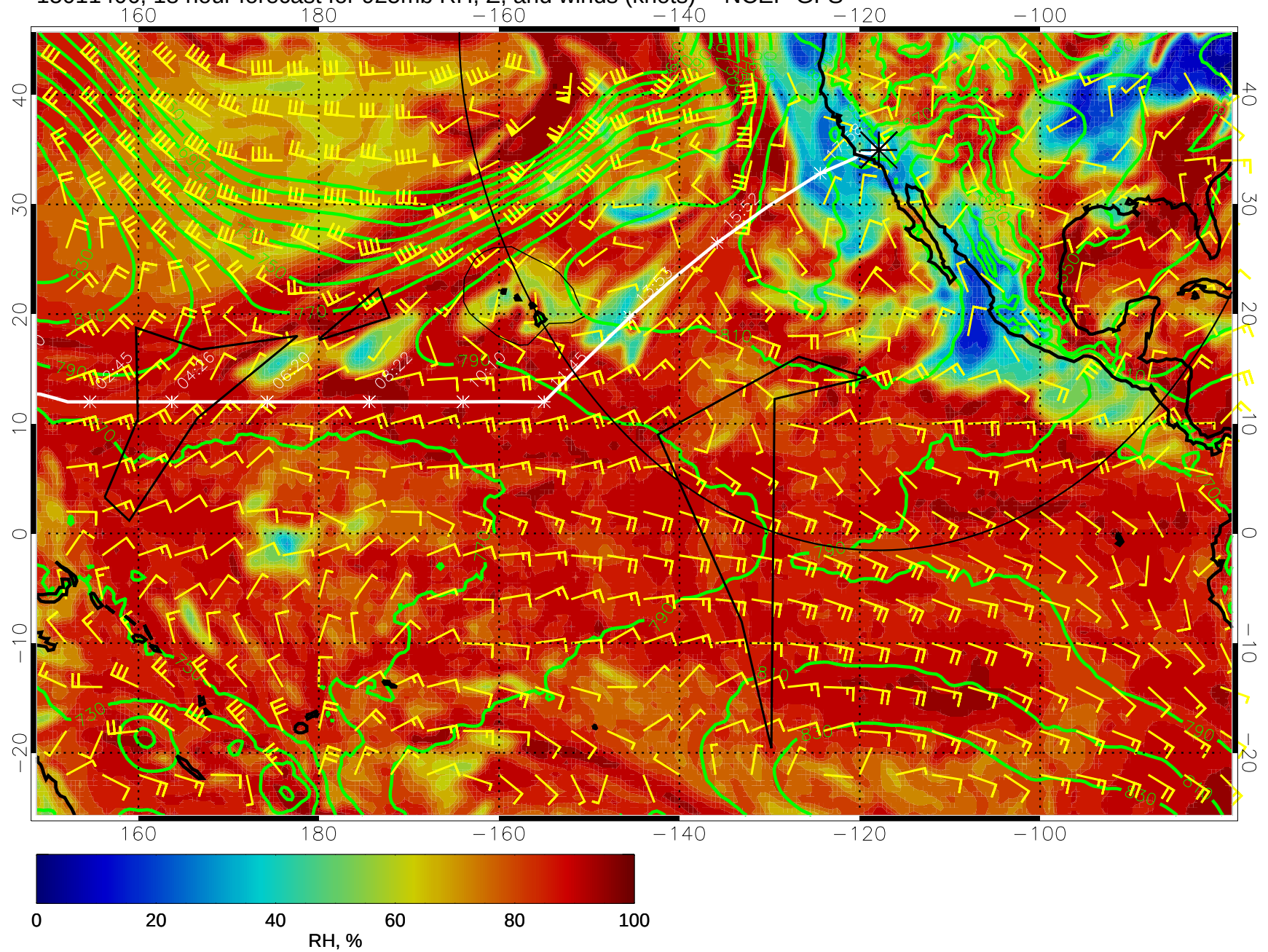
15011406, 18 hour forecast for 925mb RH, Z, and winds (knots) -- NCEP GFS
