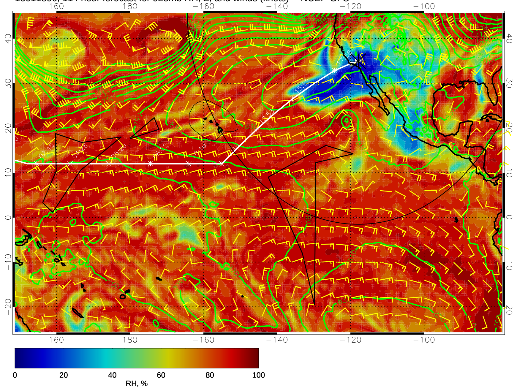
15011806, 114 hour forecast for 925mb RH, Z, and winds (knots) -- NCEP GFS
