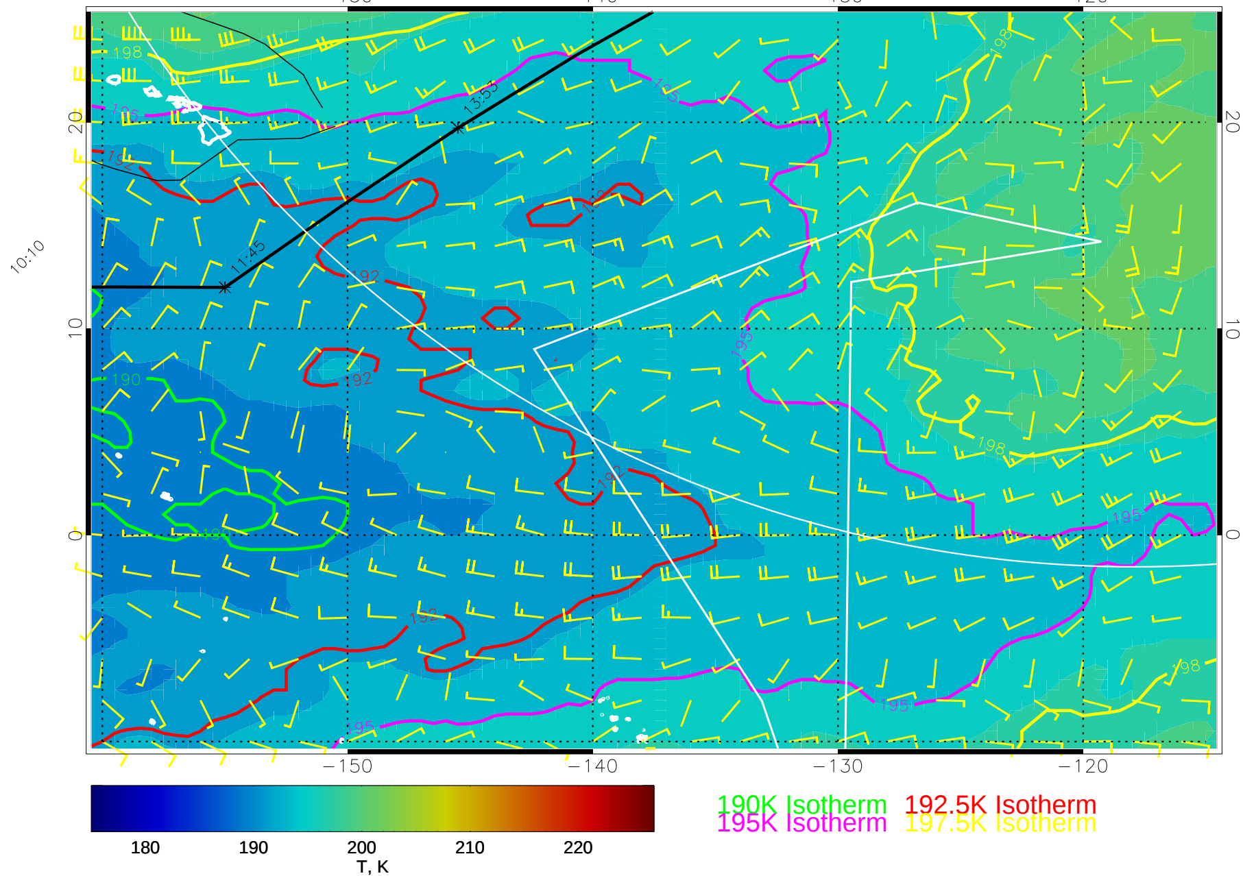
15011806, 114 hour forecast for 70mb T and winds (knots) -- NCEP GFS
