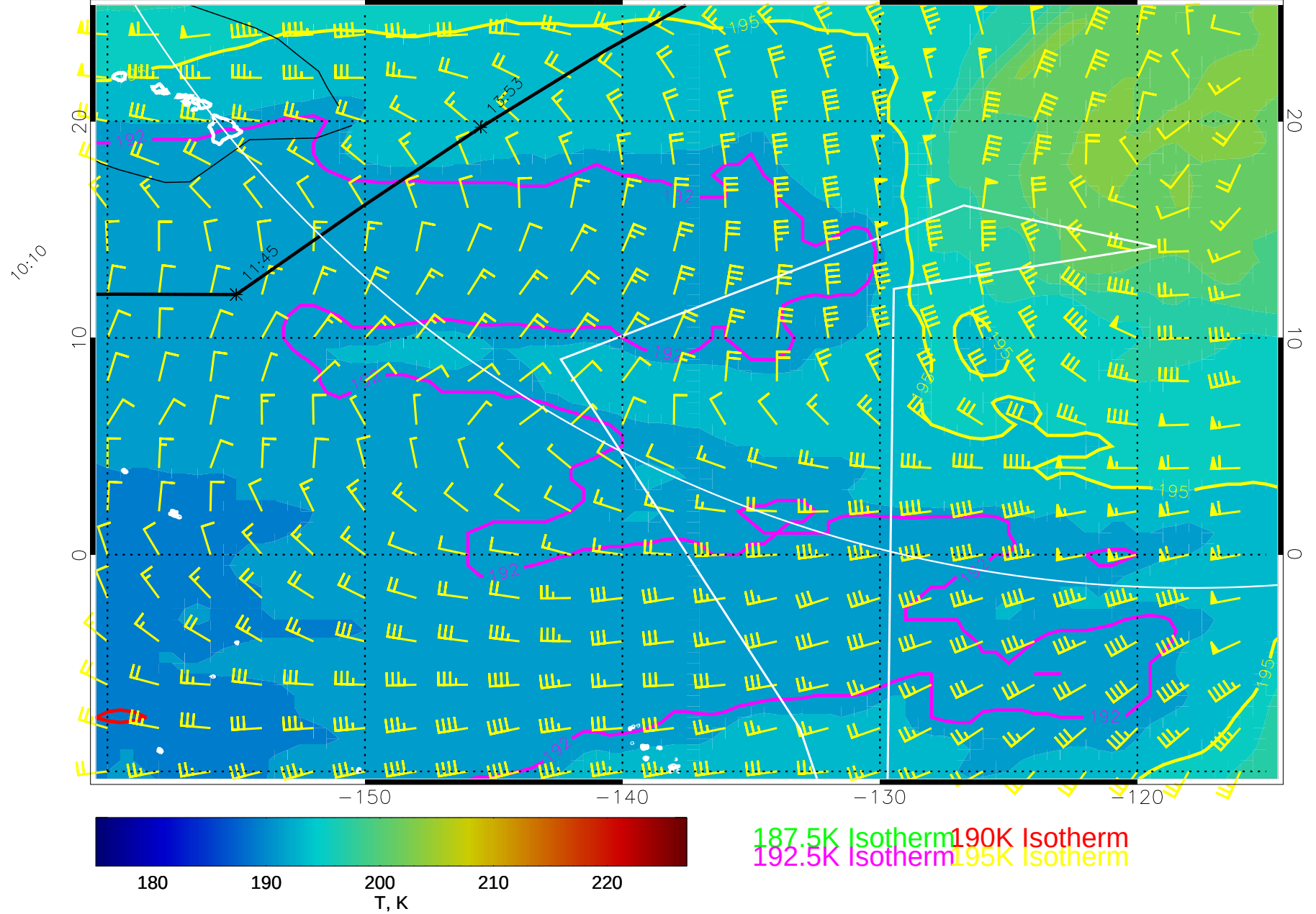
15011618, 78 hour forecast for 100mb T and winds (knots) -- NCEP GFS
