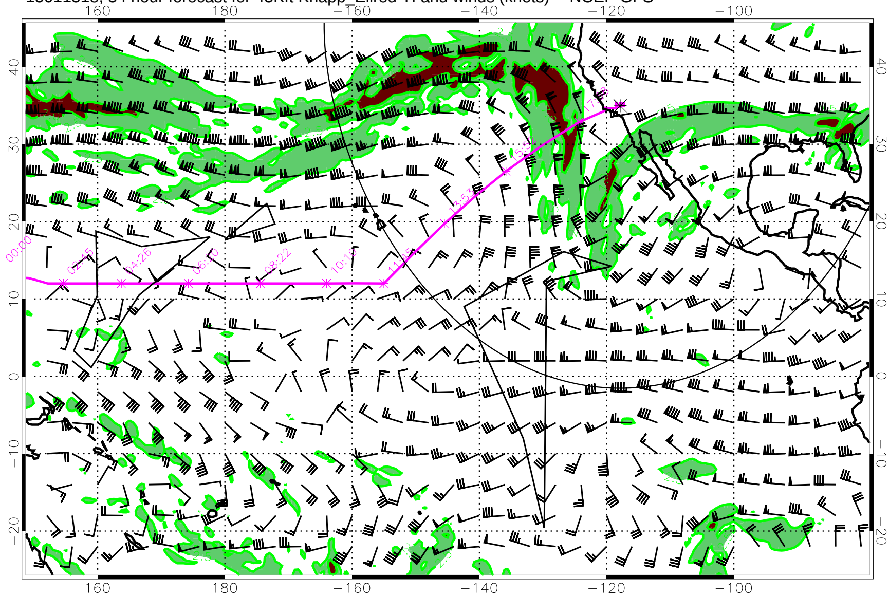
15011518, 54 hour forecast for 45Kft Knapp_Ellrod TI and winds (knots) -- NCEP GFS
