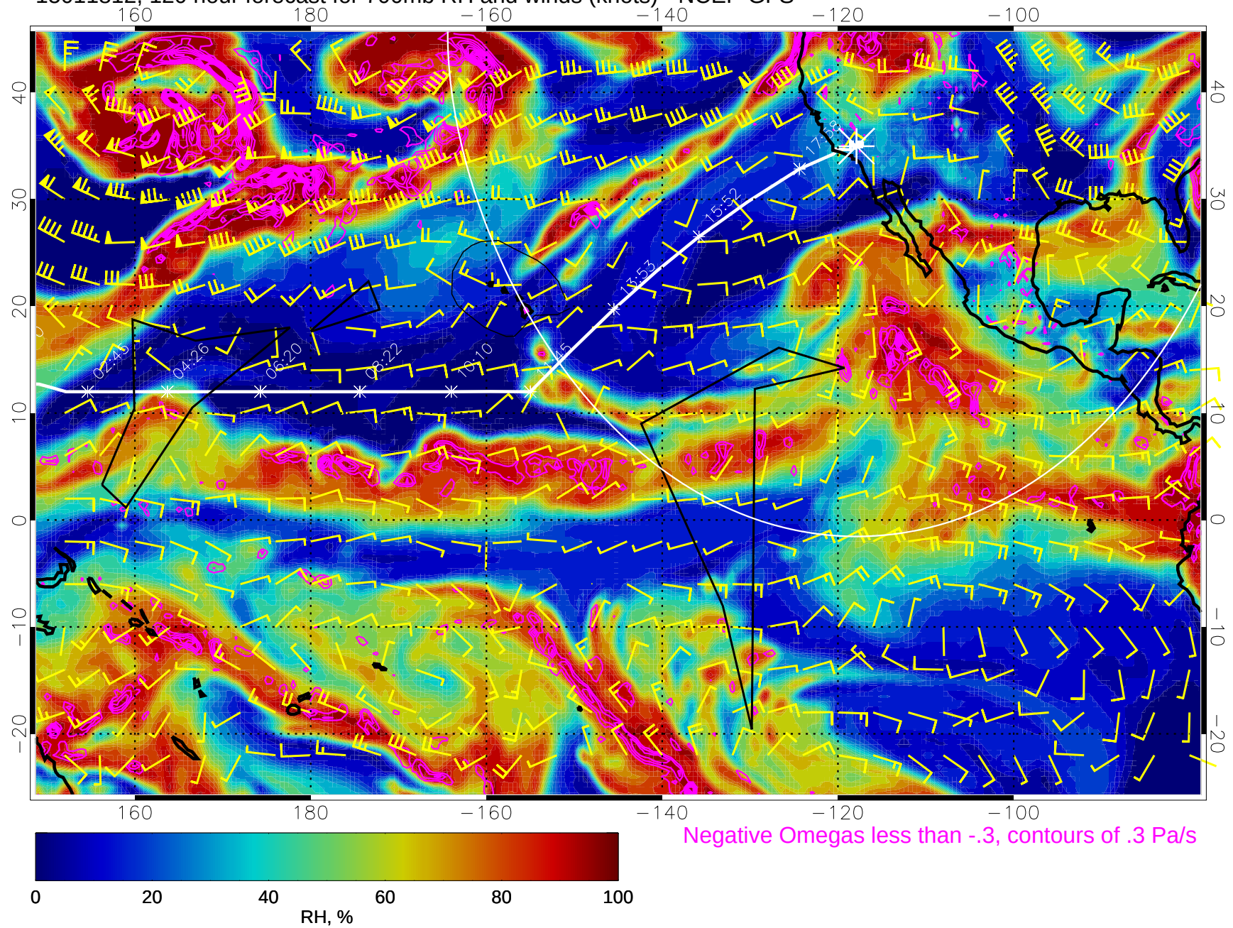
15011812, 120 hour forecast for 700mb RH and winds (knots) - NCEP GFS
