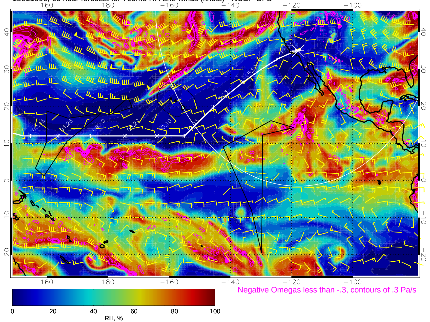
15011600, 60 hour forecast for 700mb RH and winds (knots) - NCEP GFS
