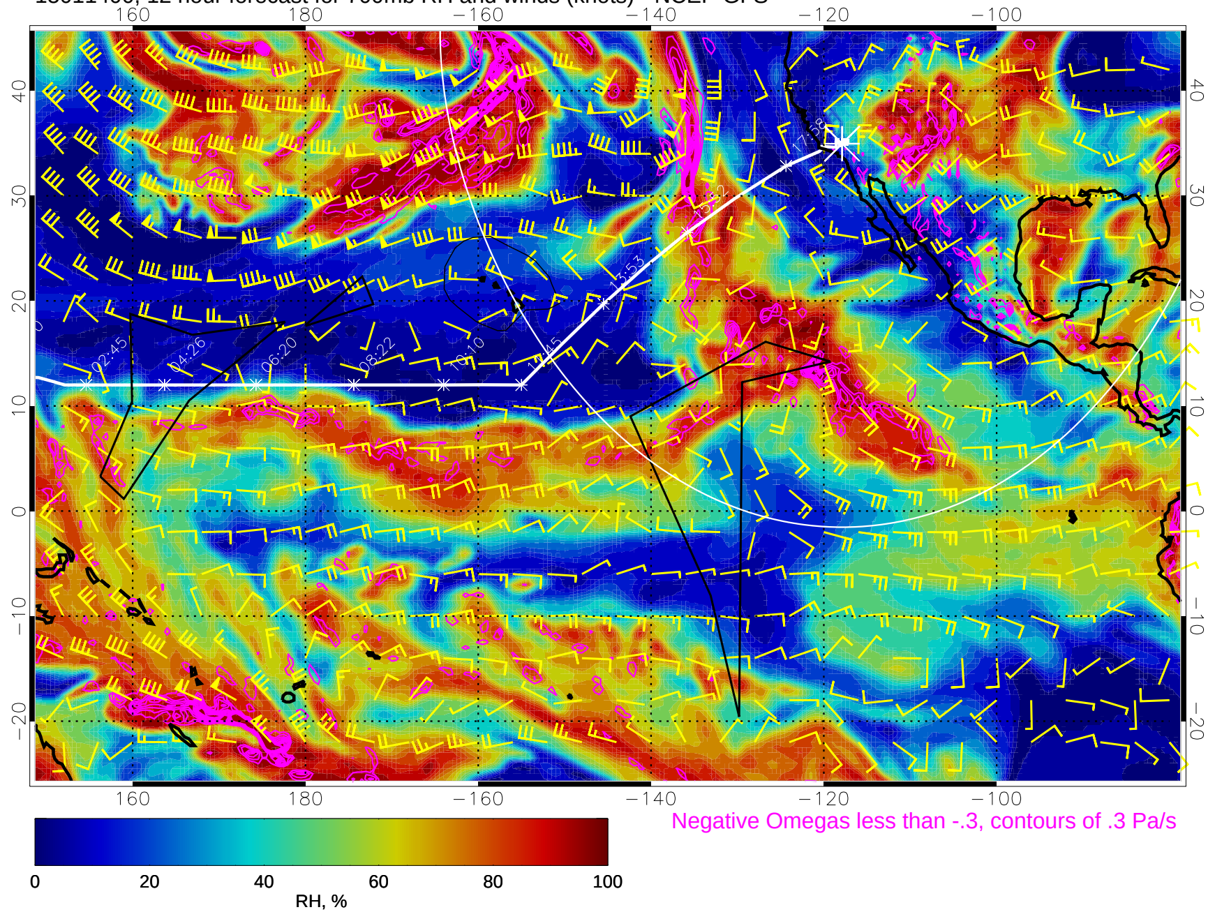
15011400, 12 hour forecast for 700mb RH and winds (knots) - NCEP GFS
