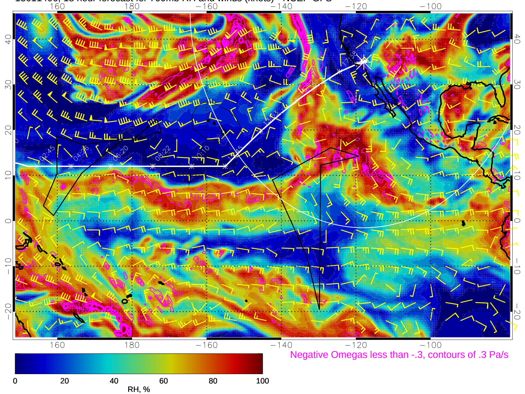
15011406, 18 hour forecast for 700mb RH and winds (knots) - NCEP GFS
