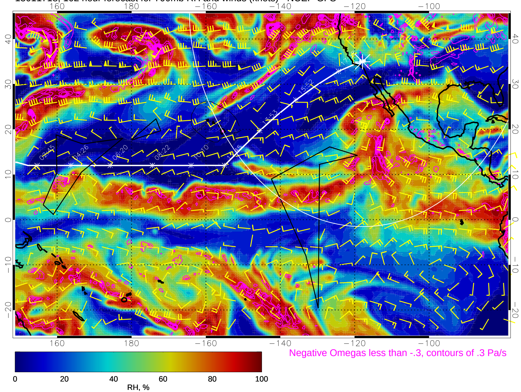
15011718, 102 hour forecast for 700mb RH and winds (knots) - NCEP GFS
