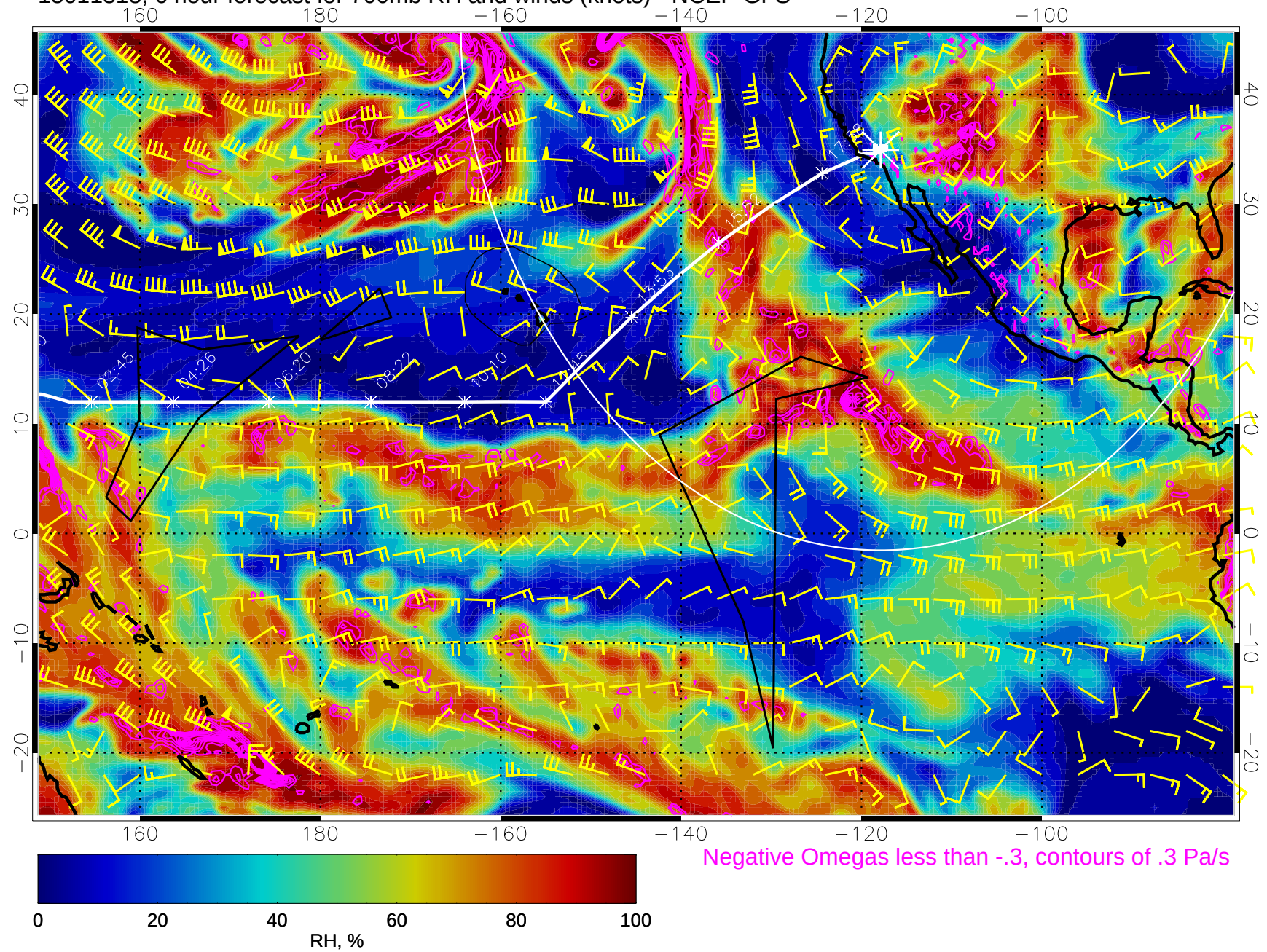
15011318, 6 hour forecast for 700mb RH and winds (knots) - NCEP GFS
