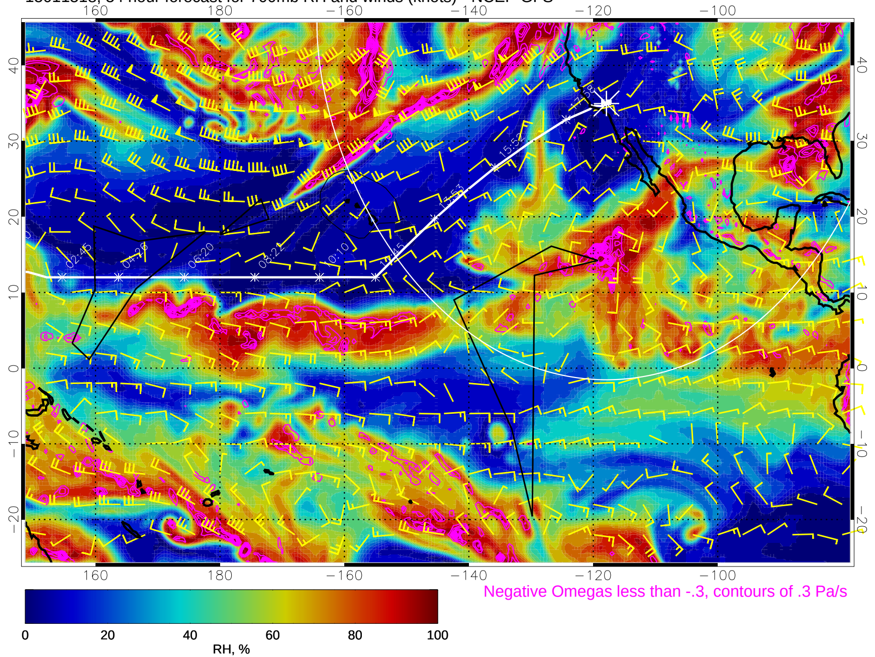
15011518, 54 hour forecast for 700mb RH and winds (knots) - NCEP GFS
