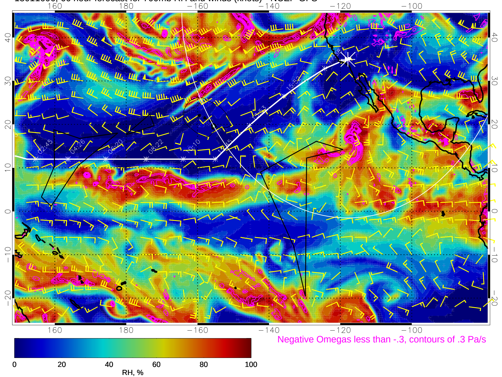
15011606, 66 hour forecast for 700mb RH and winds (knots) - NCEP GFS
