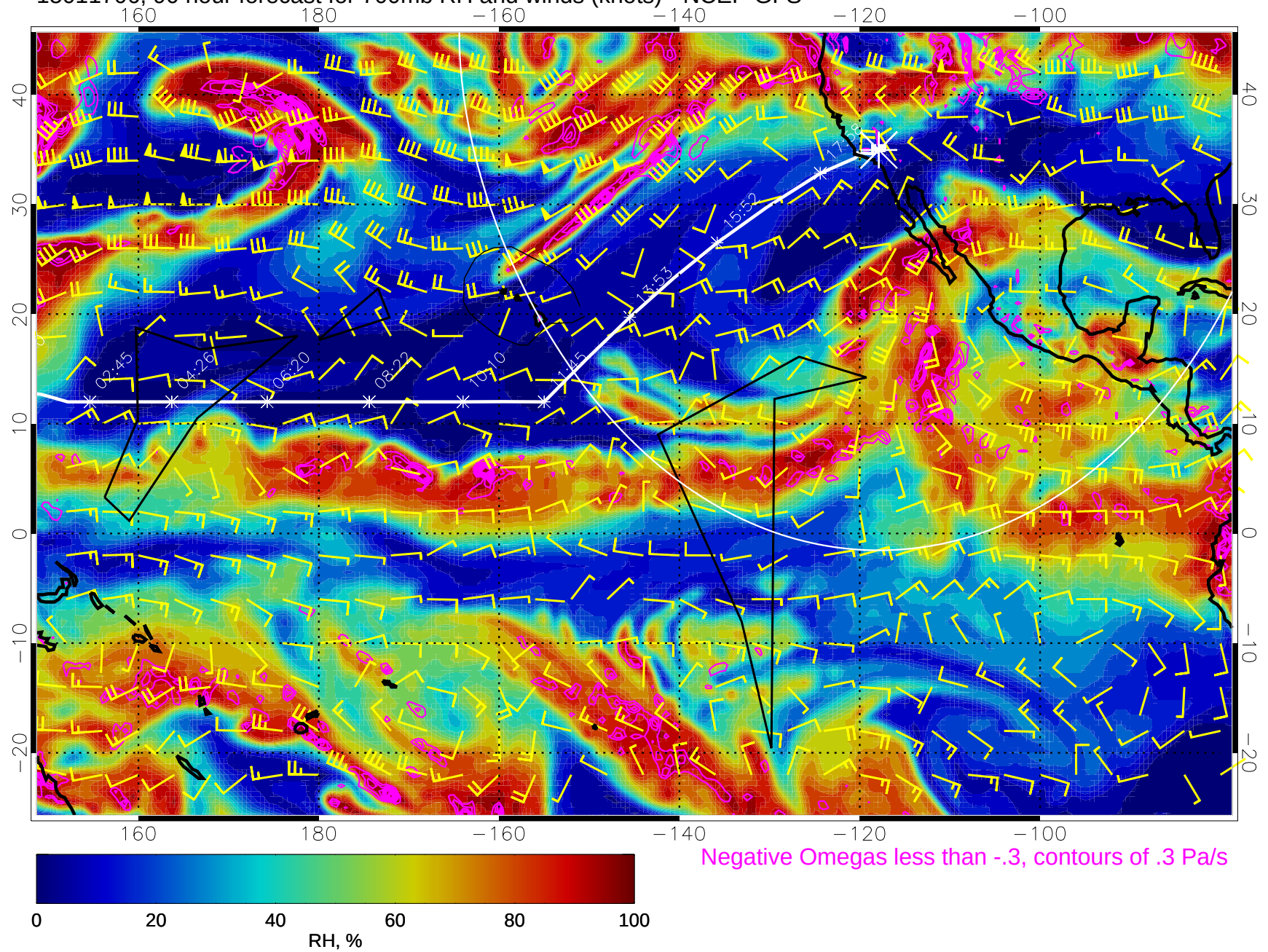
15011706, 90 hour forecast for 700mb RH and winds (knots) - NCEP GFS
