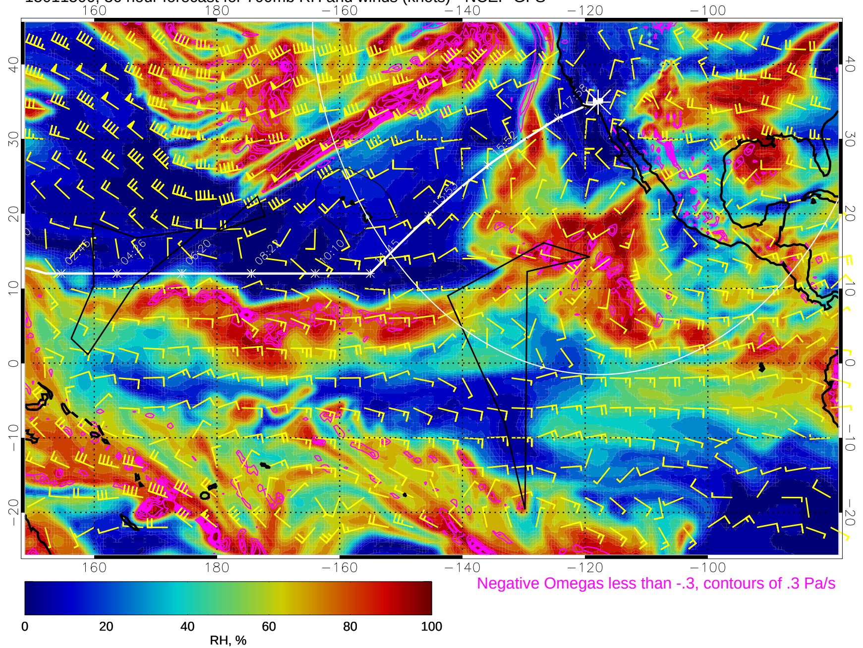
15011500, 36 hour forecast for 700mb RH and winds (knots) - NCEP GFS
