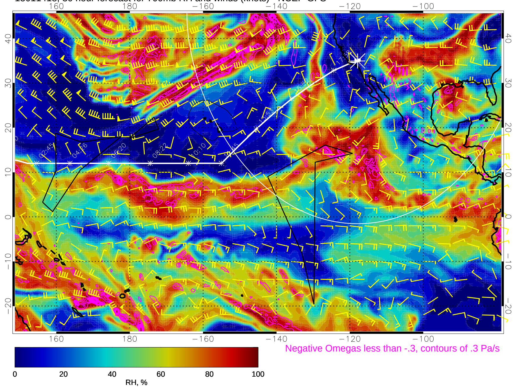
15011418, 30 hour forecast for 700mb RH and winds (knots) - NCEP GFS
