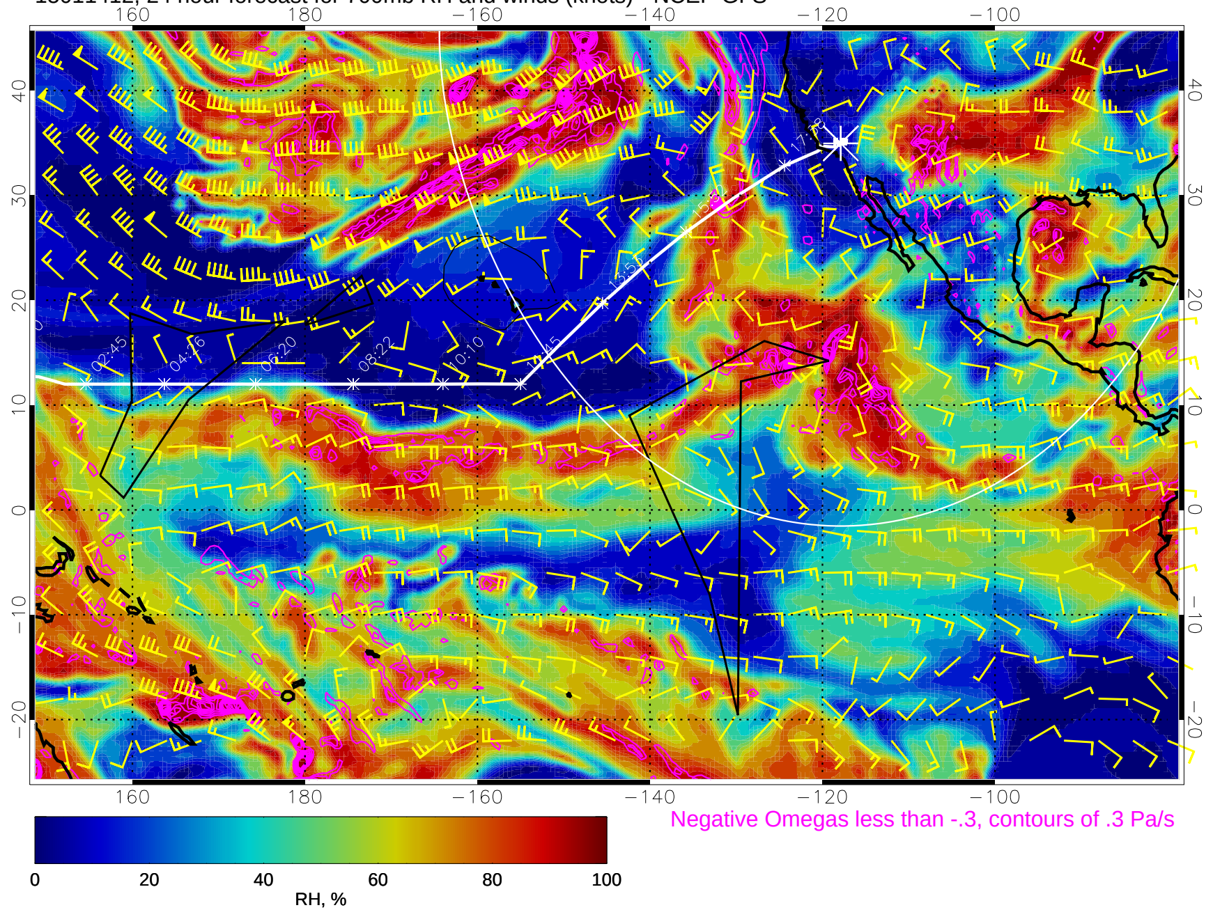
15011412, 24 hour forecast for 700mb RH and winds (knots) - NCEP GFS
