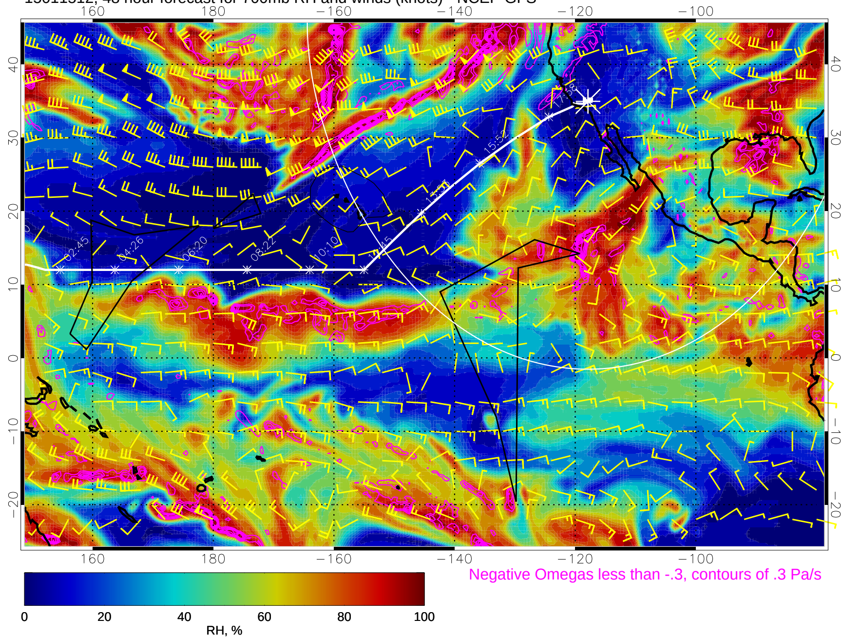
15011512, 48 hour forecast for 700mb RH and winds (knots) - NCEP GFS
