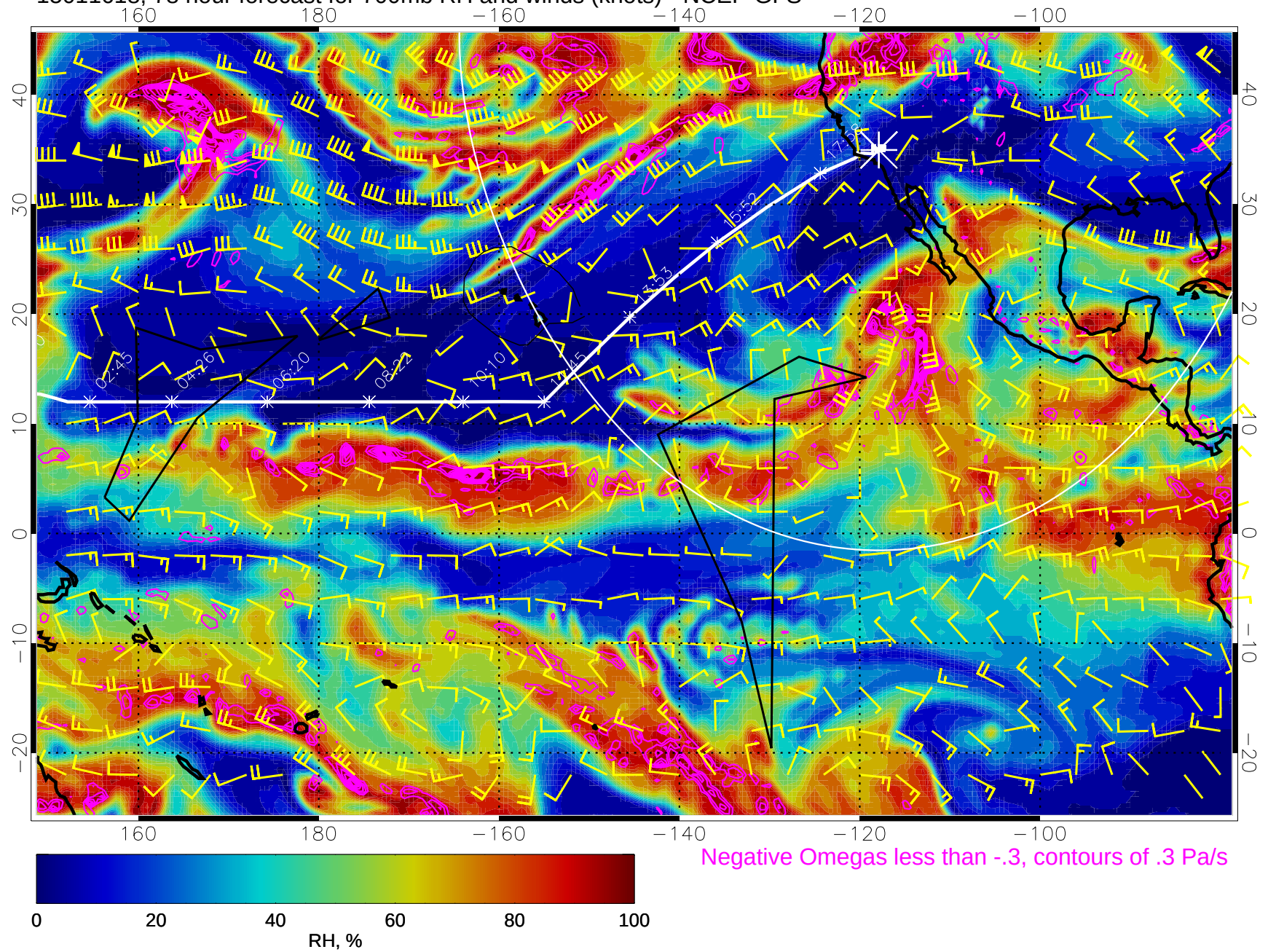
15011618, 78 hour forecast for 700mb RH and winds (knots) - NCEP GFS
