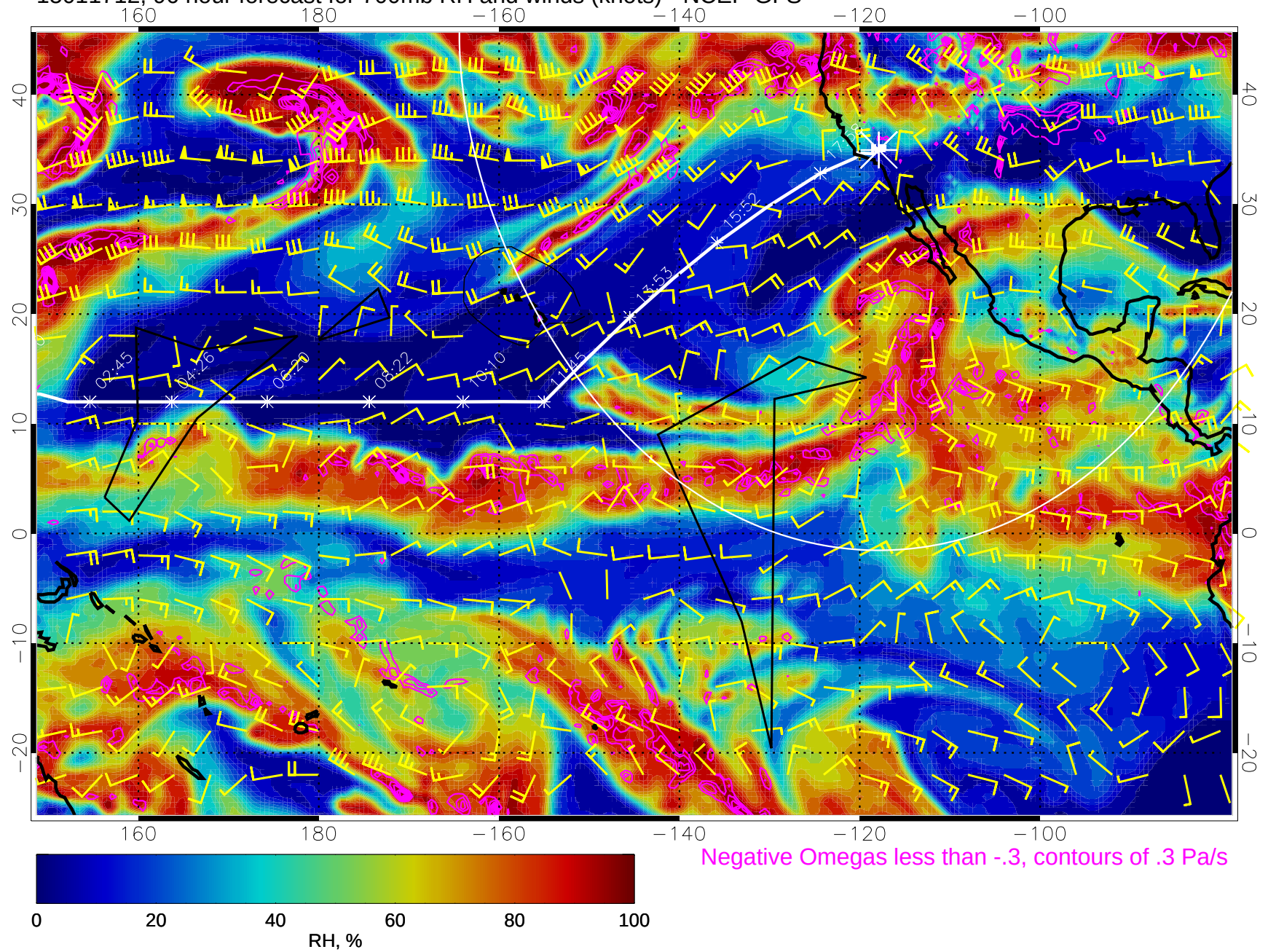
15011712, 96 hour forecast for 700mb RH and winds (knots) - NCEP GFS
