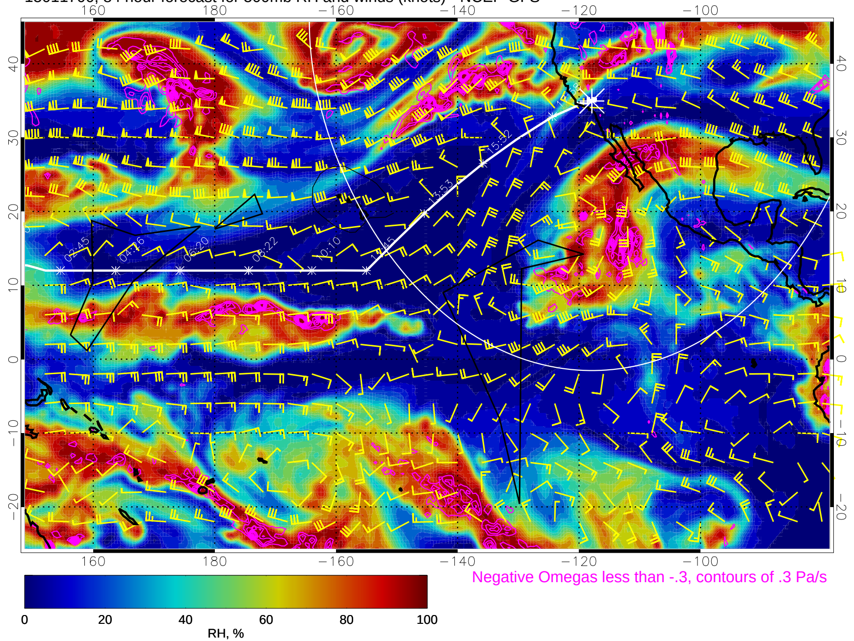
15011700, 84 hour forecast for 500mb RH and winds (knots) - NCEP GFS
