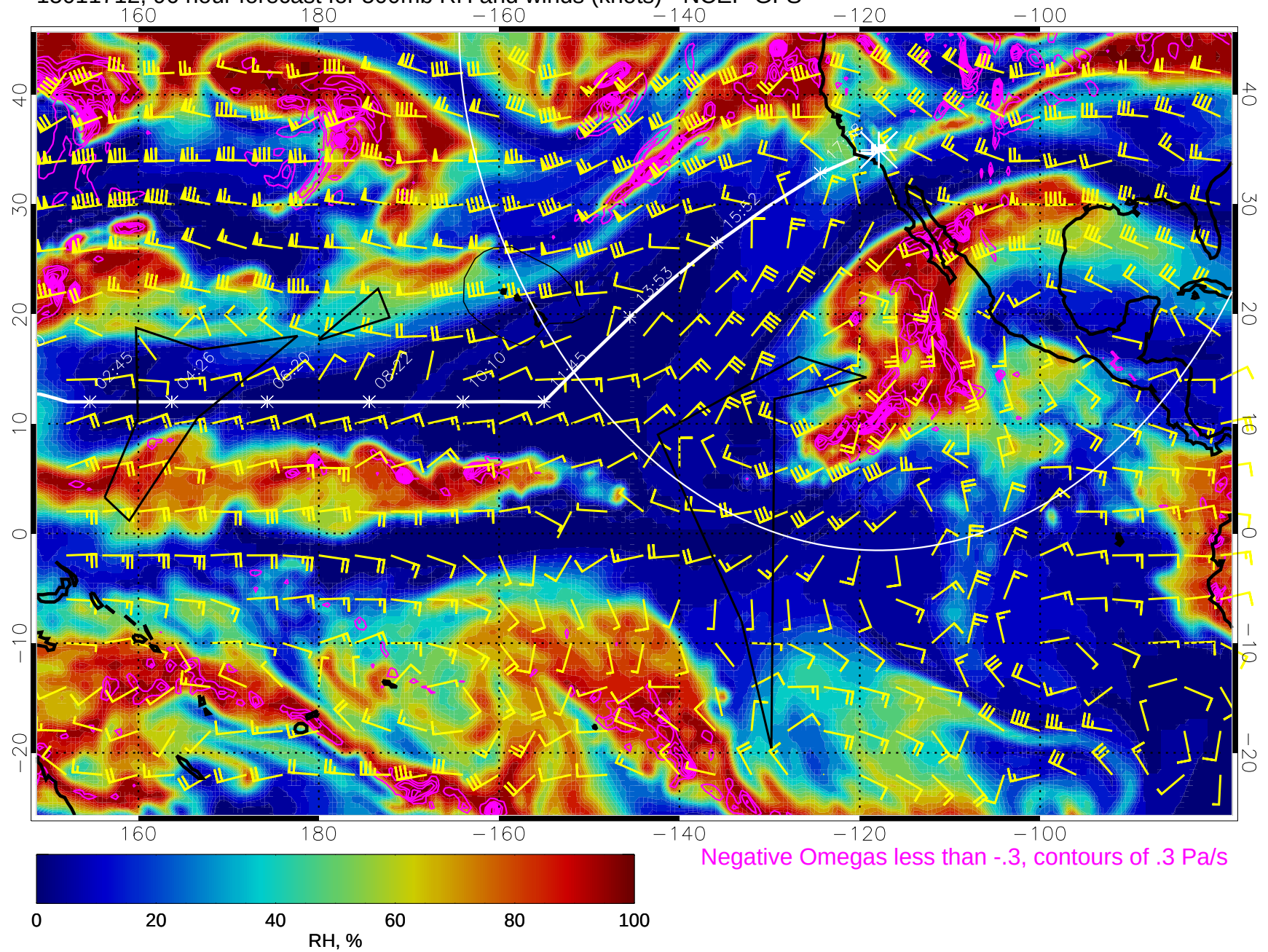
15011712, 96 hour forecast for 500mb RH and winds (knots) - NCEP GFS
