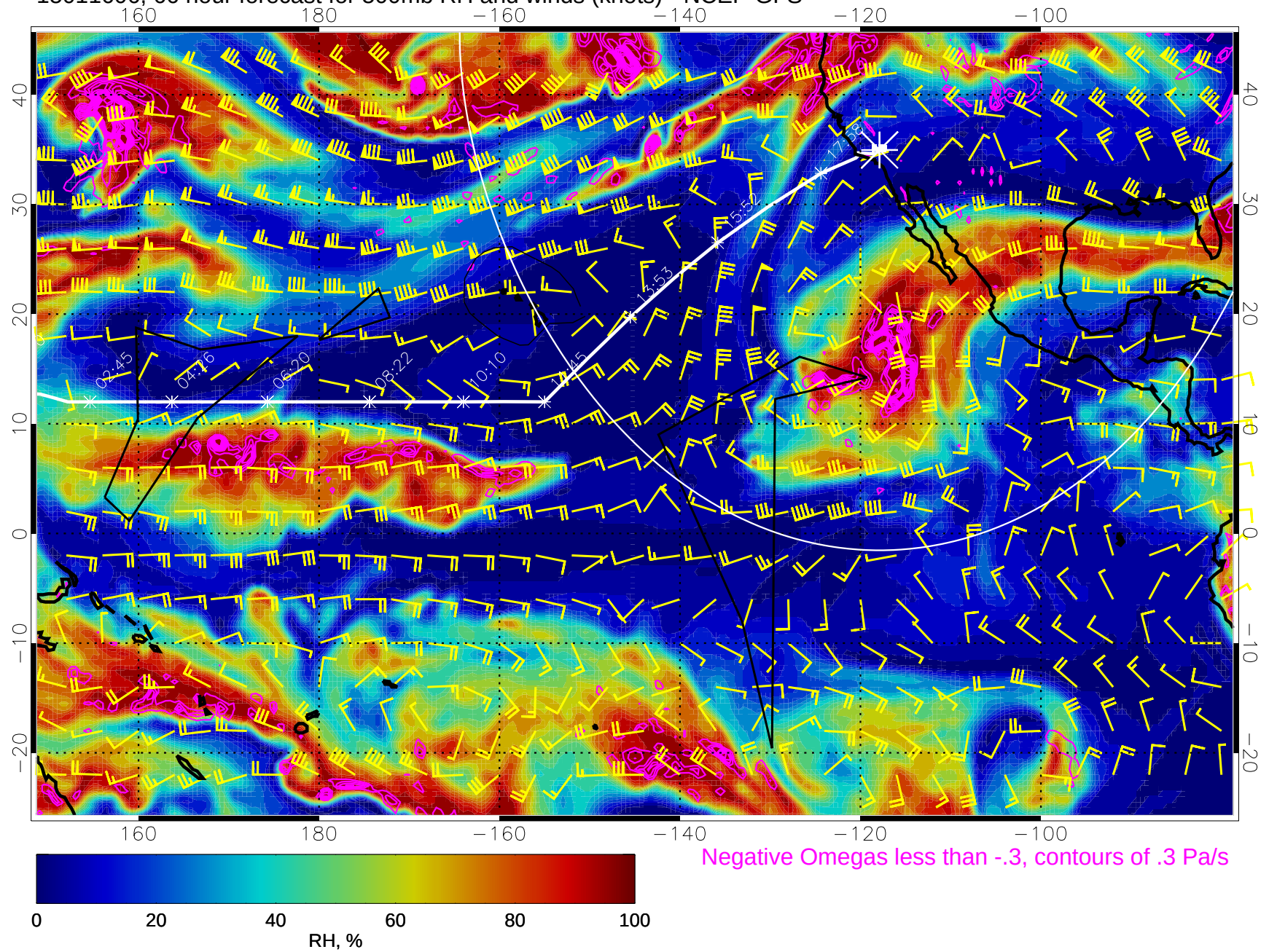
15011606, 66 hour forecast for 500mb RH and winds (knots) - NCEP GFS
