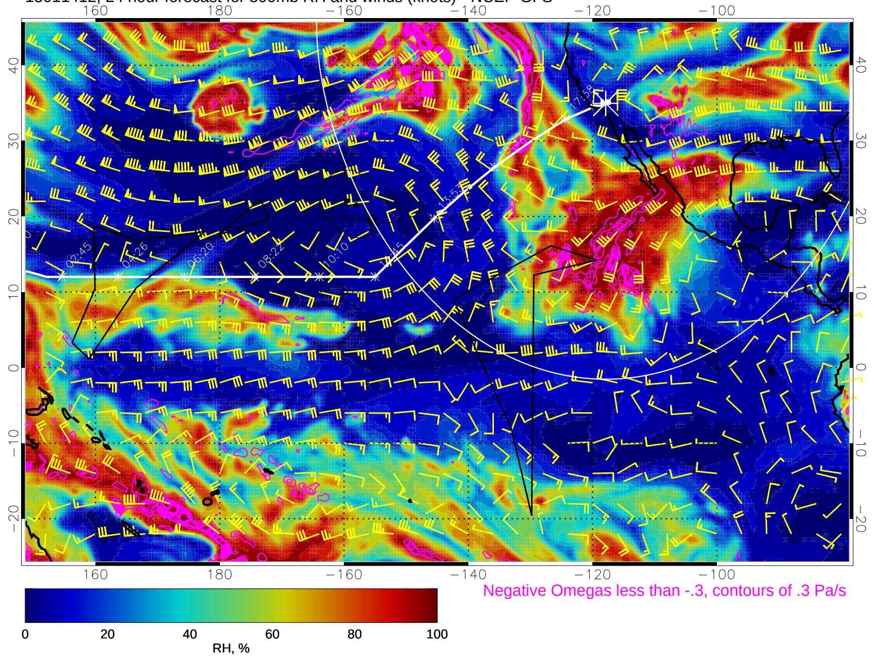
15011412, 24 hour forecast for 500mb RH and winds (knots) - NCEP GFS
