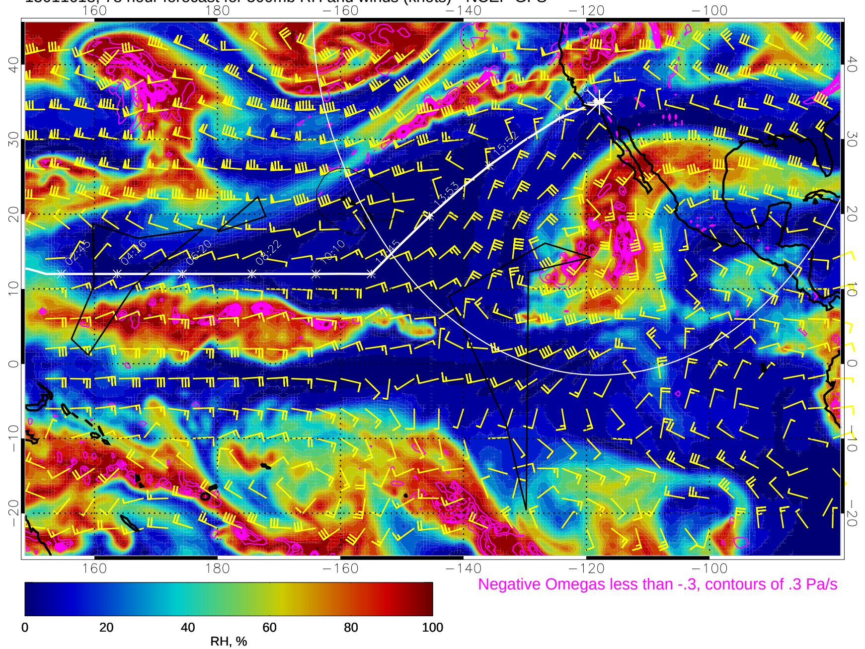
15011618, 78 hour forecast for 500mb RH and winds (knots) - NCEP GFS
