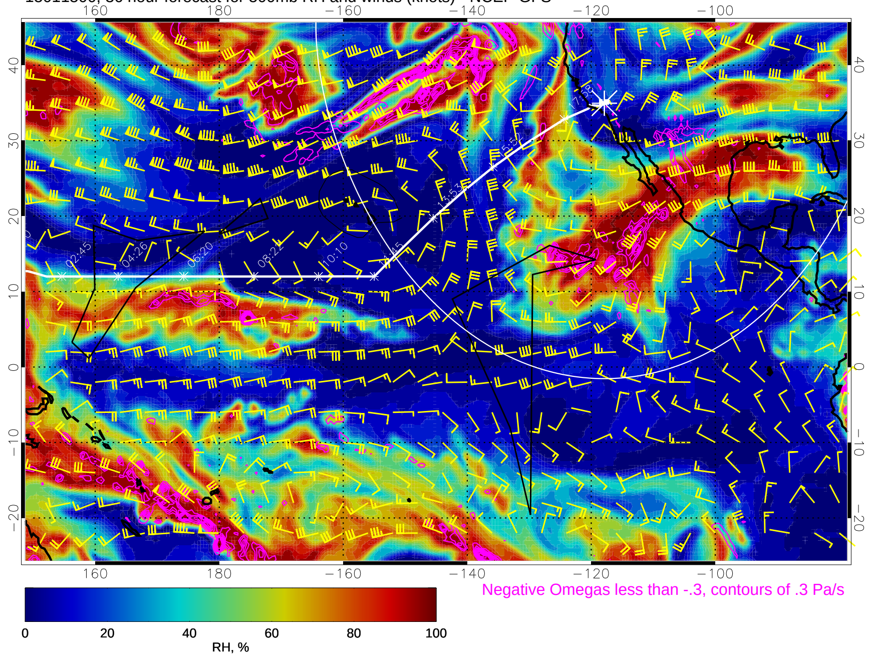
15011500, 36 hour forecast for 500mb RH and winds (knots) - NCEP GFS
