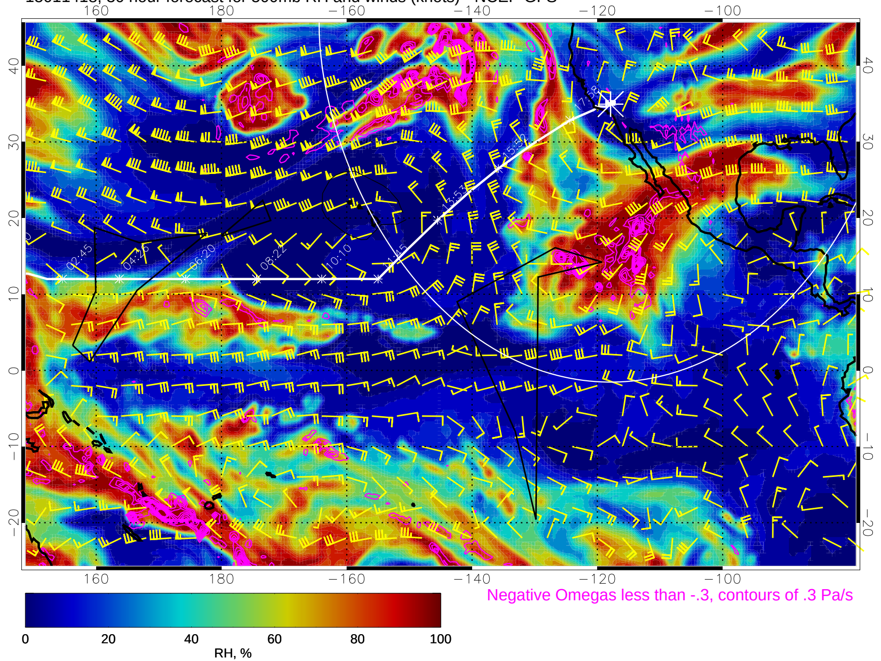
15011418, 30 hour forecast for 500mb RH and winds (knots) - NCEP GFS
