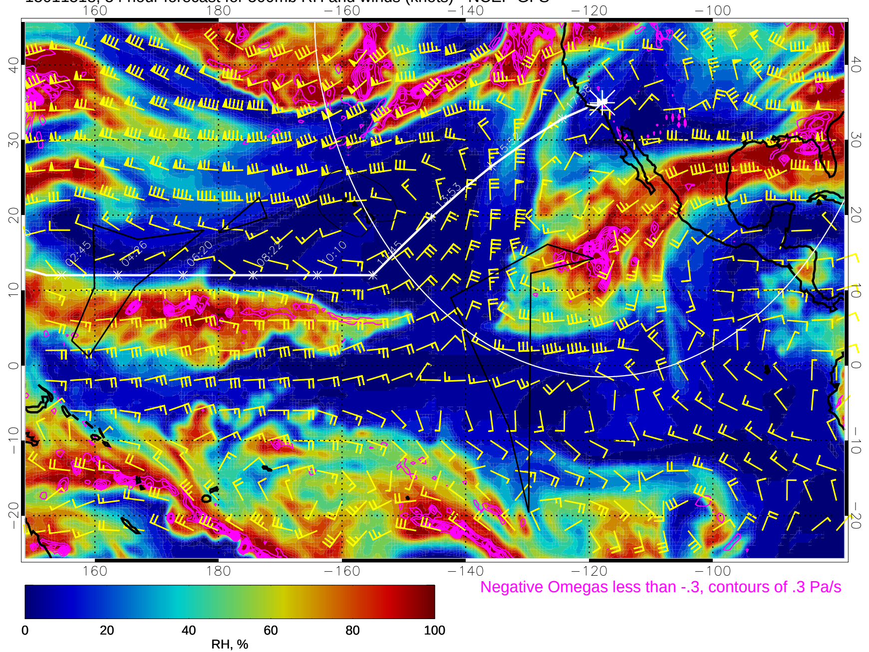
15011518, 54 hour forecast for 500mb RH and winds (knots) - NCEP GFS
