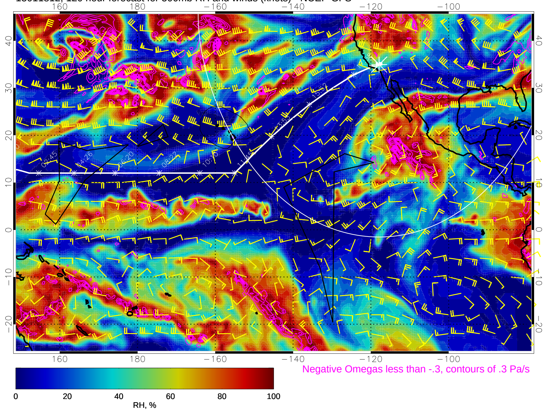
15011812, 120 hour forecast for 500mb RH and winds (knots) - NCEP GFS
