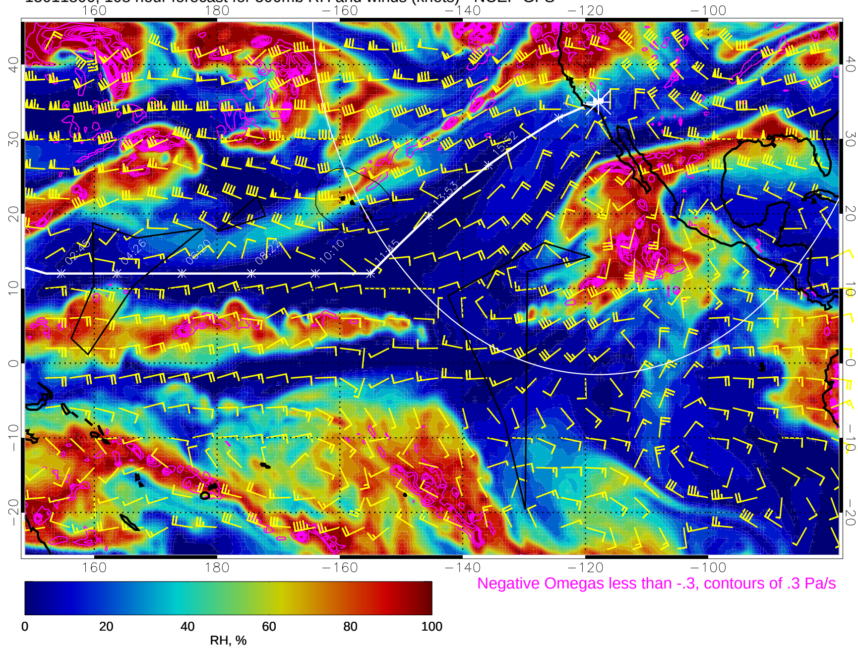
15011800, 108 hour forecast for 500mb RH and winds (knots) - NCEP GFS
