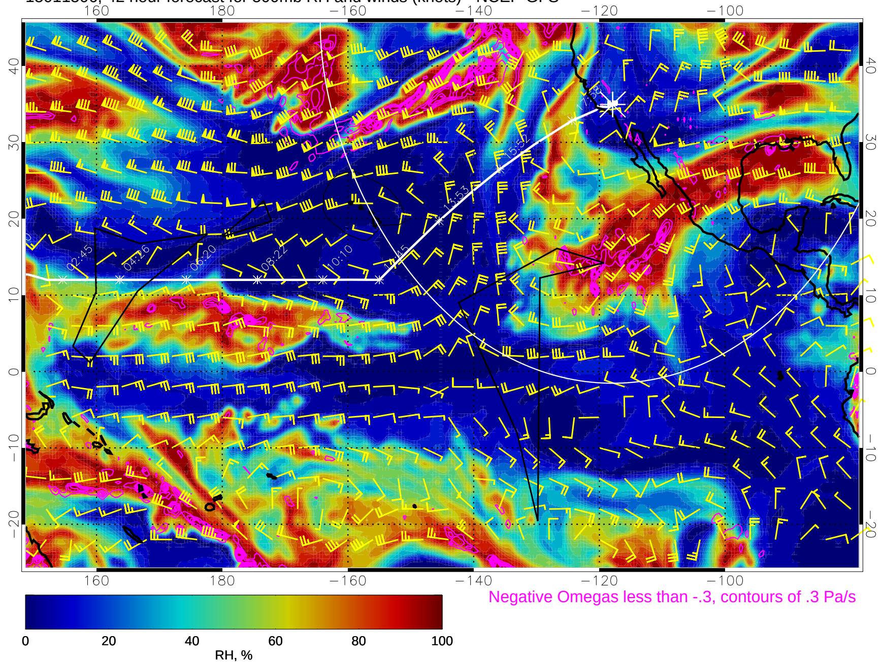
15011506, 42 hour forecast for 500mb RH and winds (knots) - NCEP GFS
