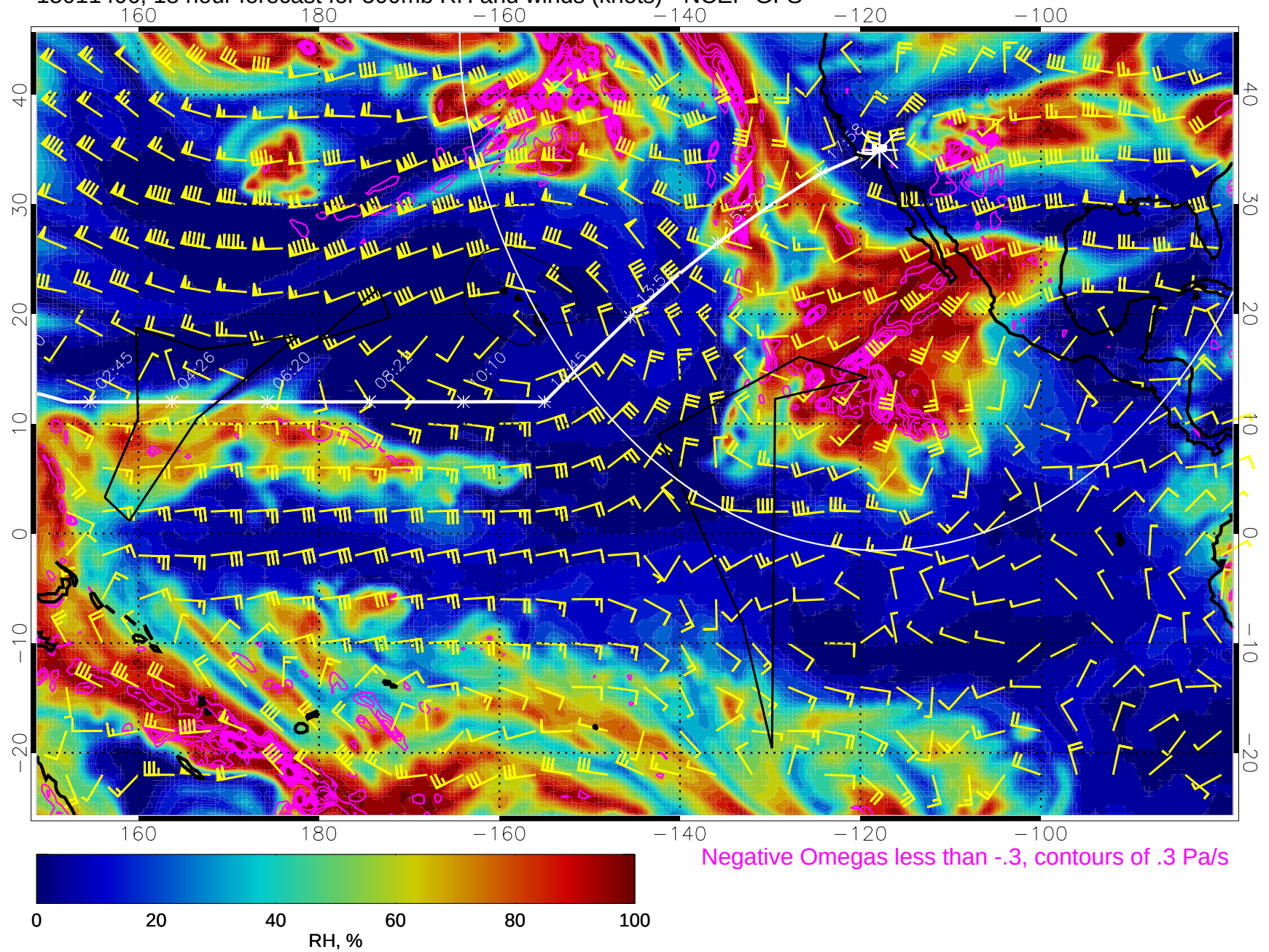
15011406, 18 hour forecast for 500mb RH and winds (knots) - NCEP GFS
