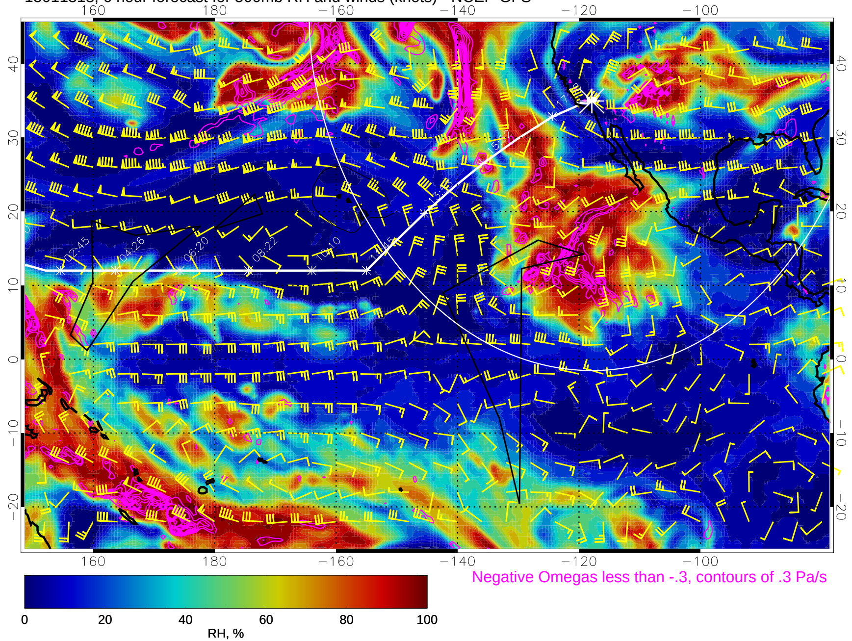
15011318, 6 hour forecast for 500mb RH and winds (knots) - NCEP GFS
