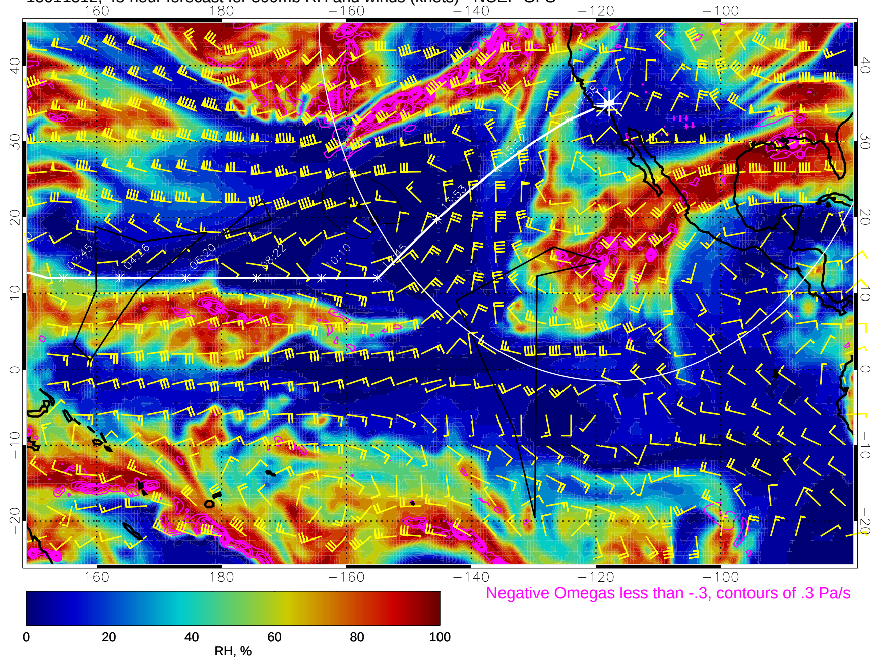
15011512, 48 hour forecast for 500mb RH and winds (knots) - NCEP GFS
