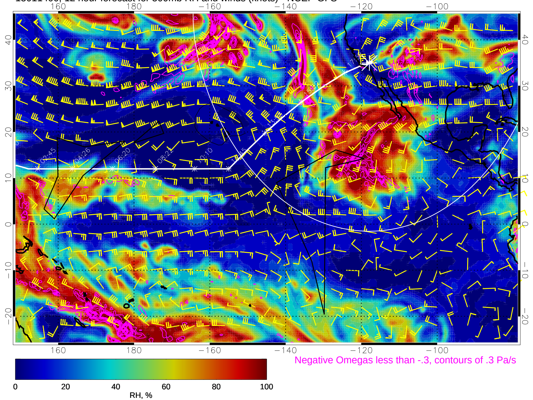
15011400, 12 hour forecast for 500mb RH and winds (knots) - NCEP GFS
