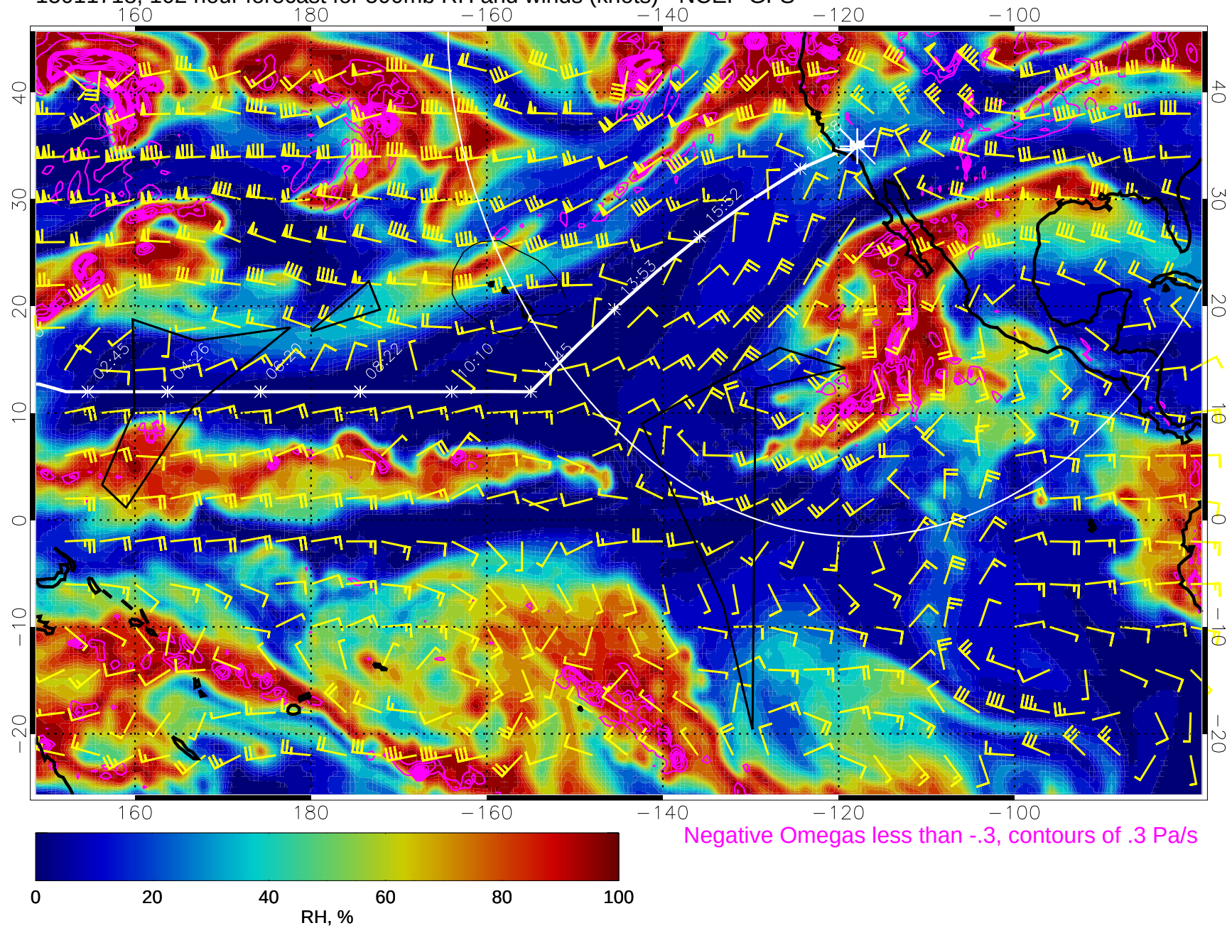
15011718, 102 hour forecast for 500mb RH and winds (knots) - NCEP GFS
