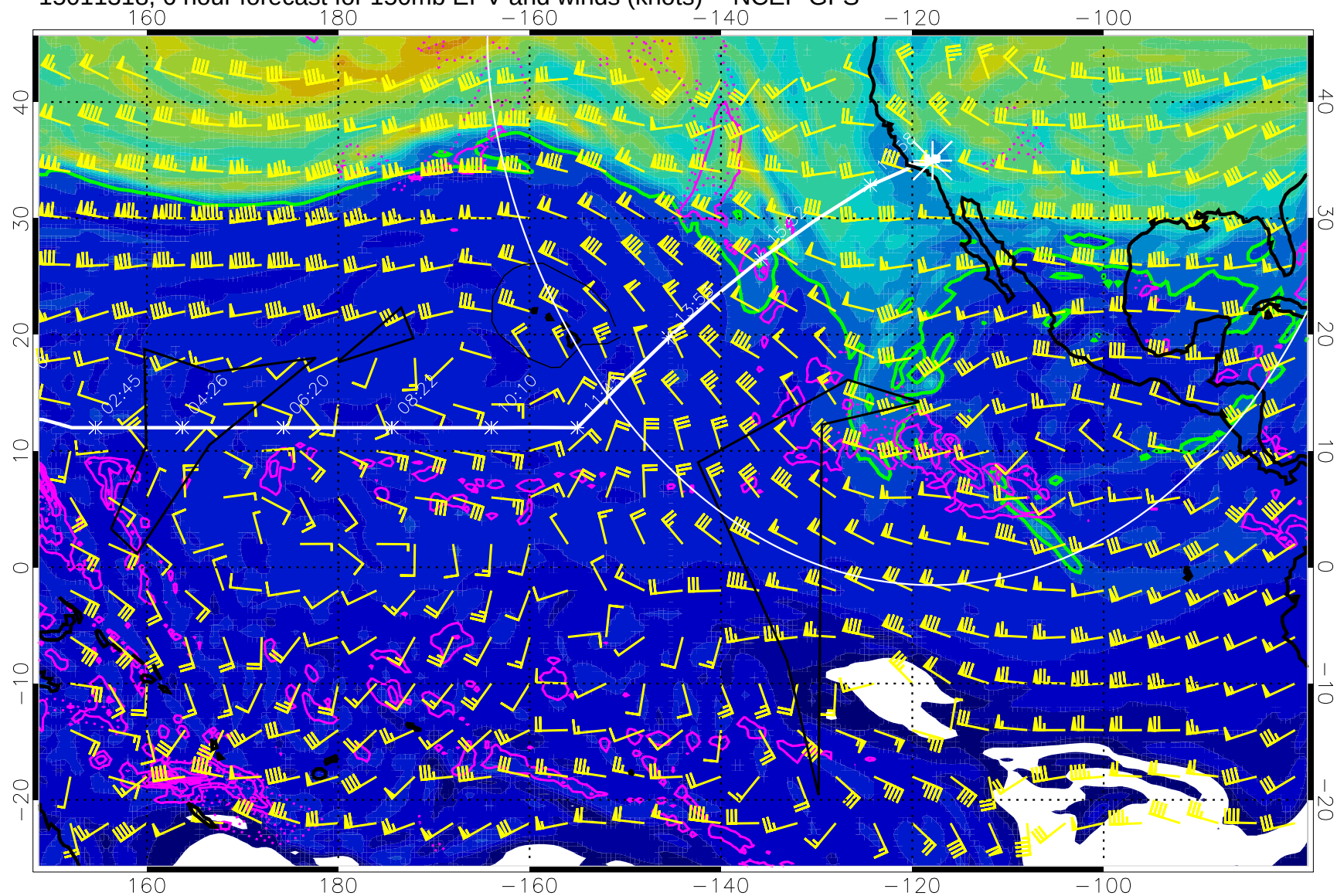
15011318, 6 hour forecast for 150mb EPV and winds (knots) -- NCEP GFS
