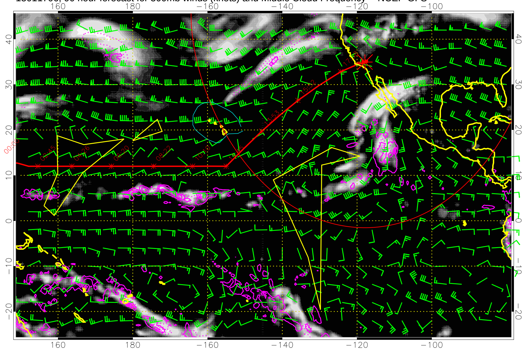
15011706, 90 hour forecast for 500mb winds (knots) and Middle Cloud Frequency -- NCEP GFS
