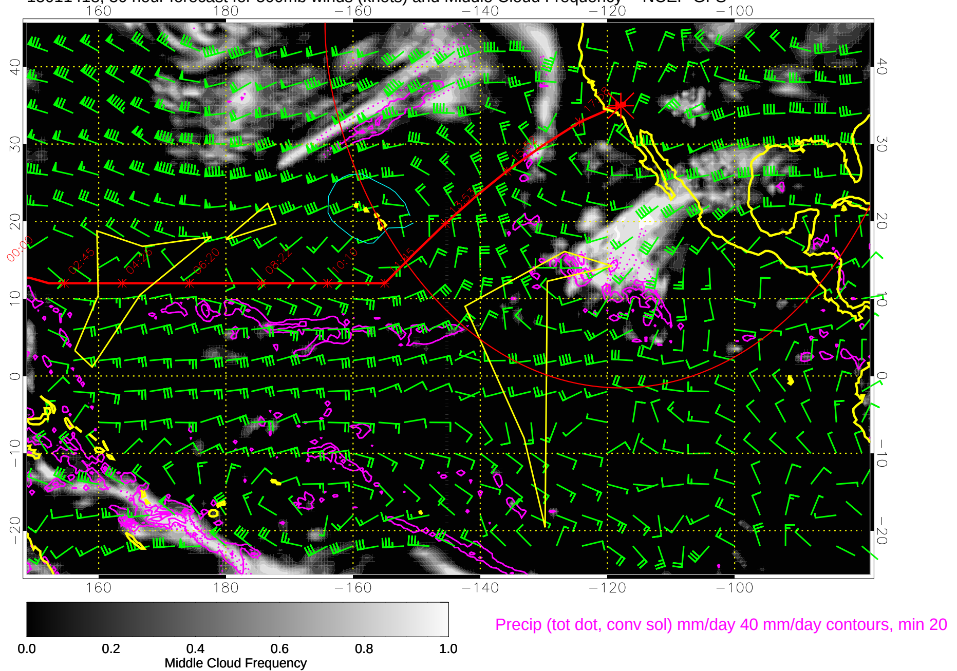
15011418, 30 hour forecast for 500mb winds (knots) and Middle Cloud Frequency -- NCEP GFS
