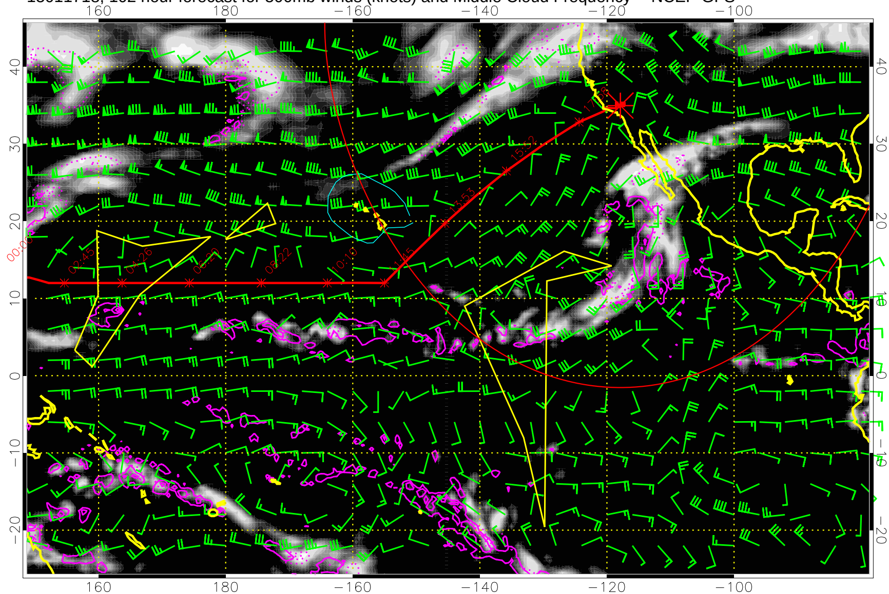
15011718, 102 hour forecast for 500mb winds (knots) and Middle Cloud Frequency -- NCEP GFS
