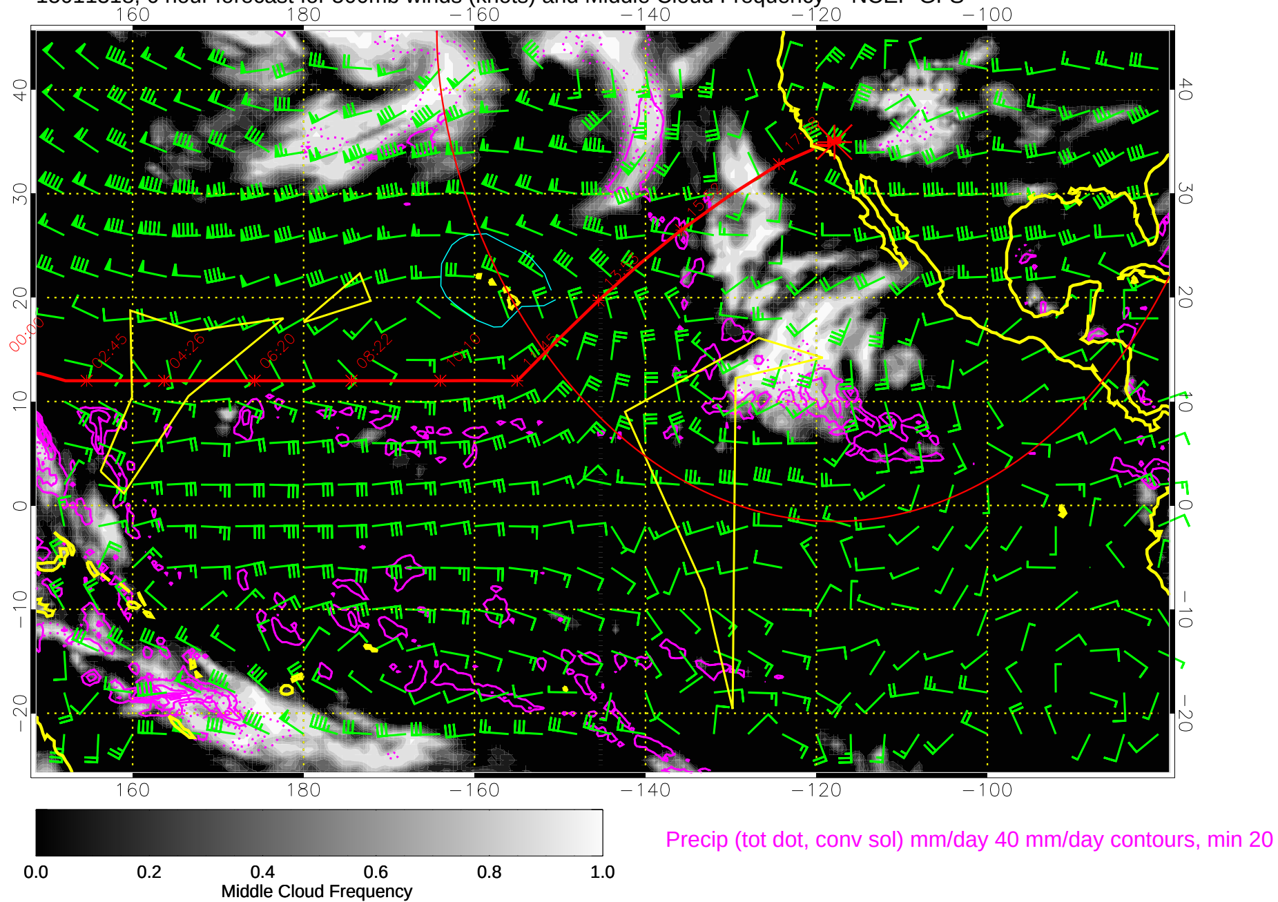
15011318, 6 hour forecast for 500mb winds (knots) and Middle Cloud Frequency -- NCEP GFS
