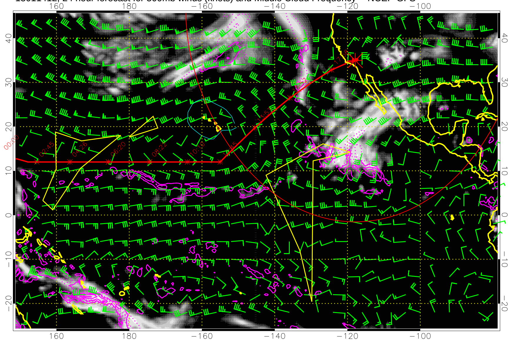
15011412, 24 hour forecast for 500mb winds (knots) and Middle Cloud Frequency -- NCEP GFS
