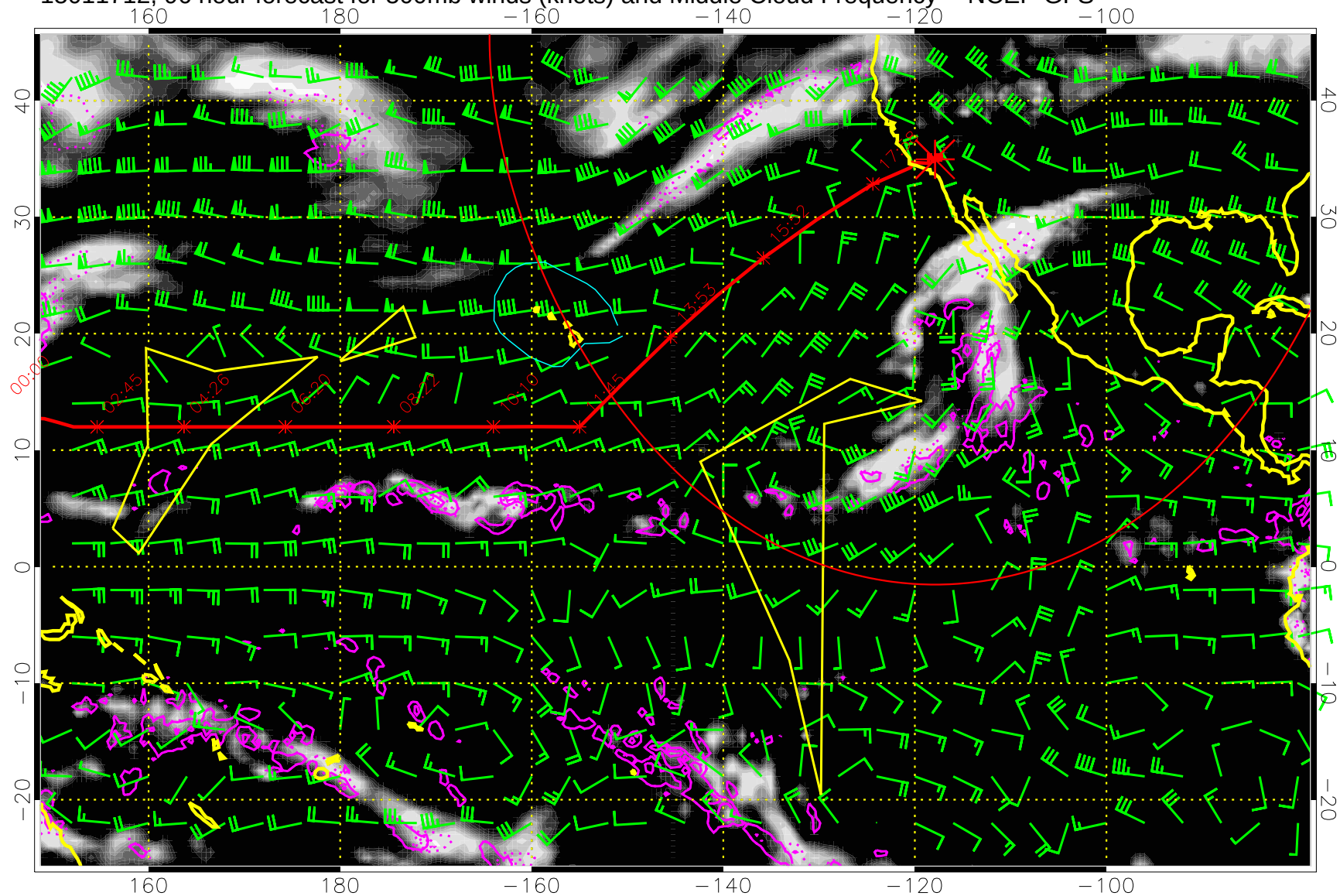
15011712, 96 hour forecast for 500mb winds (knots) and Middle Cloud Frequency -- NCEP GFS
