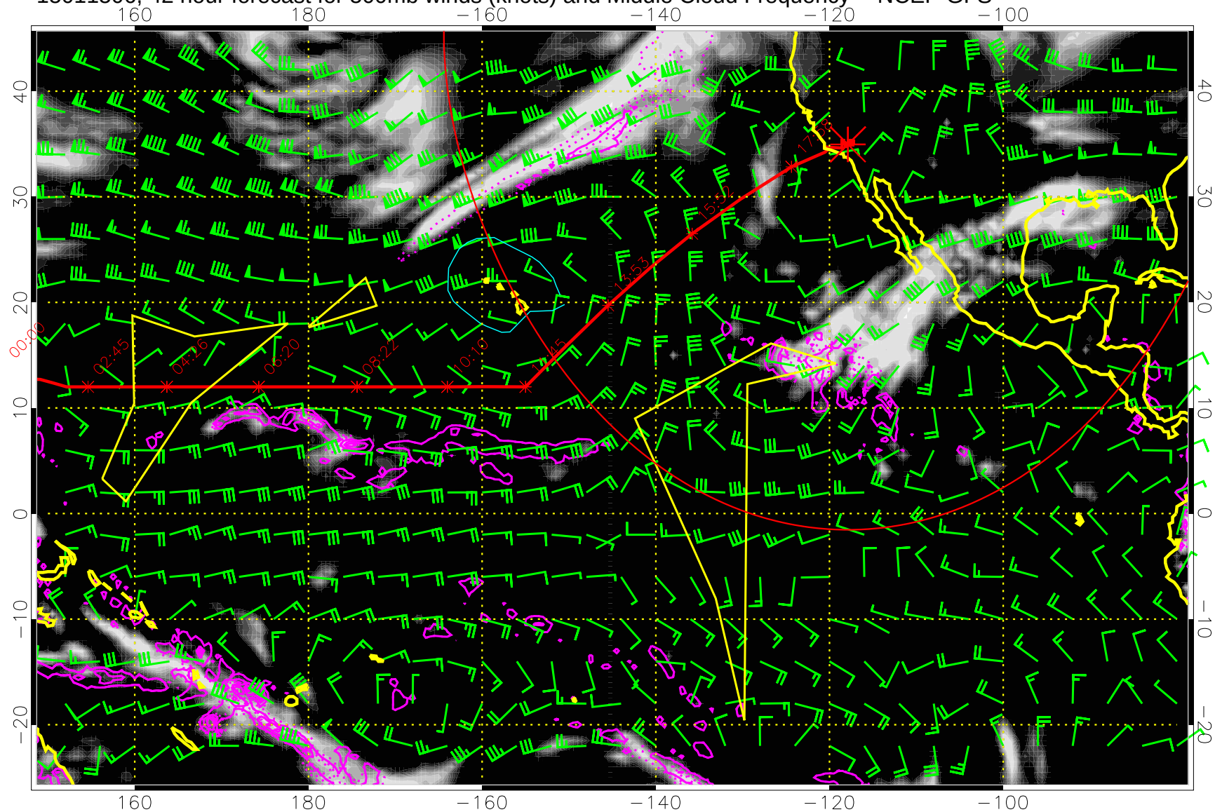
15011506, 42 hour forecast for 500mb winds (knots) and Middle Cloud Frequency -- NCEP GFS
