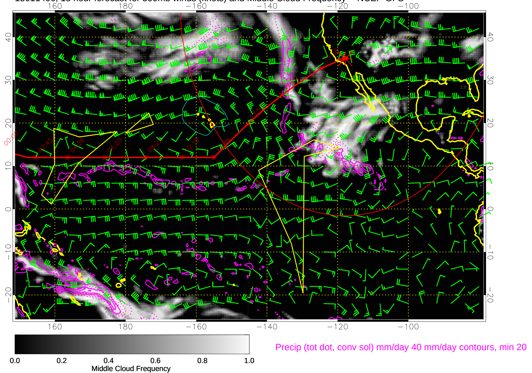
15011406, 18 hour forecast for 500mb winds (knots) and Middle Cloud Frequency -- NCEP GFS
