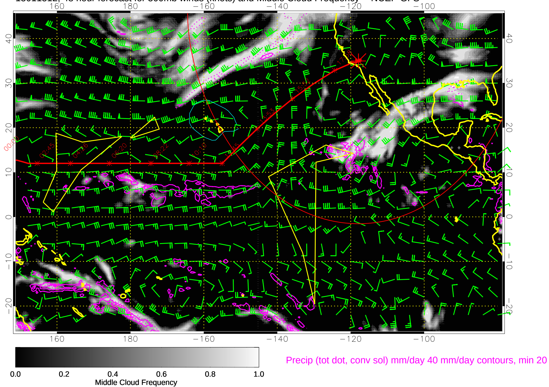
15011512, 48 hour forecast for 500mb winds (knots) and Middle Cloud Frequency -- NCEP GFS
