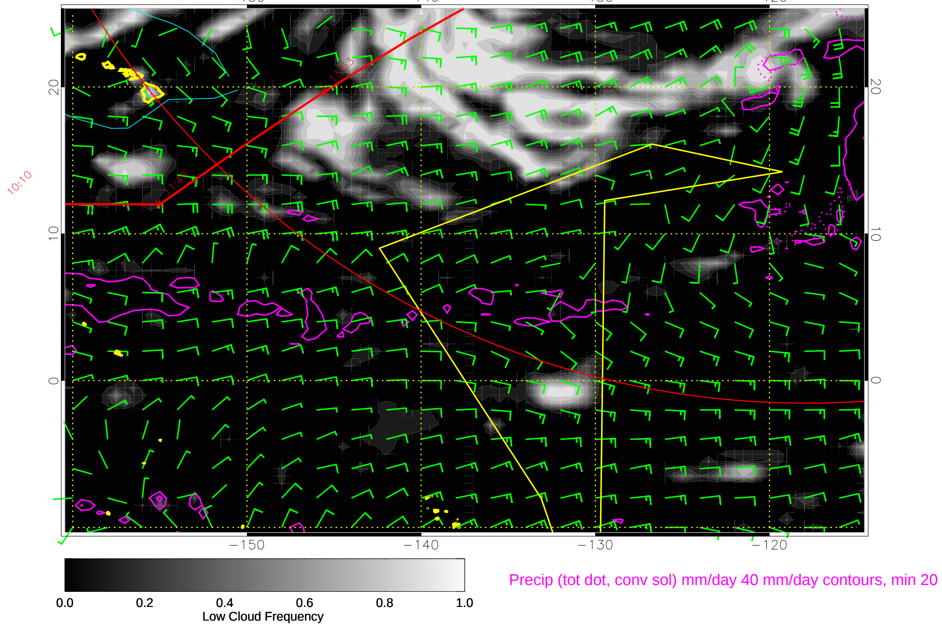
15011718, 102 hour forecast for 850mb winds (knots) and Low Cloud Frequency -- NCEP GFS
