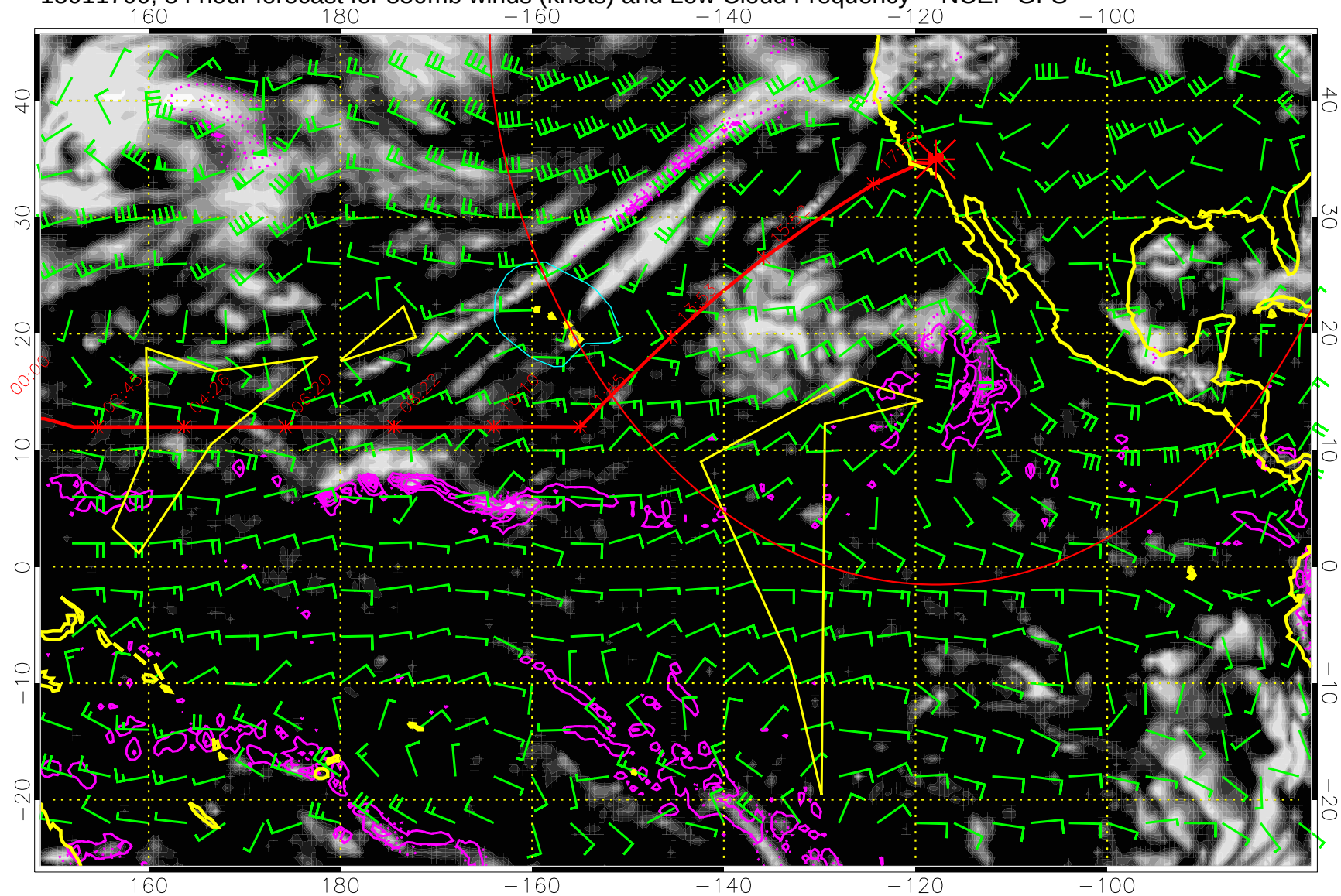
15011700, 84 hour forecast for 850mb winds (knots) and Low Cloud Frequency -- NCEP GFS
