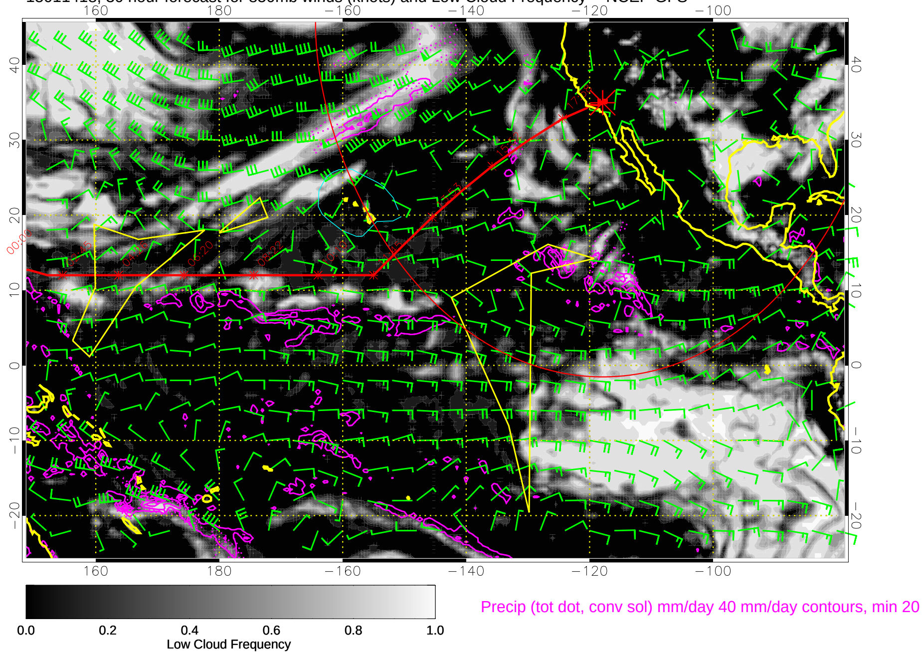
15011418, 30 hour forecast for 850mb winds (knots) and Low Cloud Frequency -- NCEP GFS
