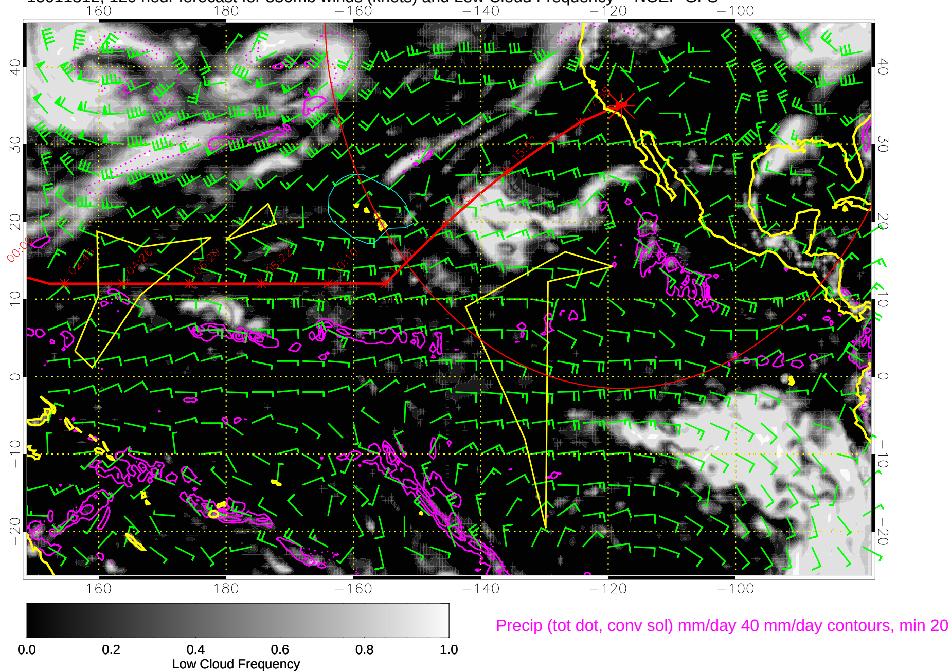
15011812, 120 hour forecast for 850mb winds (knots) and Low Cloud Frequency -- NCEP GFS
