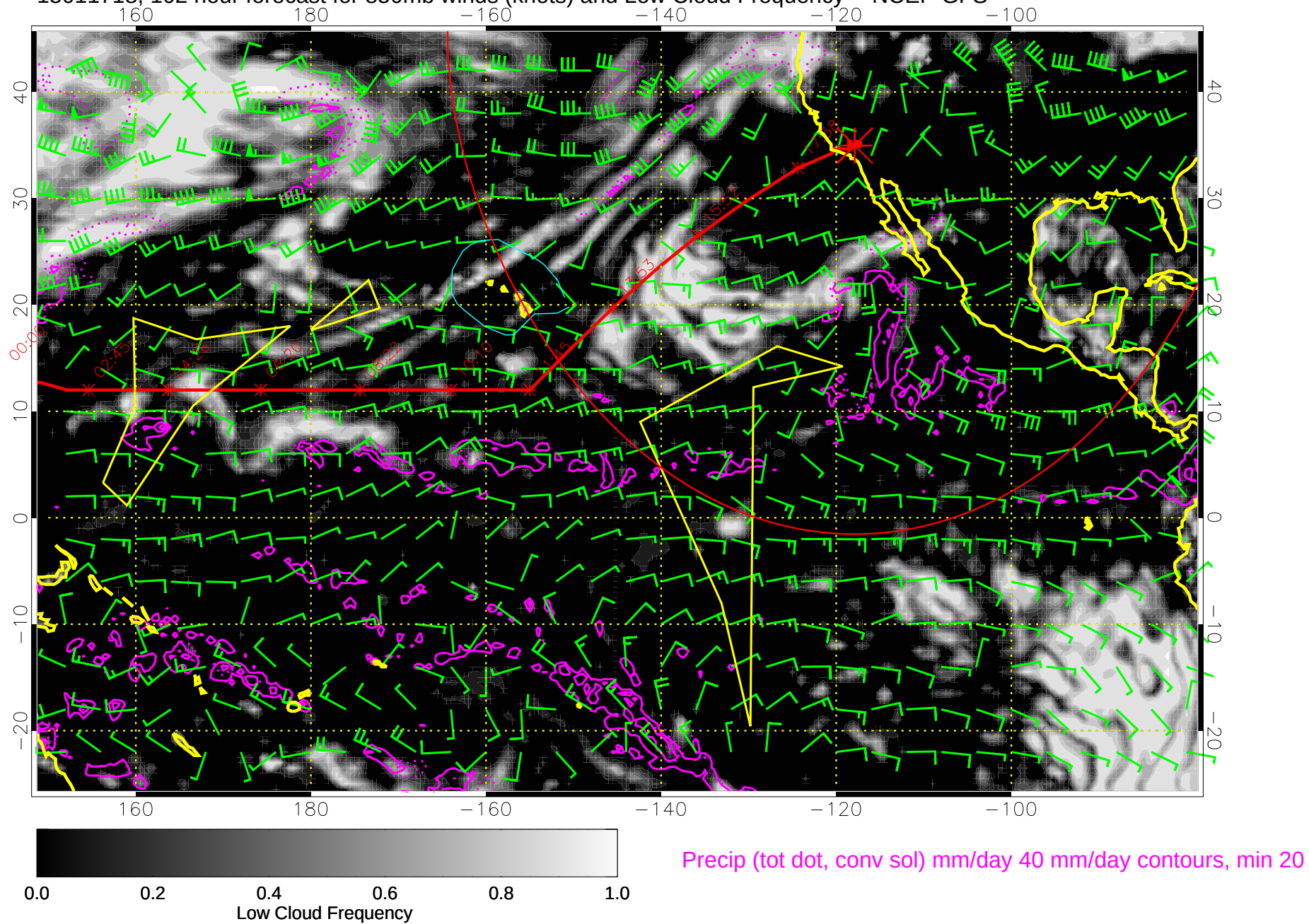
15011718, 102 hour forecast for 850mb winds (knots) and Low Cloud Frequency -- NCEP GFS
