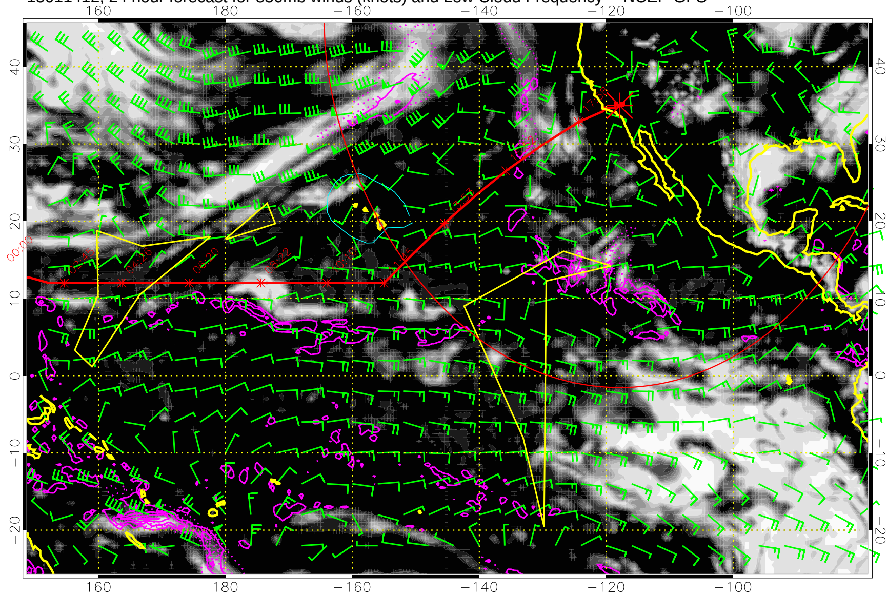
15011412, 24 hour forecast for 850mb winds (knots) and Low Cloud Frequency -- NCEP GFS
