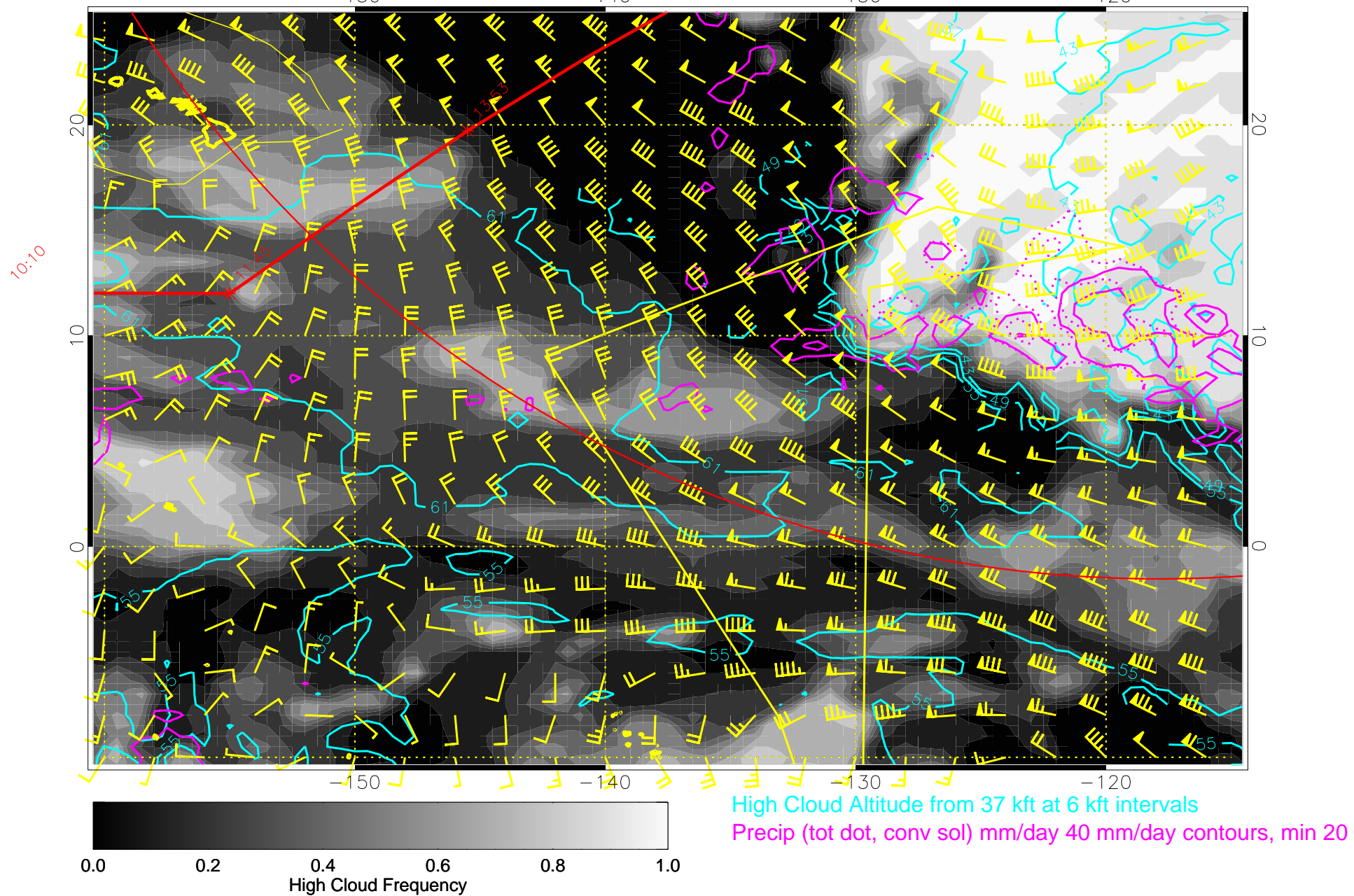
15011318, 6 hour forecast for 150mb winds (knots) and High Cloud Frequency -- NCEP GFS
