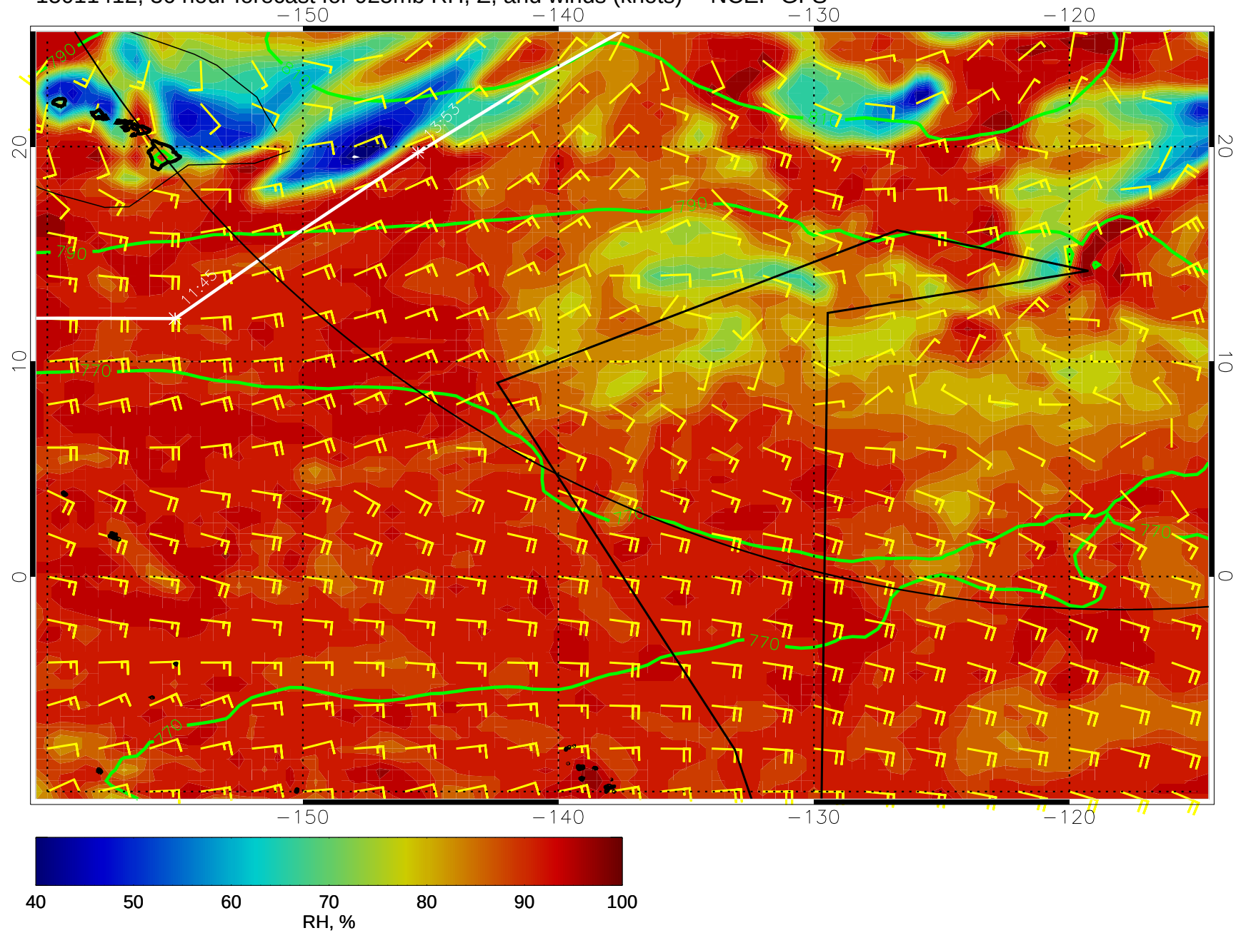
15011412, 36 hour forecast for 925mb RH, Z, and winds (knots) -- NCEP GFS
