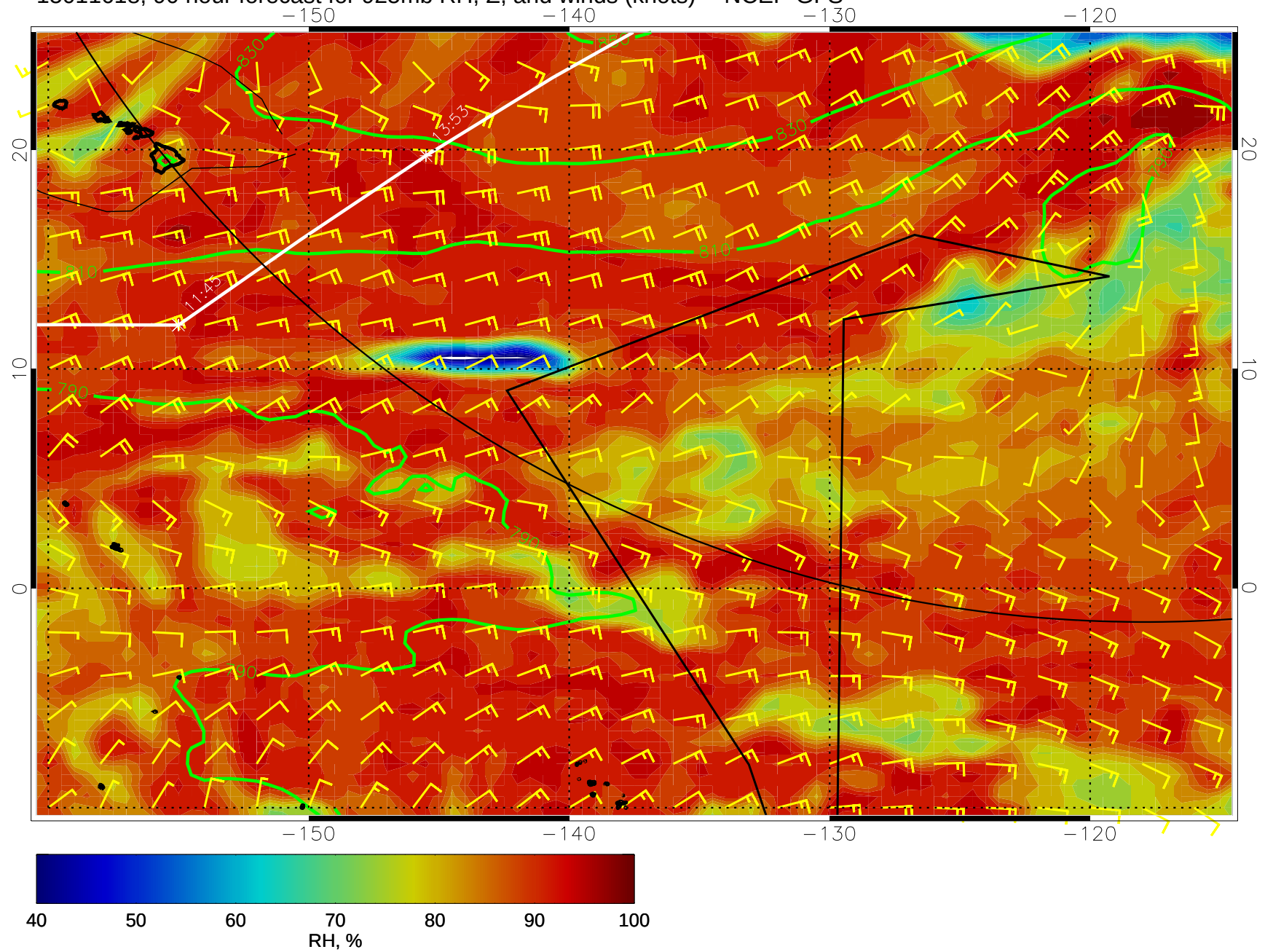
15011618, 90 hour forecast for 925mb RH, Z, and winds (knots) -- NCEP GFS
