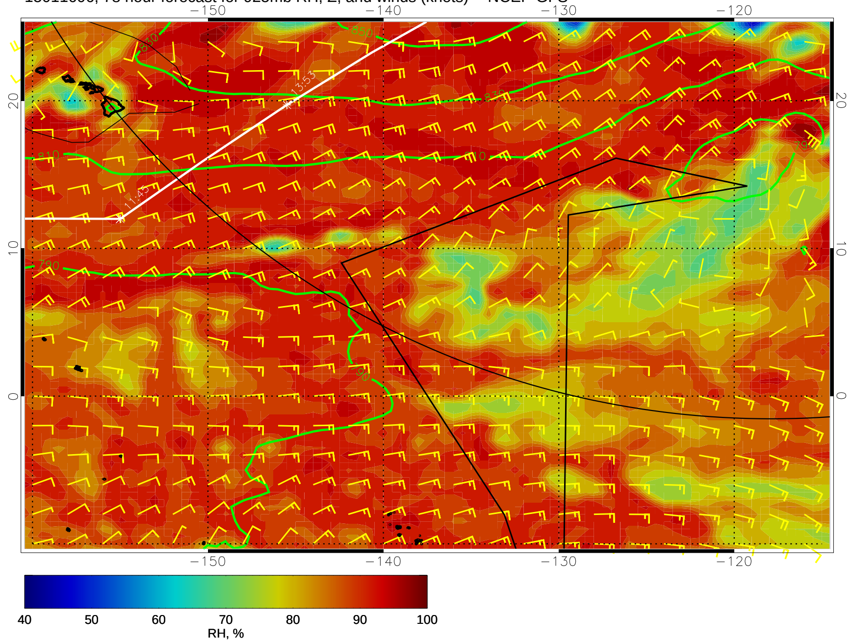
15011606, 78 hour forecast for 925mb RH, Z, and winds (knots) -- NCEP GFS
