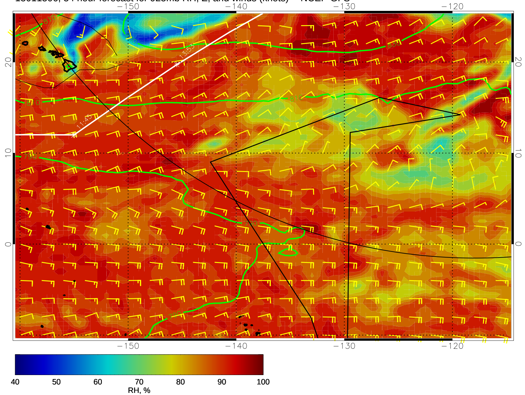
15011506, 54 hour forecast for 925mb RH, Z, and winds (knots) -- NCEP GFS
