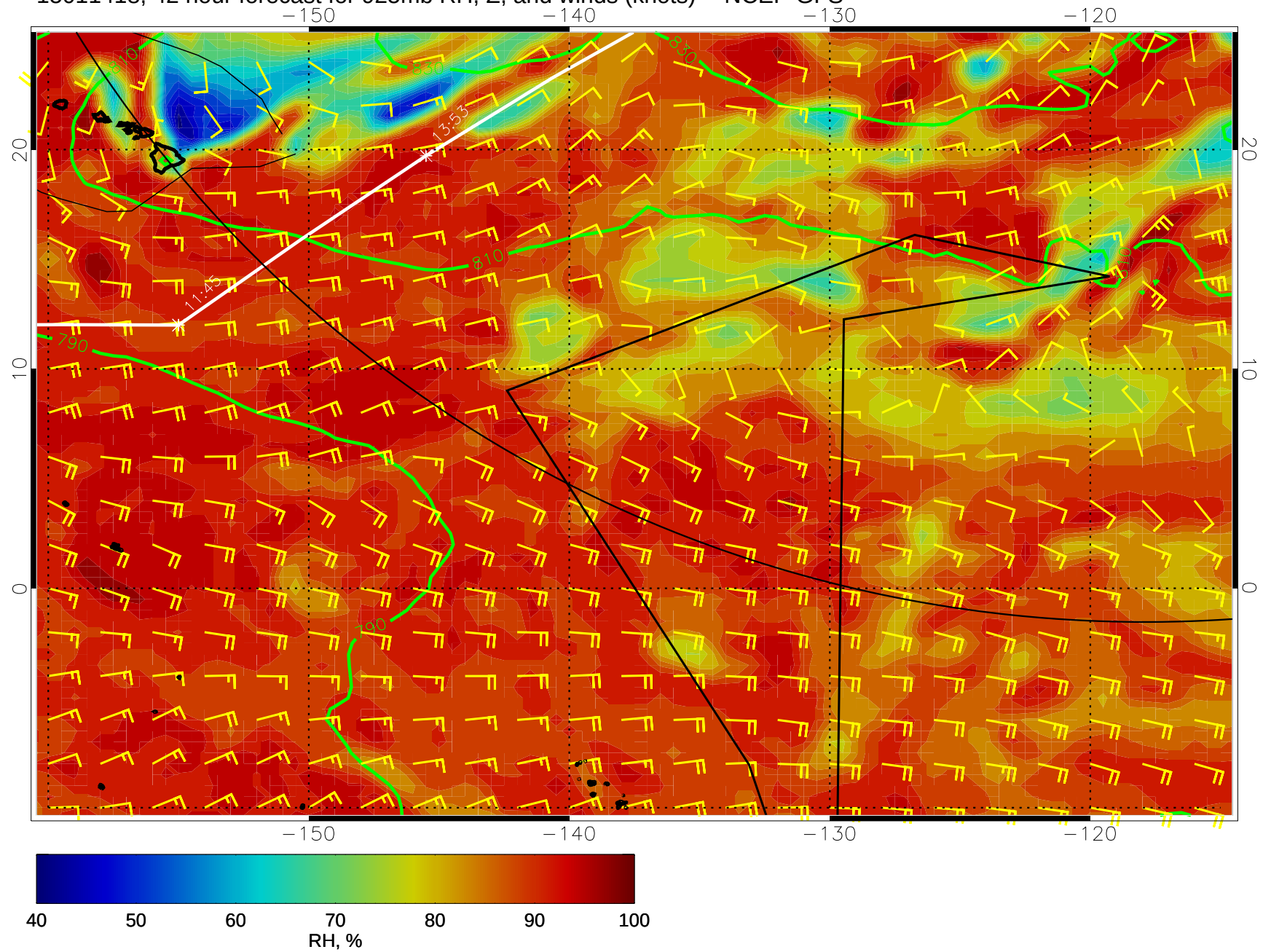
15011418, 42 hour forecast for 925mb RH, Z, and winds (knots) -- NCEP GFS
