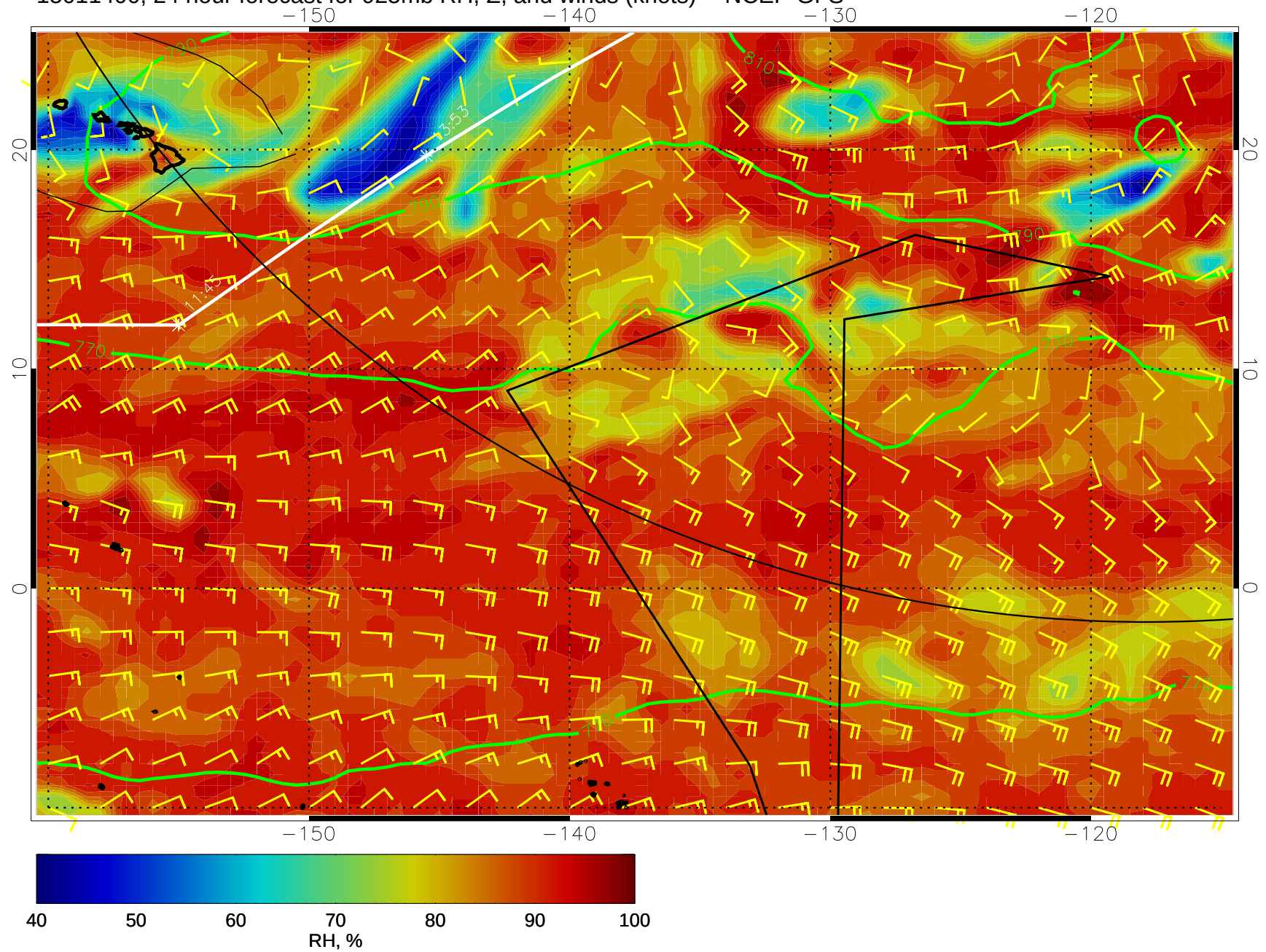
15011400, 24 hour forecast for 925mb RH, Z, and winds (knots) -- NCEP GFS
