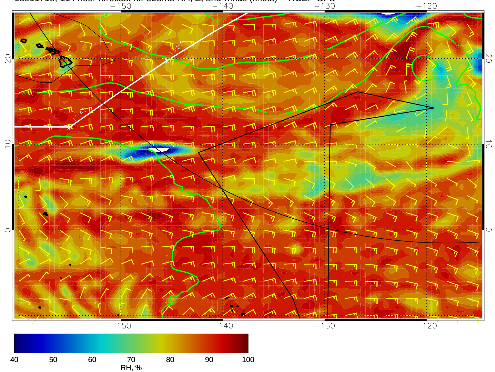
15011718, 114 hour forecast for 925mb RH, Z, and winds (knots) -- NCEP GFS
