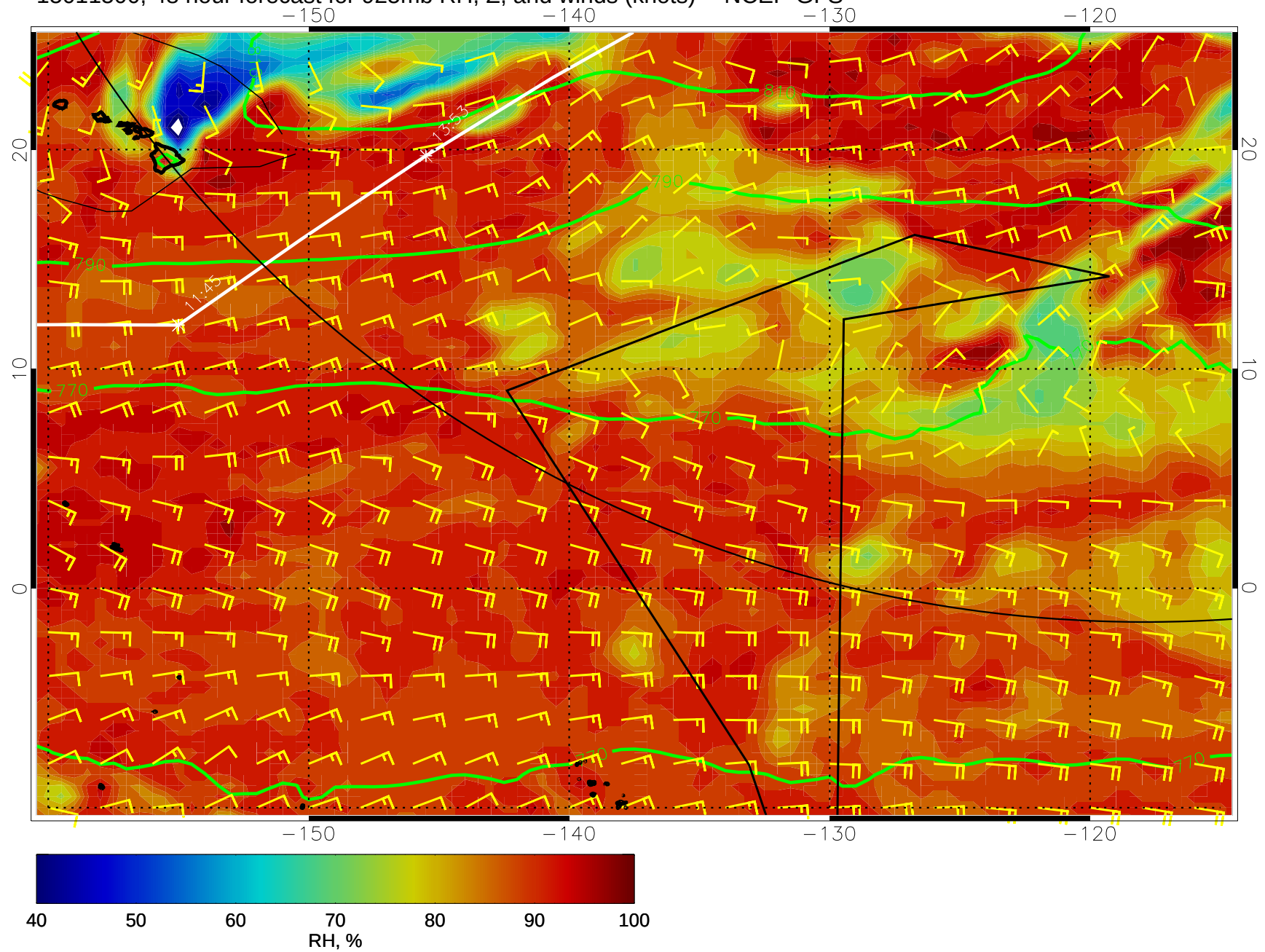
15011500, 48 hour forecast for 925mb RH, Z, and winds (knots) -- NCEP GFS
