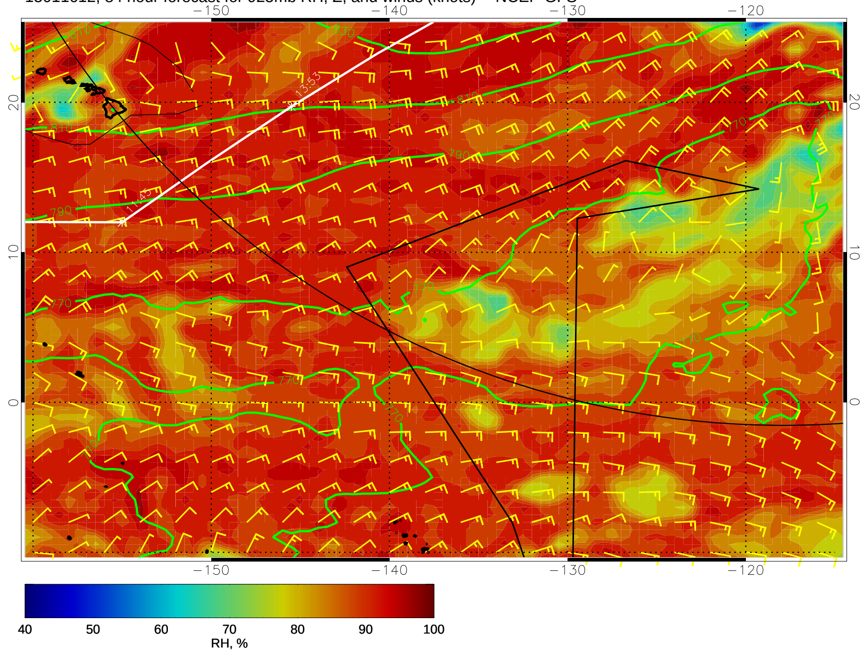
15011612, 84 hour forecast for 925mb RH, Z, and winds (knots) -- NCEP GFS
