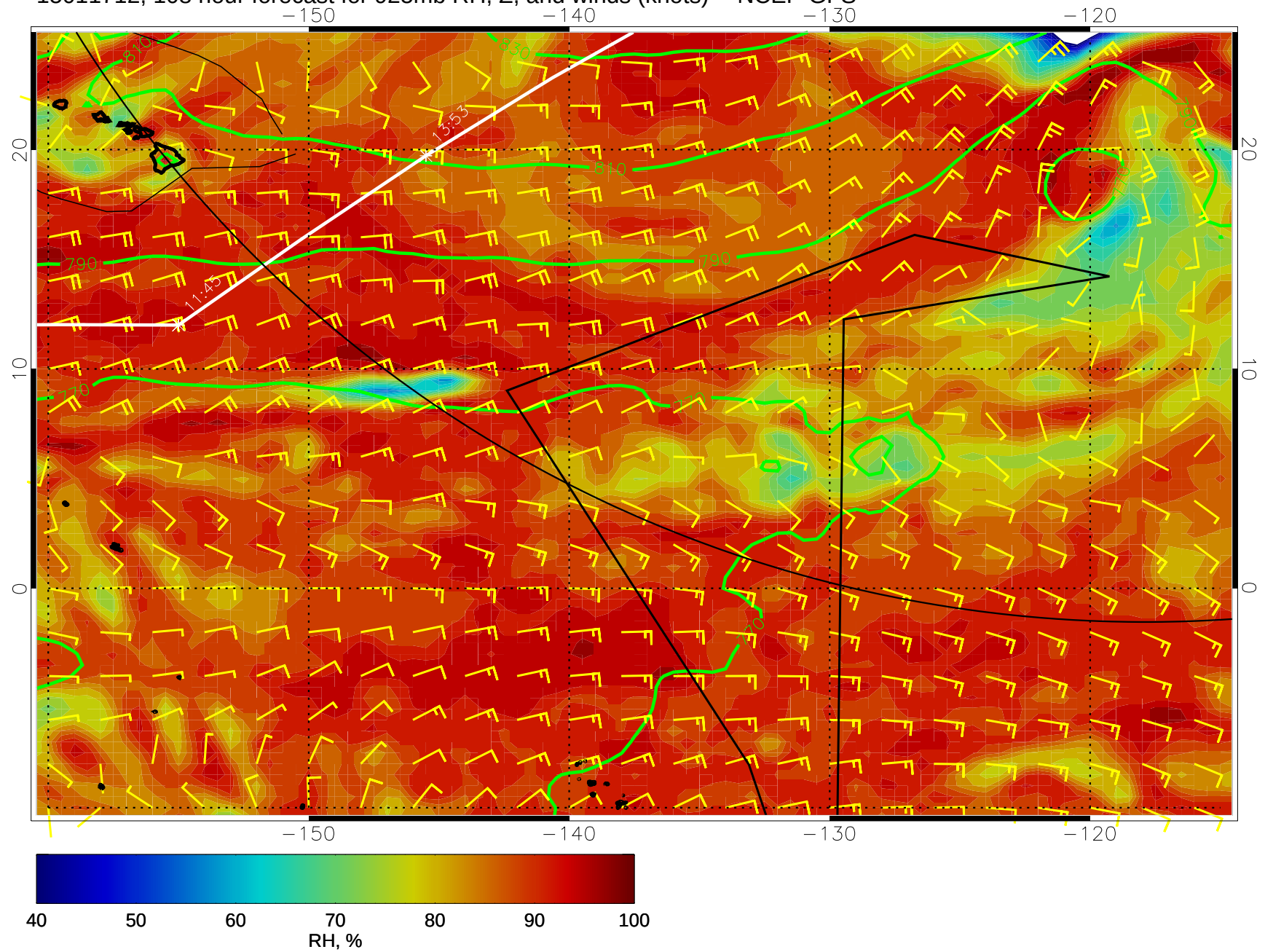
15011712, 108 hour forecast for 925mb RH, Z, and winds (knots) -- NCEP GFS
