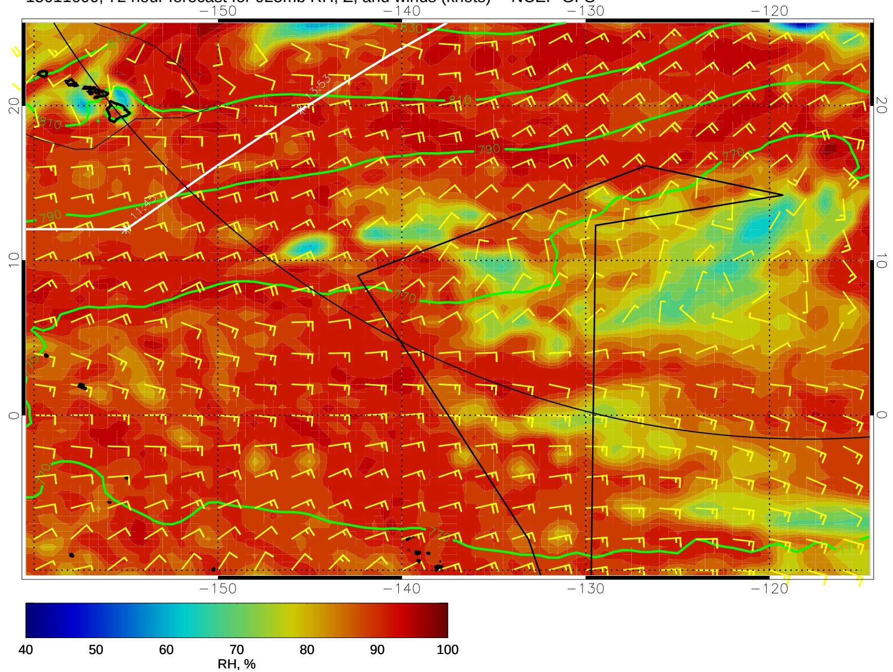
15011600, 72 hour forecast for 925mb RH, Z, and winds (knots) -- NCEP GFS
