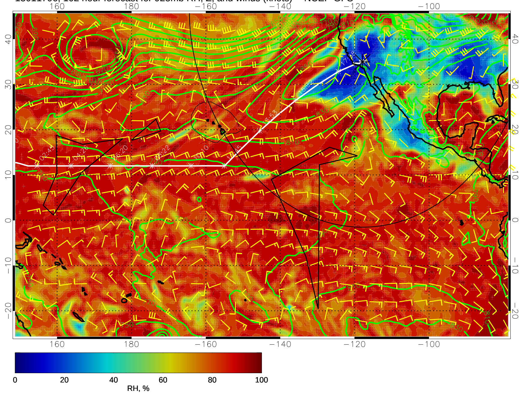
15011706, 102 hour forecast for 925mb RH, Z, and winds (knots) -- NCEP GFS
