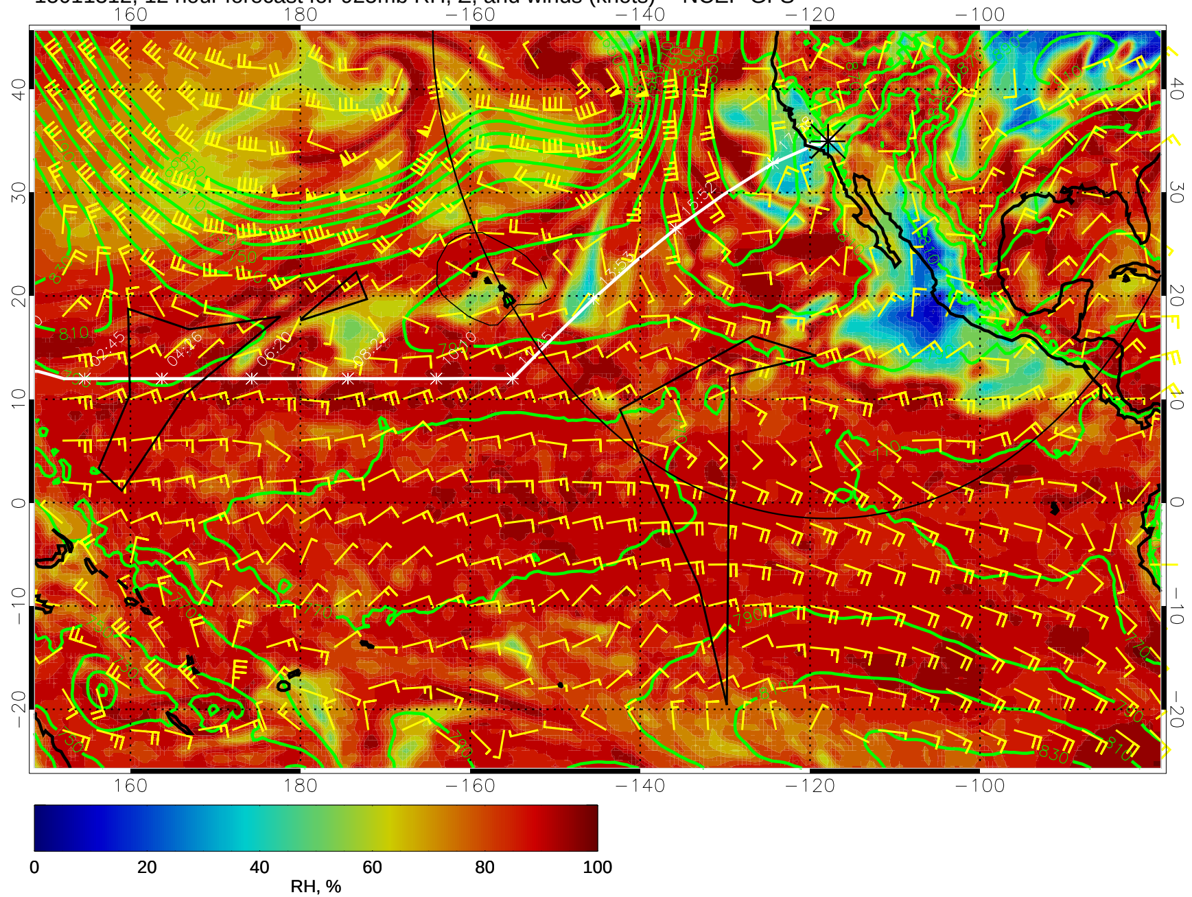
15011312, 12 hour forecast for 925mb RH, Z, and winds (knots) -- NCEP GFS
