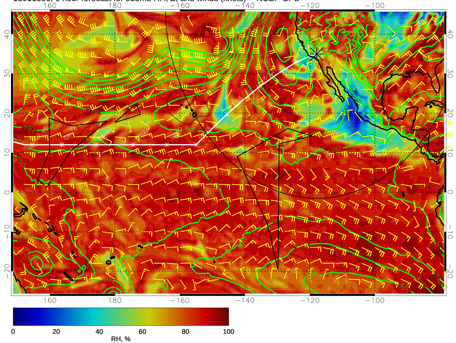
15011306, 6 hour forecast for 925mb RH, Z, and winds (knots) -- NCEP GFS
