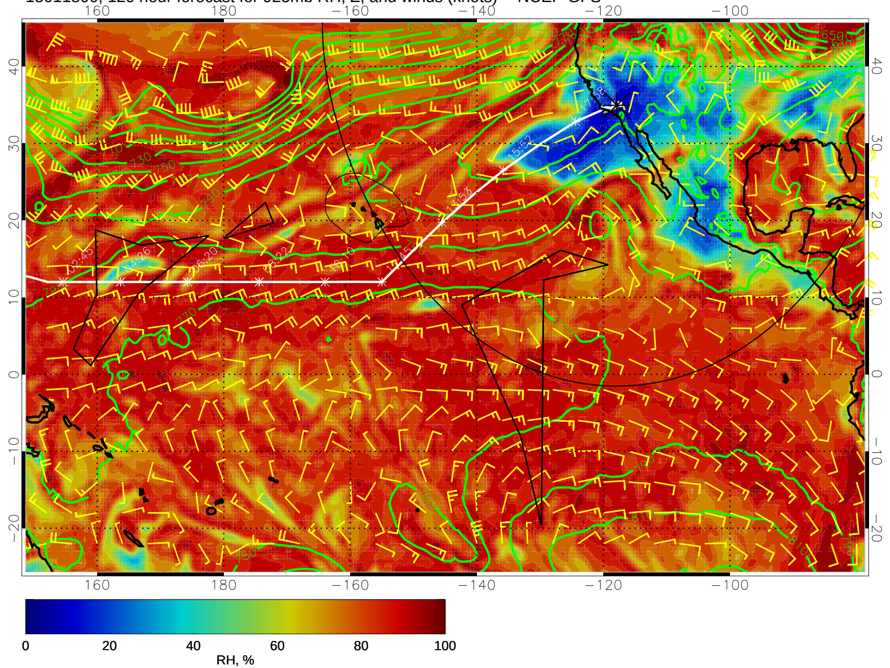
15011800, 120 hour forecast for 925mb RH, Z, and winds (knots) -- NCEP GFS
