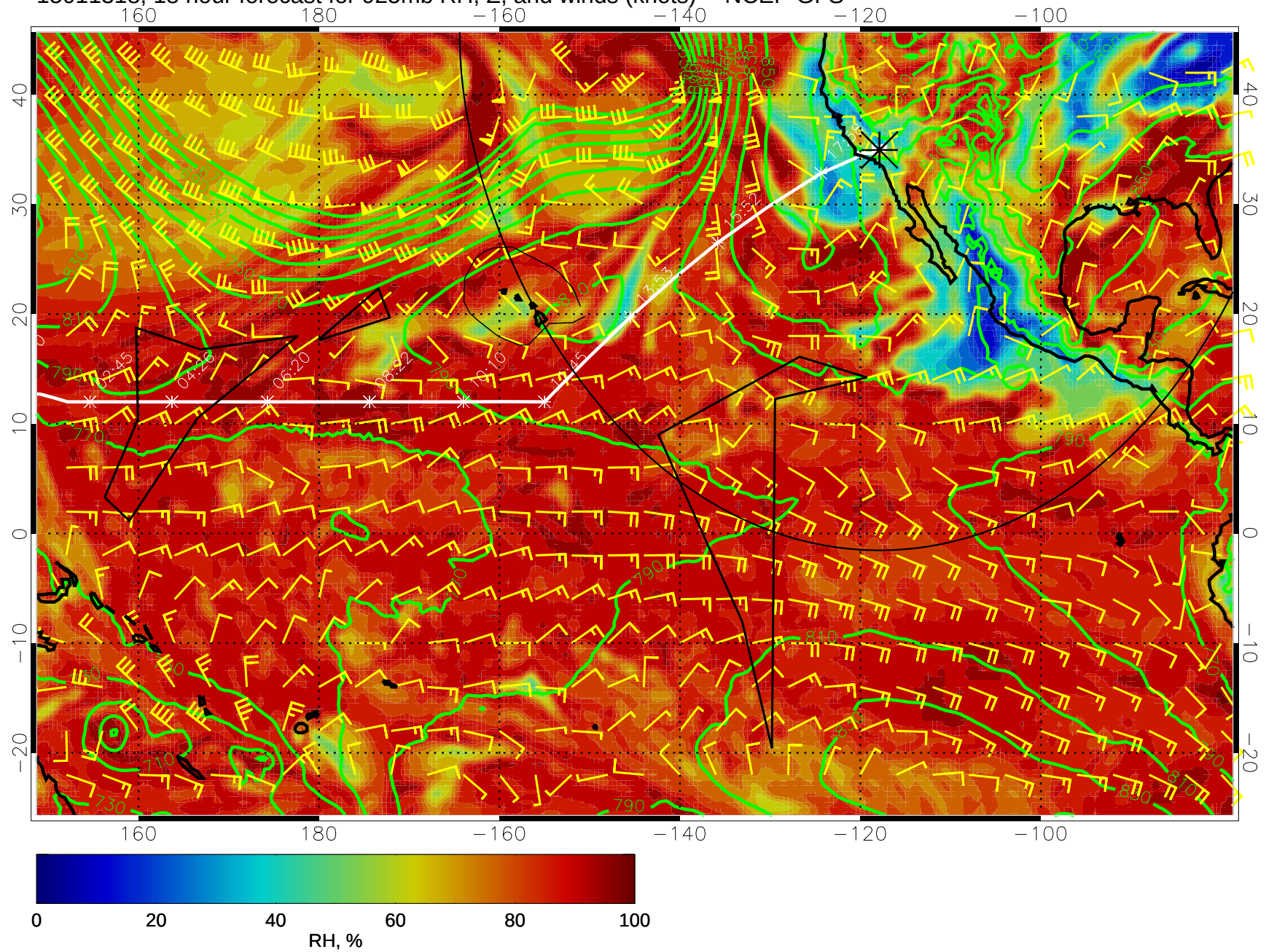
15011318, 18 hour forecast for 925mb RH, Z, and winds (knots) -- NCEP GFS
