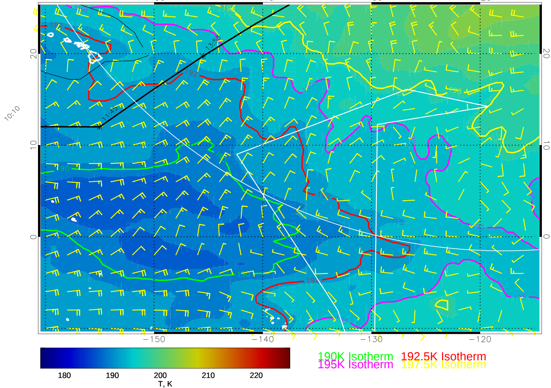
15011306, 6 hour forecast for 70mb T and winds (knots) -- NCEP GFS
