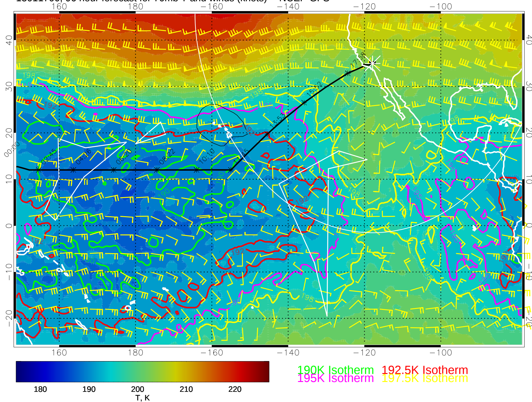
15011700, 96 hour forecast for 70mb T and winds (knots) -- NCEP GFS
