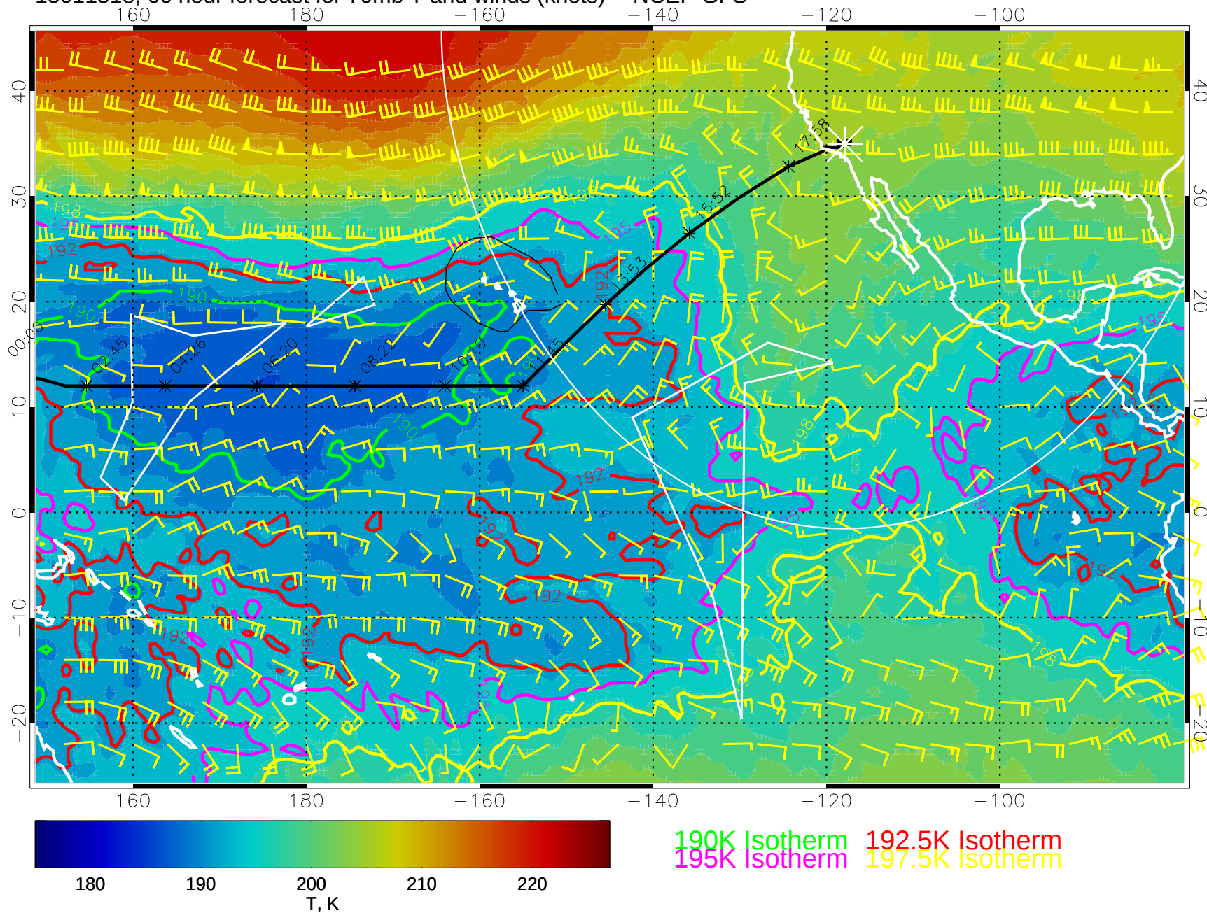
15011518, 66 hour forecast for 70mb T and winds (knots) -- NCEP GFS
