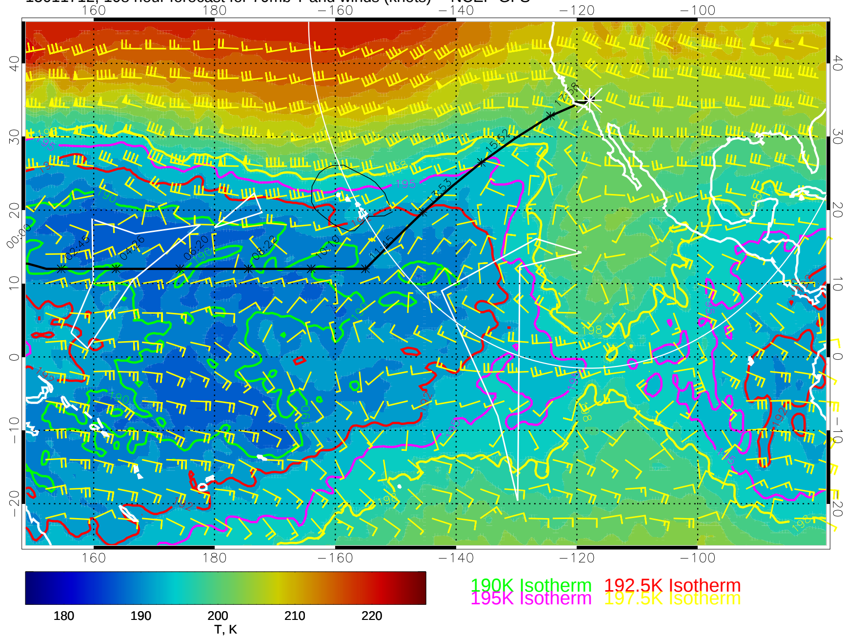
15011712, 108 hour forecast for 70mb T and winds (knots) -- NCEP GFS
