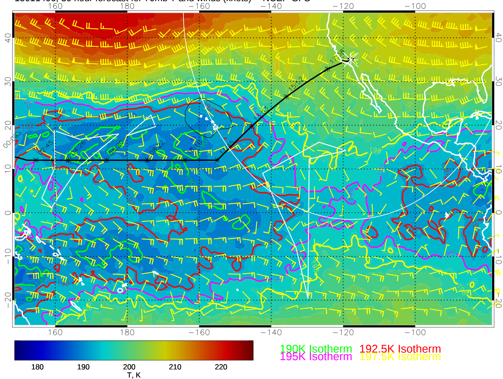
15011406, 30 hour forecast for 70mb T and winds (knots) -- NCEP GFS
