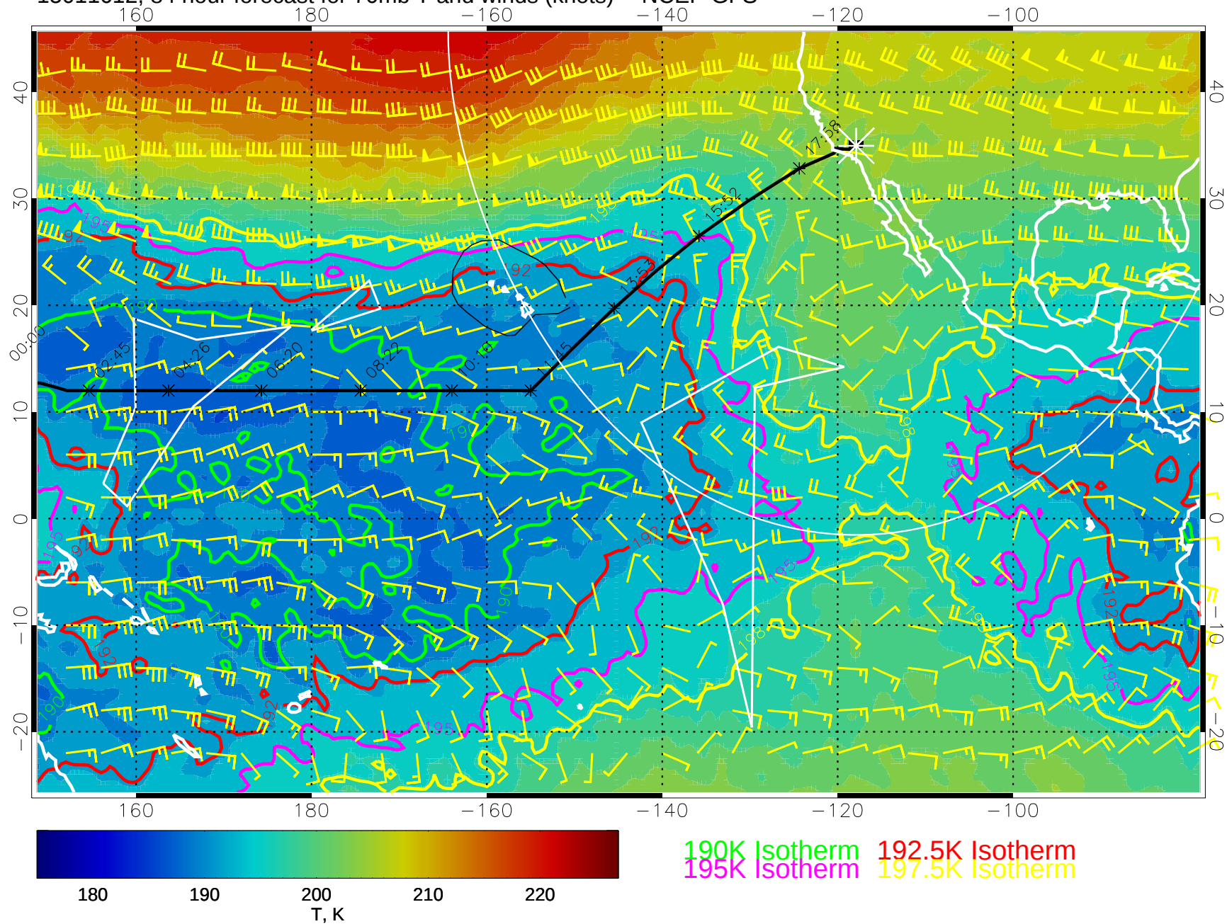
15011612, 84 hour forecast for 70mb T and winds (knots) -- NCEP GFS
