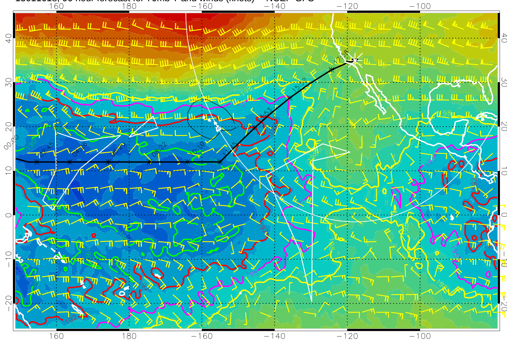
15011618, 90 hour forecast for 70mb T and winds (knots) -- NCEP GFS
