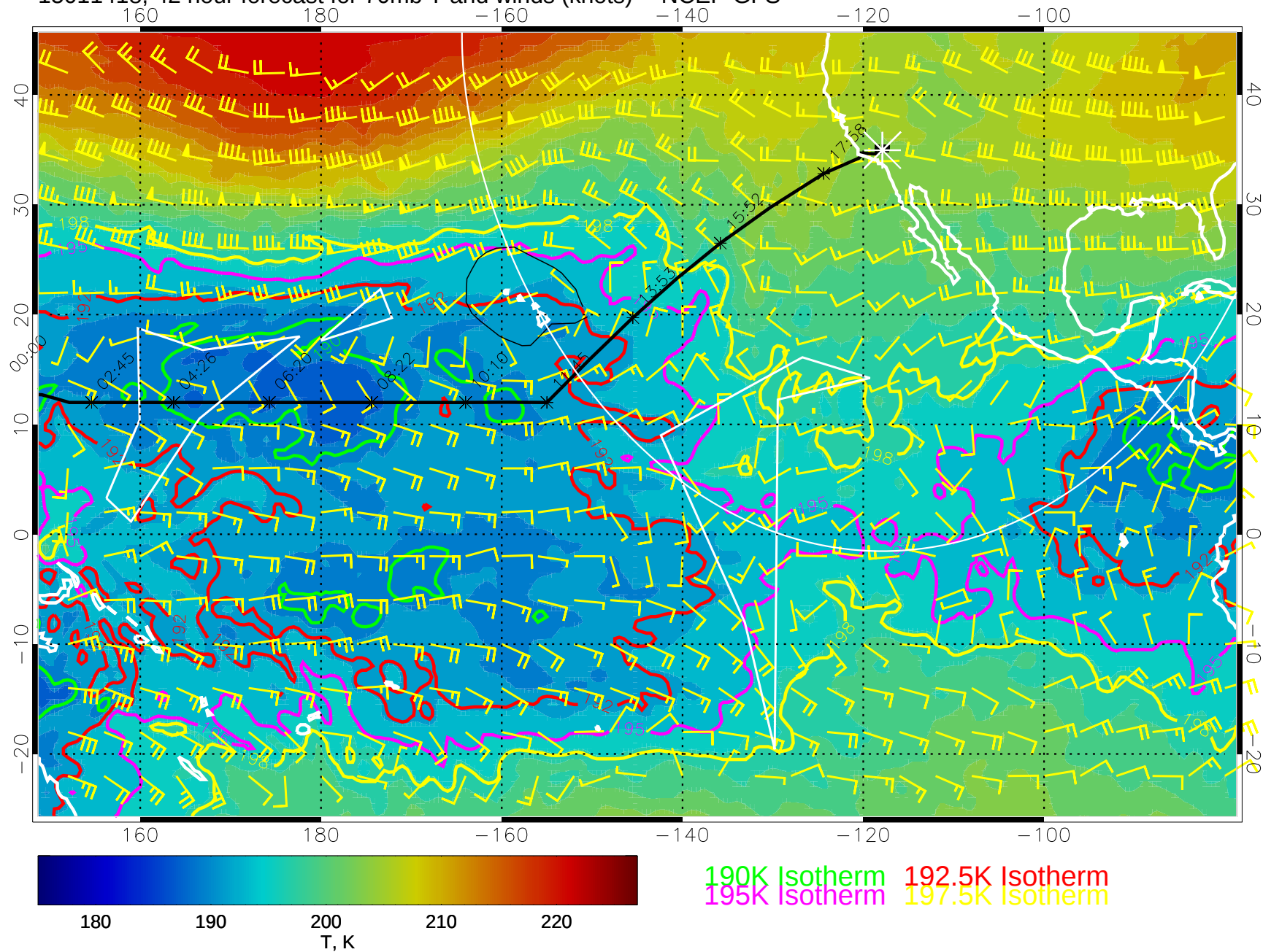
15011418, 42 hour forecast for 70mb T and winds (knots) -- NCEP GFS
