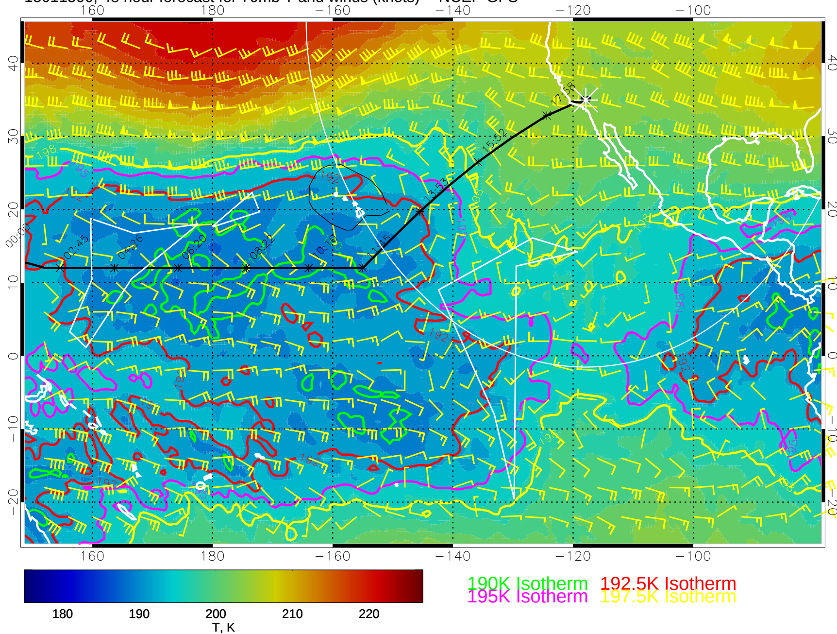
15011500, 48 hour forecast for 70mb T and winds (knots) -- NCEP GFS
