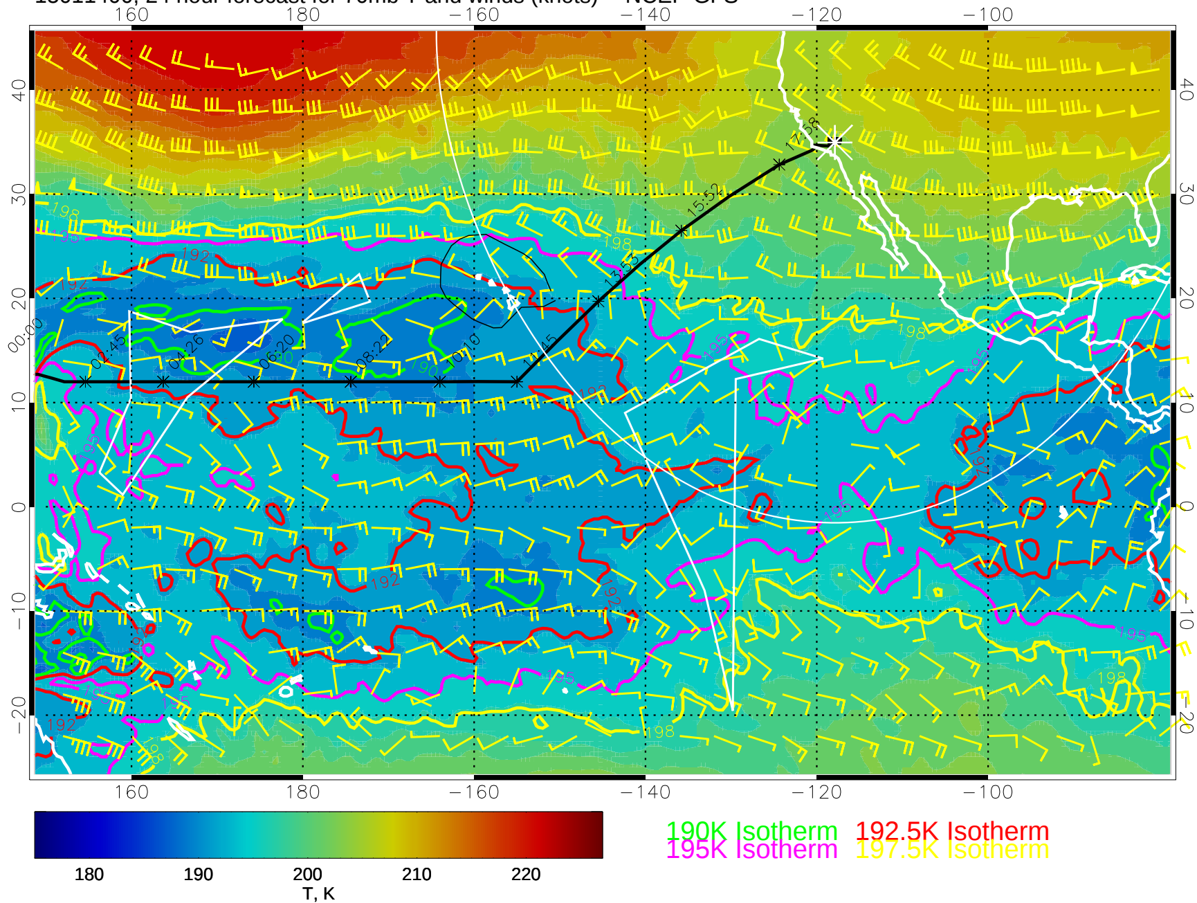
15011400, 24 hour forecast for 70mb T and winds (knots) -- NCEP GFS
