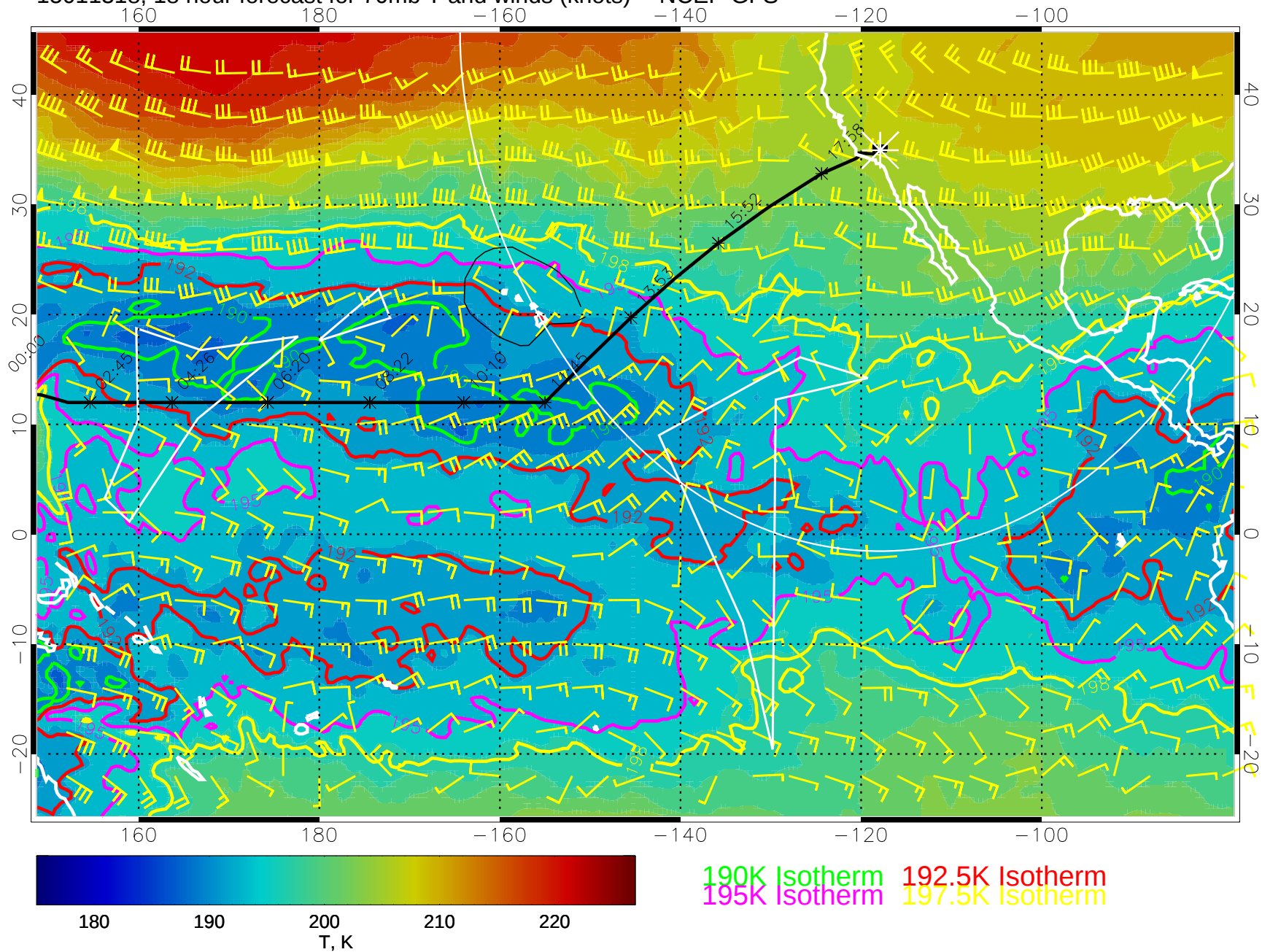
15011318, 18 hour forecast for 70mb T and winds (knots) -- NCEP GFS
