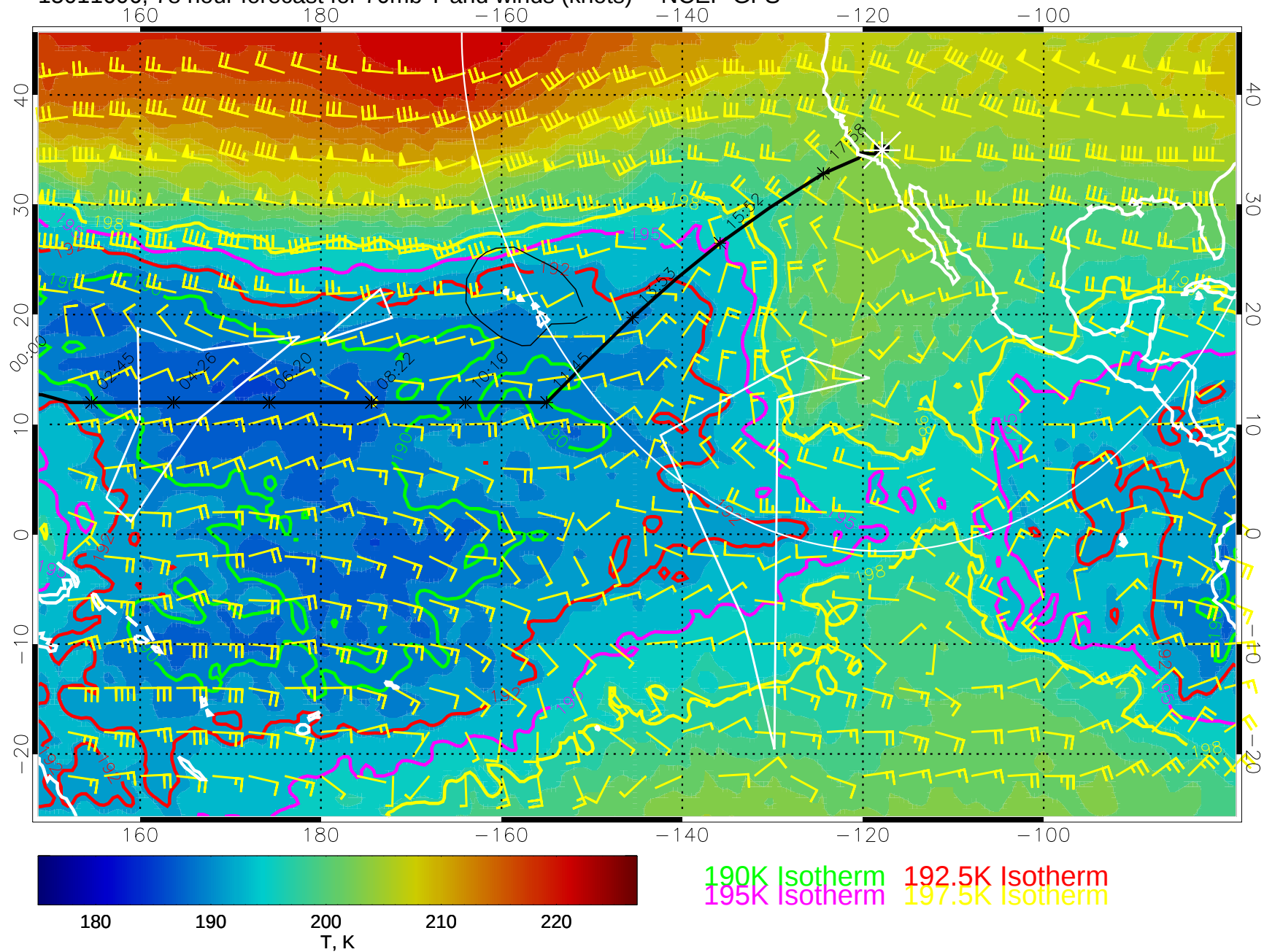
15011606, 78 hour forecast for 70mb T and winds (knots) -- NCEP GFS
