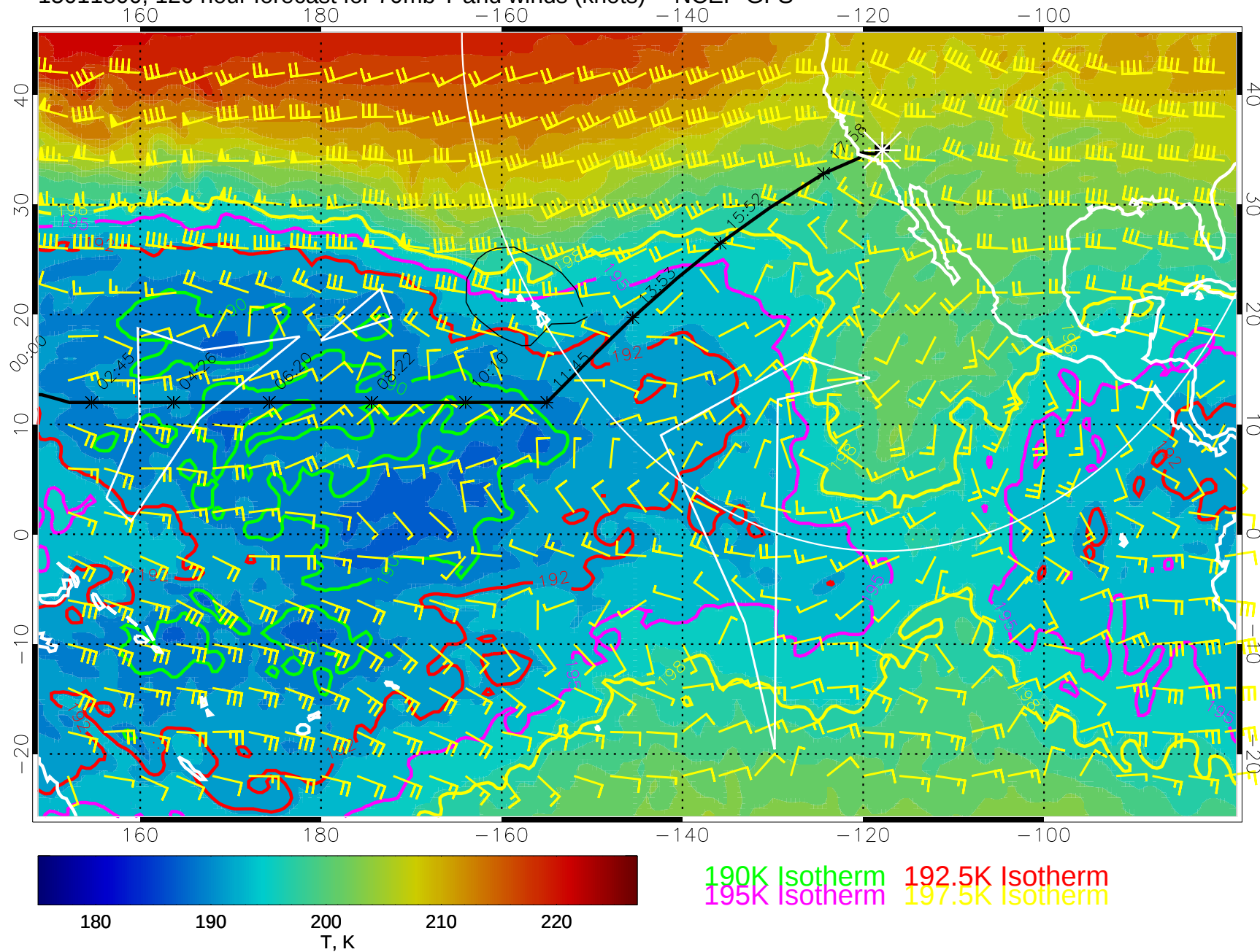
15011800, 120 hour forecast for 70mb T and winds (knots) -- NCEP GFS
