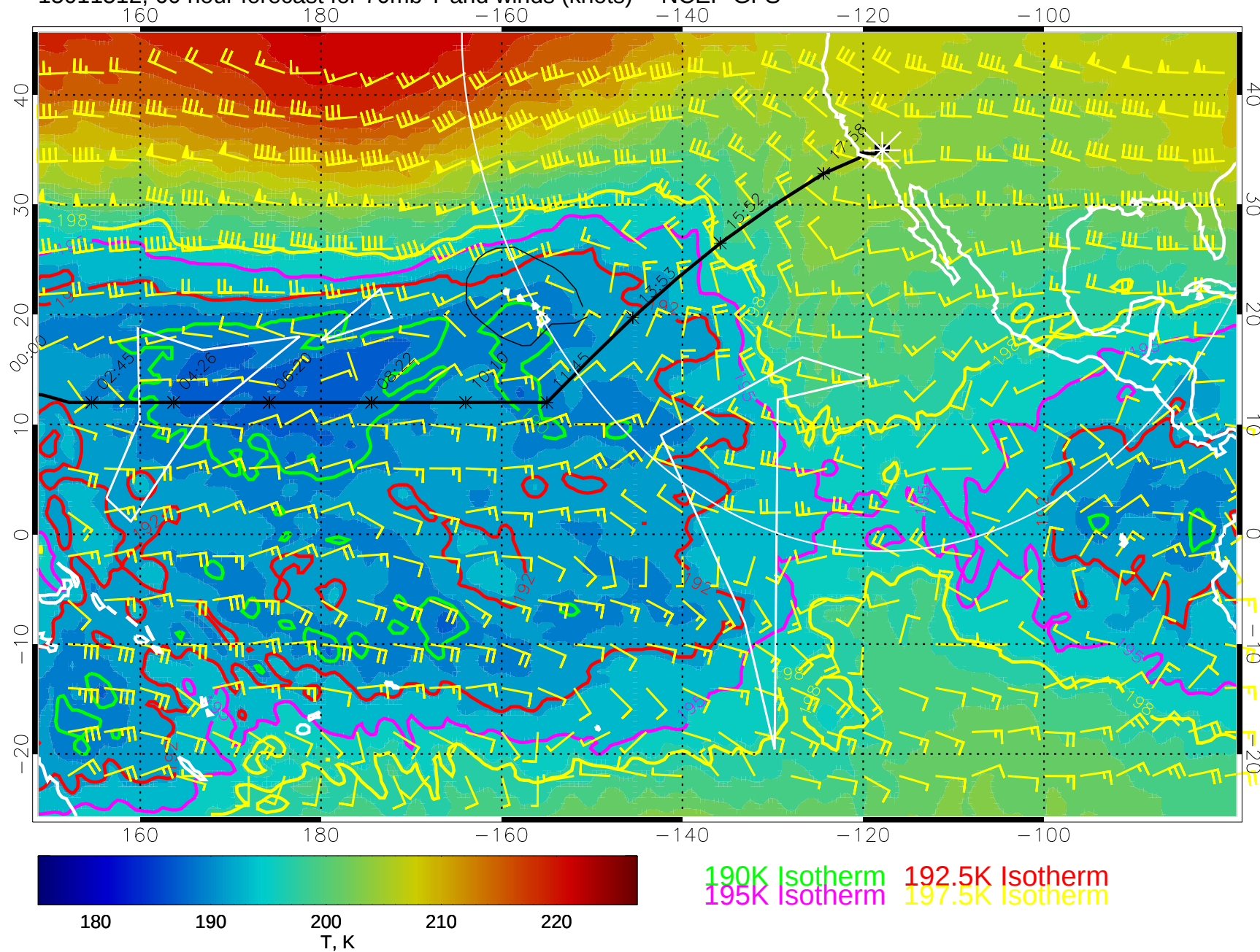
15011512, 60 hour forecast for 70mb T and winds (knots) -- NCEP GFS
