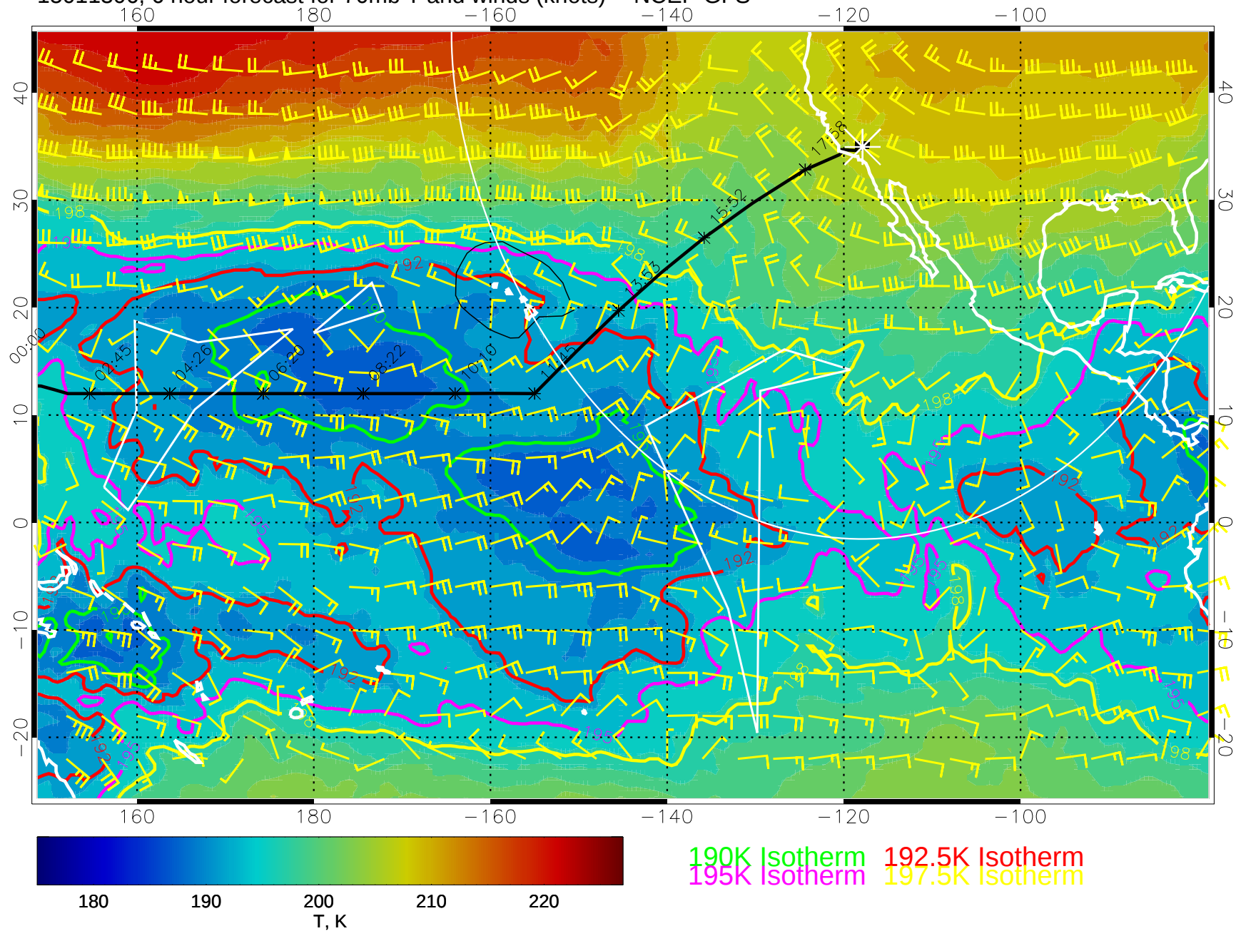
15011306, 6 hour forecast for 70mb T and winds (knots) -- NCEP GFS
