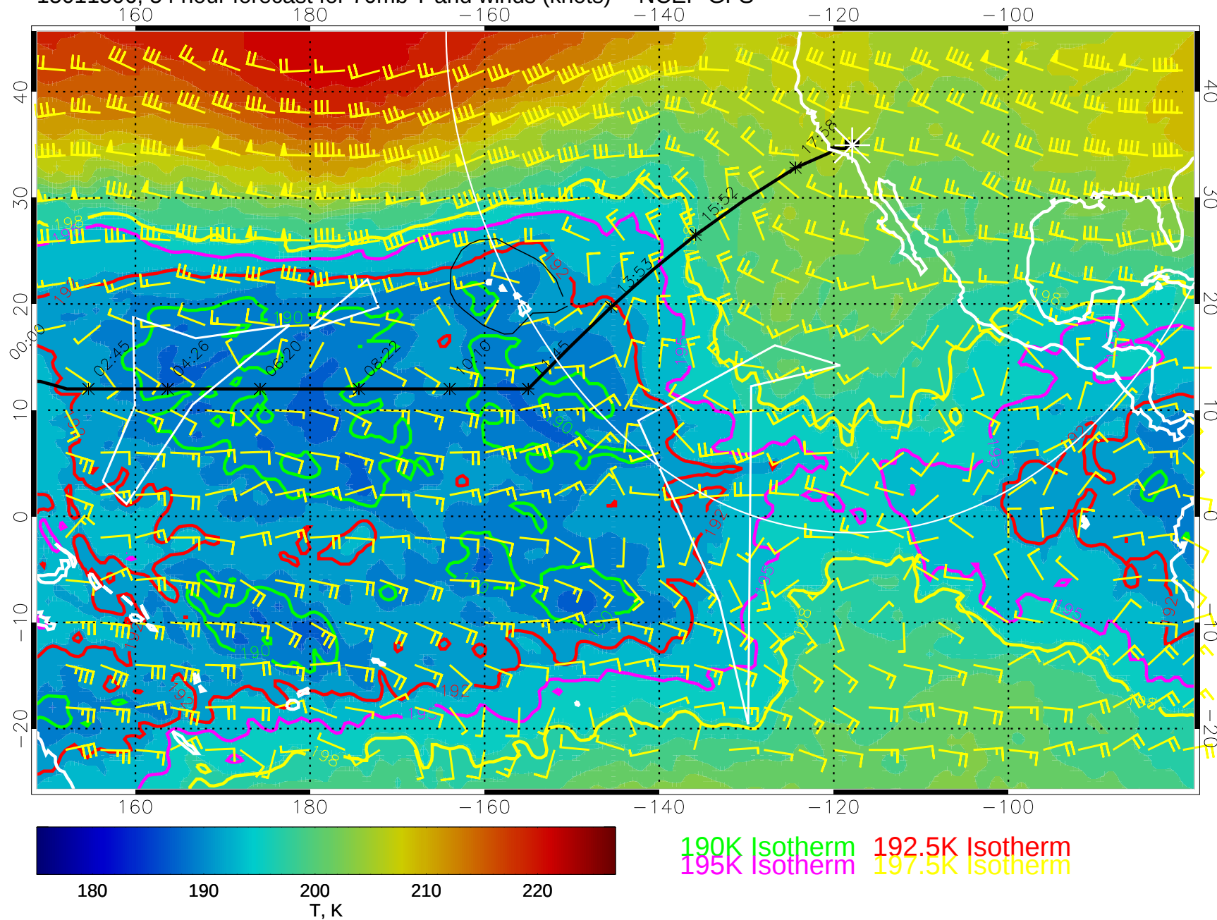
15011506, 54 hour forecast for 70mb T and winds (knots) -- NCEP GFS
