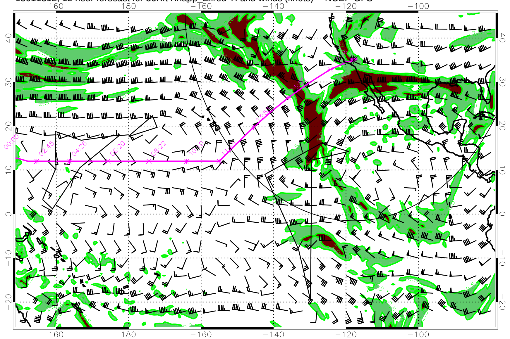
15011312, 12 hour forecast for 36Kft Knapp_Ellrod TI and winds (knots) -- NCEP GFS
