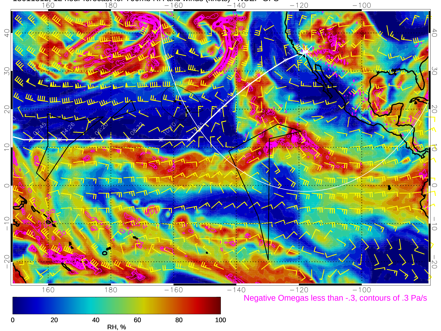
15011312, 12 hour forecast for 700mb RH and winds (knots) - NCEP GFS
