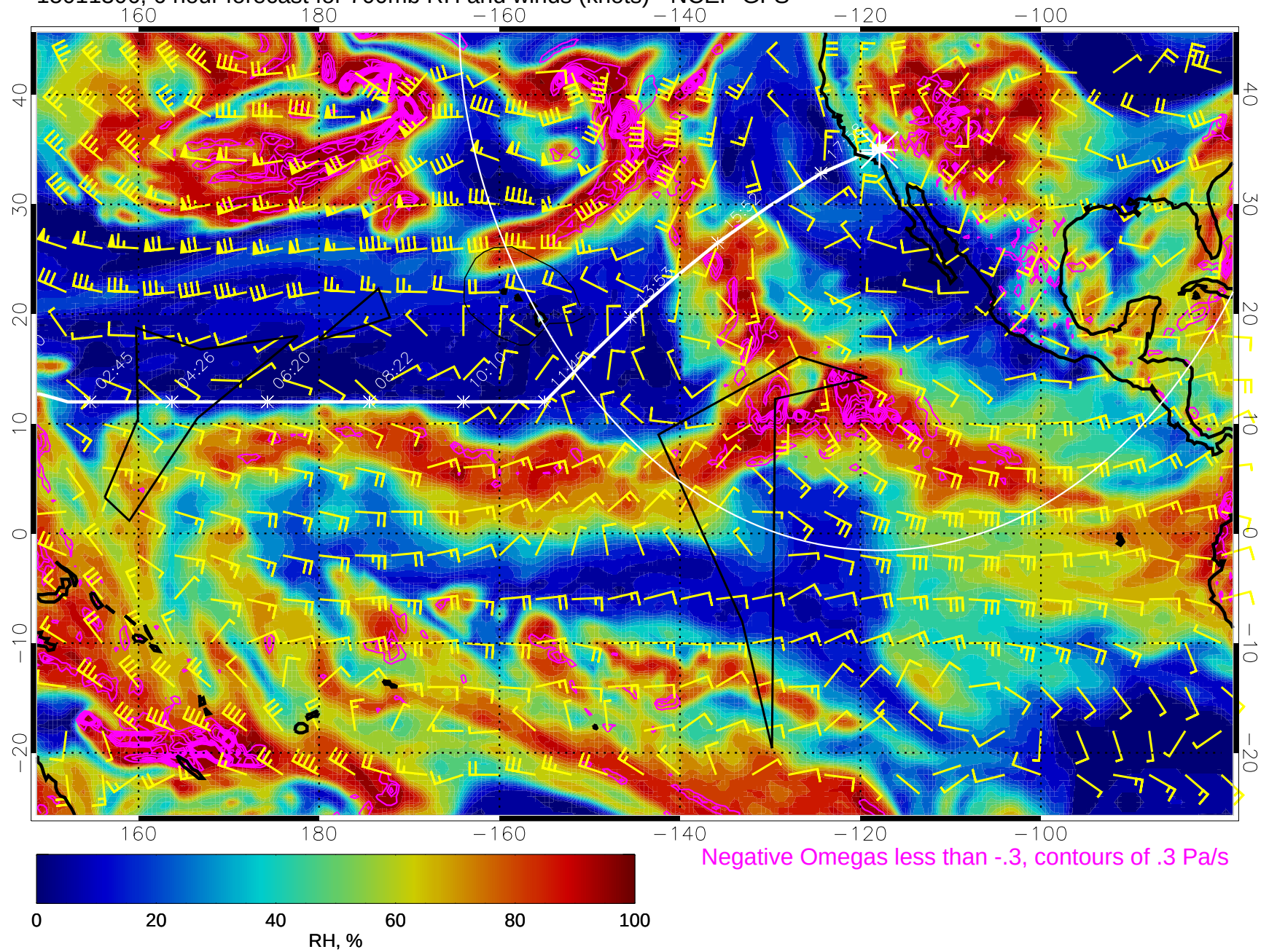
15011306, 6 hour forecast for 700mb RH and winds (knots) - NCEP GFS
