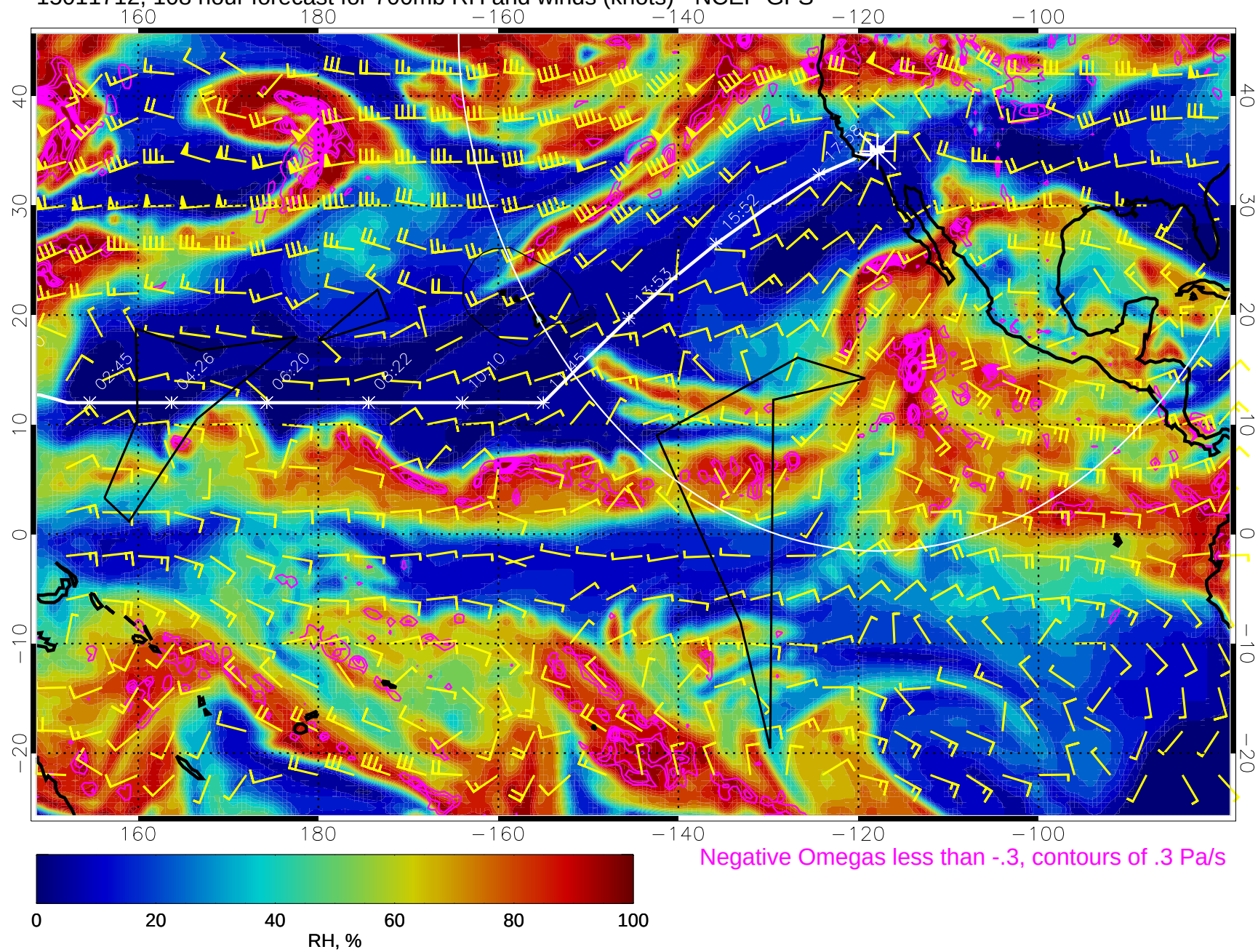
15011712, 108 hour forecast for 700mb RH and winds (knots) - NCEP GFS
