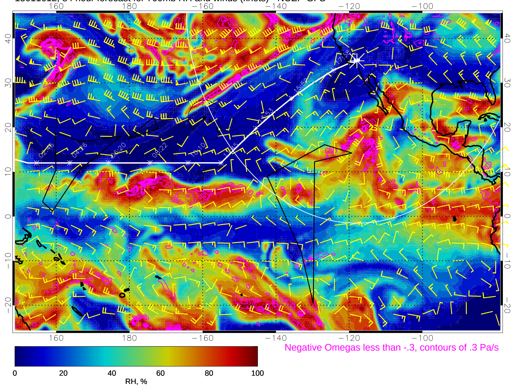
15011612, 84 hour forecast for 700mb RH and winds (knots) - NCEP GFS
