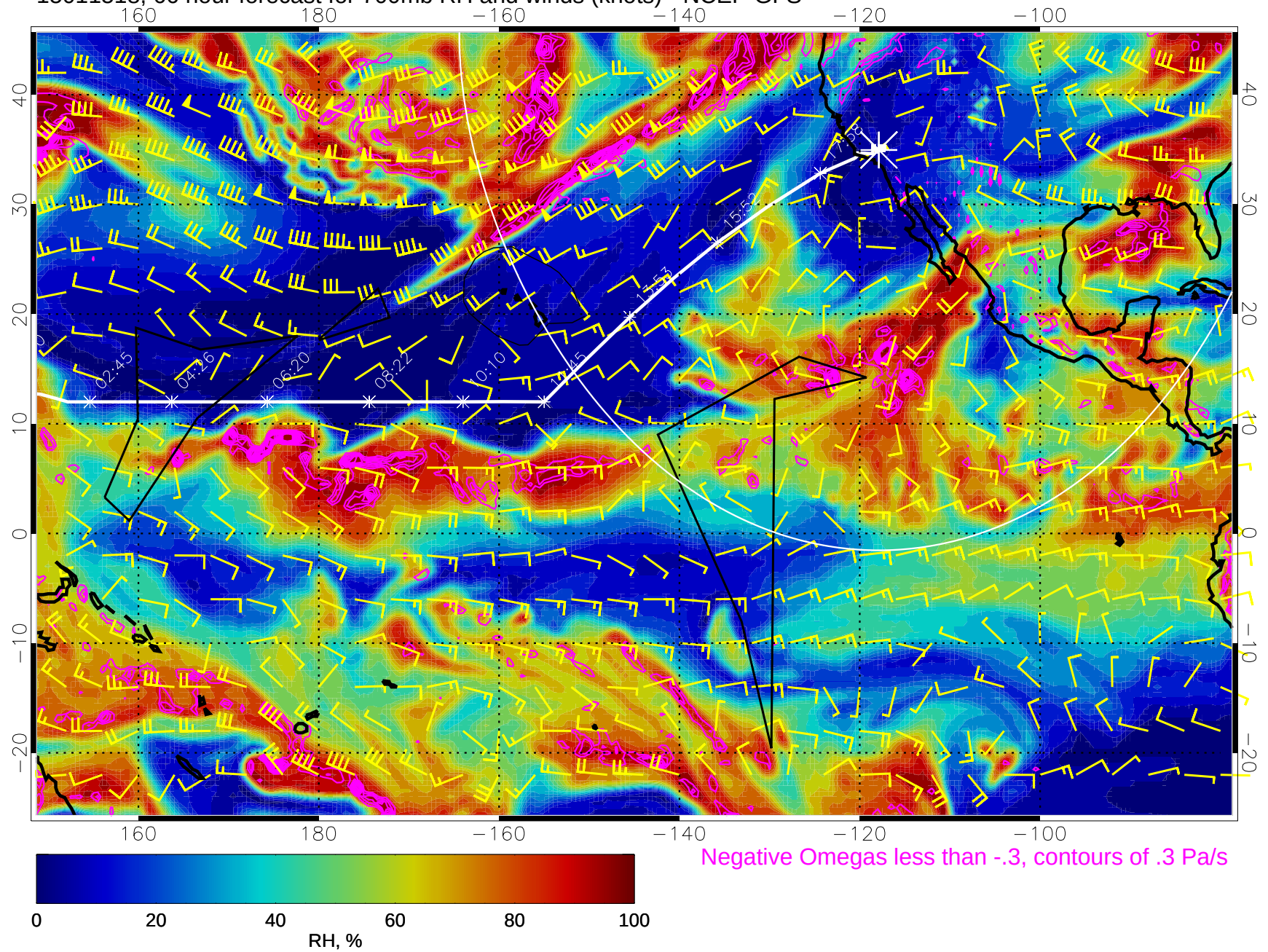
15011518, 66 hour forecast for 700mb RH and winds (knots) - NCEP GFS
