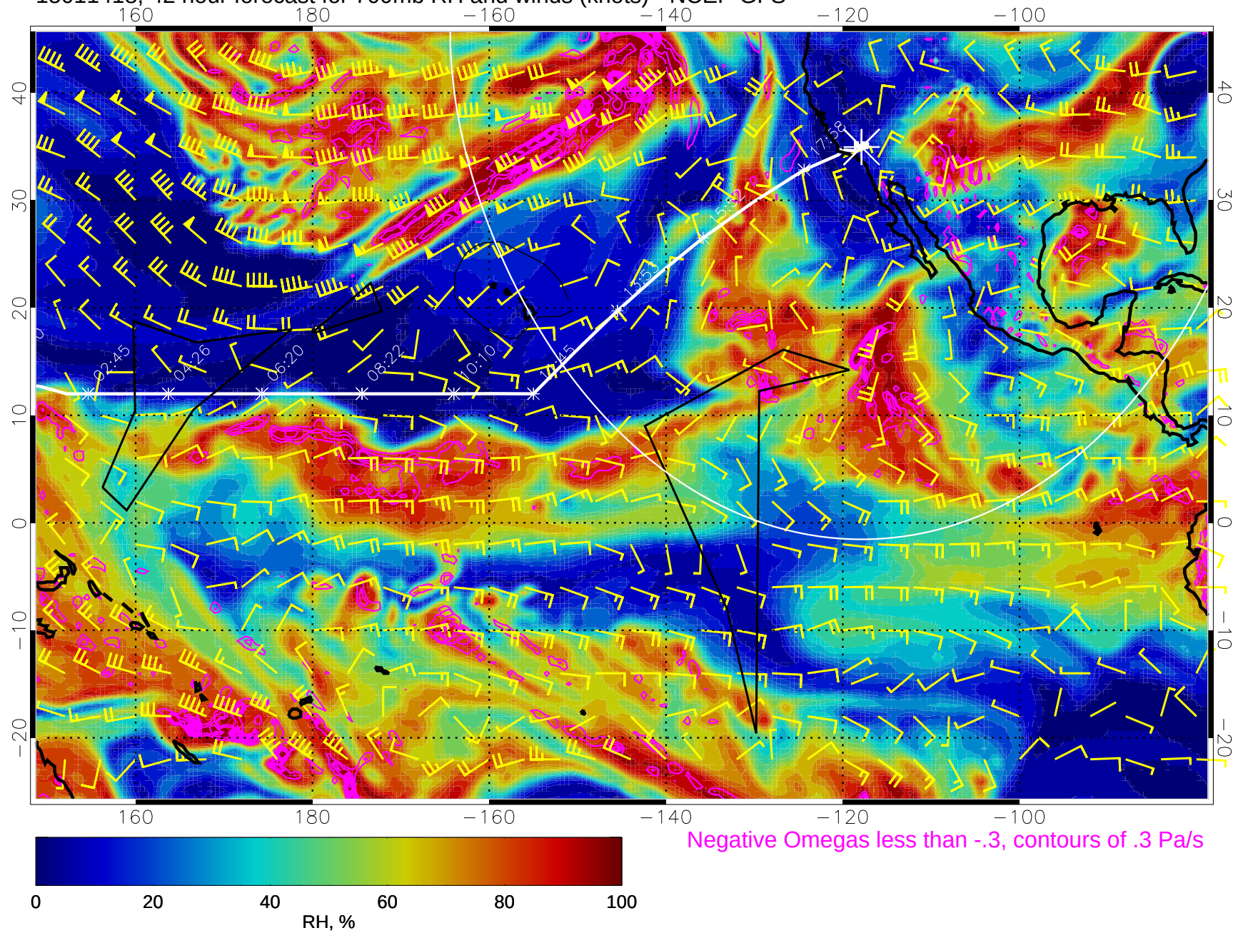
15011418, 42 hour forecast for 700mb RH and winds (knots) - NCEP GFS
