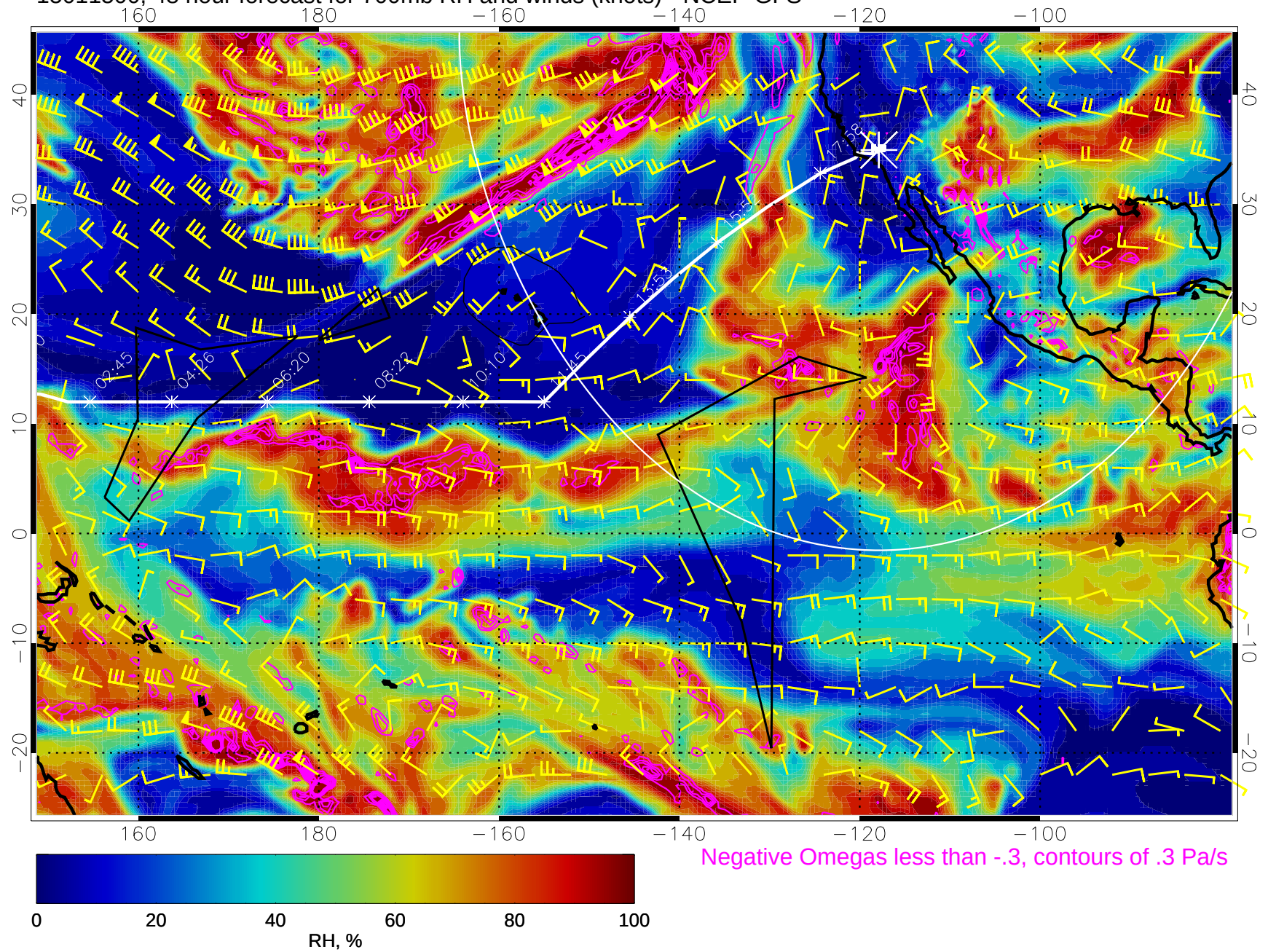
15011500, 48 hour forecast for 700mb RH and winds (knots) - NCEP GFS
