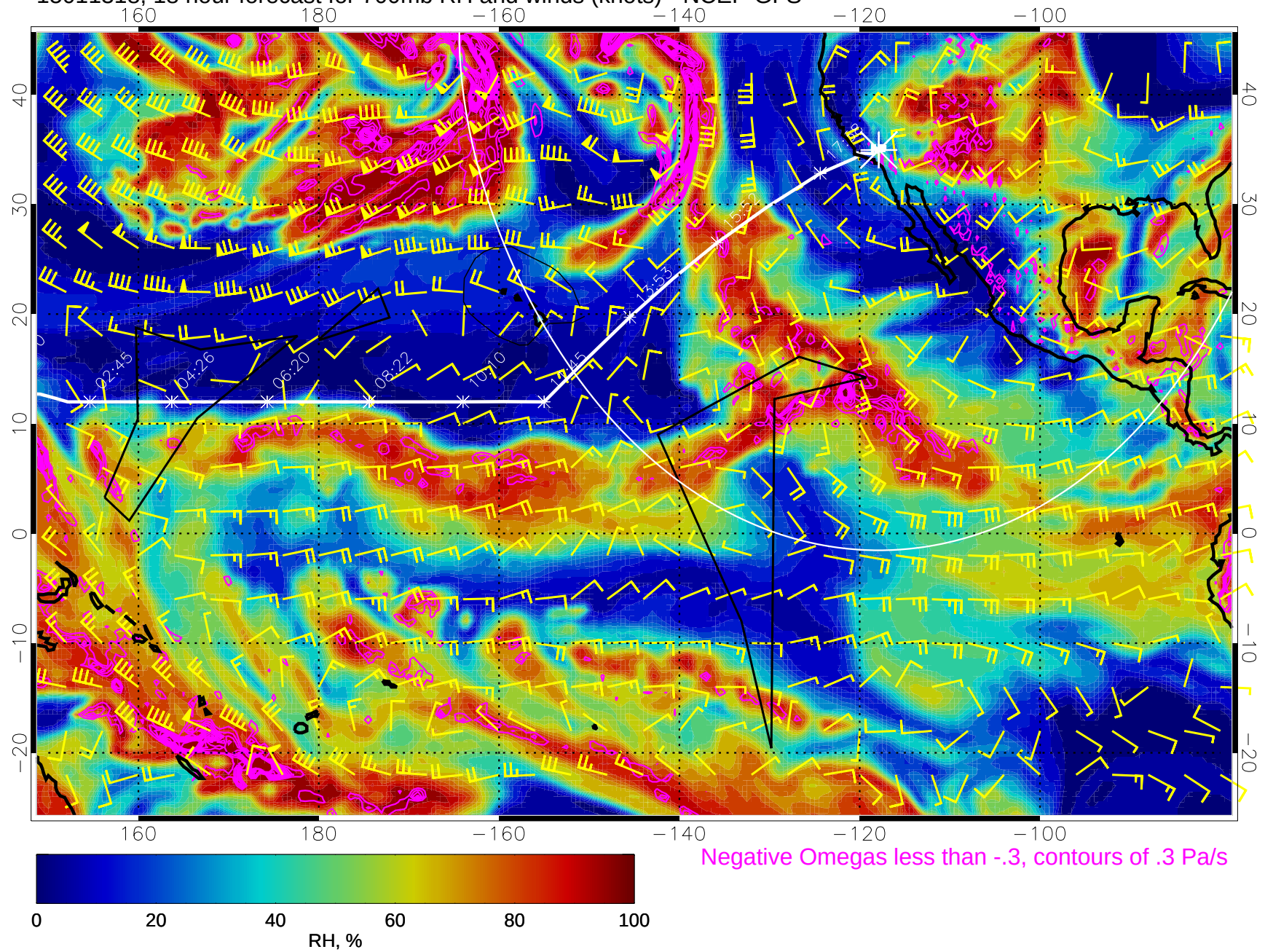
15011318, 18 hour forecast for 700mb RH and winds (knots) - NCEP GFS
