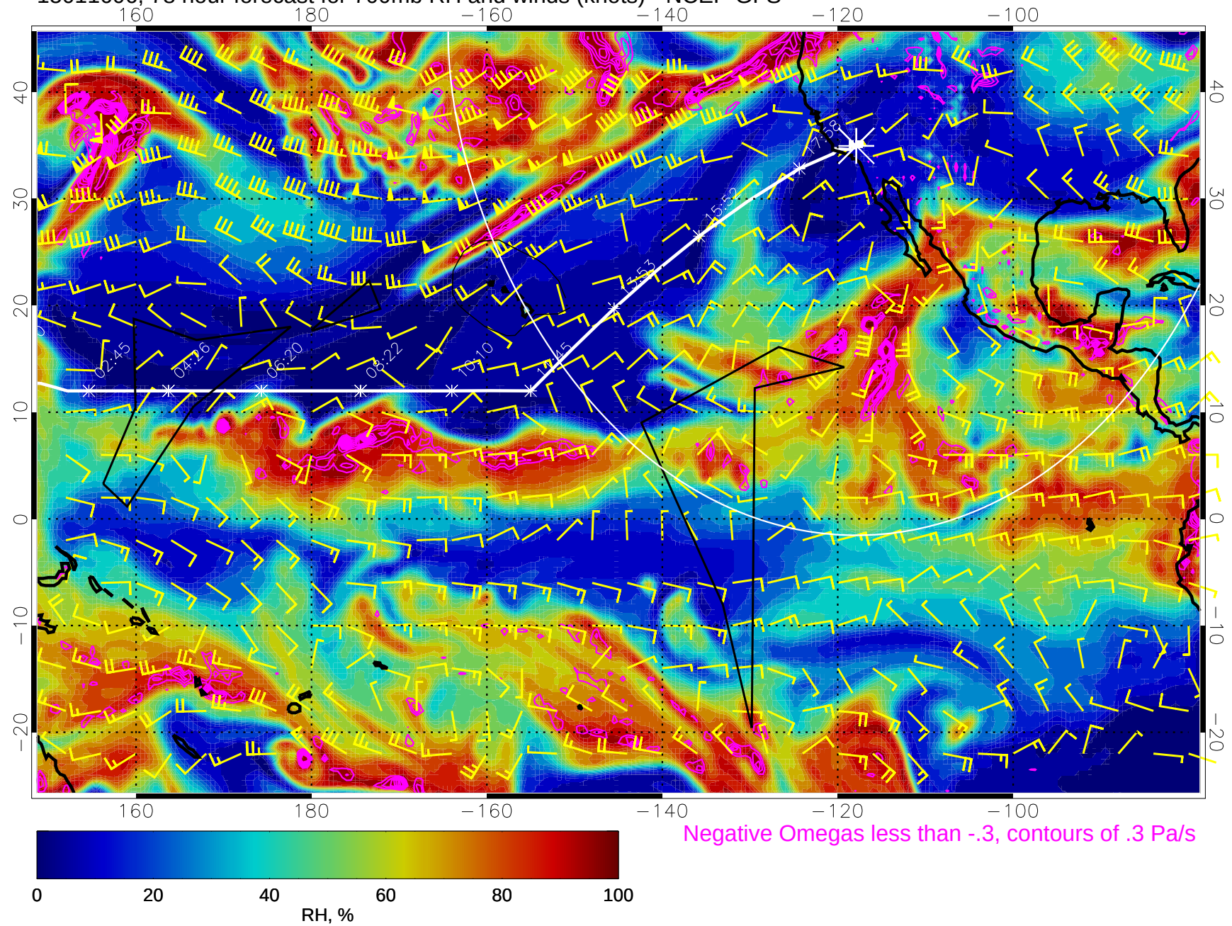
15011606, 78 hour forecast for 700mb RH and winds (knots) - NCEP GFS
