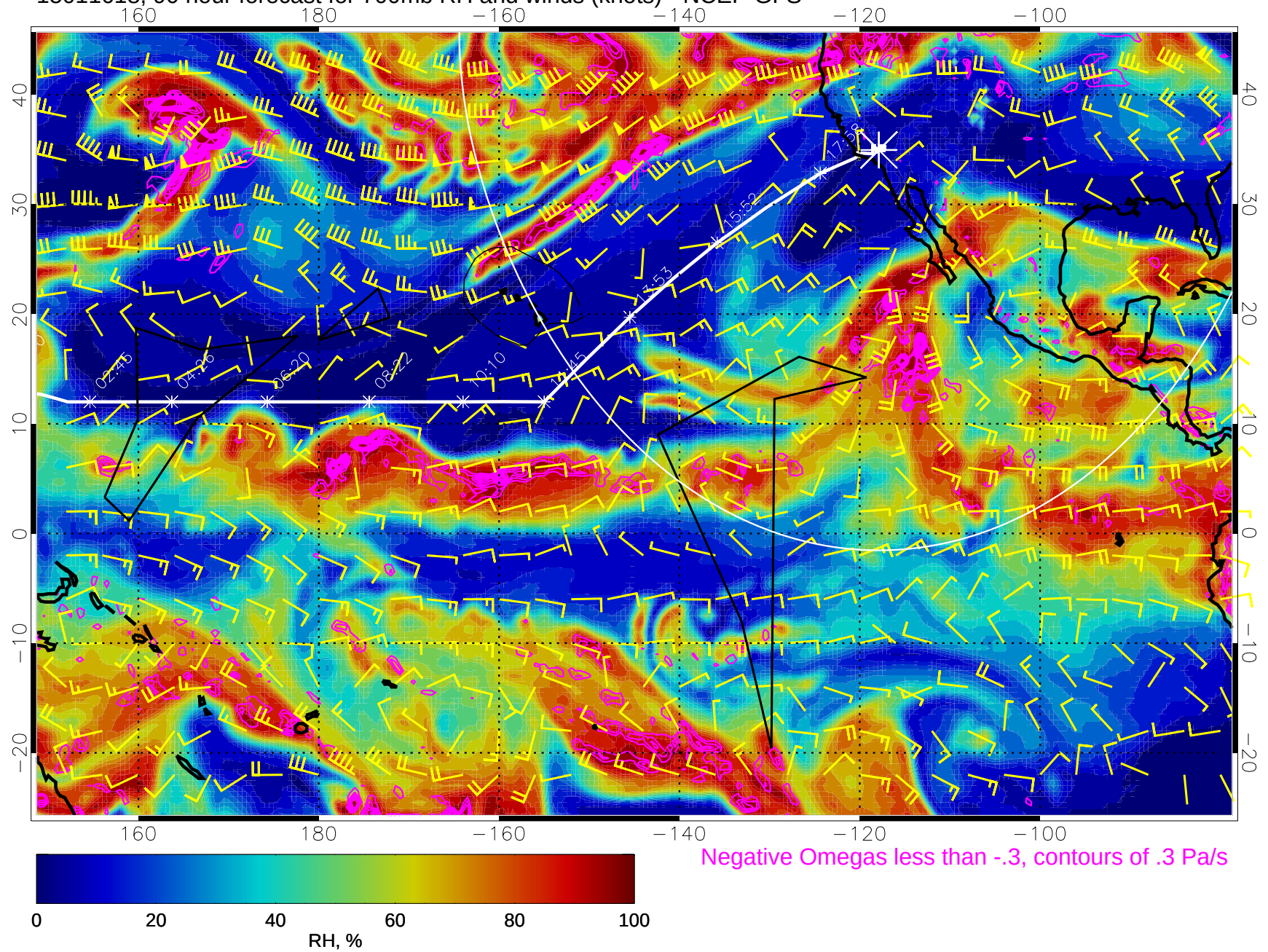
15011618, 90 hour forecast for 700mb RH and winds (knots) - NCEP GFS
