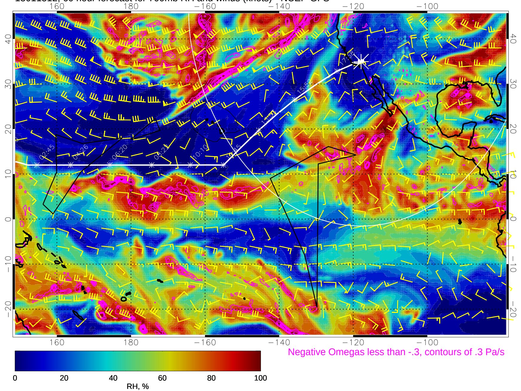
15011512, 60 hour forecast for 700mb RH and winds (knots) - NCEP GFS
