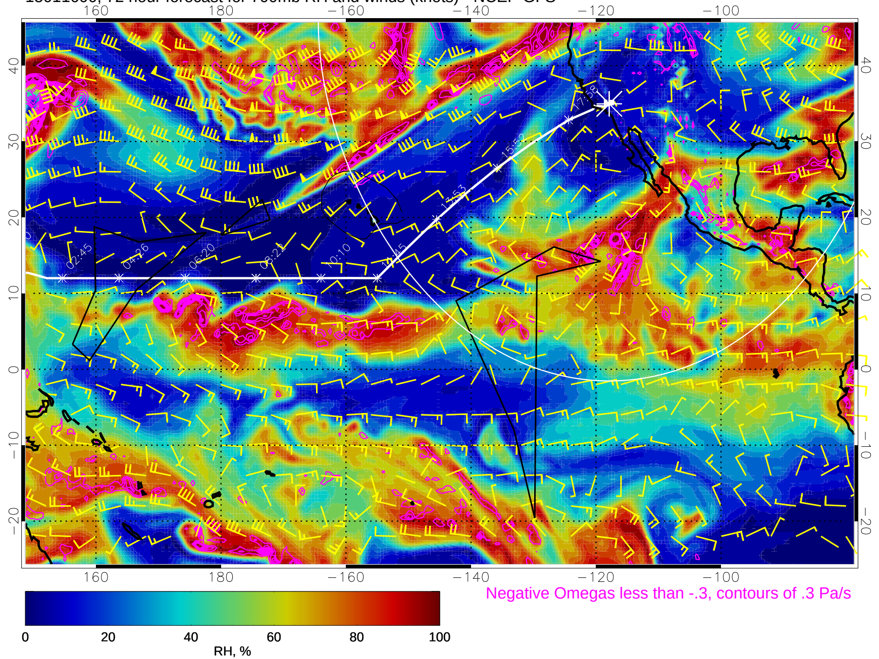
15011600, 72 hour forecast for 700mb RH and winds (knots) - NCEP GFS
