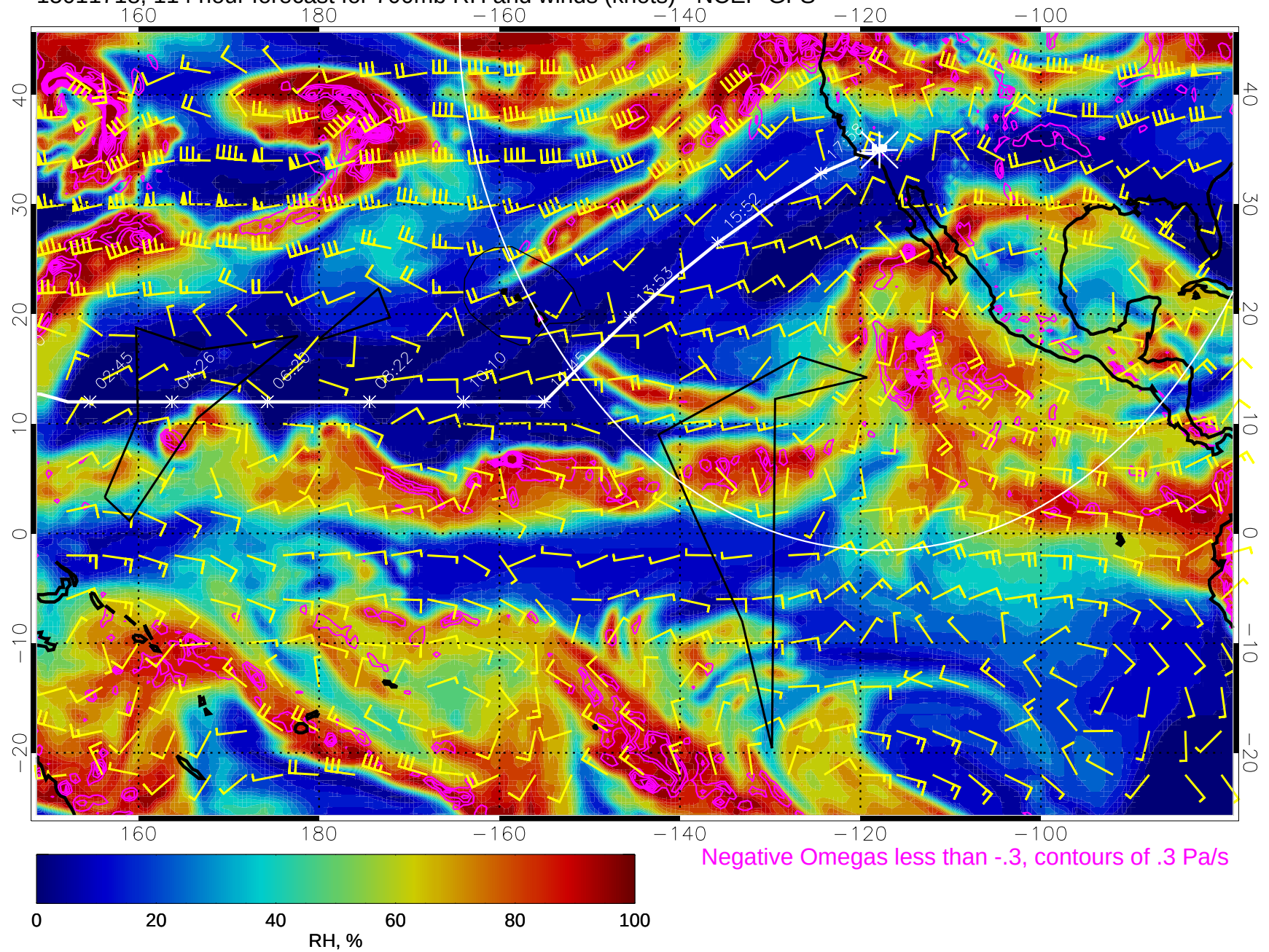
15011718, 114 hour forecast for 700mb RH and winds (knots) - NCEP GFS
