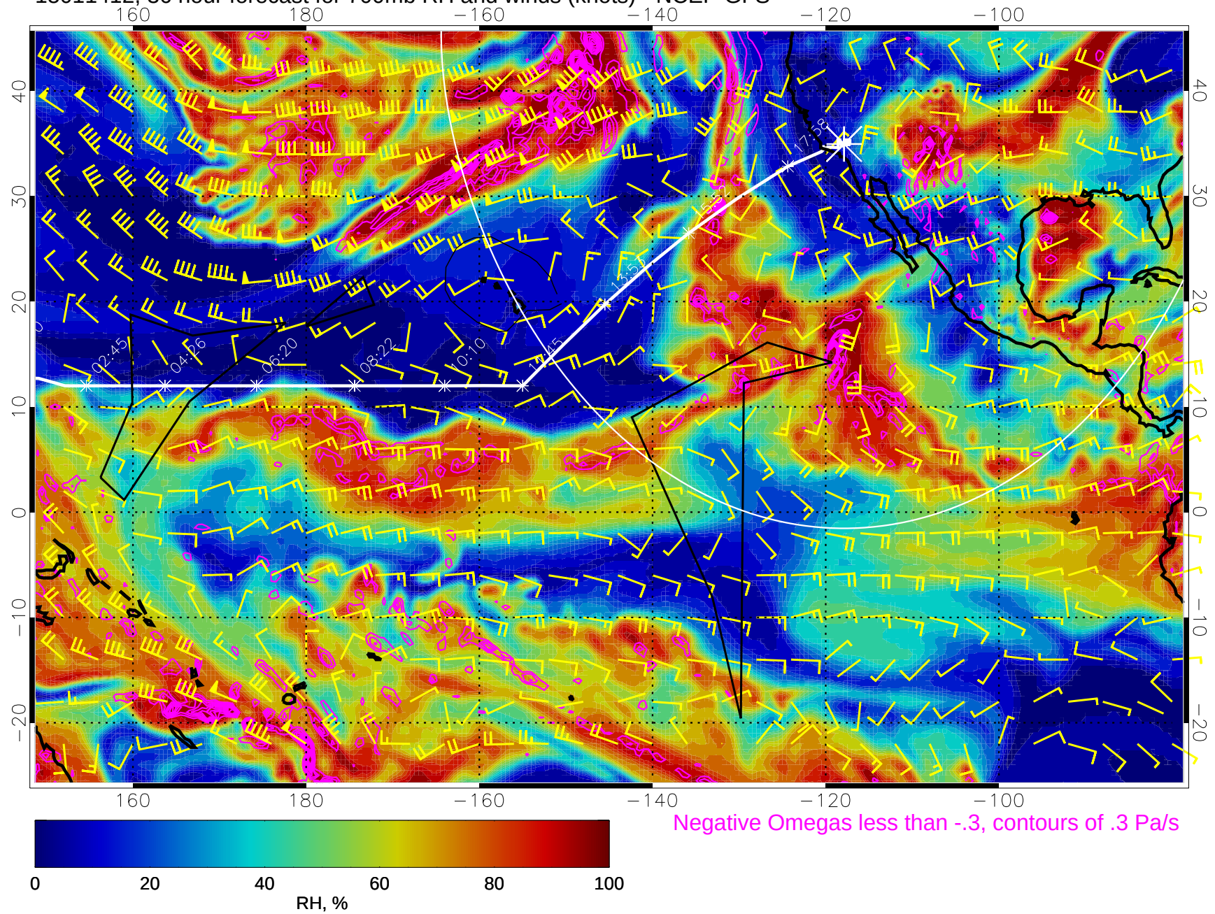
15011412, 36 hour forecast for 700mb RH and winds (knots) - NCEP GFS
