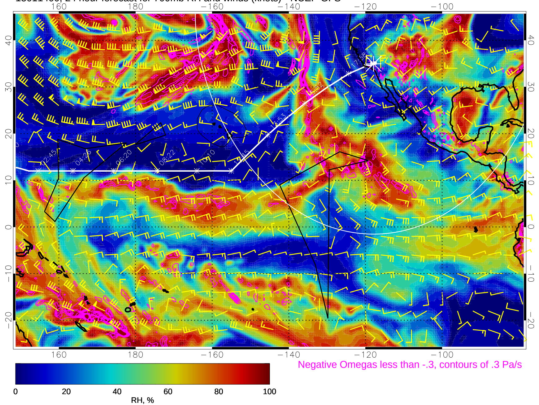
15011400, 24 hour forecast for 700mb RH and winds (knots) - NCEP GFS
