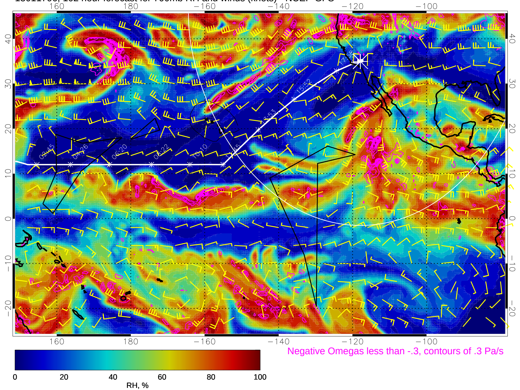
15011706, 102 hour forecast for 700mb RH and winds (knots) - NCEP GFS
