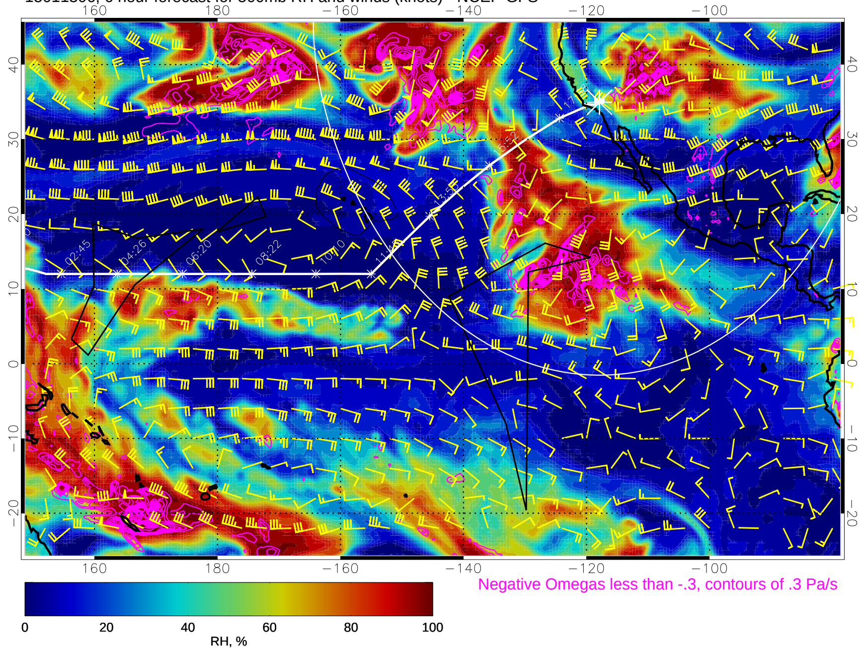
15011306, 6 hour forecast for 500mb RH and winds (knots) - NCEP GFS
