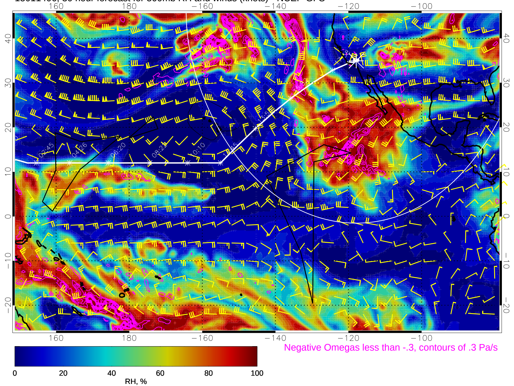
15011406, 30 hour forecast for 500mb RH and winds (knots) - NCEP GFS
