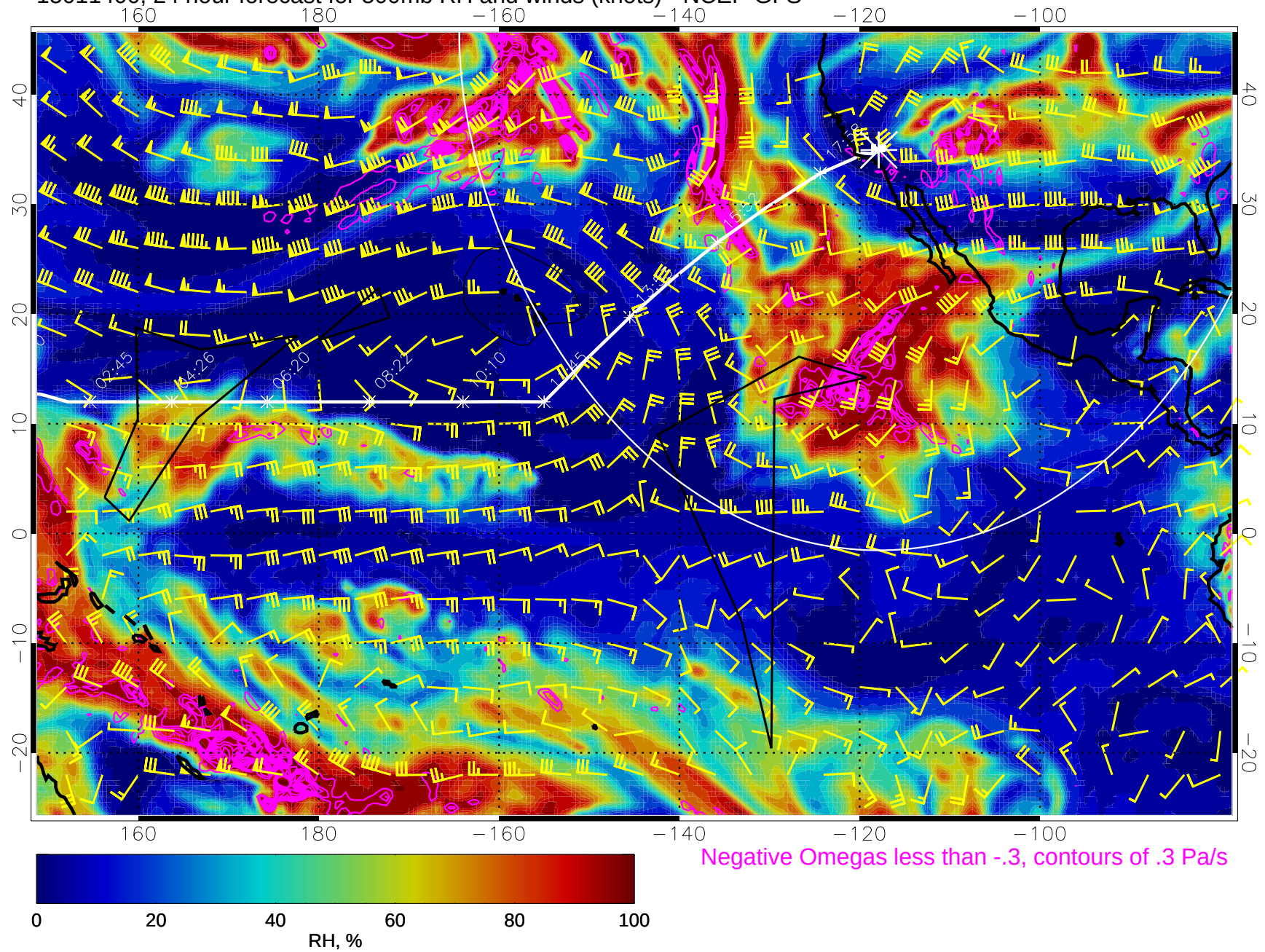
15011400, 24 hour forecast for 500mb RH and winds (knots) - NCEP GFS
