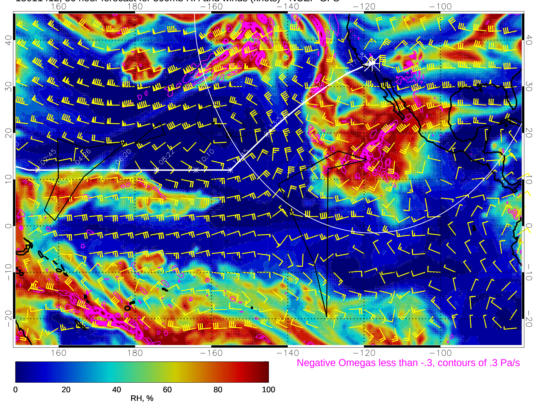
15011412, 36 hour forecast for 500mb RH and winds (knots) - NCEP GFS
