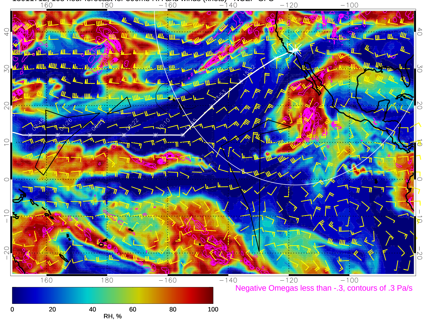
15011712, 108 hour forecast for 500mb RH and winds (knots) - NCEP GFS
