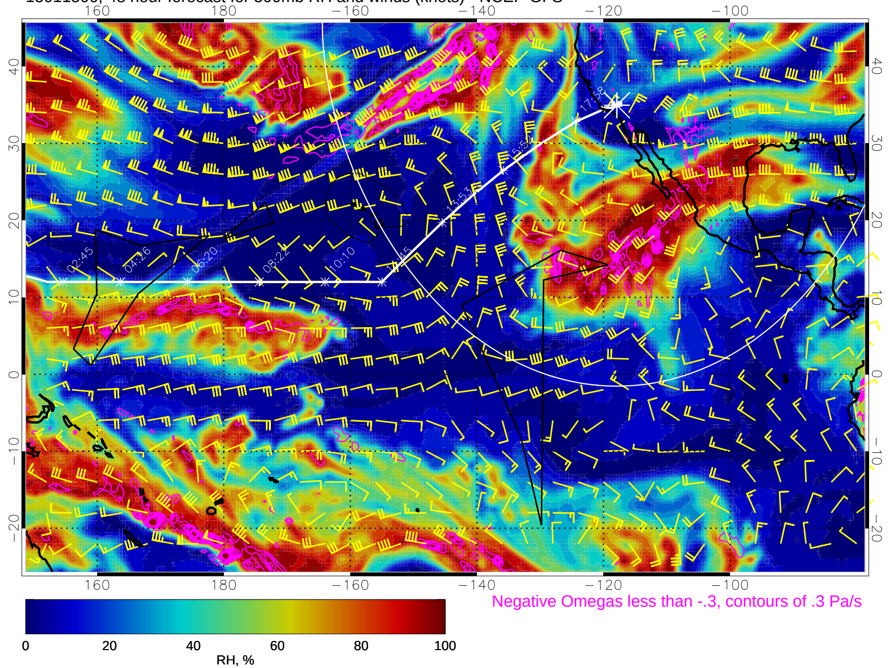
15011500, 48 hour forecast for 500mb RH and winds (knots) - NCEP GFS
