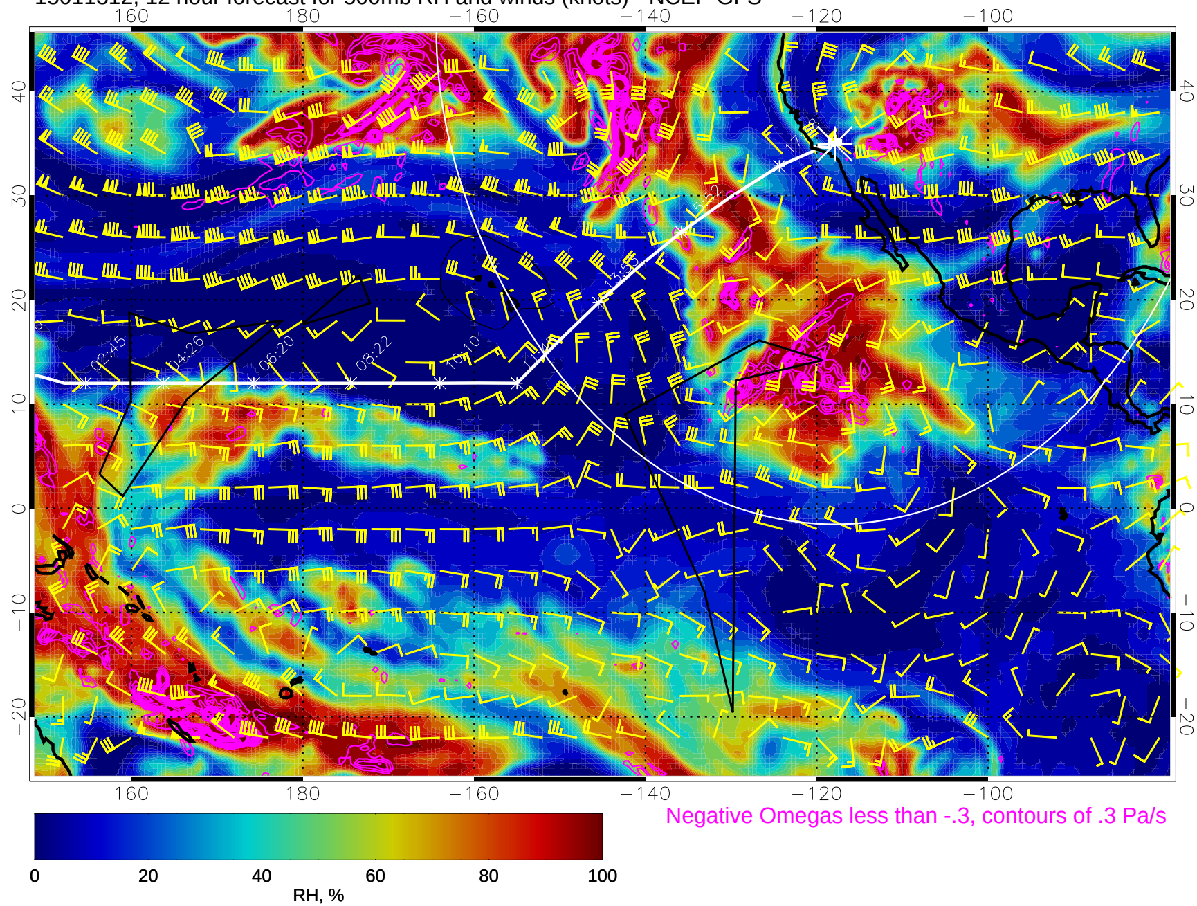
15011312, 12 hour forecast for 500mb RH and winds (knots) - NCEP GFS
