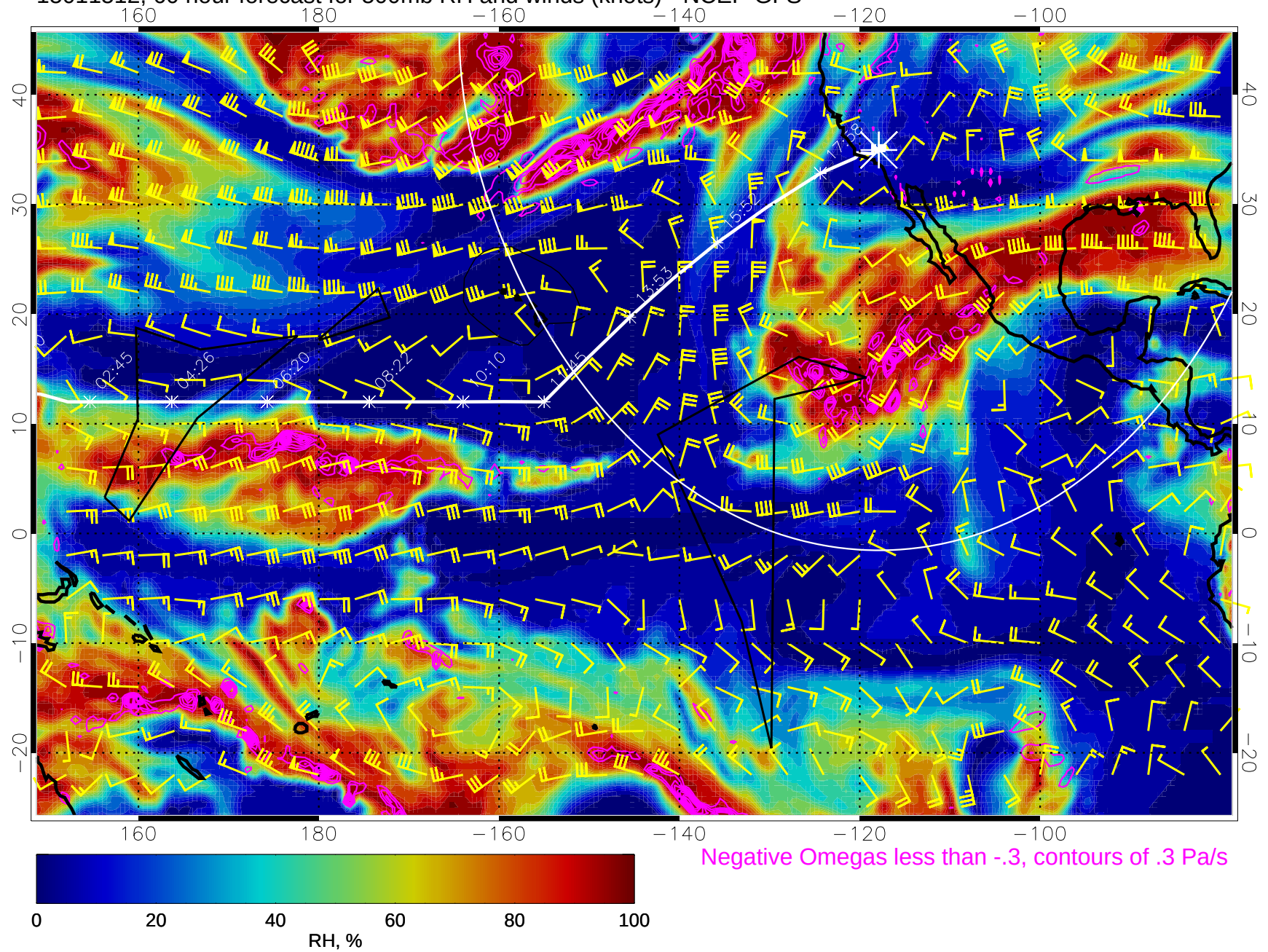
15011512, 60 hour forecast for 500mb RH and winds (knots) - NCEP GFS
