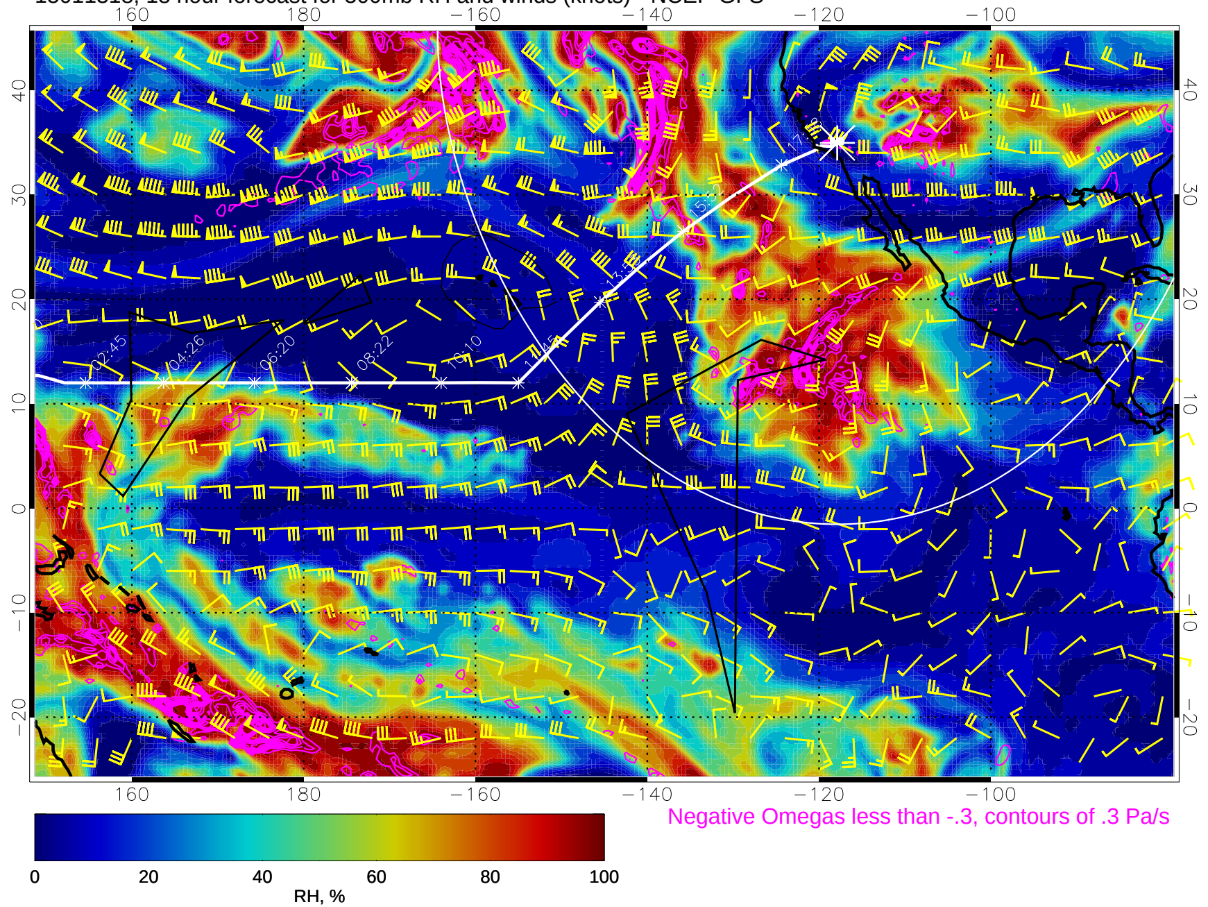
15011318, 18 hour forecast for 500mb RH and winds (knots) - NCEP GFS
