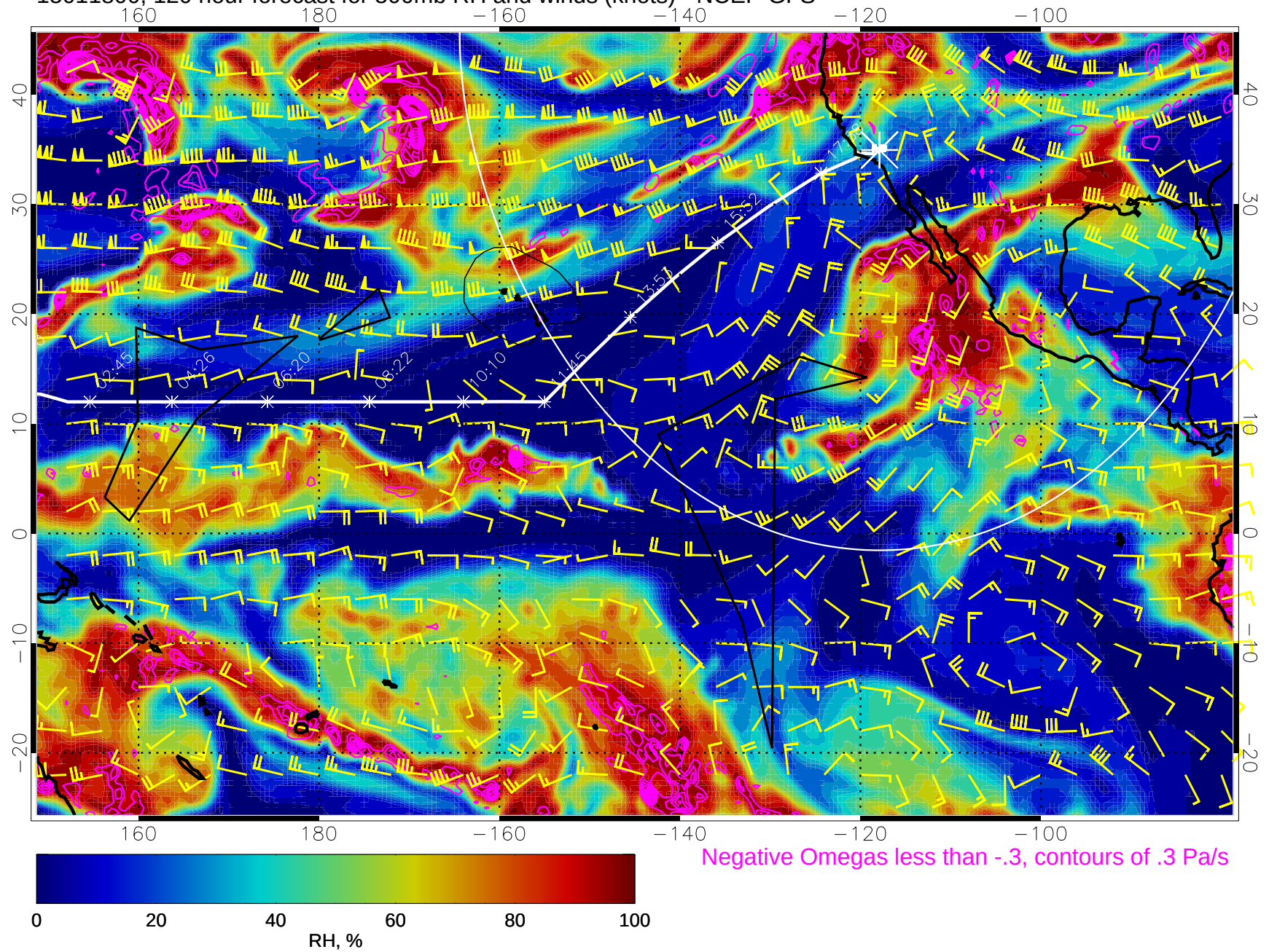
15011800, 120 hour forecast for 500mb RH and winds (knots) - NCEP GFS
