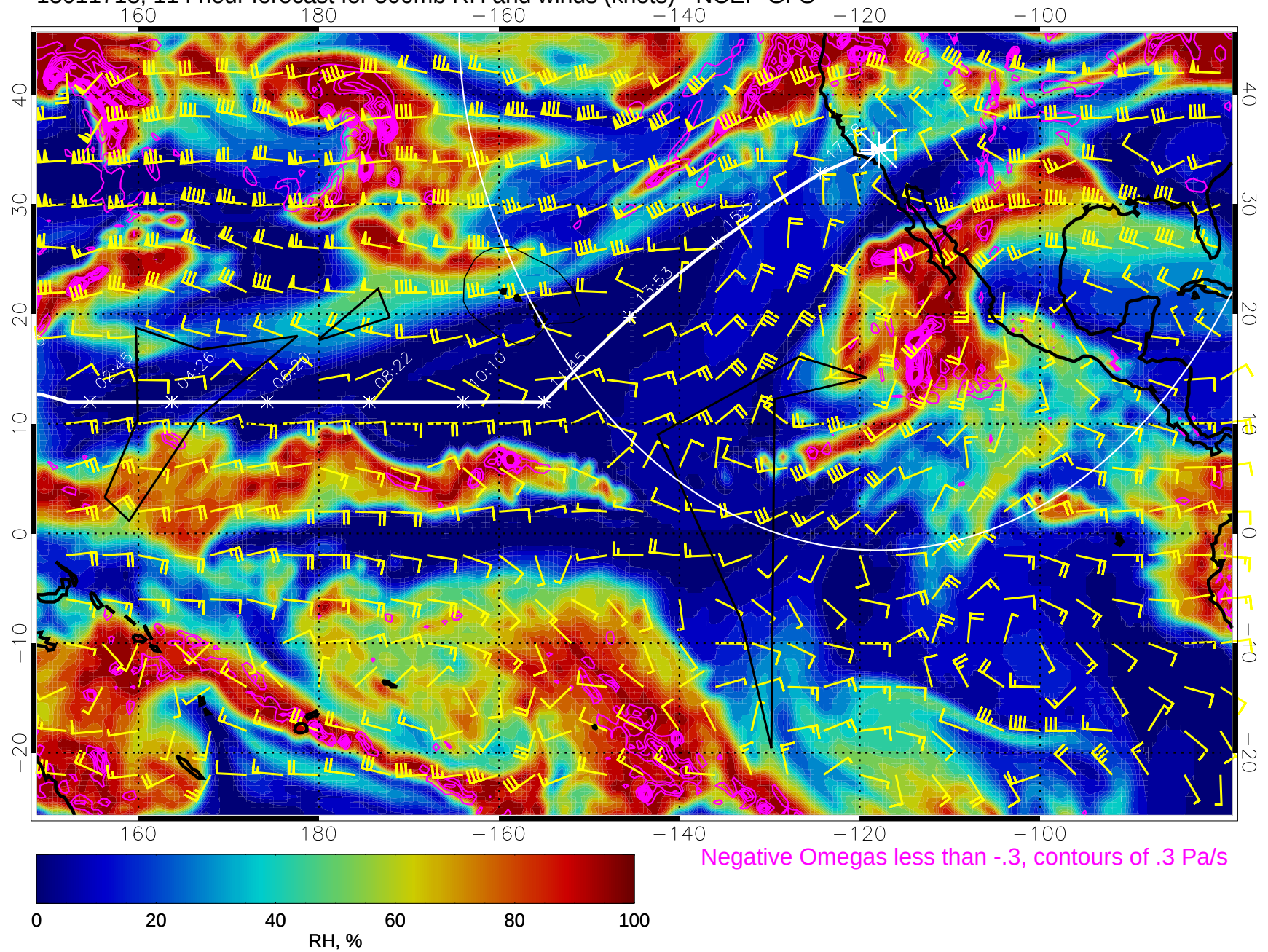
15011718, 114 hour forecast for 500mb RH and winds (knots) - NCEP GFS
