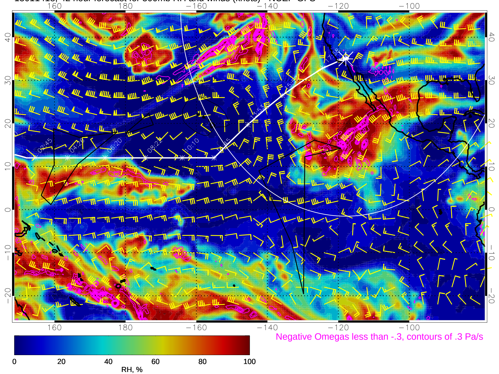
15011418, 42 hour forecast for 500mb RH and winds (knots) - NCEP GFS
