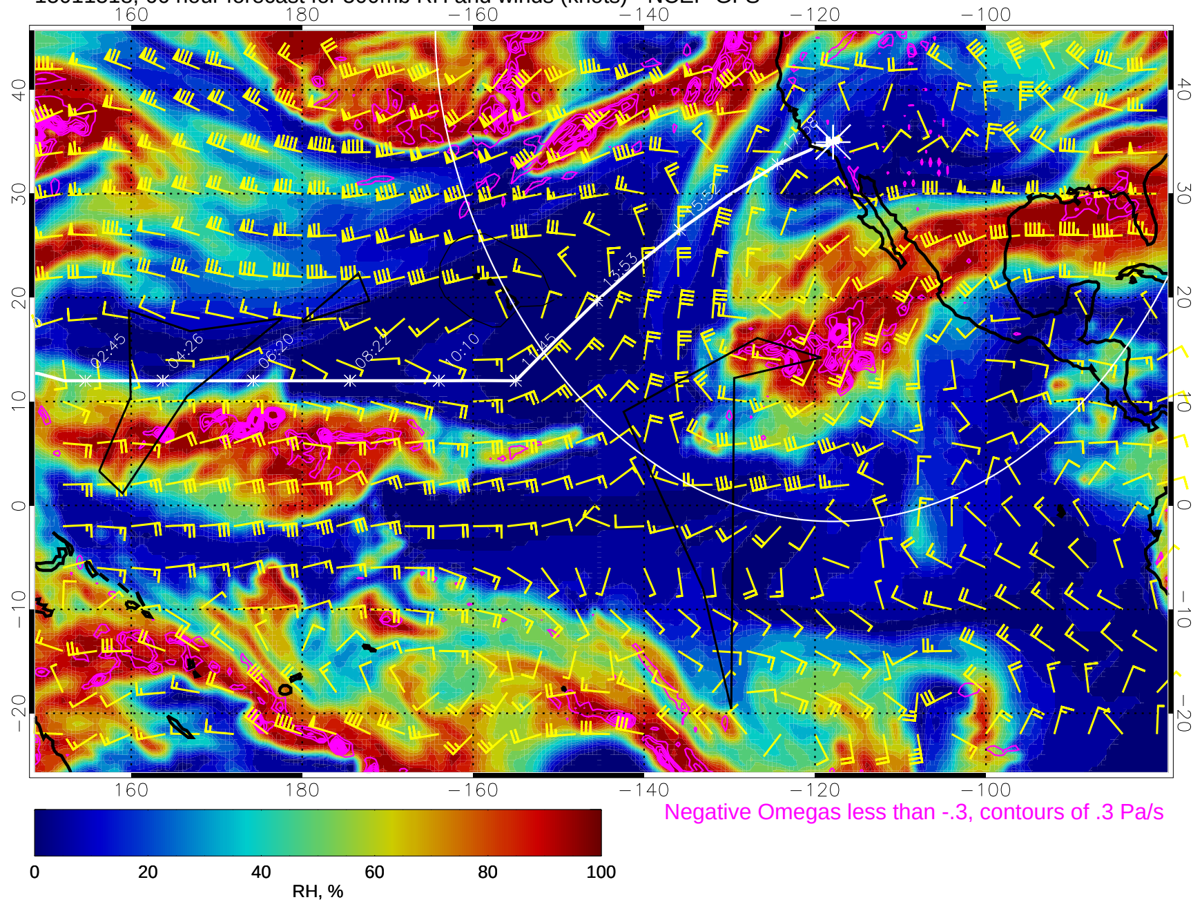
15011518, 66 hour forecast for 500mb RH and winds (knots) - NCEP GFS
