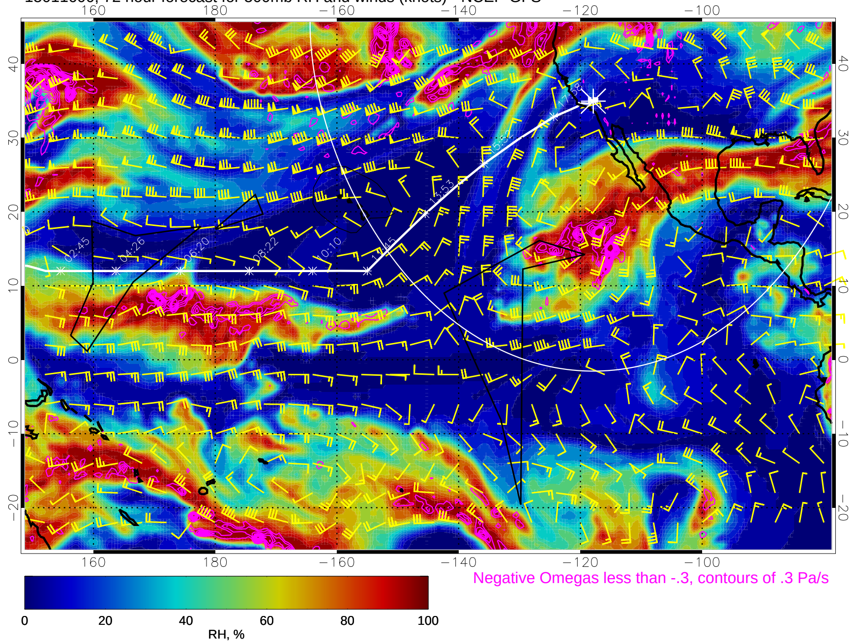
15011600, 72 hour forecast for 500mb RH and winds (knots) - NCEP GFS
