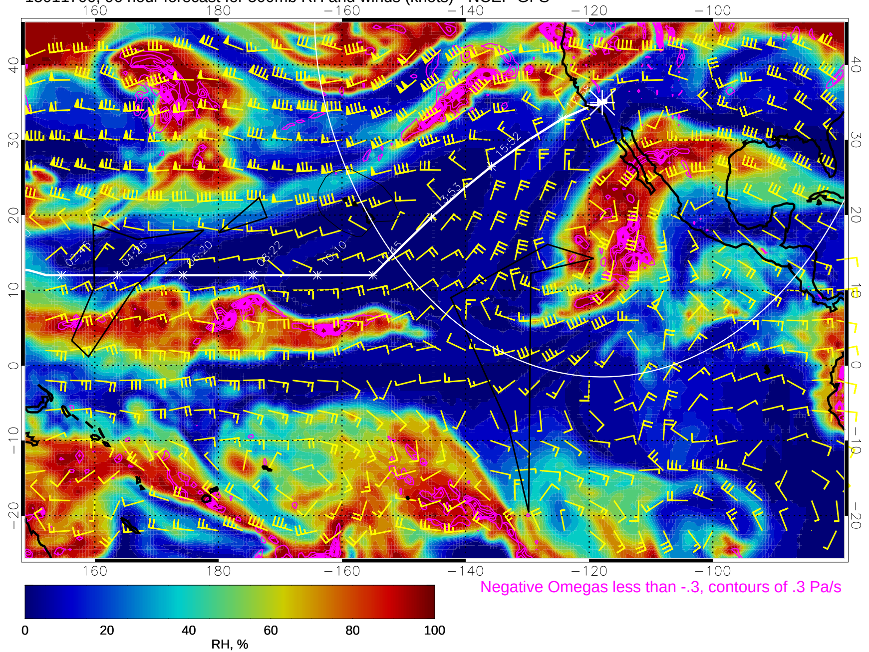
15011700, 96 hour forecast for 500mb RH and winds (knots) - NCEP GFS
