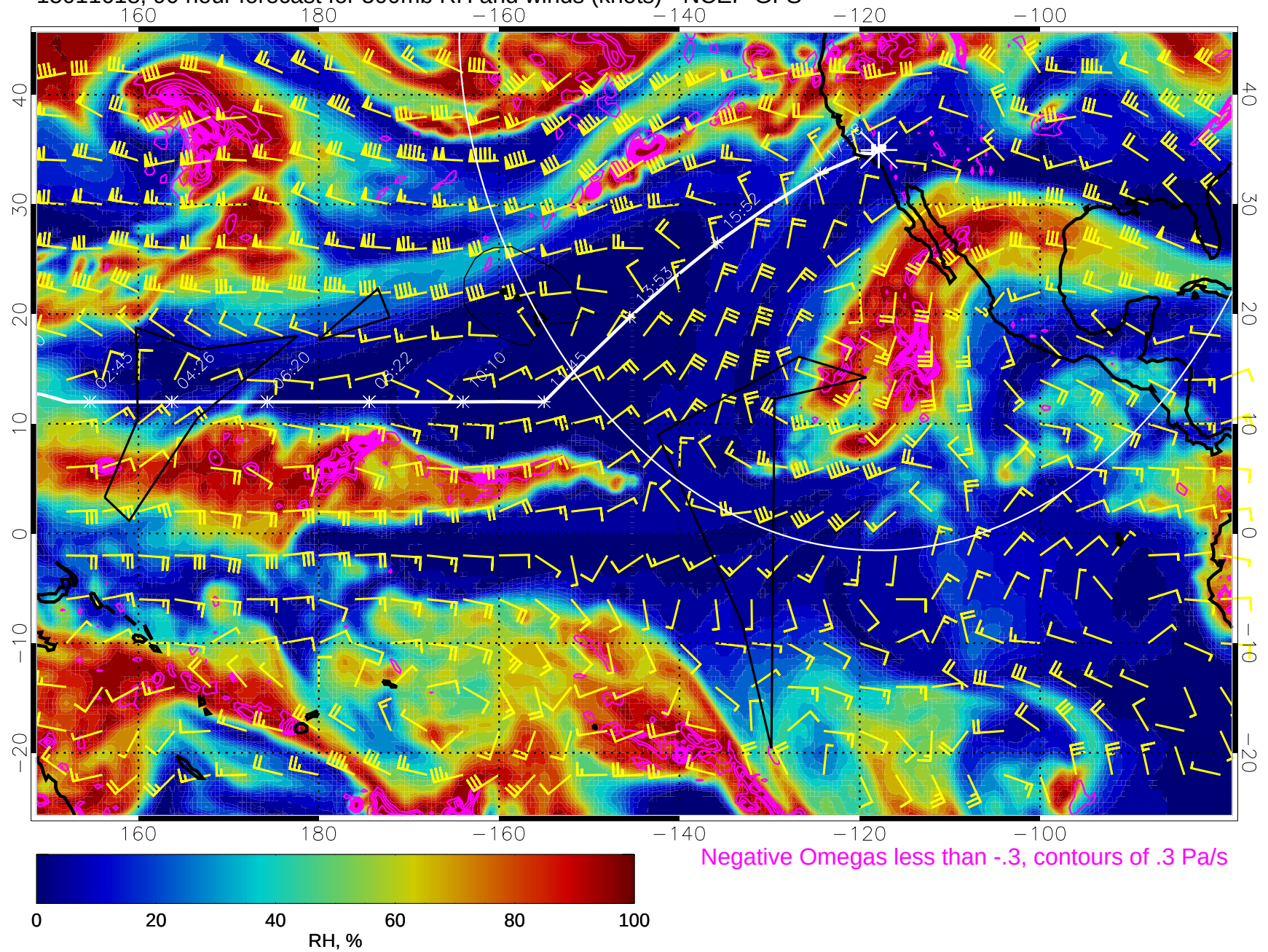
15011618, 90 hour forecast for 500mb RH and winds (knots) - NCEP GFS
