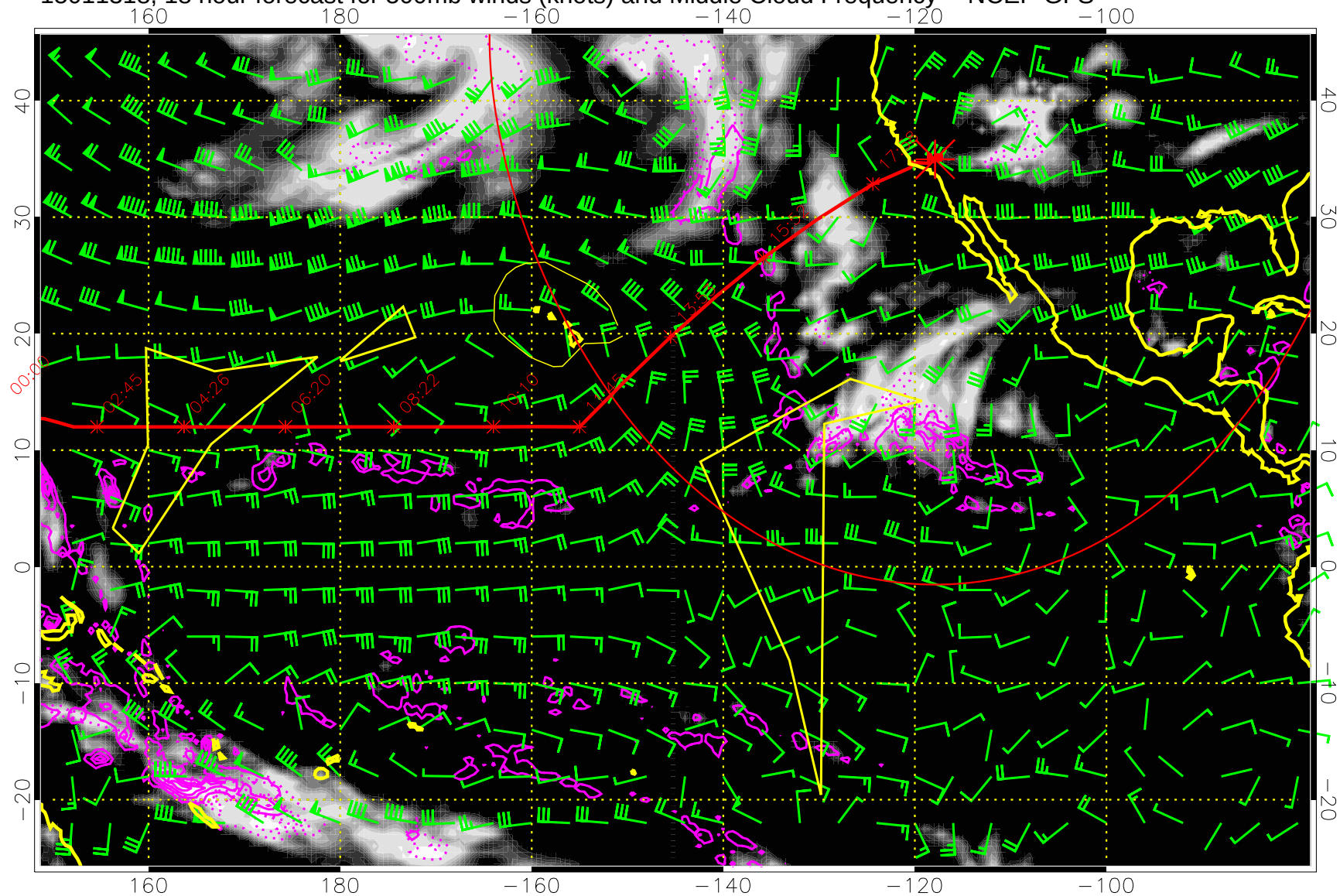
15011318, 18 hour forecast for 500mb winds (knots) and Middle Cloud Frequency -- NCEP GFS
