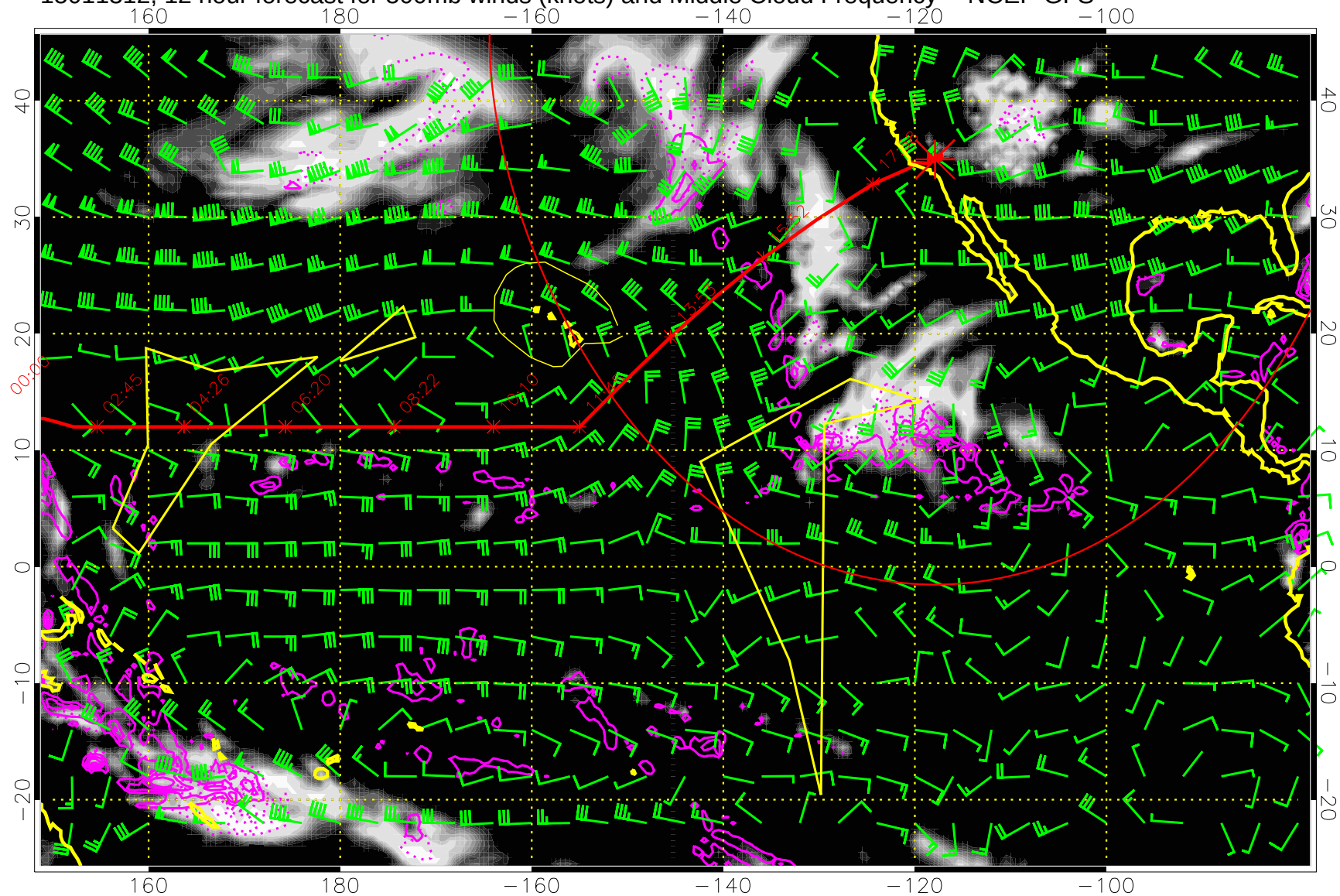
15011312, 12 hour forecast for 500mb winds (knots) and Middle Cloud Frequency -- NCEP GFS
