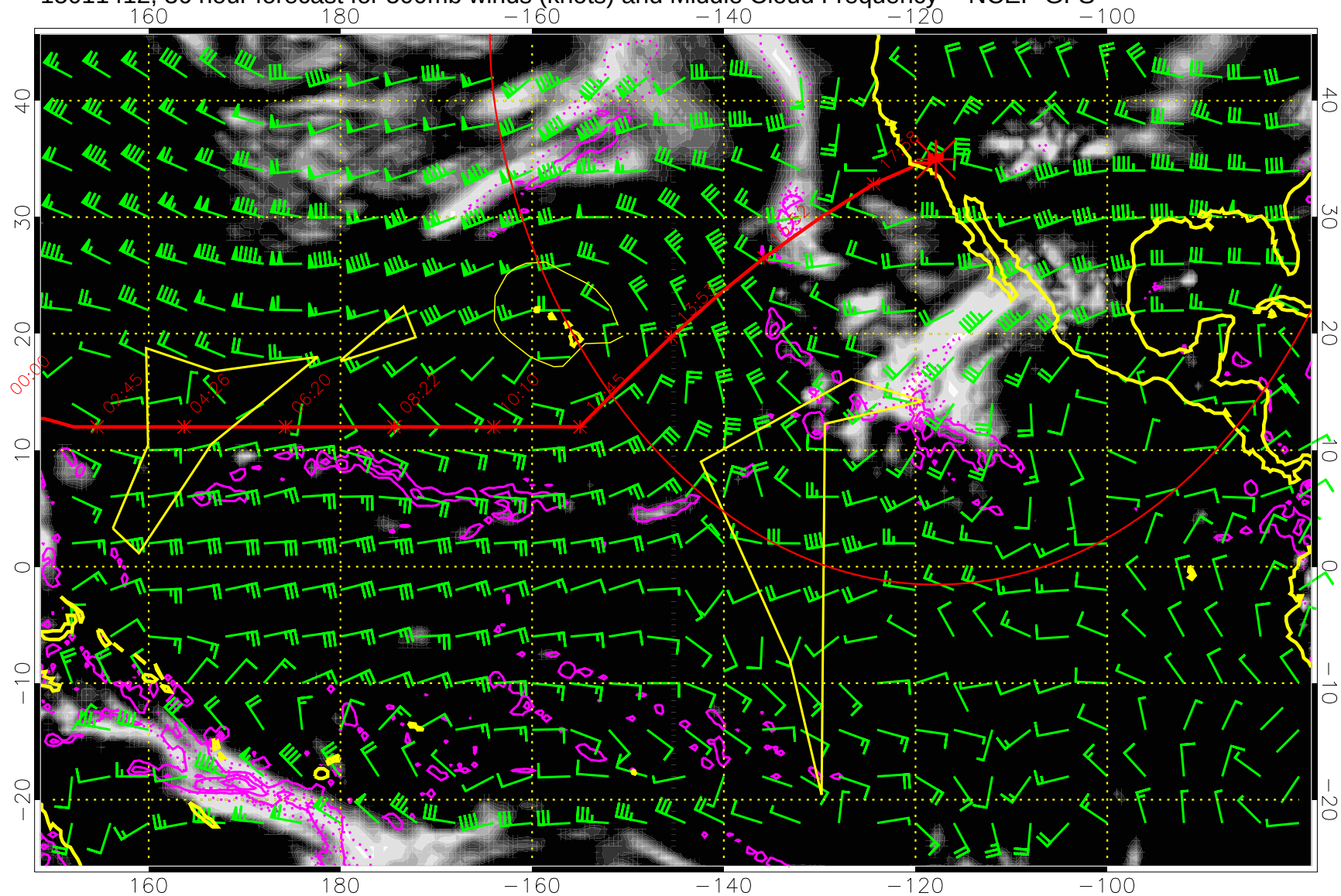
15011412, 36 hour forecast for 500mb winds (knots) and Middle Cloud Frequency -- NCEP GFS
