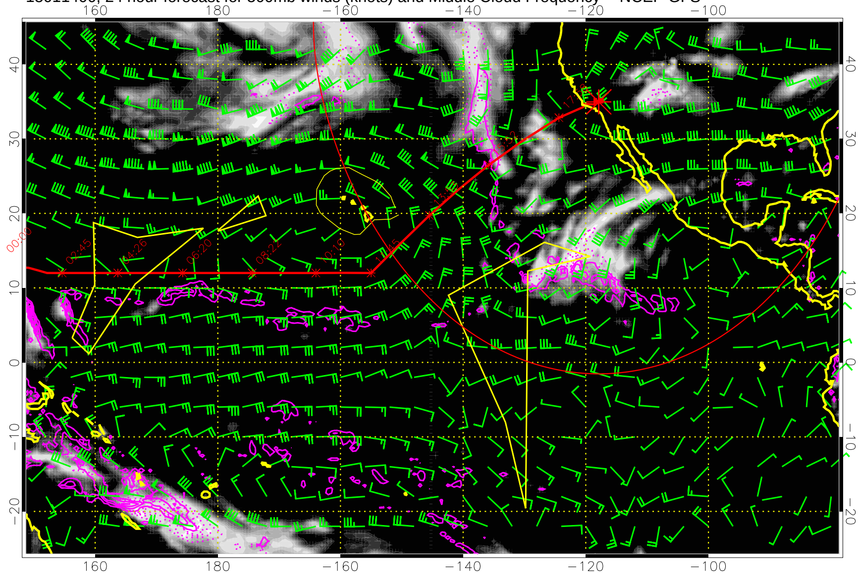
15011400, 24 hour forecast for 500mb winds (knots) and Middle Cloud Frequency -- NCEP GFS
