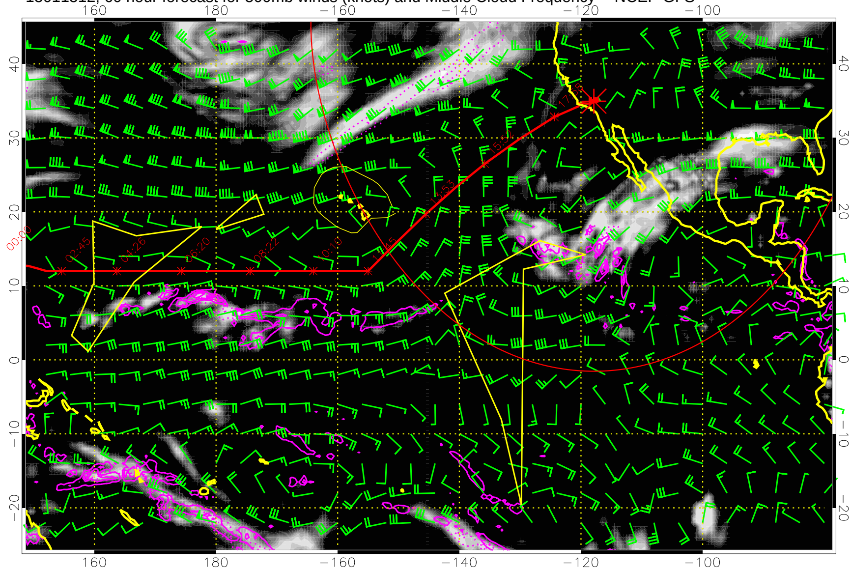
15011512, 60 hour forecast for 500mb winds (knots) and Middle Cloud Frequency -- NCEP GFS
