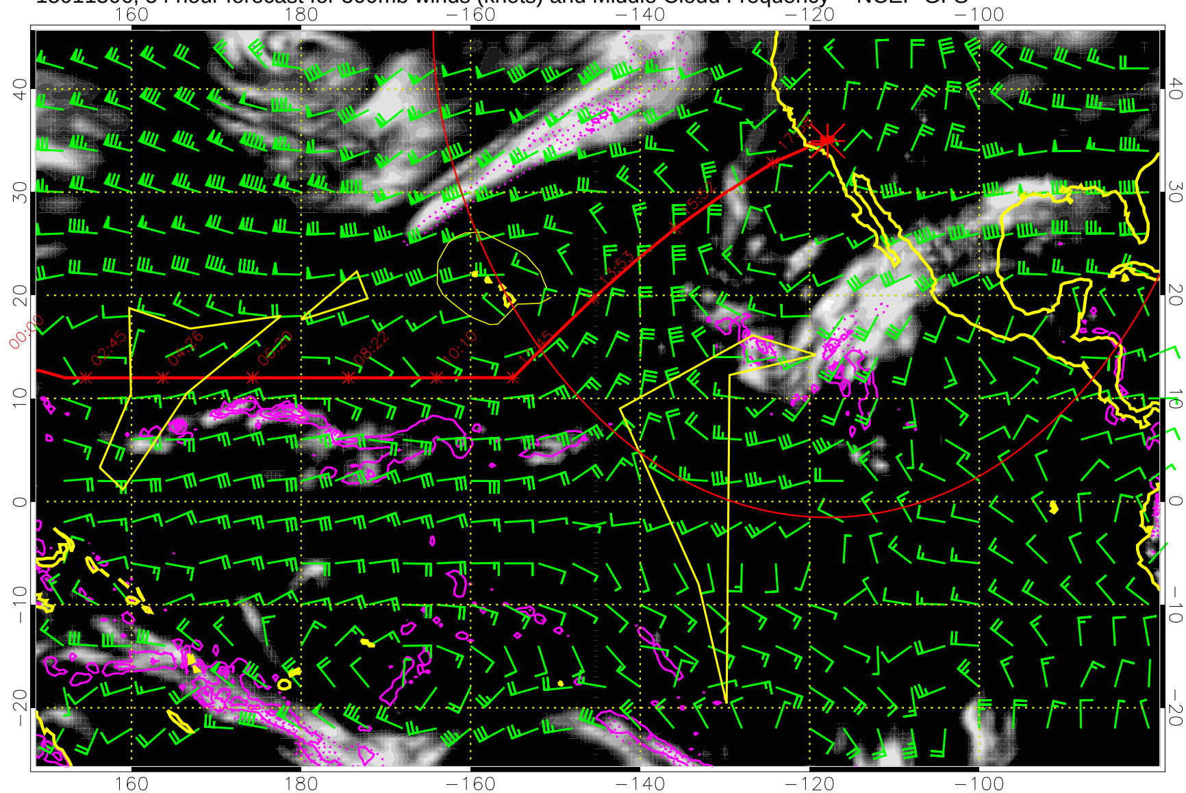
15011506, 54 hour forecast for 500mb winds (knots) and Middle Cloud Frequency -- NCEP GFS
