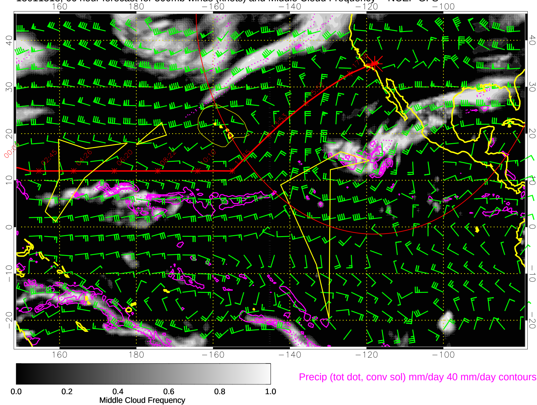
15011518, 66 hour forecast for 500mb winds (knots) and Middle Cloud Frequency -- NCEP GFS
