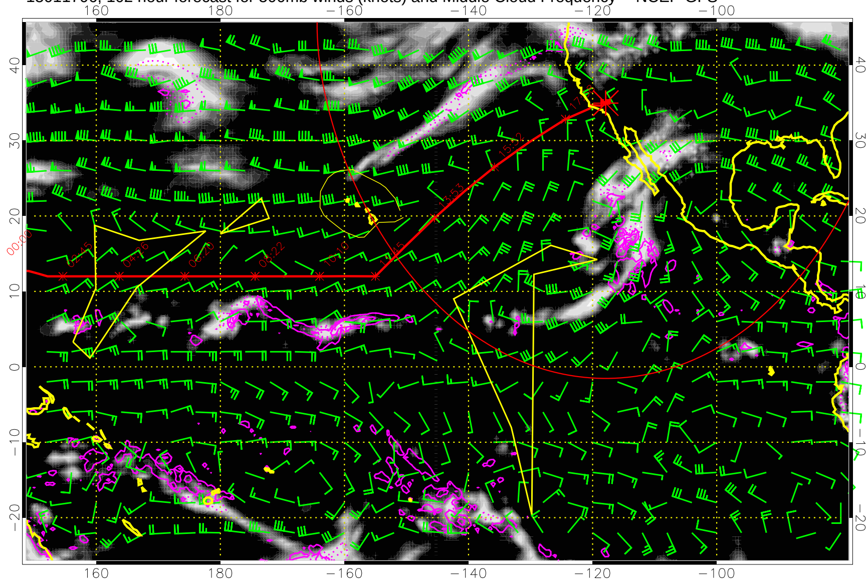
15011706, 102 hour forecast for 500mb winds (knots) and Middle Cloud Frequency -- NCEP GFS
