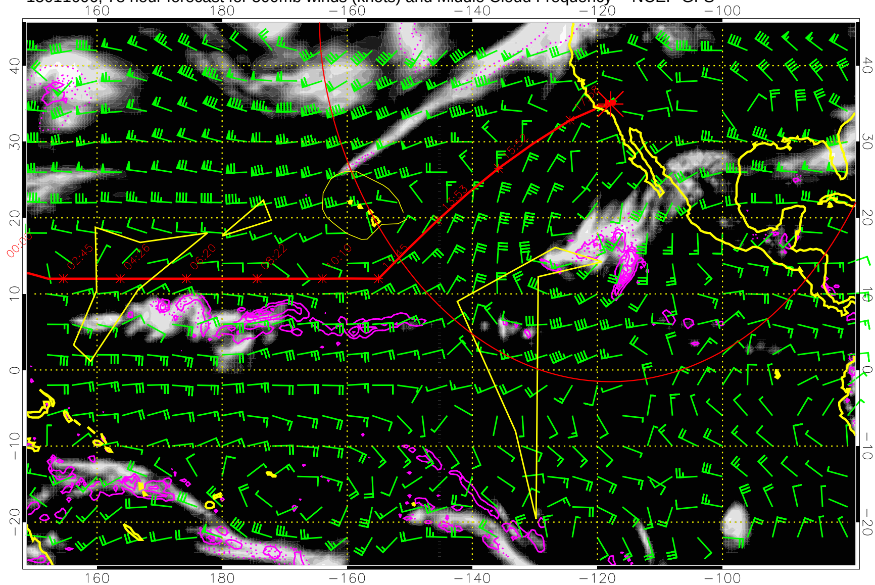
15011606, 78 hour forecast for 500mb winds (knots) and Middle Cloud Frequency -- NCEP GFS
