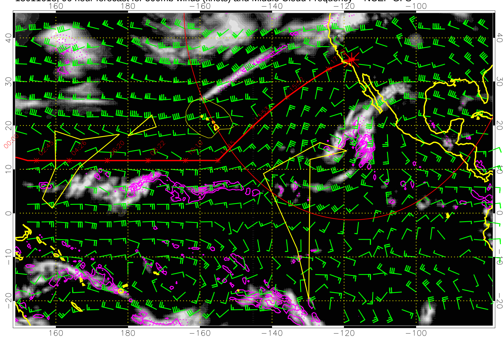
15011618, 90 hour forecast for 500mb winds (knots) and Middle Cloud Frequency -- NCEP GFS
