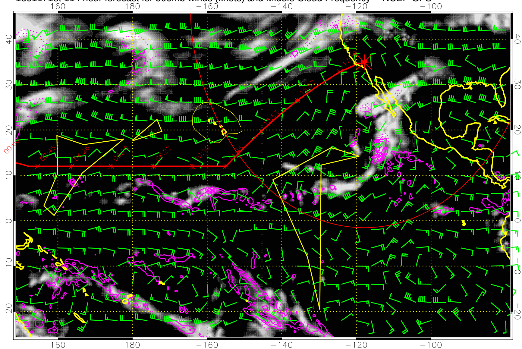
15011718, 114 hour forecast for 500mb winds (knots) and Middle Cloud Frequency -- NCEP GFS
