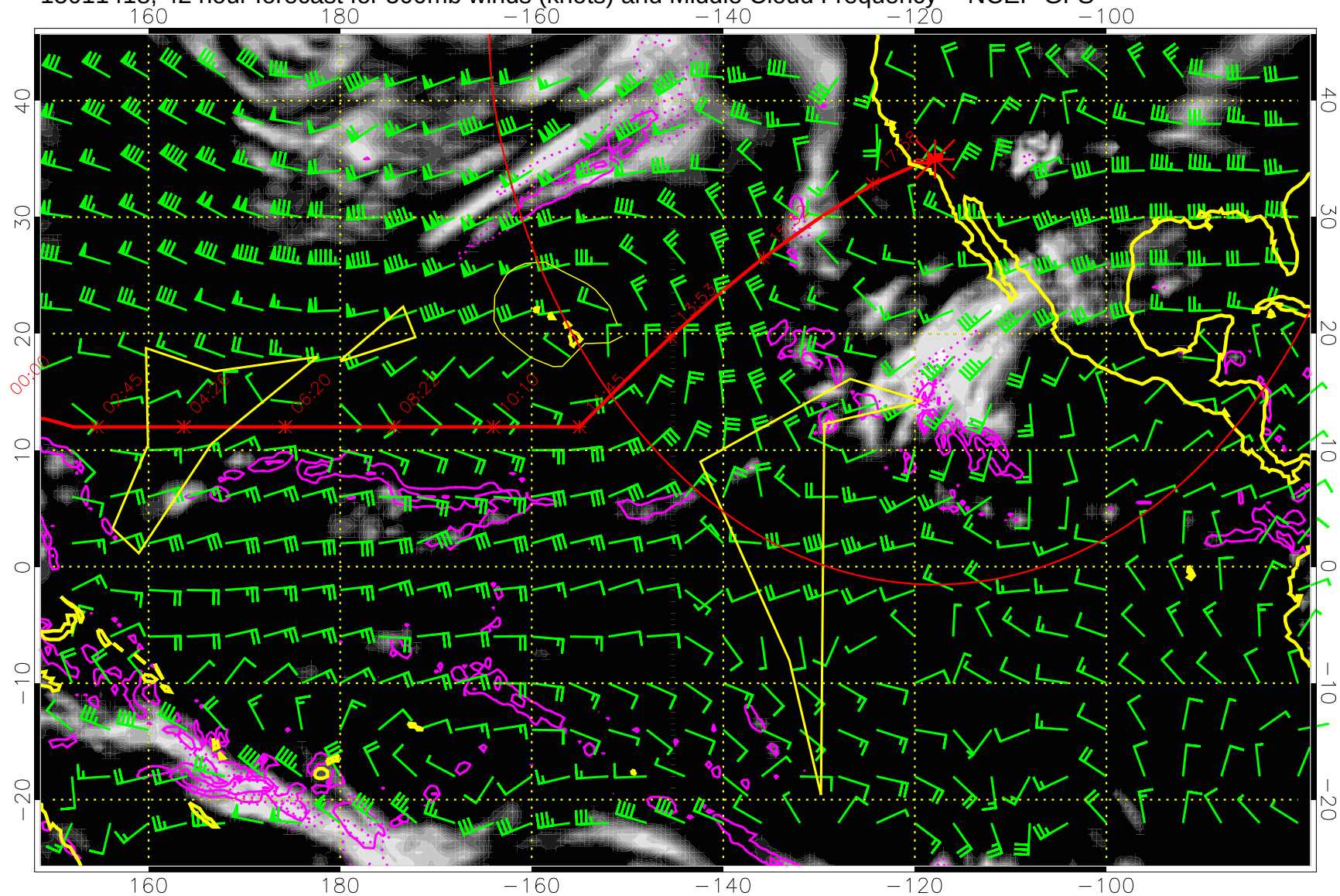
15011418, 42 hour forecast for 500mb winds (knots) and Middle Cloud Frequency -- NCEP GFS
