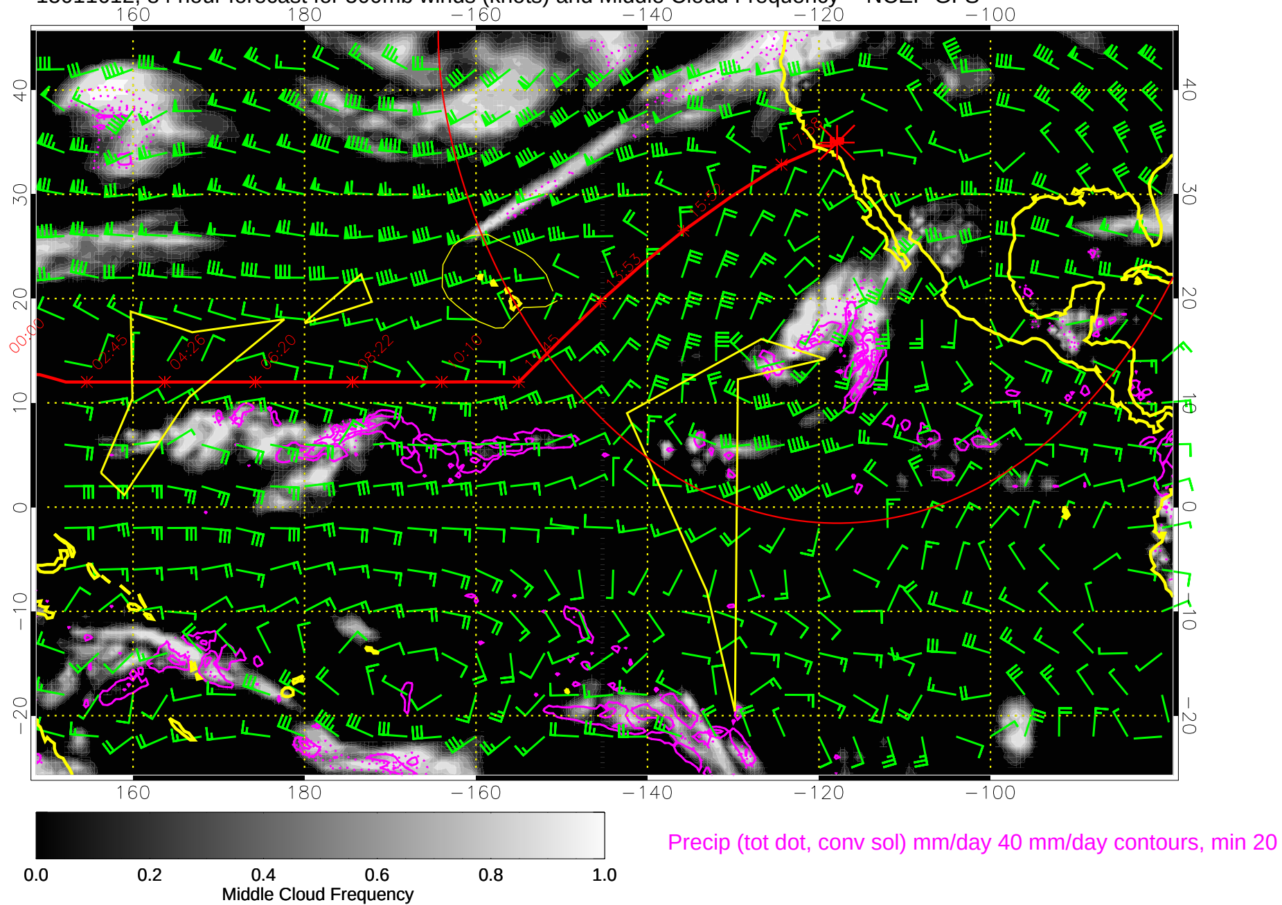
15011612, 84 hour forecast for 500mb winds (knots) and Middle Cloud Frequency -- NCEP GFS
