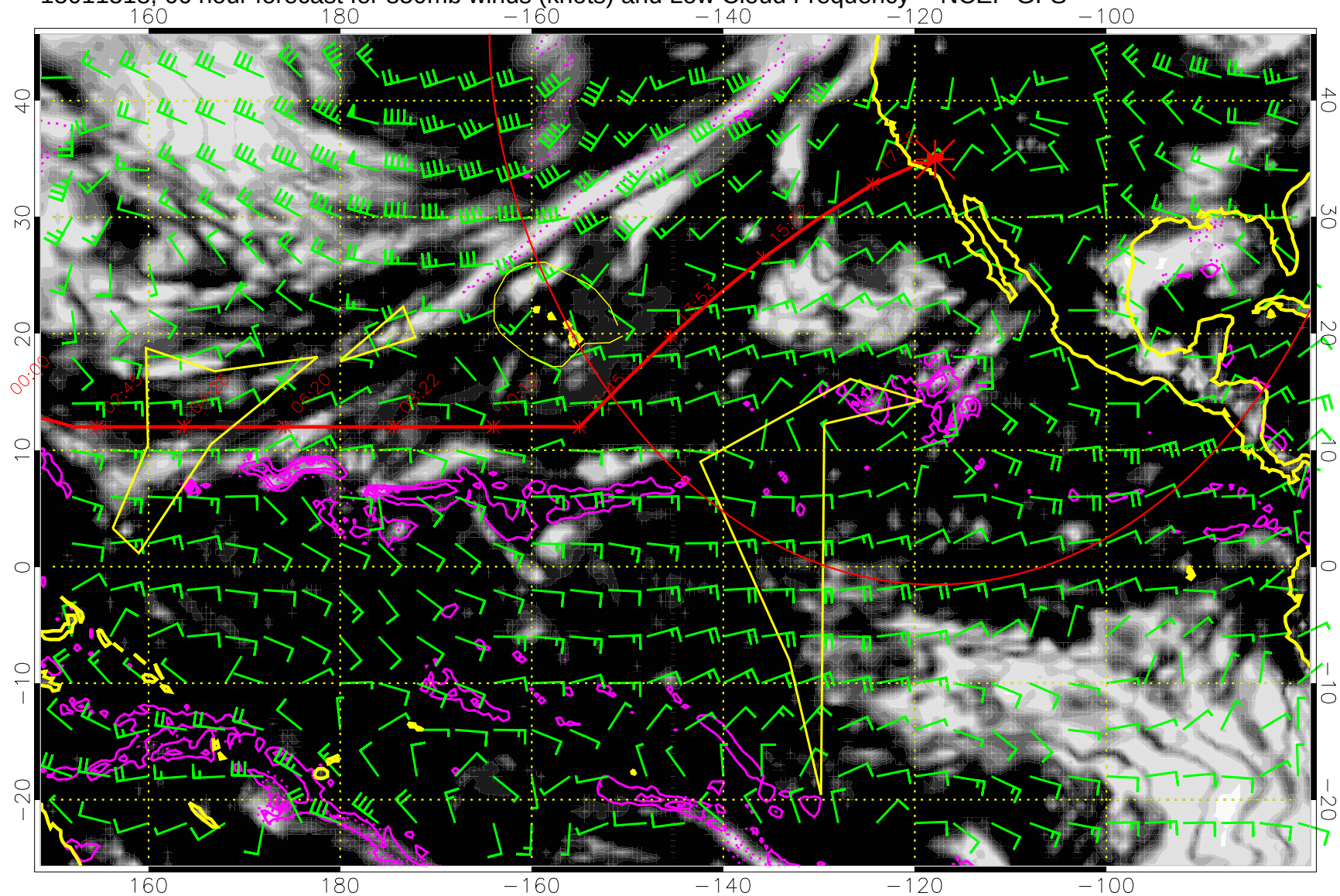
15011518, 66 hour forecast for 850mb winds (knots) and Low Cloud Frequency -- NCEP GFS
