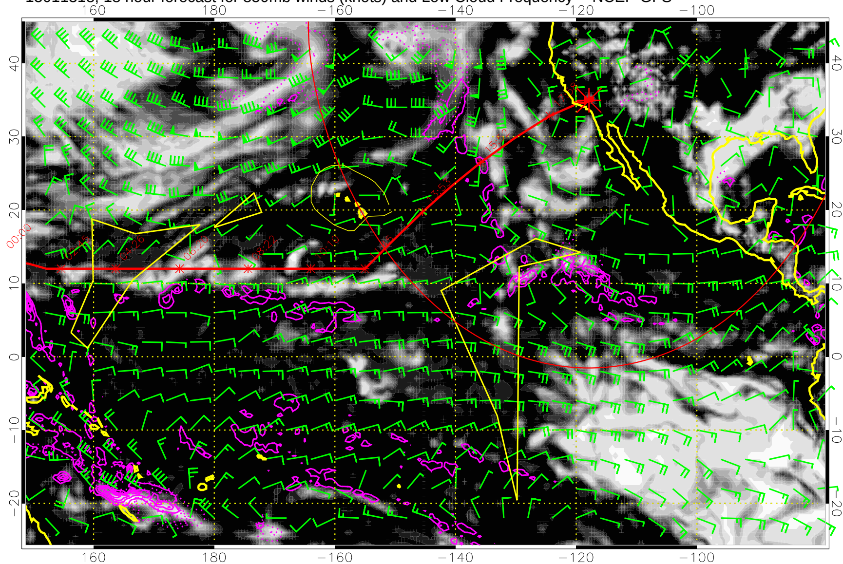
15011318, 18 hour forecast for 850mb winds (knots) and Low Cloud Frequency -- NCEP GFS
