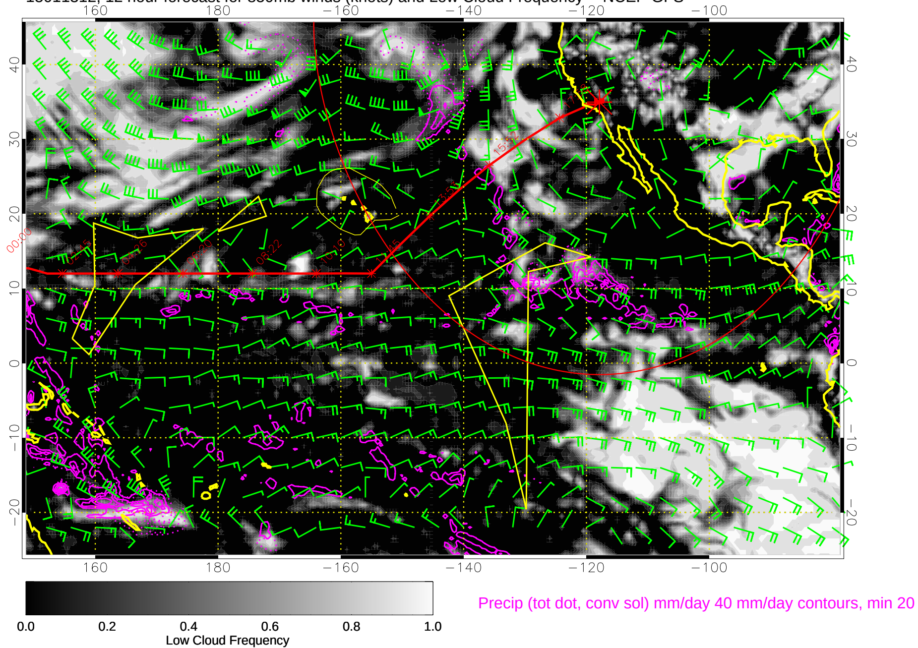
15011312, 12 hour forecast for 850mb winds (knots) and Low Cloud Frequency -- NCEP GFS
