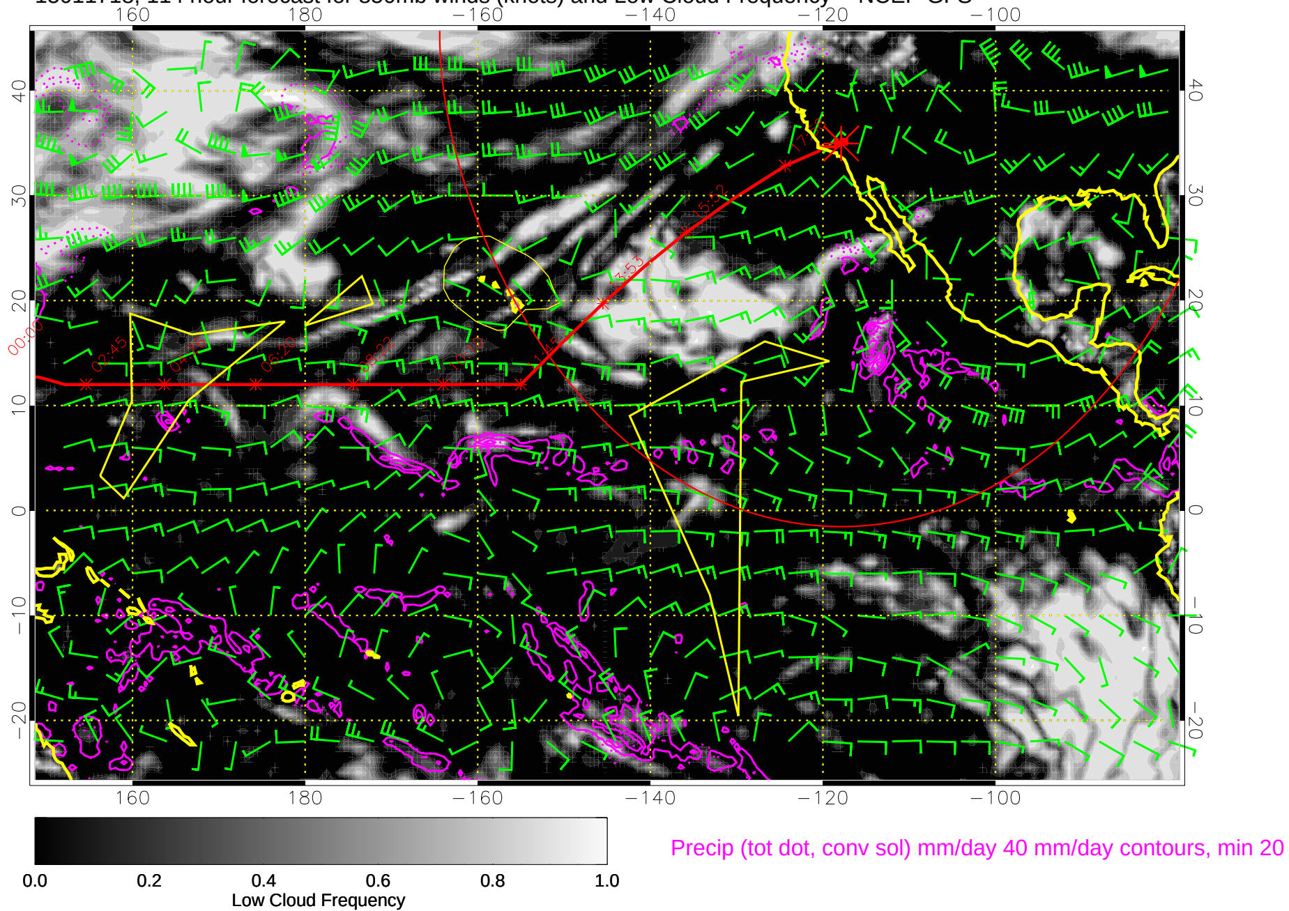
15011718, 114 hour forecast for 850mb winds (knots) and Low Cloud Frequency -- NCEP GFS
