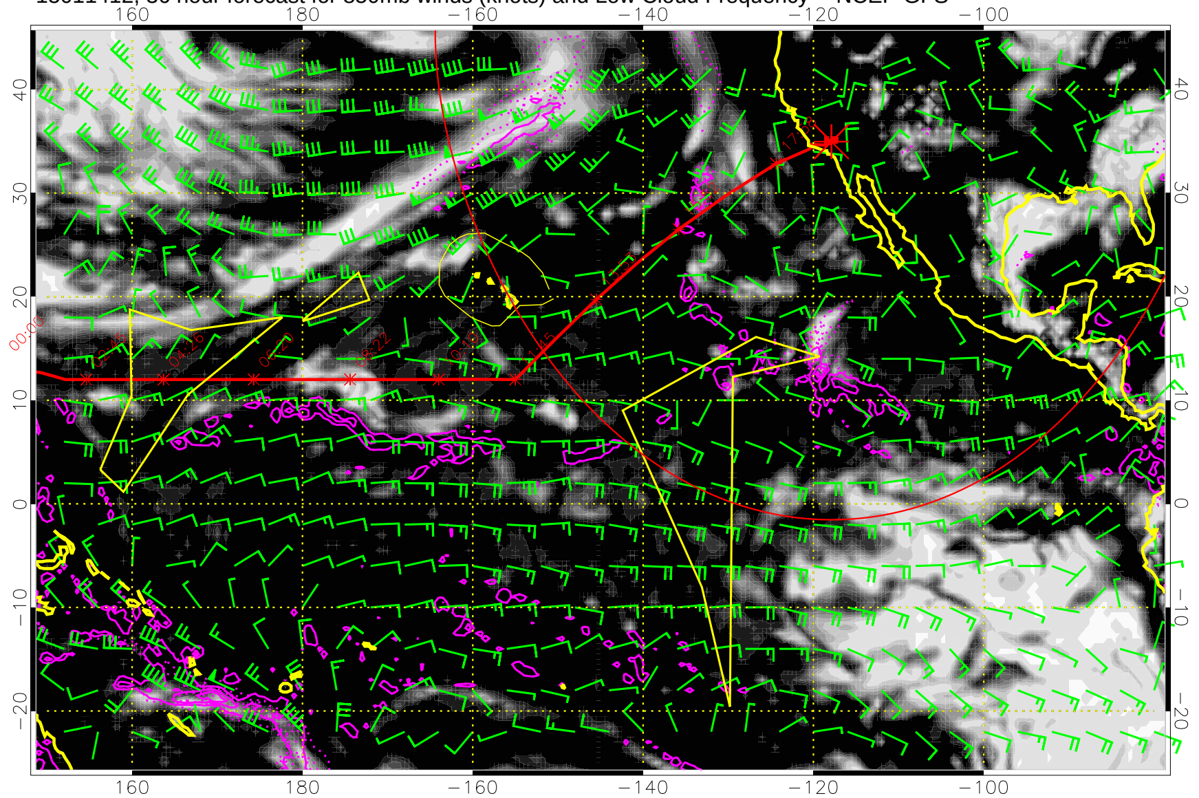
15011412, 36 hour forecast for 850mb winds (knots) and Low Cloud Frequency -- NCEP GFS
