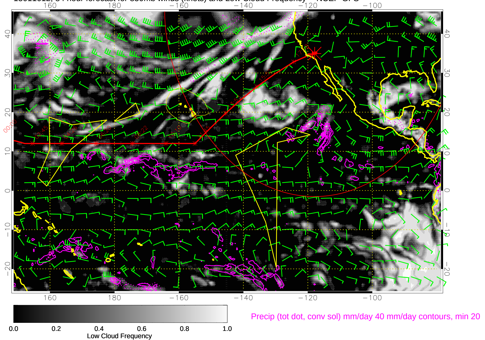
15011612, 84 hour forecast for 850mb winds (knots) and Low Cloud Frequency -- NCEP GFS
