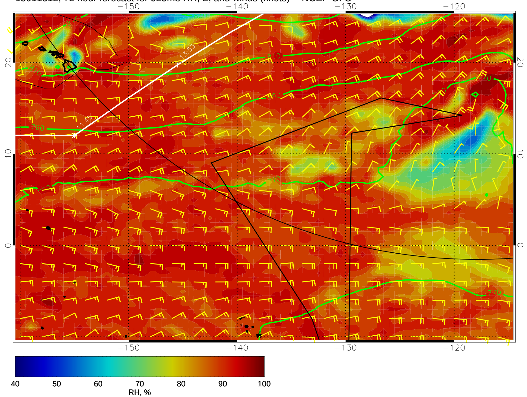
15011512, 72 hour forecast for 925mb RH, Z, and winds (knots) -- NCEP GFS
