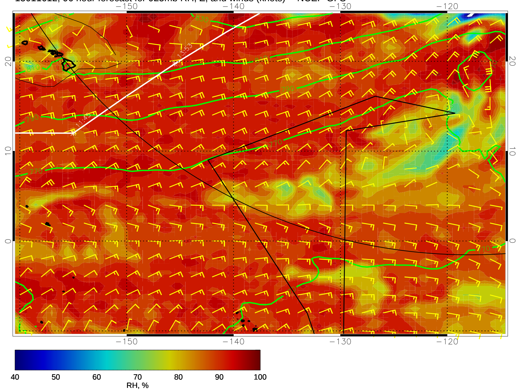
15011612, 96 hour forecast for 925mb RH, Z, and winds (knots) -- NCEP GFS
