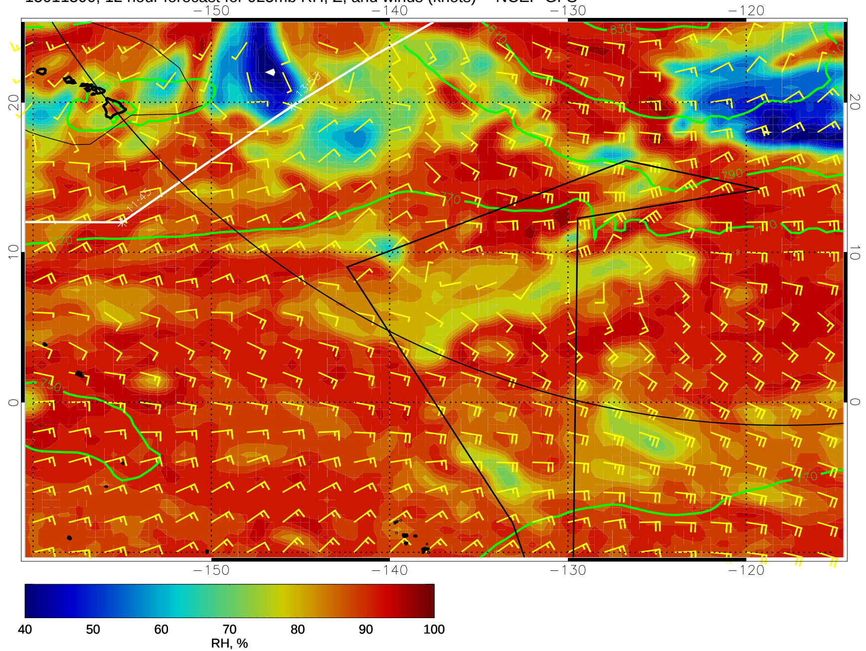
15011300, 12 hour forecast for 925mb RH, Z, and winds (knots) -- NCEP GFS
