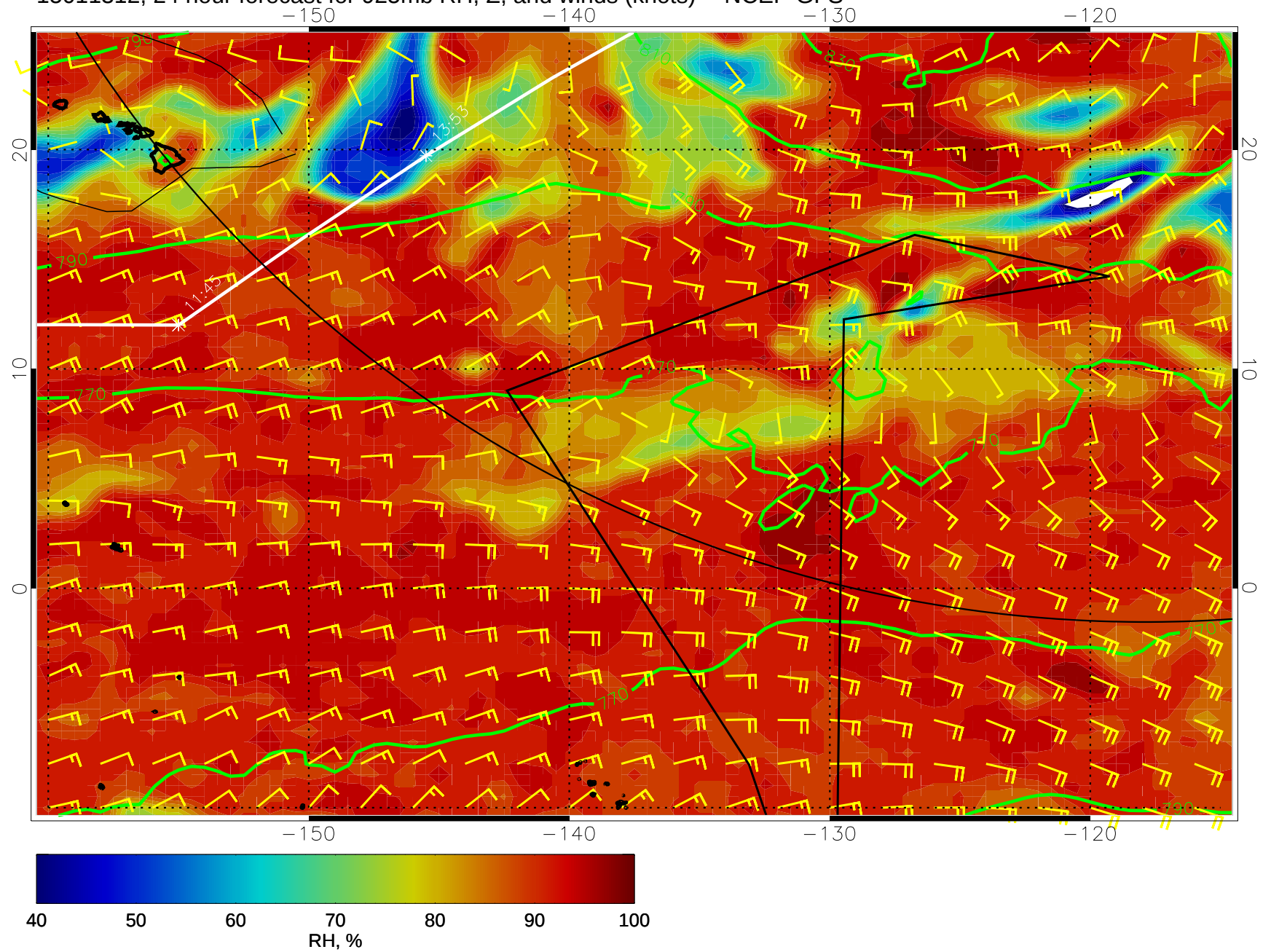
15011312, 24 hour forecast for 925mb RH, Z, and winds (knots) -- NCEP GFS
