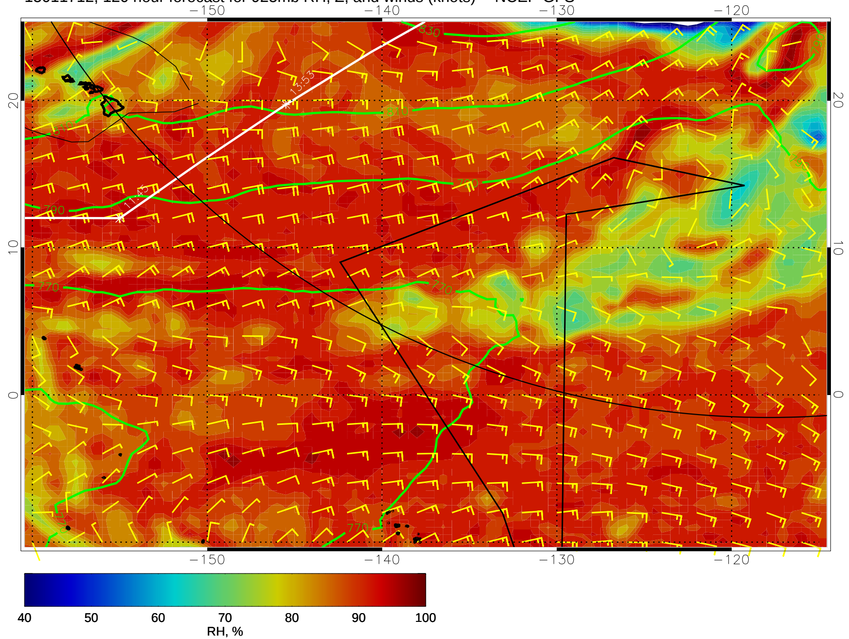
15011712, 120 hour forecast for 925mb RH, Z, and winds (knots) -- NCEP GFS
