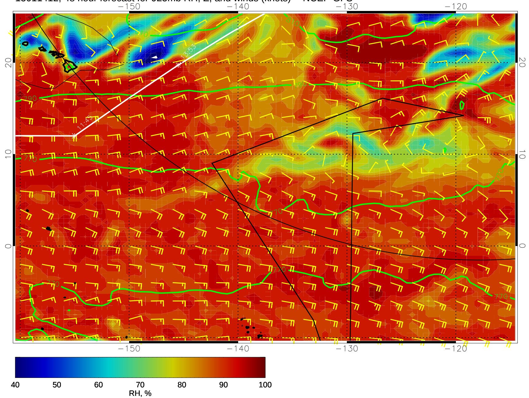
15011412, 48 hour forecast for 925mb RH, Z, and winds (knots) -- NCEP GFS
