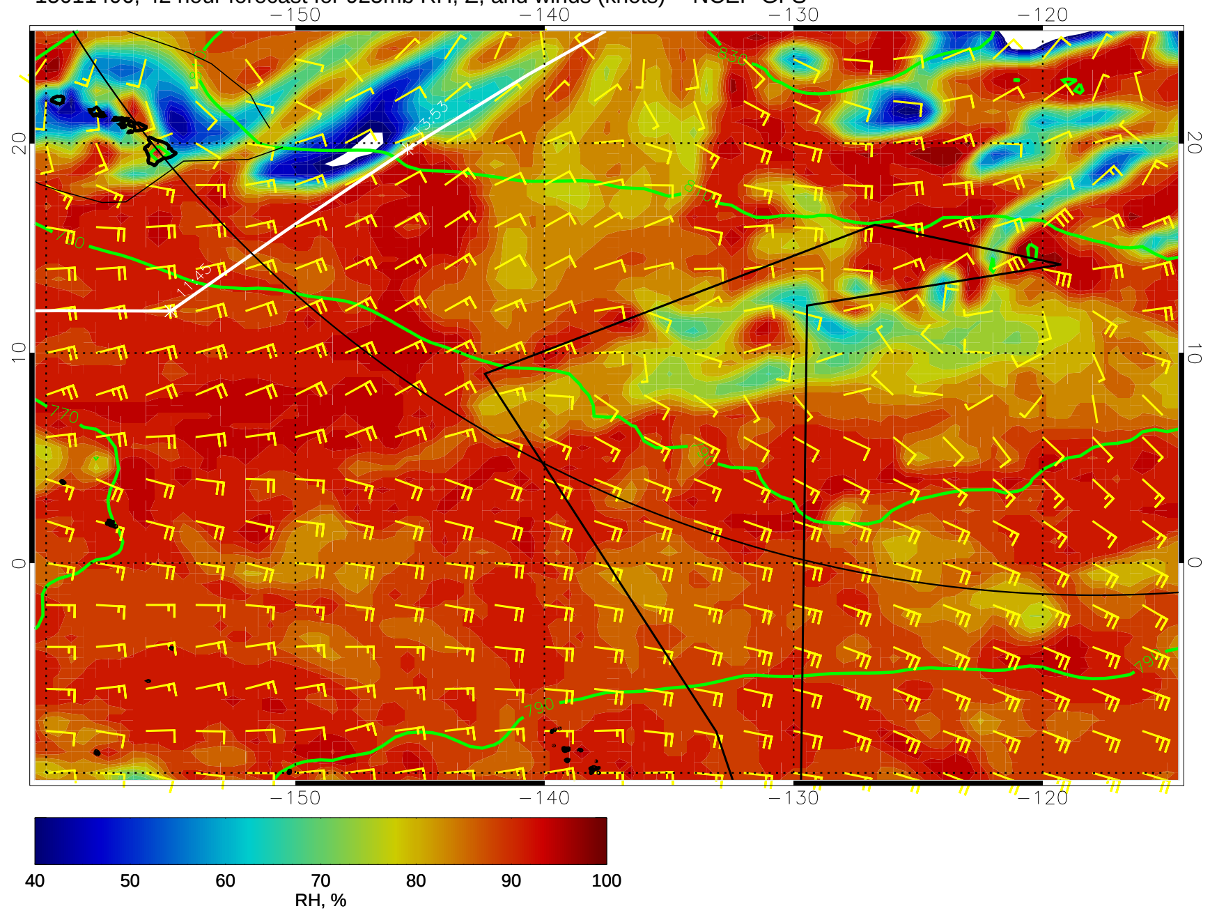
15011406, 42 hour forecast for 925mb RH, Z, and winds (knots) -- NCEP GFS
