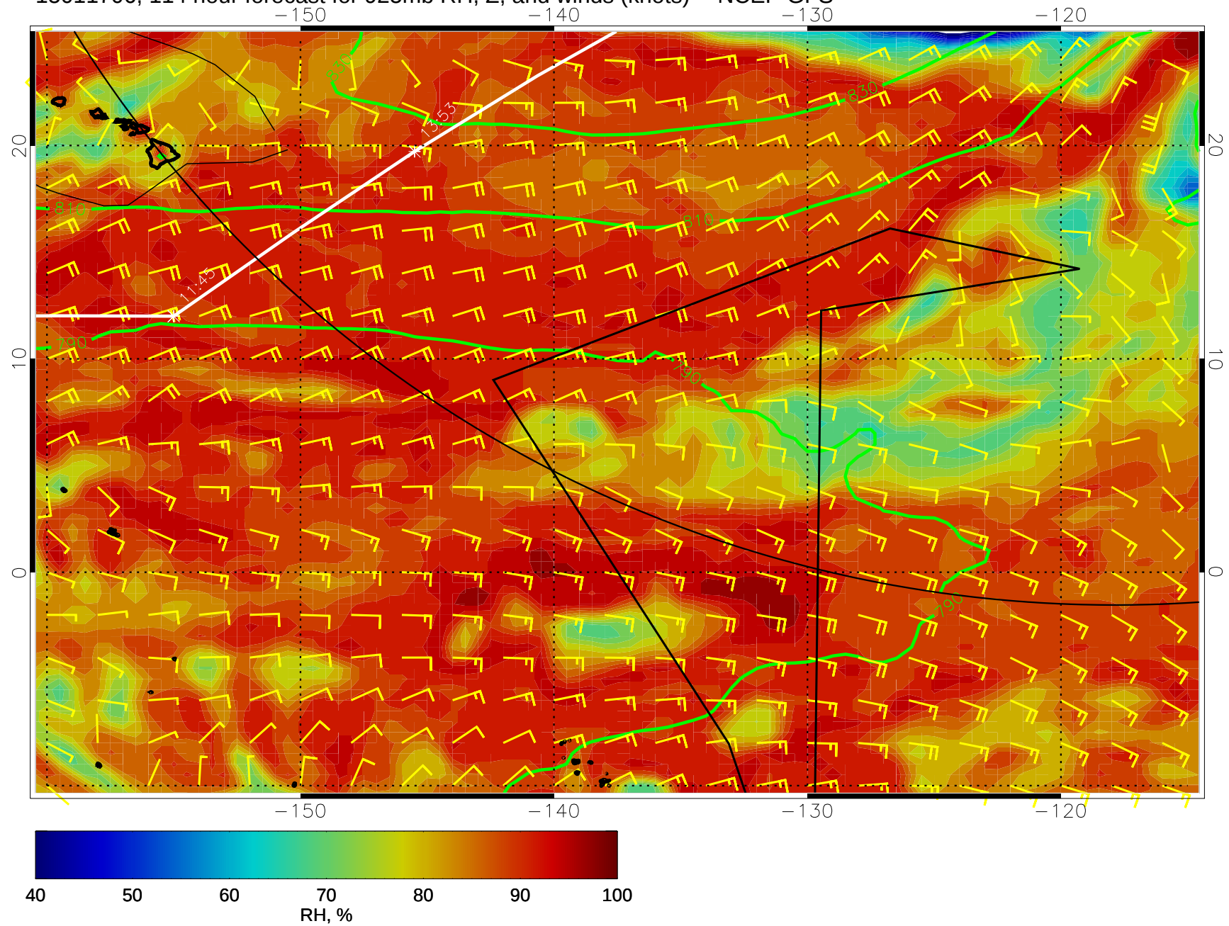
15011706, 114 hour forecast for 925mb RH, Z, and winds (knots) -- NCEP GFS
