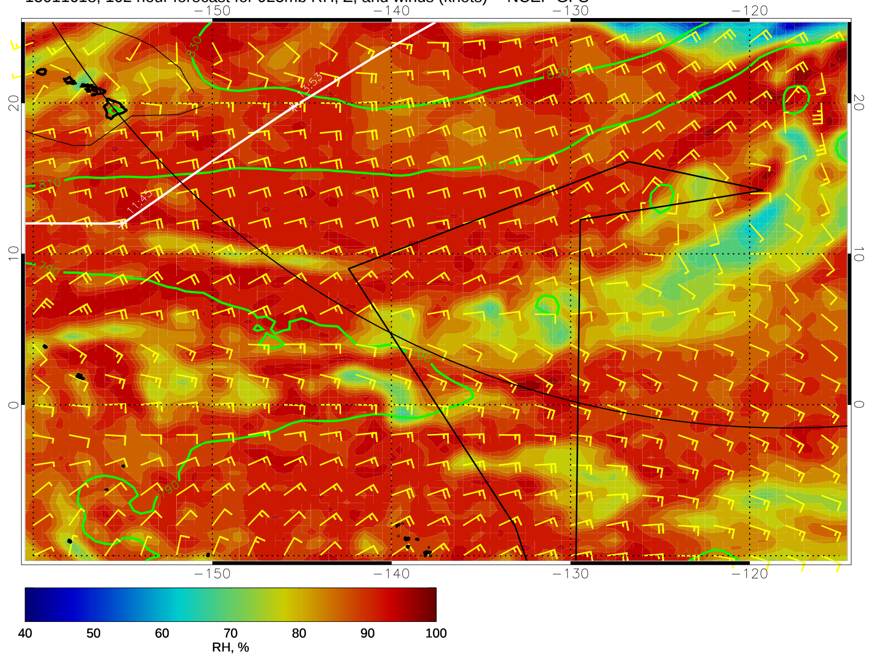
15011618, 102 hour forecast for 925mb RH, Z, and winds (knots) -- NCEP GFS
