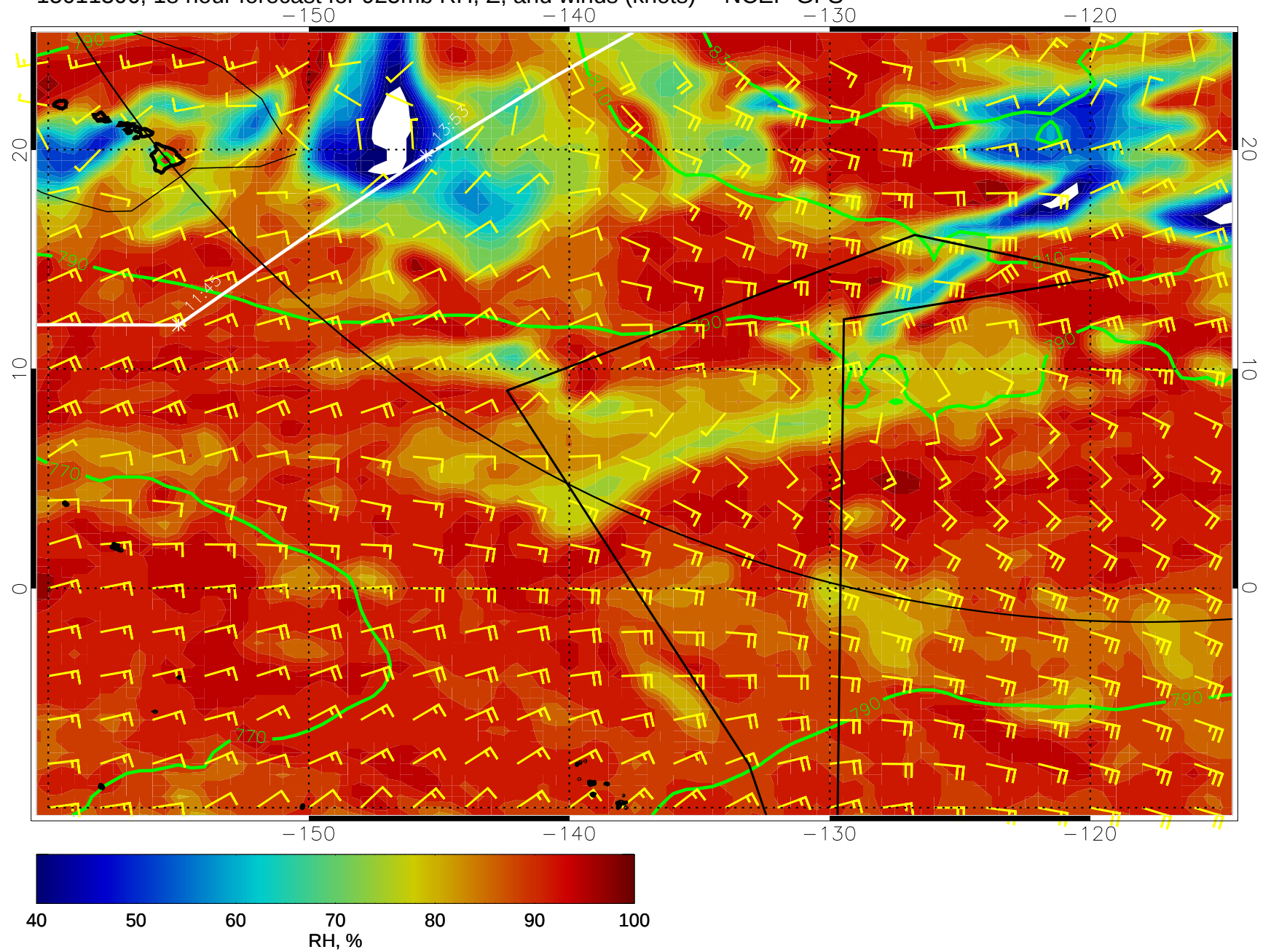
15011306, 18 hour forecast for 925mb RH, Z, and winds (knots) -- NCEP GFS
