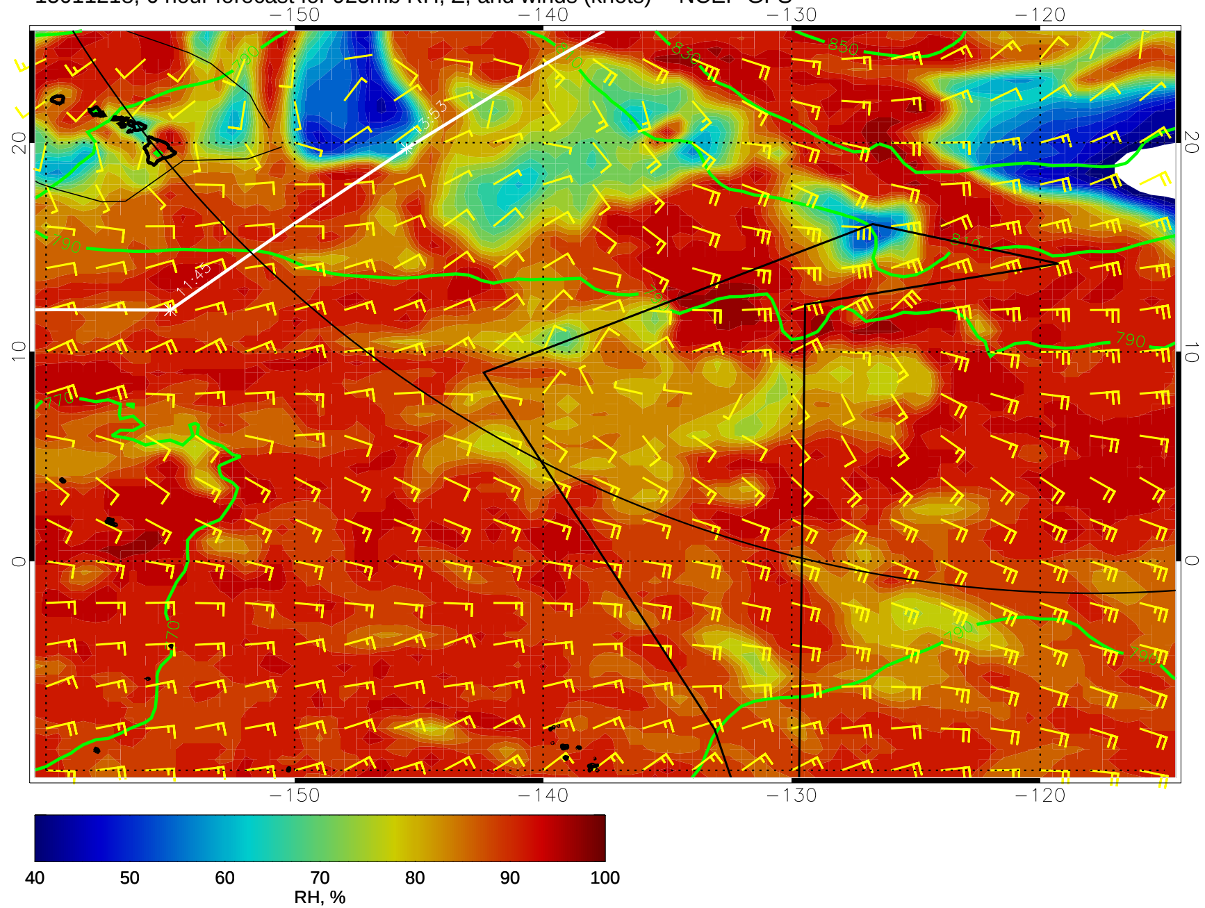
15011218, 6 hour forecast for 925mb RH, Z, and winds (knots) -- NCEP GFS
