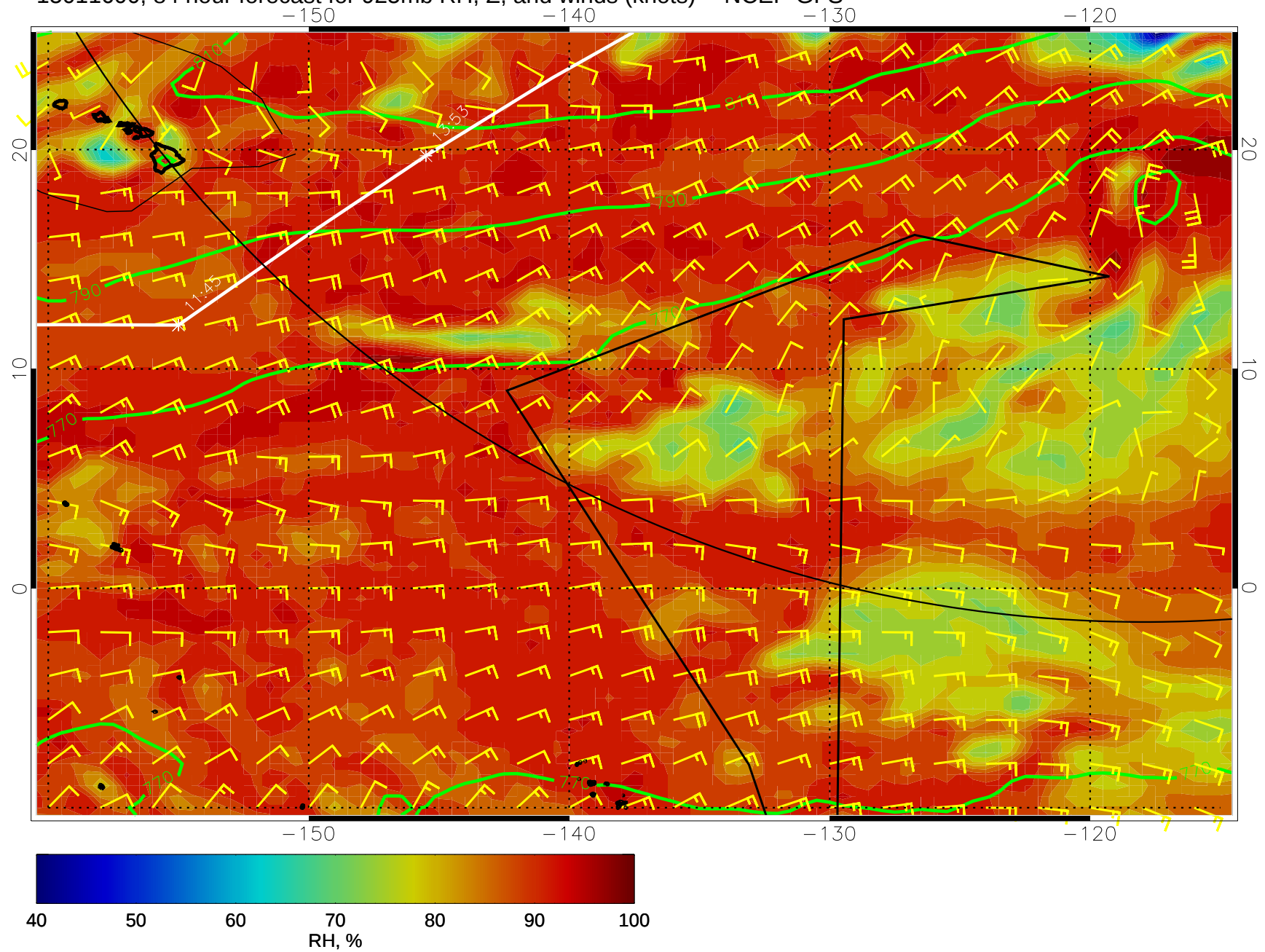
15011600, 84 hour forecast for 925mb RH, Z, and winds (knots) -- NCEP GFS
