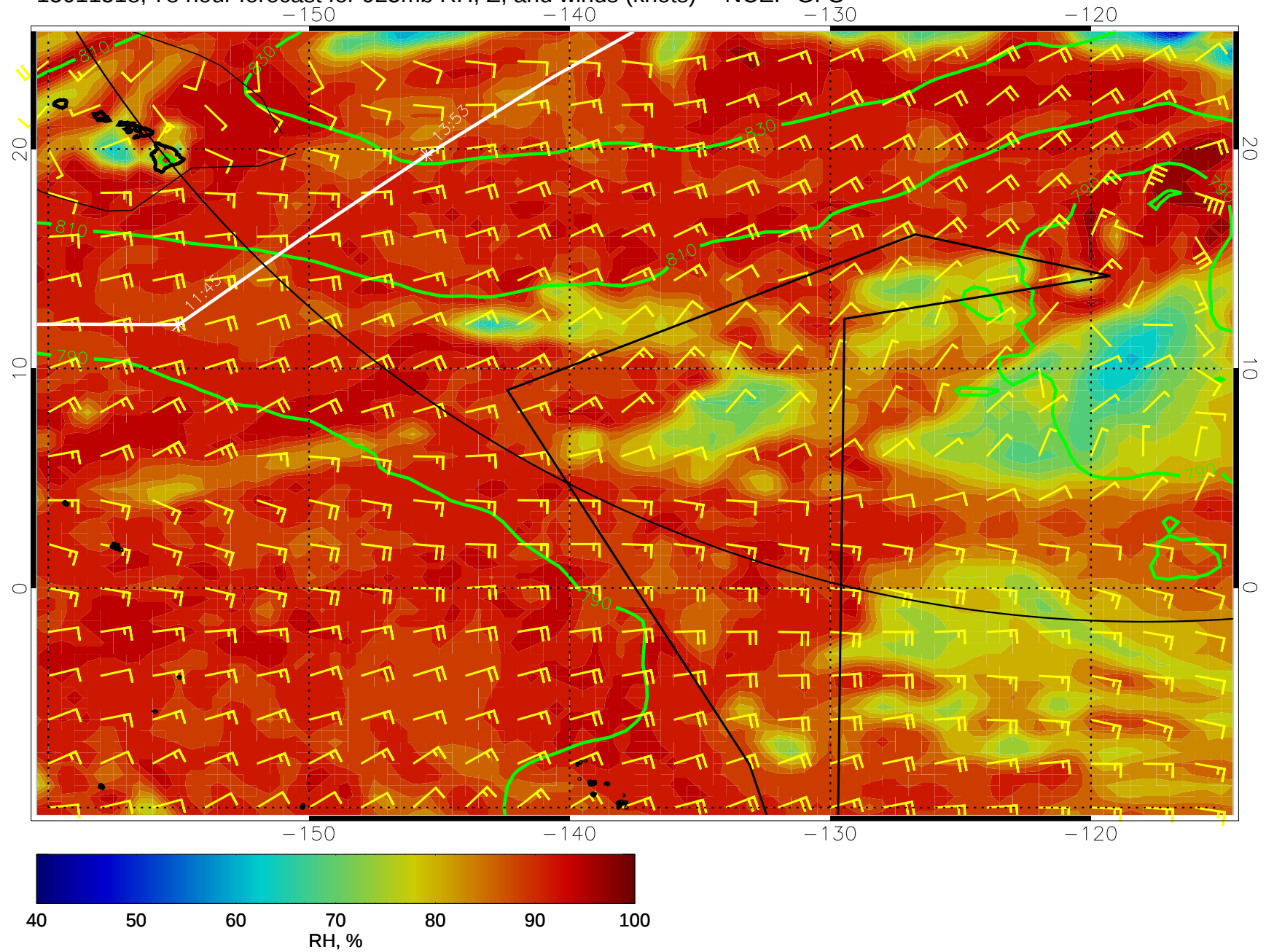
15011518, 78 hour forecast for 925mb RH, Z, and winds (knots) -- NCEP GFS
