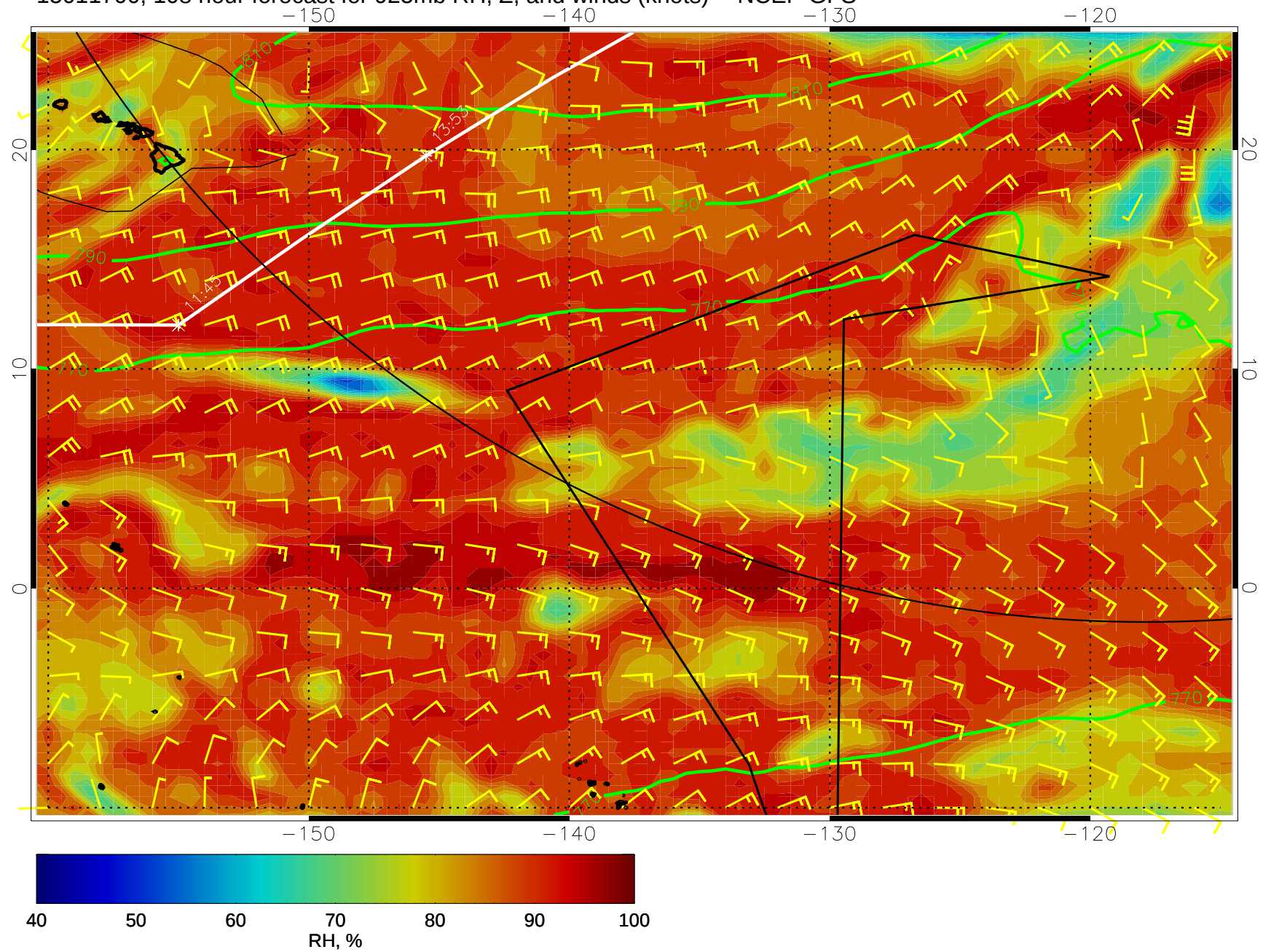
15011700, 108 hour forecast for 925mb RH, Z, and winds (knots) -- NCEP GFS
