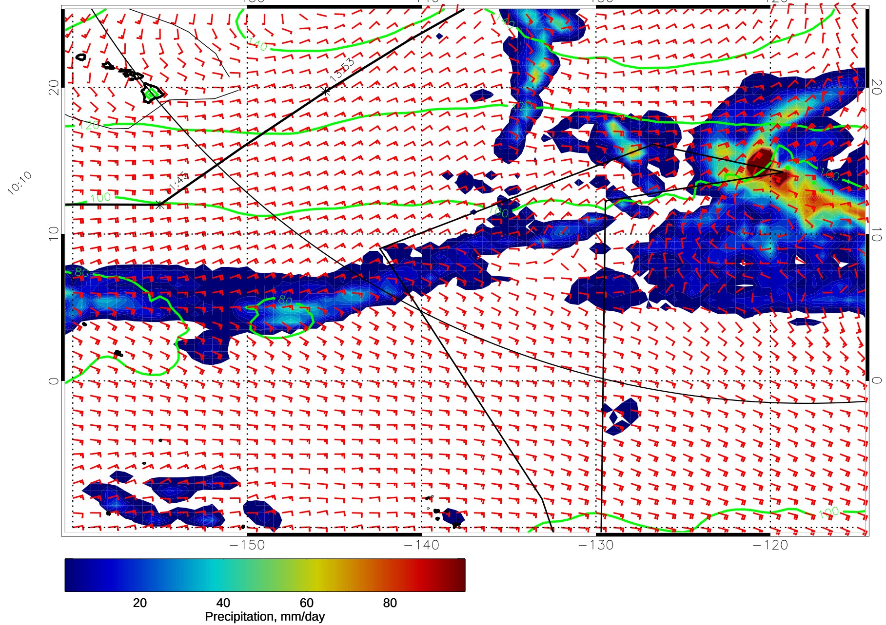
15011412, 48 hour forecast for precip, 1000mb Z, and winds (knots) -- NCEP GFS
